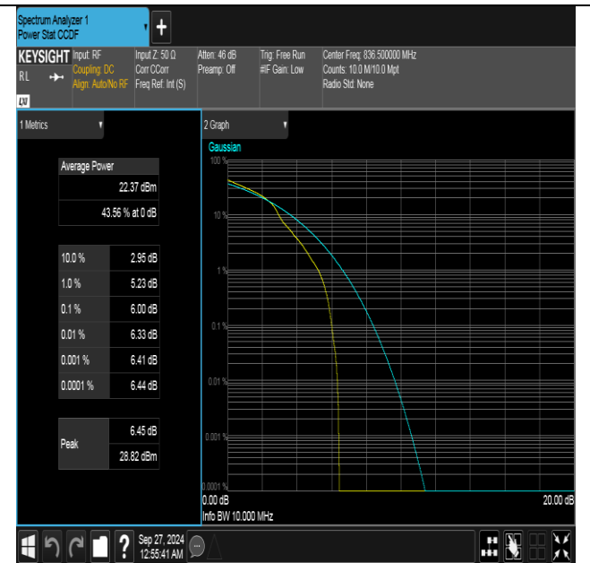
Band26(824-849)-10MHz-16QAM-26915-1RB#0-PASS
