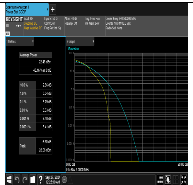
Band26(824-849)-5MHz-16QAM-27015-1RB#0-PASS
