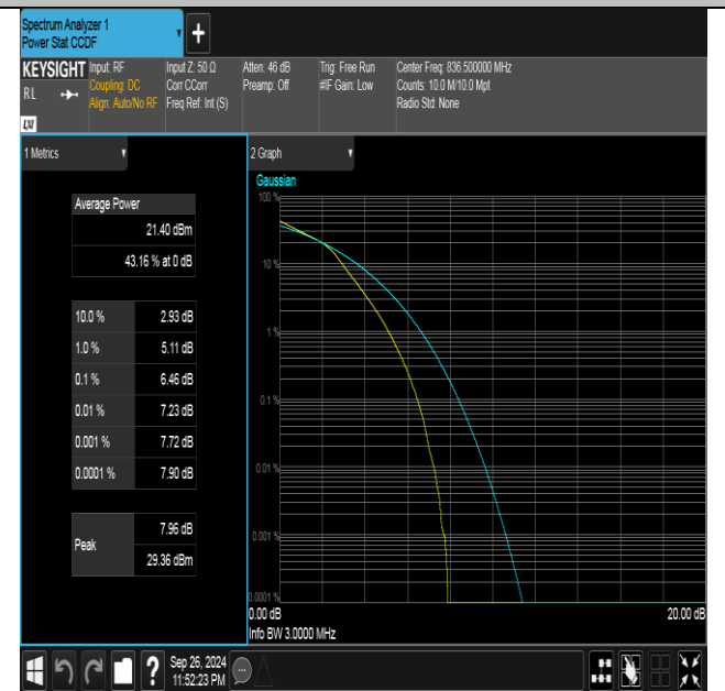
Band26(824-849)-3MHz-16QAM-26915-15RB#0-PASS
