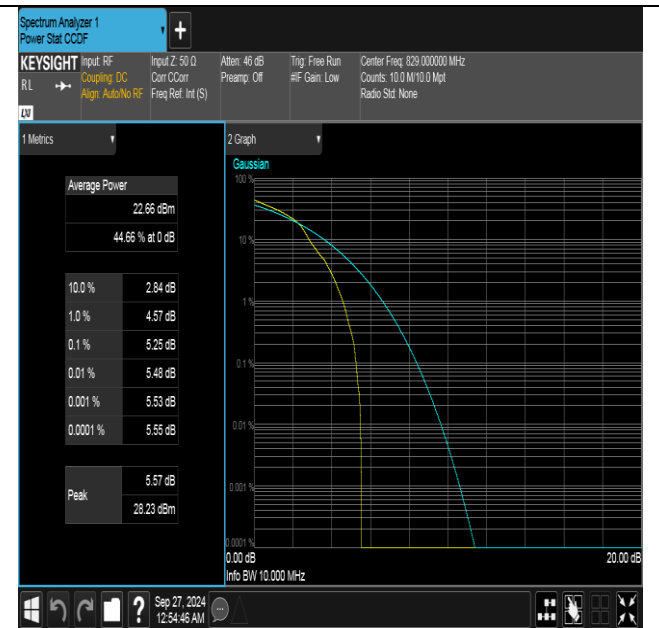
Band26(824-849)-10MHz-16QAM-26840-1RB#0-PASS
