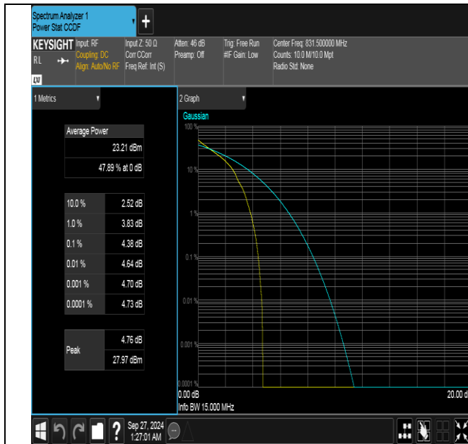
Band26(824-849)-15MHz-QPSK-26865-1RB#0-PASS
