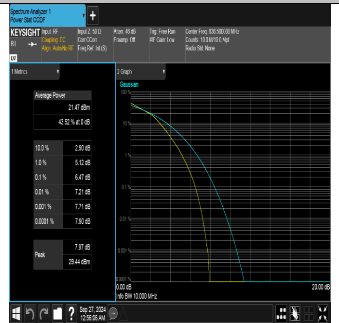
Band26(824-849)-10MHz-16QAM-26915-50RB#0-PASS
