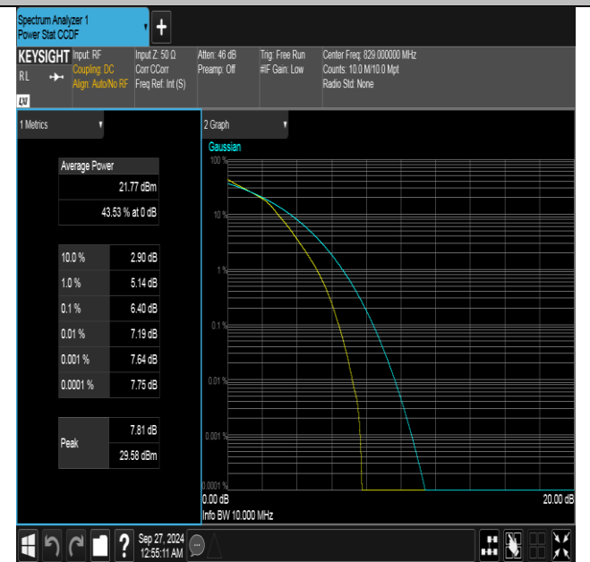
Band26(824-849)-10MHz-16QAM-26840-50RB#0-PASS
