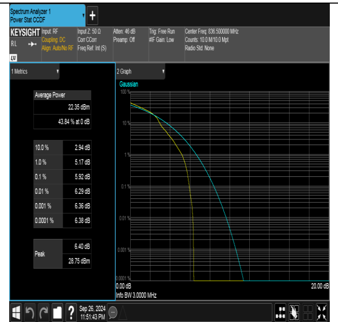
Band26(824-849)-3MHz-16QAM-26915-1RB#0-PASS
