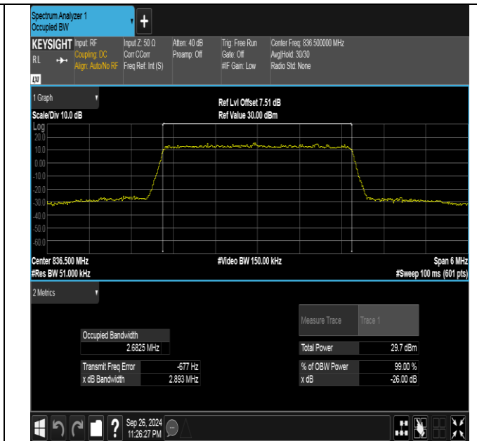
Band26(824-849)-3MHz-16QAM-26915-15RB#0-PASS
