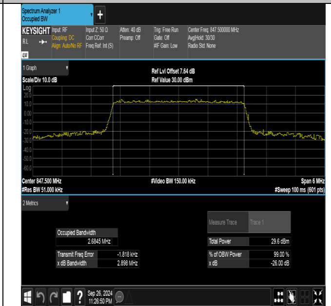
Band26(824-849)-3MHz-16QAM-27025-15RB#0-PASS
