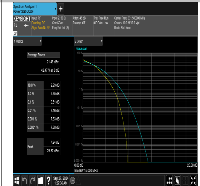
Band26(824-849)-15MHz-16QAM-26865-75RB#0-PASS
