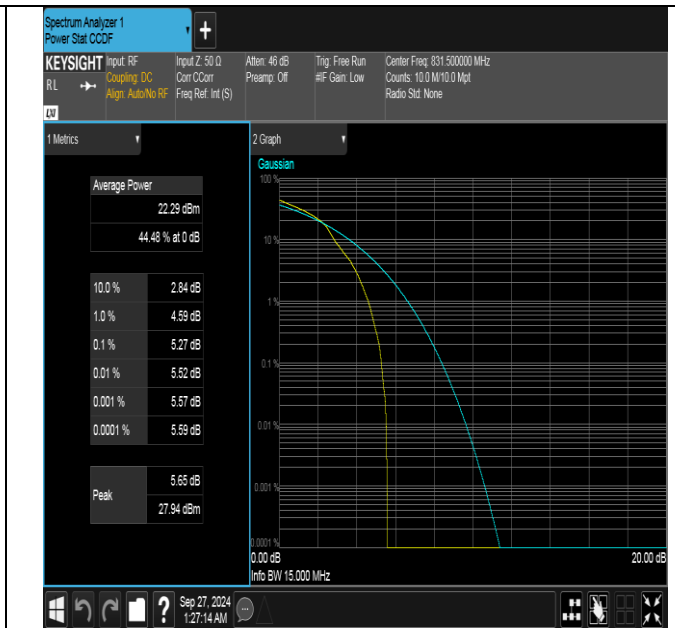
Band26(824-849)-15MHz-16QAM-26865-1RB#0-PASS
