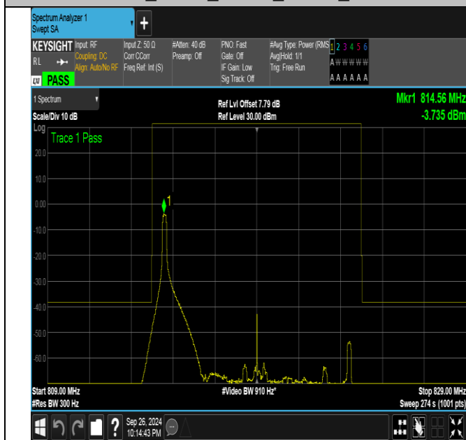
Band26_10MHz_QPSK_26740_1RB#0
