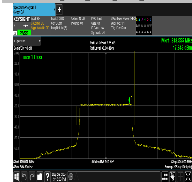
Band26_5MHz_QPSK_26715_25RB#0
