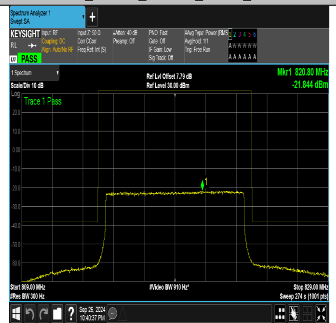
Band26_10MHz_16QAM_26740_50RB#0
