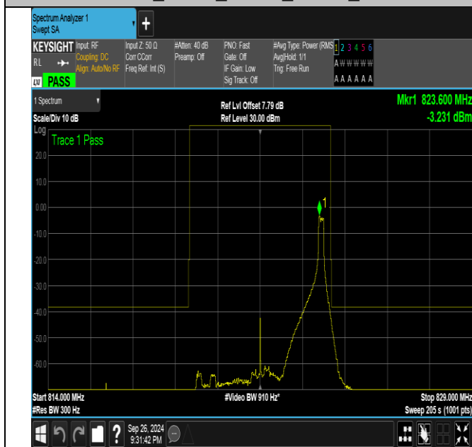
Band26_5MHz_QPSK_26765_1RB#24
