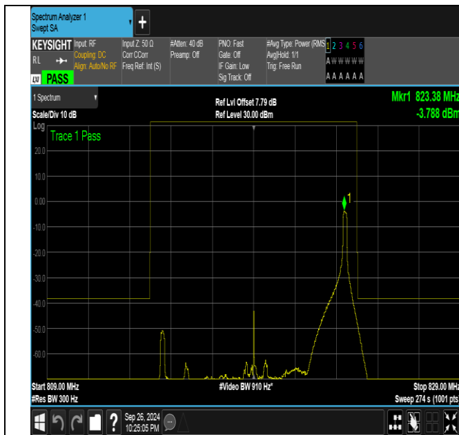
Band26_10MHz_QPSK_26740_1RB#49
