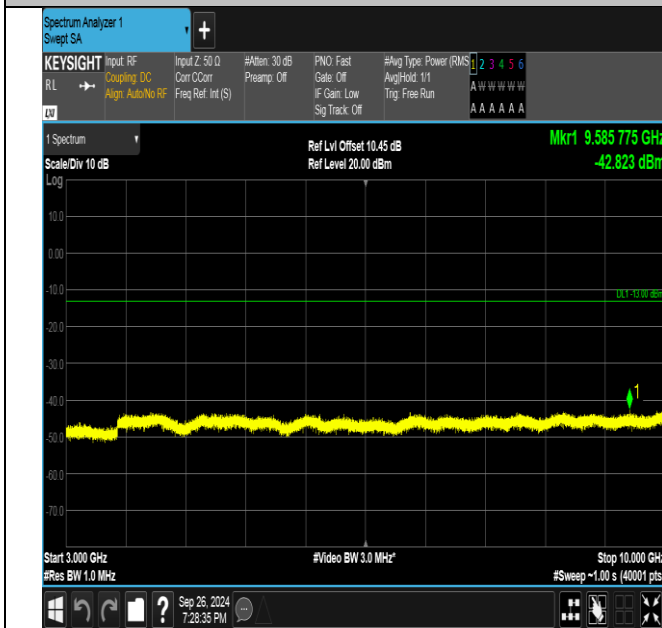
Band26_1.4MHz_QPSK_26783_6RB#0_3000~10000_3000~10000
