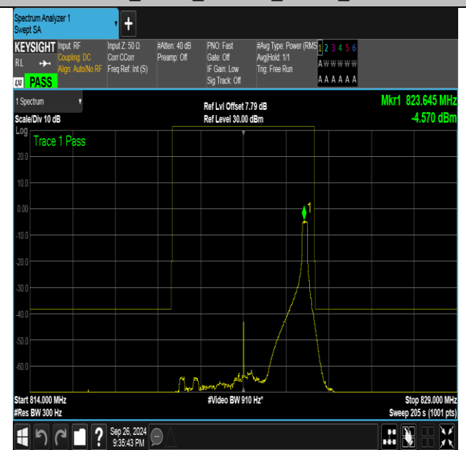
Band26_5MHz_16QAM_26765_1RB#24
