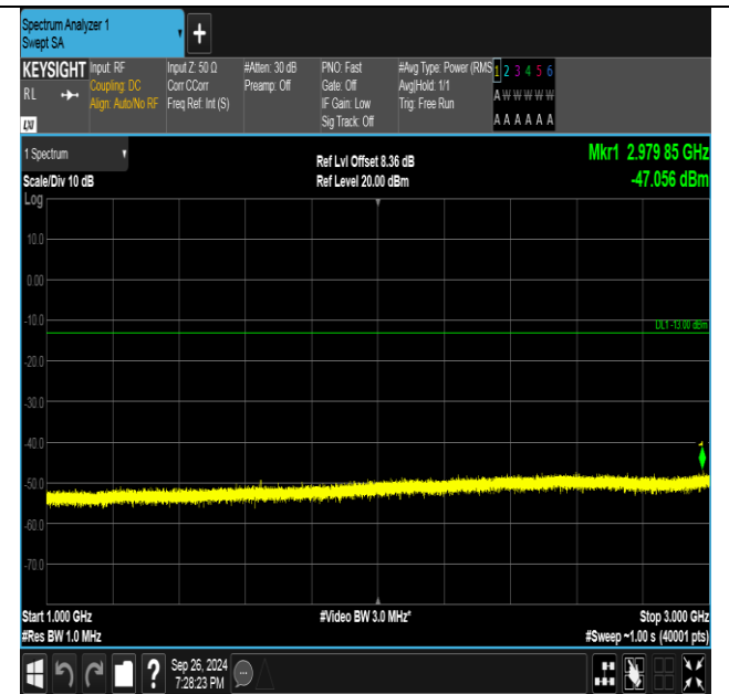
Band26_1.4MHz_QPSK_26783_6RB#0_1000~3000_1000~3000
