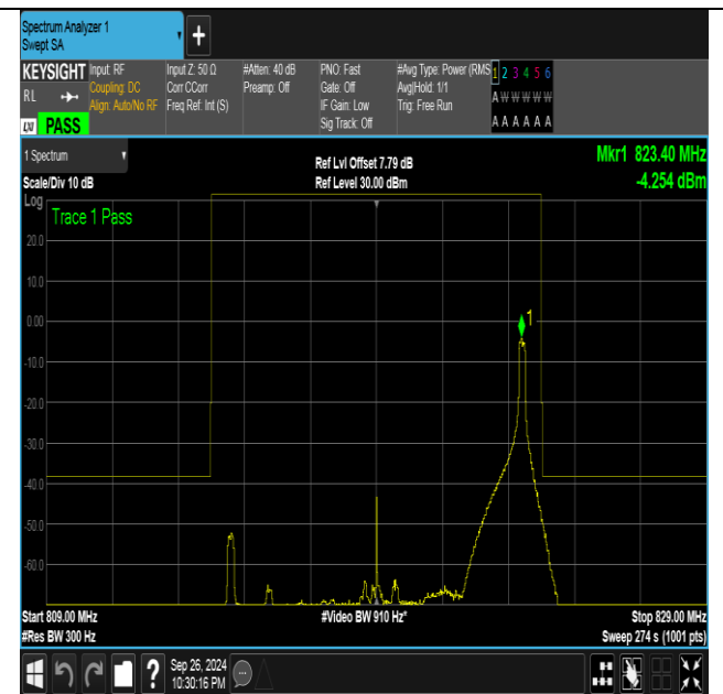
Band26_10MHz_16QAM_26740_1RB#49
