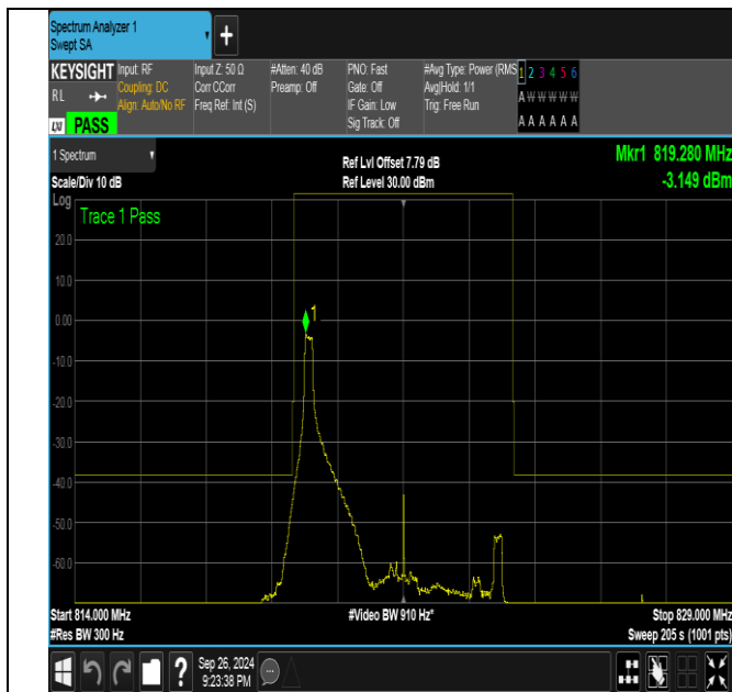
Band26_5MHz_QPSK_26765_1RB#0
