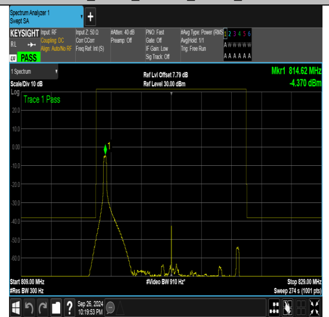
Band26_10MHz_16QAM_26740_1RB#0
