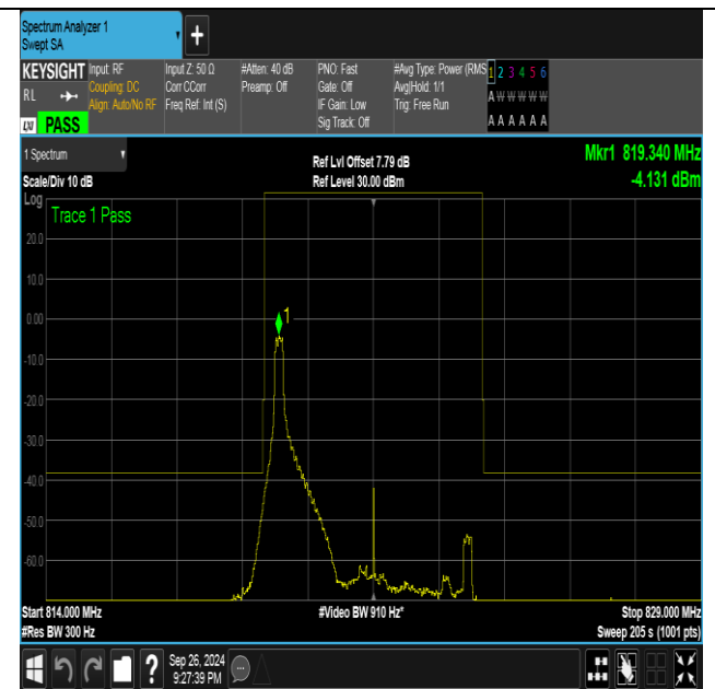
Band26_5MHz_16QAM_26765_1RB#0
