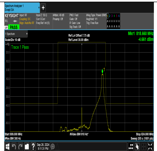
Band26_5MHz_16QAM_26715_1RB#24
