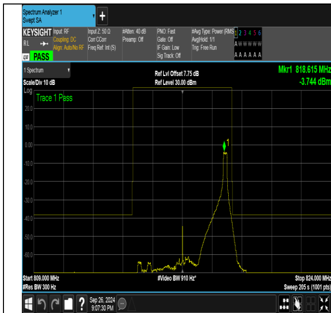
Band26_5MHz_QPSK_26715_1RB#24
