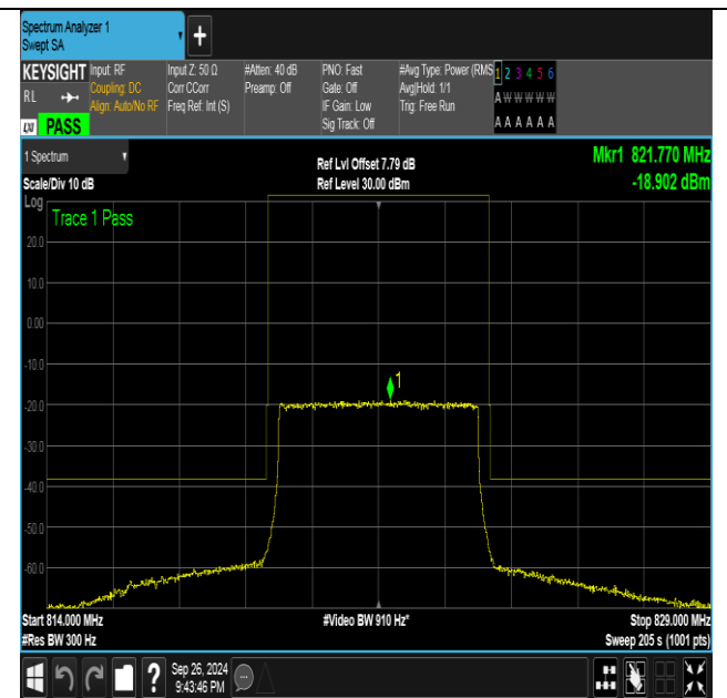
Band26_5MHz_16QAM_26765_25RB#0
