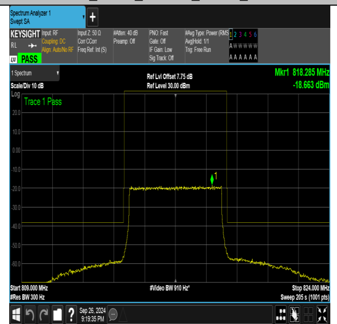
Band26_5MHz_16QAM_26715_25RB#0
