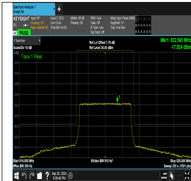
Band26_5MHz_QPSK_26765_25RB#0
