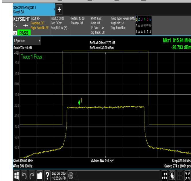
Band26_10MHz_QPSK_26740_50RB#0
