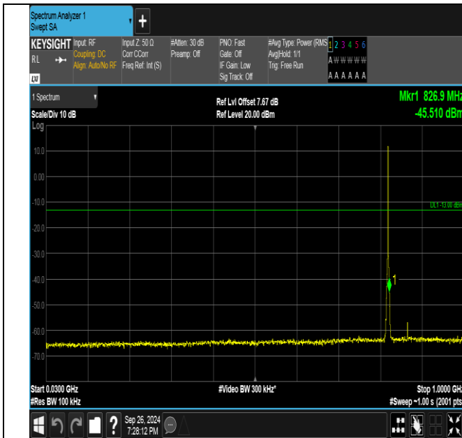
Band26_1.4MHz_QPSK_26783_6RB#0_30~1000_30~1000
