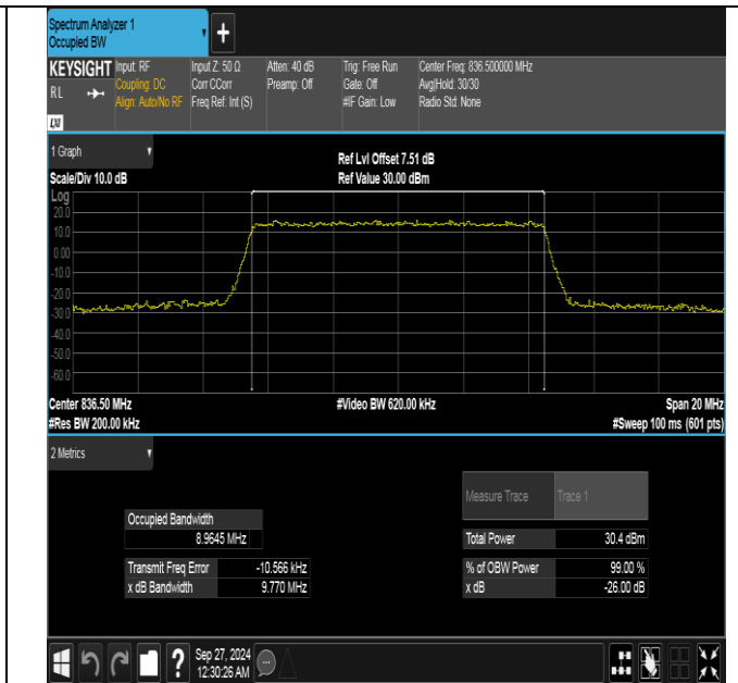
Band26(824-849)-10MHz-16QAM-26915-50RB#0-PASS
