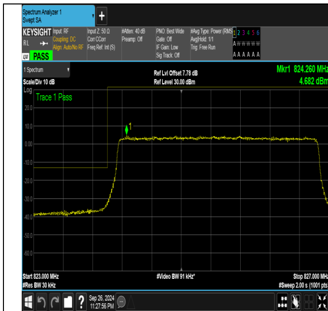
Band26_3MHz_QPSK_26805_15RB#0
