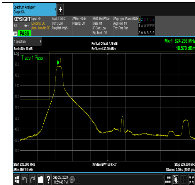
Band26_5MHz_QPSK_26815_1RB#0
