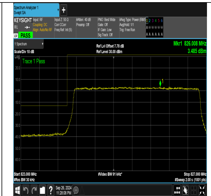
Band26_3MHz_16QAM_26805_15RB#0
