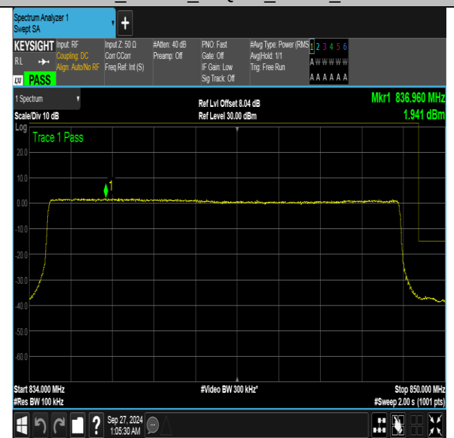
Band26_15MHz_16QAM_26965_75RB#0
