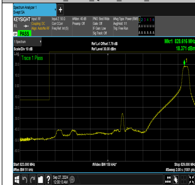
Band26_5MHz_QPSK_26815_1RB#24
