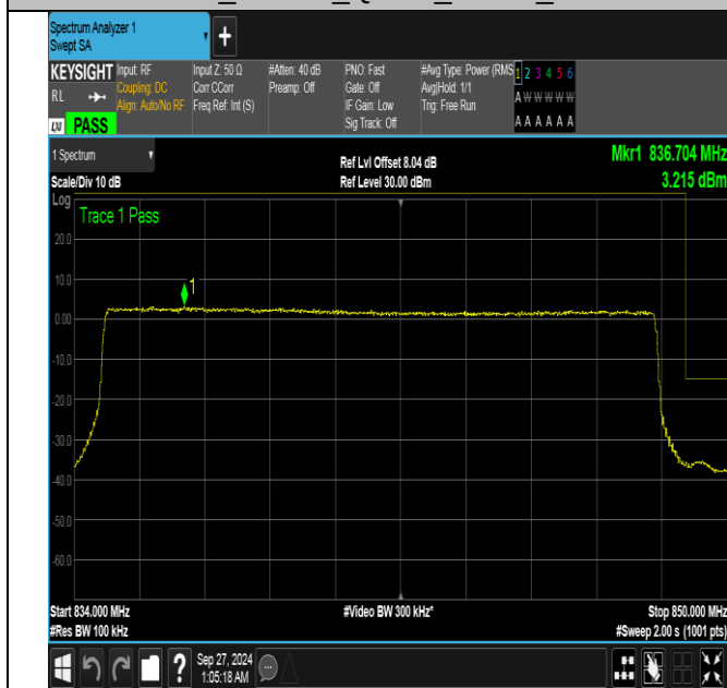
Band26_15MHz_QPSK_26965_75RB#0
