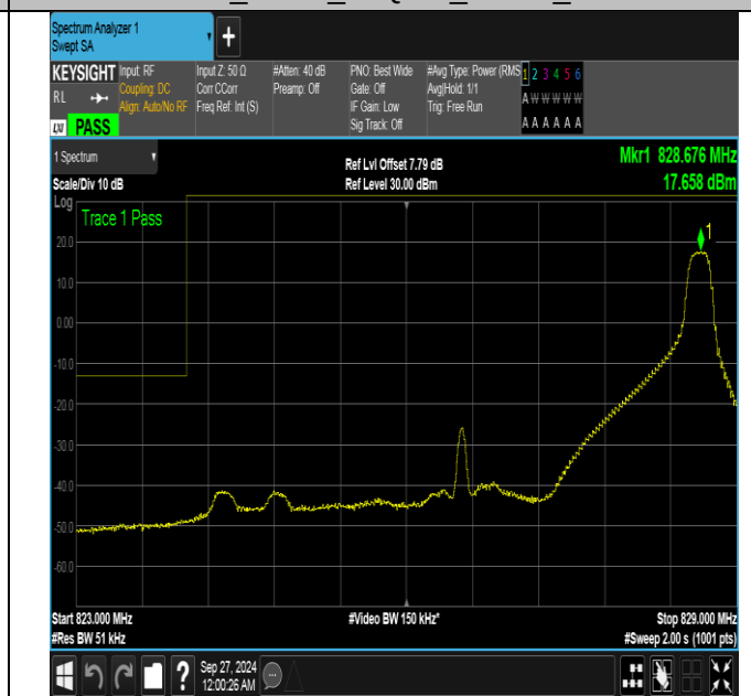
Band26_5MHz_16QAM_26815_1RB#24
