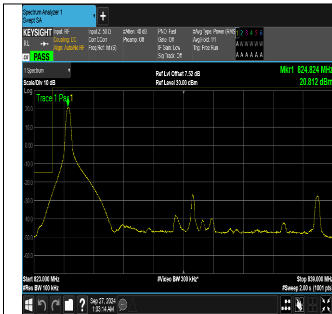
Band26_15MHz_QPSK_26865_1RB#0
