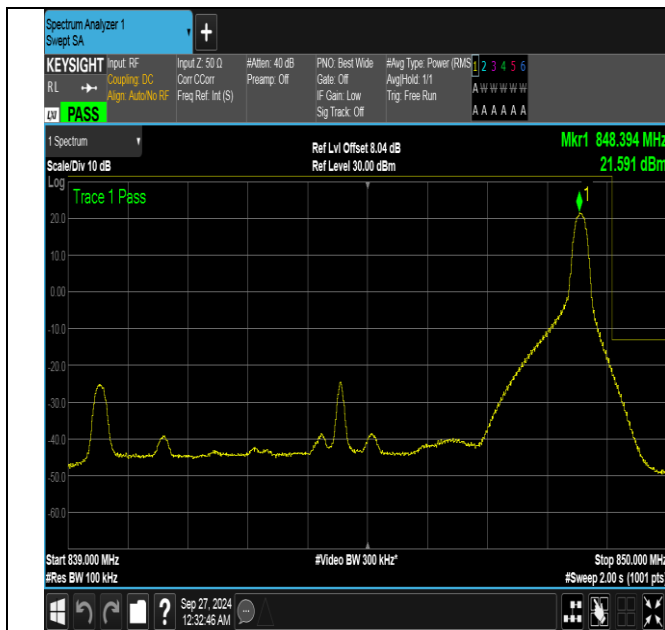
Band26_10MHz_QPSK_26990_1RB#49
