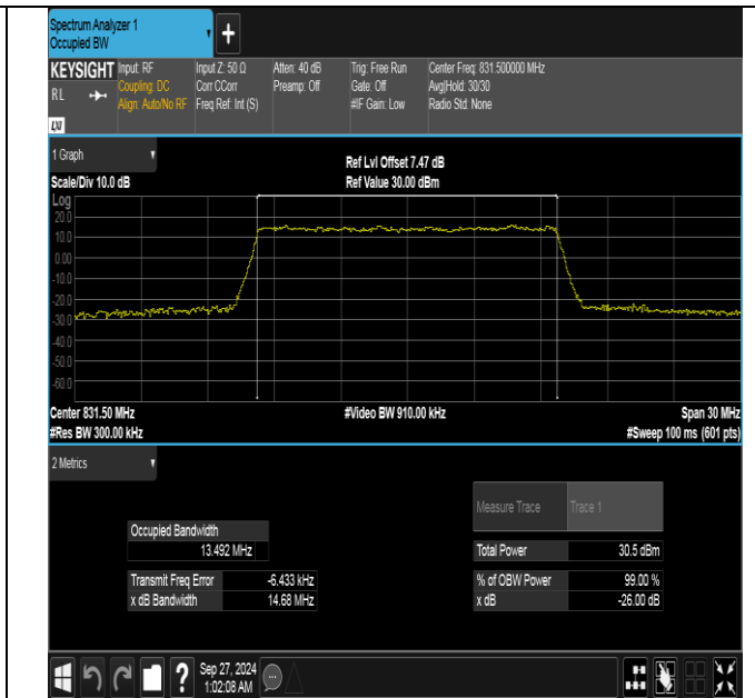
Band26(824-849)-15MHz-16QAM-26865-75RB#0-PASS
