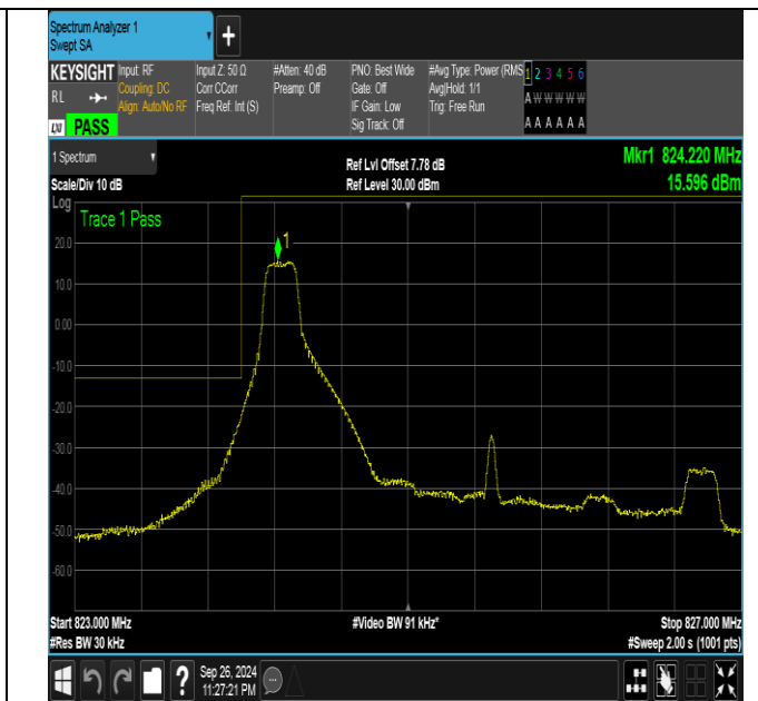
Band26_3MHz_16QAM_26805_1RB#0
