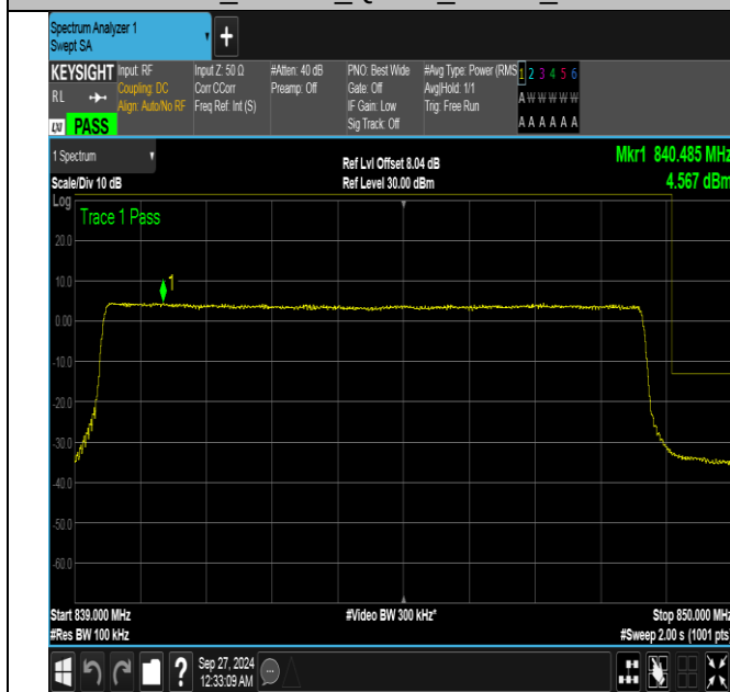
Band26_10MHz_QPSK_26990_50RB#0
