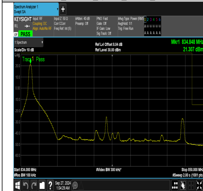
Band26_15MHz_QPSK_26965_1RB#0
