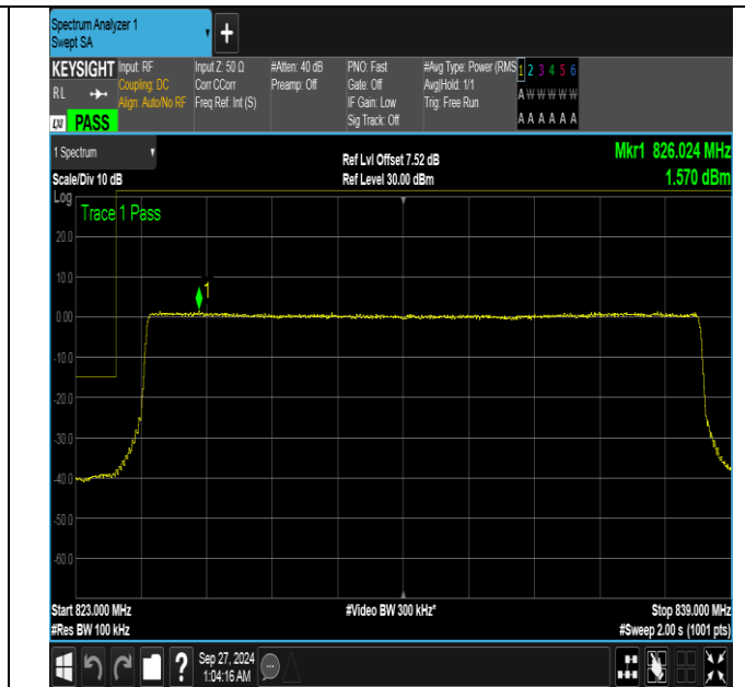
Band26_15MHz_16QAM_26865_75RB#0
