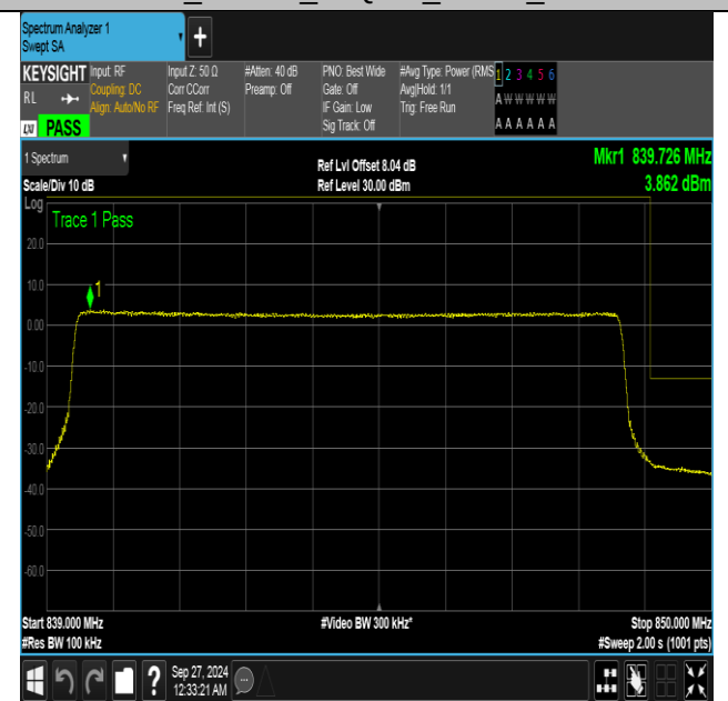
Band26_10MHz_16QAM_26990_50RB#0
