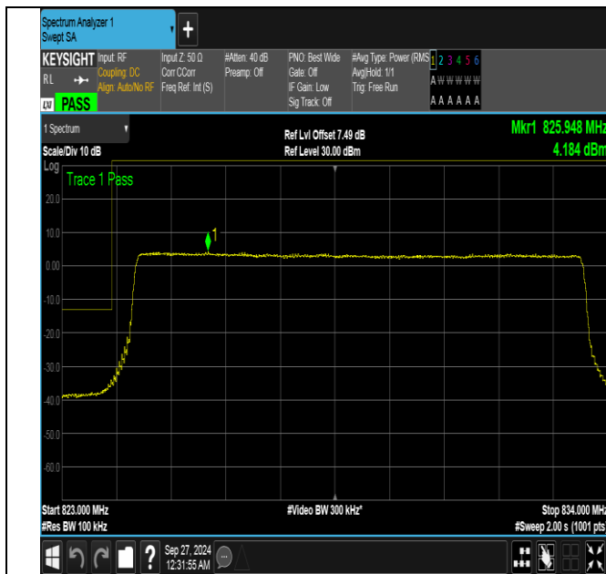
Band26_10MHz_QPSK_26840_50RB#0
