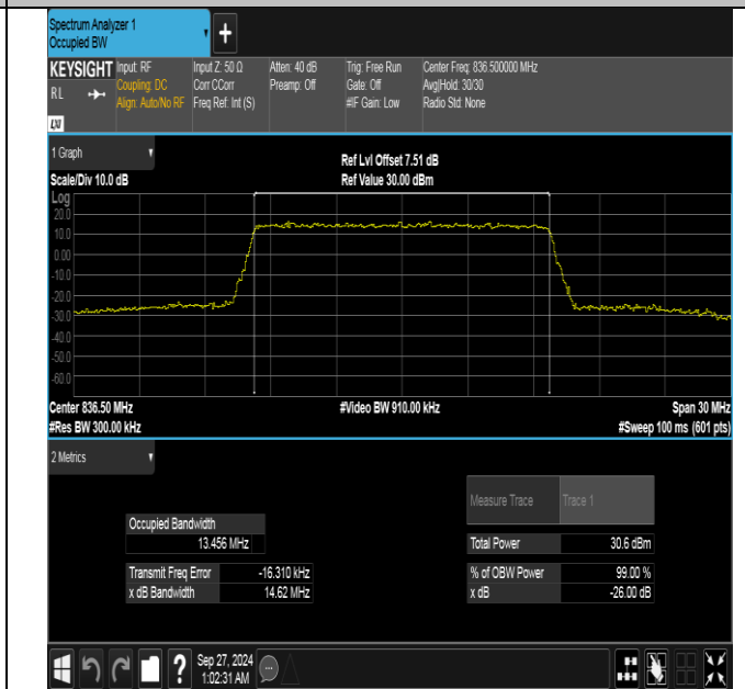
Band26(824-849)-15MHz-16QAM-26915-75RB#0-PASS
