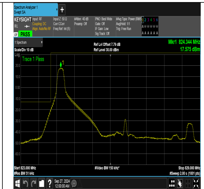
Band26_5MHz_16QAM_26815_1RB#0
