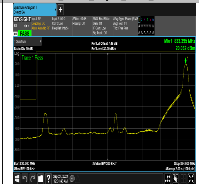
Band26_10MHz_16QAM_26840_1RB#49
