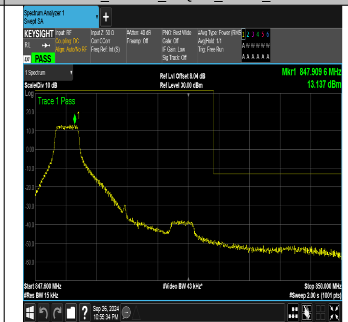
Band26_1.4MHz_16QAM_27033_1RB#0
