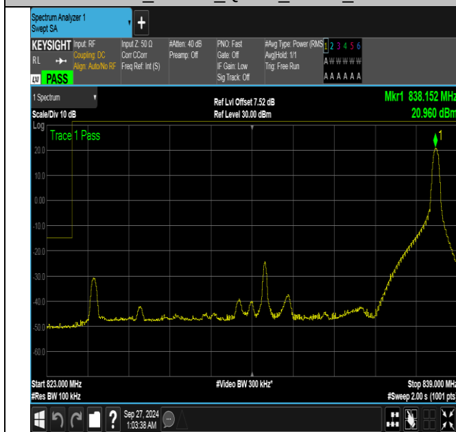
Band26_15MHz_QPSK_26865_1RB#74
