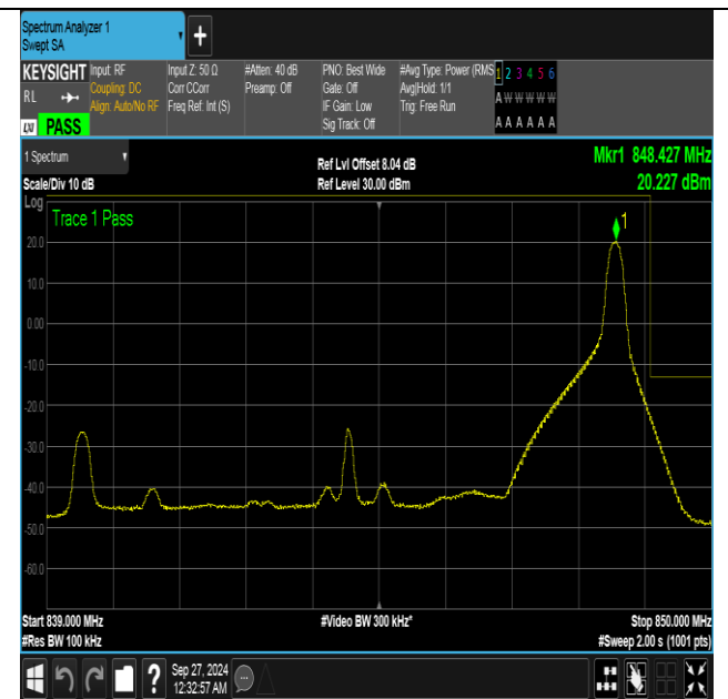
Band26_10MHz_16QAM_26990_1RB#49
