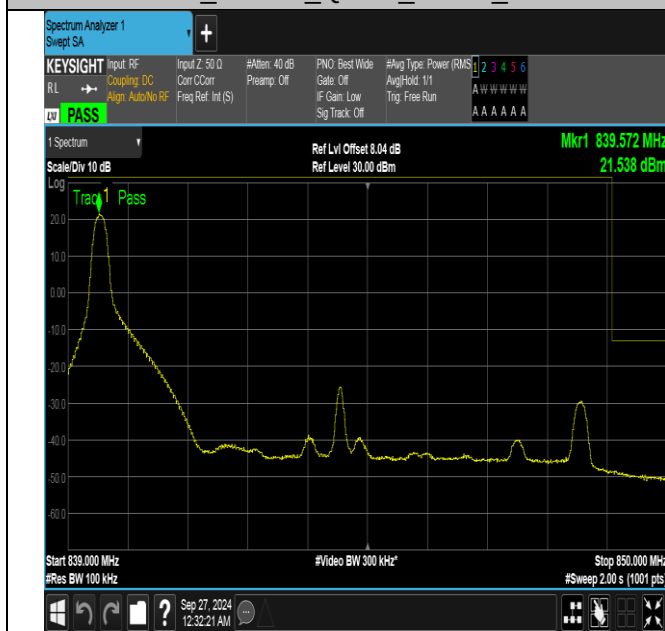
Band26_10MHz_QPSK_26990_1RB#0
