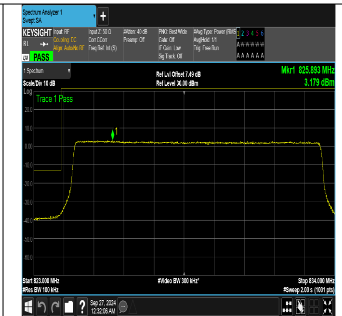
Band26_10MHz_16QAM_26840_50RB#0
