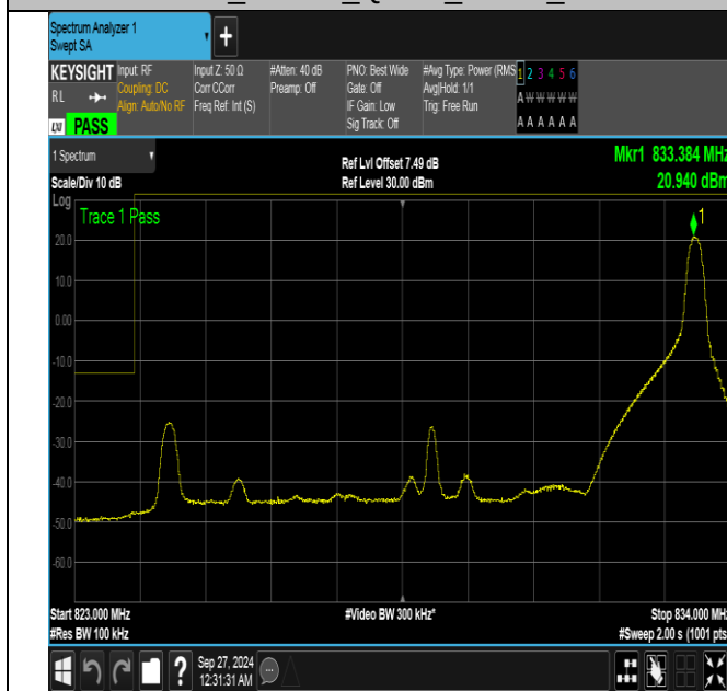
Band26_10MHz_QPSK_26840_1RB#49
