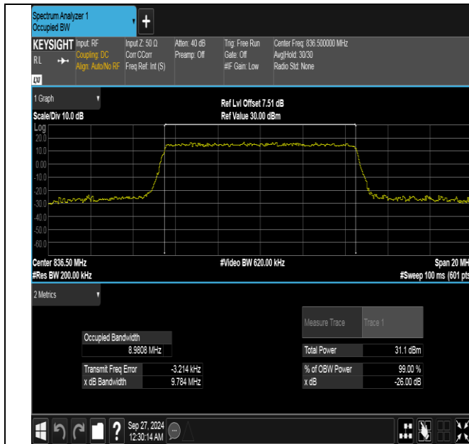
Band26(824-849)-10MHz-QPSK-26915-50RB#0-PASS
