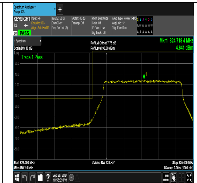
Band26_1.4MHz_16QAM_26797_6RB#0
