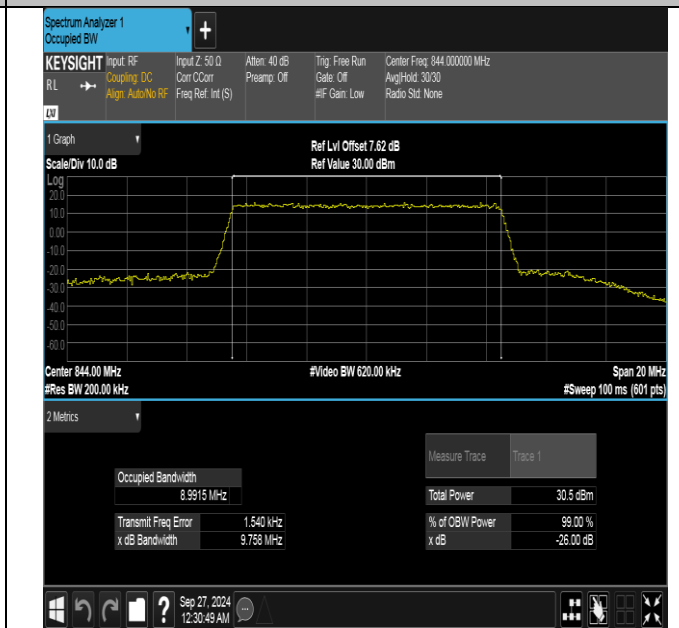
Band26(824-849)-10MHz-16QAM-26990-50RB#0-PASS
