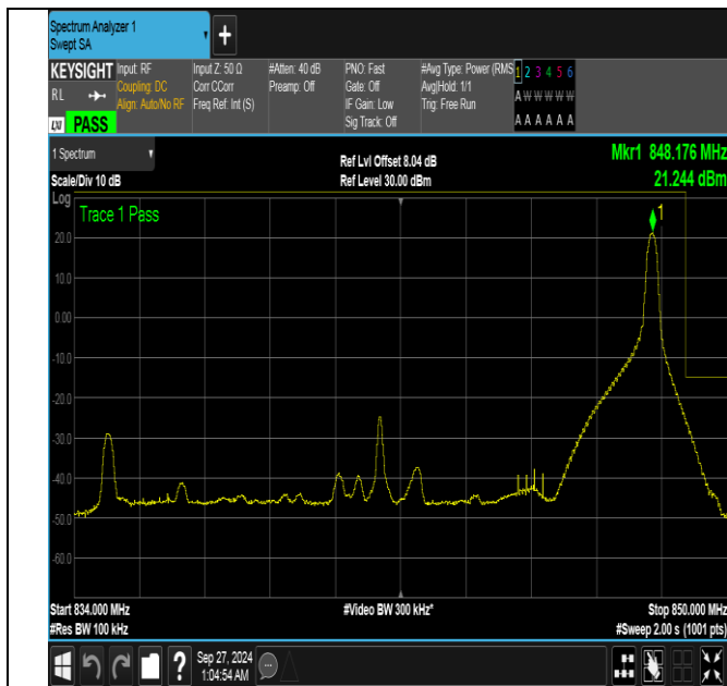
Band26_15MHz_QPSK_26965_1RB#74
