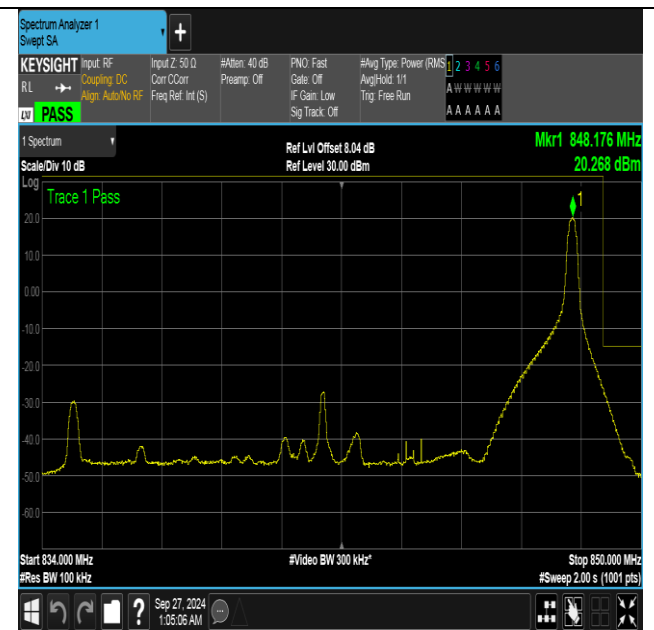
Band26_15MHz_16QAM_26965_1RB#74
