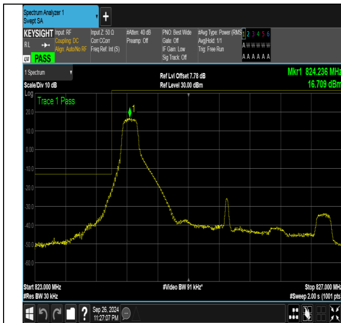
Band26_3MHz_QPSK_26805_1RB#0
