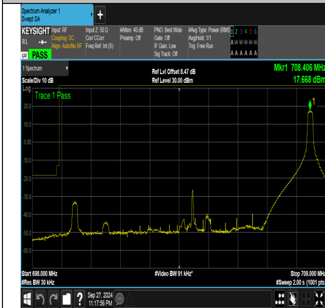
Band12_10MHz_QPSK_23060_1RB#49
