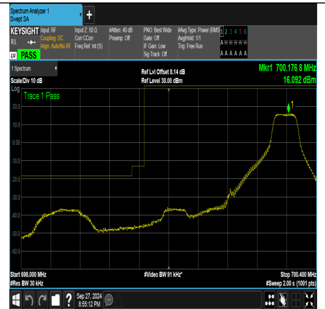
Band12_1.4MHz_16QAM_23017_1RB#5
