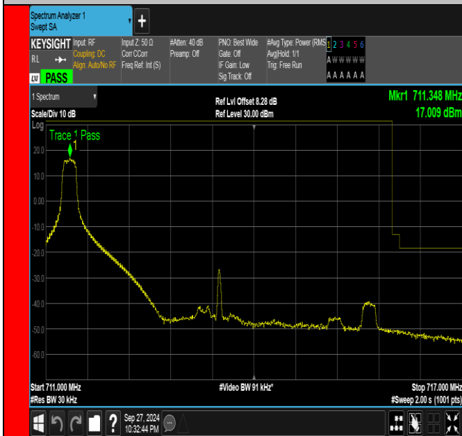
Band12_5MHz_16QAM_23155_1RB#0
