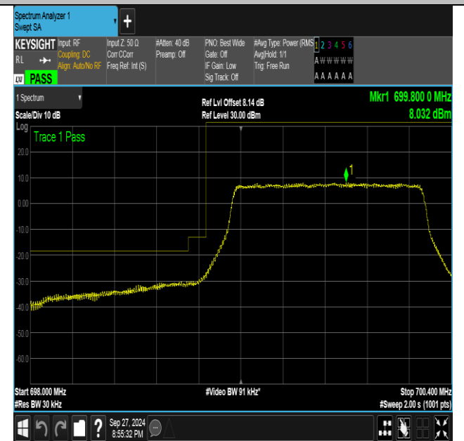
Band12_1.4MHz_16QAM_23017_6RB#0
