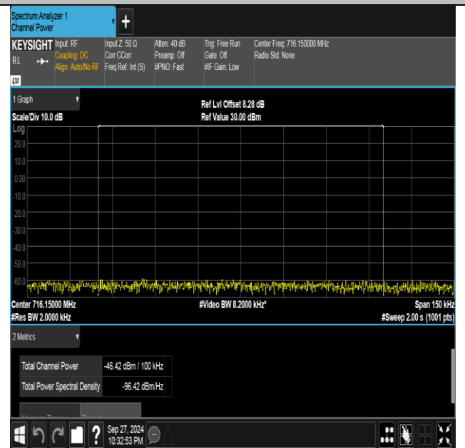
Band12_5MHz_16QAM_23155_1RB#0_Final1
