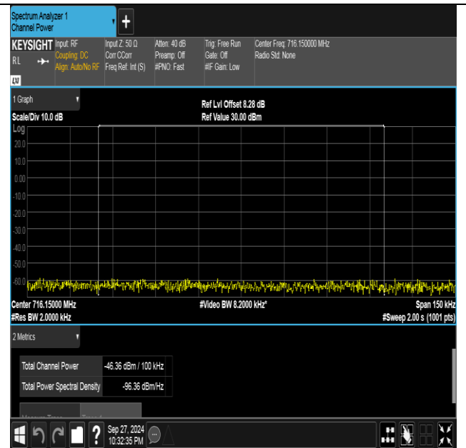
Band12_5MHz_QPSK_23155_1RB#0_Final1
