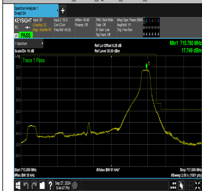
Band12_3MHz_QPSK_23165_1RB#14
