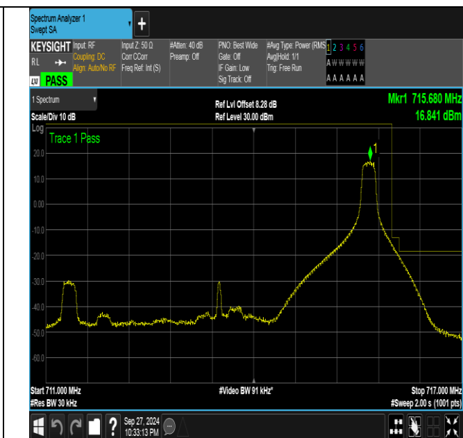
Band12_5MHz_16QAM_23155_1RB#24
