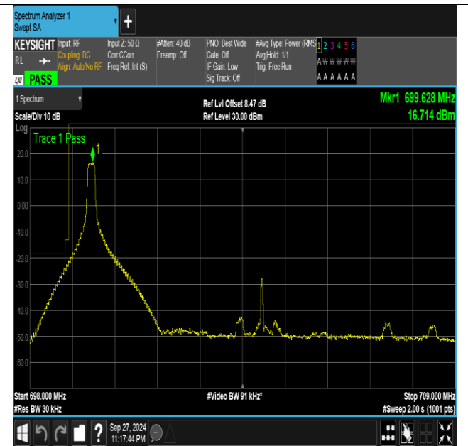
Band12_10MHz_16QAM_23060_1RB#0
