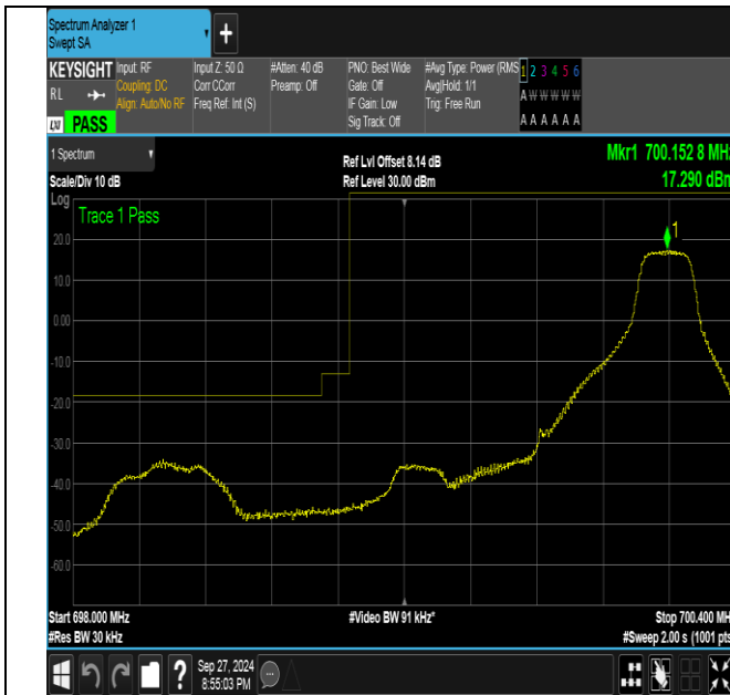
Band12_1.4MHz_QPSK_23017_1RB#5
