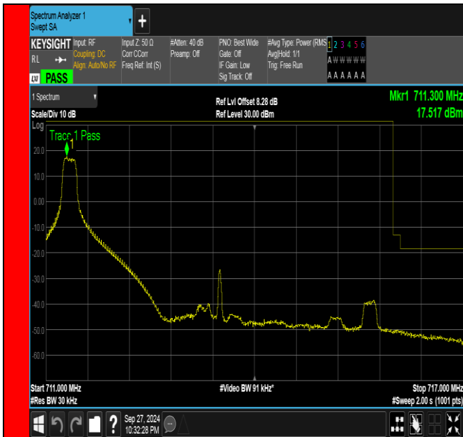
Band12_5MHz_QPSK_23155_1RB#0
