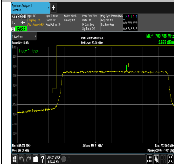
Band12_3MHz_QPSK_23025_15RB#0
