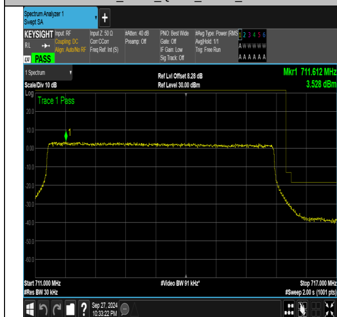
Band12_5MHz_QPSK_23155_25RB#0
