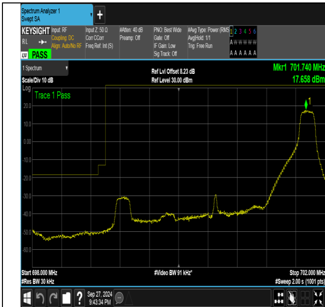
Band12_3MHz_QPSK_23025_1RB#14
