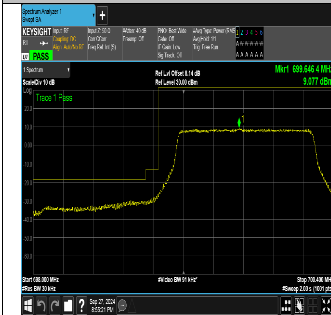
Band12_1.4MHz_QPSK_23017_6RB#0
