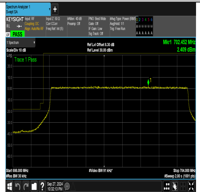
Band12_5MHz_16QAM_23035_25RB#0
