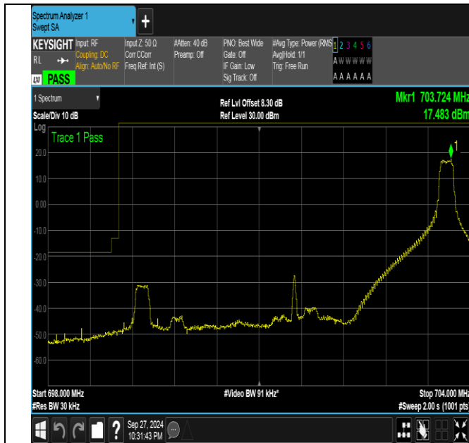
Band12_5MHz_QPSK_23035_1RB#24
