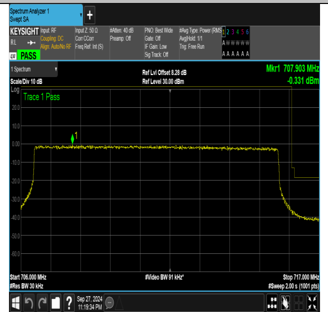
Band12_10MHz_16QAM_23130_50RB#0
