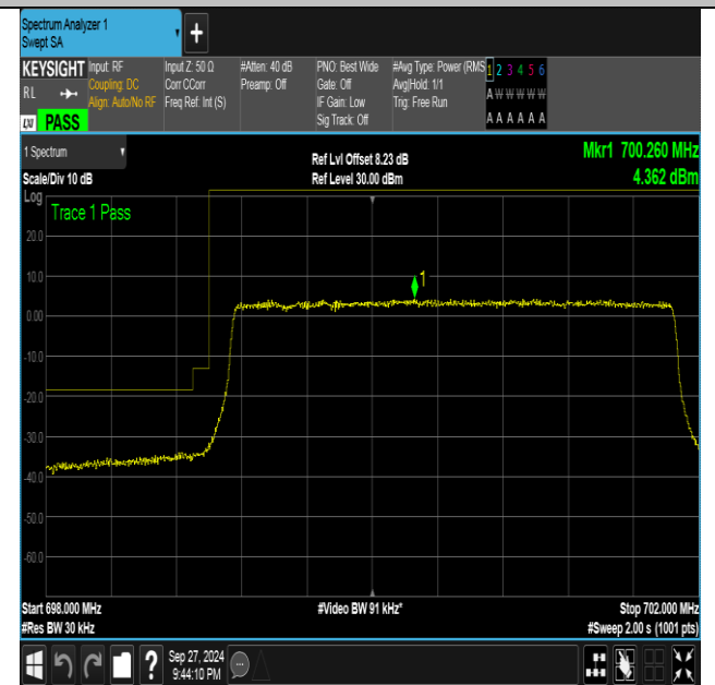
Band12_3MHz_16QAM_23025_15RB#0
