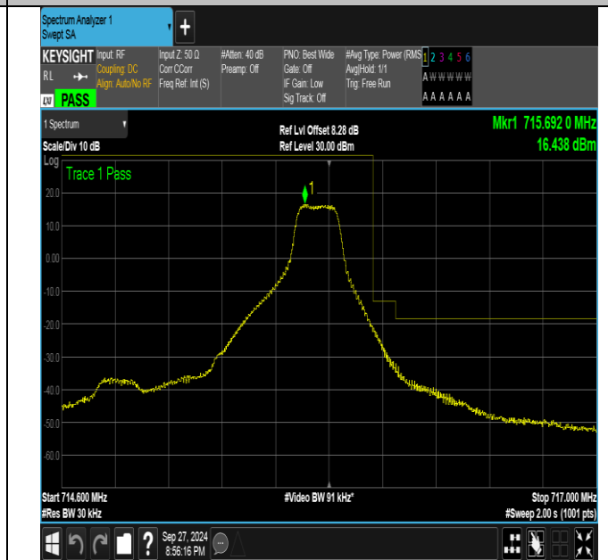
Band12_1.4MHz_16QAM_23173_1RB#5
