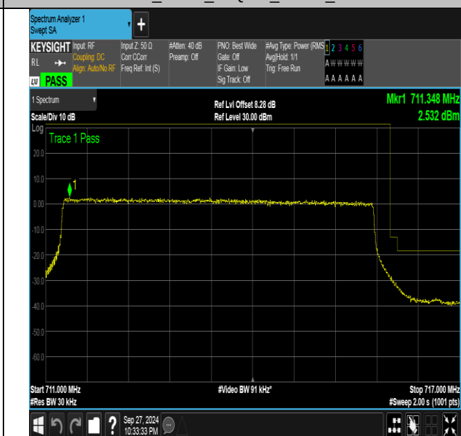
Band12_5MHz_16QAM_23155_25RB#0
