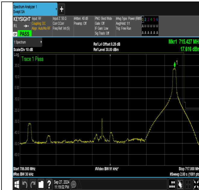
Band12_10MHz_QPSK_23130_1RB#49
