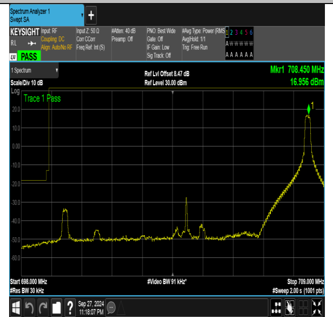
Band12_10MHz_16QAM_23060_1RB#49
