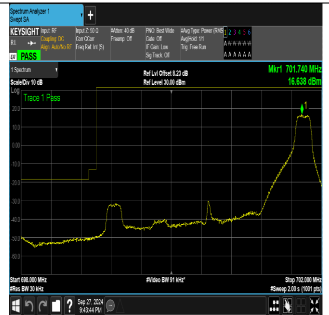
Band12_3MHz_16QAM_23025_1RB#14
