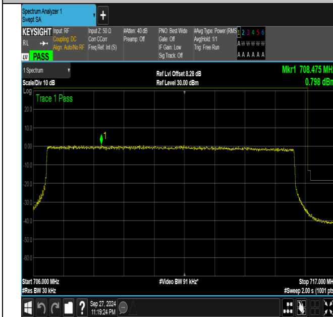
Band12_10MHz_QPSK_23130_50RB#0
