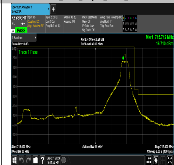
Band12_3MHz_16QAM_23165_1RB#14
