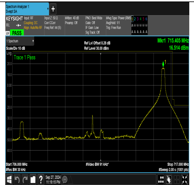
Band12_10MHz_16QAM_23130_1RB#49
