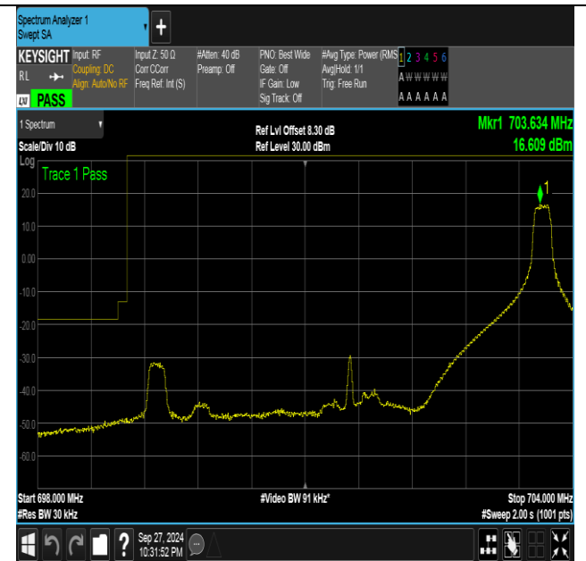
Band12_5MHz_16QAM_23035_1RB#24
