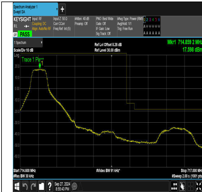
Band12_1.4MHz_QPSK_23173_1RB#0
