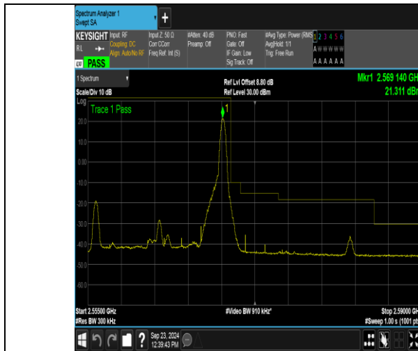
Band7_15MHz_QPSK_21375_1RB#74
