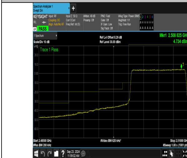
Band7_10MHz_QPSK_20800_50RB#0
