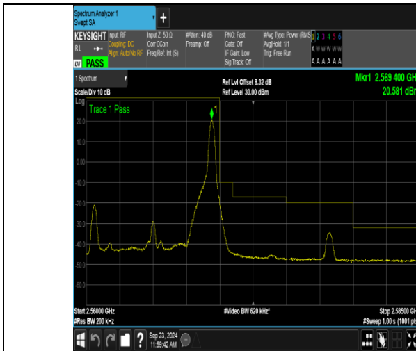
Band7_10MHz_QPSK_21400_1RB#49
