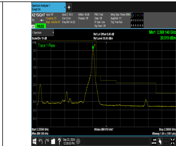
Band7_15MHz_16QAM_21375_1RB#74
