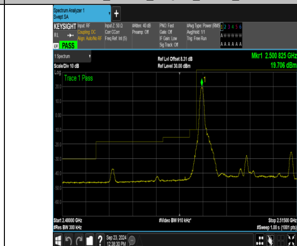
Band7_15MHz_16QAM_20825_1RB#0
