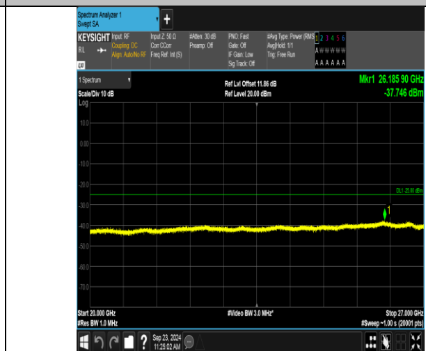
Band7_5MHz_16QAM_20775_25RB#0_20000~27000_20000~27000
