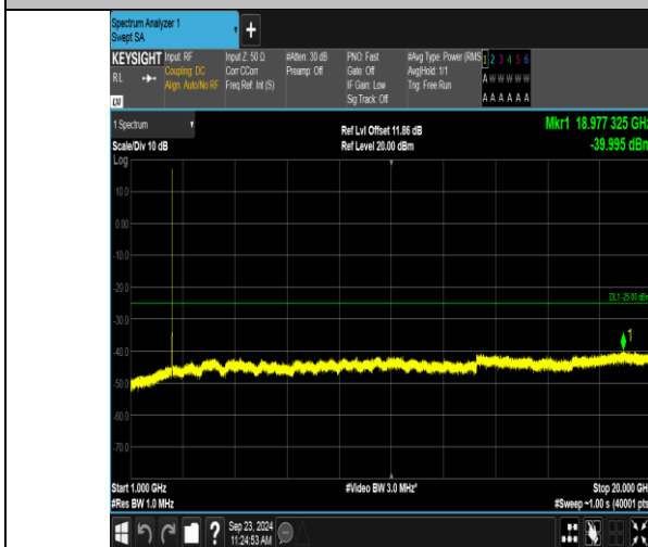
Band7_5MHz_16QAM_20775_25RB#0_1000~20000_1000~20000
