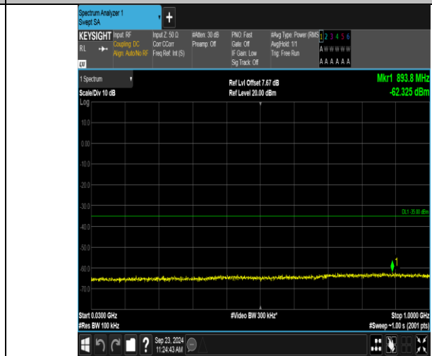
Band7_5MHz_16QAM_20775_25RB#0_30~1000_30~1000
