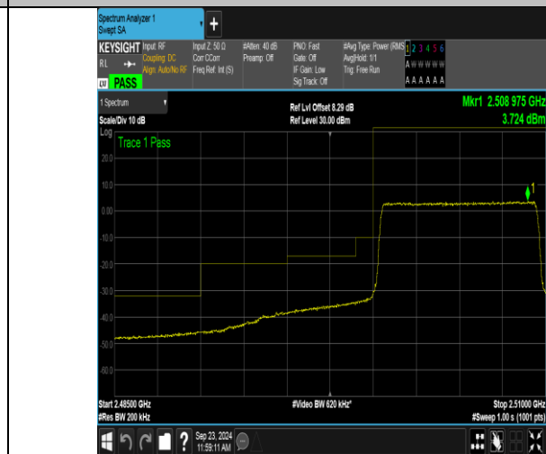
Band7_10MHz_16QAM_20800_50RB#0
