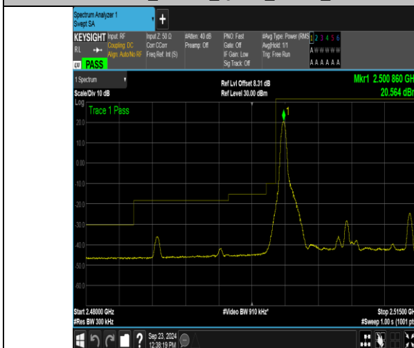
Band7_15MHz_QPSK_20825_1RB#0
