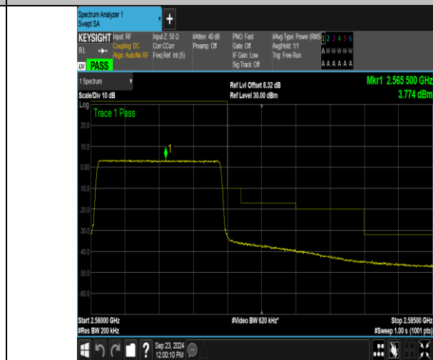
Band7_10MHz_16QAM_21400_50RB#0
