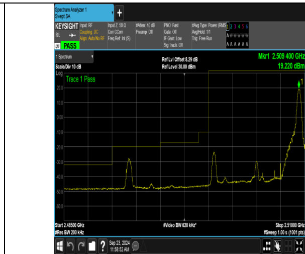
Band7_10MHz_16QAM_20800_1RB#49
