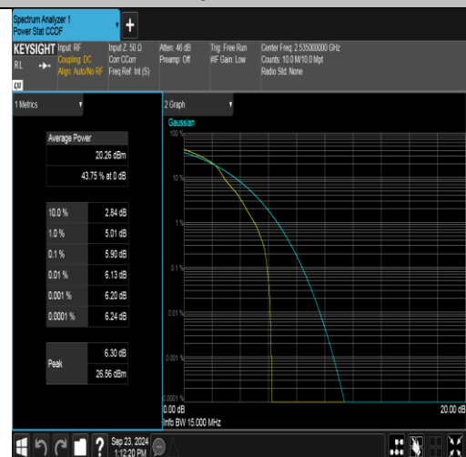
Band7-15MHz-16QAM-21100-1RB#0-PASS
