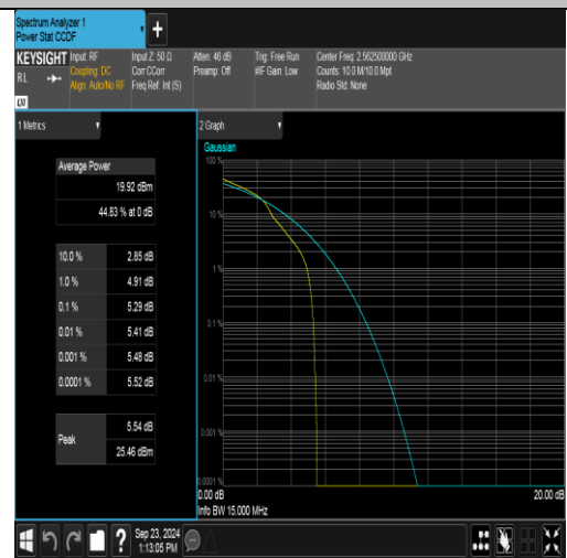
Band7-15MHz-16QAM-21375-1RB#0-PASS
