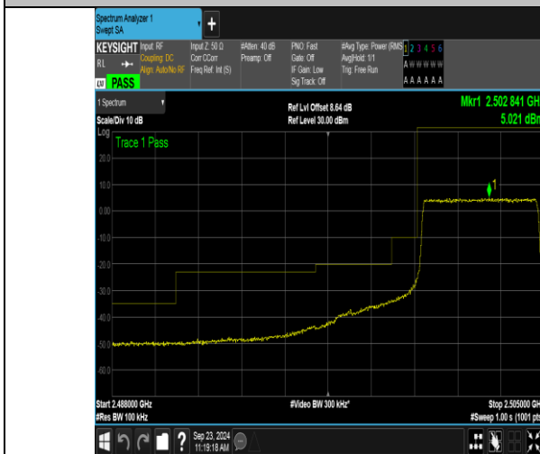
Band7_5MHz_QPSK_20775_25RB#0
