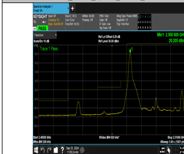
Band7_10MHz_QPSK_20800_1RB#0
