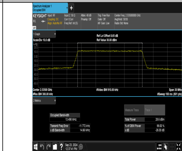
Band7-15MHz-16QAM-21100-75RB#0-PASS
