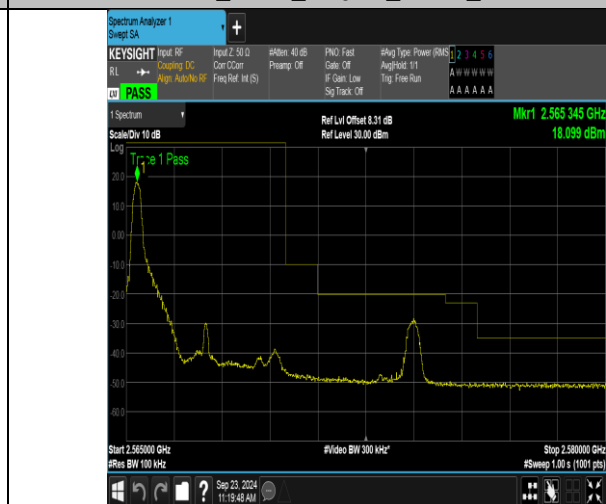
Band7_5MHz_16QAM_21425_1RB#0
