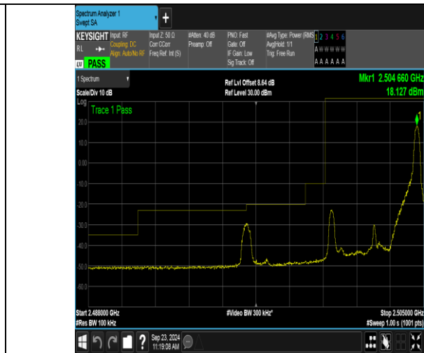
Band7_5MHz_16QAM_20775_1RB#24
