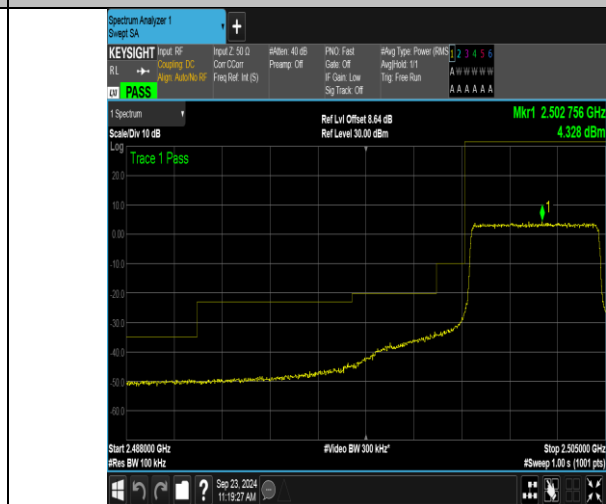
Band7_5MHz_16QAM_20775_25RB#0
