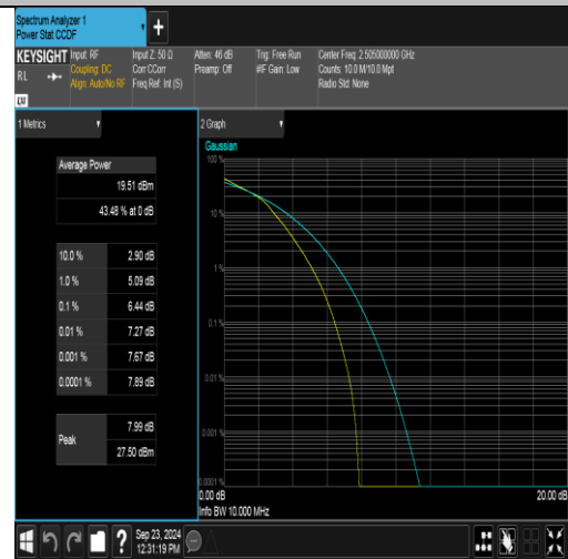
Band7-10MHz-16QAM-20800-50RB#0-PASS
