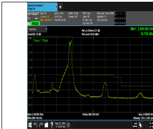
Band7_5MHz_QPSK_21425_1RB#24
