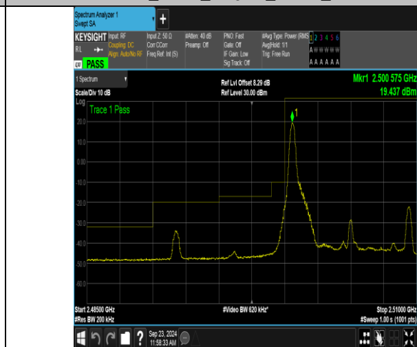
Band7_10MHz_16QAM_20800_1RB#0
