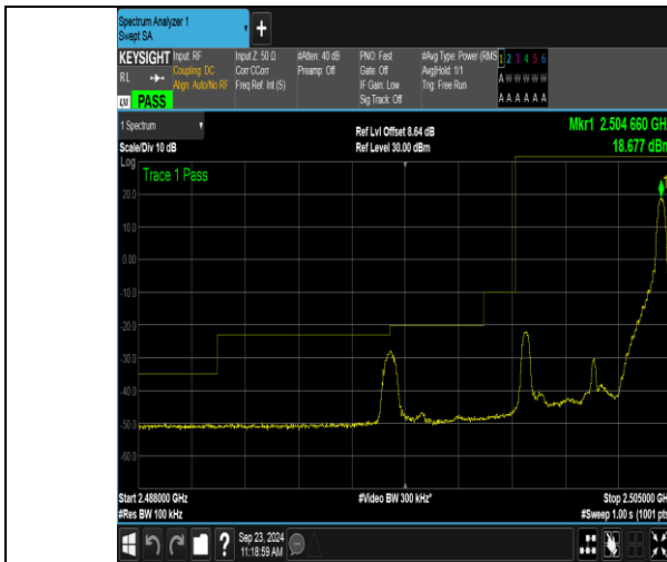
Band7_5MHz_QPSK_20775_1RB#24
