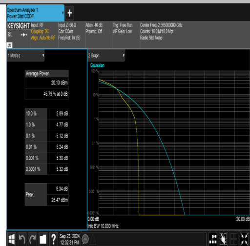
Band7-10MHz-16QAM-21400-1RB#0-PASS
