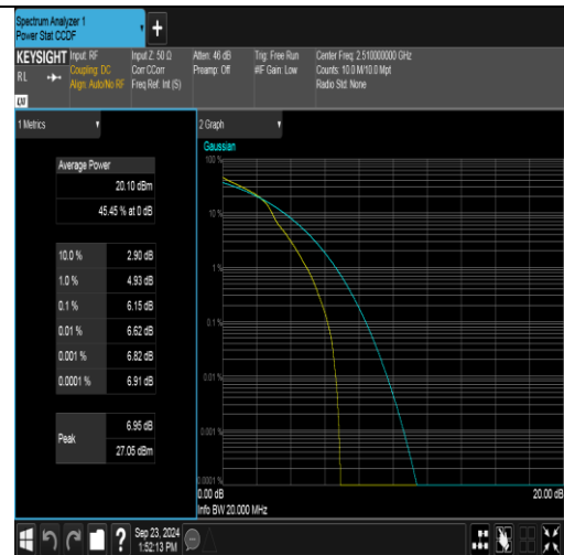
Band7-20MHz-16QAM-20850-1RB#0-PASS
