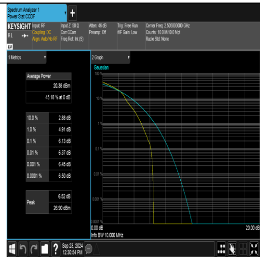
Band7-10MHz-16QAM-20800-1RB#0-PASS
