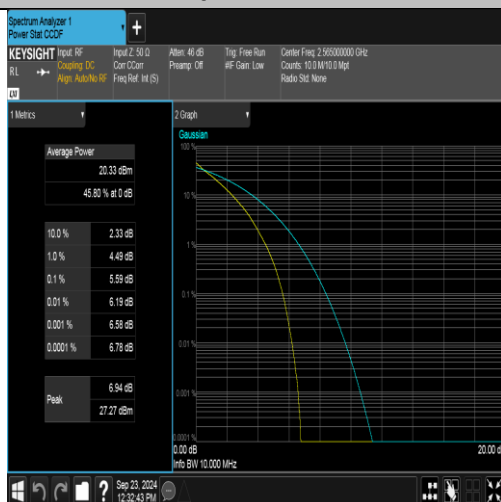
Band7-10MHz-QPSK-21400-50RB#0-PASS
