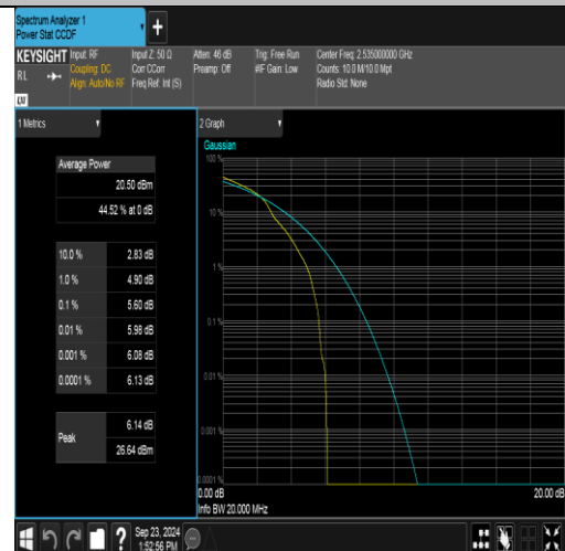
Band7-20MHz-16QAM-21100-1RB#0-PASS
