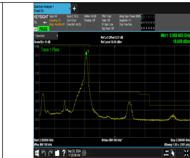
Band7_5MHz_16QAM_21425_1RB#24
