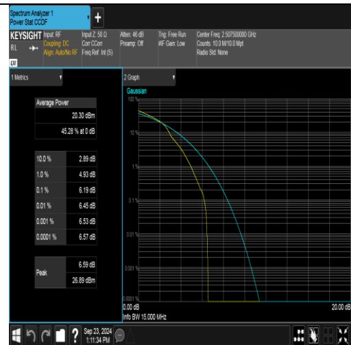
Band7-15MHz-16QAM-20825-1RB#0-PASS
