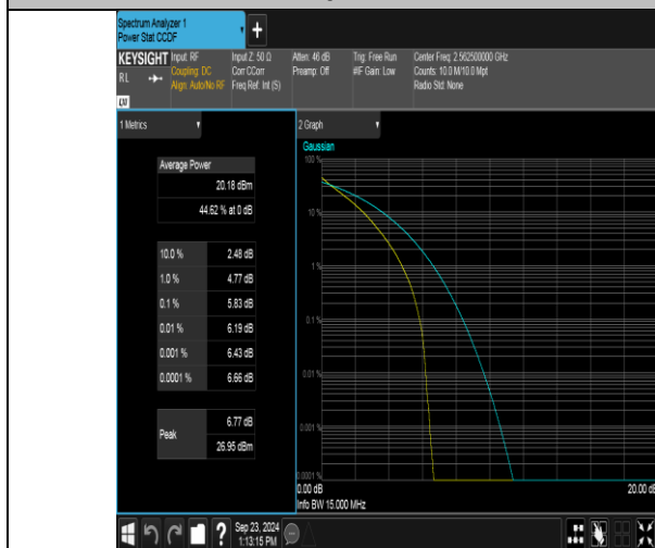
Band7-15MHz-QPSK-21375-75RB#0-PASS
