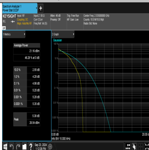
Band7-15MHz-QPSK-21100-1RB#0-PASS
