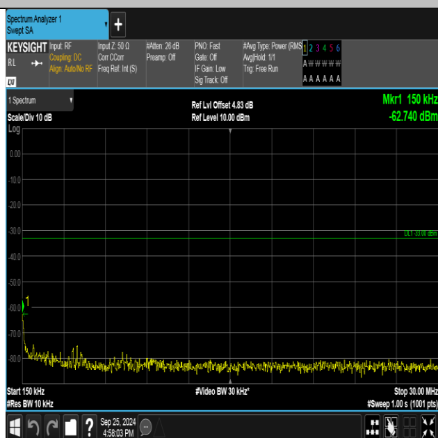
Band2-9538-2-0.15~30MHz-PASS
