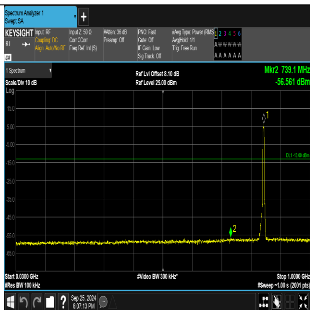
Band5-4233-3-30~1000MHz-PASS
