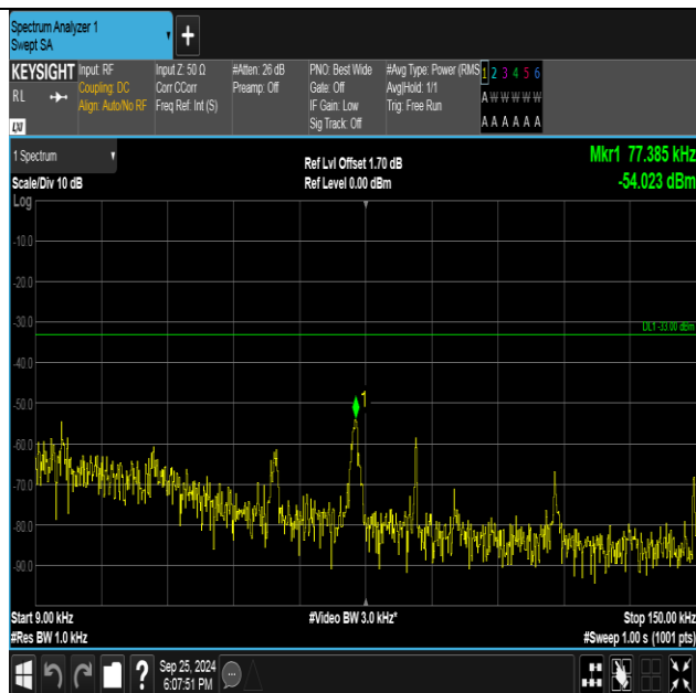
Band5-4132-4-0.009~0.15MHz-PASS
