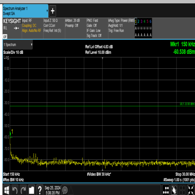
Band2-9538-4-0.15~30MHz-PASS
