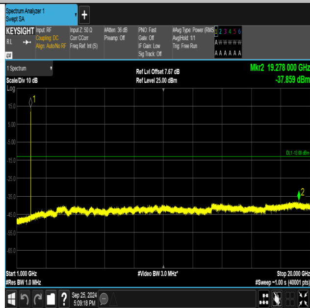
Band2-9538-5-1000~20000MHz-PASS
