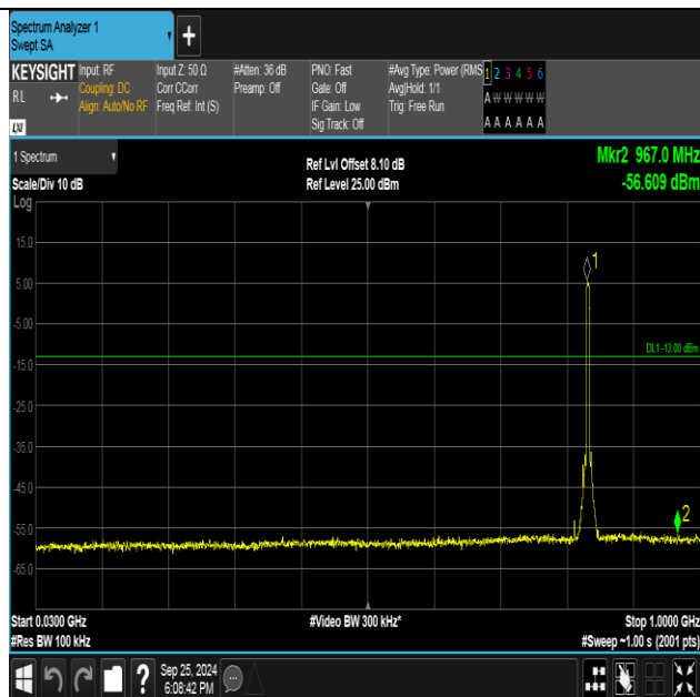
Band5-4182-4-30~1000MHz-PASS
