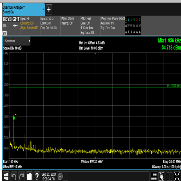
Band5-4182-4-0.15~30MHz-PASS
