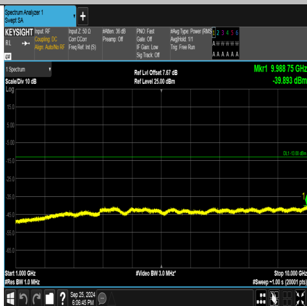
Band5-4182-3-1000~10000MHz-PASS
