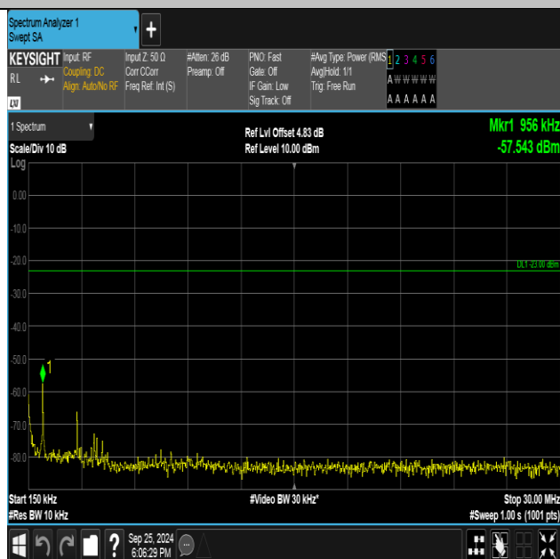
Band5-4182-3-0.15~30MHz-PASS
