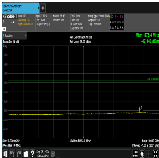
Band2-9538-4-30~1000MHz-PASS
