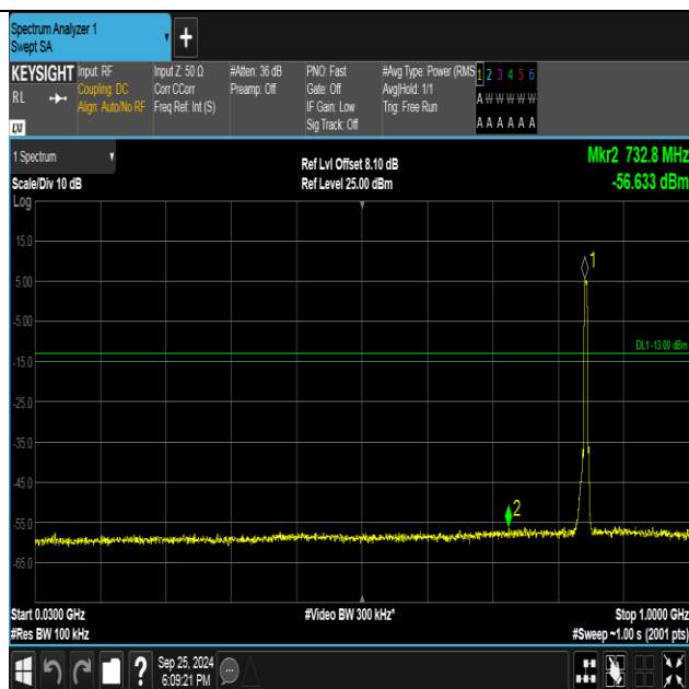
Band5-4233-4-30~1000MHz-PASS
