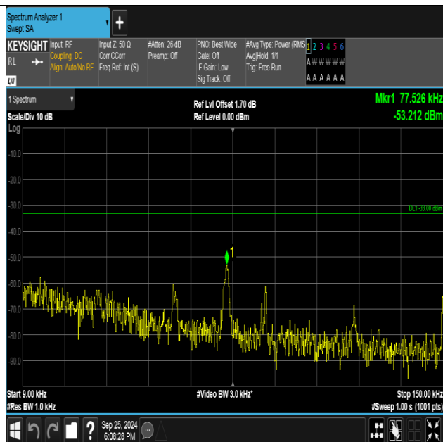
Band5-4182-4-0.009~0.15MHz-PASS
