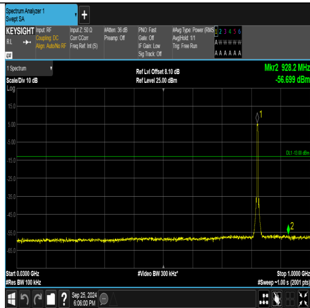
Band5-4132-3-30~1000MHz-PASS
