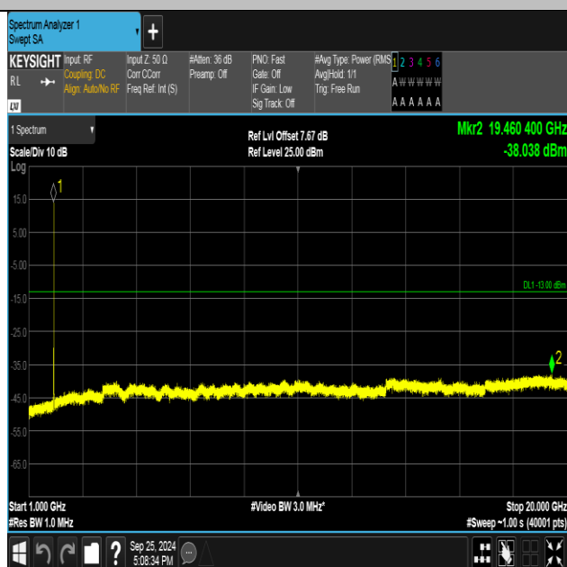
Band2-9400-5-1000~20000MHz-PASS
