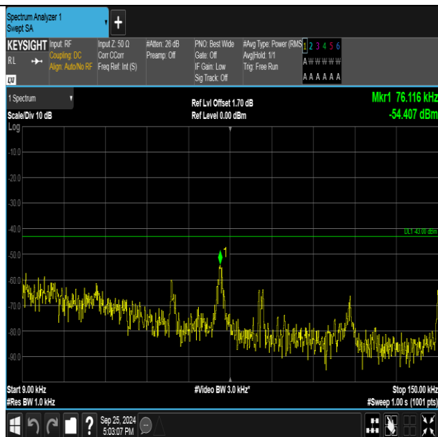
Band2-9262-4-0.009~0.15MHz-PASS
