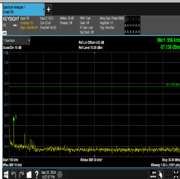
Band5-4132-4-0.15~30MHz-PASS
