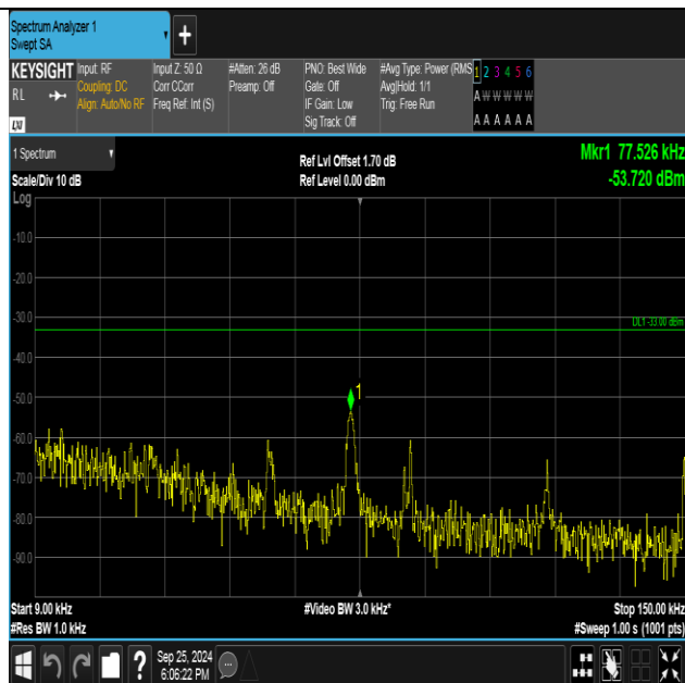
Band5-4182-3-0.009~0.15MHz-PASS
