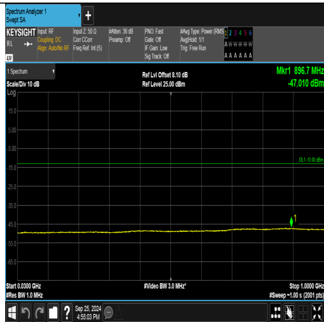
Band2-9262-2-30~1000MHz-PASS
