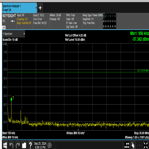
Band5-4233-4-0.15~30MHz-PASS
