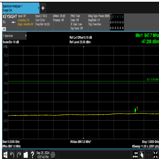
Band2-9262-5-30~1000MHz-PASS
