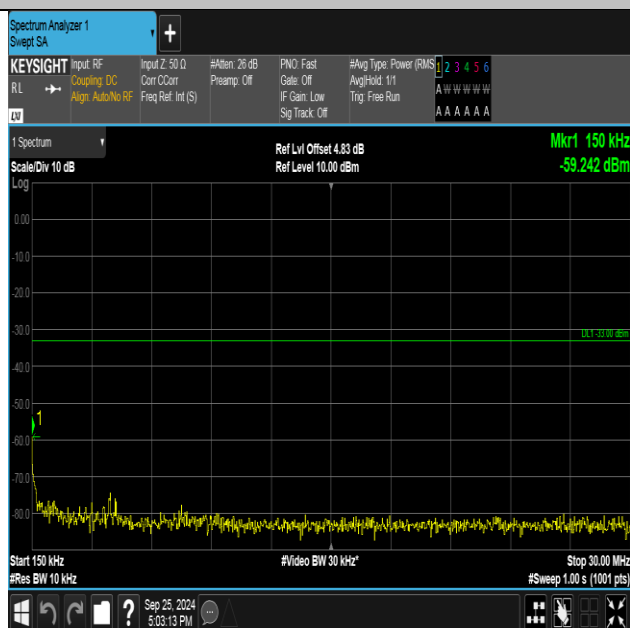
Band2-9262-4-0.15~30MHz-PASS
