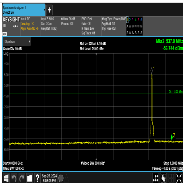
Band5-4132-4-30~1000MHz-PASS
