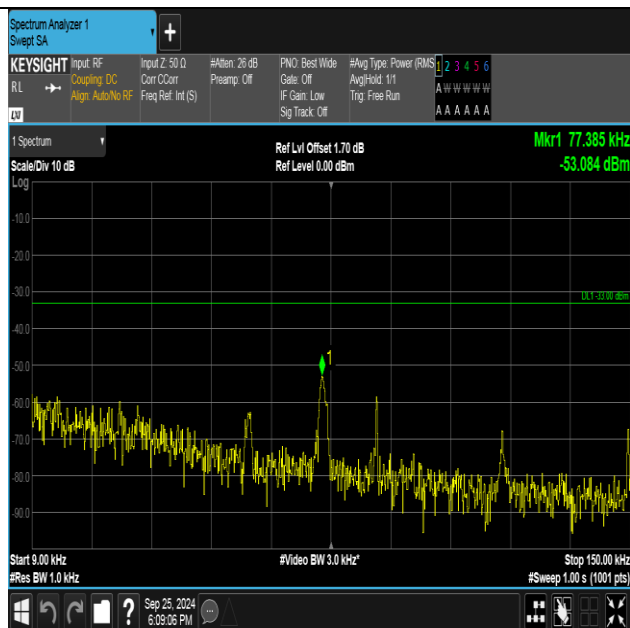
Band5-4233-4-0.009~0.15MHz-PASS
