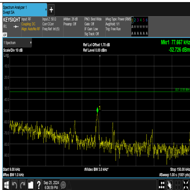
Band5-4233-3-0.009~0.15MHz-PASS
