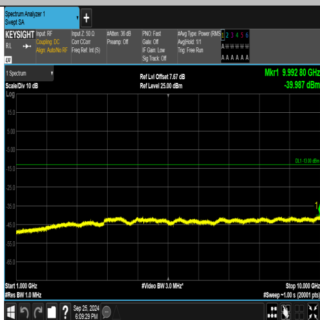
Band5-4233-4-1000~10000MHz-PASS
