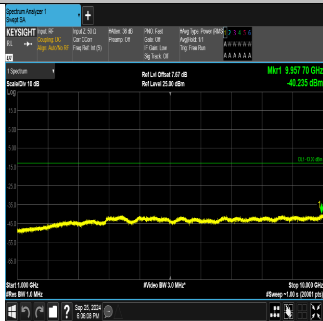
Band5-4132-3-1000~10000MHz-PASS
