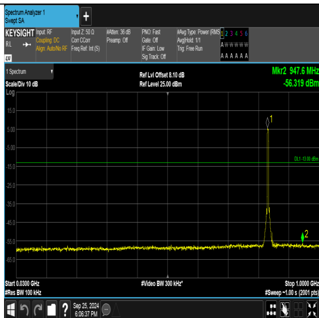
Band5-4182-3-30~1000MHz-PASS
