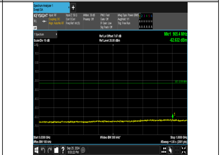
Band4_3MHz_16QAM_19965_15RB#0_30~1000_30~1000
