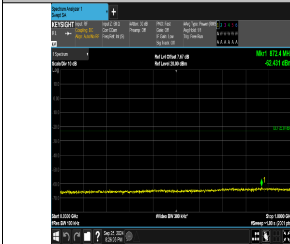
Band4_1.4MHz_QPSK_20393_1RB#5_30~1000_30~1000
