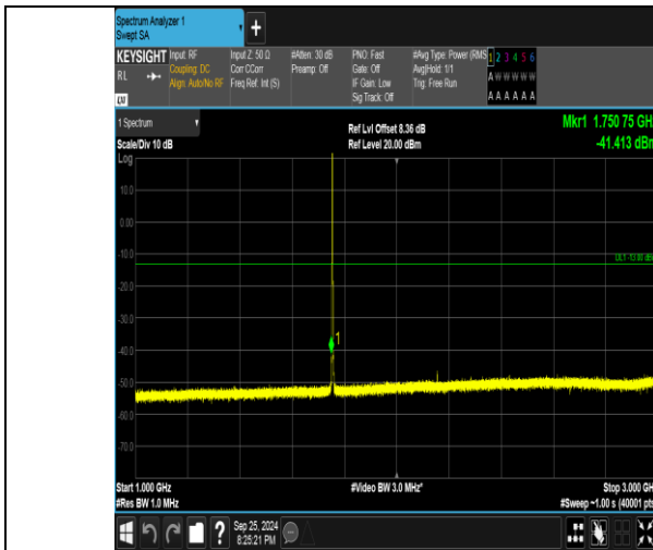
Band4_1.4MHz_16QAM_20393_1RB#0_1000~3000_1000~3000
