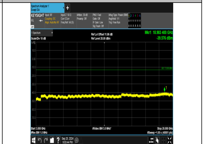
Band4_3MHz_16QAM_19965_15RB#0_3000~20000_3000~20000
