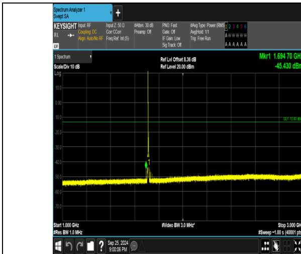
Band4_3MHz_16QAM_19965_1RB#0_1000~3000_1000~3000
