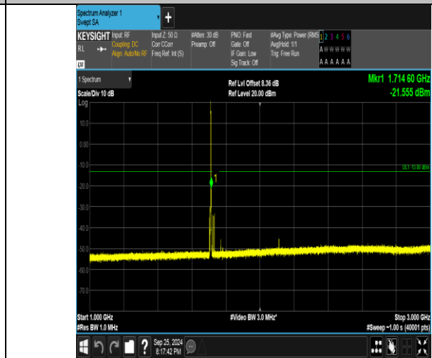
Band4_1.4MHz_QPSK_19957_6RB#0_1000~3000_1000~3000
