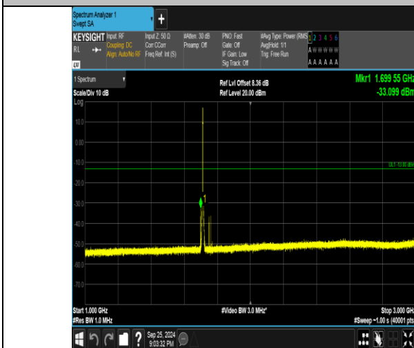
Band4_3MHz_16QAM_19965_15RB#0_1000~3000_1000~3000
