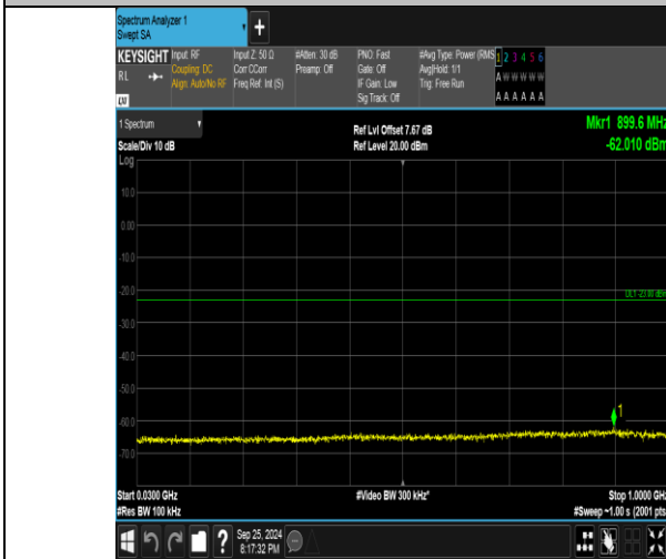
Band4_1.4MHz_QPSK_19957_6RB#0_30~1000_30~1000
