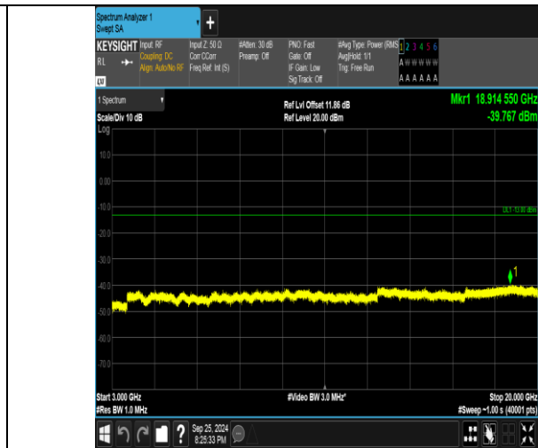
Band4_1.4MHz_16QAM_20393_1RB#0_3000~20000_3000~20000
