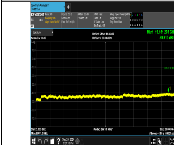
Band4_3MHz_QPSK_19965_1RB#14_3000~20000_3000~20000
