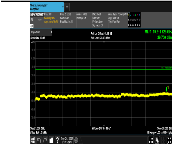
Band4_1.4MHz_QPSK_19957_6RB#0_3000~20000_3000~20000
