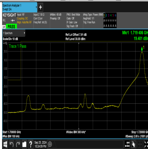
Band4_10MHz_QPSK_20000_1RB#49
