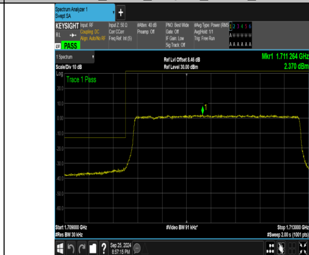
Band4_3MHz_16QAM_19965_15RB#0
