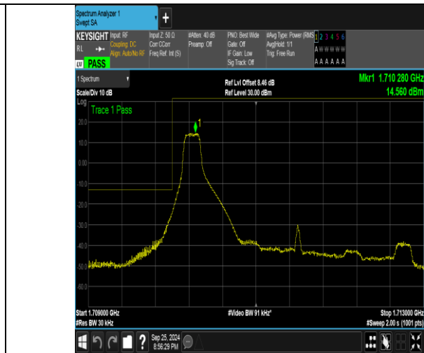
Band4_3MHz_16QAM_19965_1RB#0
