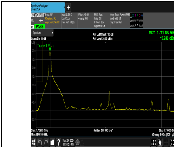
Band4_20MHz_QPSK_20050_1RB#0
