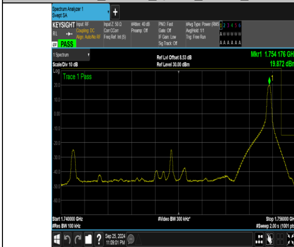
Band4_15MHz_QPSK_20325_1RB#74
