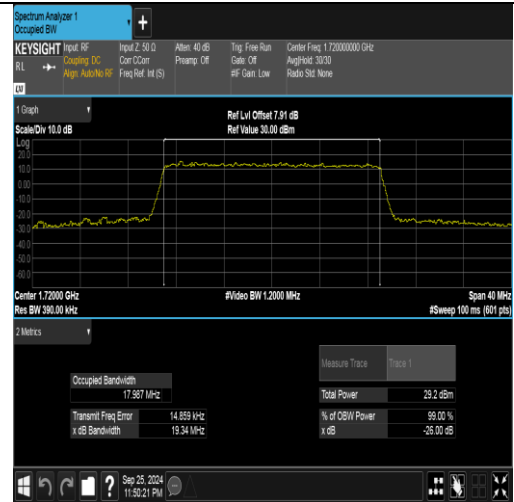
Band4-20MHz-16QAM-20050-100RB#0-PASS
