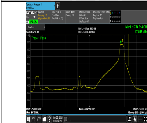
Band4_5MHz_QPSK_20375_1RB#24
