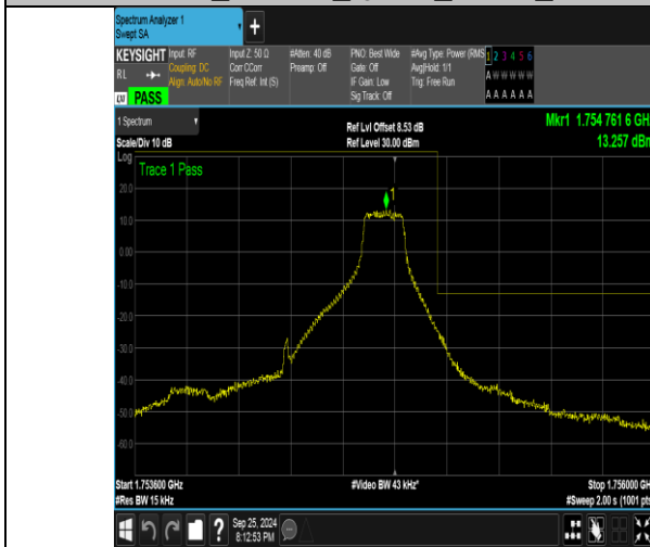
Band4_1.4MHz_QPSK_20393_1RB#5
