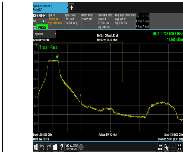
Band4_1.4MHz_16QAM_20393_1RB#0
