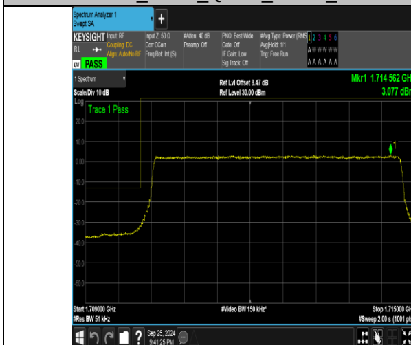
Band4_5MHz_QPSK_19975_25RB#0
