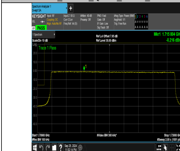
Band4_20MHz_QPSK_20050_100RB#0
