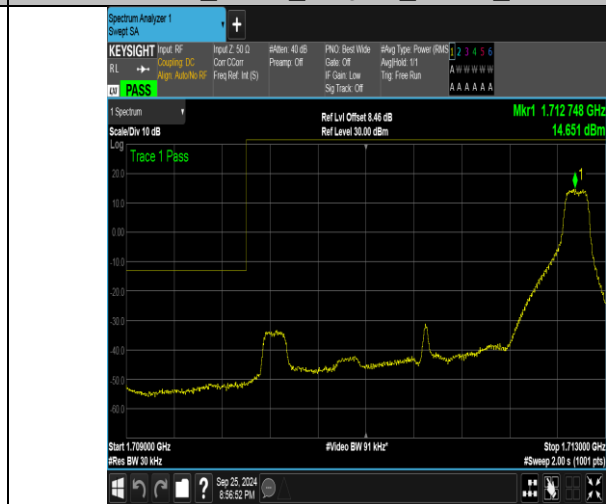
Band4_3MHz_16QAM_19965_1RB#14
