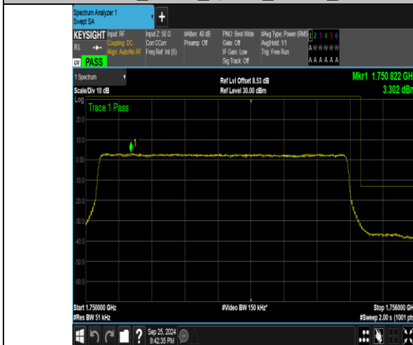
Band4_5MHz_QPSK_20375_25RB#0
