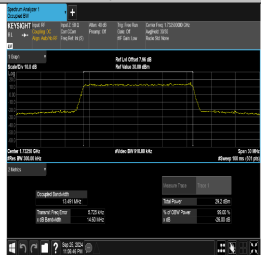
Band4-15MHz-16QAM-20175-75RB#0-PASS
