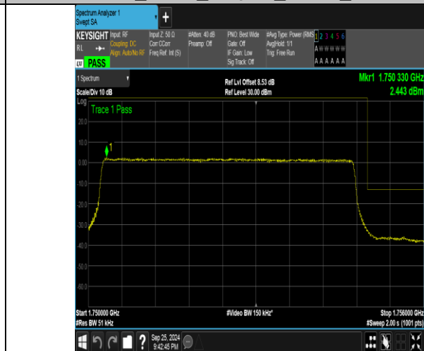
Band4_5MHz_16QAM_20375_25RB#0
