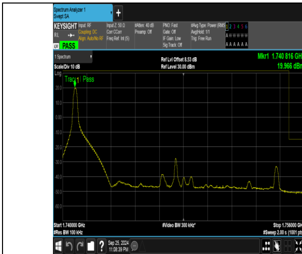
Band4_15MHz_QPSK_20325_1RB#0
