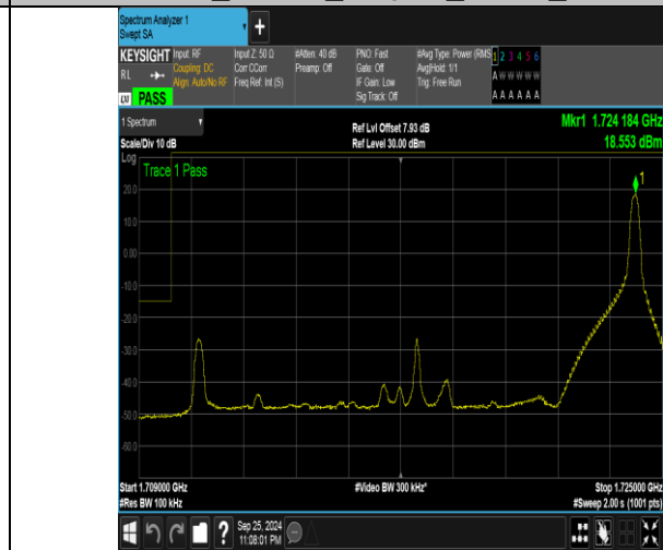
Band4_15MHz_16QAM_20025_1RB#74
