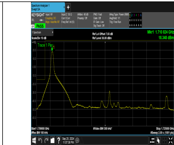
Band4_15MHz_16QAM_20025_1RB#0
