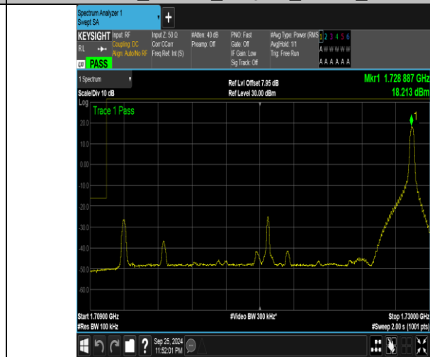
Band4_20MHz_16QAM_20050_1RB#99
