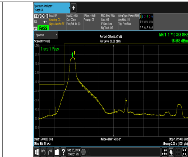
Band4_5MHz_16QAM_19975_1RB#0
