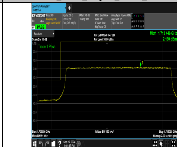
Band4_5MHz_16QAM_19975_25RB#0
