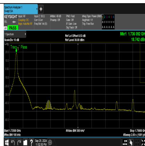
Band4_20MHz_16QAM_20300_1RB#0
