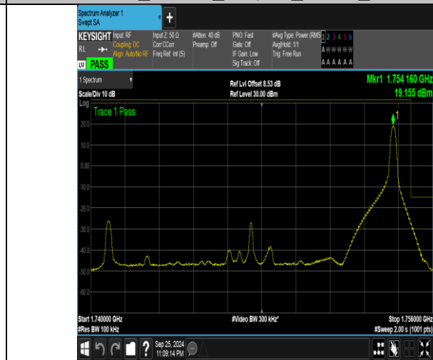
Band4_15MHz_16QAM_20325_1RB#74
