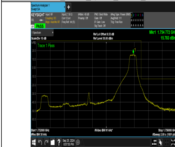
Band4_3MHz_QPSK_20385_1RB#14
