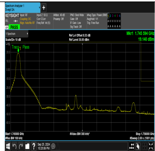
Band4_10MHz_16QAM_20350_1RB#0
