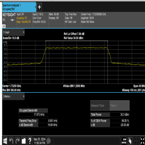
Band4-20MHz-QPSK-20175-100RB#0-PASS
