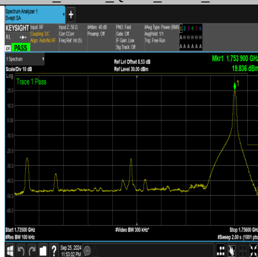
Band4_20MHz_QPSK_20300_1RB#99
