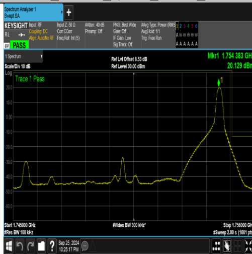
Band4_10MHz_QPSK_20350_1RB#49
