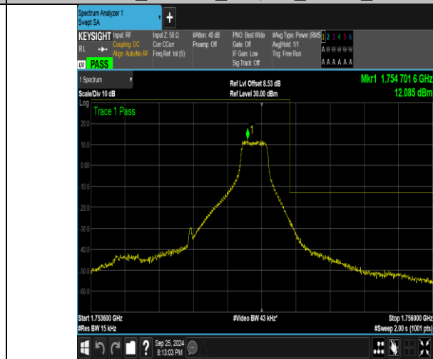
Band4_1.4MHz_16QAM_20393_1RB#5
