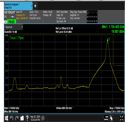
Band4_10MHz_16QAM_20350_1RB#49
