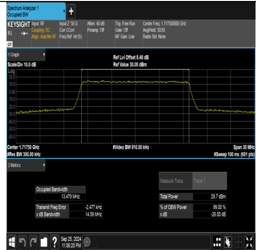
Band4-15MHz-16QAM-2025-75RB#0-PASS
