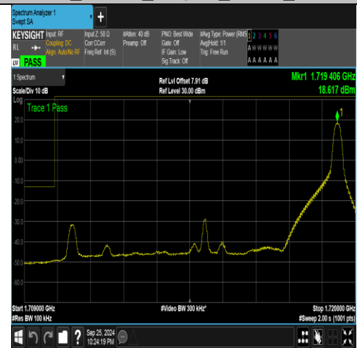
Band4_10MHz_16QAM_20000_1RB#49
