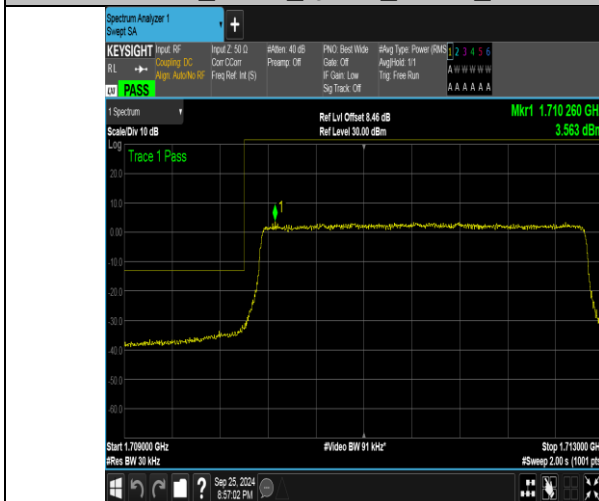
Band4_3MHz_QPSK_19965_15RB#0
