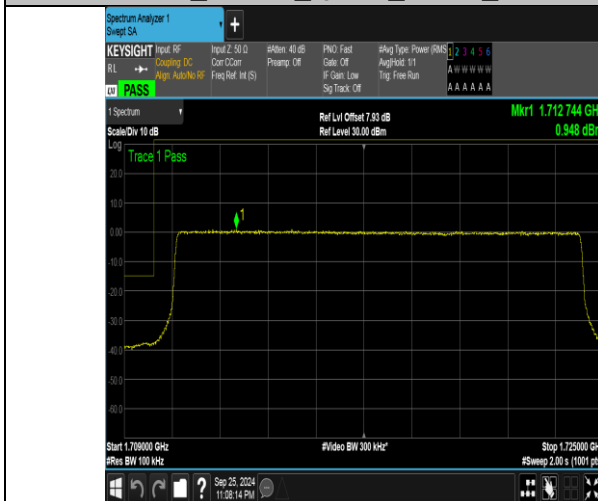
Band4_15MHz_QPSK_20025_75RB#0
