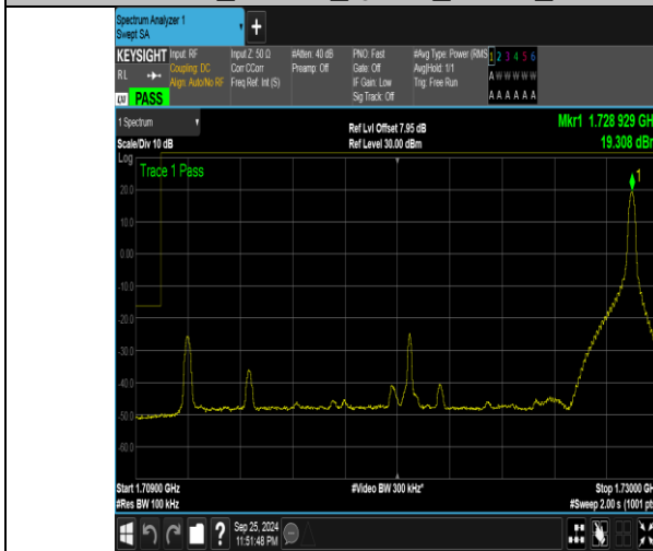
Band4_20MHz_QPSK_20050_1RB#99
