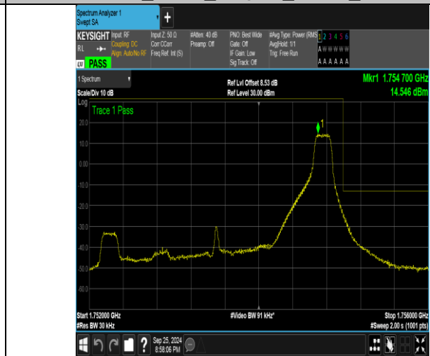
Band4_3MHz_16QAM_20385_1RB#14
