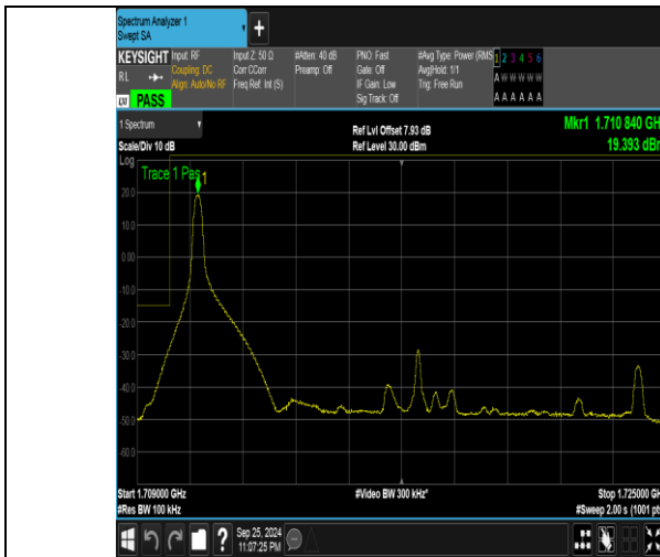
Band4_15MHz_QPSK_20025_1RB#0
