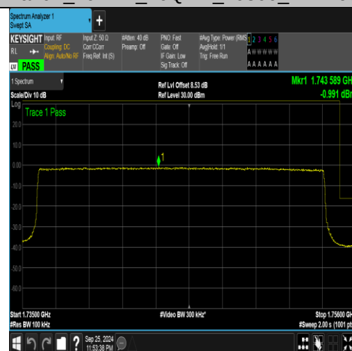
Band4_20MHz_16QAM_20300_100RB#0
