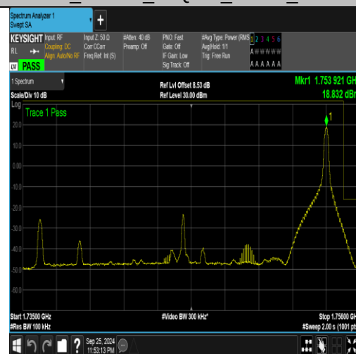
Band4_20MHz_16QAM_20300_1RB#99
