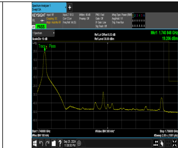
Band4_15MHz_16QAM_20325_1RB#0
