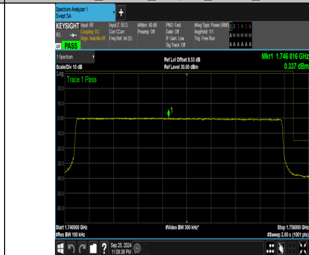
Band4_15MHz_16QAM_20325_75RB#0
