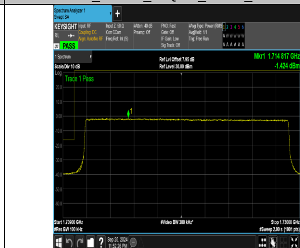
Band4_20MHz_16QAM_20050_100RB#0
