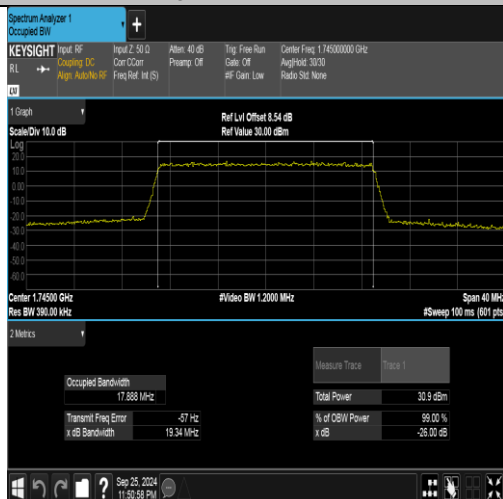
Band4-20MHz-QPSK-20300-100RB#0-PASS
