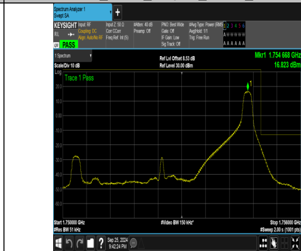
Band4_5MHz_16QAM_20375_1RB#24
