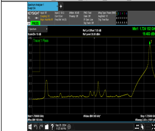
Band4_15MHz_QPSK_20025_1RB#74
