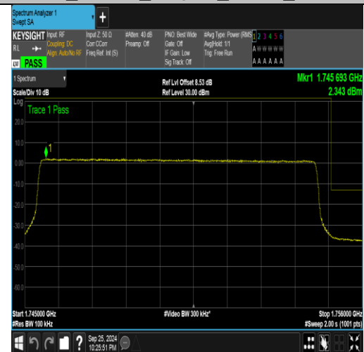
Band4_10MHz_16QAM_20350_50RB#0
