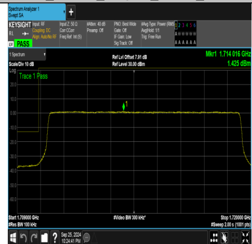
Band4_10MHz_16QAM_20000_50RB#0
