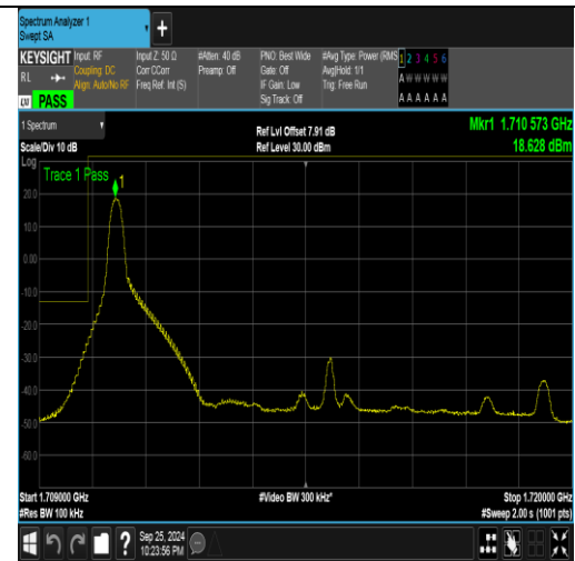
Band4_10MHz_16QAM_20000_1RB#0
