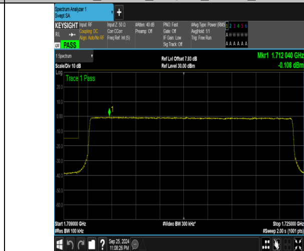
Band4_15MHz_16QAM_20025_75RB#0
