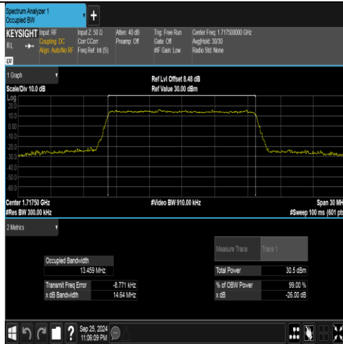
Band4-15MHz-QPSK-2025-75RB#0-PASS
