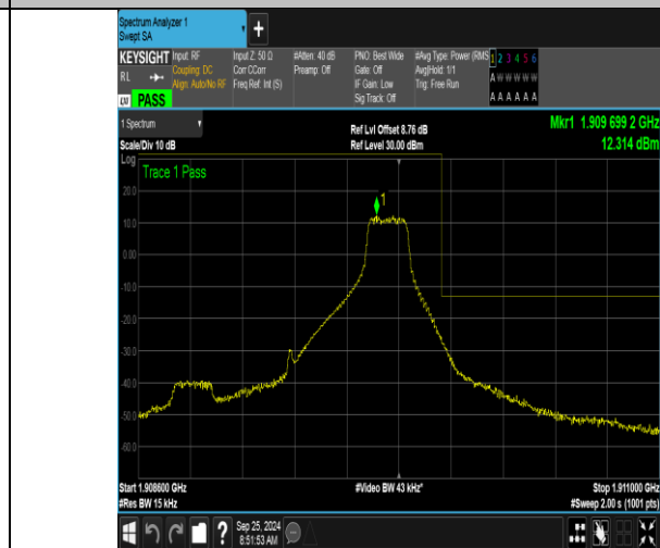
Band2_1.4MHz_16QAM_19193_1RB#5
