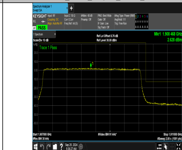
Band2_3MHz_16QAM_19185_15RB#0
