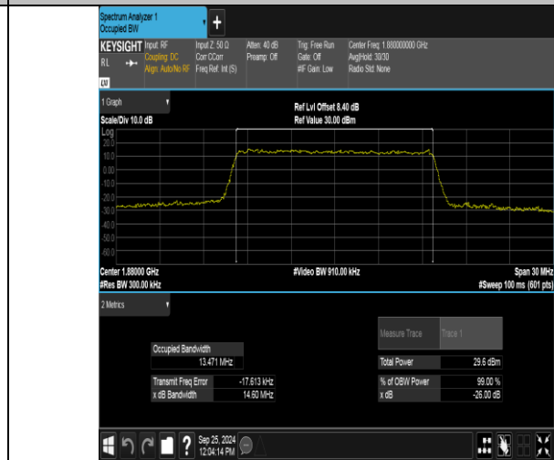
Band2-15MHz-16QAM-18900-75RB#0-PASS
