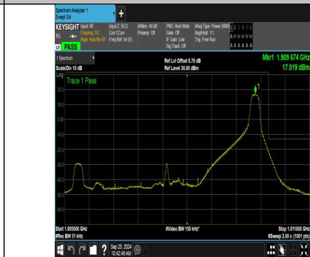
Band2_5MHz_16QAM_19175_1RB#24
