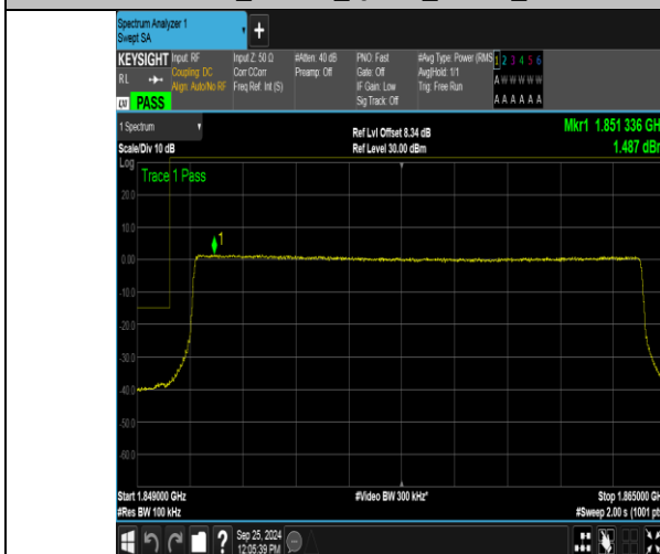
Band2_15MHz_QPSK_18675_75RB#0
