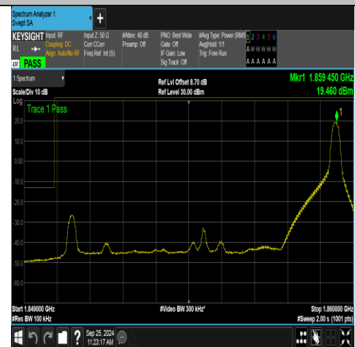
Band2_10MHz_16QAM_18650_1RB#49
