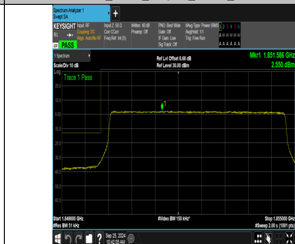
Band2_5MHz_16QAM_18625_25RB#0
