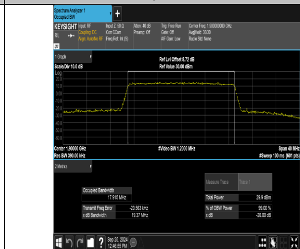
Band2-20MHz-16QAM-19100-100RB#0-PASS
