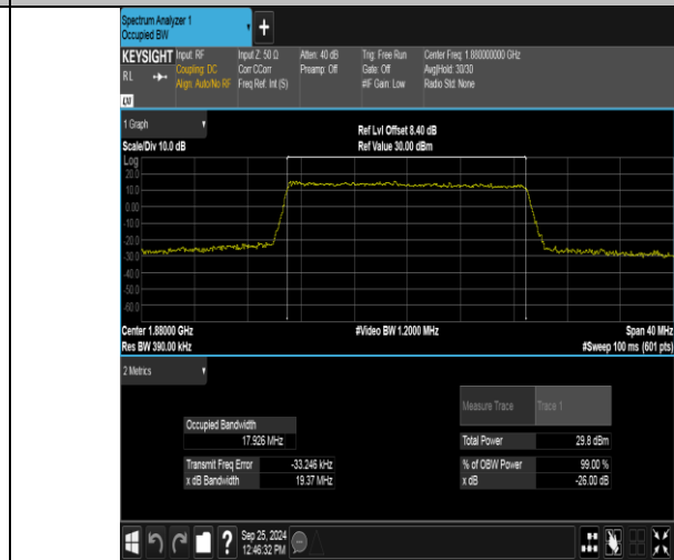
Band2-20MHz-16QAM-18900-100RB#0-PASS
