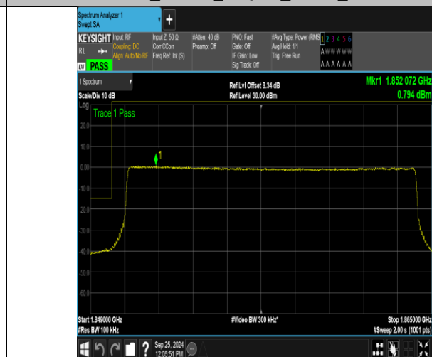
Band2_15MHz_16QAM_18675_75RB#0
