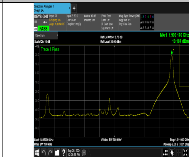
Band2_15MHz_16QAM_19125_1RB#74
