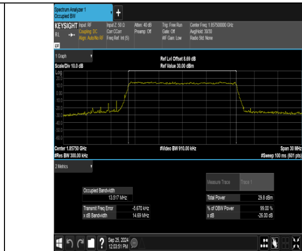
Band2-15MHz-16QAM-18675-75RB#0-PASS
