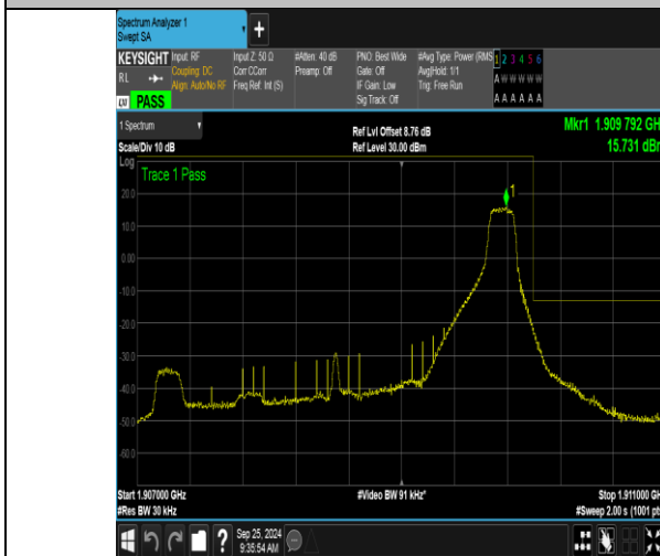
Band2_3MHz_QPSK_19185_1RB#14
