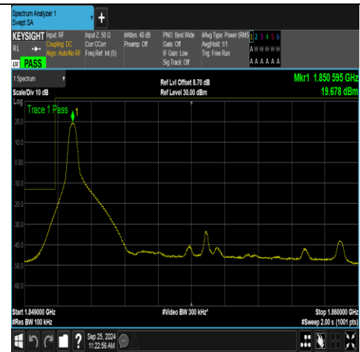
Band2_10MHz_16QAM_18650_1RB#0
