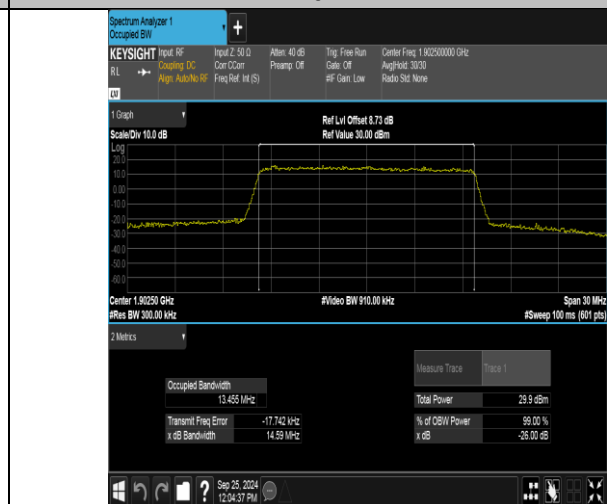
Band2-15MHz-16QAM-19125-75RB#0-PASS
