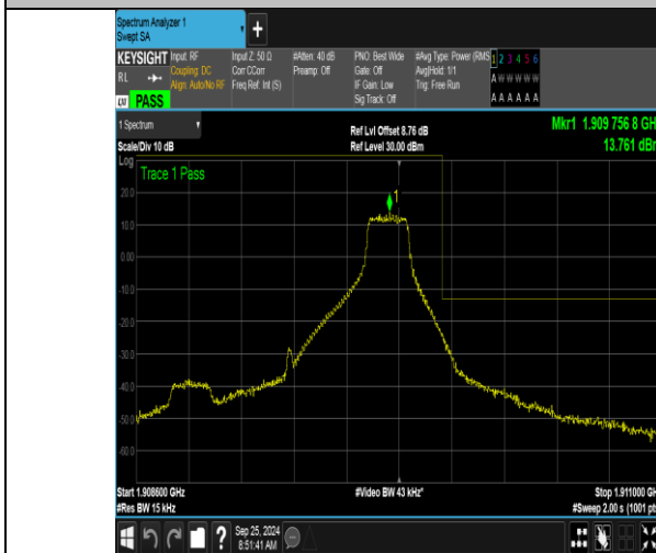
Band2_1.4MHz_QPSK_19193_1RB#5
