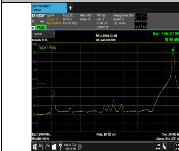
Band2_15MHz_QPSK_18675_1RB#74
