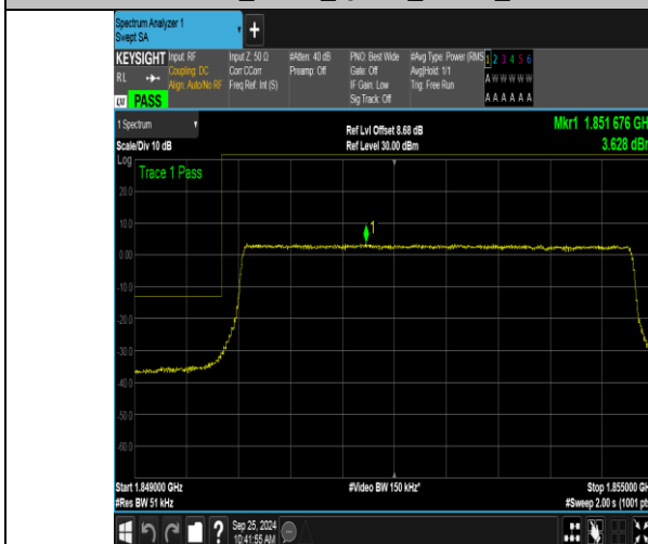
Band2_5MHz_QPSK_18625_25RB#0
