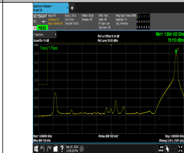
Band2_15MHz_16QAM_18675_1RB#74
