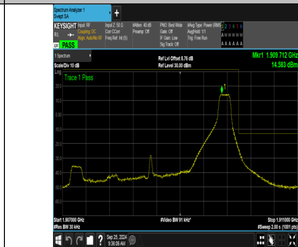
Band2_3MHz_16QAM_19185_1RB#14
