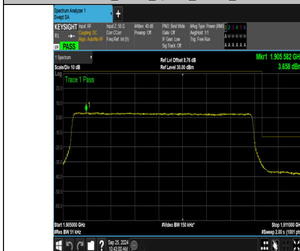
Band2_5MHz_QPSK_19175_25RB#0
