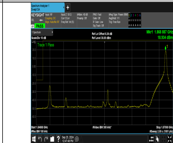
Band2_20MHz_16QAM_18700_1RB#99
