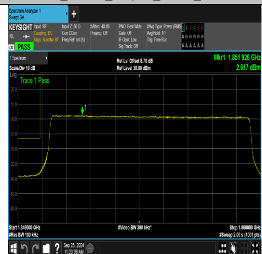
Band2_10MHz_16QAM_18650_50RB#0
