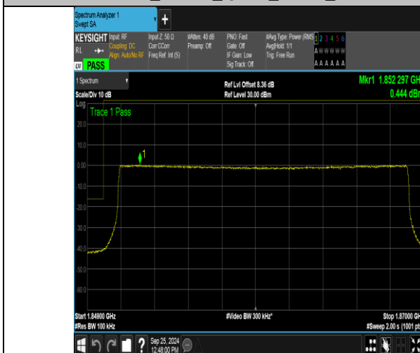
Band2_20MHz_QPSK_18700_100RB#0
