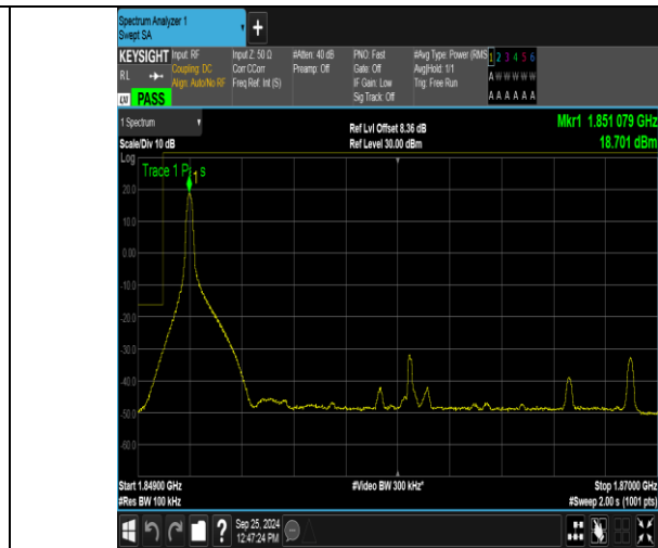
Band2_20MHz_16QAM_18700_1RB#0
