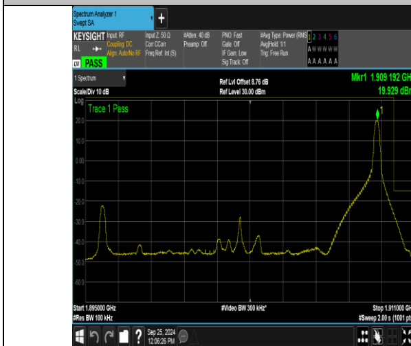
Band2_15MHz_QPSK_19125_1RB#74
