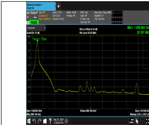
Band2_15MHz_QPSK_19125_1RB#0
