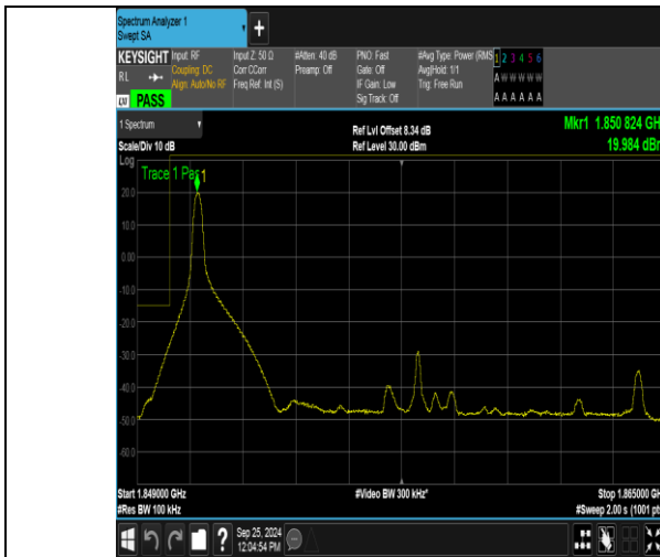
Band2_15MHz_QPSK_18675_1RB#0
