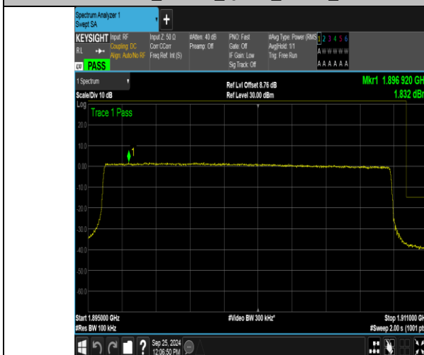
Band2_15MHz_QPSK_19125_75RB#0
