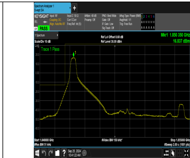
Band2_5MHz_16QAM_18625_1RB#0
