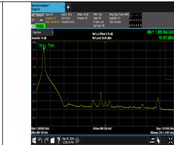
Band2_15MHz_16QAM_19125_1RB#0
