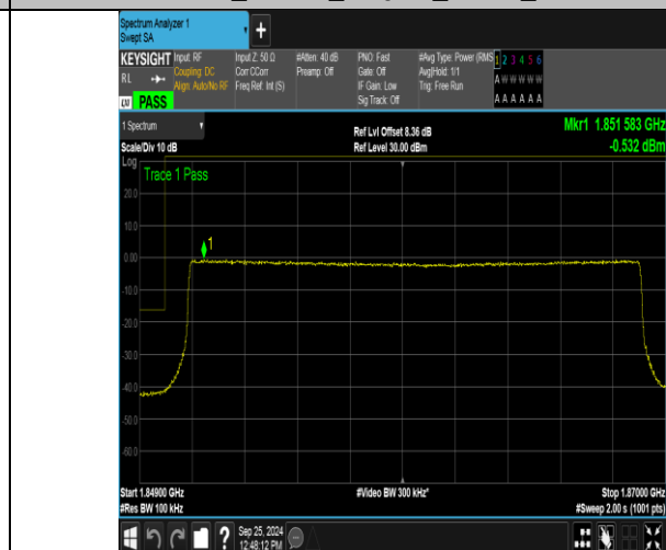
Band2_20MHz_16QAM_18700_100RB#0
