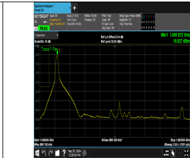
Band2_15MHz_16QAM_18675_1RB#0
