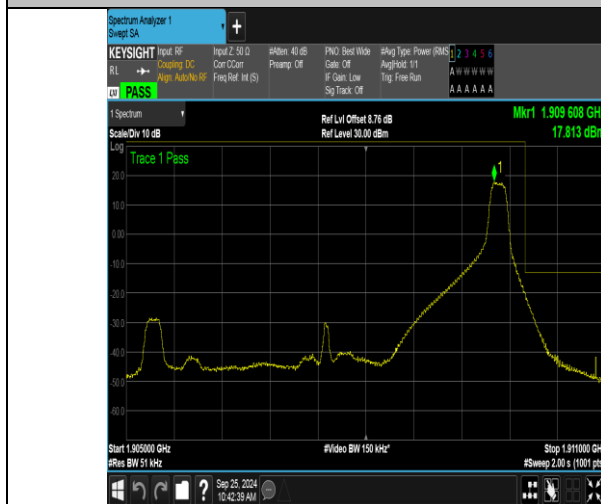
Band2_5MHz_QPSK_19175_1RB#24
