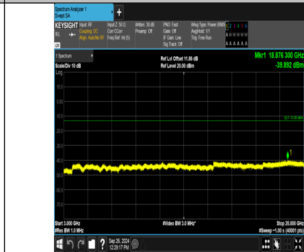
Band4_20MHz_QPSK_20175_1RB#0_3000~20000_3000~20000
