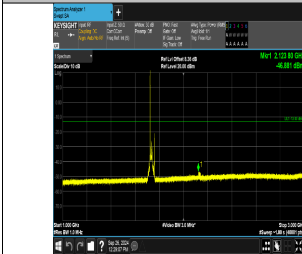
Band4_20MHz_QPSK_20175_1RB#0_1000~3000_1000~3000
