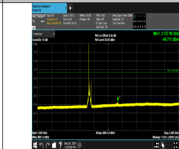
Band4_20MHz_16QAM_20175_1RB#0_1000~3000_1000~3000
