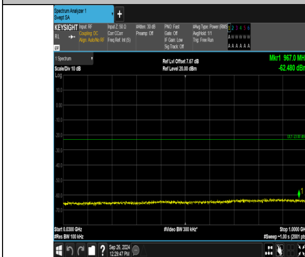
Band4_20MHz_16QAM_20175_1RB#0_30~1000_30~1000
