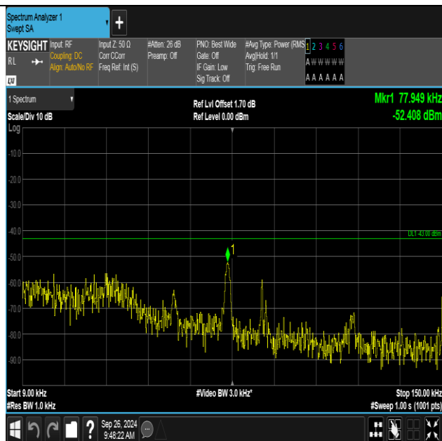
Band4-1513-2-0.009~0.15MHz-PASS
