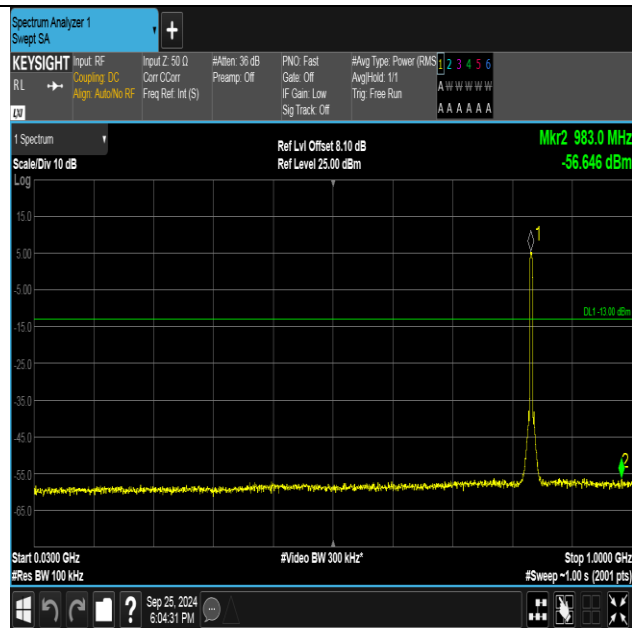
Band5-4182-2-30~1000MHz-PASS
