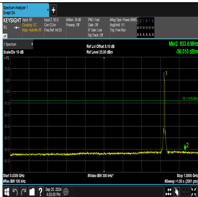
Band5-4132-2-30~1000MHz-PASS
