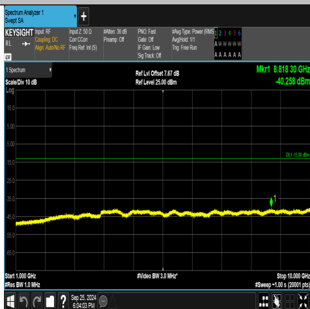
Band5-4132-2-1000~10000MHz-PASS
