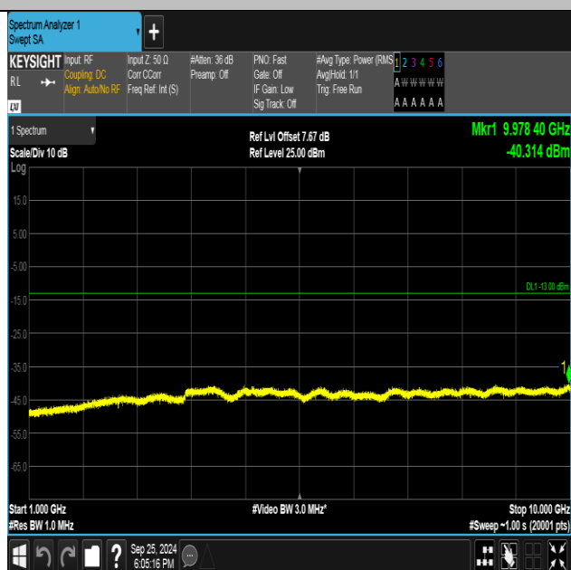
Band5-4233-2-1000~10000MHz-PASS
