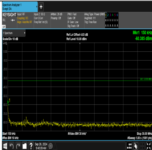
Band4-1312-1-0.15~30MHz-PASS
