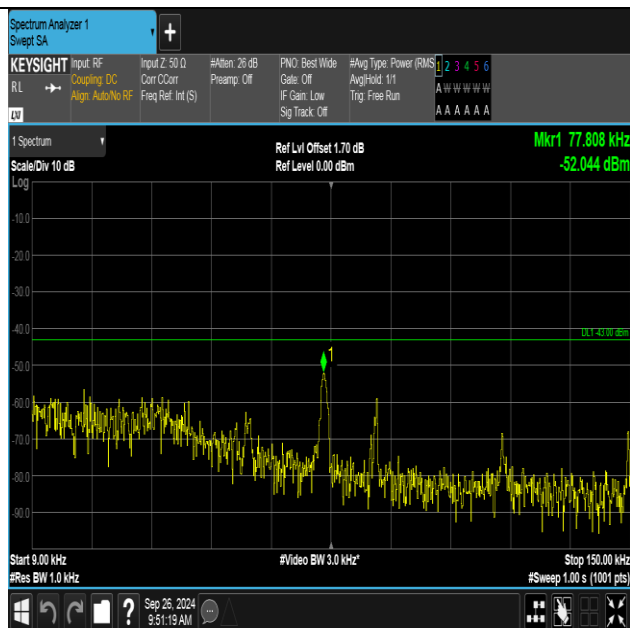
Band4-1312-4-0.009~0.15MHz-PASS
