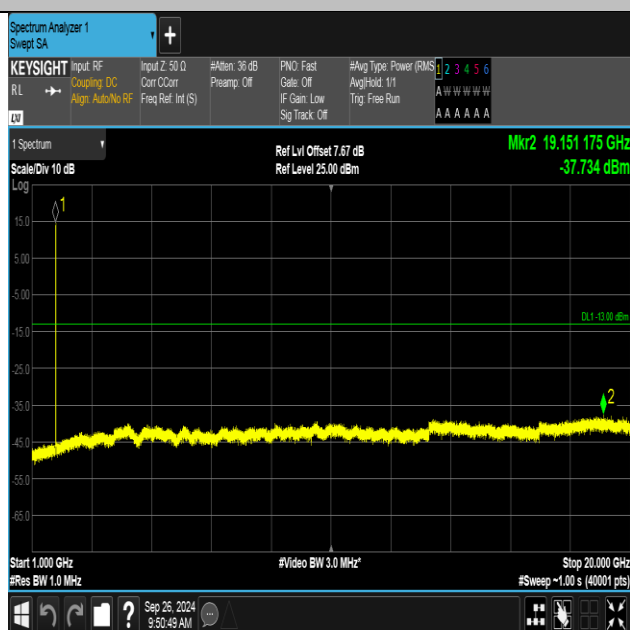
Band4-1513-3-1000~20000MHz-PASS
