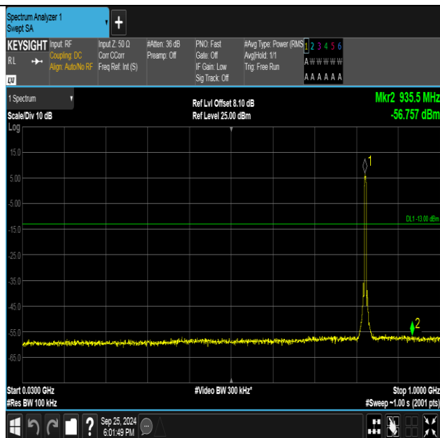
Band5-4132-1-30~1000MHz-PASS
