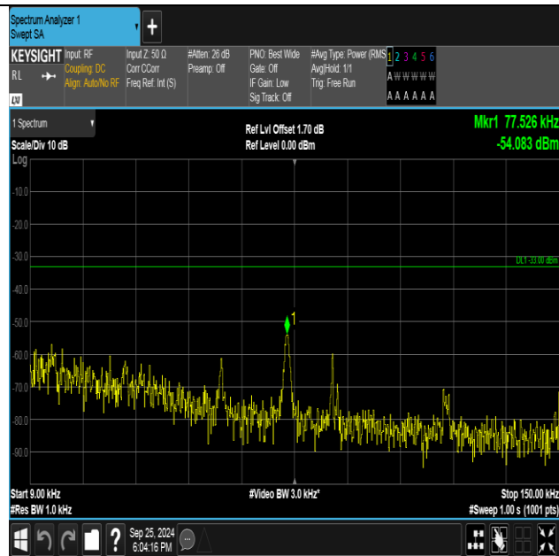
Band5-4182-2-0.009~0.15MHz-PASS
