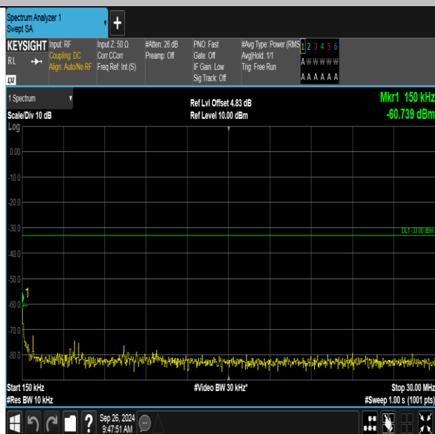
Band4-1413-2-0.15~30MHz-PASS
