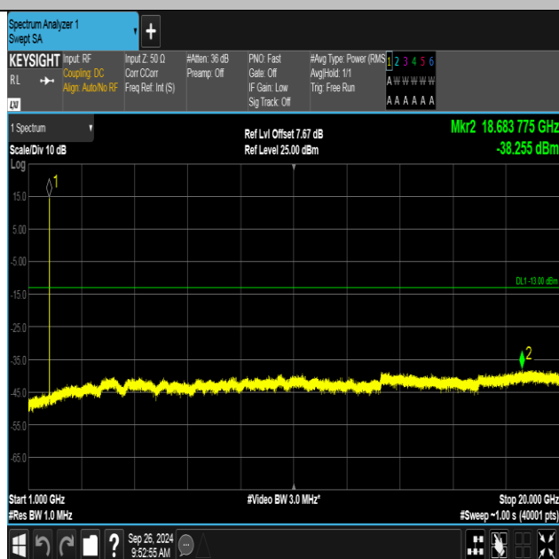
Band4-1513-4-1000~20000MHz-PASS
