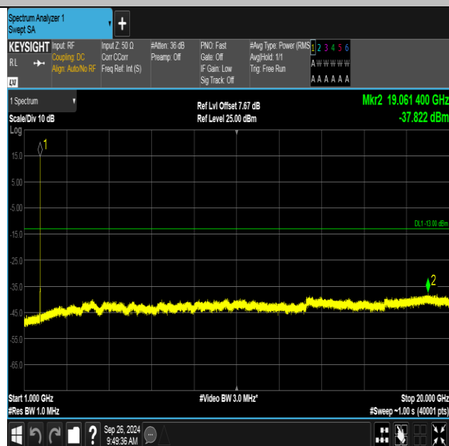
Band4-1312-3-1000~20000MHz-PASS
