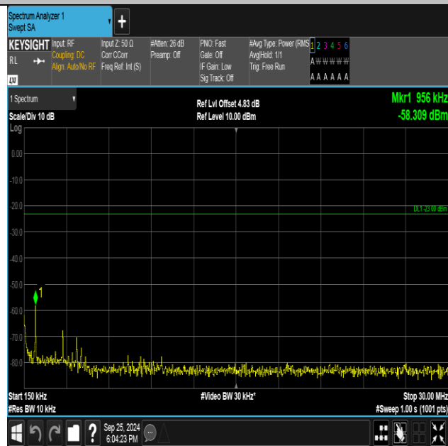
Band5-4182-2-0.15~30MHz-PASS
