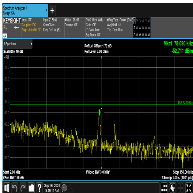
Band4-1312-3-0.009~0.15MHz-PASS
