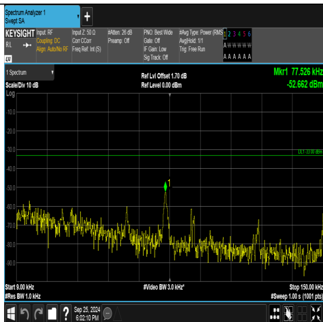
Band5-4182-1-0.009~0.15MHz-PASS
