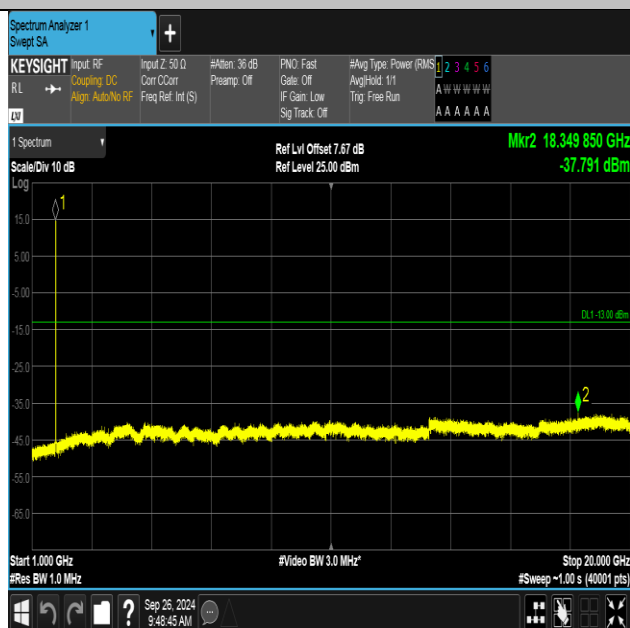
Band4-1513-2-1000~20000MHz-PASS
