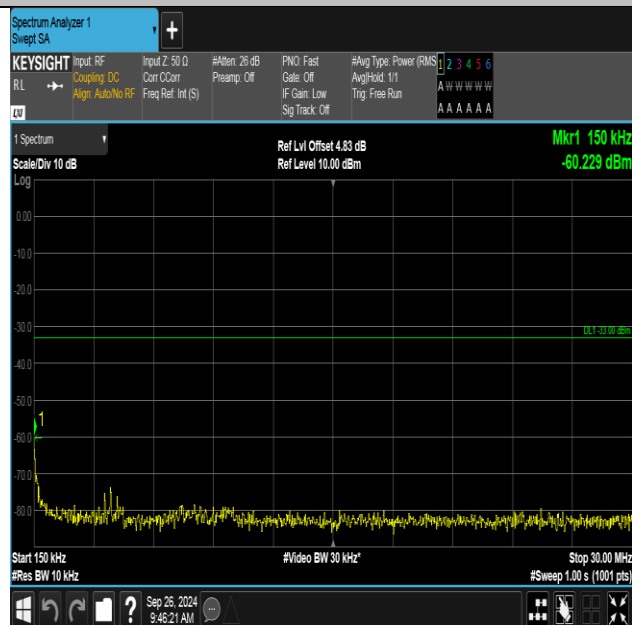
Band4-1513-1-0.15~30MHz-PASS
