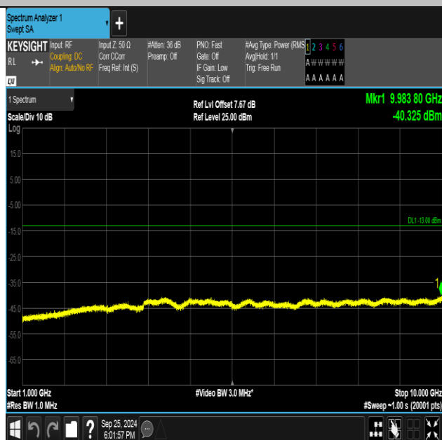
Band5-4132-1-1000~10000MHz-PASS
