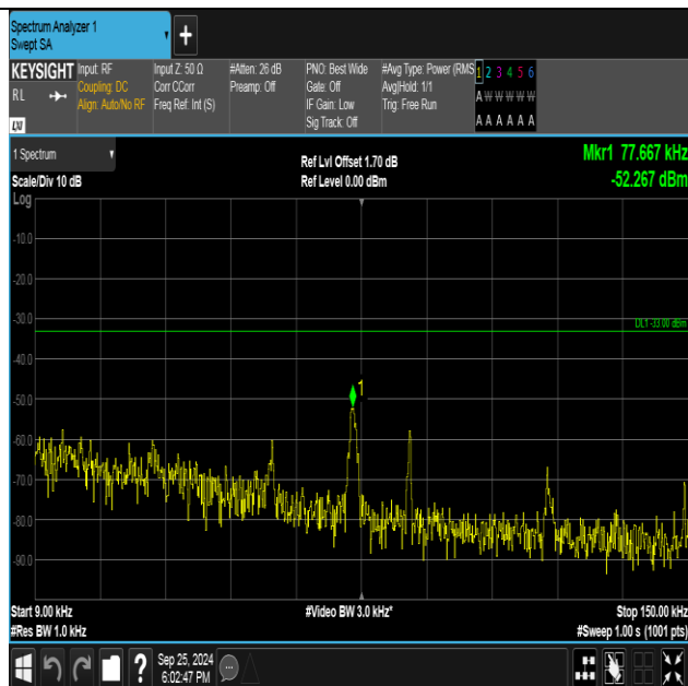
Band5-4233-1-0.009~0.15MHz-PASS
