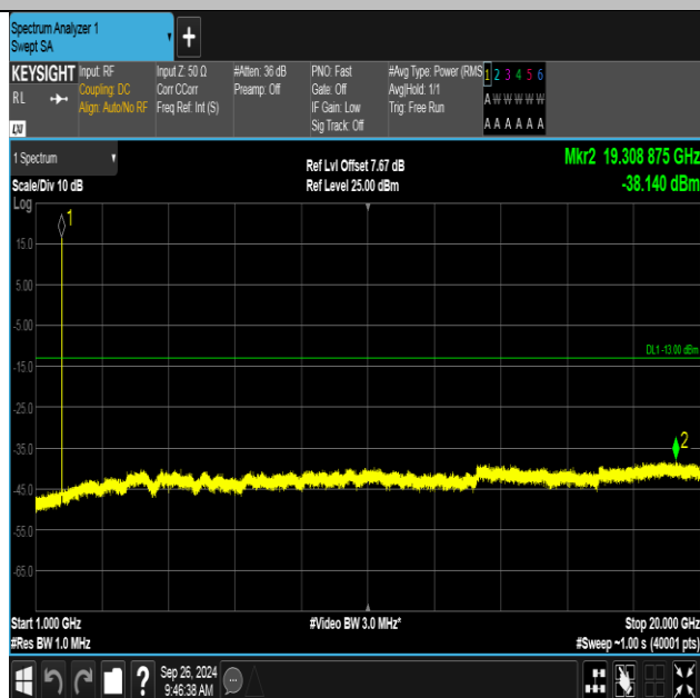
Band4-1513-1-1000~20000MHz-PASS
