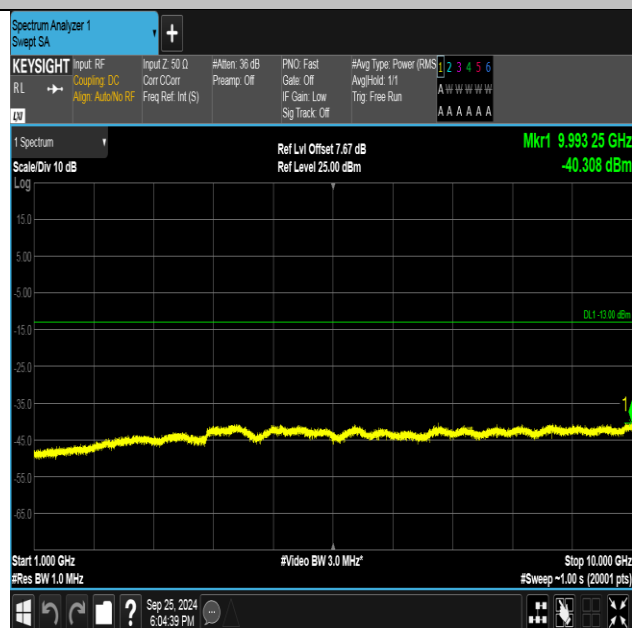
Band5-4182-2-1000~10000MHz-PASS
