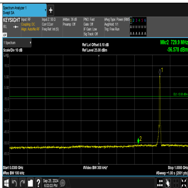
Band5-4233-1-30~1000MHz-PASS
