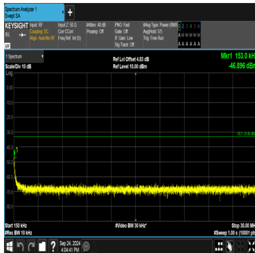
EGPRS1900-661-2-0.15~30MHz-PASS
