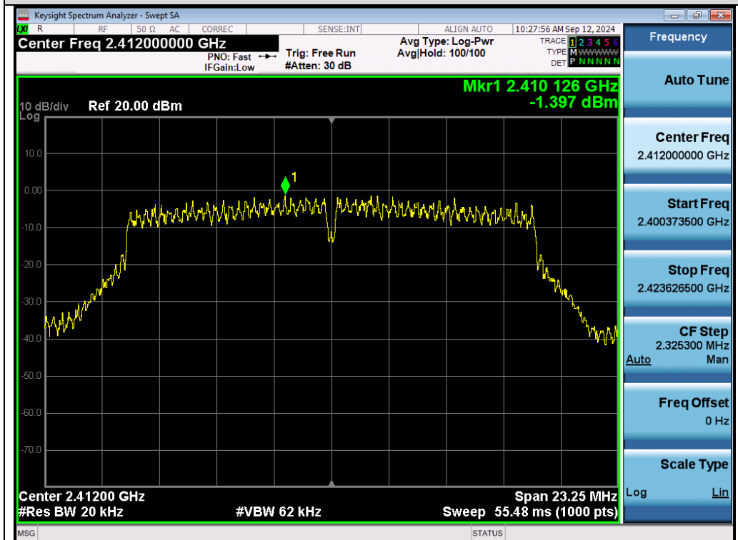
Test_Graph_802.11g_ANT1_2412_6Mbps_PSD
