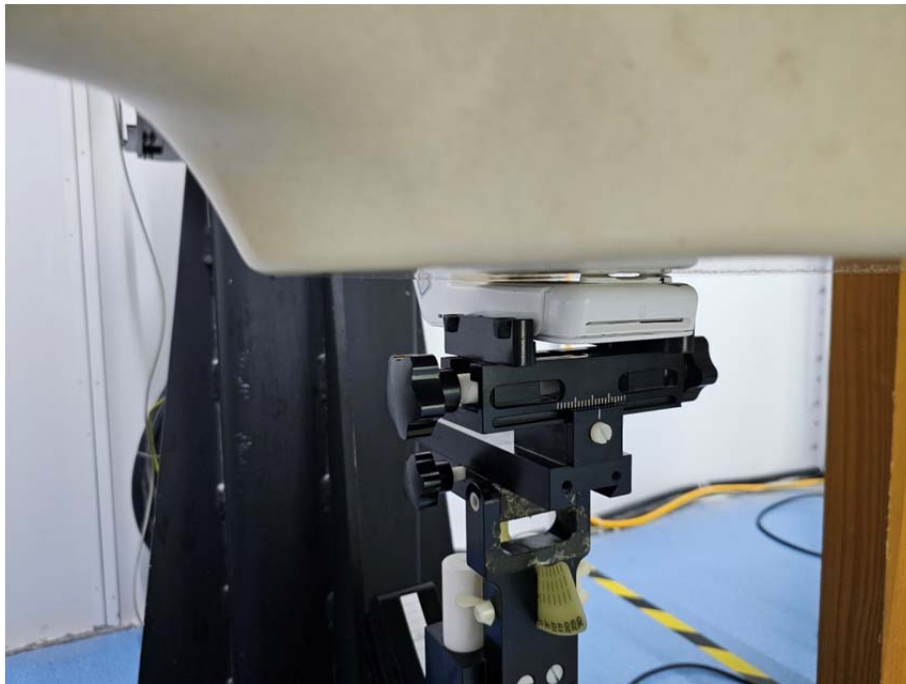
Handheld Back Setup Photo For WWAN (0mm)
