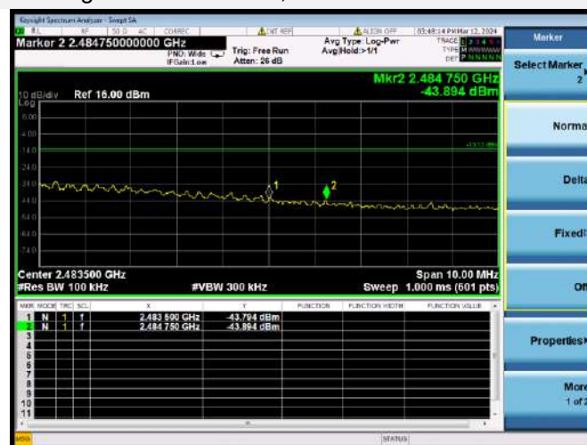
802.11g HIGH CHANNEL, BAND EDGE
