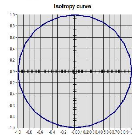
Isotropy: +/- 0.18% (+/-0.01dB)
