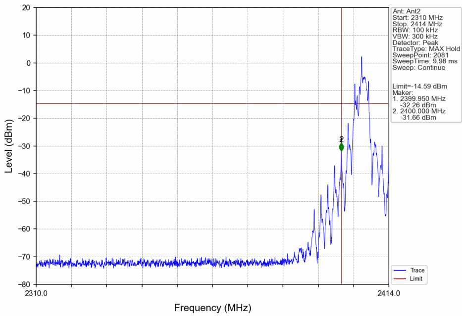
GFSK_LCH_2406MHz_Ant2_NTNV
