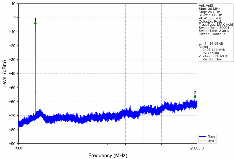
GFSK_LCH_2406MHz_Ant2_NTNV
