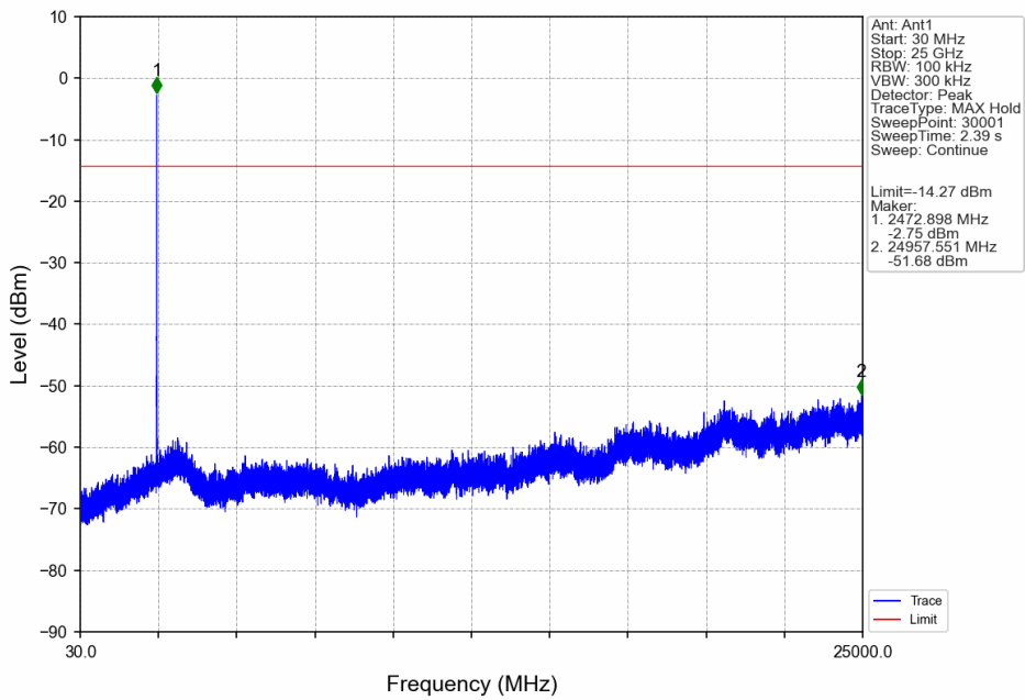
GFSK_HCH_2472MHz_Ant1_NTNV
