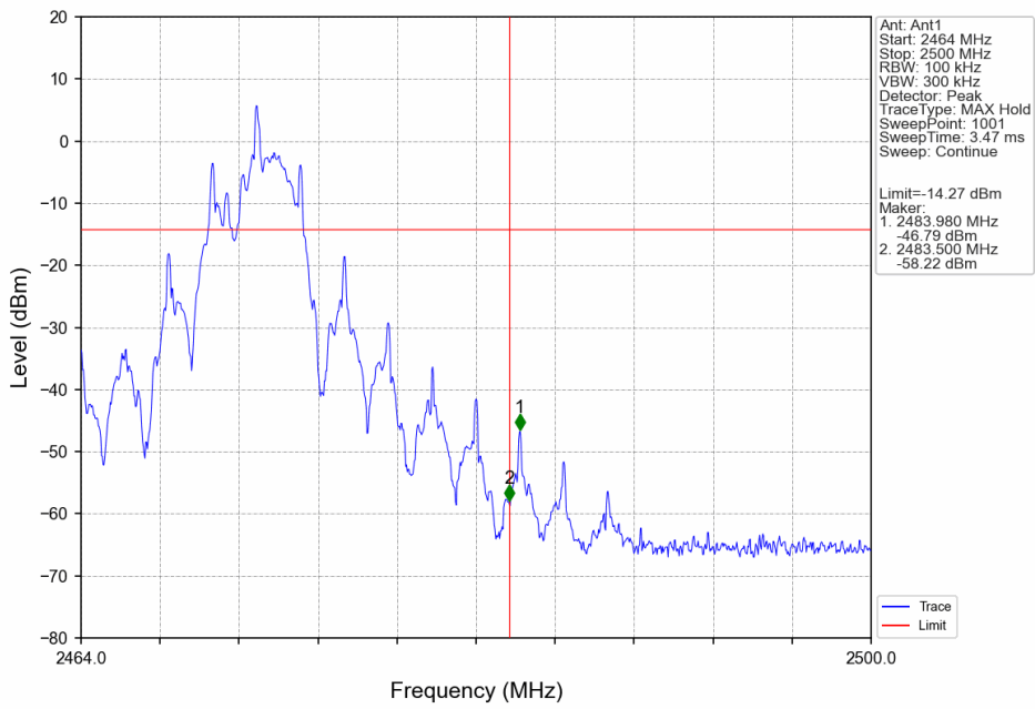
GFSK_HCH_2472MHz_Ant1_NTNV
