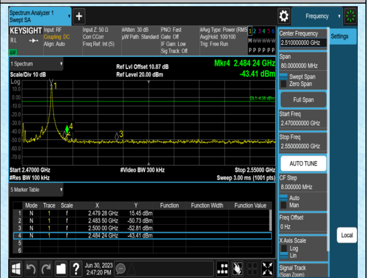
TX-Ant2-2479.4
