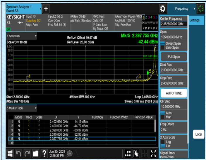
TX-Ant1-2402.6
