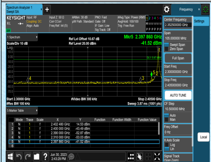
TX-Ant2-2402.6
