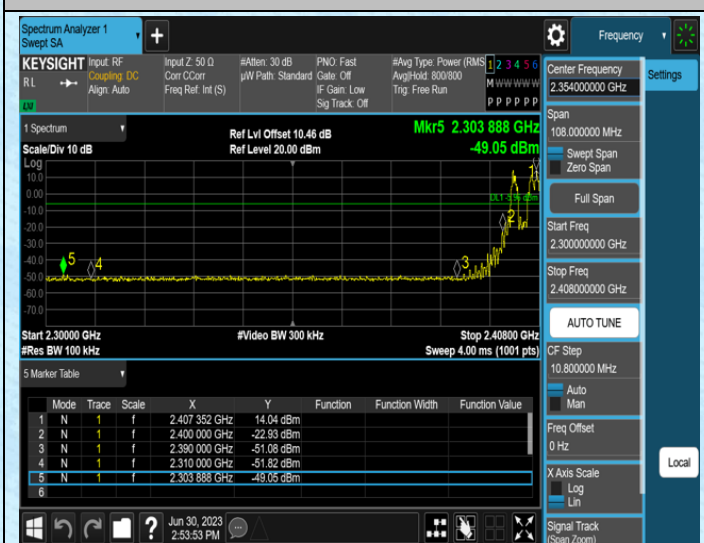
TX-Ant1-Hop_2402.6
