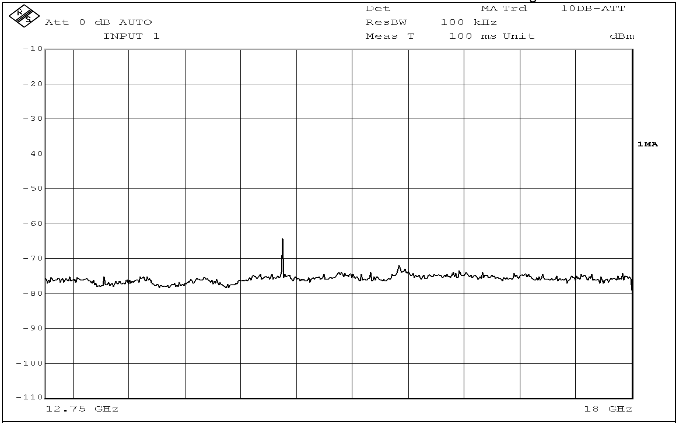
Fig A3 High Channel Conducted Spurious Emissions 12.75GHz -18GHz
