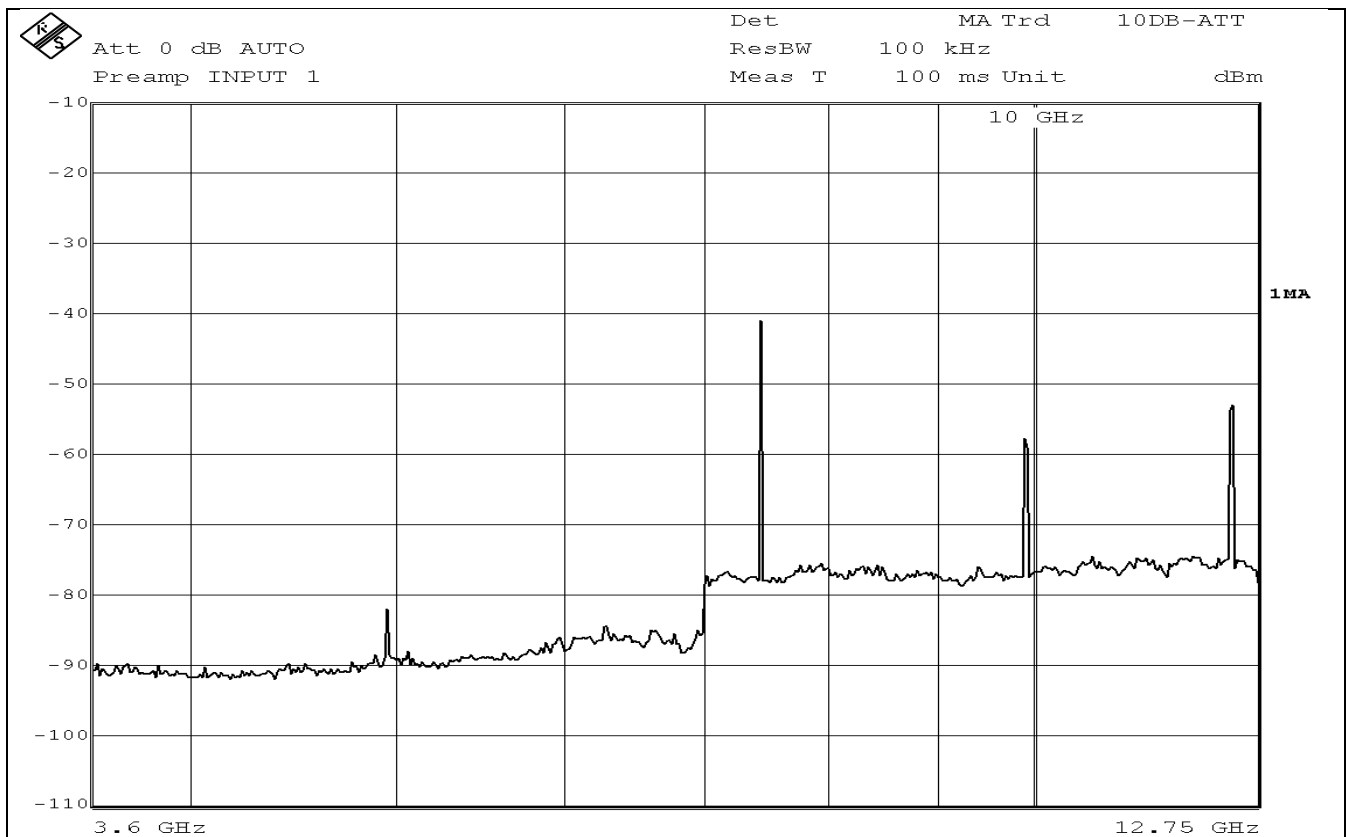
Fig A2 High Channel Conducted Spurious Emissions 3.6GHz-12.75GHz
