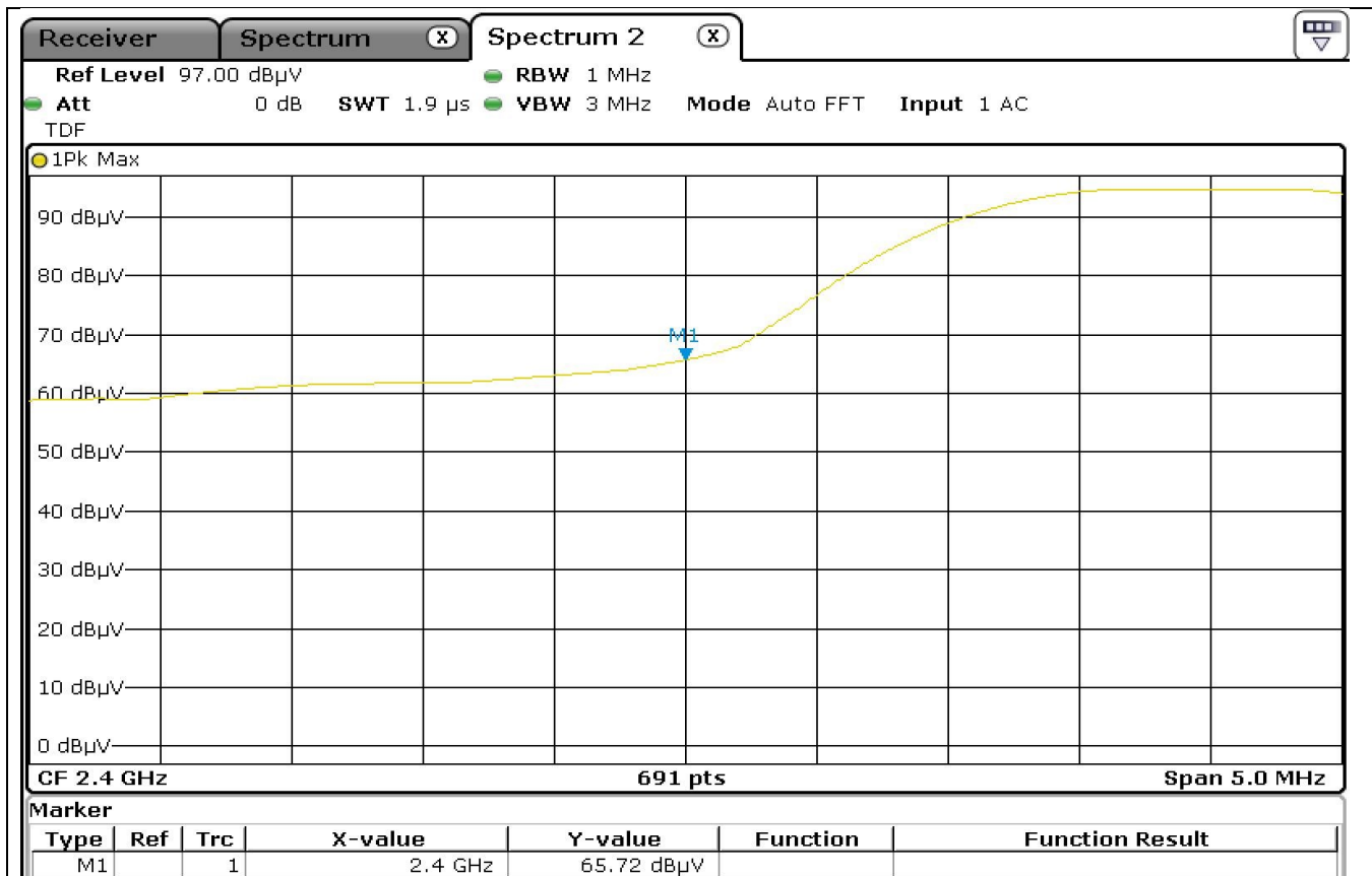
Fig B2 Low Channel Band Edge Vertical peak at 3 metres
