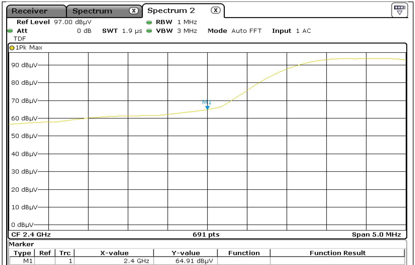
Fig B1 Low Channel Band Edge Vertical peak at 3 metres
