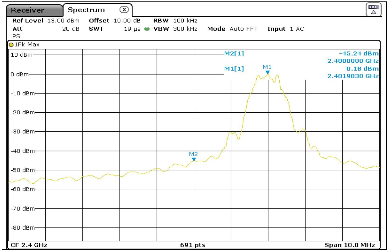
Fig A6 Lower Band Edge Low Channel Conducted
