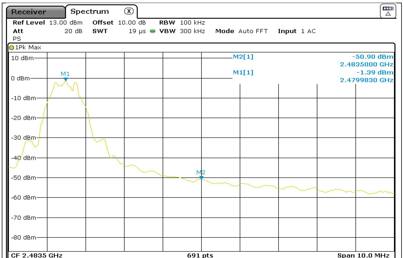
Fig A7 Upper band edge High Channel Conducted
