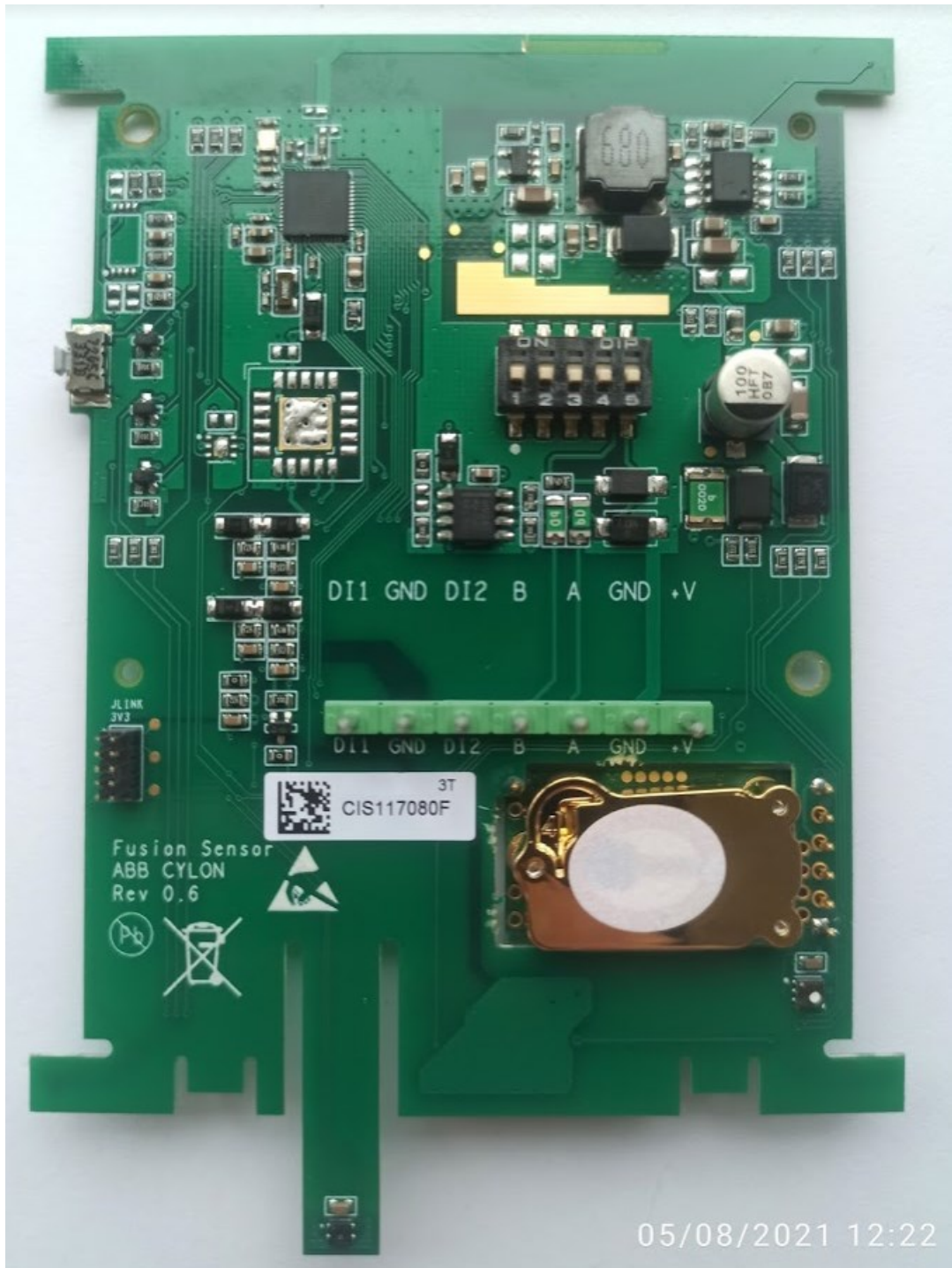
PCBA back side
