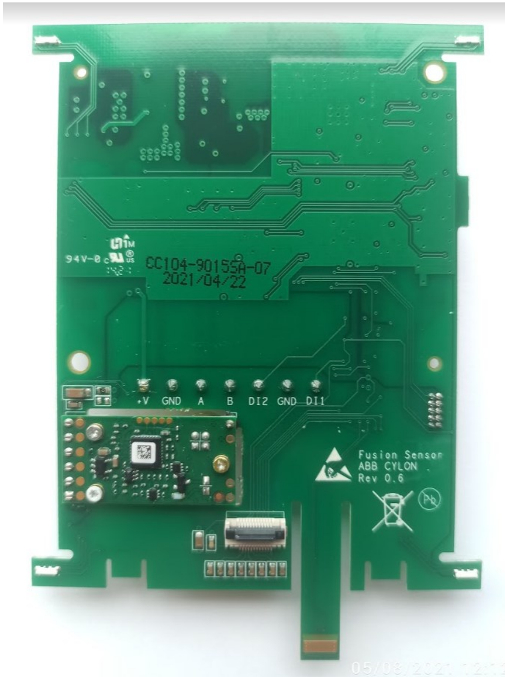
PCBA front without LCD
