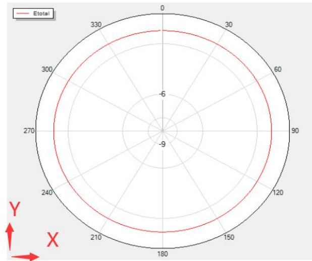
Theta=0 Freq=2466MHz
