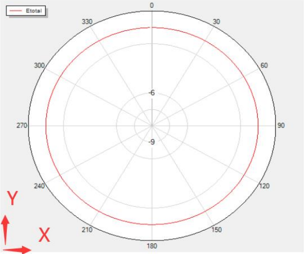
Theta=0 Freq=2472MHz
