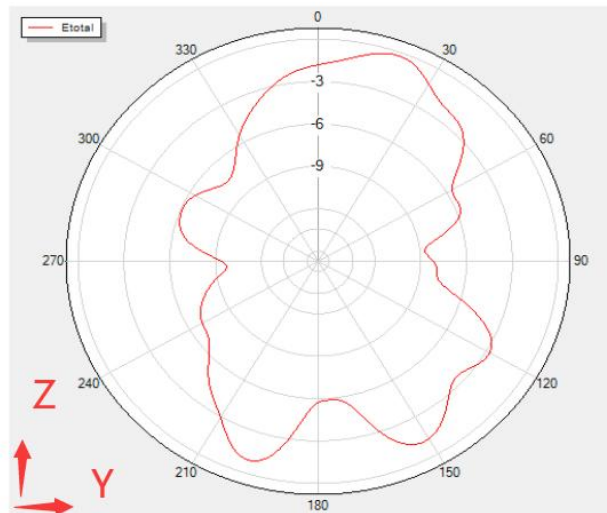
Phi=90 Freq=2446MHz
