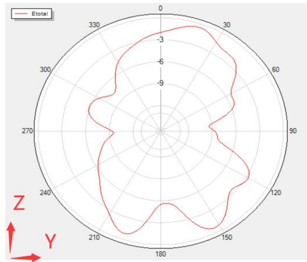
Phi=90 Freq=2434MHz
