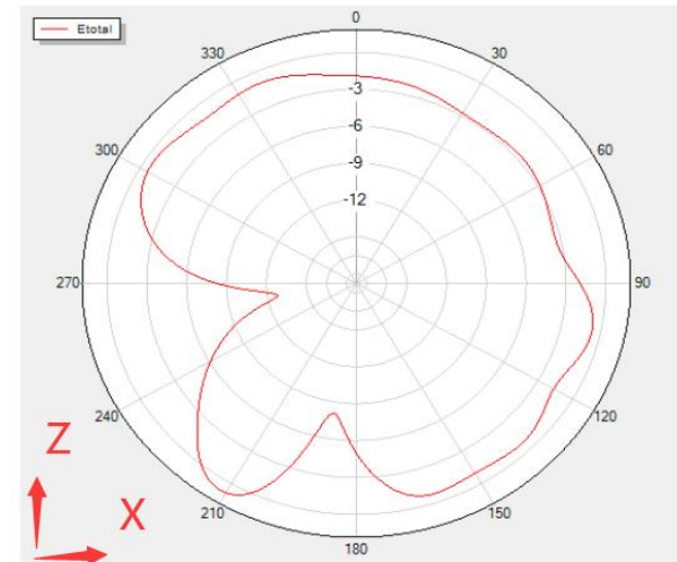
Phi=0 Freq=2416MHz
