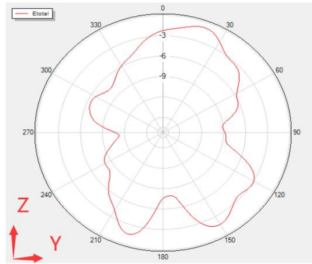
Phi=90 Freq=2466MHz
