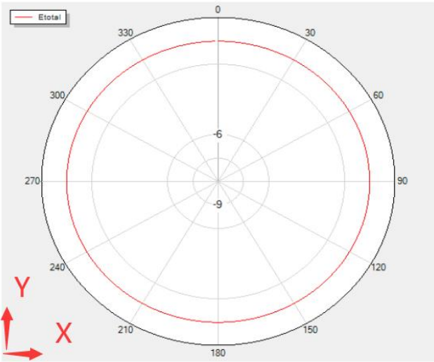
Theta=0 Freq=2454MHz
