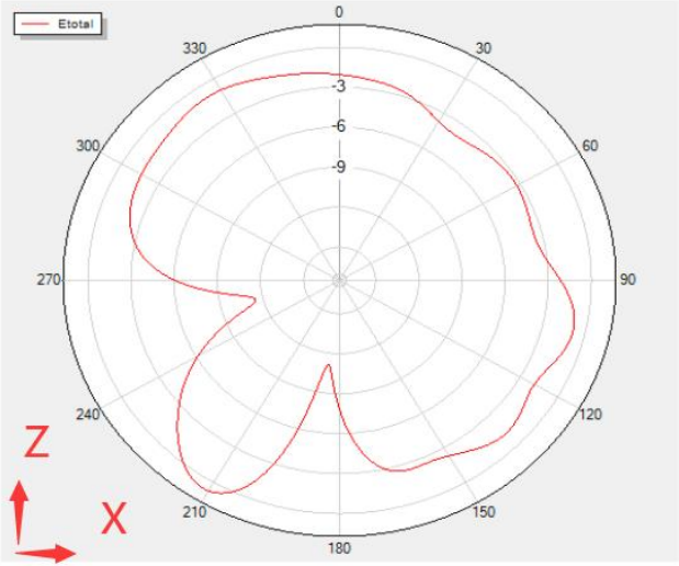
Phi=0 Freq=2472MHz
