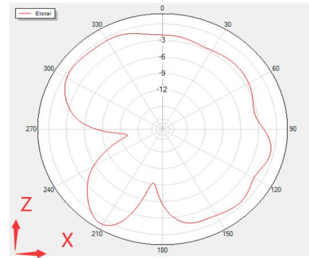
Phi=0 Freq=2434MHz
