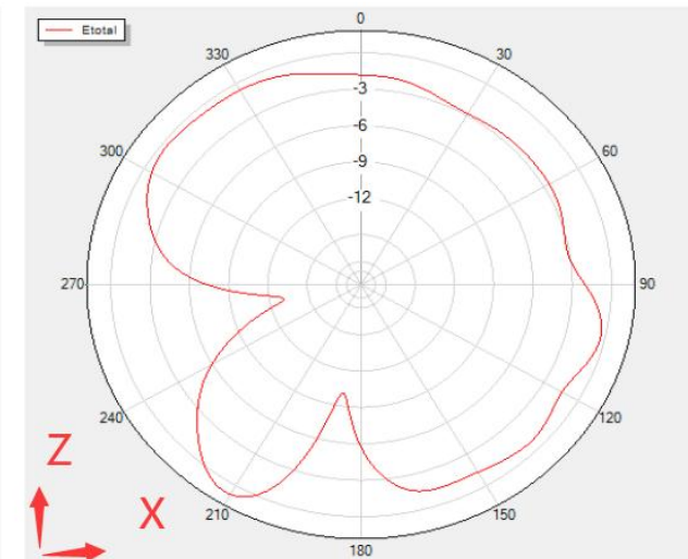
Phi=0 Freq=2446MHz
