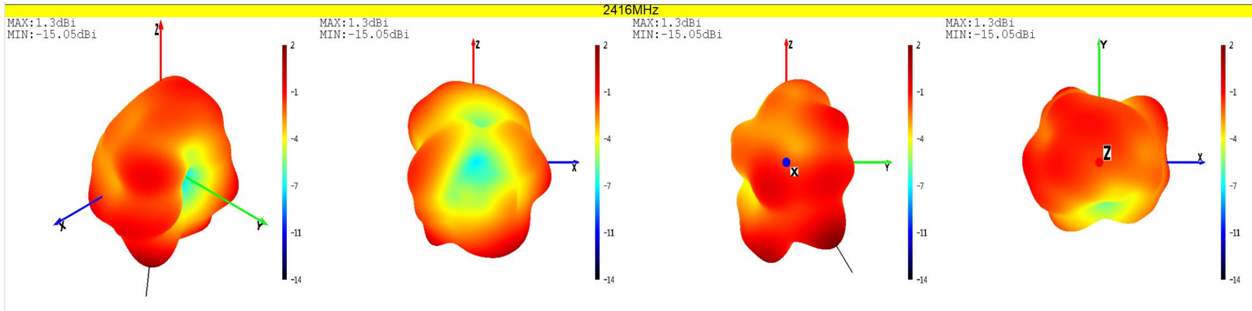
Theta=0 Freq=2416MHz
