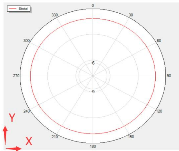
Theta=0 Freq=2410MHz
