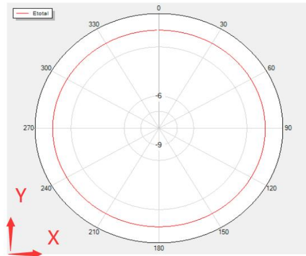
Theta=0 Freq=2434MHz
