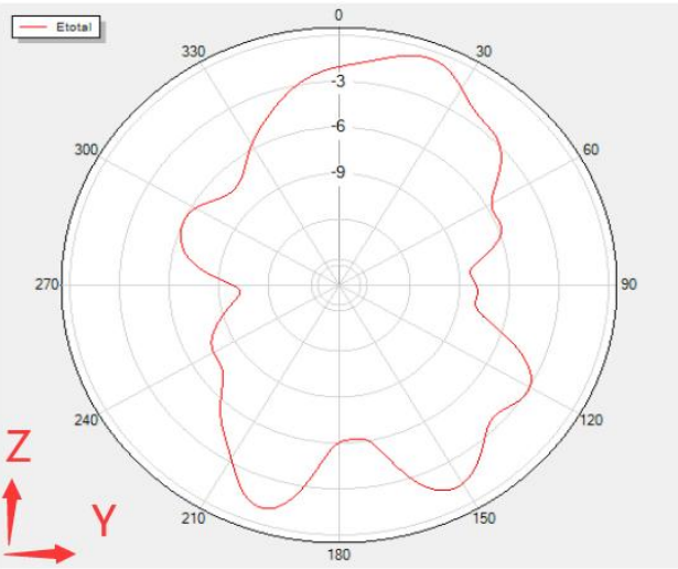
Phi=90 Freq=2454MHz
