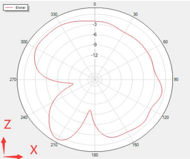
Phi=0 Freq=2454MHz
