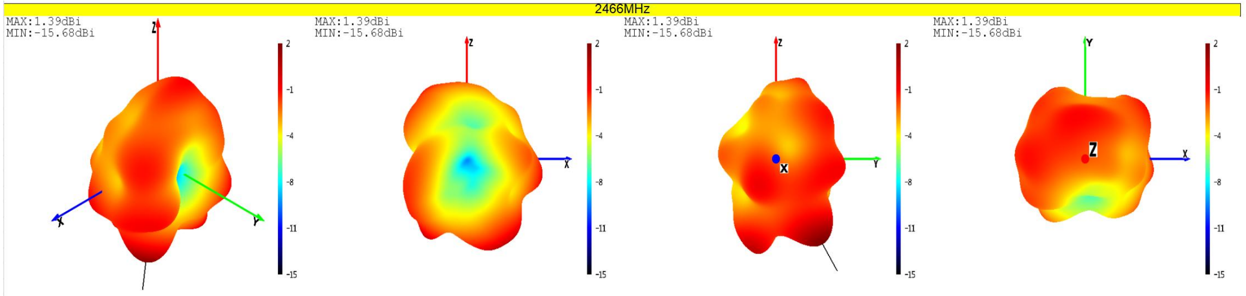
Theta=0 Freq=2466MHz
