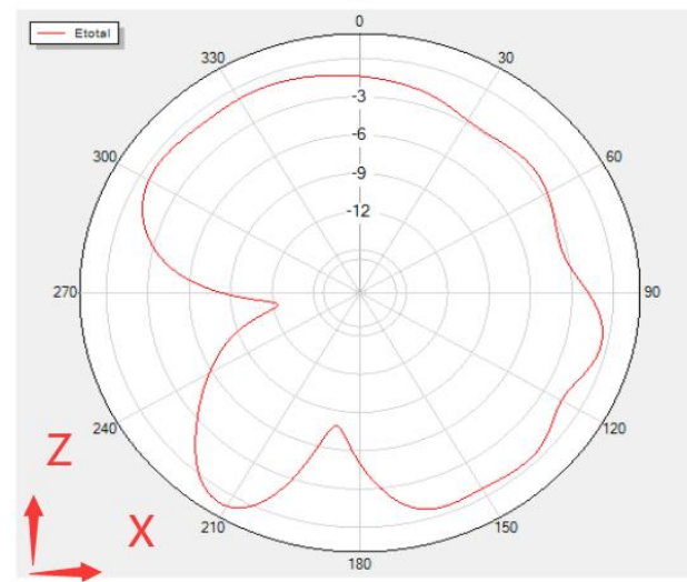
Phi=0 Freq=2410MHz
