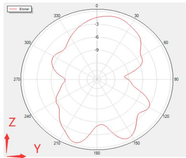
Phi=90 Freq=2410MHz
