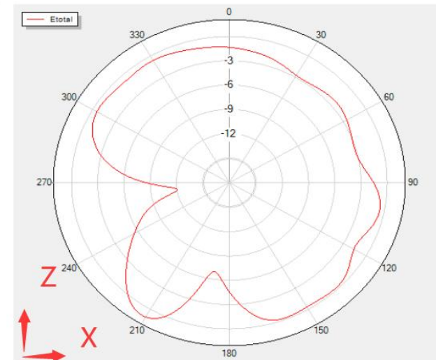
Phi=0 Freq=2402MHz
