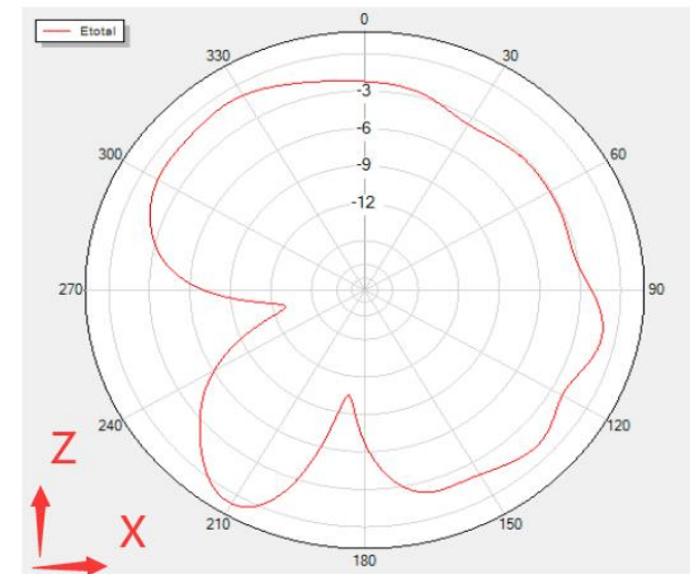
Phi=0 Freq=2460MHz
