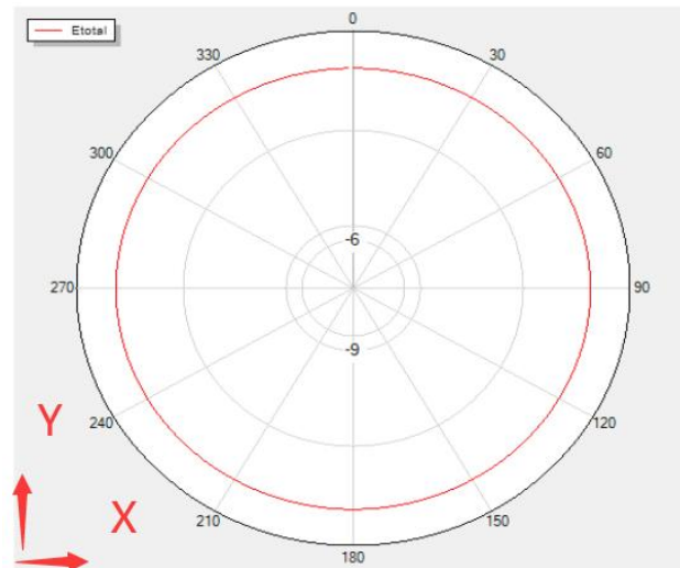
Theta=0 Freq=2402MHz
