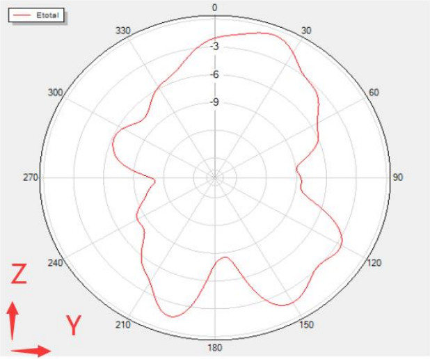
Phi=90 Freq=2472MHz
