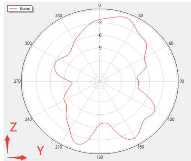
Phi=90 Freq=2460MHz
