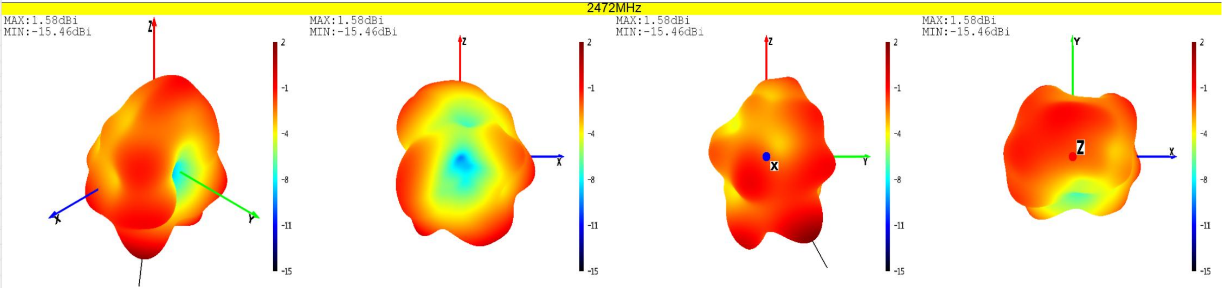
Theta=0 Freq=2472MHz
