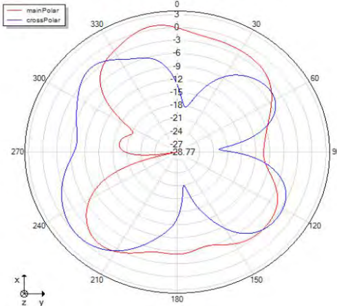
Theta=90 freq=2434MHz
