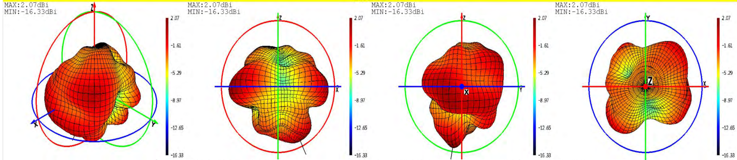
Phi=0 freq=2466MHz
