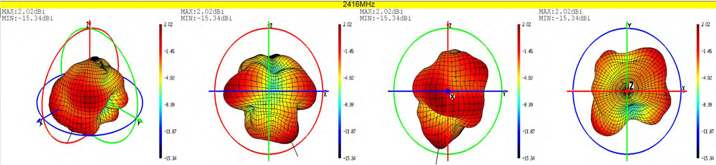
Phi=0 freq=2416MHz
