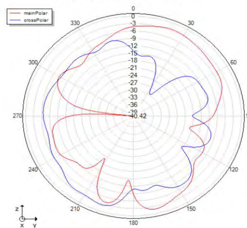
Phi=90 freq=2466MHz
