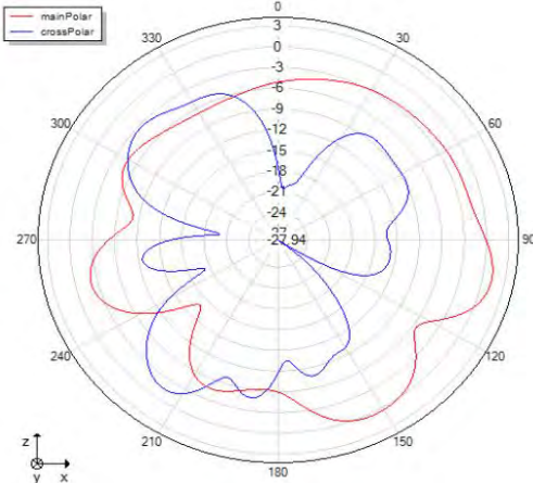
Phi=0 freq=2434MHz
