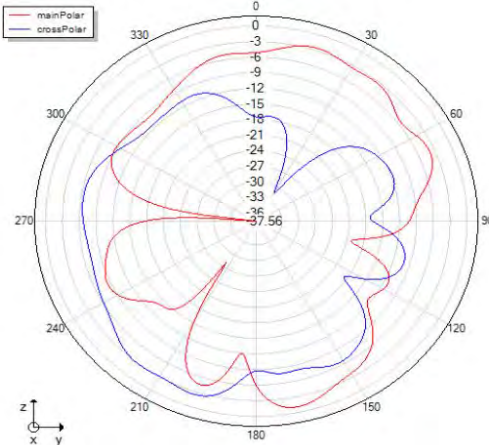
Phi=90 freq=2434MHz
