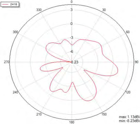
Phi=0 freq=2416MHz
