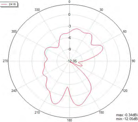
Phi=90 freq=2416MHz
