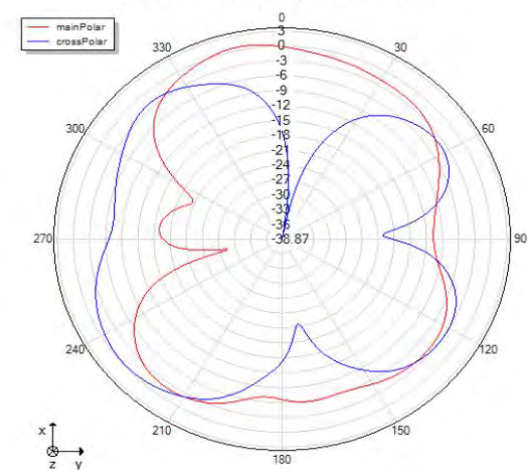
Theta=90 freq=2466MHz
