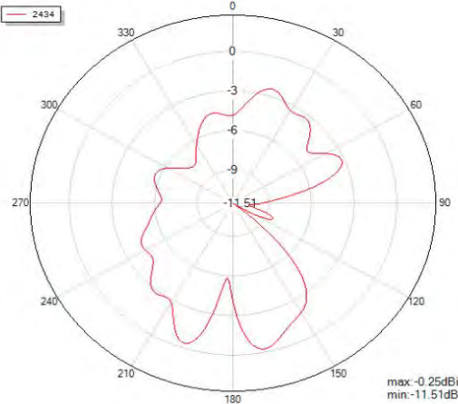
Phi=90 freq=2434MHz
