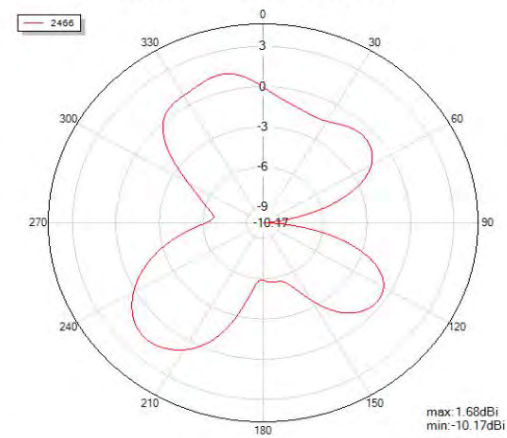
Theta=90 freq=2466MHz
