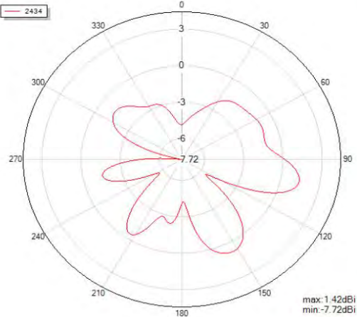
Phi=0 freq=2434MHz
