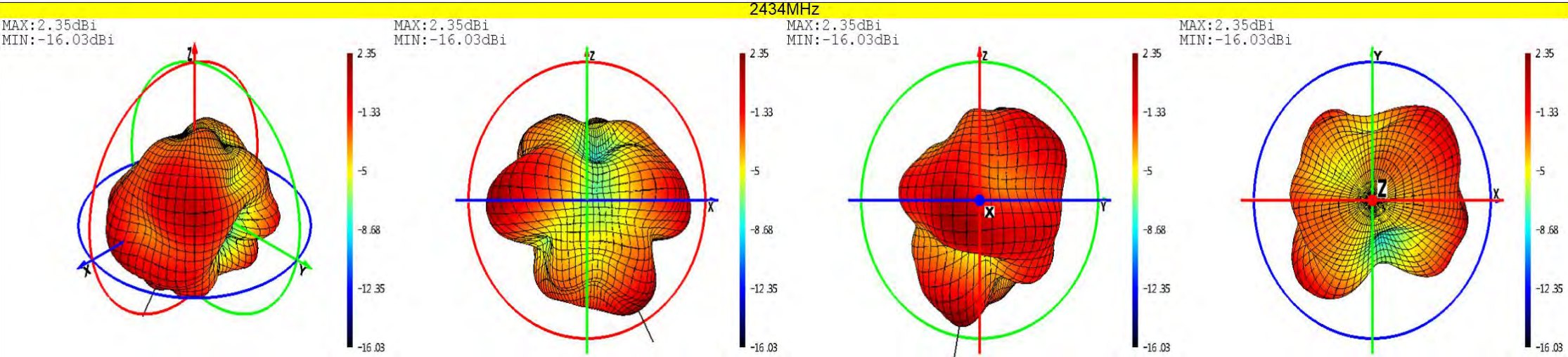
Phi=0 freq=2434MHz
