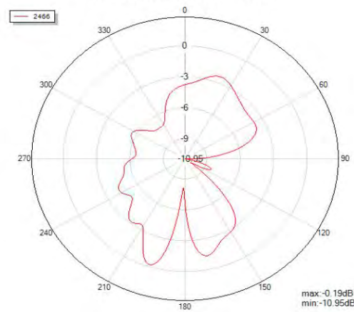
Phi=90 freq=2466MHz
