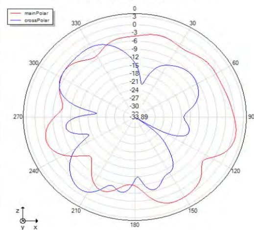
Phi=0 freq=2466MHz
