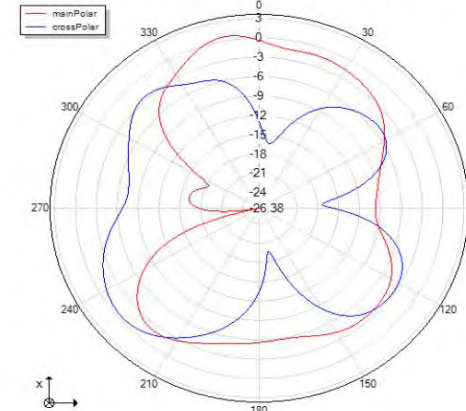
Theta=90 freq=2416MHz
