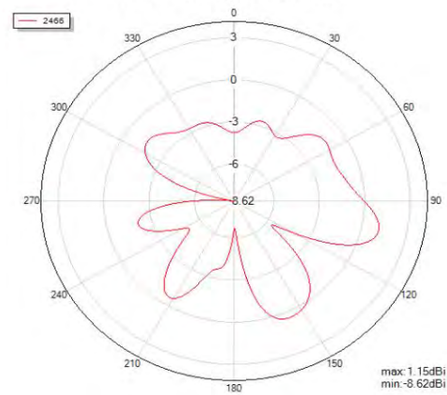
Phi=0 freq=2466MHz
