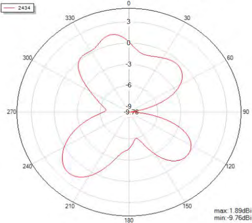
Theta=90 freq=2434MHz
