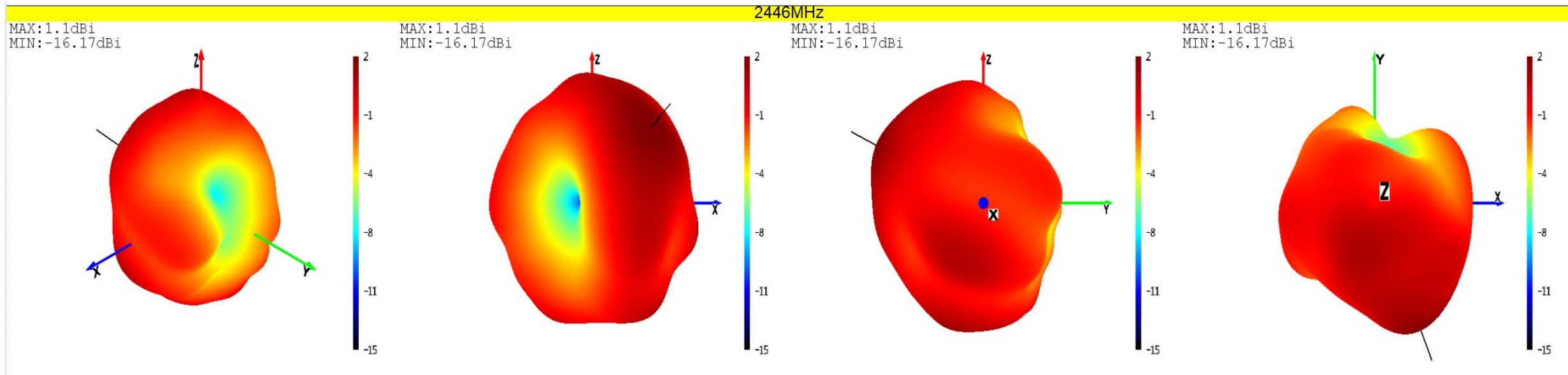
Theta=0 Freq=2446MHz
