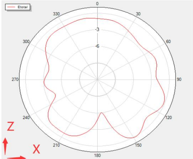
Phi=0 Freq=2440MHz
