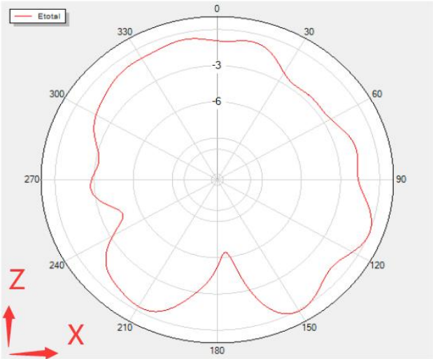
Phi=0 Freq=2460MHz
