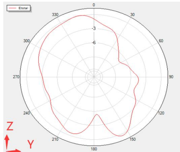
Phi=90 Freq=2428MHz
