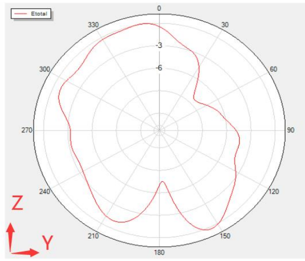
Phi=90 Freq=2480MHz
