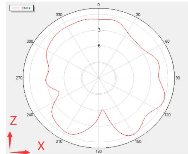
Phi=0 Freq=2454MHz
