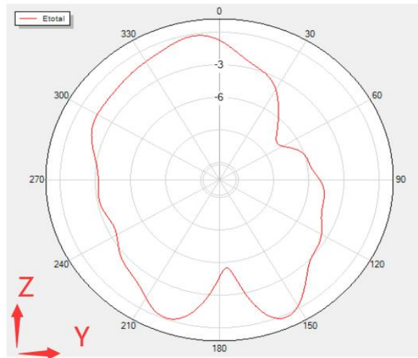
Phi=90 Freq=2416MHz
