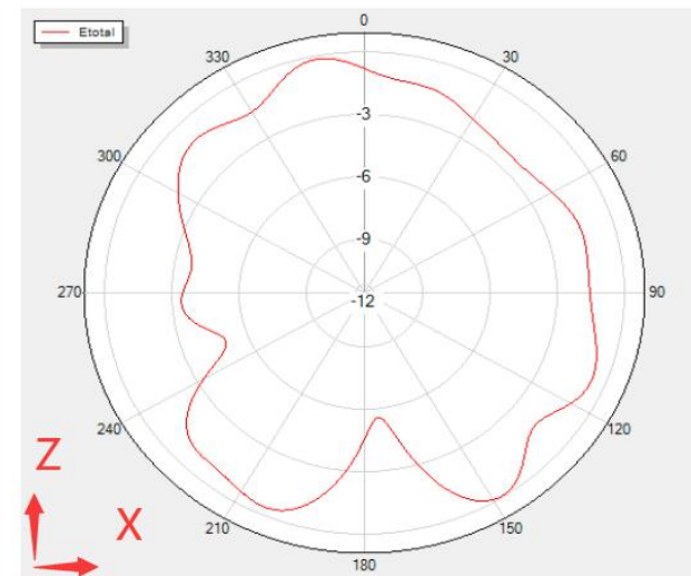
Phi=0 Freq=2422MHz
