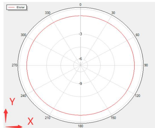
Theta=0 Freq=2446MHz
