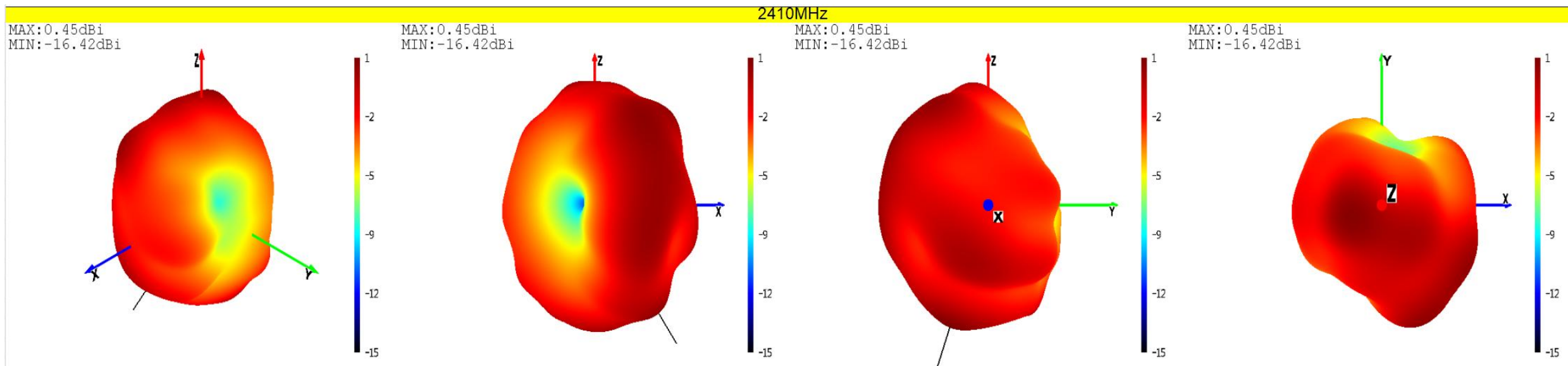
Theta=0 Freq=2410MHz
