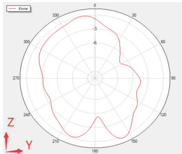
Phi=90 Freq=2422MHz
