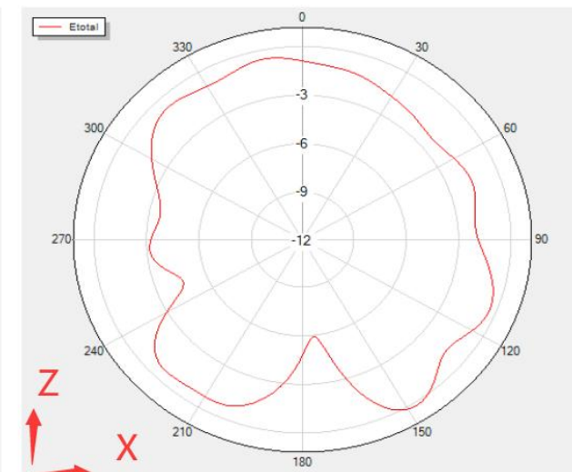
Phi=0 Freq=2434MHz
