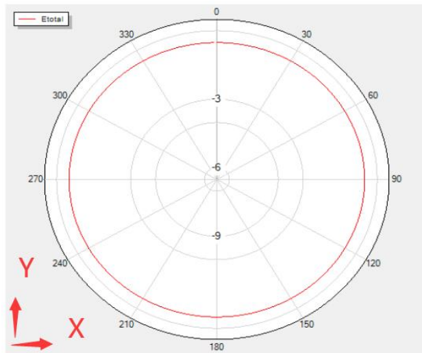
Theta=0 Freq=2410MHz
