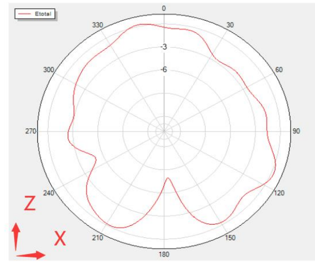
Phi=0 Freq=2480MHz
