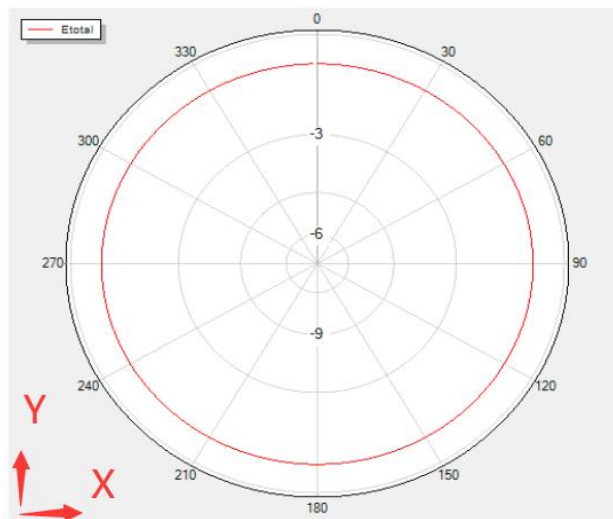
Theta=0 Freq=2434MHz
