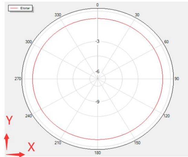
Theta=0 Freq=2416MHz
