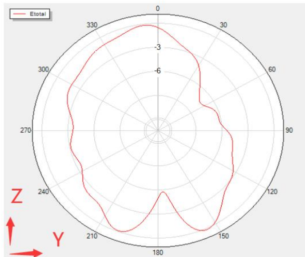
Phi=90 Freq=2410MHz
