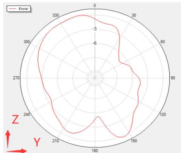
Phi=90 Freq=2446MHz
