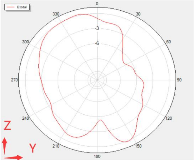
Phi=90 Freq=2440MHz
