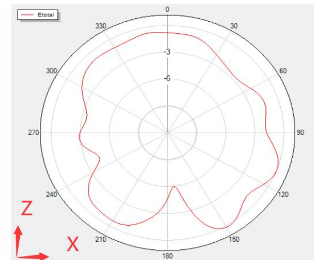
Phi=0 Freq=2446MHz
