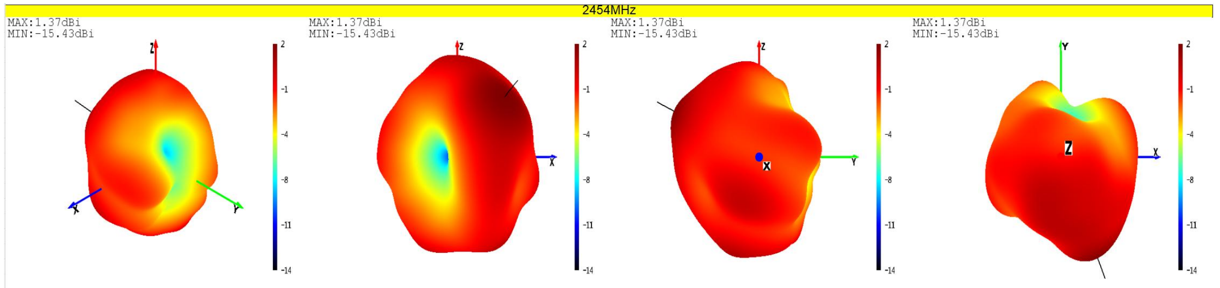
Theta=0 Freq=2454MHz
