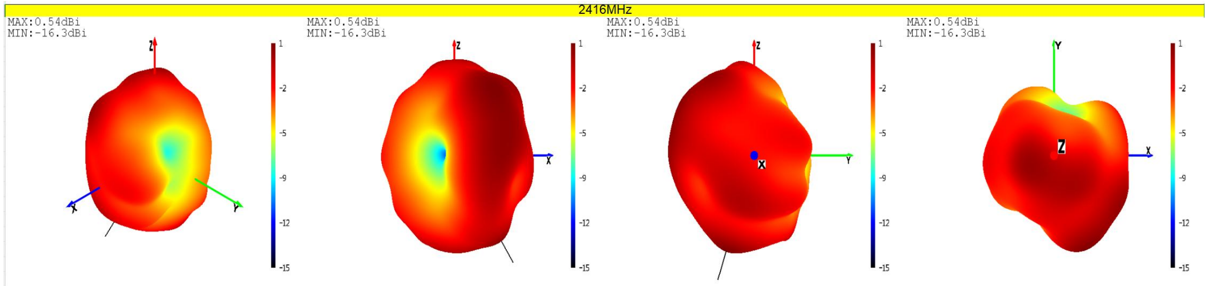
Theta=0 Freq=2416MHz
