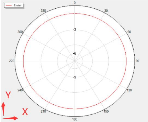
Theta=0 Freq=2440MHz
