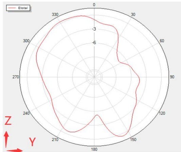
Phi=90 Freq=2454MHz
