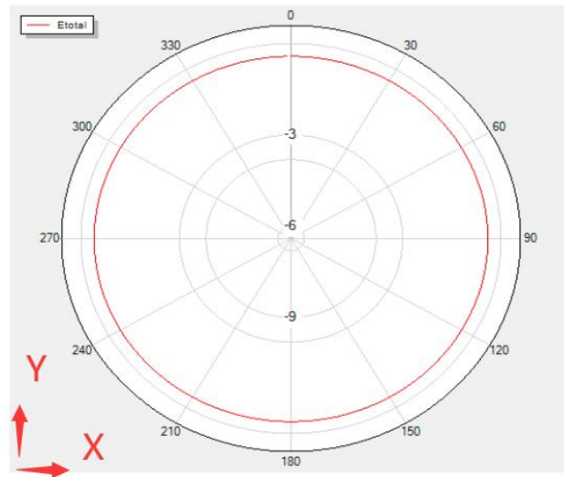
Theta=0 Freq=2480MHz
