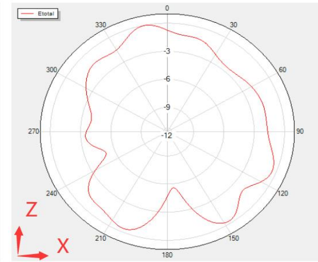
Phi=0 Freq=2416MHz
