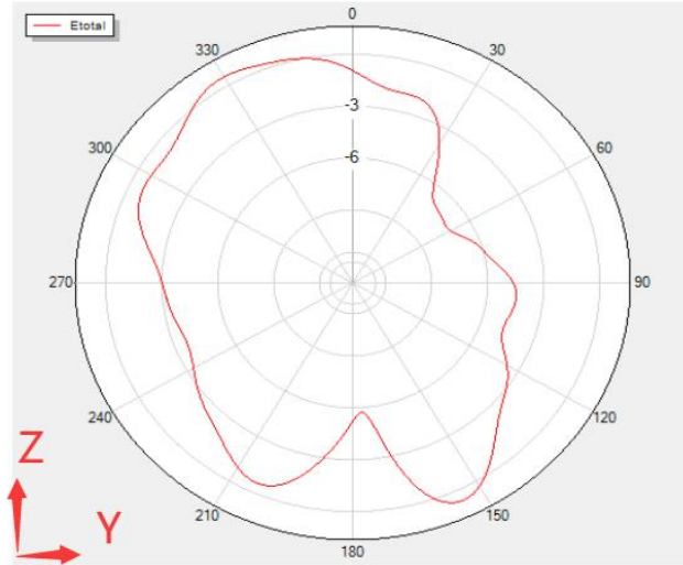
Phi=90 Freq=2460MHz
