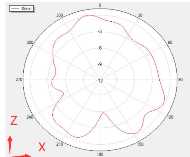
Phi=0 Freq=2410MHz
