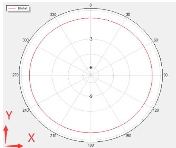
Theta=0 Freq=2422MHz
