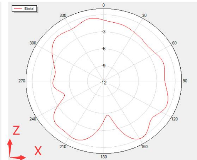
Phi=0 Freq=2428MHz
