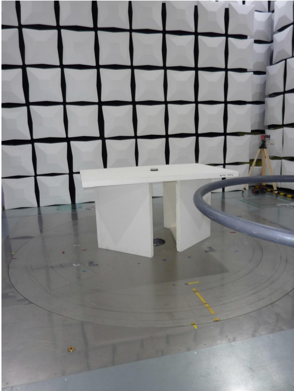
Test setup semi anechoic chamber spurious emissions from 9 kHz to 30 MHz
