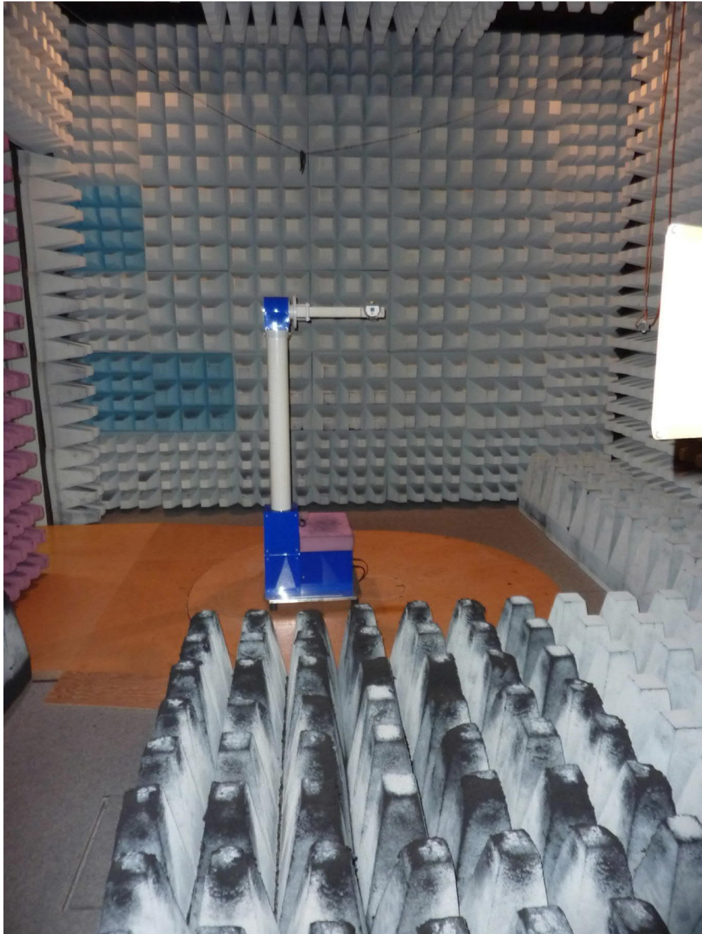
Test setup fully anechoic chamber spurious emissions below 10.6 GHz with 3 m distance
