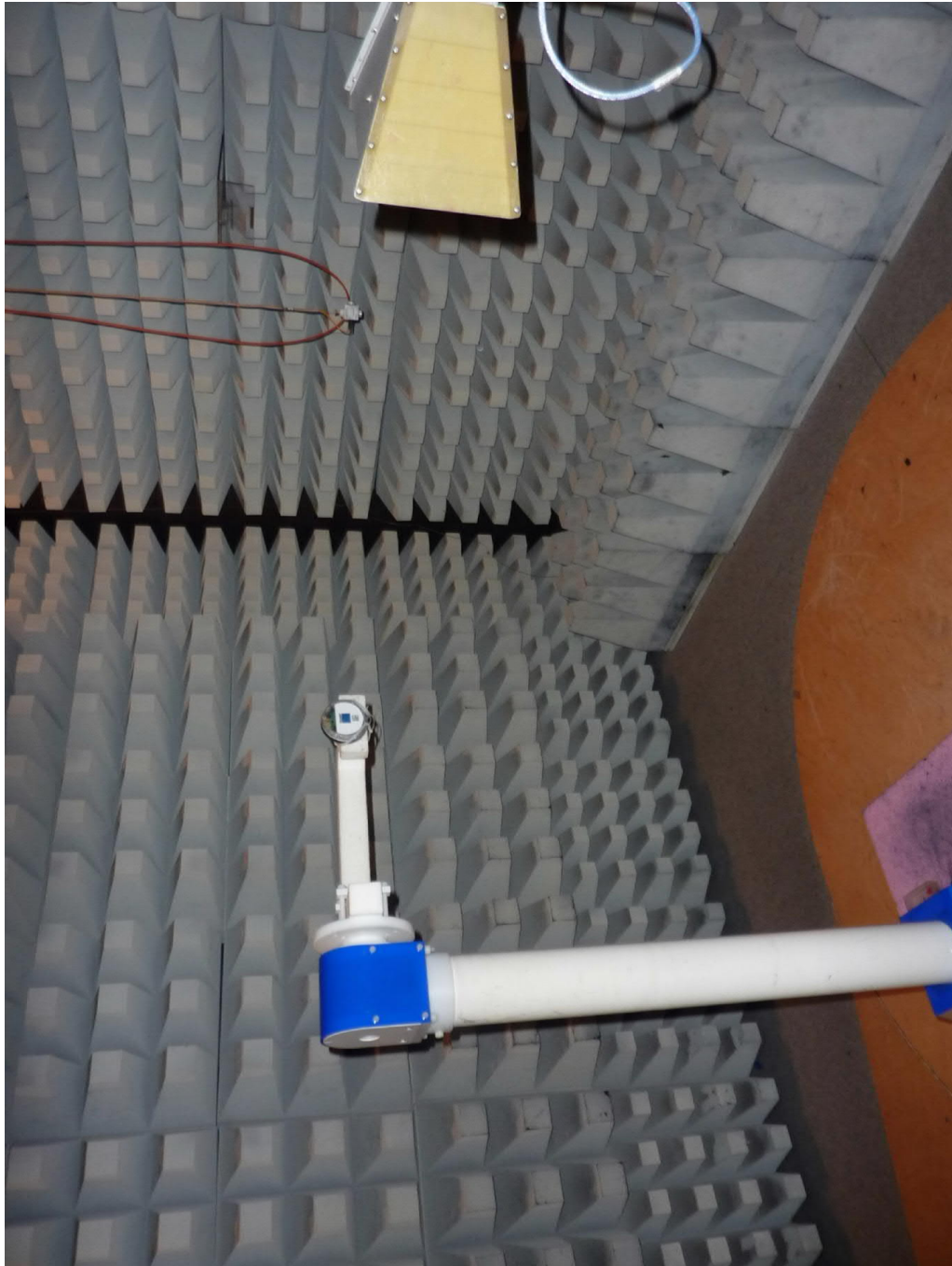
Test setup fully anechoic chamber spurious emissions below 10.6 GHz with 1 m distance
