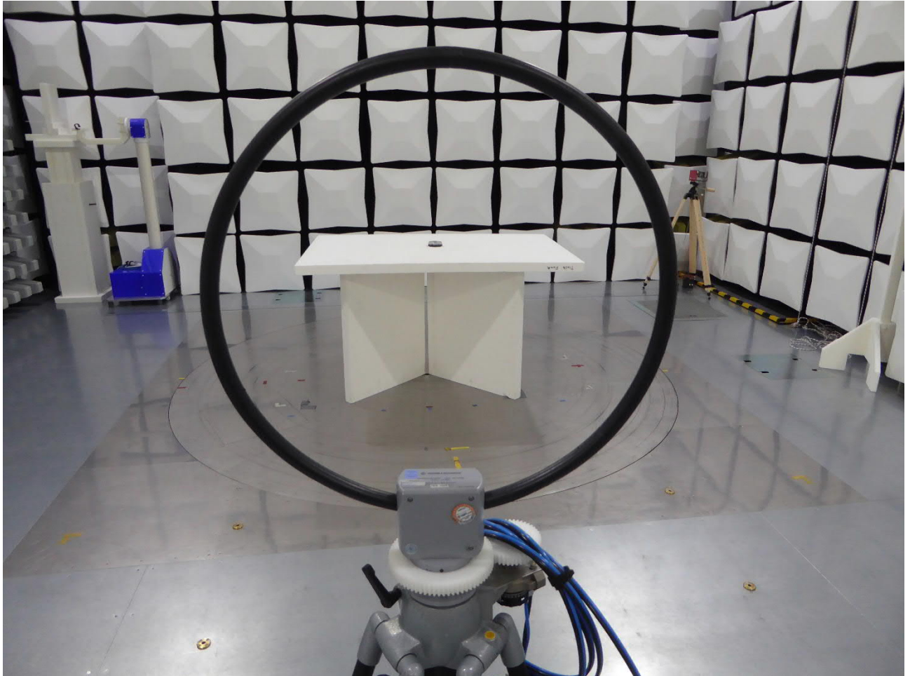
Test setup semi anechoic chamber 9 kHz – 30 MHz (Pos 1)
