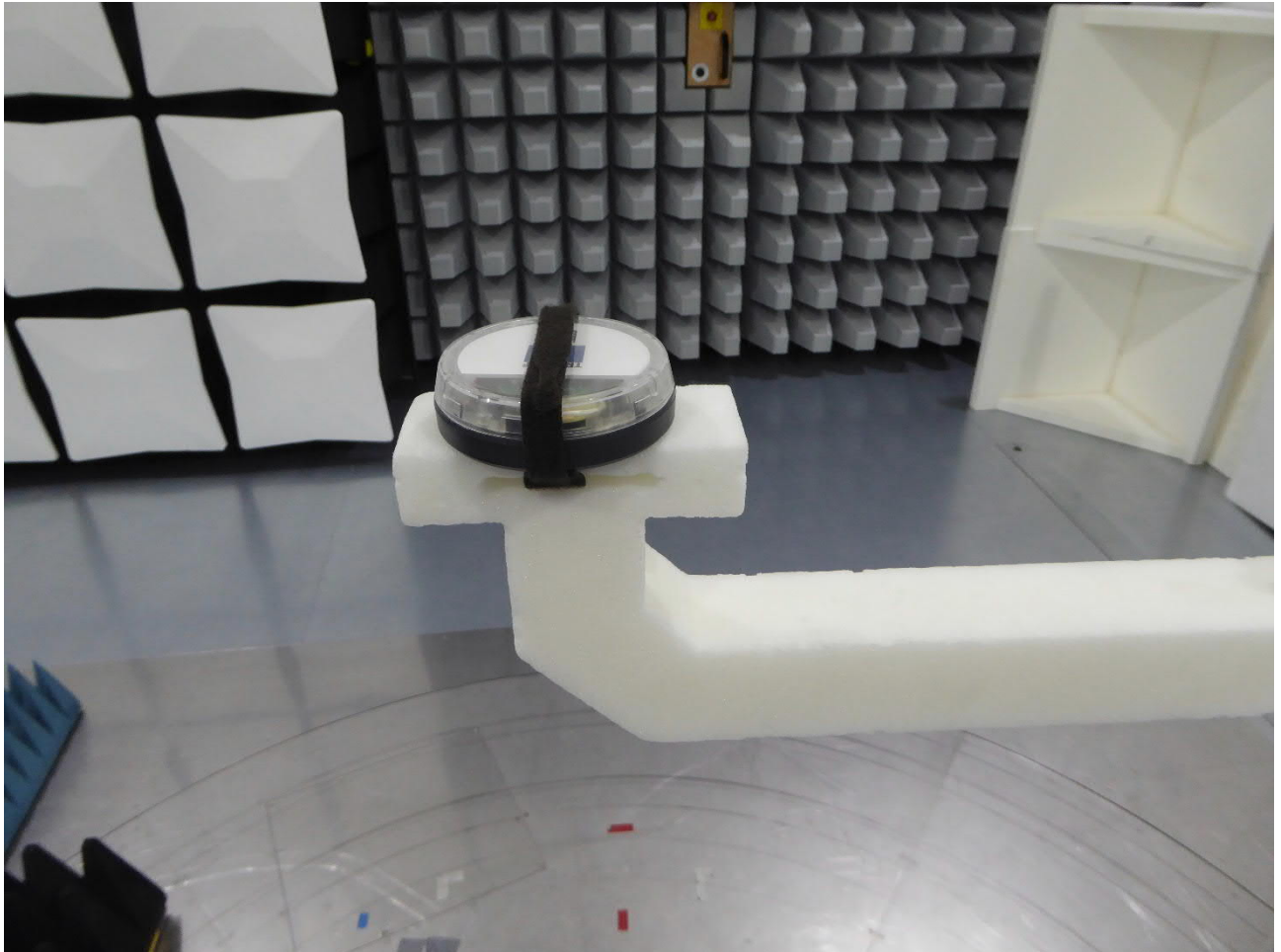
Test setup semi anechoic chamber with ground absorbers (Positioner)
