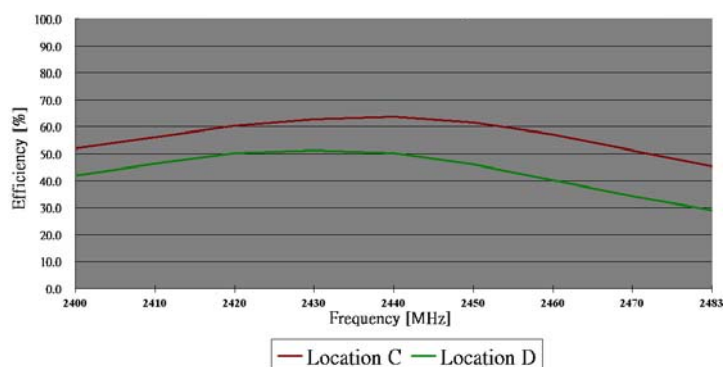
Radiation Efficiency
