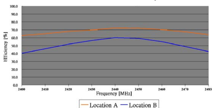
Radiation Efficiency
