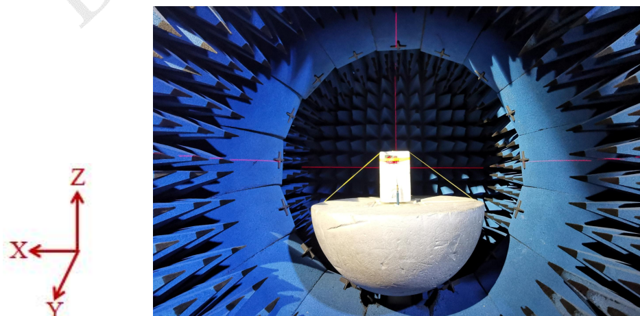
Front view
