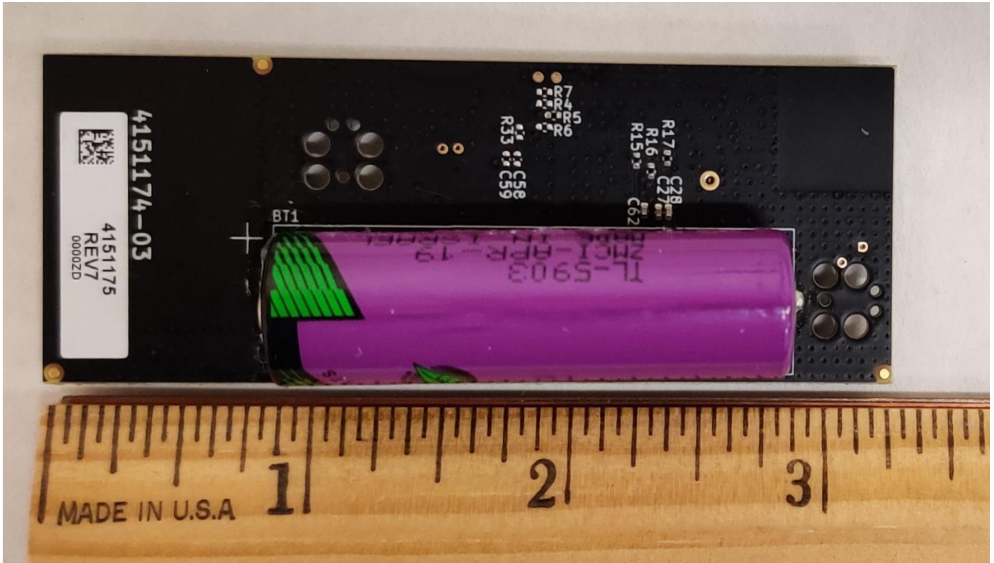
Figure 1: Internal Bottom – with Battery, No Resistor
