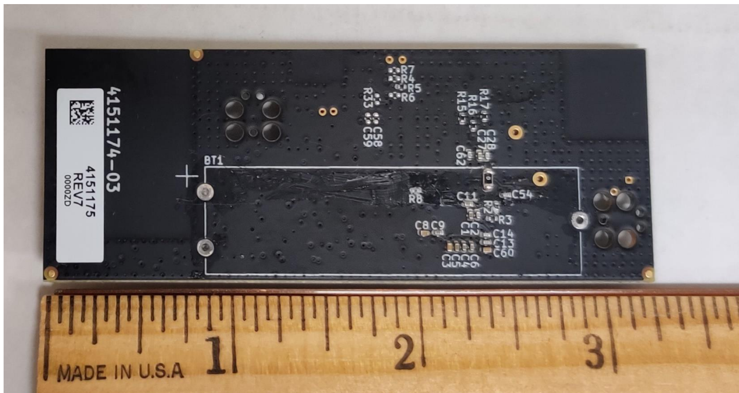
Figure 4: Internal Bottom - with Resistor, No Battery
