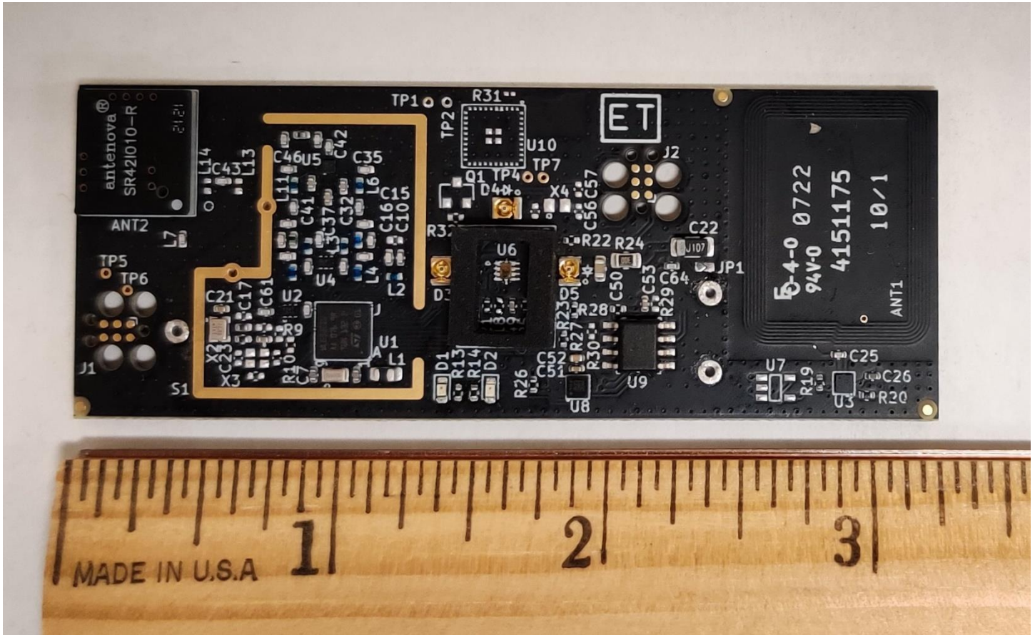
Figure 5: Internal Top - No Shield
