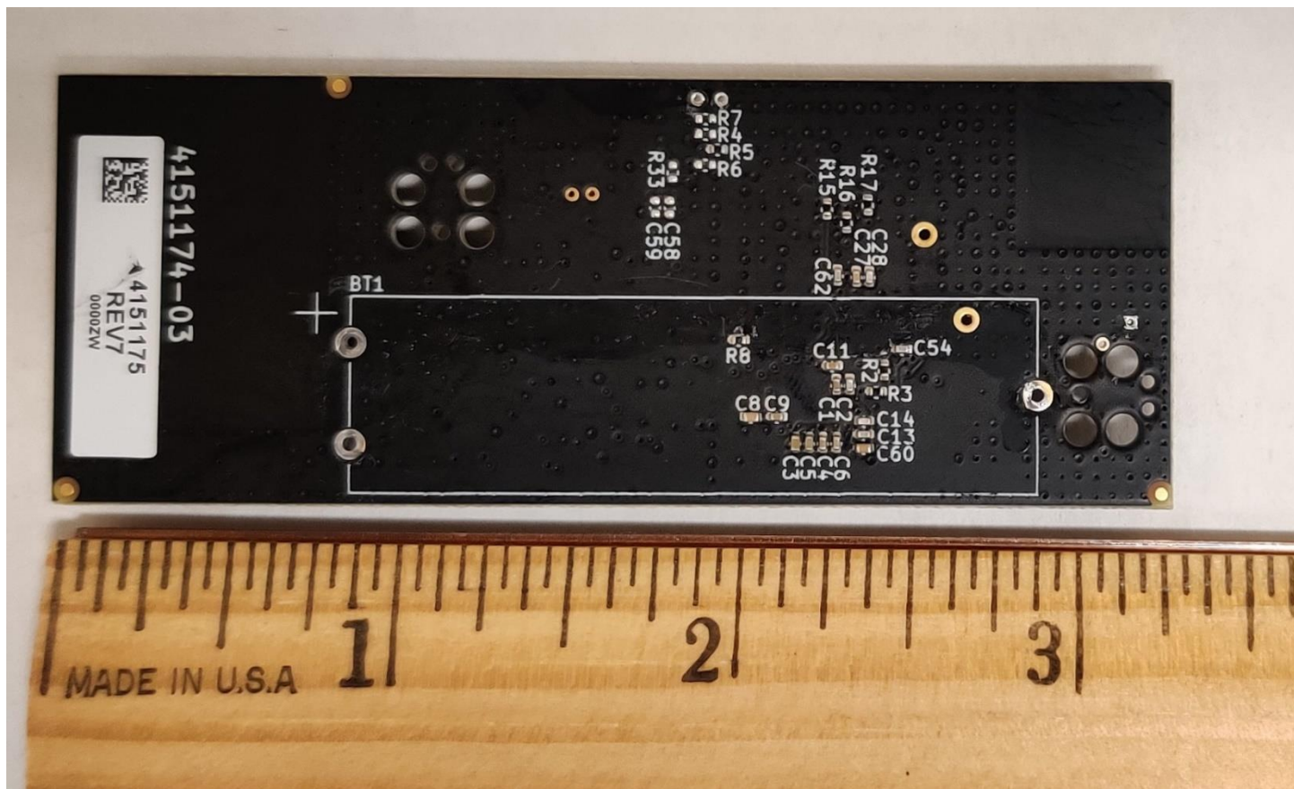
Figure 3: Internal Bottom - No Resistor, No Battery
