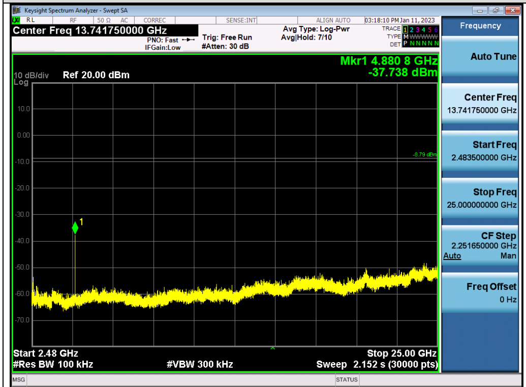
Test_Graph_2.4G_ANT1_2441.5_4Mbps_Higher Band Emissions
