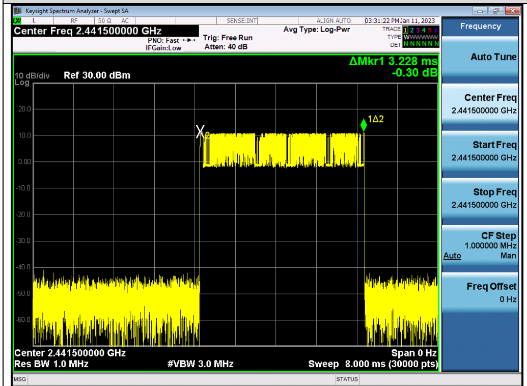
Test_Graph_2.4G_HOP_ANT1_NA_4Mbps_2441.5_Time per Burst
