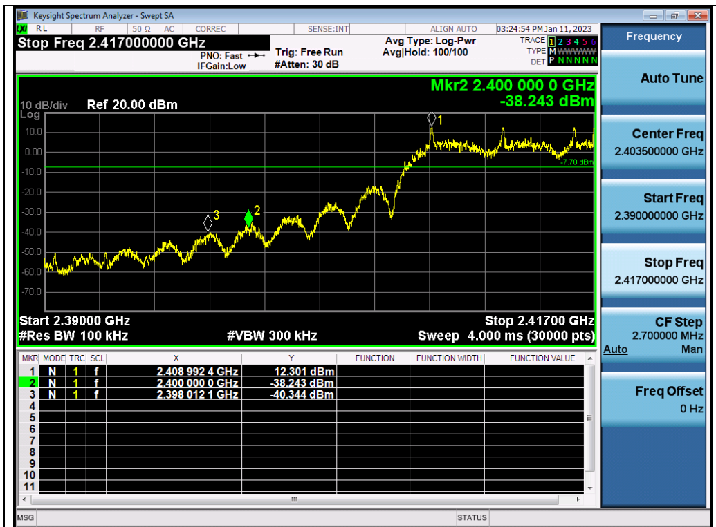
Test_Graph_2.4G_HOP_ANT1_NA_4Mbps_Lower Band Edge Emissions
