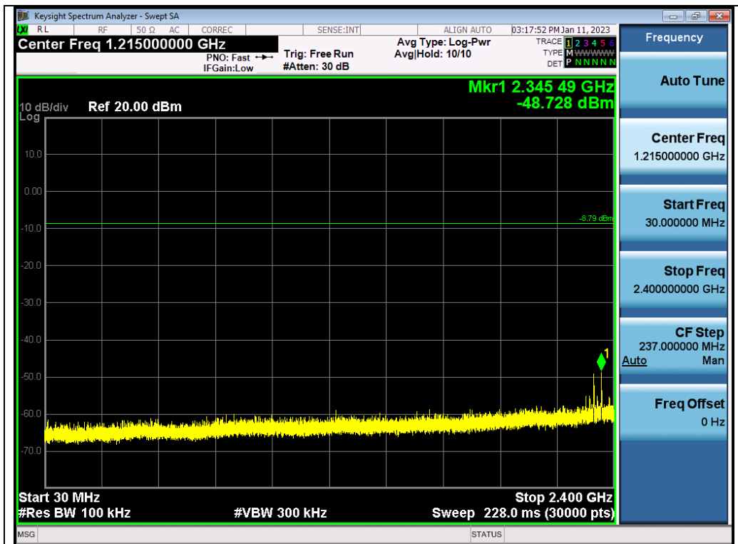
Test_Graph_2.4G_ANT1_2441.5_4Mbps_Lower Band Emissions
