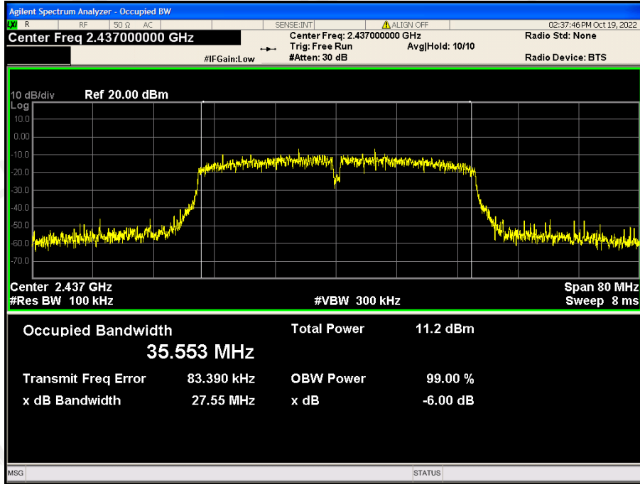
CH06: 2437MHz
