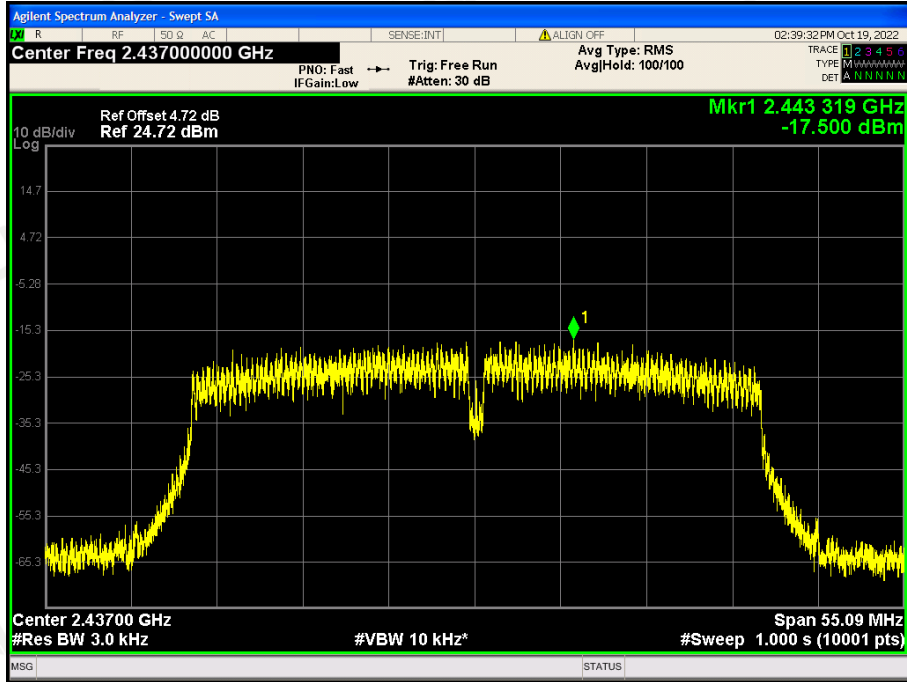
CH06: 2437MHz
