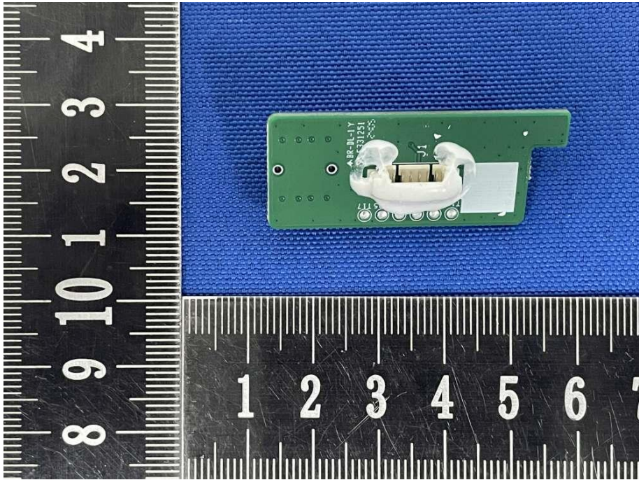
EUT Internal View 17
