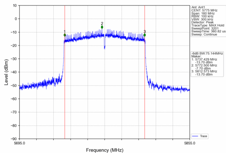
802.11ac(VHT80)_MCH_5775MHz_AntA_NTNV
