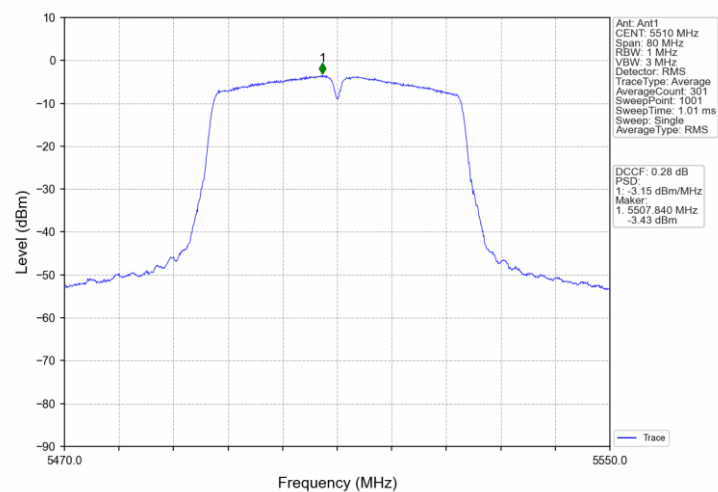
802.11ac(VHT40)_MCH_5550MHz_AntB_NTNV
