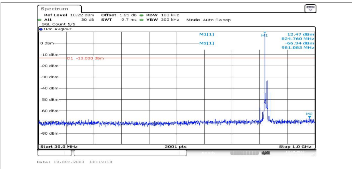
Band5-10MHz-QPSK-20450-1RB#0-Range3:30~1000MHz-PASS
