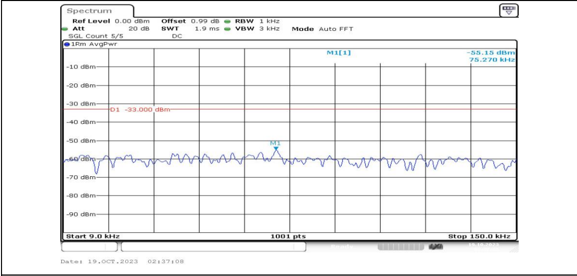
Band5-10MHz-16QAM-20525-1RB#0-Range1:0.009~0.15MHz-PASS
