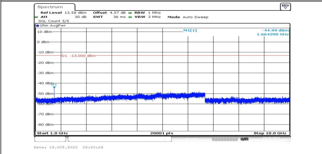
Band5-10MHz-QPSK-20525-1RB#0-Range4:1000~10000MHz-PASS
