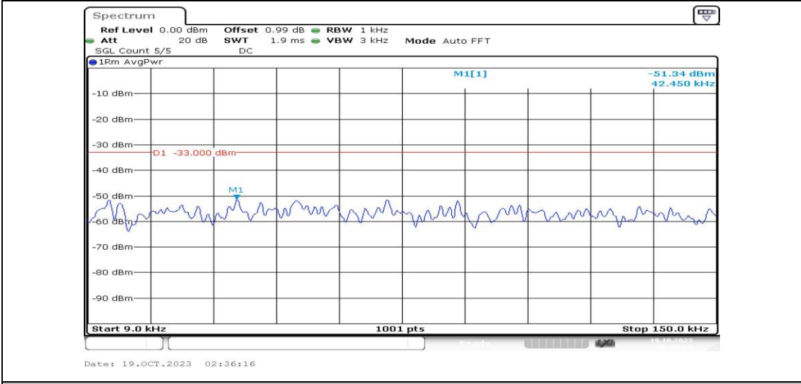
Band5-10MHz-16QAM-20450-1RB#0-Range1:0.009~0.15MHz-PASS
