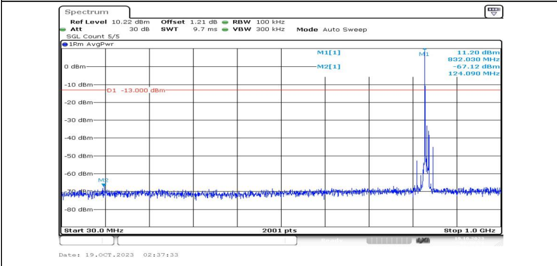
Band5-10MHz-16QAM-20525-1RB#0-Range3:30~1000MHz-PASS
