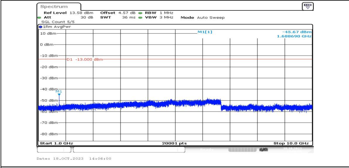
Band5-5MHz-QPSK-20625-1RB#0-Range4:1000~10000MHz-PASS
