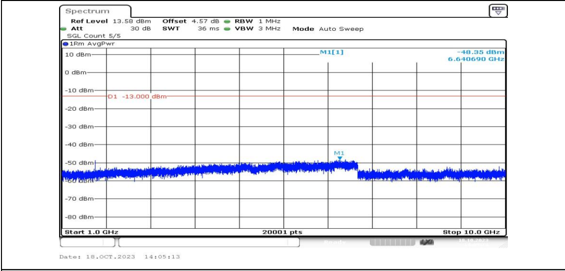
Band5-5MHz-16QAM-20525-1RB#0-Range4:1000~10000MHz-PASS
