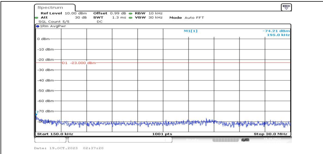
Band5-10MHz-16QAM-20525-1RB#0-Range2:0.15~30MHz-PASS
