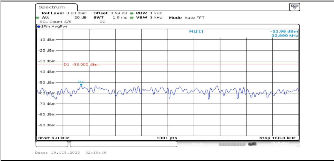
Band5-10MHz-QPSK-20525-1RB#0-Range1:0.009~0.15MHz-PASS
