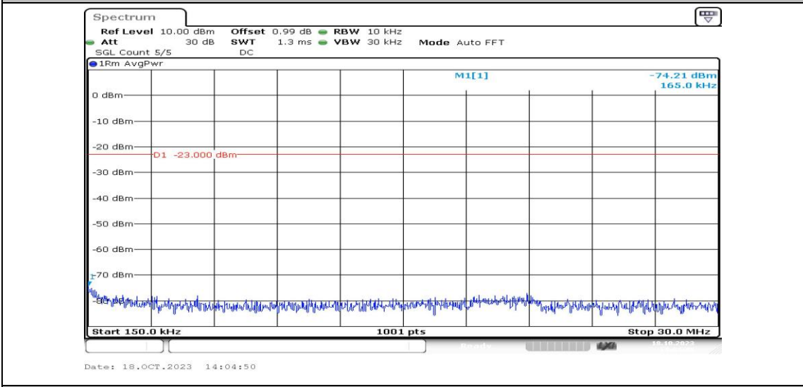
Band5-5MHz-16QAM-20525-1RB#0-Range2:0.15~30MHz-PASS
