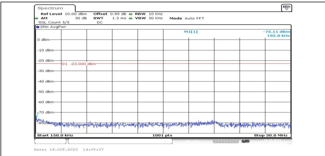
Band5-5MHz-QPSK-20625-1RB#0-Range2:0.15~30MHz-PASS
