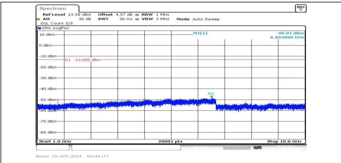
Band5-10MHz-QPSK-20600-1RB#0-Range4:1000~10000MHz-PASS
