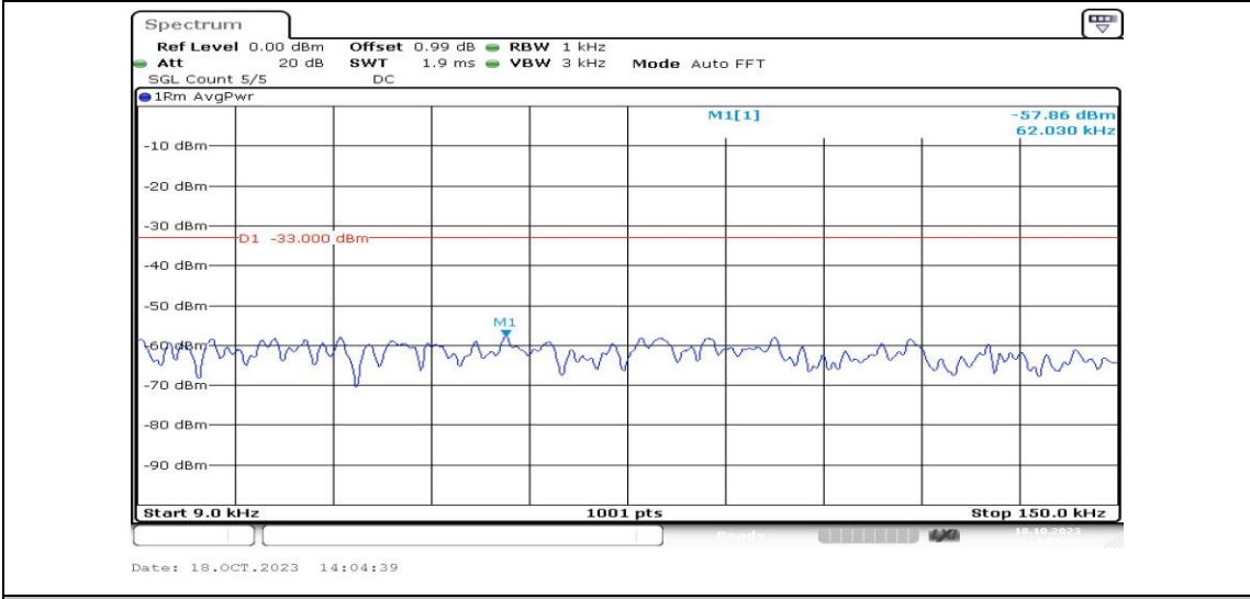
Band5-5MHz-16QAM-20525-1RB#0-Range1:0.009~0.15MHz-PASS
