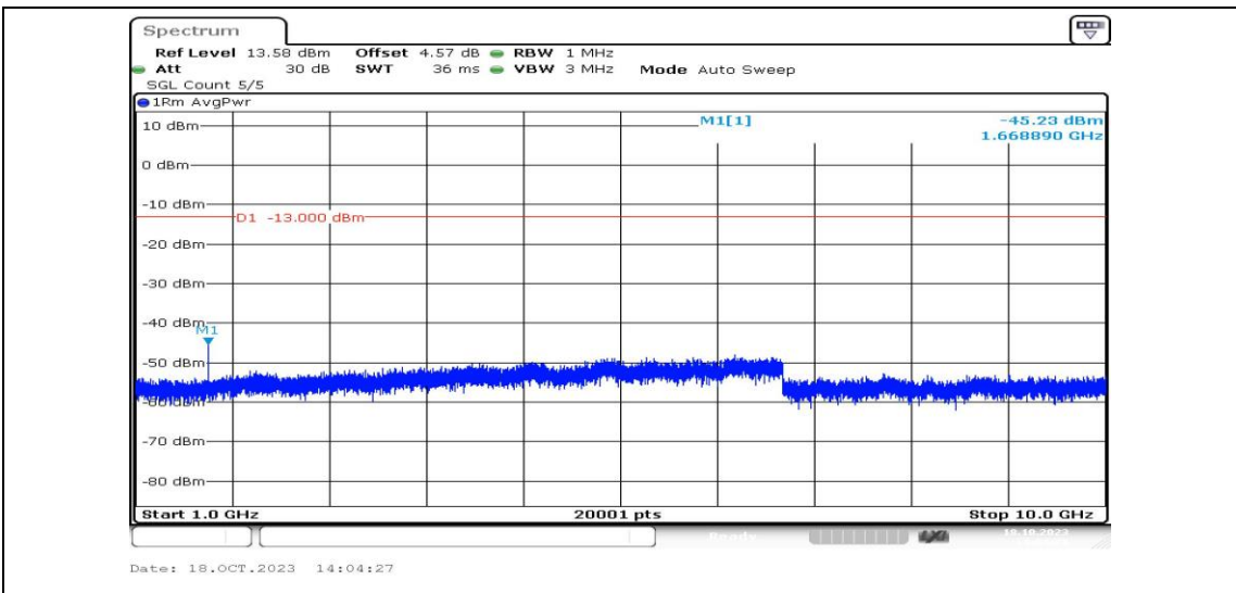
Band5-5MHz-QPSK-20525-1RB#0-Range4:1000~10000MHz-PASS
