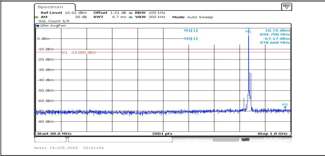
Band5-10MHz-QPSK-20600-1RB#0-Range3:30~1000MHz-PASS
