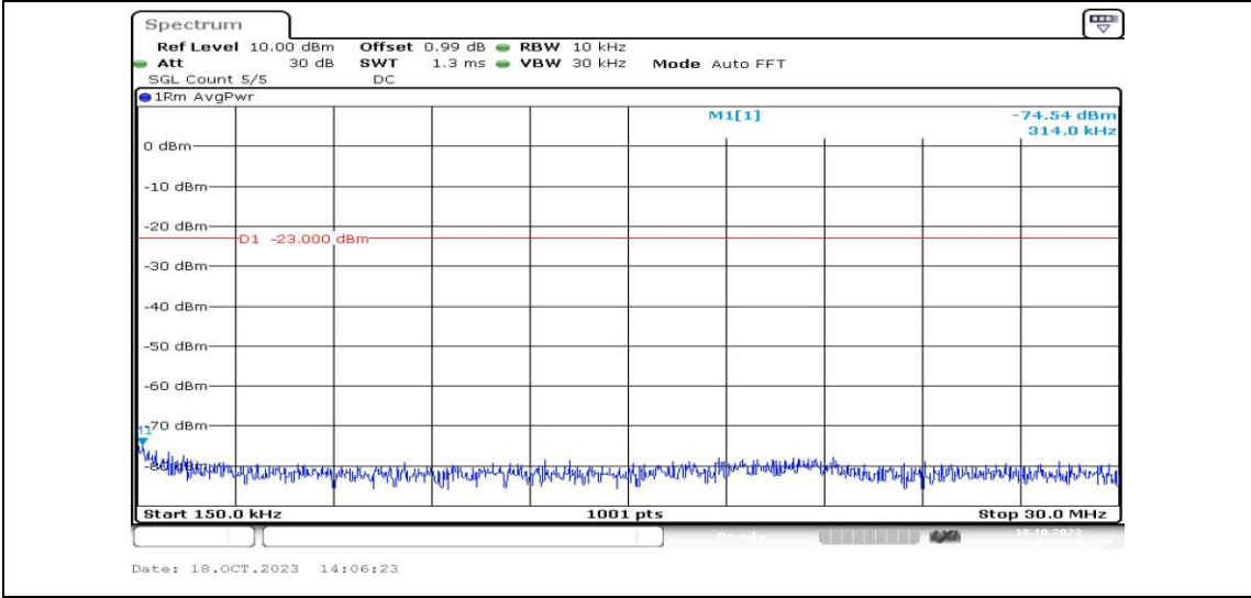
Band5-5MHz-16QAM-20625-1RB#0-Range2:0.15~30MHz-PASS
