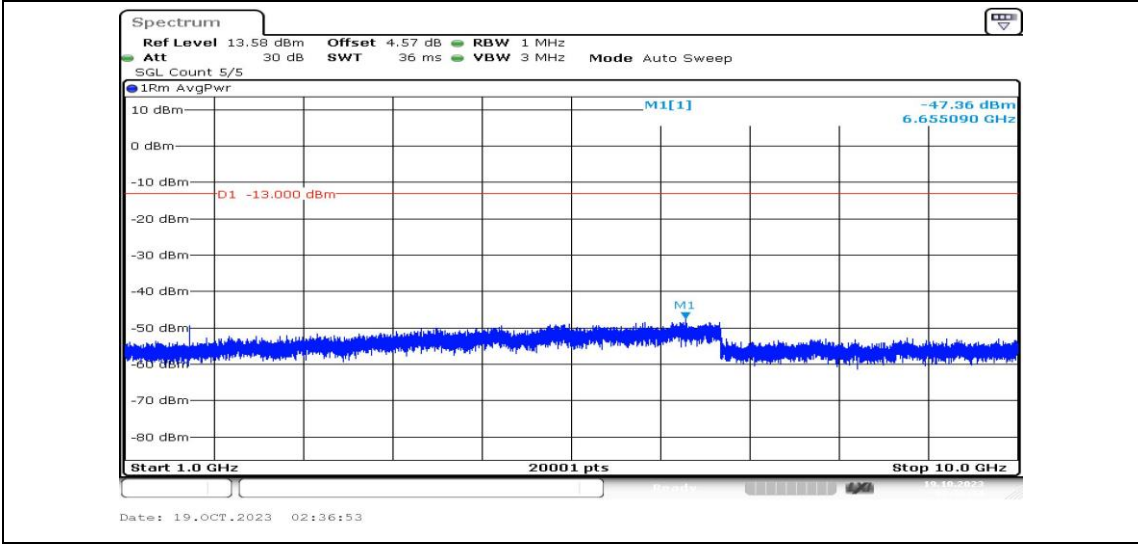
Band5-10MHz-16QAM-20450-1RB#0-Range4:1000~10000MHz-PASS
