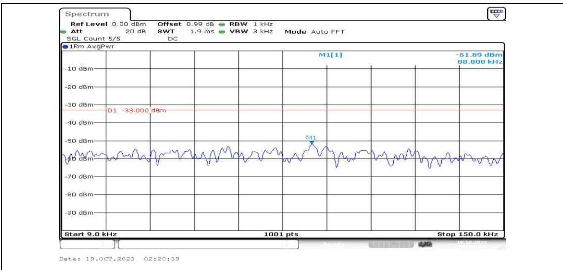
Band5-10MHz-QPSK-20600-1RB#0-Range1:0.009~0.15MHz-PASS
