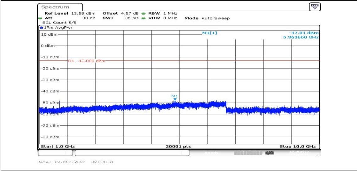
Band5-10MHz-QPSK-20450-1RB#0-Range4:1000~10000MHz-PASS
