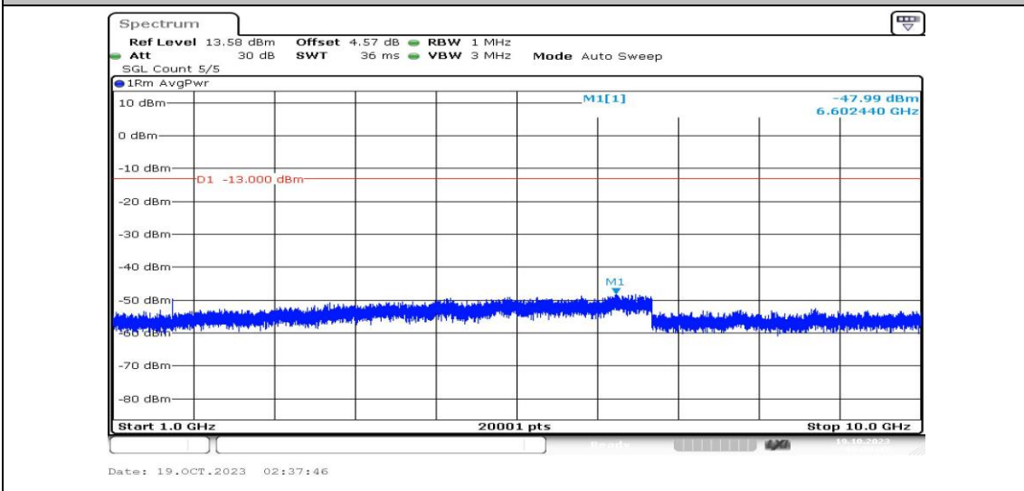
Band5-10MHz-16QAM-20525-1RB#0-Range4:1000~10000MHz-PASS
