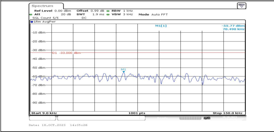
Band5-5MHz-QPSK-20625-1RB#0-Range1:0.009~0.15MHz-PASS
