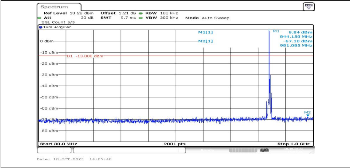
Band5-5MHz-QPSK-20625-1RB#0-Range3:30~1000MHz-PASS
