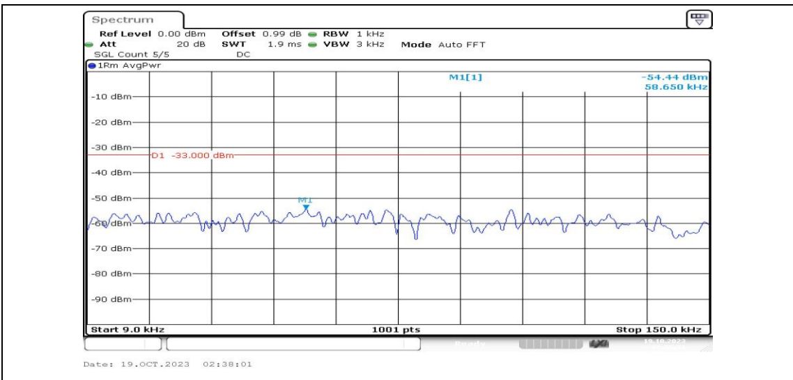
Band5-10MHz-16QAM-20600-1RB#0-Range1:0.009~0.15MHz-PASS
