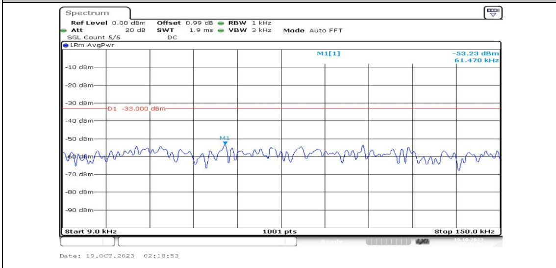
Band5-10MHz-QPSK-20450-1RB#0-Range1:0.009~0.15MHz-PASS
