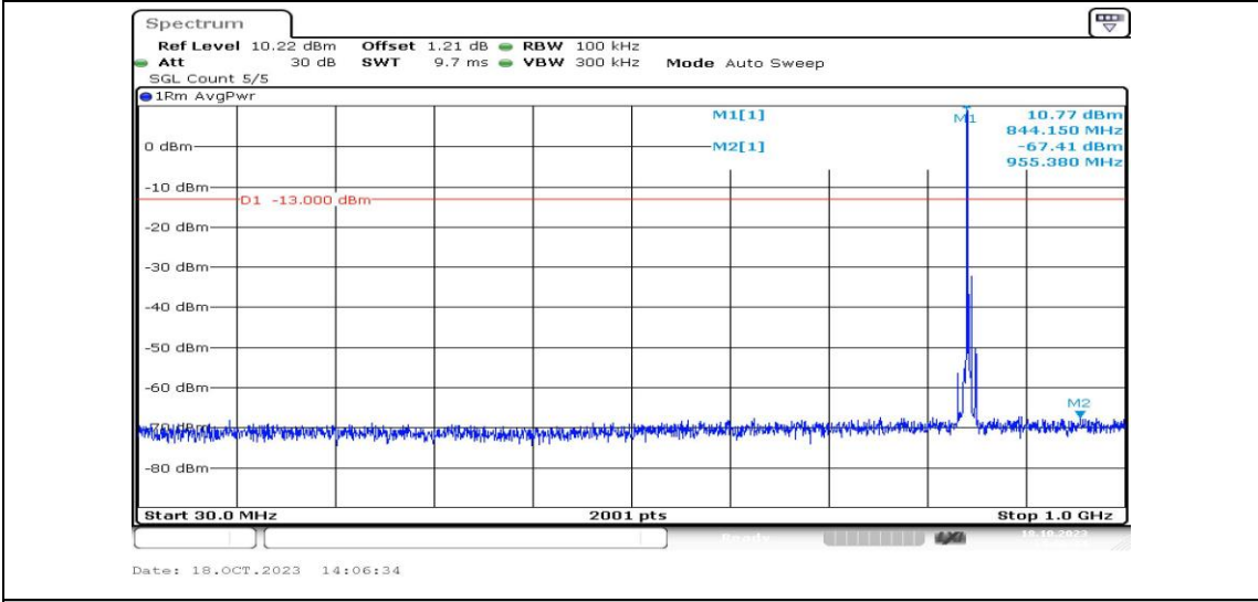
Band5-5MHz-16QAM-20625-1RB#0-Range3:30~1000MHz-PASS
