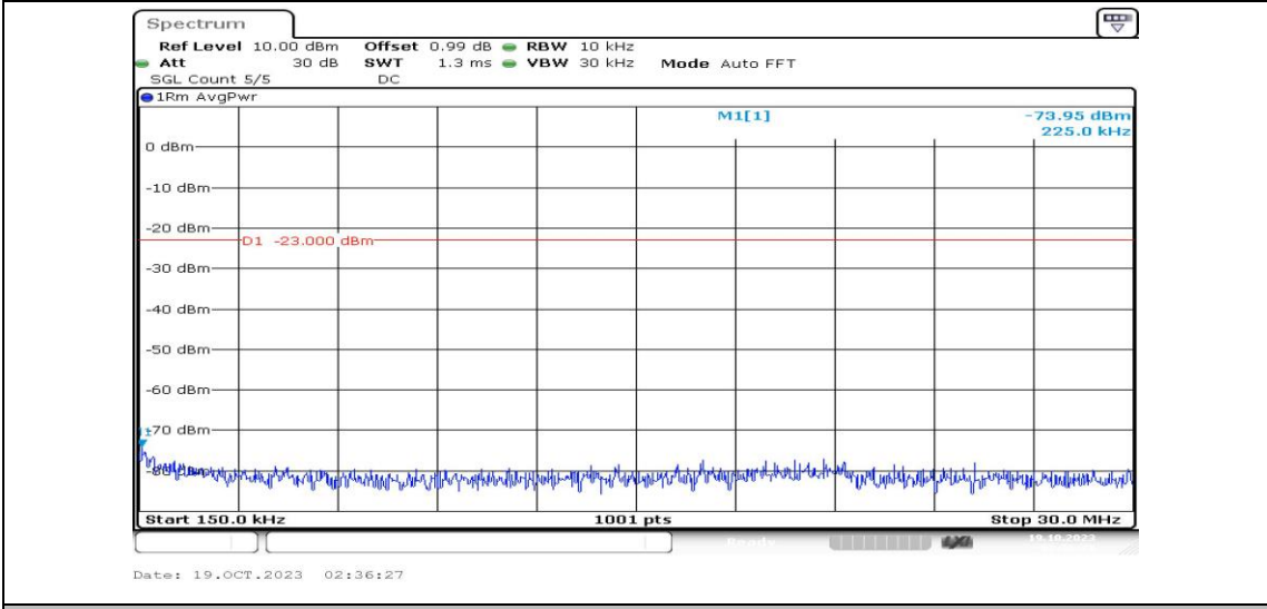
Band5-10MHz-16QAM-20450-1RB#0-Range2:0.15~30MHz-PASS
