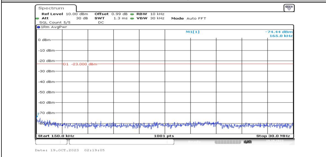
Band5-10MHz-QPSK-20450-1RB#0-Range2:0.15~30MHz-PASS
