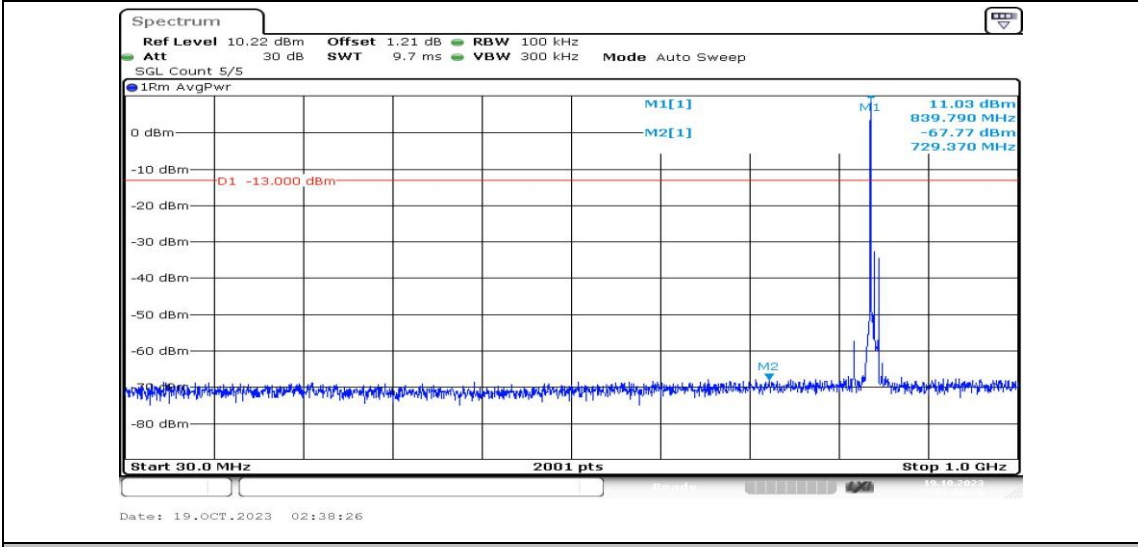
Band5-10MHz-16QAM-20600-1RB#0-Range3:30~1000MHz-PASS
