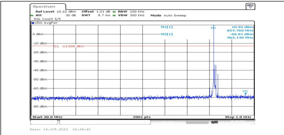
Band5-10MHz-16QAM-20450-1RB#0-Range3:30~1000MHz-PASS
