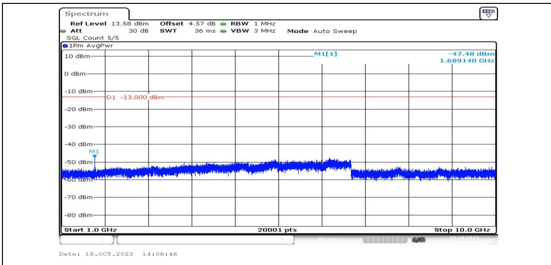
Band5-5MHz-16QAM-20625-1RB#0-Range4:1000~10000MHz-PASS
