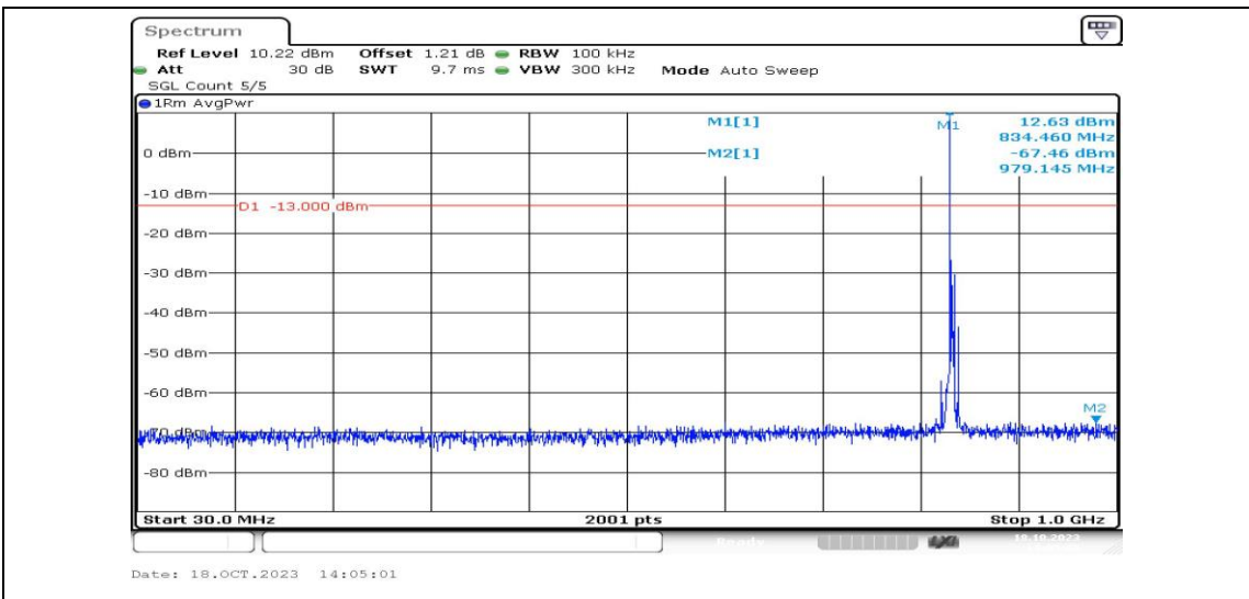
Band5-5MHz-16QAM-20525-1RB#0-Range3:30~1000MHz-PASS
