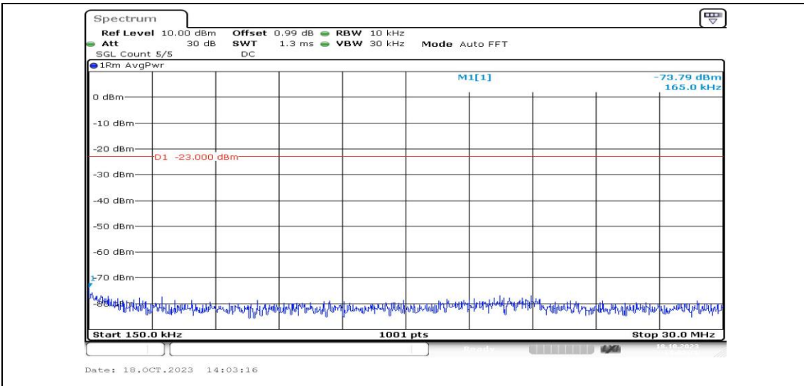
Band5-5MHz-16QAM-20425-1RB#0-Range2:0.15~30MHz-PASS
