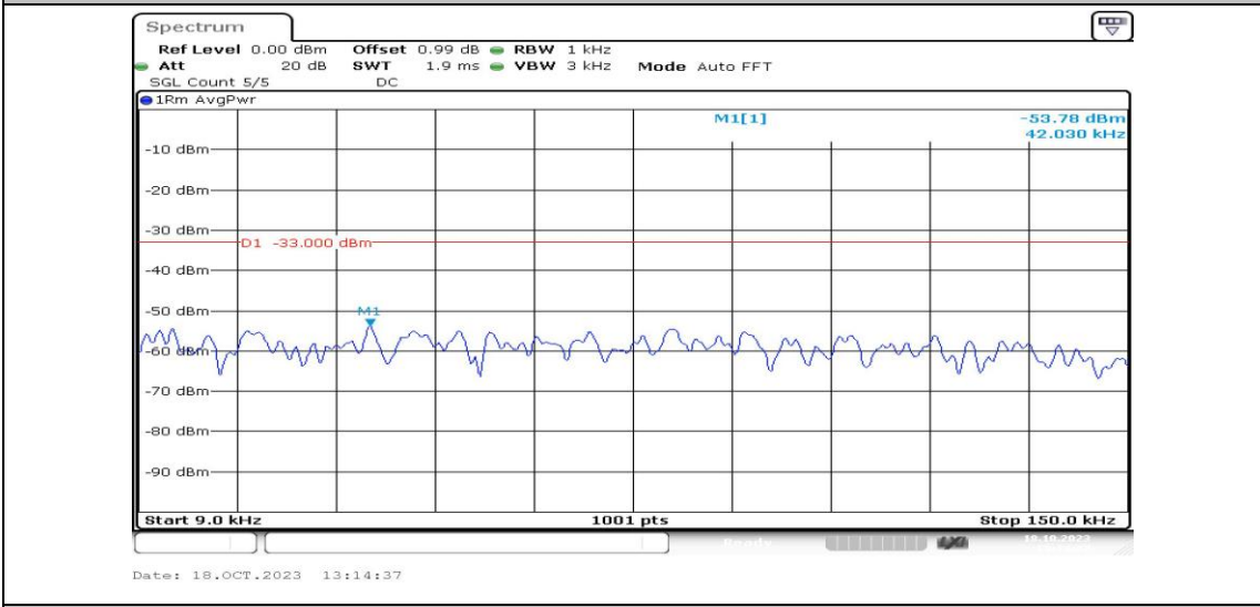
Band5-1.4MHz-16QAM-20407-1RB#0-Range1:0.009~0.15MHz-PASS
