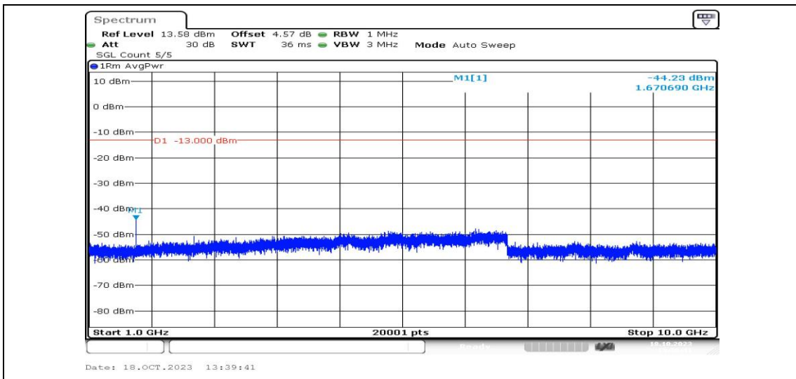
Band5-3MHz-QPSK-20525-1RB#0-Range4:1000~10000MHz-PASS
