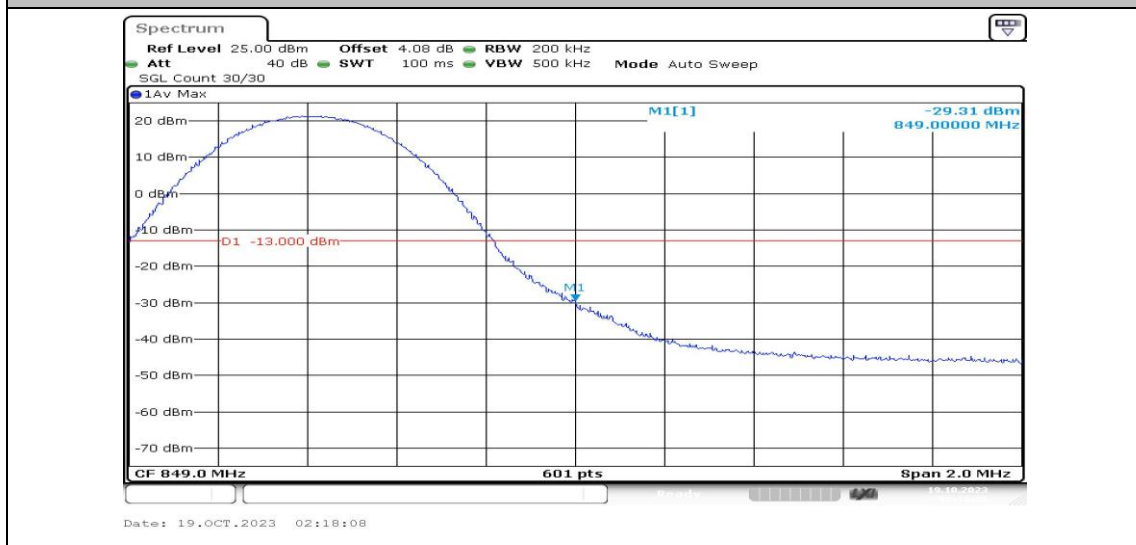
Band5-10MHz-QPSK-20600-1RB#49-PASS
