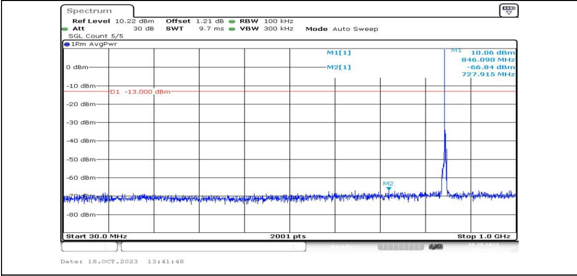
Band5-3MHz-16QAM-20635-1RB#0-Range3:30~1000MHz-PASS
