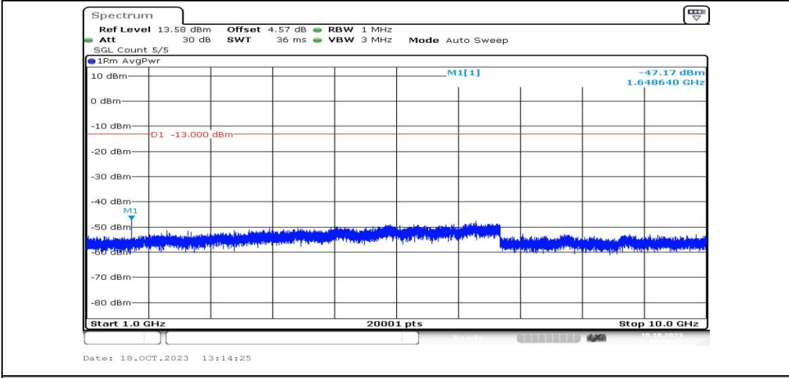
Band5-1.4MHz-QPSK-20407-1RB#0-Range4:1000~10000MHz-PASS
