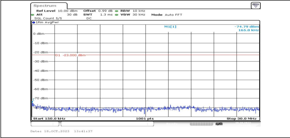
Band5-3MHz-16QAM-20635-1RB#0-Range2:0.15~30MHz-PASS
