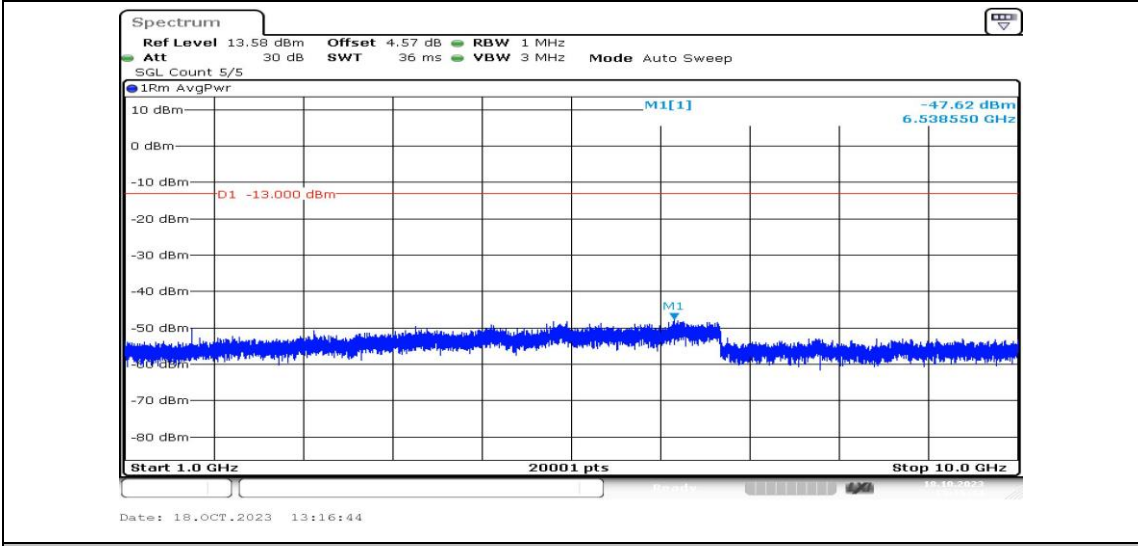
Band5-1.4MHz-16QAM-20525-1RB#0-Range4:1000~10000MHz-PASS
