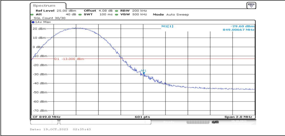
Band5-10MHz-16QAM-20600-1RB#49-PASS
