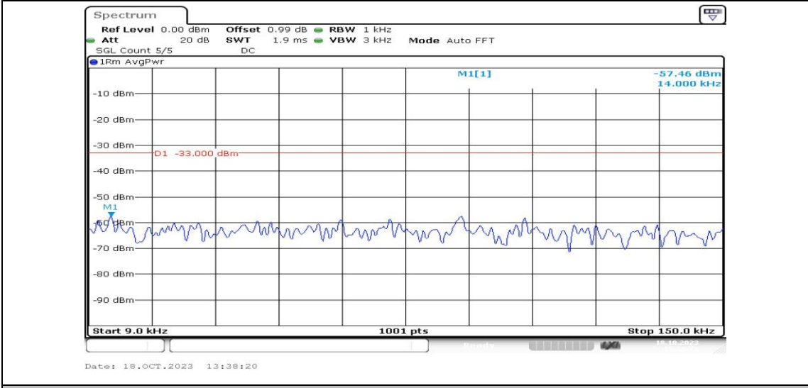
Band5-3MHz-16QAM-20415-1RB#0-Range1:0.009~0.15MHz-PASS
