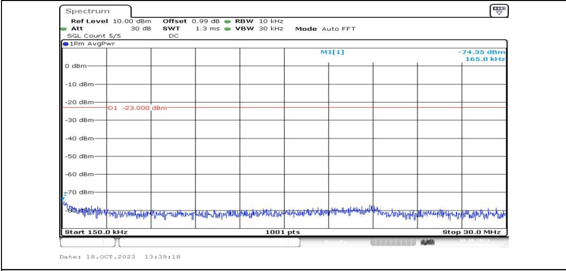
Band5-3MHz-QPSK-20525-1RB#0-Range2:0.15~30MHz-PASS
