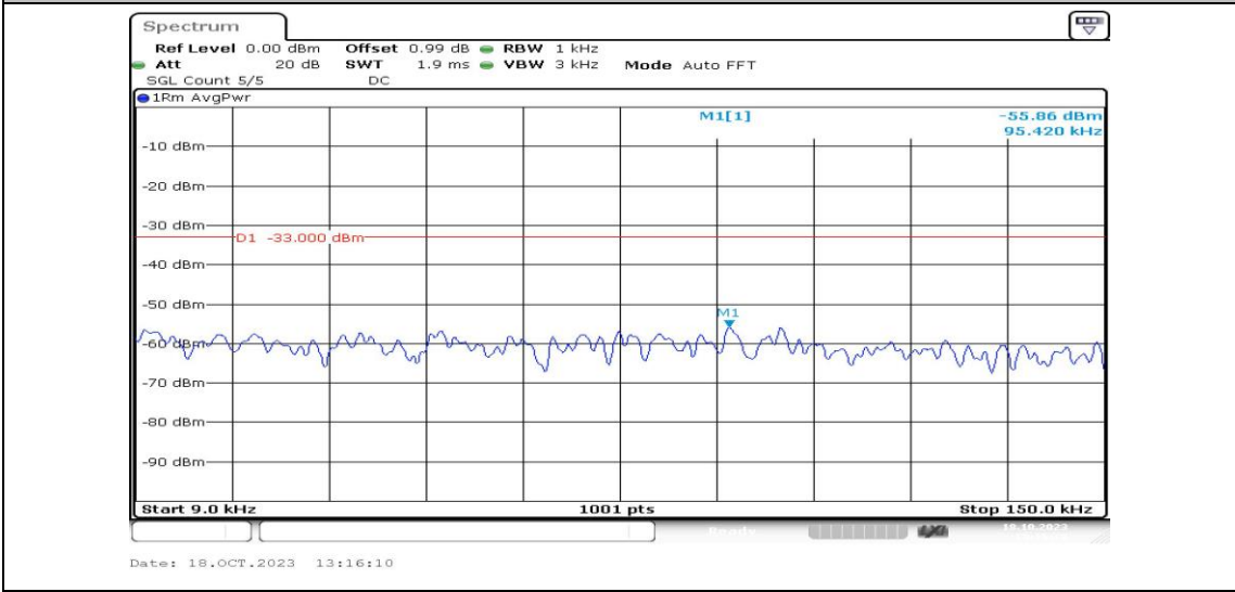
Band5-1.4MHz-16QAM-20525-1RB#0-Range1:0.009~0.15MHz-PASS
