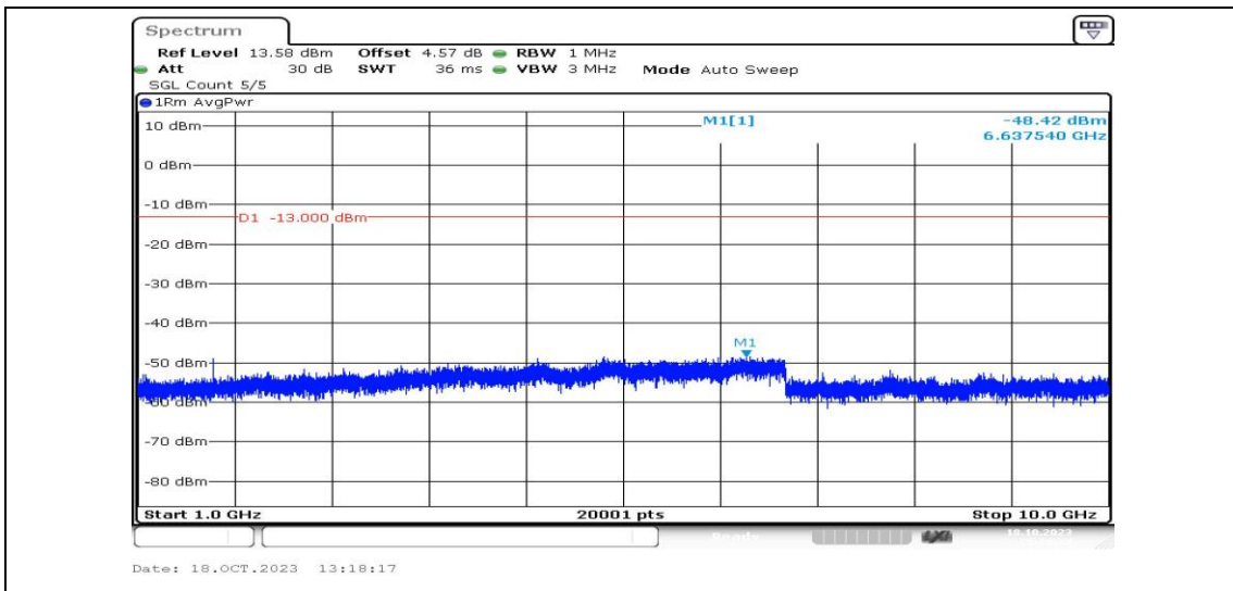
Band5-1.4MHz-16QAM-20643-1RB#0-Range4:1000~10000MHz-PASS
