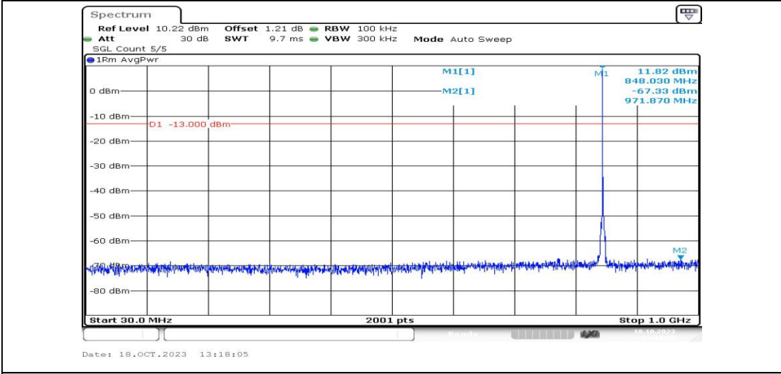
Band5-1.4MHz-16QAM-20643-1RB#0-Range3:30~1000MHz-PASS
