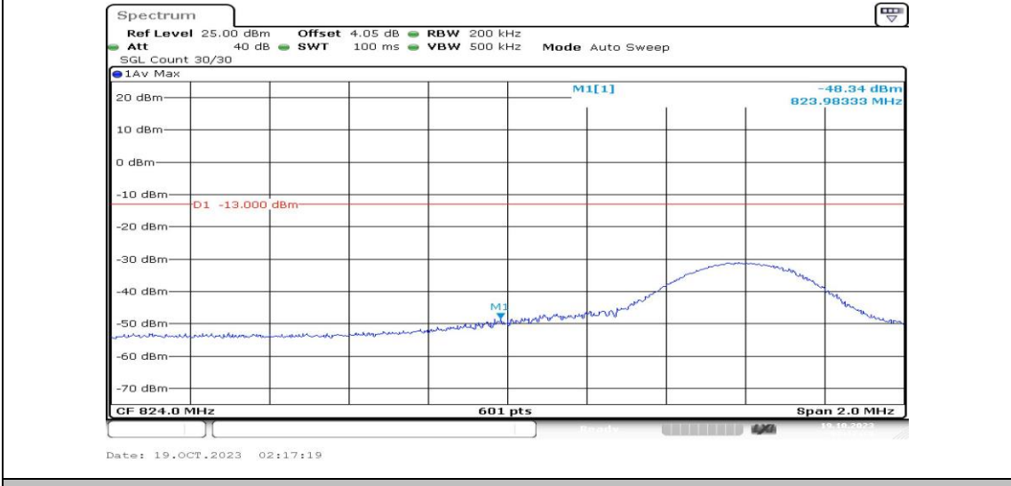
Band5-10MHz-QPSK-20450-1RB#49-PASS
