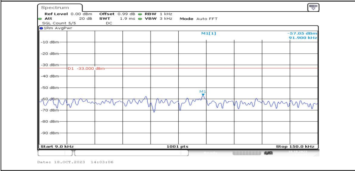
Band5-5MHz-16QAM-20425-1RB#0-Range1:0.009~0.15MHz-PASS
