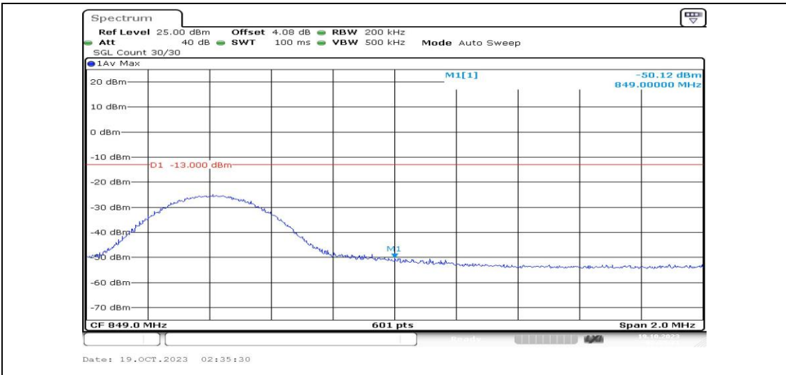
Band5-10MHz-16QAM-20600-1RB#0-PASS
