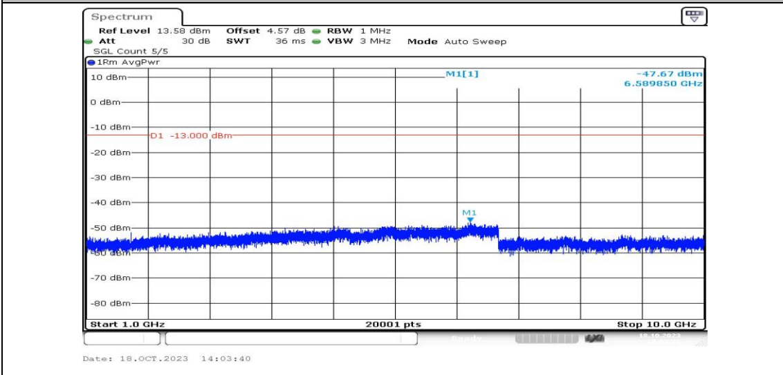
Band5-5MHz-16QAM-20425-1RB#0-Range4:1000~10000MHz-PASS
