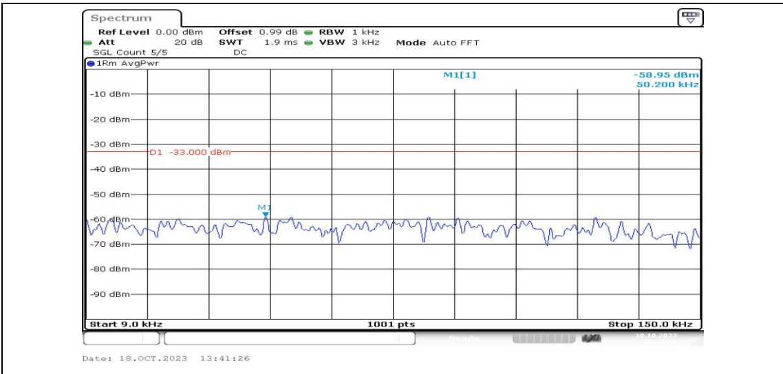
Band5-3MHz-16QAM-20635-1RB#0-Range1:0.009~0.15MHz-PASS
