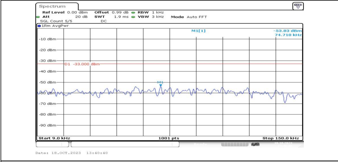
Band5-3MHz-QPSK-20635-1RB#0-Range1:0.009~0.15MHz-PASS
