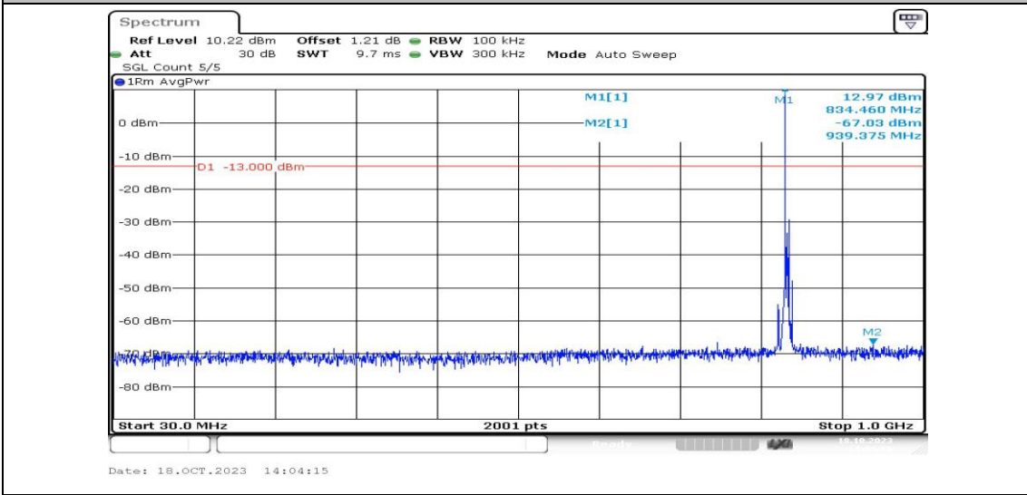
Band5-5MHz-QPSK-20525-1RB#0-Range3:30~1000MHz-PASS
