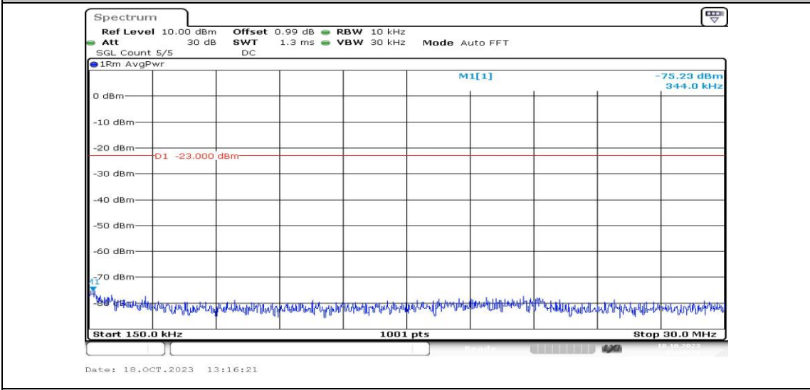
Band5-1.4MHz-16QAM-20525-1RB#0-Range2:0.15~30MHz-PASS
