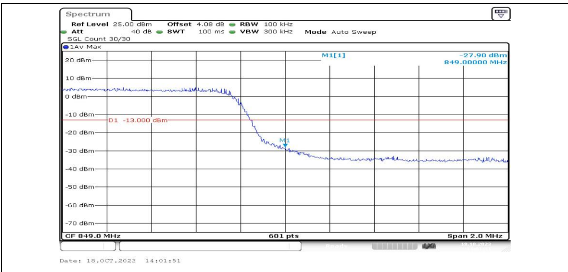
Band5-5MHz-16QAM-20625-25RB#0-PASS
