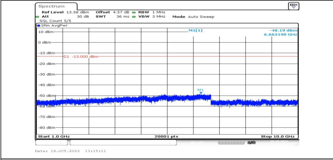
Band5-1.4MHz-16QAM-20407-1RB#0-Range4:1000~10000MHz-PASS
