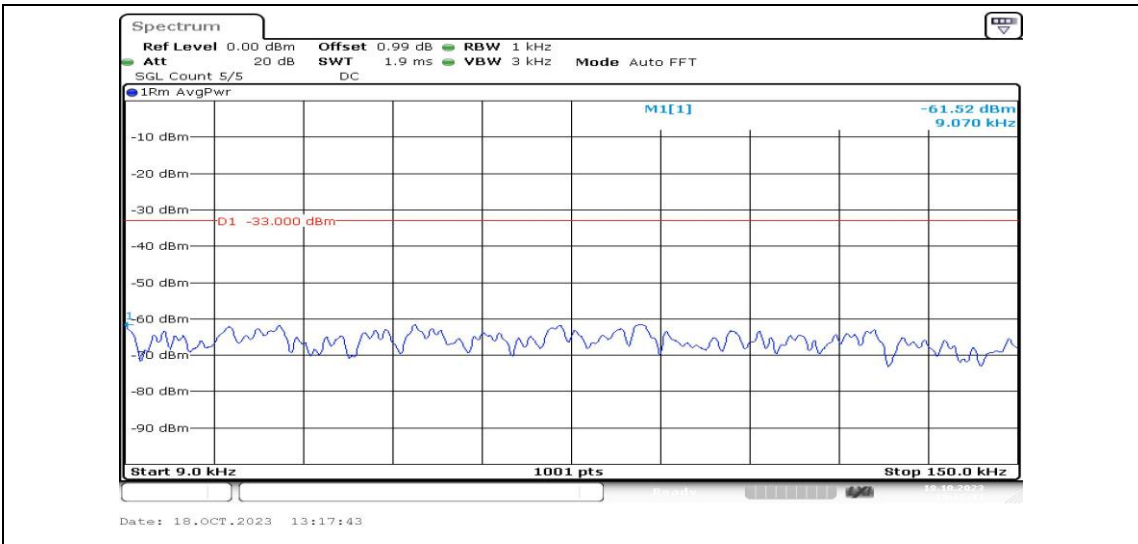
Band5-1.4MHz-16QAM-20643-1RB#0-Range1:0.009~0.15MHz-PASS
