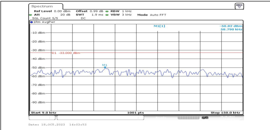
Band5-5MHz-QPSK-20525-1RB#0-Range1:0.009~0.15MHz-PASS
