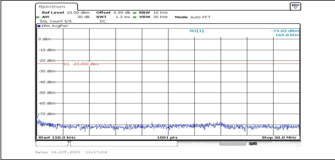
Band5-1.4MHz-16QAM-20643-1RB#0-Range2:0.15~30MHz-PASS
