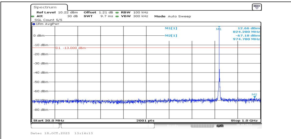
Band5-1.4MHz-QPSK-20407-1RB#0-Range3:30~1000MHz-PASS
