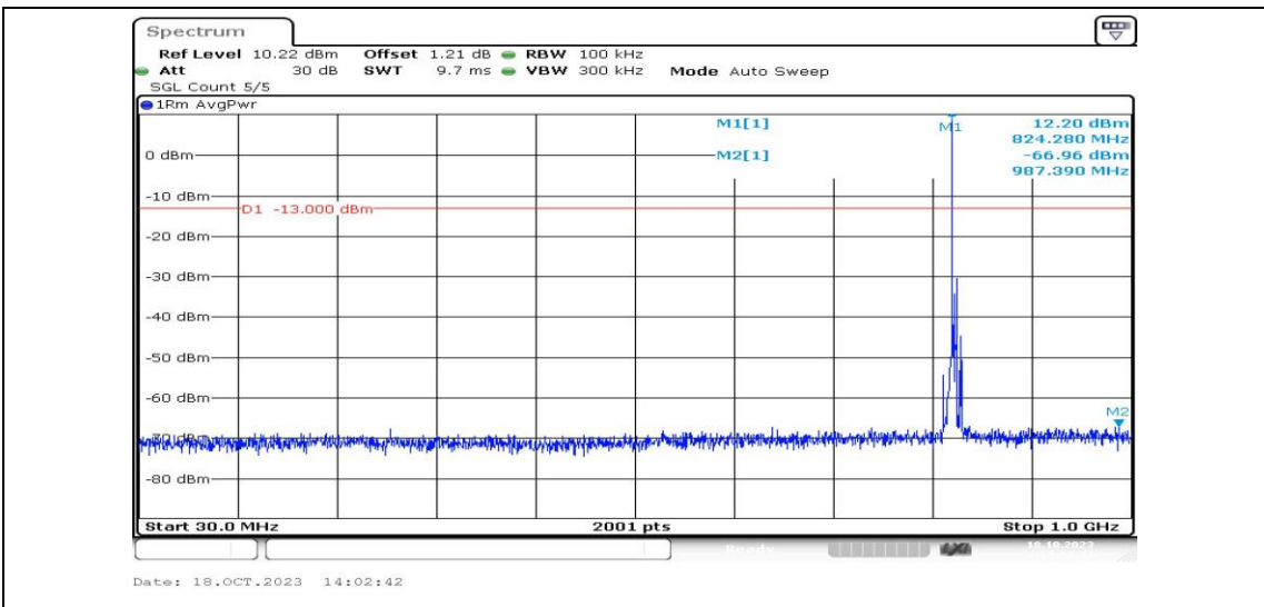
Band5-5MHz-QPSK-20425-1RB#0-Range3:30~1000MHz-PASS
