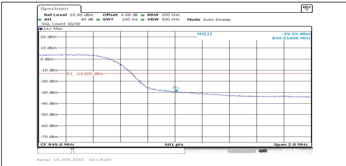
Band5-10MHz-QPSK-20600-50RB#0-PASS
