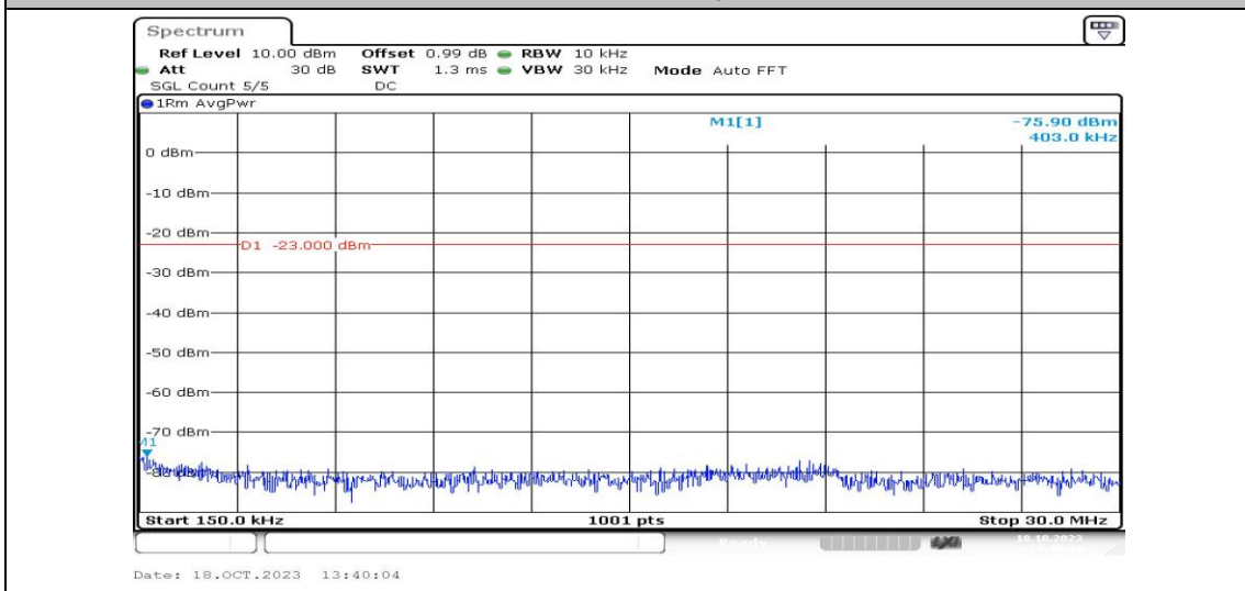
Band5-3MHz-16QAM-20525-1RB#0-Range2:0.15~30MHz-PASS
