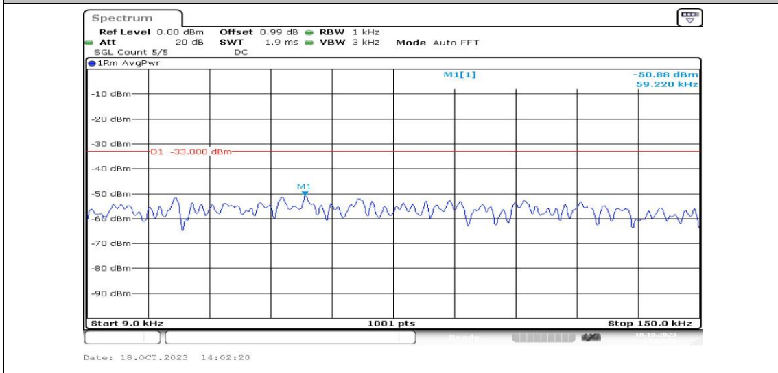
Band5-5MHz-QPSK-20425-1RB#0-Range1:0.009~0.15MHz-PASS
