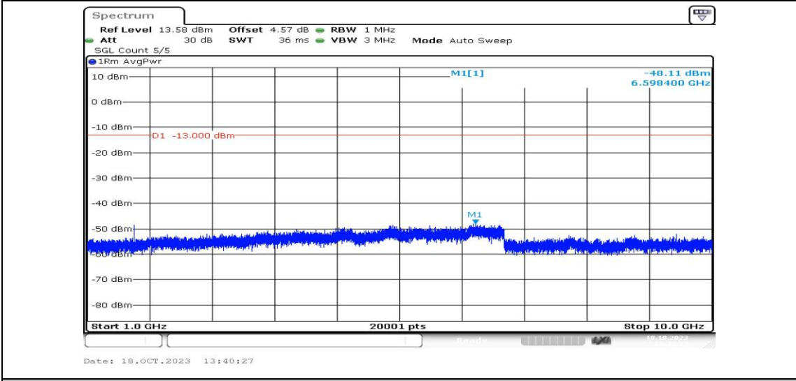
Band5-3MHz-16QAM-20525-1RB#0-Range4:1000~10000MHz-PASS
