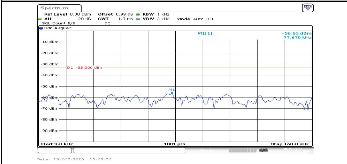
Band5-3MHz-16QAM-20525-1RB#0-Range1:0.009~0.15MHz-PASS
