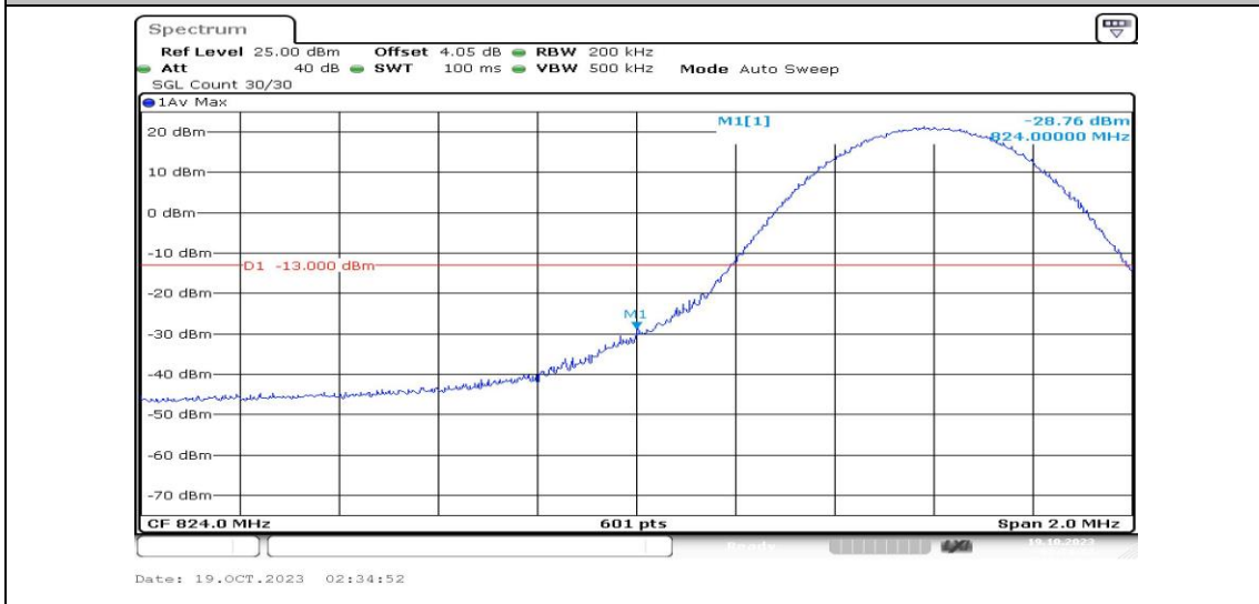
Band5-10MHz-16QAM-20450-1RB#0-PASS
