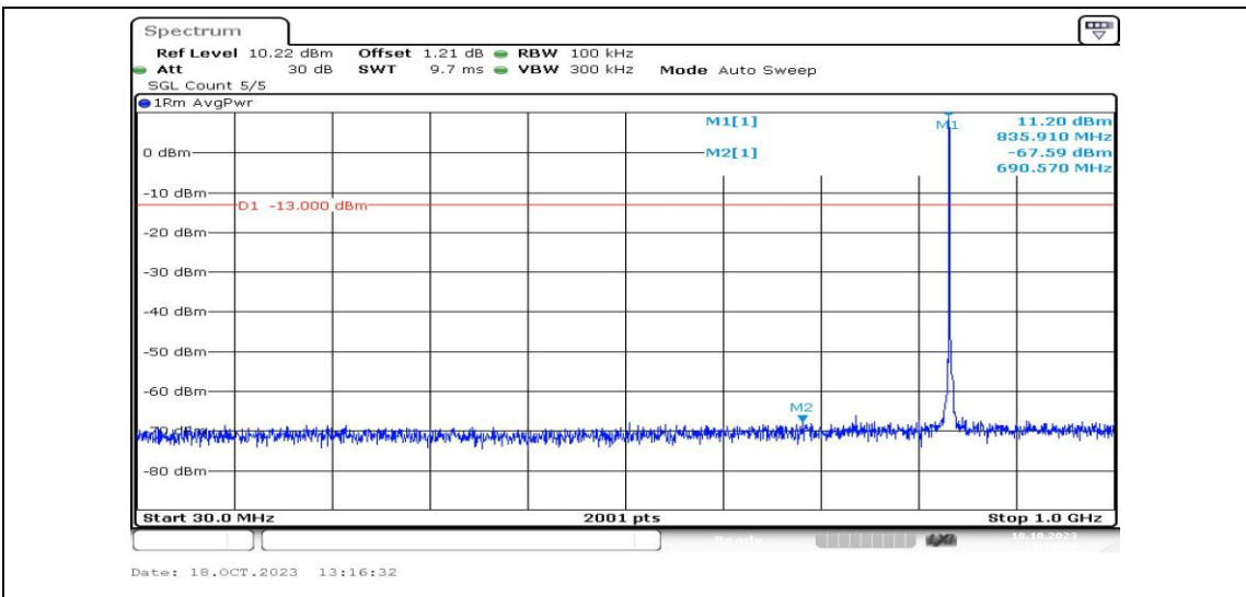
Band5-1.4MHz-16QAM-20525-1RB#0-Range3:30~1000MHz-PASS
