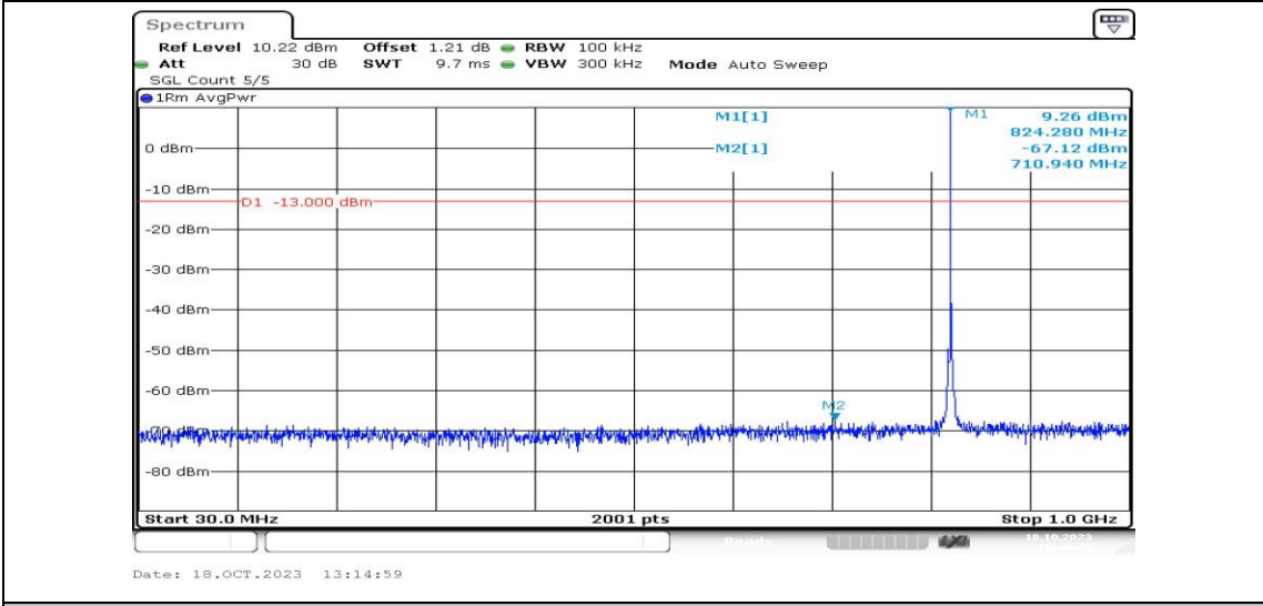
Band5-1.4MHz-16QAM-20407-1RB#0-Range3:30~1000MHz-PASS
