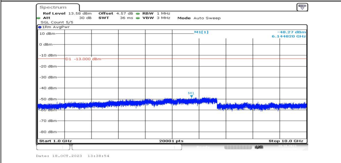
Band5-3MHz-16QAM-20415-1RB#0-Range4:1000~10000MHz-PASS
