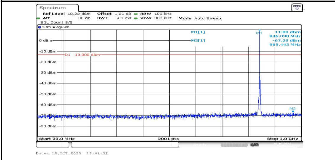
Band5-3MHz-QPSK-20635-1RB#0-Range3:30~1000MHz-PASS
