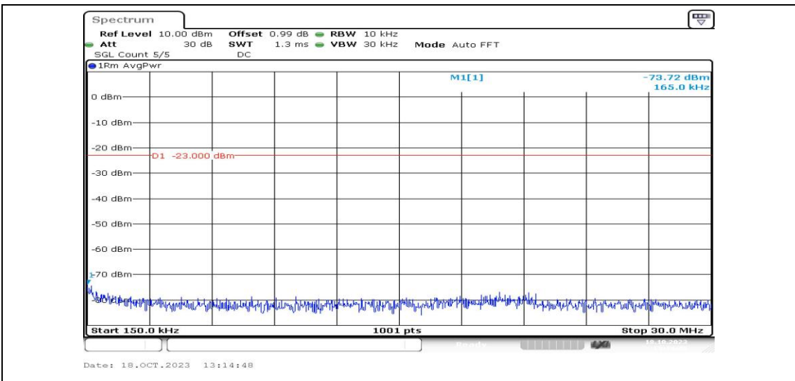
Band5-1.4MHz-16QAM-20407-1RB#0-Range2:0.15~30MHz-PASS
