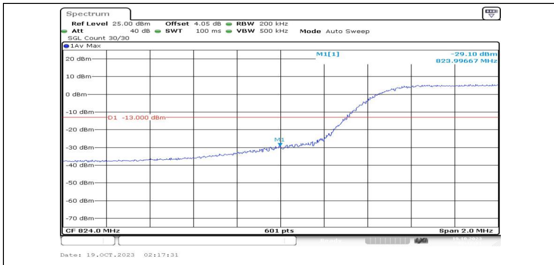
Band5-10MHz-QPSK-20450-50RB#0-PASS
