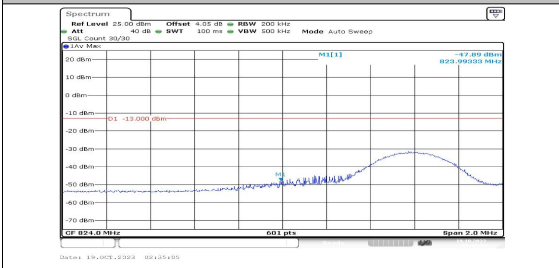
Band5-10MHz-16QAM-20450-1RB#49-PASS
