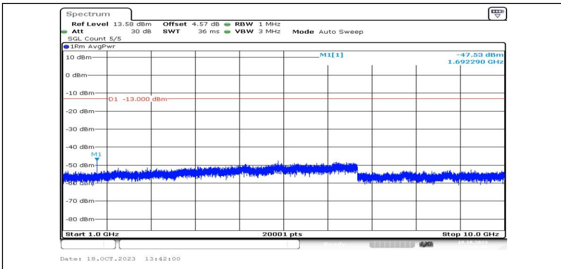
Band5-3MHz-16QAM-20635-1RB#0-Range4:1000~10000MHz-PASS
