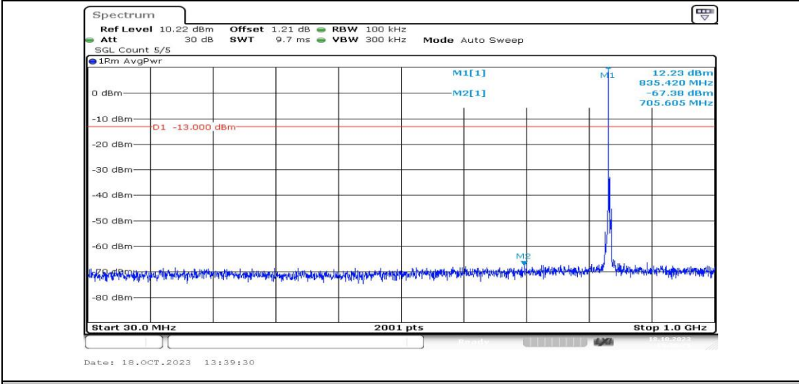
Band5-3MHz-QPSK-20525-1RB#0-Range3:30~1000MHz-PASS
