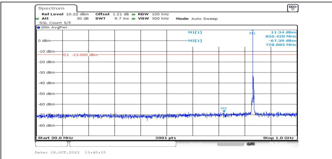
Band5-3MHz-16QAM-20525-1RB#0-Range3:30~1000MHz-PASS
