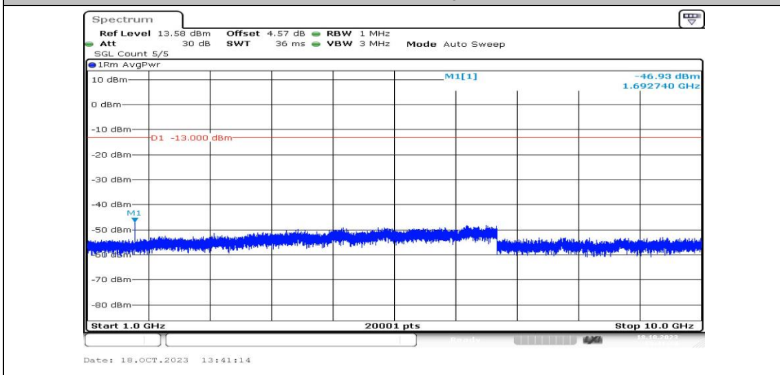
Band5-3MHz-QPSK-20635-1RB#0-Range4:1000~10000MHz-PASS
