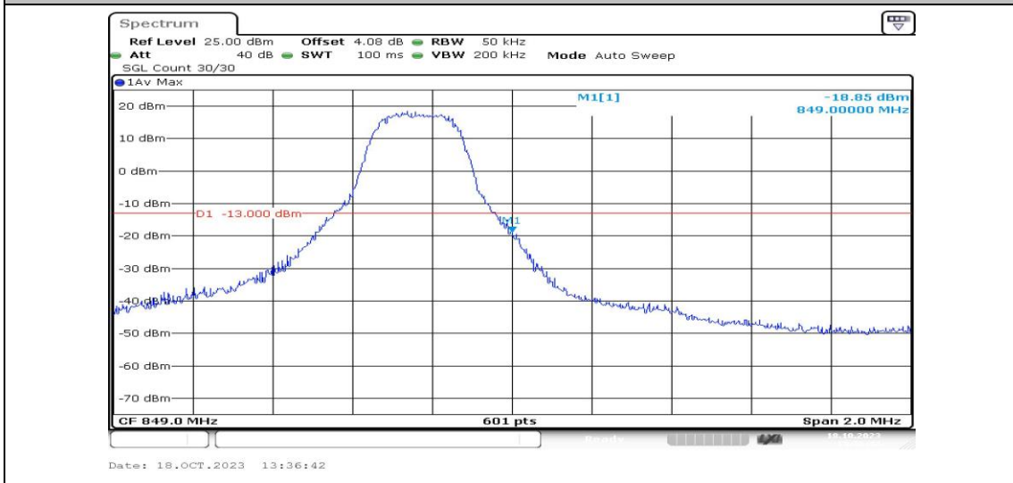
Band5-3MHz-16QAM-20635-1RB#14-PASS
