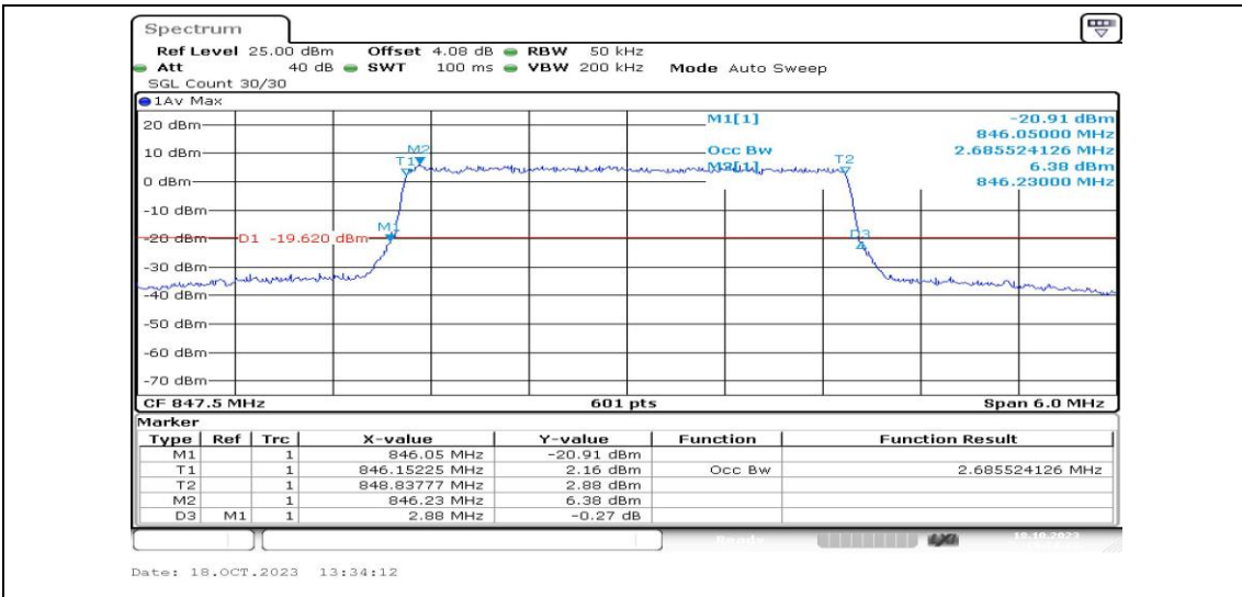
Band5-3MHz-16QAM-20635-15RB#0-PASS
