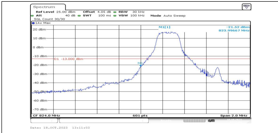
Band5-1.4MHz-QPSK-20407-1RB#0-PASS
