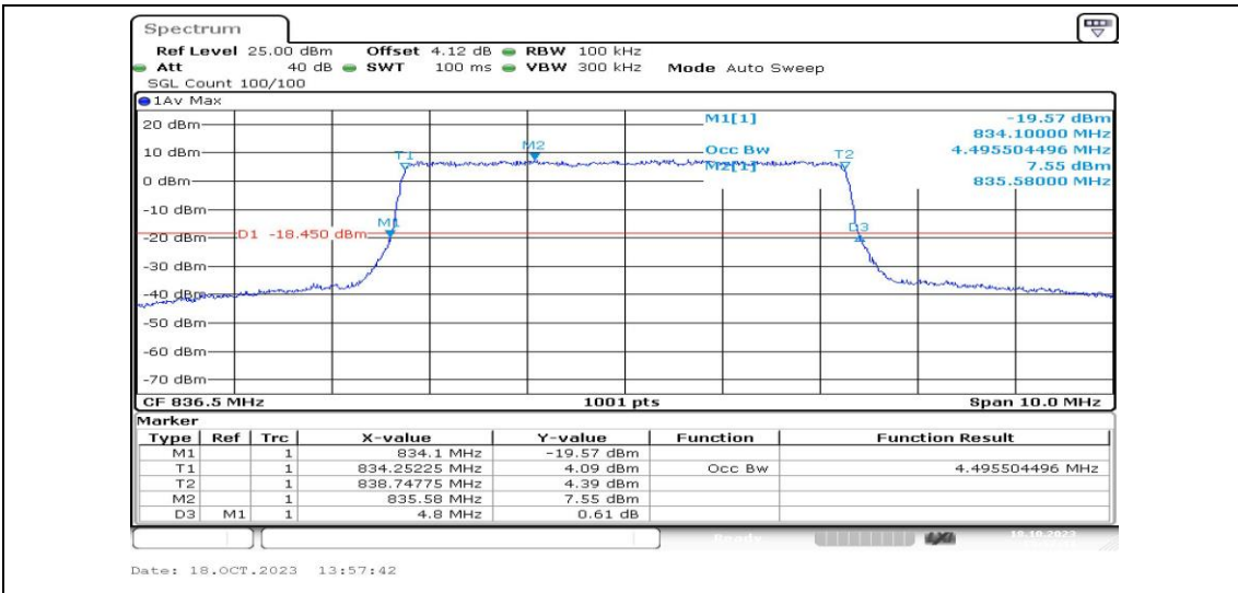
Band5-5MHz-QPSK-20525-25RB#0-PASS
