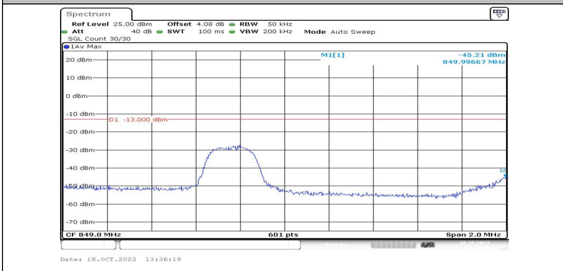
Band5-3MHz-16QAM-20635-1RB#0-PASS
