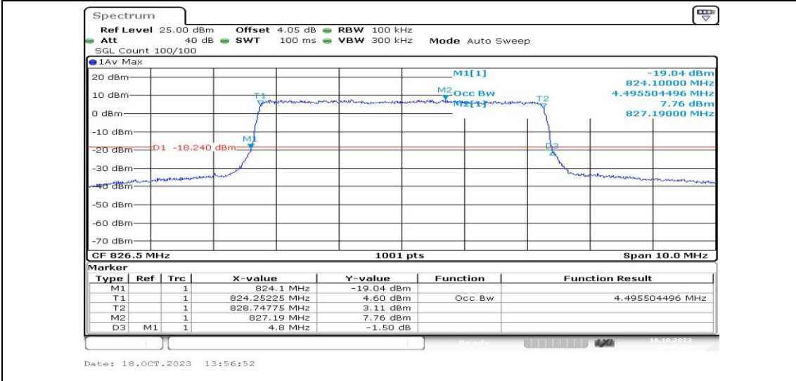
Band5-5MHz-QPSK-20425-25RB#0-PASS
