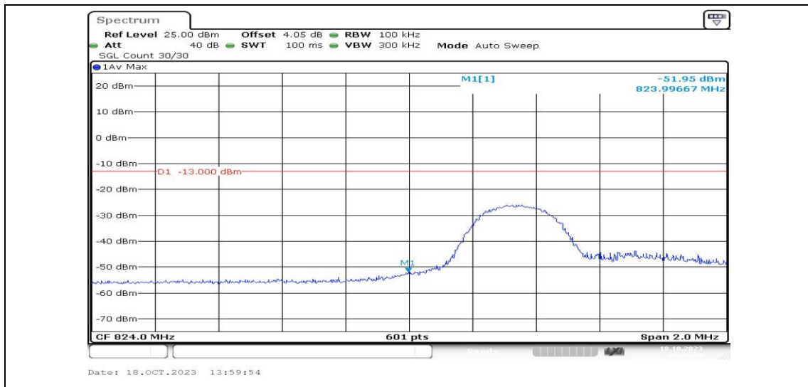
Band5-5MHz-QPSK-20425-1RB#24-PASS
