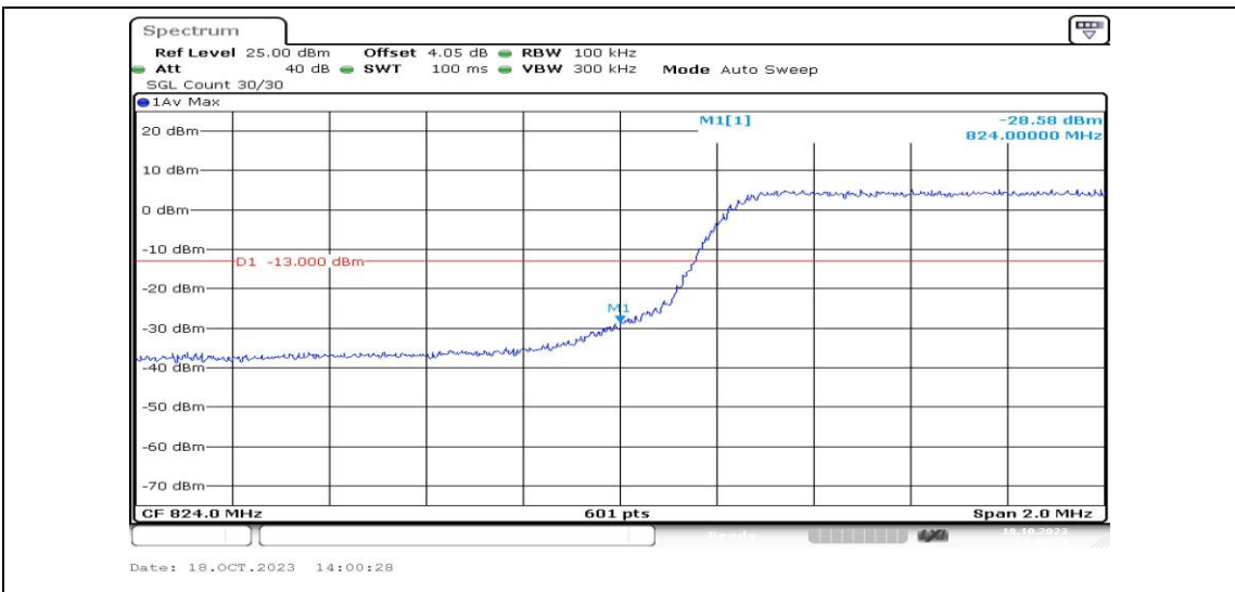
Band5-5MHz-16QAM-20425-25RB#0-PASS
