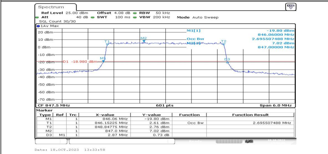
Band5-3MHz-QPSK-20635-15RB#0-PASS
