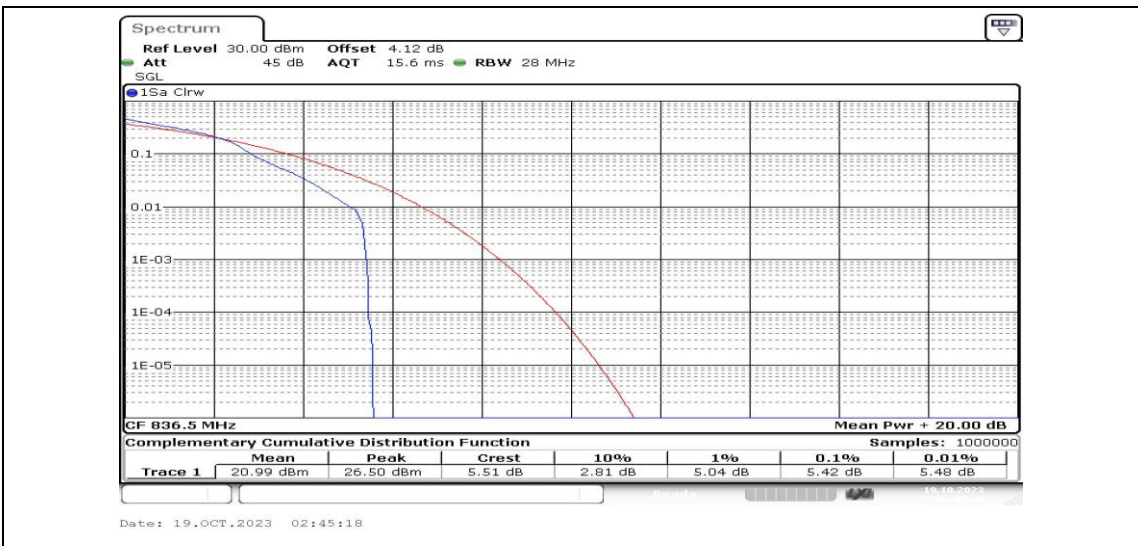
Band5-10MHz-16QAM-20525-1RB#0-PASS
