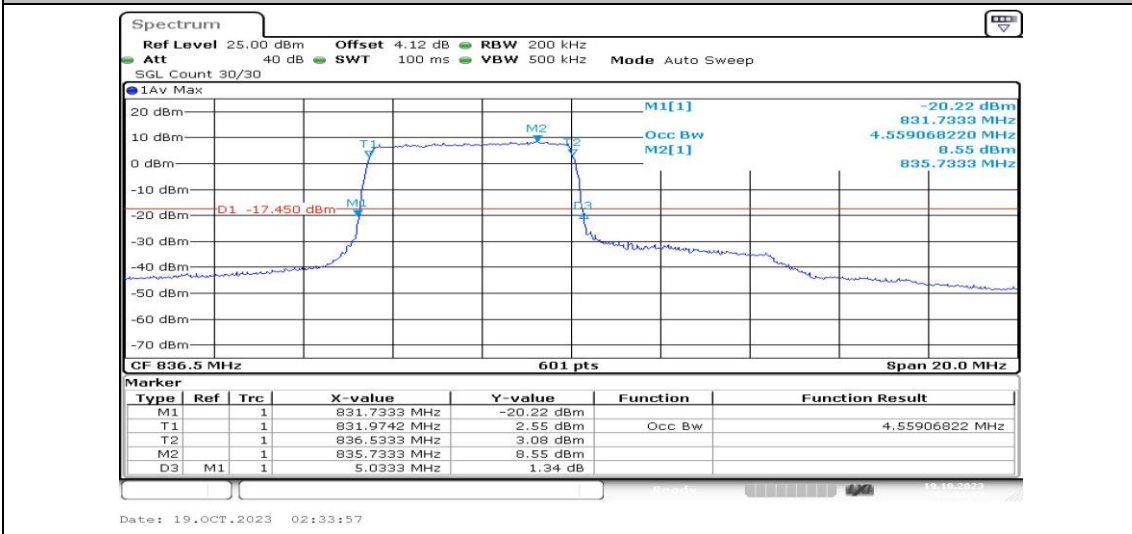
Band5-10MHz-16QAM-20525-25RB#0-PASS
