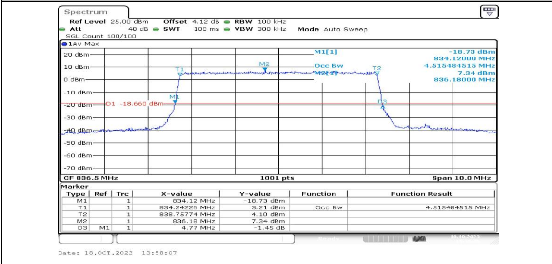
Band5-5MHz-16QAM-20525-25RB#0-PASS
