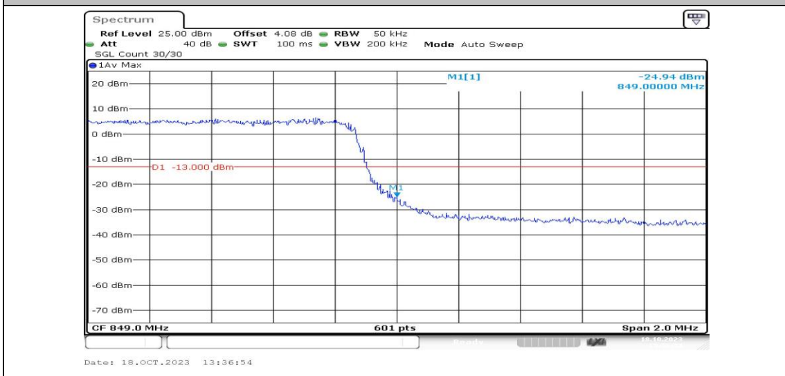
Band5-3MHz-QPSK-20635-15RB#0-PASS
