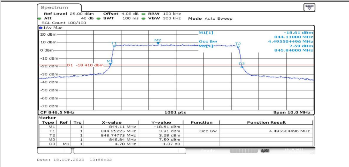
Band5-5MHz-QPSK-20625-25RB#0-PASS
