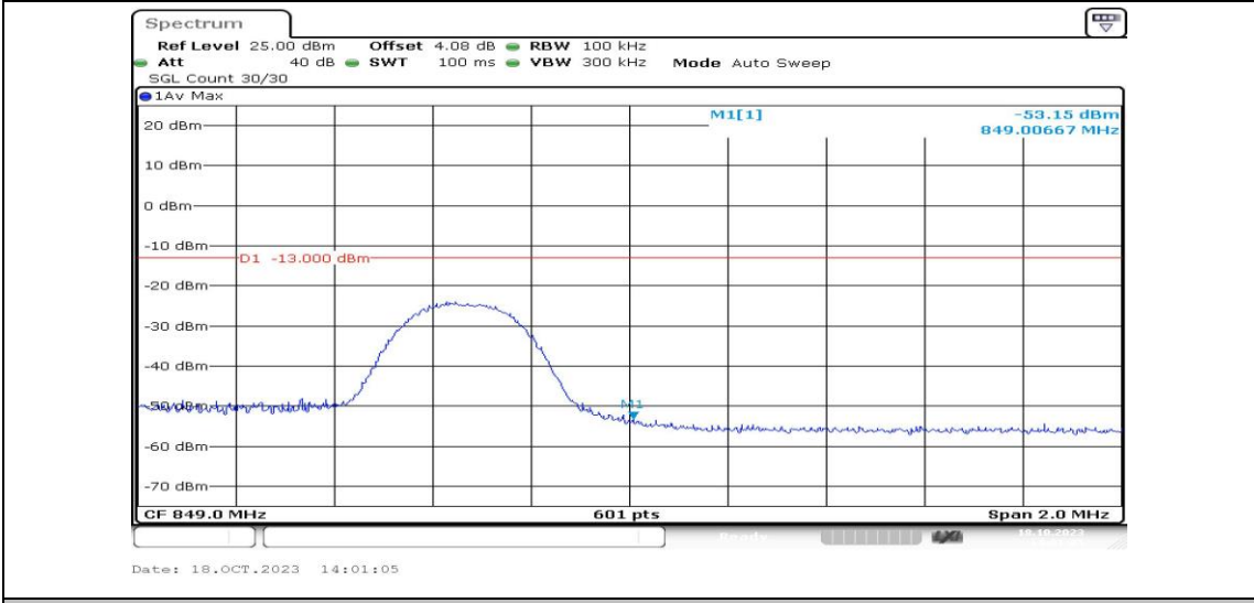
Band5-5MHz-16QAM-20625-1RB#0-PASS
