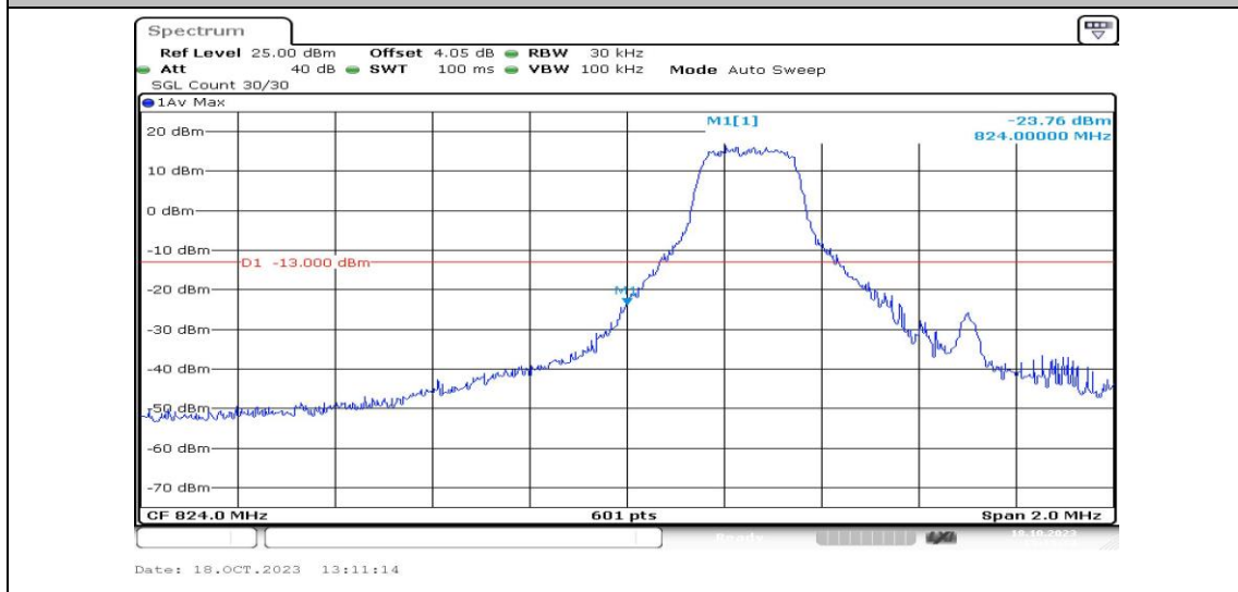
Band5-1.4MHz-16QAM-20407-1RB#0-PASS
