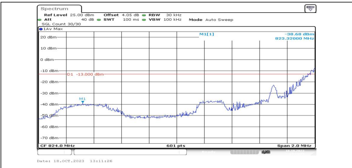
Band5-1.4MHz-QPSK-20407-1RB#5-PASS
