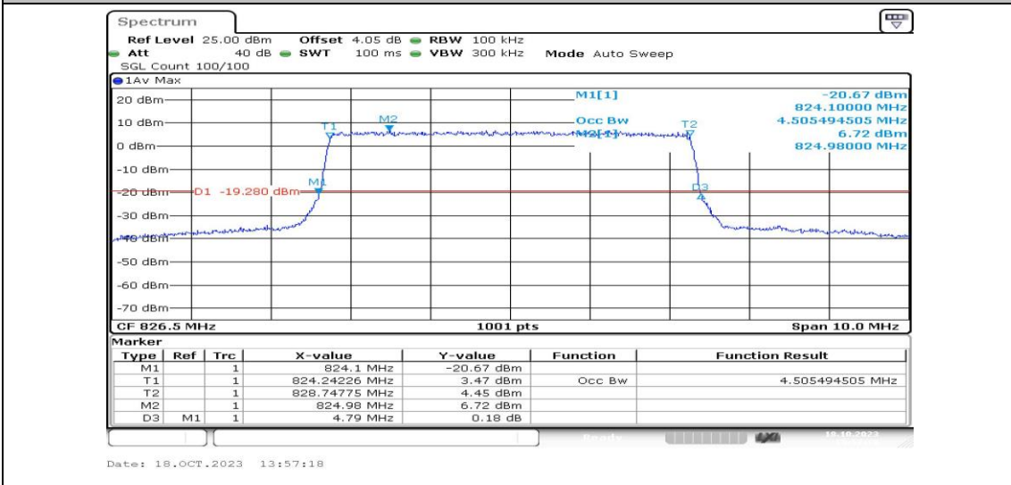
Band5-5MHz-16QAM-20425-25RB#0-PASS
