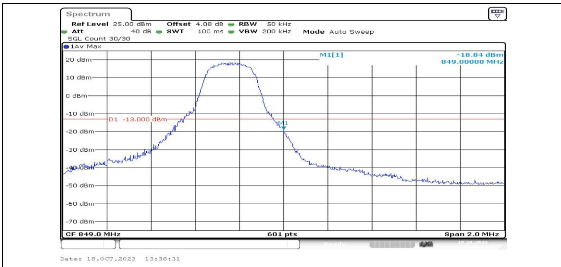
Band5-3MHz-QPSK-20635-1RB#14-PASS
