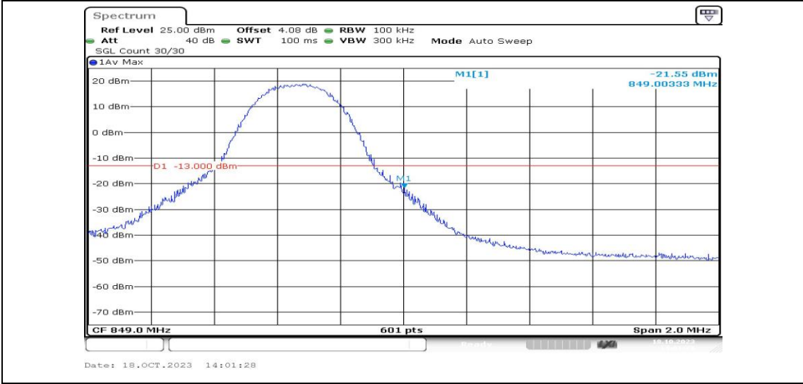
Band5-5MHz-16QAM-20625-1RB#24-PASS
