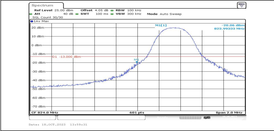
Band5-5MHz-QPSK-20425-1RB#0-PASS
