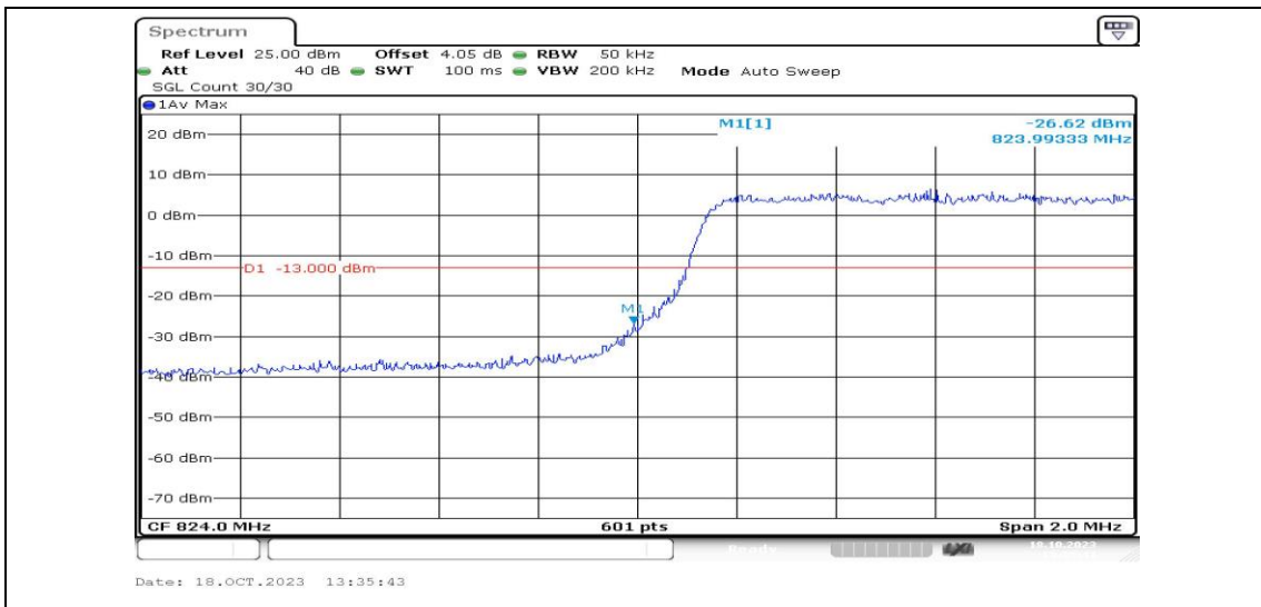
Band5-3MHz-16QAM-20415-15RB#0-PASS
