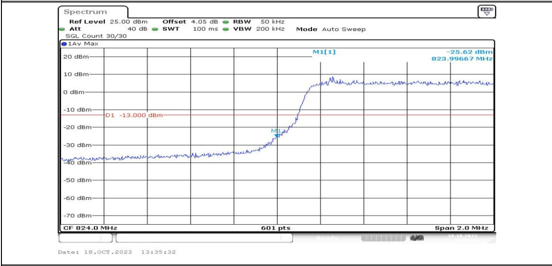
Band5-3MHz-QPSK-20415-15RB#0-PASS
