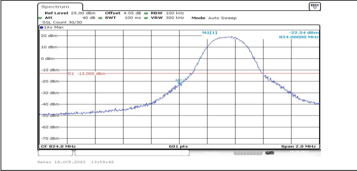
Band5-5MHz-16QAM-20425-1RB#0-PASS
