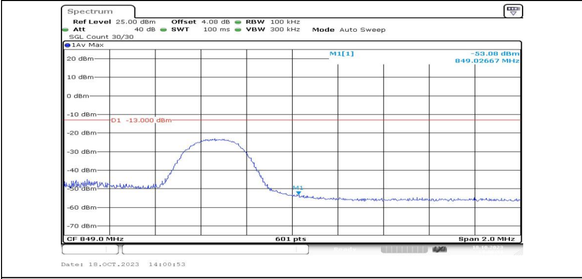
Band5-5MHz-QPSK-20625-1RB#0-PASS
