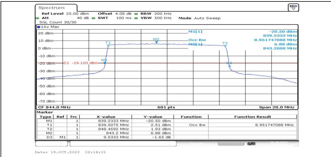
Band5-10MHz-QPSK-20600-50RB#0-PASS
