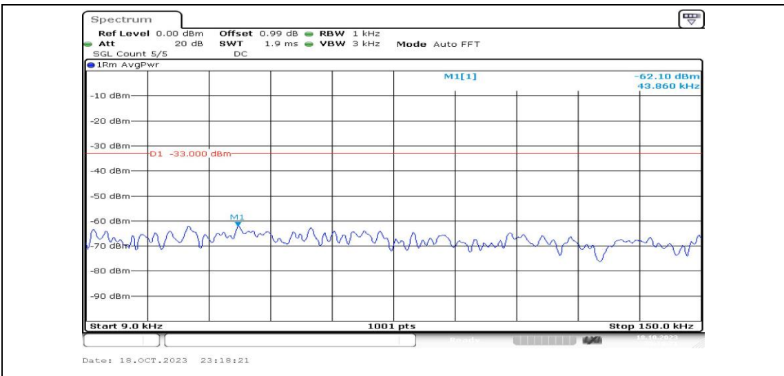
Band4-10MHz-QPSK-20350-1RB#0-Range1:0.009~0.15MHz-PASS
