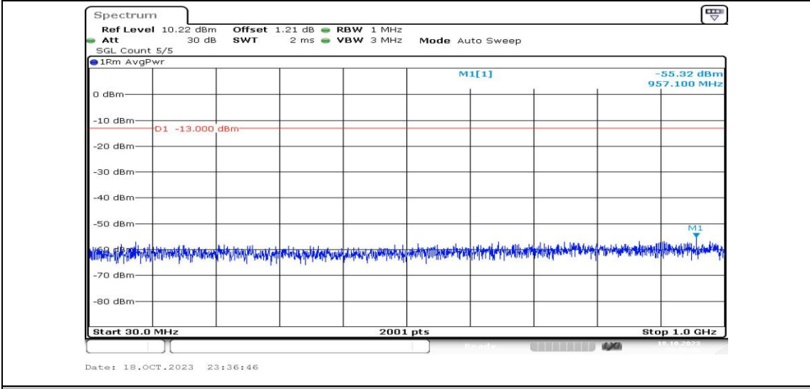
Band4-15MHz-QPSK-20325-1RB#0-Range3:30~1000MHz-PASS
