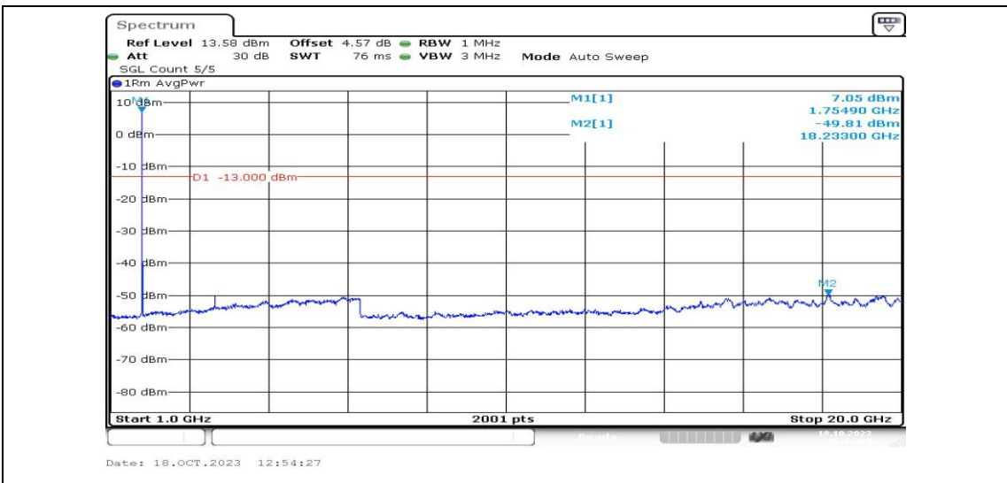
Band4-5MHz-16QAM-20375-1RB#0-Range4:1000~20000MHz-PASS
