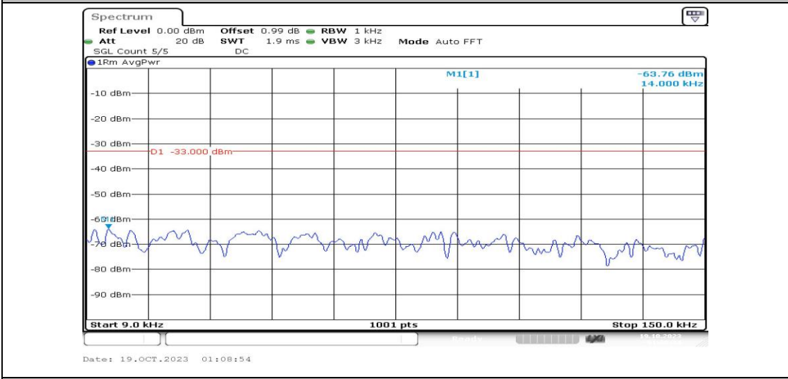
Band4-15MHz-16QAM-20175-1RB#0-Range1:0.009~0.15MHz-PASS
