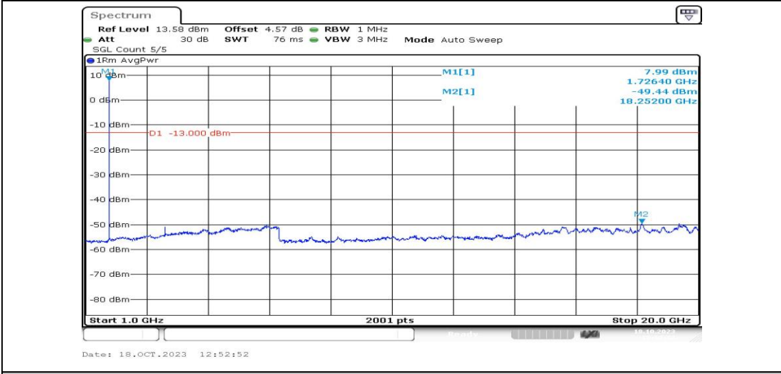
Band4-5MHz-16QAM-20175-1RB#0-Range4:1000~20000MHz-PASS
