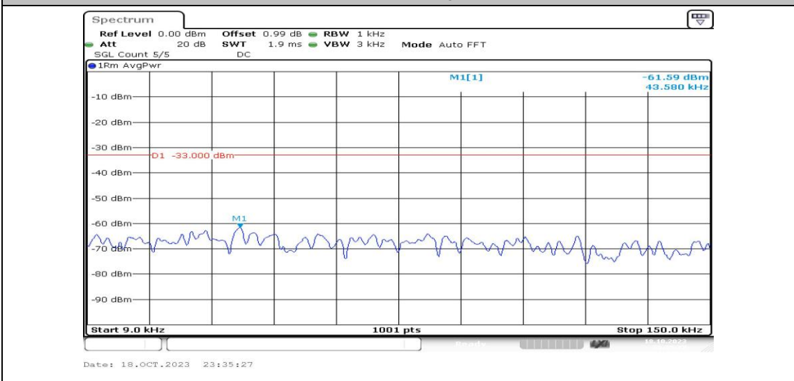
Band4-15MHz-QPSK-20175-1RB#0-Range1:0.009~0.15MHz-PASS
