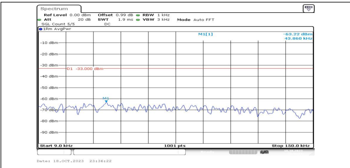
Band4-15MHz-QPSK-20325-1RB#0-Range1:0.009~0.15MHz-PASS
