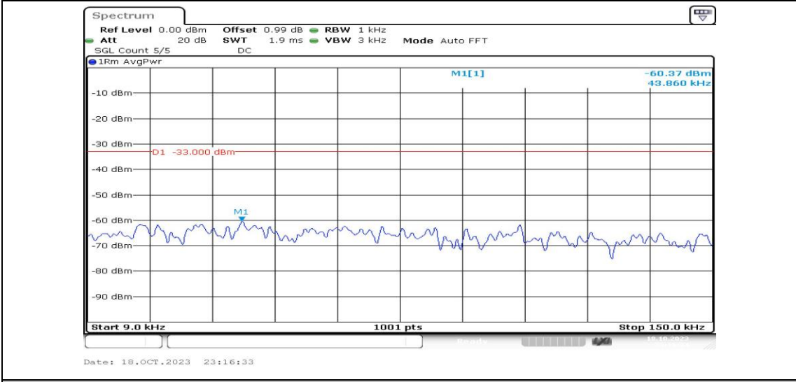
Band4-10MHz-QPSK-20000-1RB#0-Range1:0.009~0.15MHz-PASS
