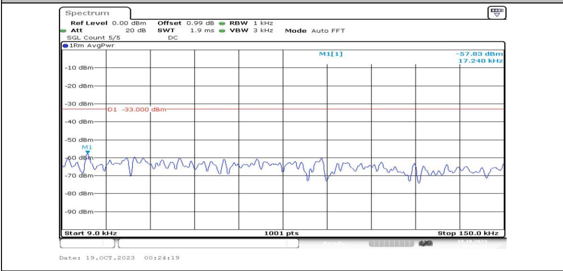
Band4-20MHz-QPSK-20175-1RB#0-Range1:0.009~0.15MHz-PASS
