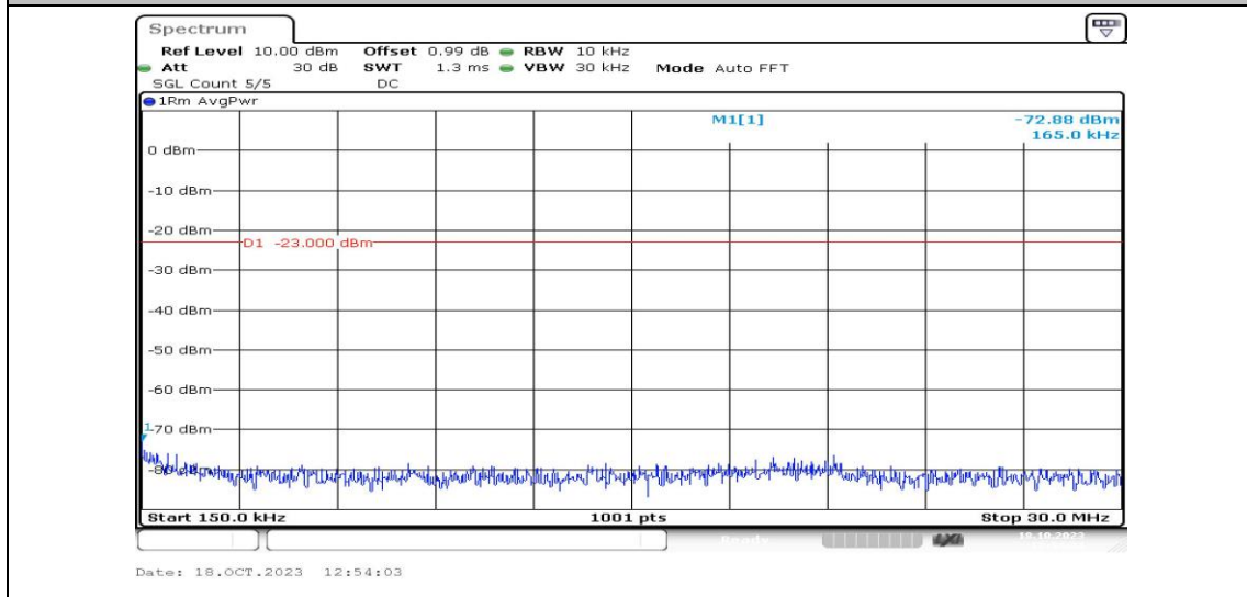
Band4-5MHz-16QAM-20375-1RB#0-Range2:0.15~30MHz-PASS
