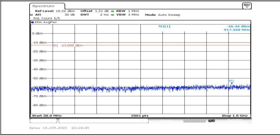
Band4-10MHz-QPSK-20350-1RB#0-Range3:30~1000MHz-PASS
