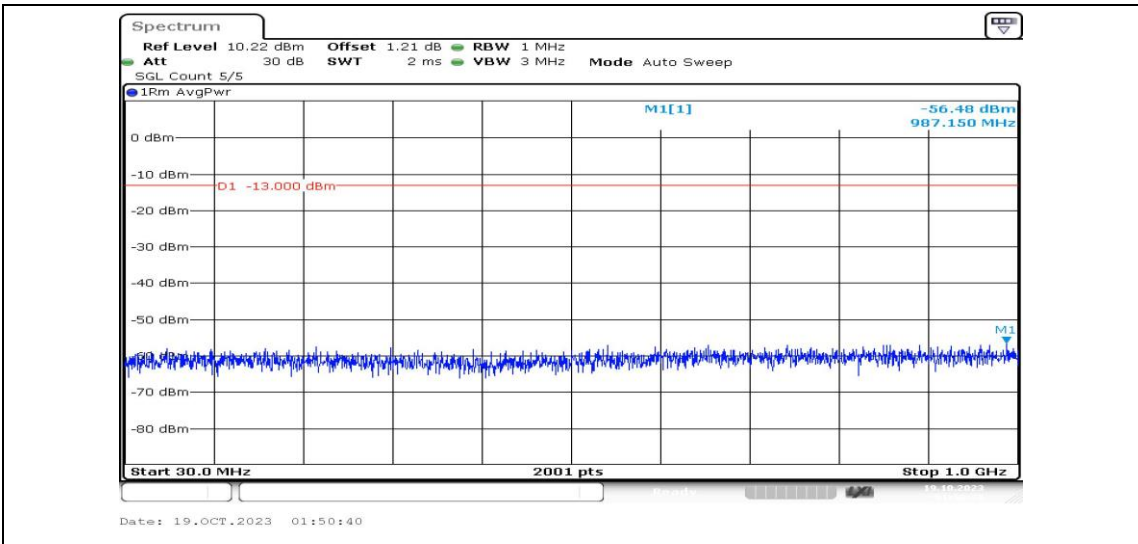
Band4-20MHz-16QAM-20050-1RB#0-Range3:30~1000MHz-PASS
