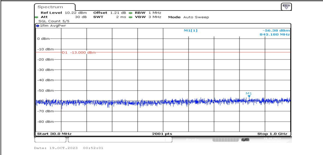
Band4-10MHz-16QAM-20175-1RB#0-Range3:30~1000MHz-PASS
