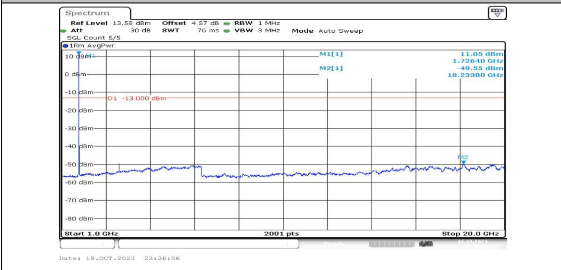
Band4-15MHz-QPSK-20175-1RB#0-Range4:1000~20000MHz-PASS
