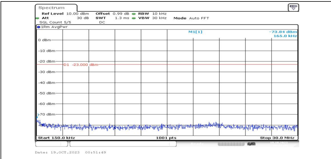
Band4-10MHz-16QAM-20175-1RB#0-Range2:0.15~30MHz-PASS
