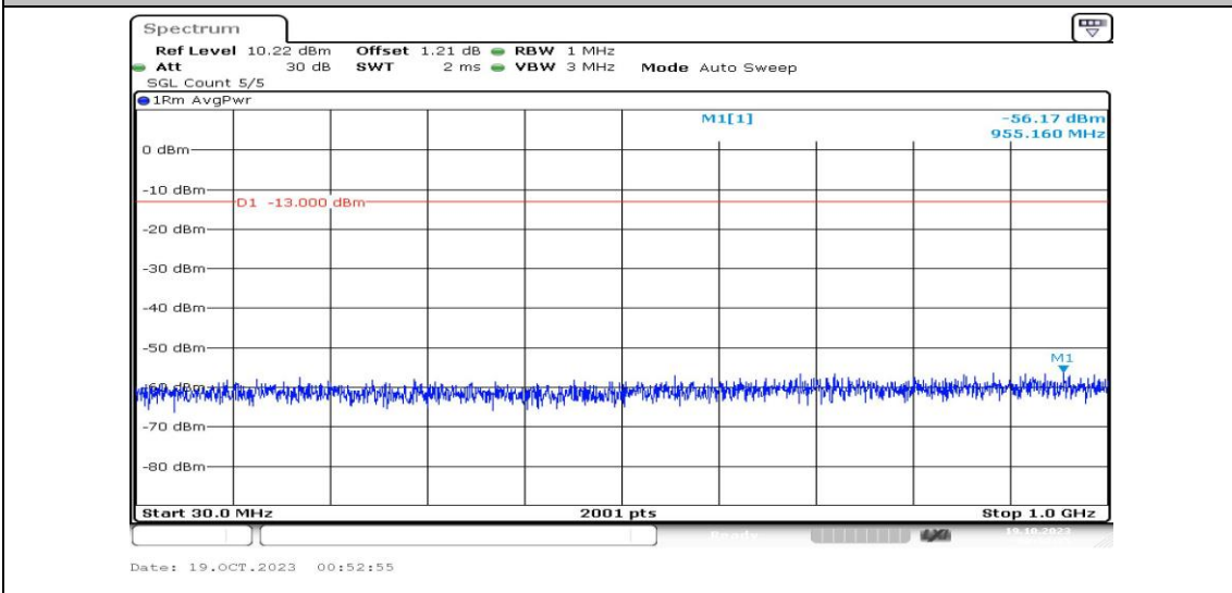
Band4-10MHz-16QAM-20350-1RB#0-Range3:30~1000MHz-PASS
