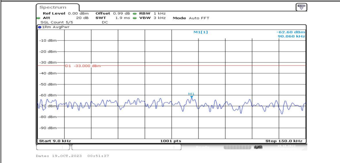
Band4-10MHz-16QAM-20175-1RB#0-Range1:0.009~0.15MHz-PASS
