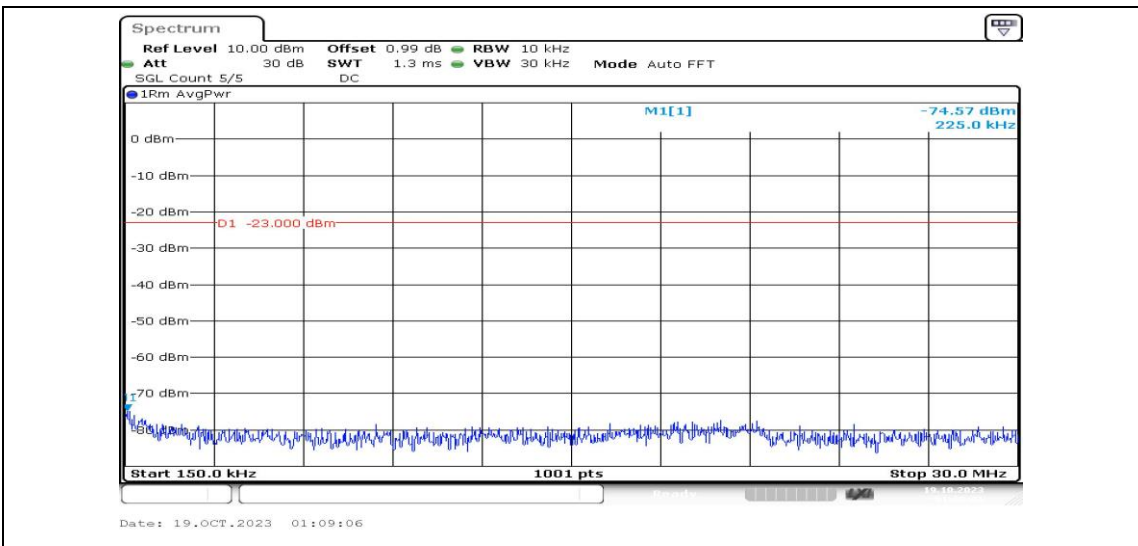
Band4-15MHz-16QAM-20175-1RB#0-Range2:0.15~30MHz-PASS
