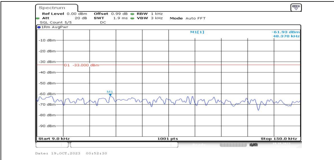
Band4-10MHz-16QAM-20350-1RB#0-Range1:0.009~0.15MHz-PASS
