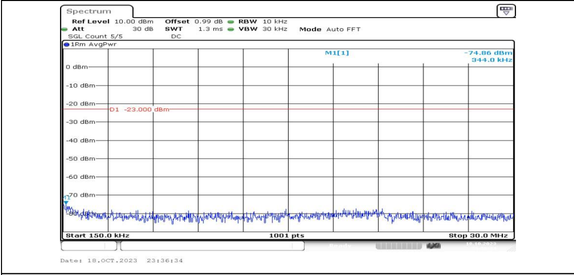
Band4-15MHz-QPSK-20325-1RB#0-Range2:0.15~30MHz-PASS
