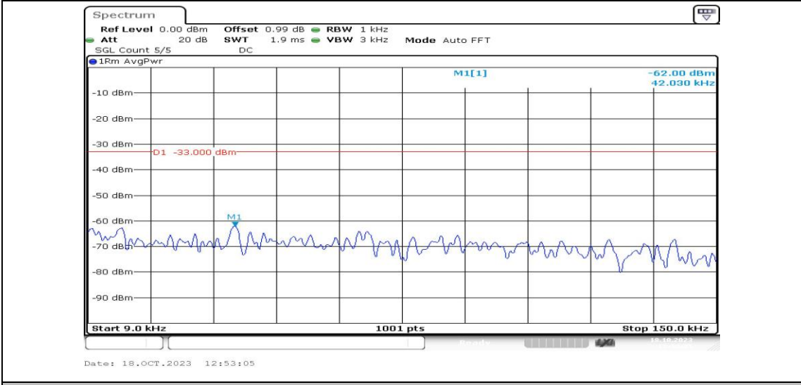
Band4-5MHz-QPSK-20375-1RB#0-Range1:0.009~0.15MHz-PASS
