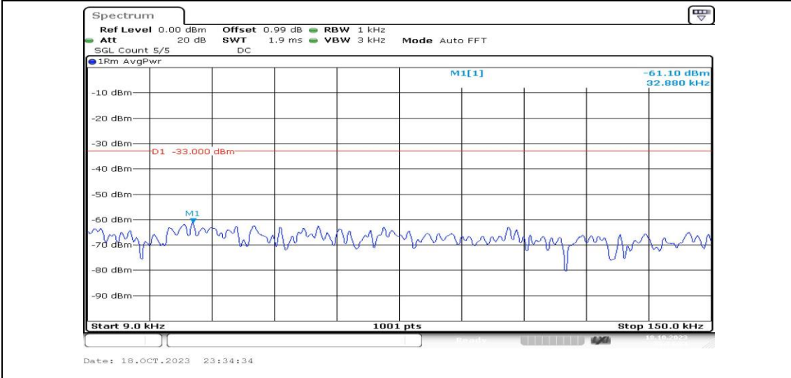
Band4-15MHz-QPSK-20025-1RB#0-Range1:0.009~0.15MHz-PASS
