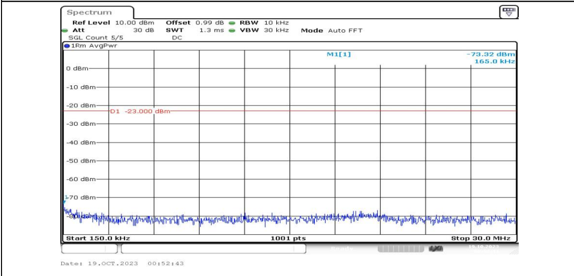
Band4-10MHz-16QAM-20350-1RB#0-Range2:0.15~30MHz-PASS
