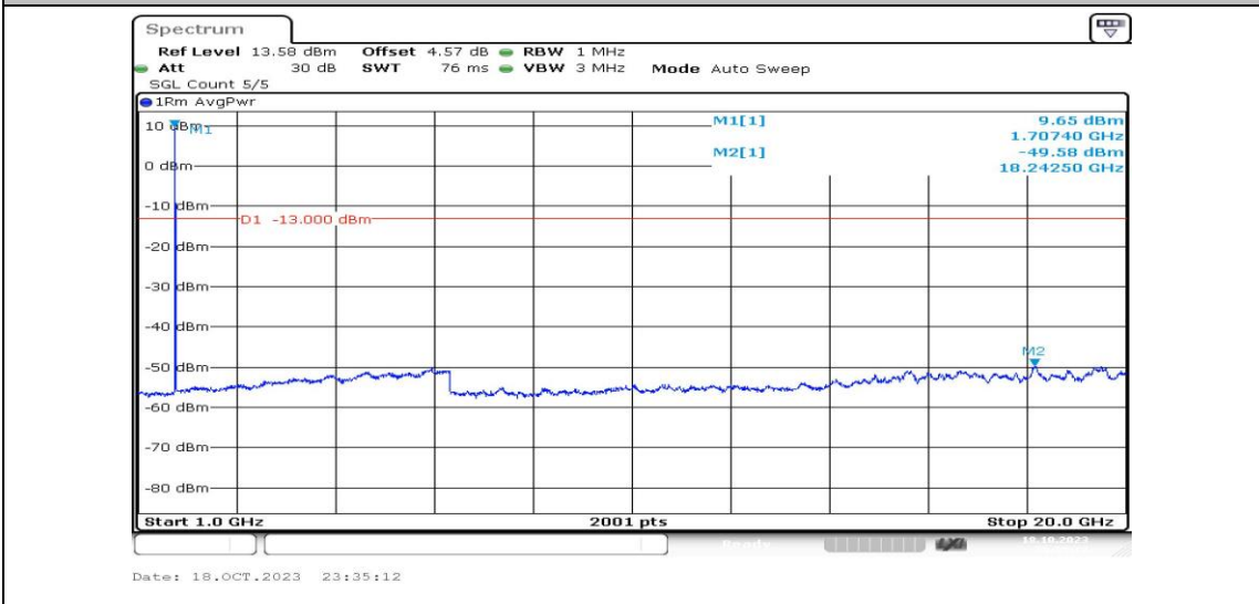
Band4-15MHz-QPSK-20025-1RB#0-Range4:1000~20000MHz-PASS
