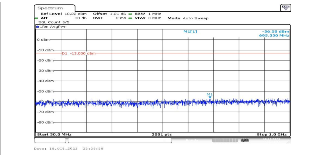
Band4-15MHz-QPSK-20025-1RB#0-Range3:30~1000MHz-PASS
