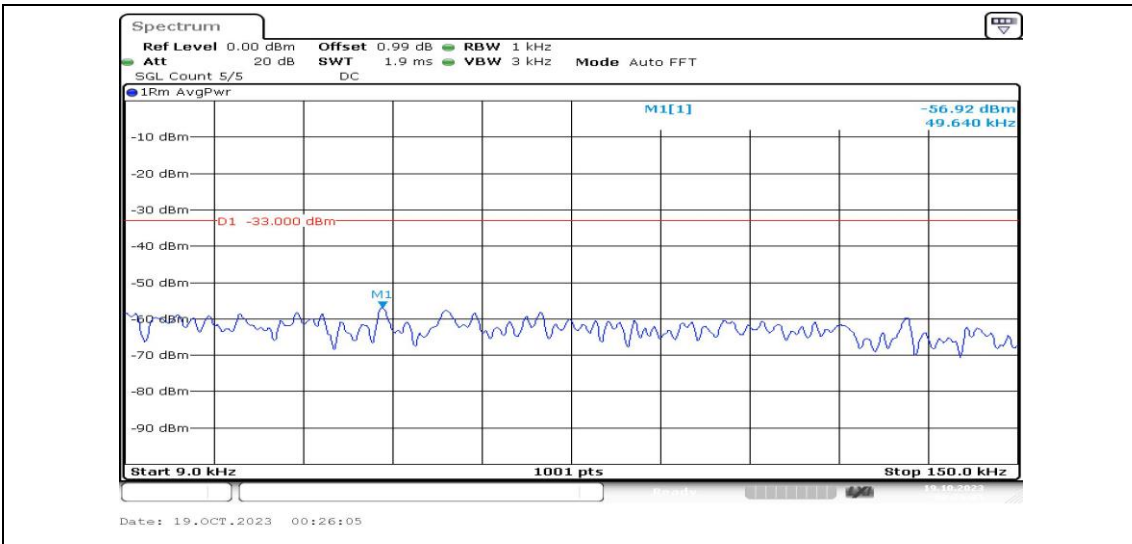
Band4-20MHz-QPSK-20300-1RB#0-Range1:0.009~0.15MHz-PASS
