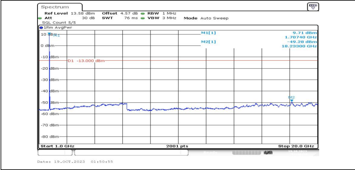
Band4-20MHz-16QAM-20050-1RB#0-Range4:1000~20000MHz-PASS
