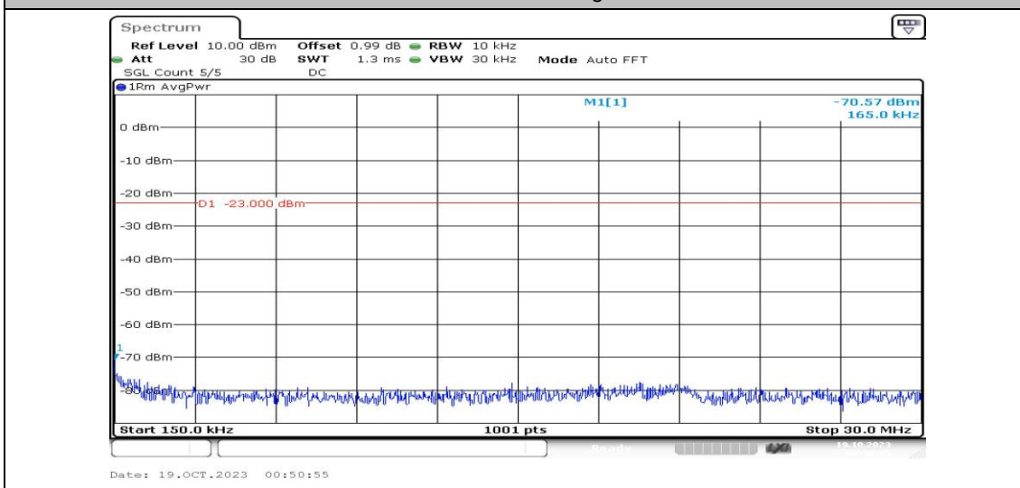
Band4-10MHz-16QAM-20000-1RB#0-Range2:0.15~30MHz-PASS
