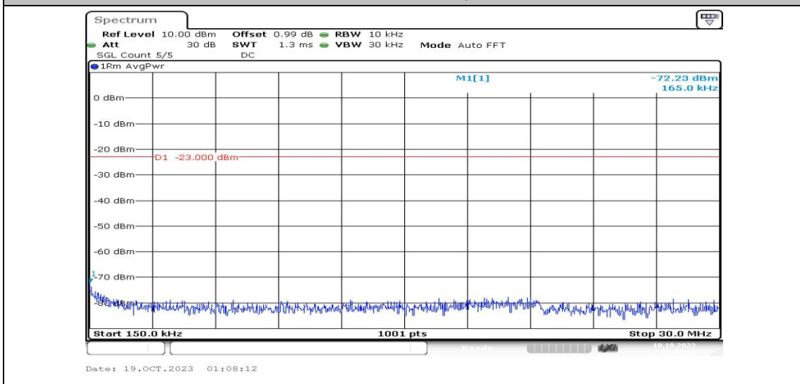
Band4-15MHz-16QAM-20025-1RB#0-Range2:0.15~30MHz-PASS
