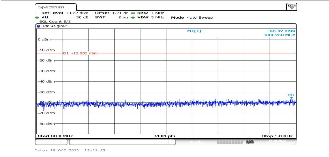
Band4-5MHz-QPSK-20375-1RB#0-Range3:30~1000MHz-PASS
