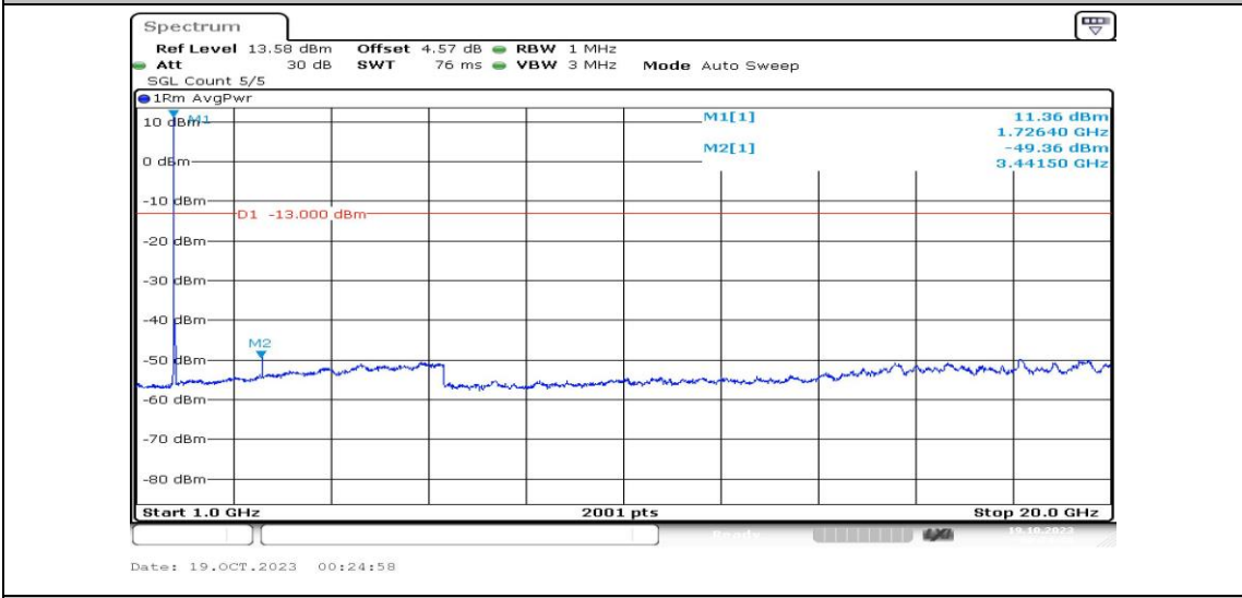
Band4-20MHz-QPSK-20175-1RB#0-Range4:1000~20000MHz-PASS
