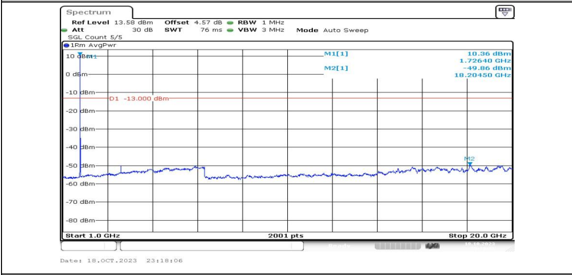
Band4-10MHz-QPSK-20175-1RB#0-Range4:1000~20000MHz-PASS
