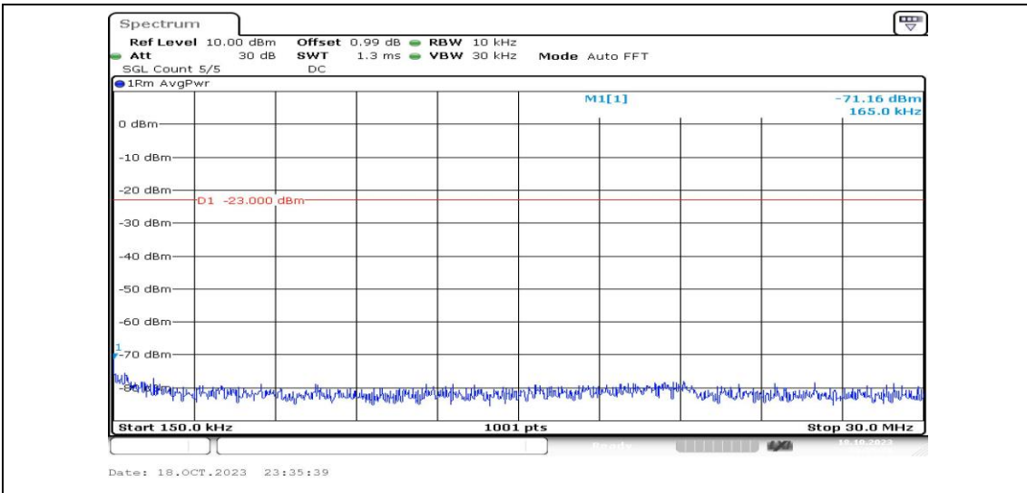
Band4-15MHz-QPSK-20175-1RB#0-Range2:0.15~30MHz-PASS
