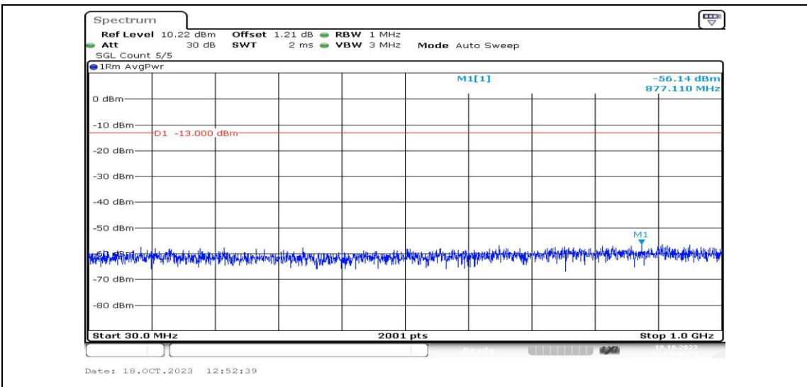
Band4-5MHz-16QAM-20175-1RB#0-Range3:30~1000MHz-PASS
