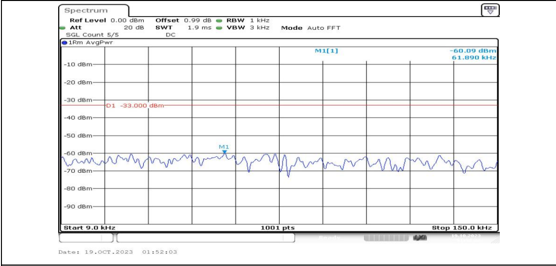
Band4-20MHz-16QAM-20175-1RB#0-Range1:0.009~0.15MHz-PASS
