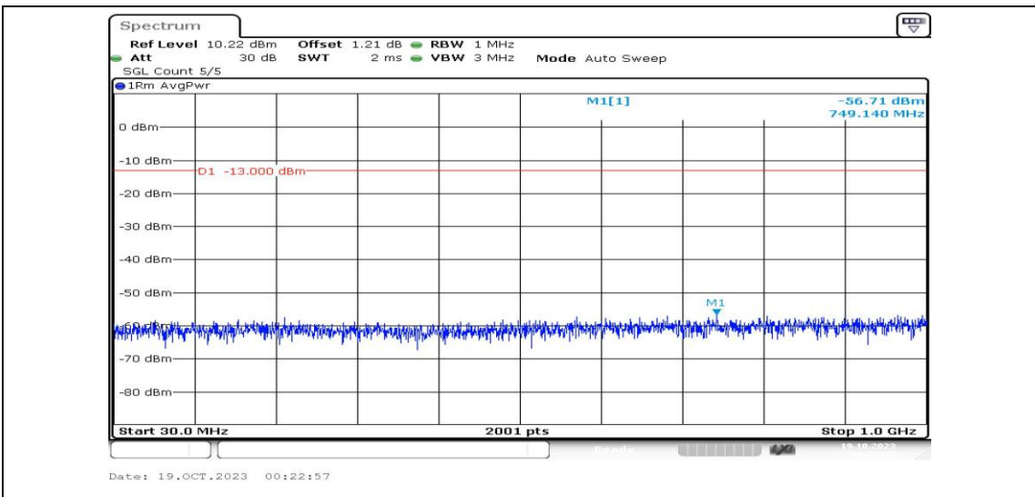
Band4-20MHz-QPSK-20050-1RB#0-Range3:30~1000MHz-PASS
