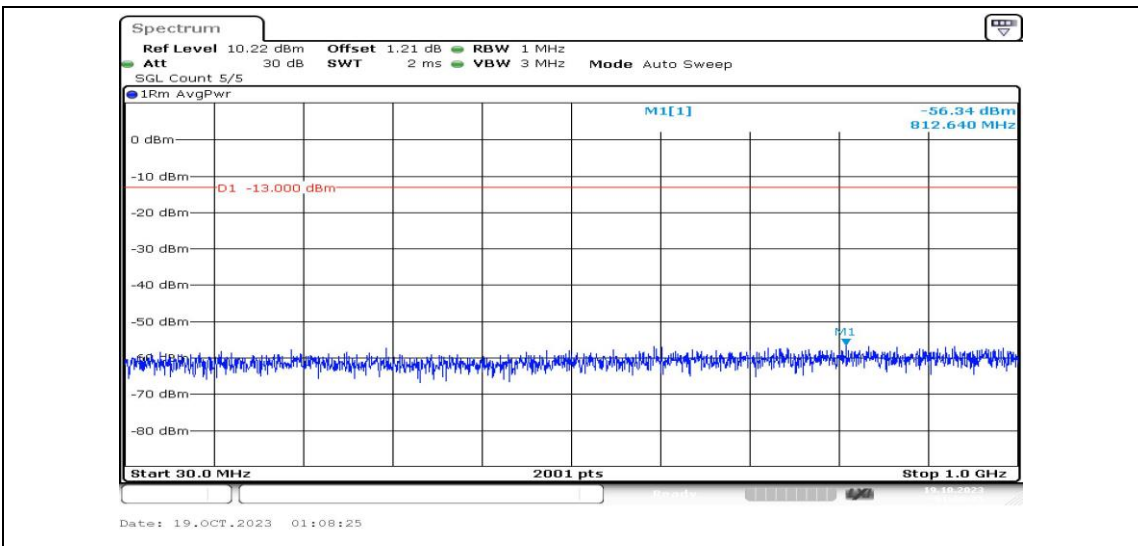
Band4-15MHz-16QAM-20025-1RB#0-Range3:30~1000MHz-PASS
