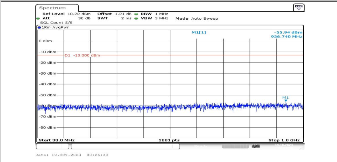
Band4-20MHz-QPSK-20300-1RB#0-Range3:30~1000MHz-PASS
