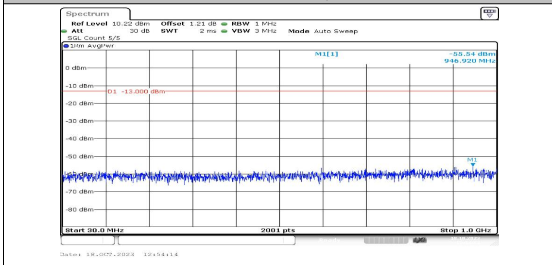
Band4-5MHz-16QAM-20375-1RB#0-Range3:30~1000MHz-PASS
