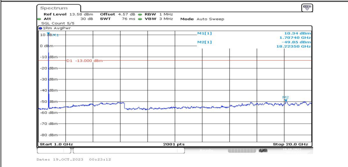
Band4-20MHz-QPSK-20050-1RB#0-Range4:1000~20000MHz-PASS
