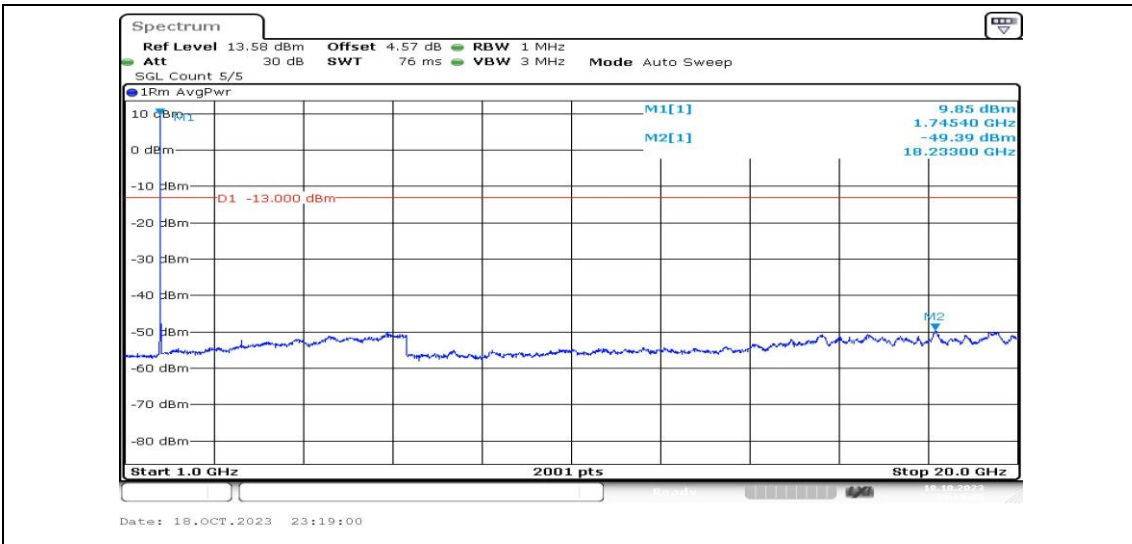
Band4-10MHz-QPSK-20350-1RB#0-Range4:1000~20000MHz-PASS
