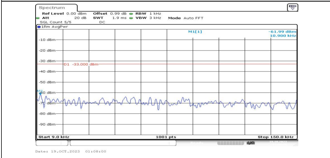
Band4-15MHz-16QAM-20025-1RB#0-Range1:0.009~0.15MHz-PASS
