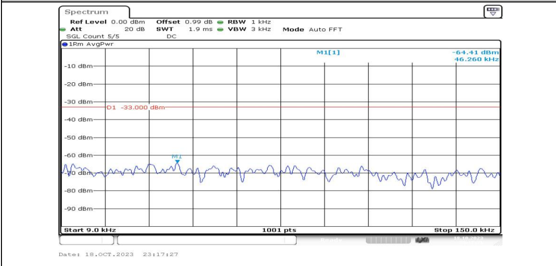
Band4-10MHz-QPSK-20175-1RB#0-Range1:0.009~0.15MHz-PASS
