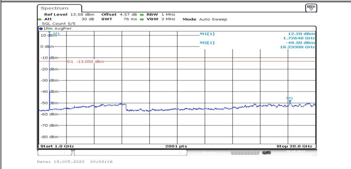
Band4-10MHz-16QAM-20175-1RB#0-Range4:1000~20000MHz-PASS
