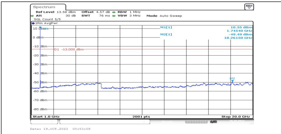
Band4-10MHz-16QAM-20350-1RB#0-Range4:1000~20000MHz-PASS
