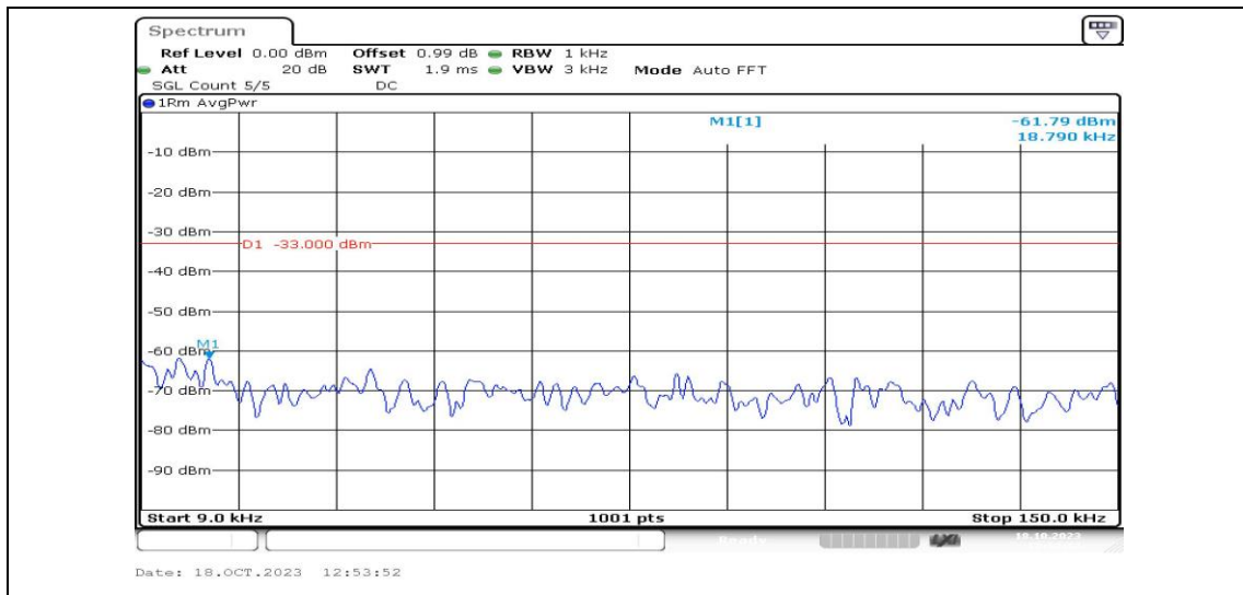
Band4-5MHz-16QAM-20375-1RB#0-Range1:0.009~0.15MHz-PASS
