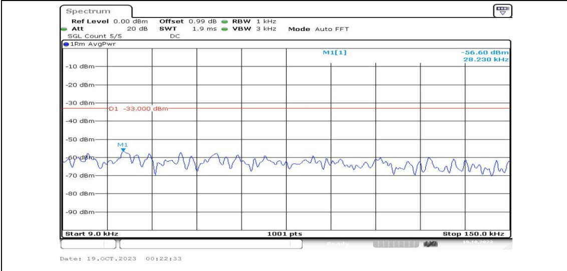
Band4-20MHz-QPSK-20050-1RB#0-Range1:0.009~0.15MHz-PASS
