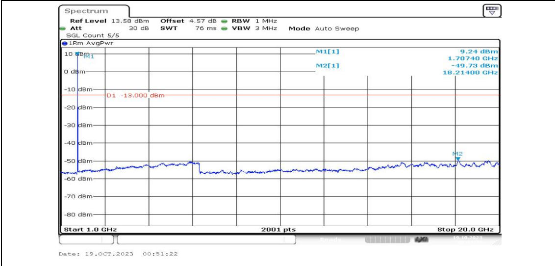
Band4-10MHz-16QAM-20000-1RB#0-Range4:1000~20000MHz-PASS
