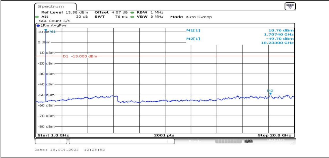
Band4-3MHz-QPSK-19965-1RB#0-Range4:1000~20000MHz-PASS
