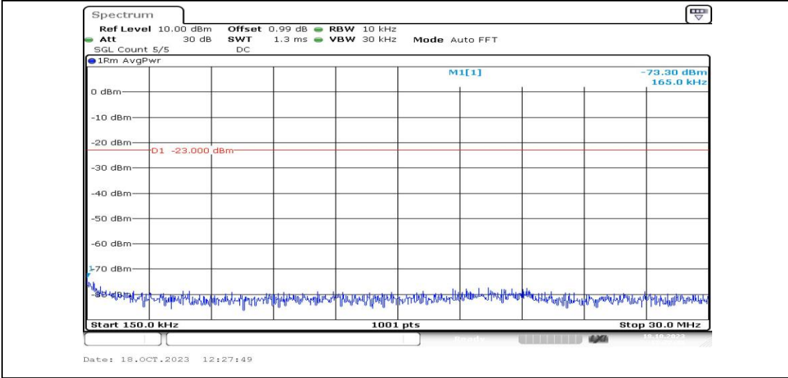
Band4-3MHz-16QAM-20175-1RB#0-Range2:0.15~30MHz-PASS
