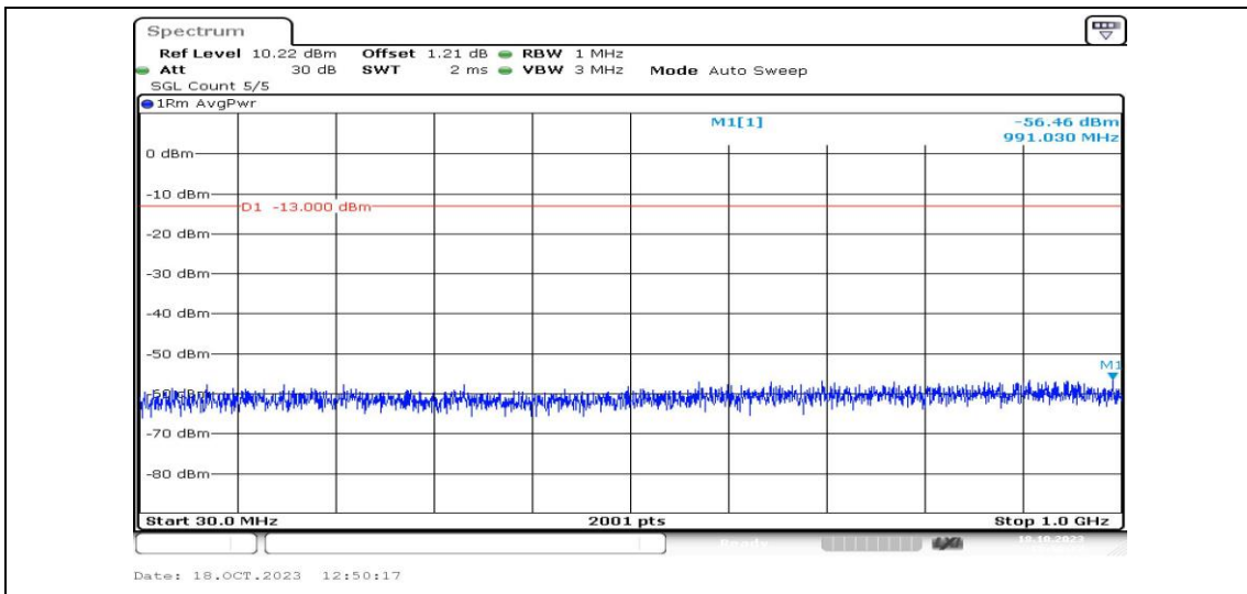
Band4-5MHz-QPSK-19975-1RB#0-Range3:30~1000MHz-PASS
