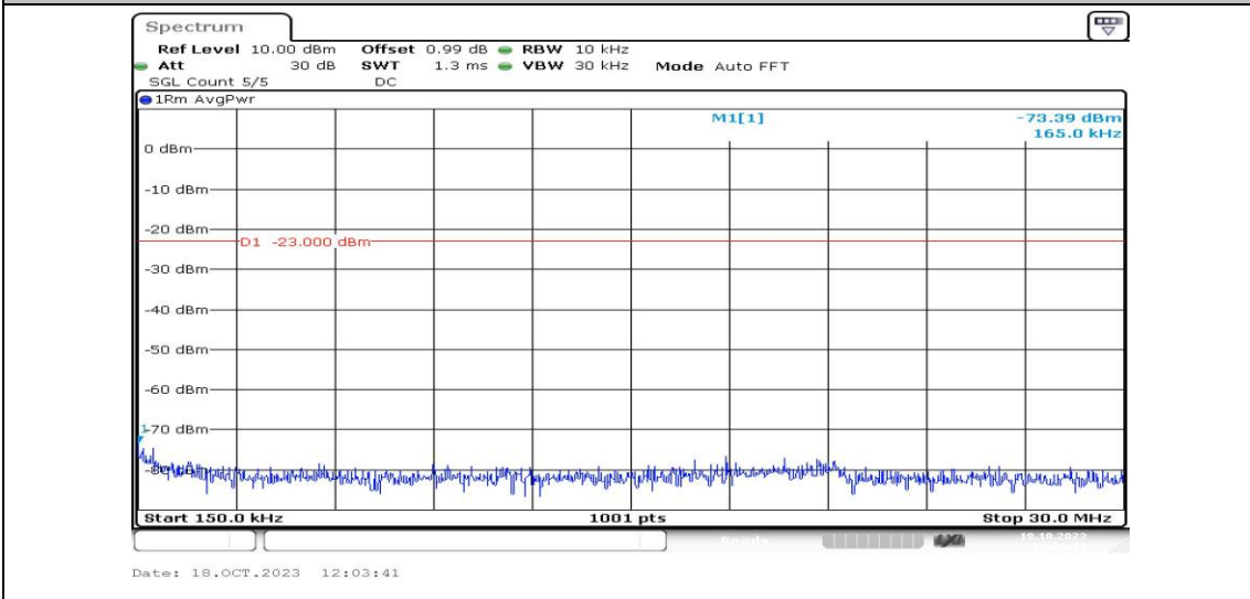
Band4-1.4MHz-16QAM-20175-1RB#0-Range2:0.15~30MHz-PASS
