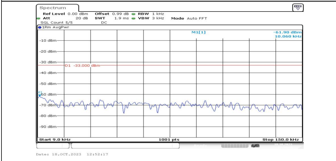
Band4-5MHz-16QAM-20175-1RB#0-Range1:0.009~0.15MHz-PASS
