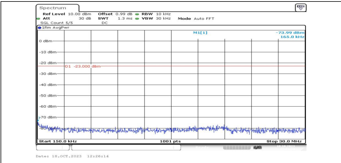
Band4-3MHz-16QAM-19965-1RB#0-Range2:0.15~30MHz-PASS
