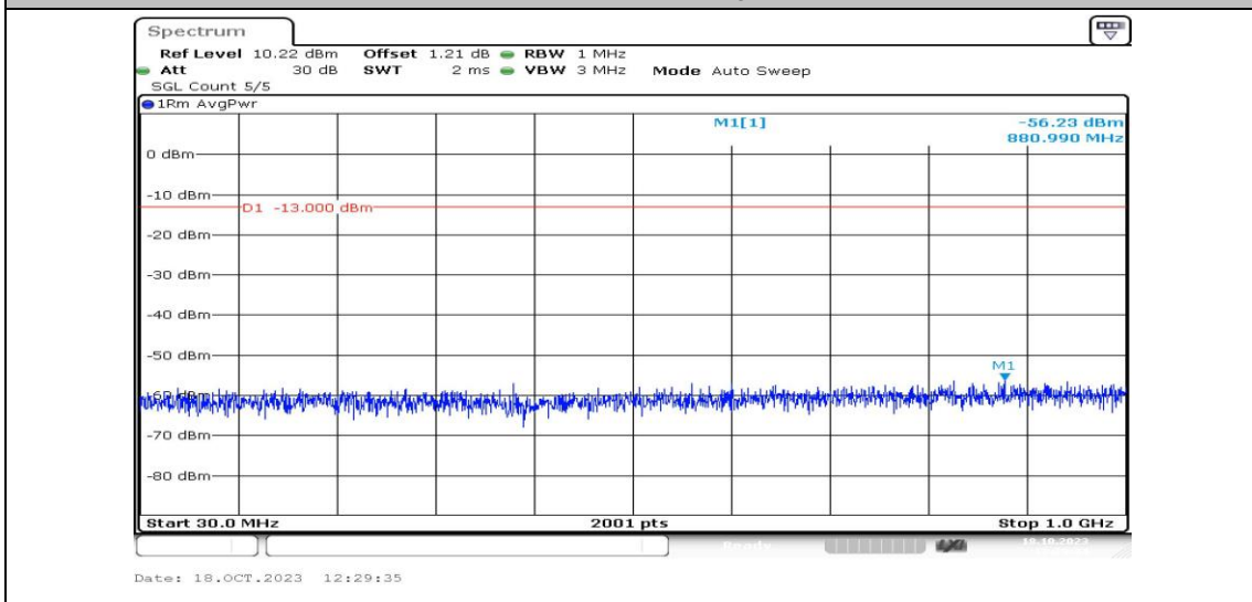
Band4-3MHz-16QAM-20385-1RB#0-Range3:30~1000MHz-PASS
