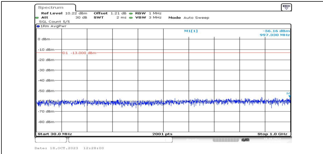
Band4-3MHz-16QAM-20175-1RB#0-Range3:30~1000MHz-PASS
