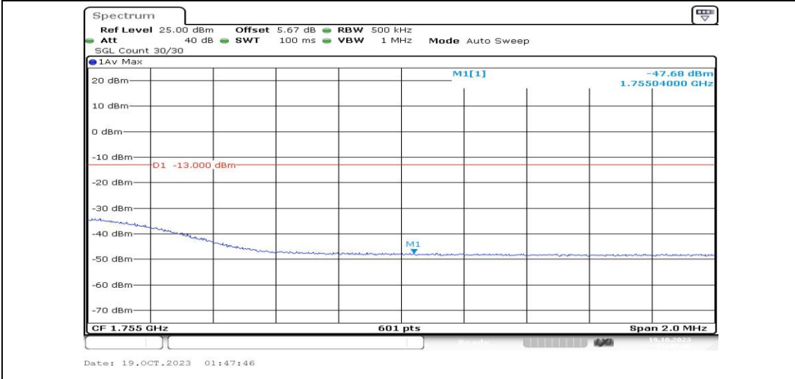
Band4-20MHz-16QAM-20300-1RB#0-PASS
