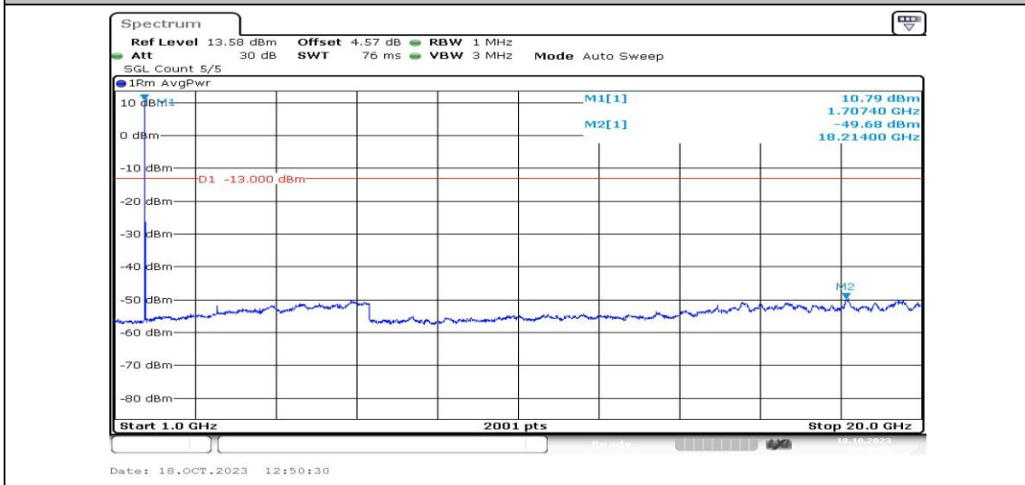
Band4-5MHz-QPSK-19975-1RB#0-Range4:1000~20000MHz-PASS
