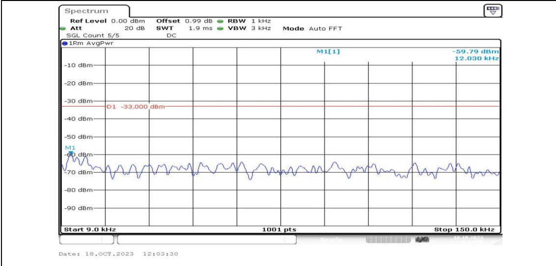
Band4-1.4MHz-16QAM-20175-1RB#0-Range1:0.009~0.15MHz-PASS
