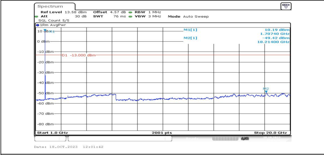
Band4-1.4MHz-QPSK-19957-1RB#0-Range4:1000~20000MHz-PASS
