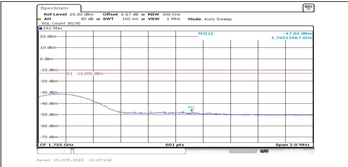
Band4-15MHz-16QAM-20325-1RB#0-PASS
