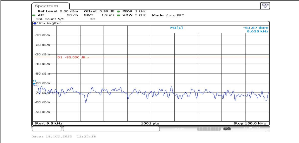
Band4-3MHz-16QAM-20175-1RB#0-Range1:0.009~0.15MHz-PASS
