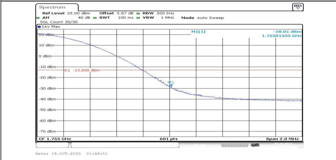
Band4-20MHz-16QAM-20300-1RB#99-PASS
