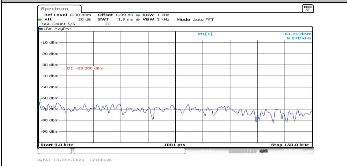
Band4-3MHz-QPSK-20385-1RB#0-Range1:0.009~0.15MHz-PASS
