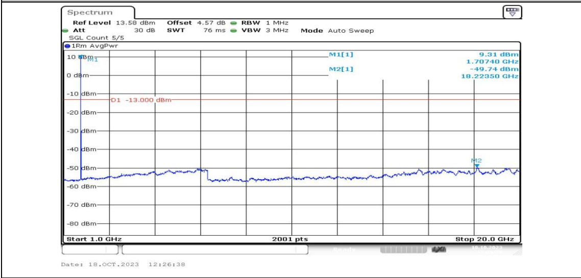
Band4-3MHz-16QAM-19965-1RB#0-Range4:1000~20000MHz-PASS
