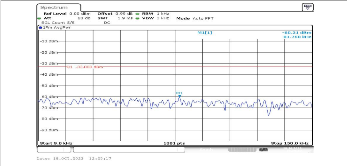
Band4-3MHz-QPSK-19965-1RB#0-Range1:0.009~0.15MHz-PASS
