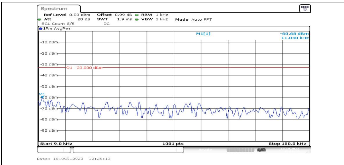
Band4-3MHz-16QAM-20385-1RB#0-Range1:0.009~0.15MHz-PASS
