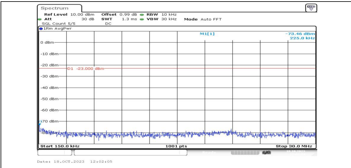
Band4-1.4MHz-16QAM-19957-1RB#0-Range2:0.15~30MHz-PASS
