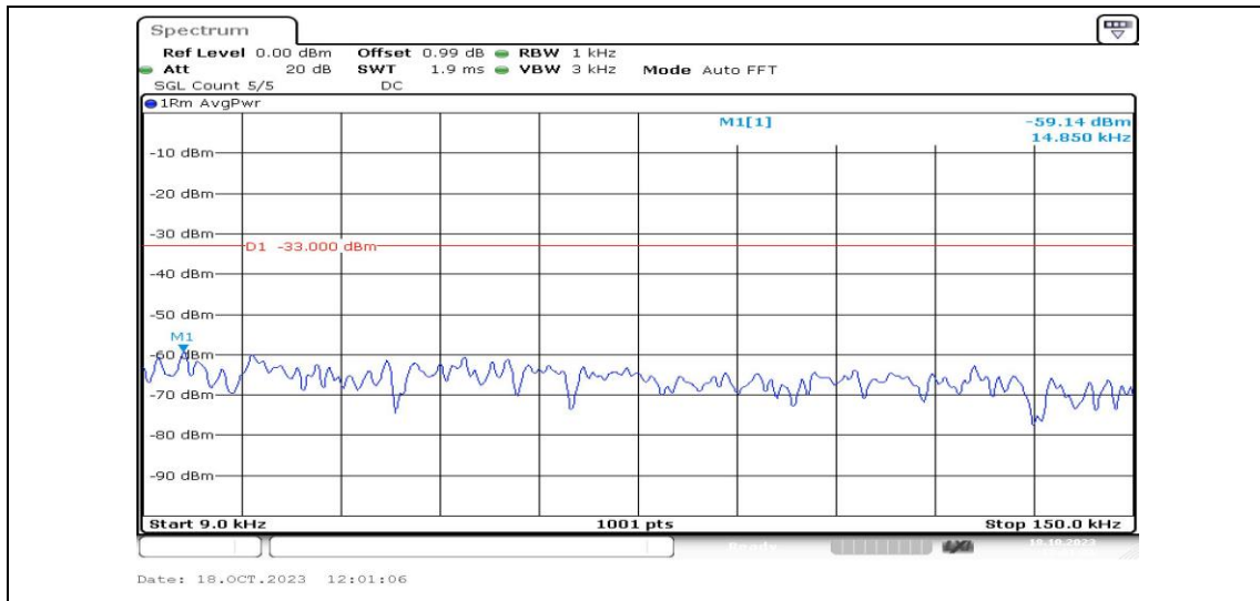
Band4-1.4MHz-QPSK-19957-1RB#0-Range1:0.009~0.15MHz-PASS
