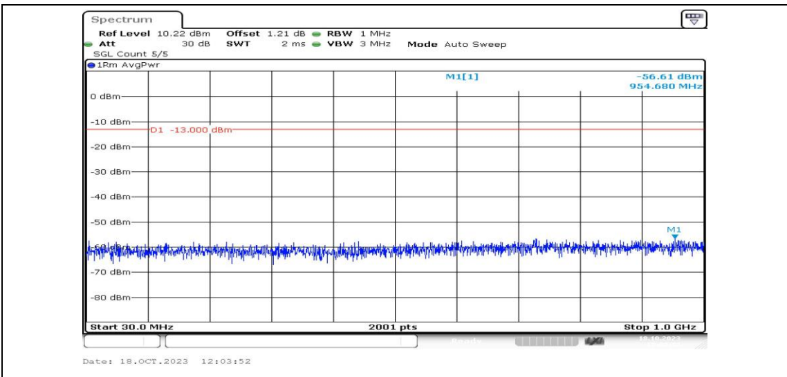
Band4-1.4MHz-16QAM-20175-1RB#0-Range3:30~1000MHz-PASS
