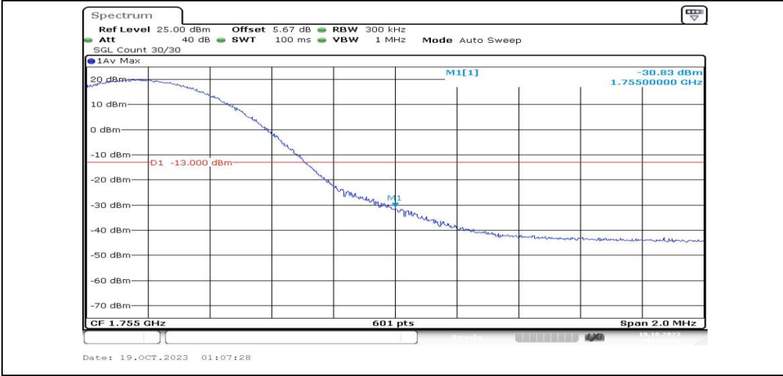
Band4-15MHz-16QAM-20325-1RB#74-PASS
