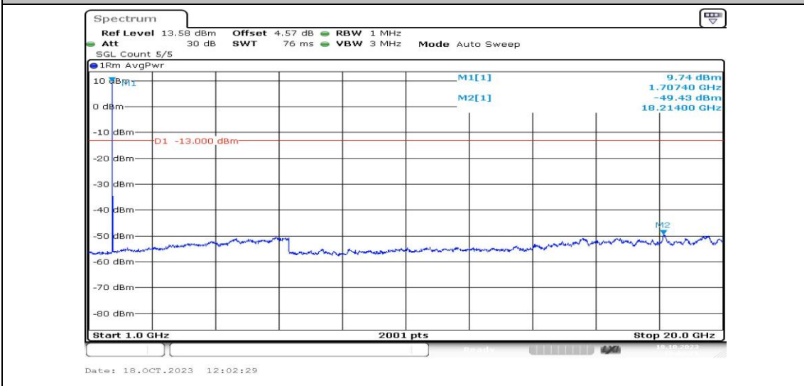
Band4-1.4MHz-16QAM-19957-1RB#0-Range4:1000~20000MHz-PASS
