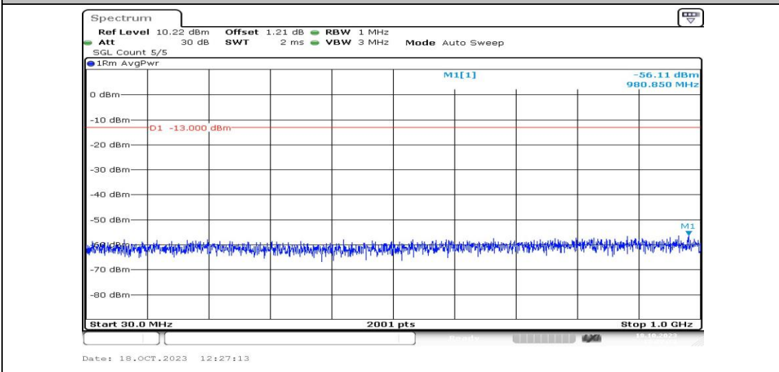
Band4-3MHz-QPSK-20175-1RB#0-Range3:30~1000MHz-PASS
