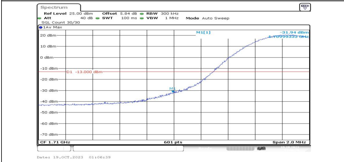
Band4-15MHz-16QAM-20025-1RB#0-PASS
