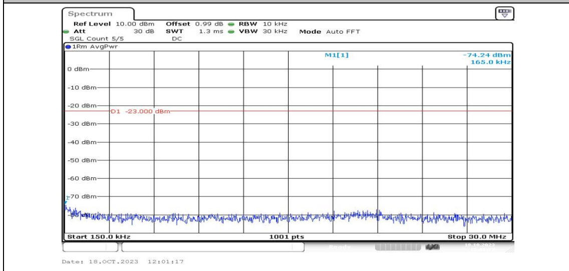
Band4-1.4MHz-QPSK-19957-1RB#0-Range2:0.15~30MHz-PASS
