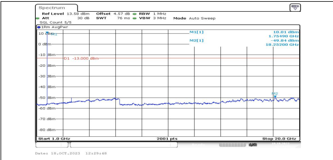
Band4-3MHz-16QAM-20385-1RB#0-Range4:1000~20000MHz-PASS
