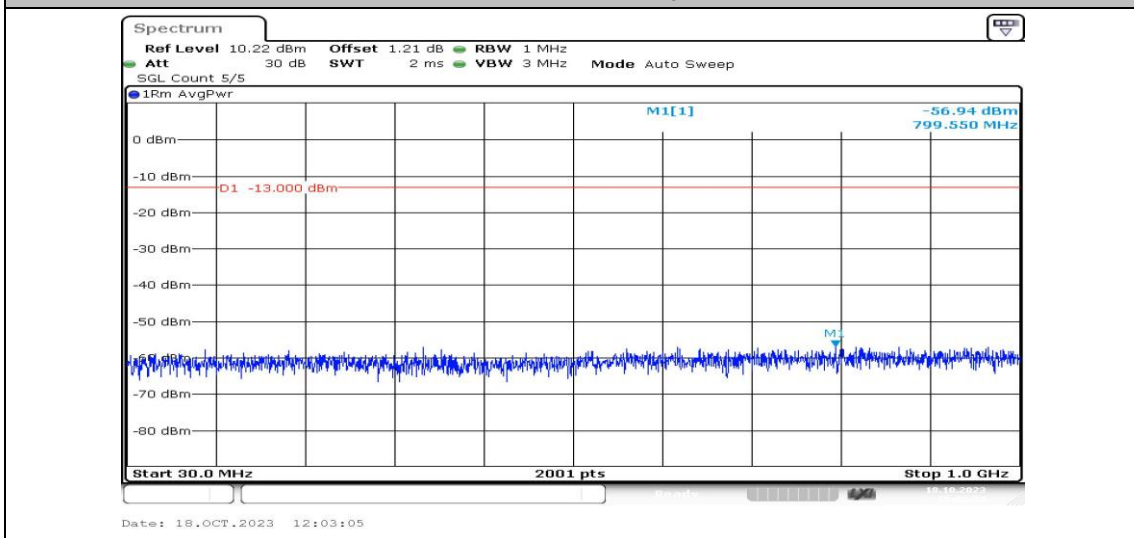
Band4-1.4MHz-QPSK-20175-1RB#0-Range3:30~1000MHz-PASS
