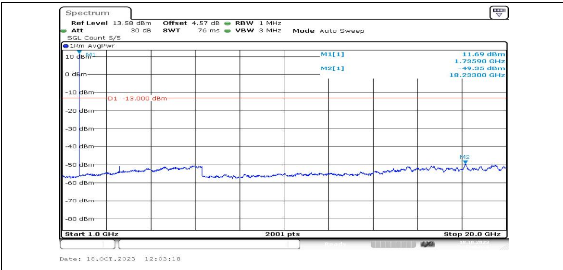
Band4-1.4MHz-QPSK-20175-1RB#0-Range4:1000~20000MHz-PASS
