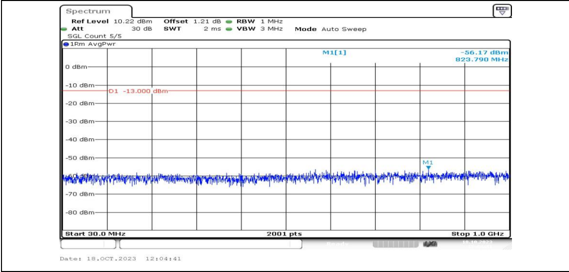
Band4-1.4MHz-QPSK-20393-1RB#0-Range3:30~1000MHz-PASS
