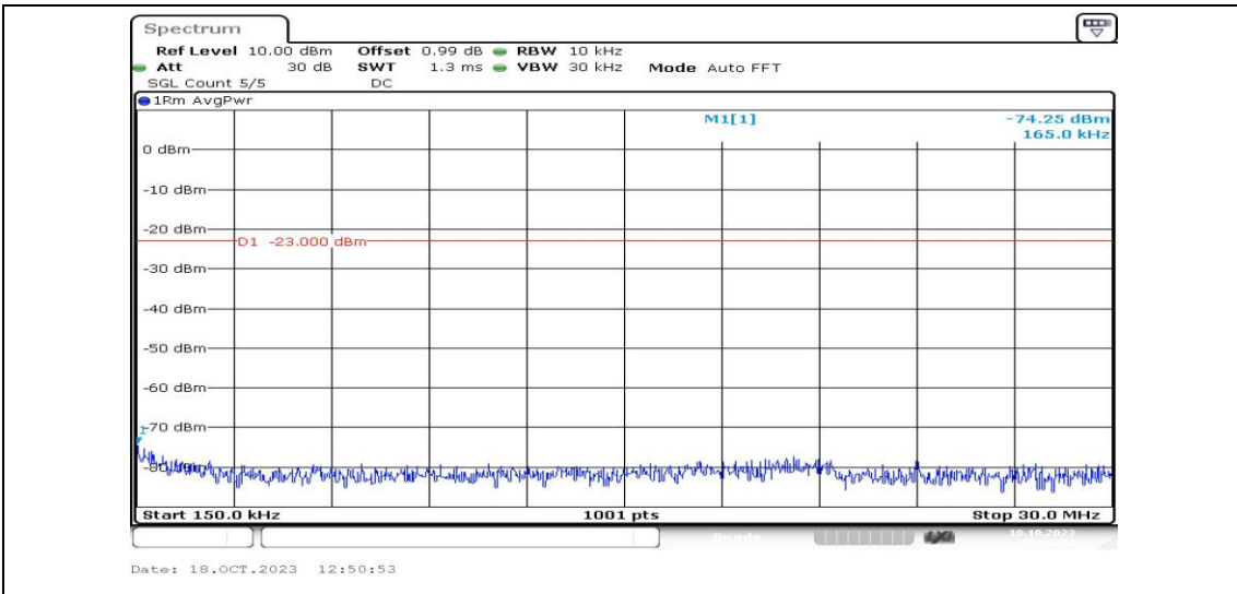
Band4-5MHz-16QAM-19975-1RB#0-Range2:0.15~30MHz-PASS
