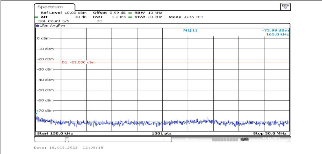
Band4-1.4MHz-16QAM-20393-1RB#0-Range2:0.15~30MHz-PASS
