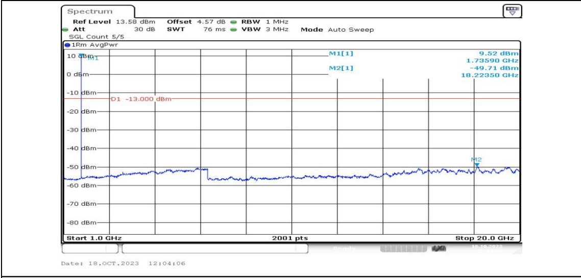
Band4-1.4MHz-16QAM-20175-1RB#0-Range4:1000~20000MHz-PASS
