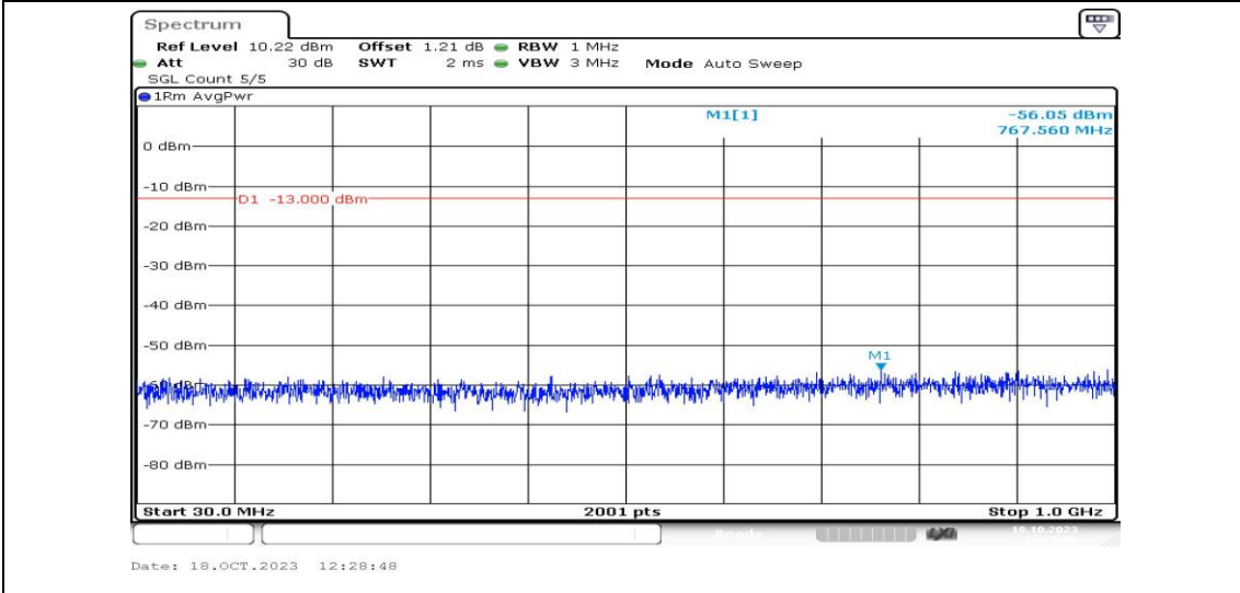
Band4-3MHz-QPSK-20385-1RB#0-Range3:30~1000MHz-PASS
