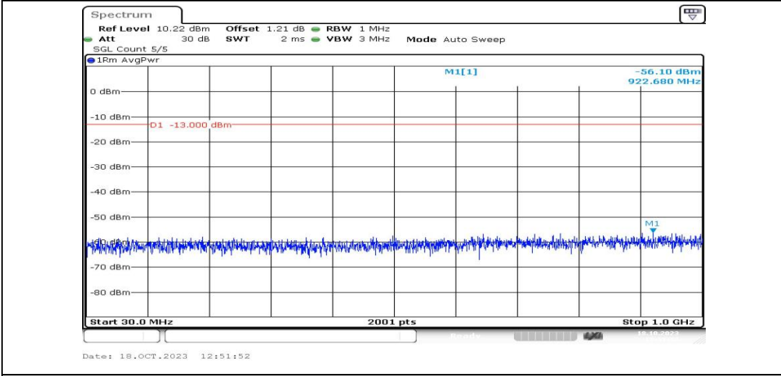
Band4-5MHz-QPSK-20175-1RB#0-Range3:30~1000MHz-PASS
