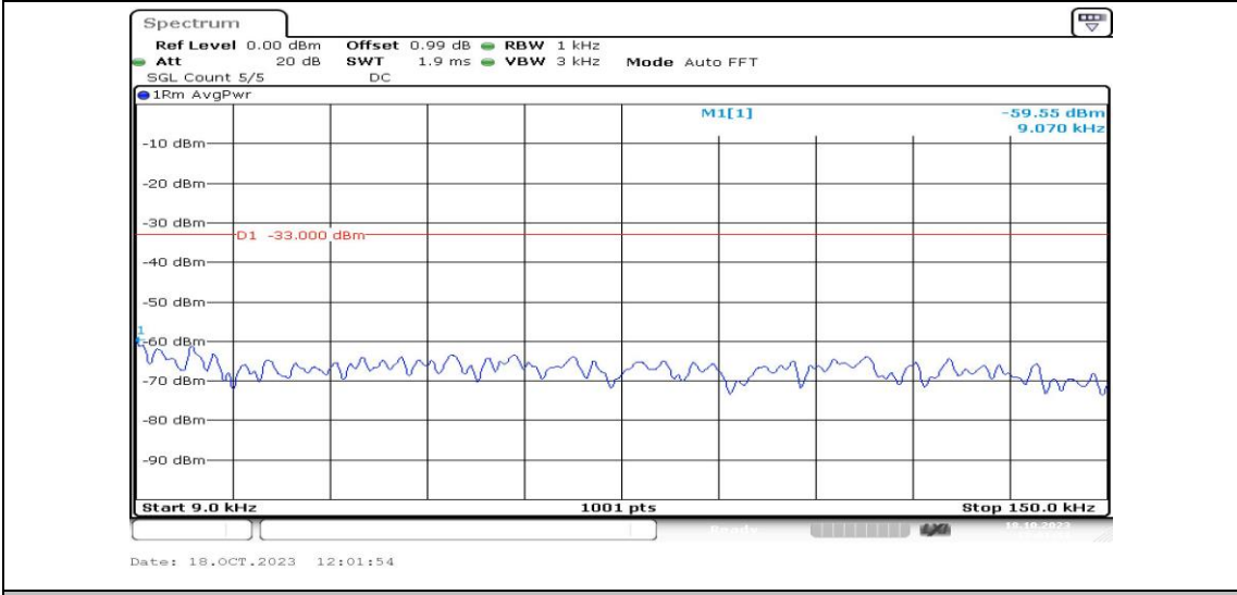
Band4-1.4MHz-16QAM-19957-1RB#0-Range1:0.009~0.15MHz-PASS
