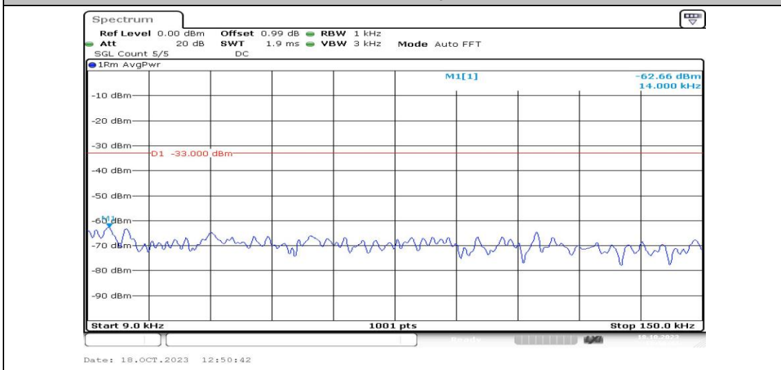
Band4-5MHz-16QAM-19975-1RB#0-Range1:0.009~0.15MHz-PASS
