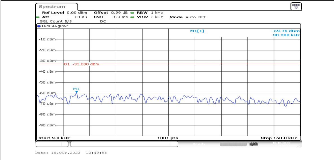
Band4-5MHz-QPSK-19975-1RB#0-Range1:0.009~0.15MHz-PASS
