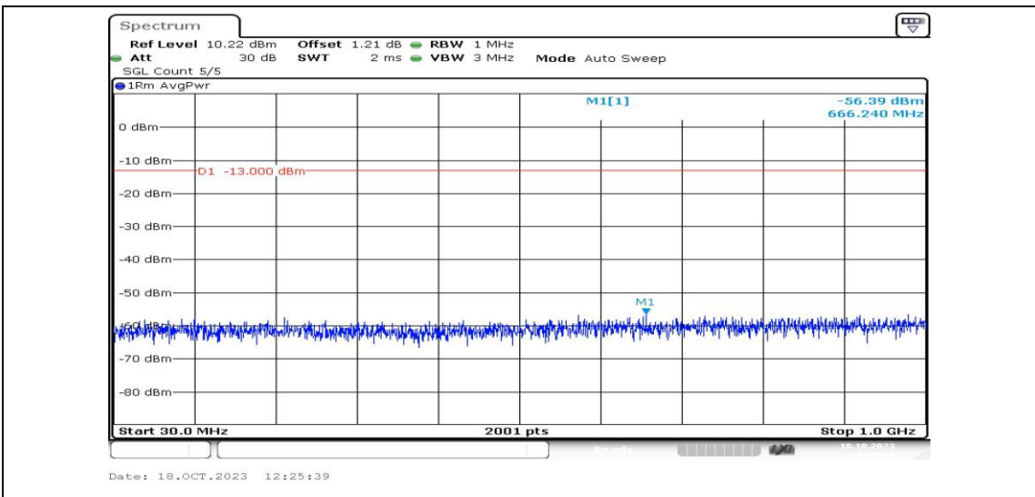
Band4-3MHz-QPSK-19965-1RB#0-Range3:30~1000MHz-PASS
