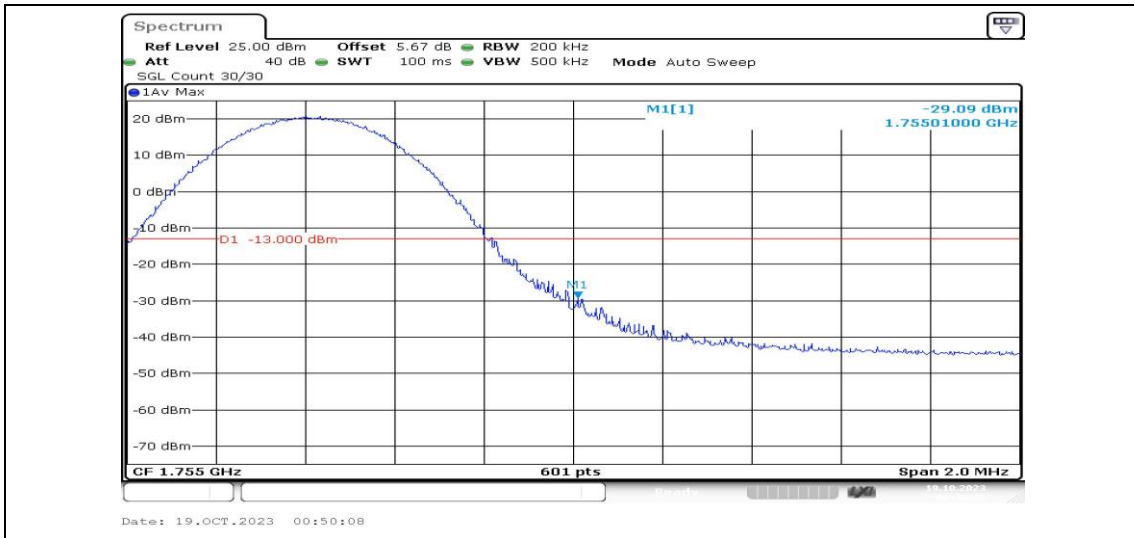
Band4-10MHz-16QAM-20350-1RB#49-PASS
