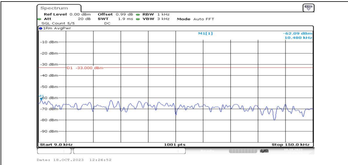
Band4-3MHz-QPSK-20175-1RB#0-Range1:0.009~0.15MHz-PASS
