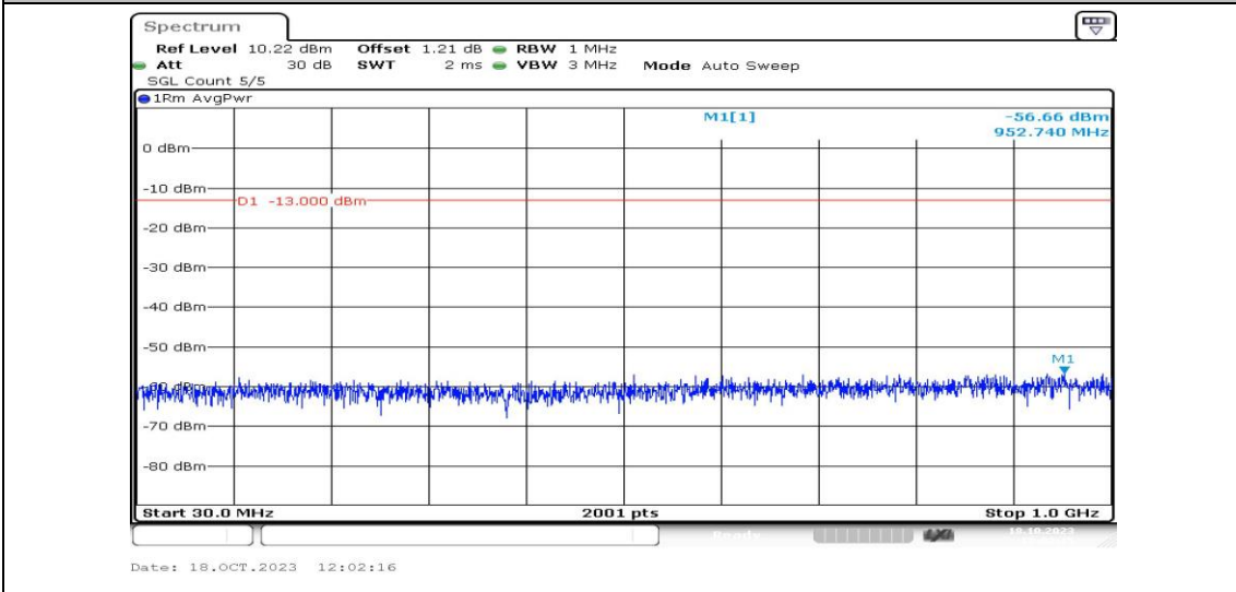
Band4-1.4MHz-16QAM-19957-1RB#0-Range3:30~1000MHz-PASS
