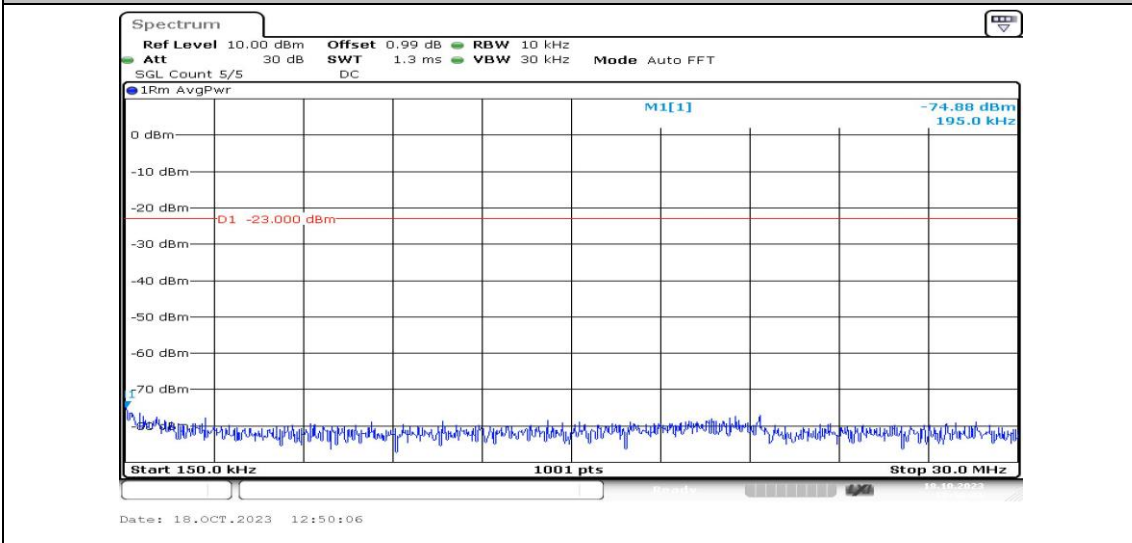
Band4-5MHz-QPSK-19975-1RB#0-Range2:0.15~30MHz-PASS
