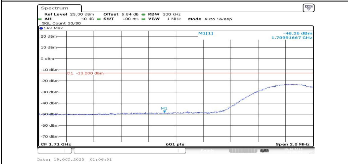
Band4-15MHz-16QAM-20025-1RB#74-PASS
