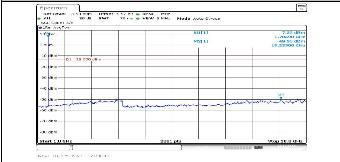
Band4-3MHz-16QAM-20175-1RB#0-Range4:1000~20000MHz-PASS
