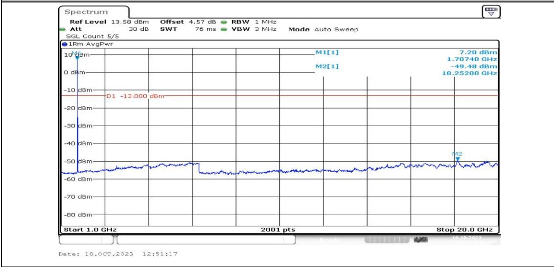
Band4-5MHz-16QAM-19975-1RB#0-Range4:1000~20000MHz-PASS
