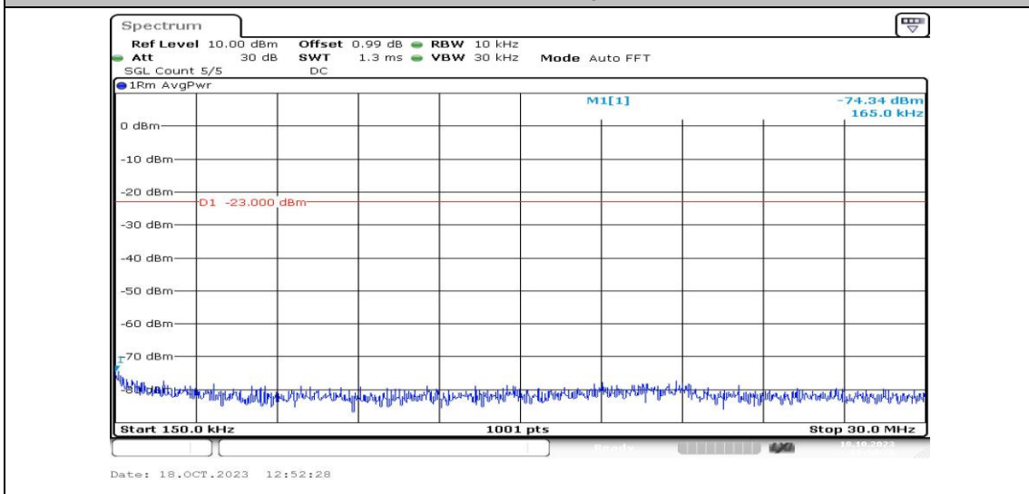
Band4-5MHz-16QAM-20175-1RB#0-Range2:0.15~30MHz-PASS
