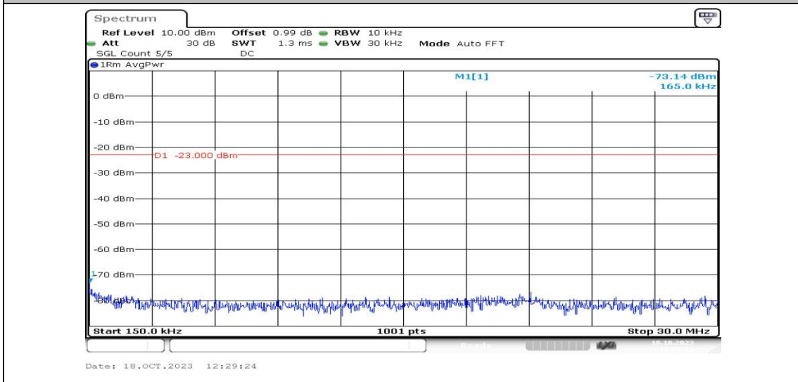
Band4-3MHz-16QAM-20385-1RB#0-Range2:0.15~30MHz-PASS
