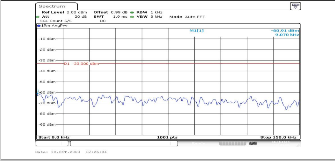
Band4-3MHz-16QAM-19965-1RB#0-Range1:0.009~0.15MHz-PASS
