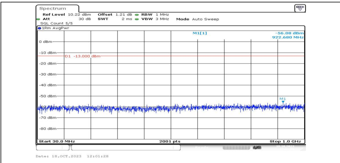
Band4-1.4MHz-QPSK-19957-1RB#0-Range3:30~1000MHz-PASS
