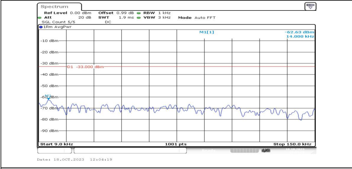
Band4-1.4MHz-QPSK-20393-1RB#0-Range1:0.009~0.15MHz-PASS
