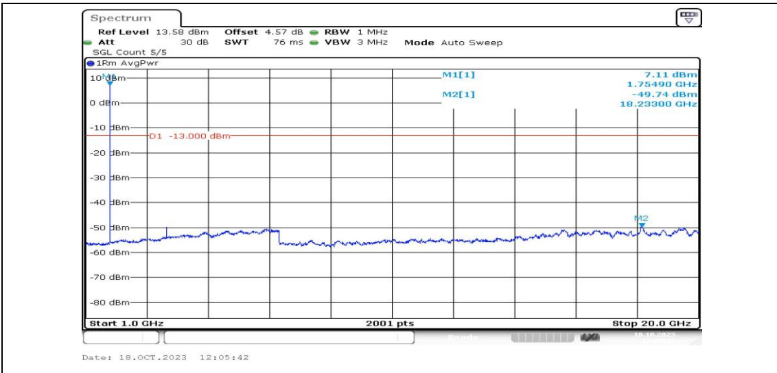
Band4-1.4MHz-16QAM-20393-1RB#0-Range4:1000~20000MHz-PASS
