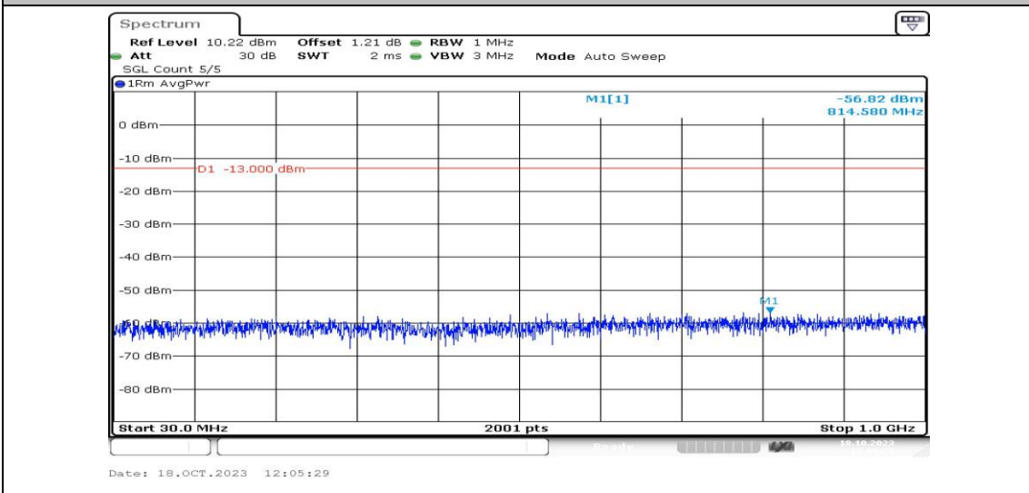
Band4-1.4MHz-16QAM-20393-1RB#0-Range3:30~1000MHz-PASS
