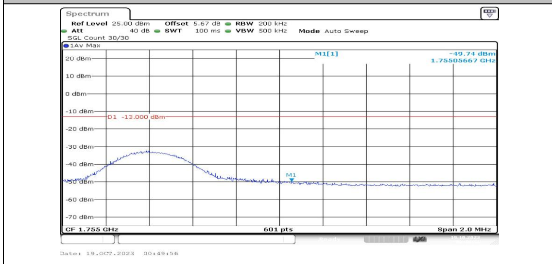
Band4-10MHz-16QAM-20350-1RB#0-PASS
