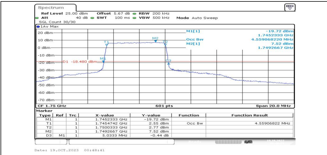
Band4-10MHz-16QAM-20350-25RB#0-PASS
