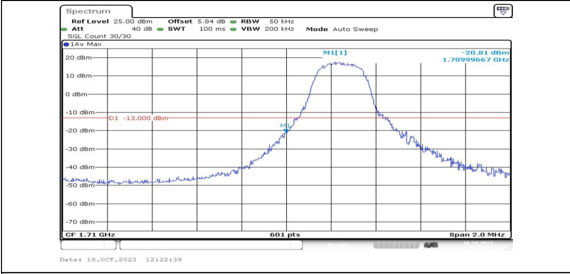
Band4-3MHz-16QAM-19965-1RB#0-PASS
