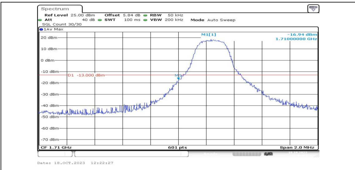
Band4-3MHz-QPSK-19965-1RB#0-PASS
