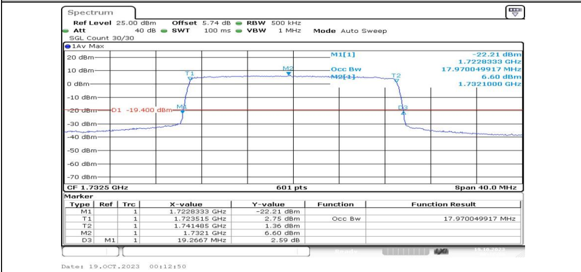
Band4-20MHz-QPSK-20175-100RB#0-PASS
