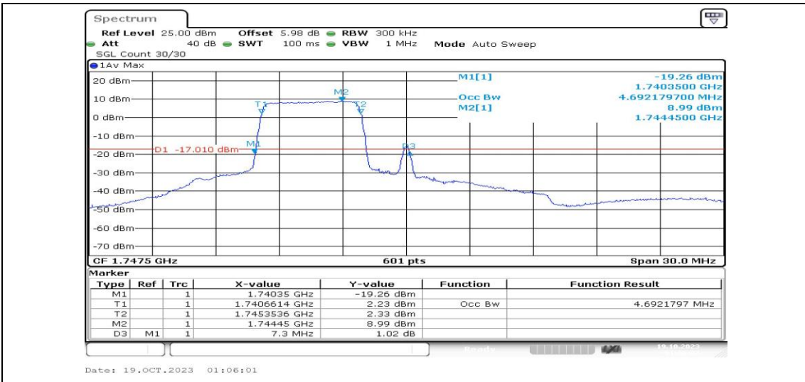
Band4-15MHz-16QAM-20325-25RB#0-PASS
