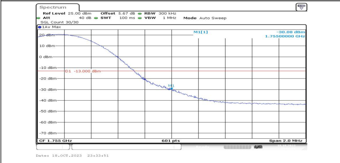
Band4-15MHz-QPSK-20325-1RB#74-PASS
