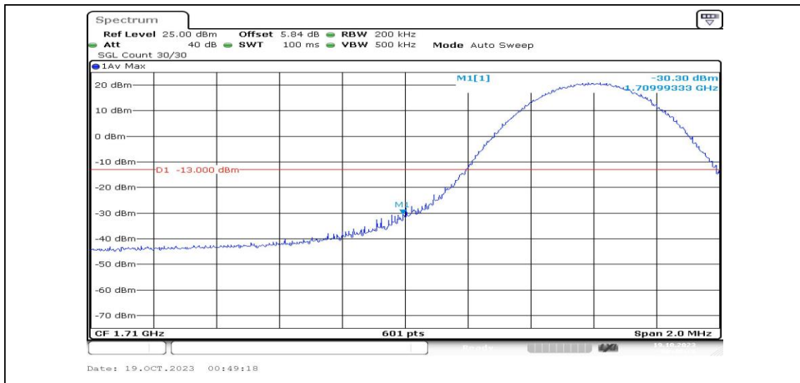
Band4-10MHz-16QAM-20000-1RB#0-PASS
