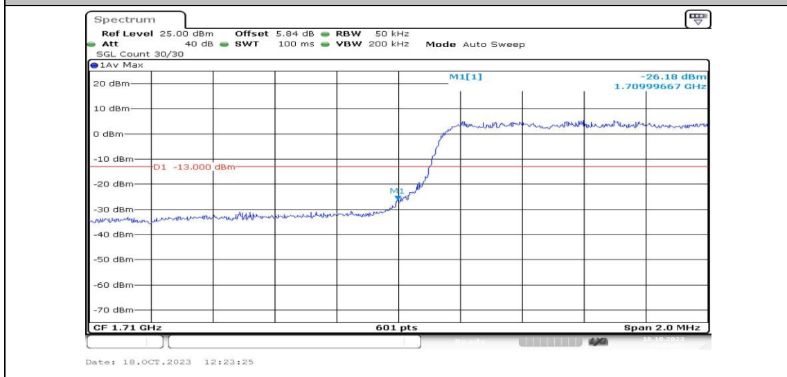
Band4-3MHz-16QAM-19965-15RB#0-PASS
