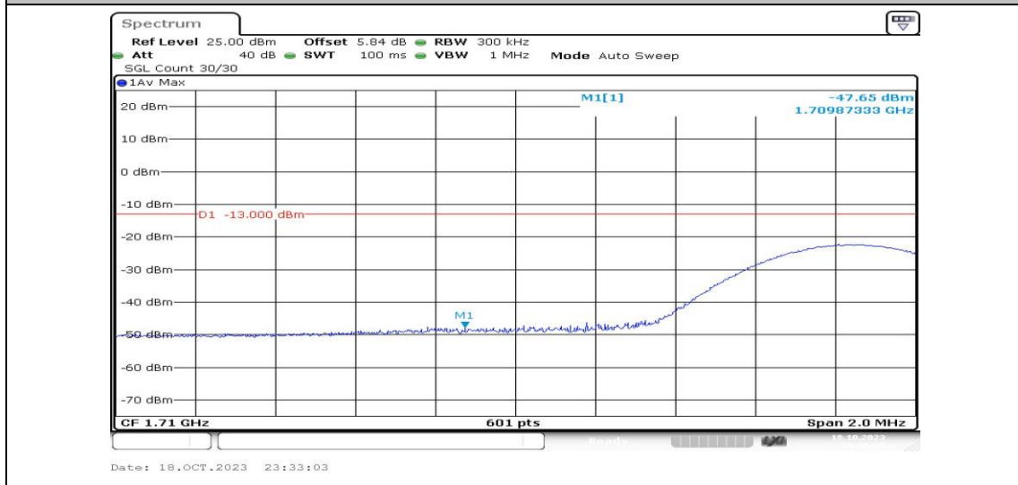
Band4-15MHz-QPSK-20025-1RB#74-PASS
