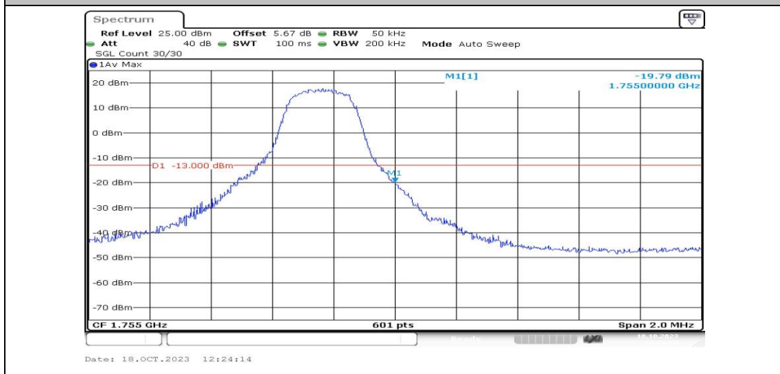
Band4-3MHz-QPSK-20385-1RB#14-PASS
