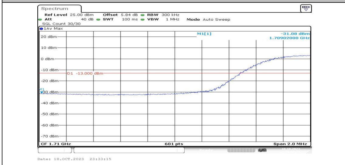
Band4-15MHz-QPSK-20025-75RB#0-PASS
