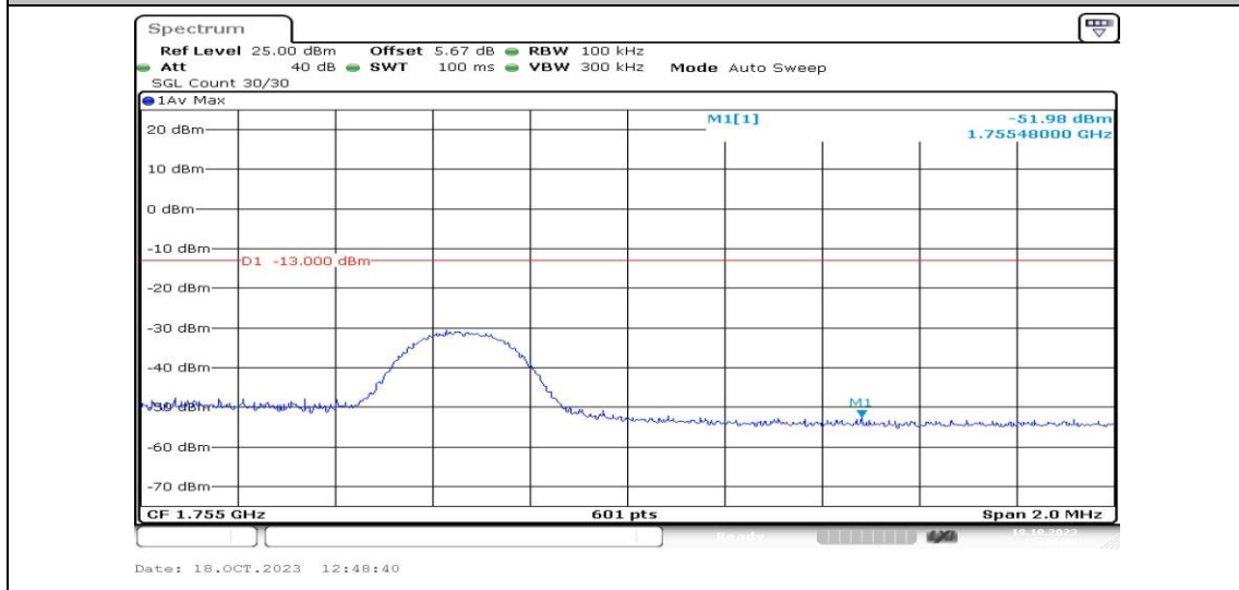
Band4-5MHz-16QAM-20375-1RB#0-PASS
