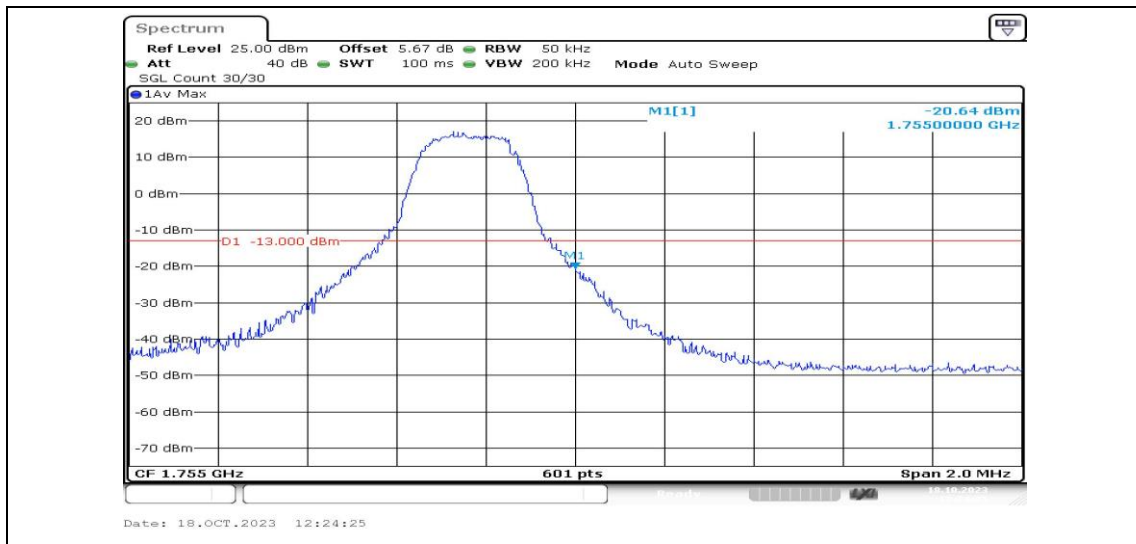
Band4-3MHz-16QAM-20385-1RB#14-PASS
