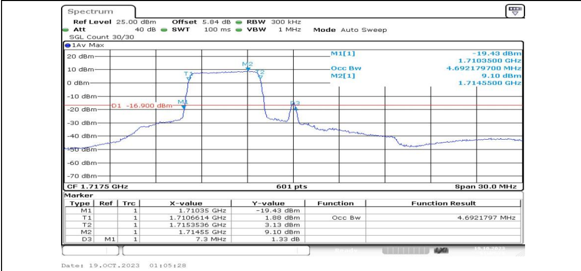
Band4-15MHz-16QAM-20025-25RB#0-PASS
