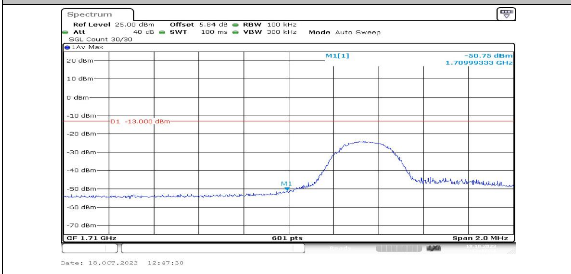
Band4-5MHz-QPSK-19975-1RB#24-PASS
