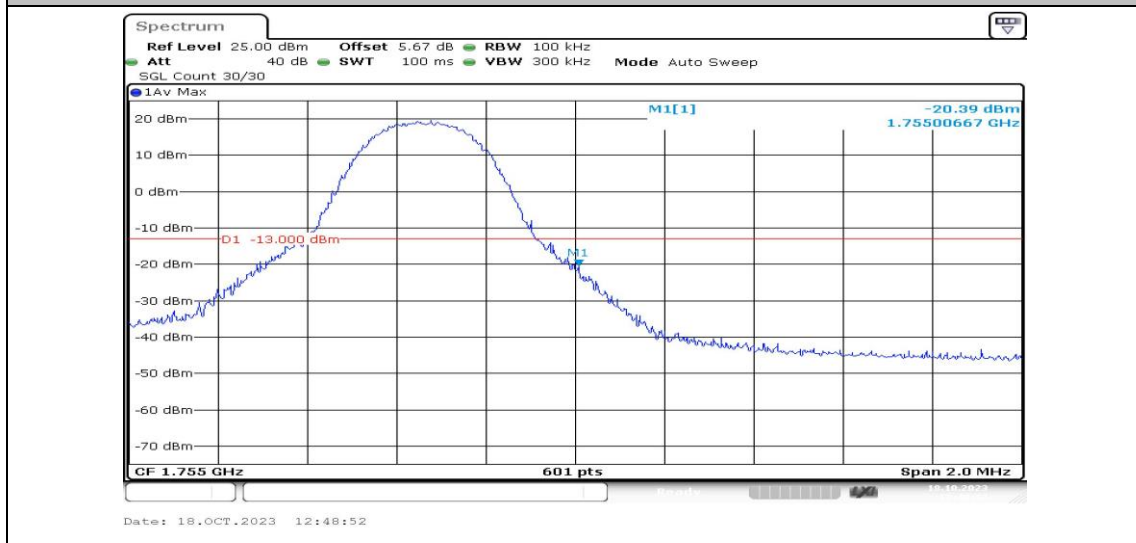
Band4-5MHz-QPSK-20375-1RB#24-PASS
