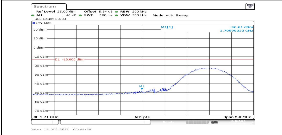
Band4-10MHz-16QAM-20000-1RB#49-PASS
