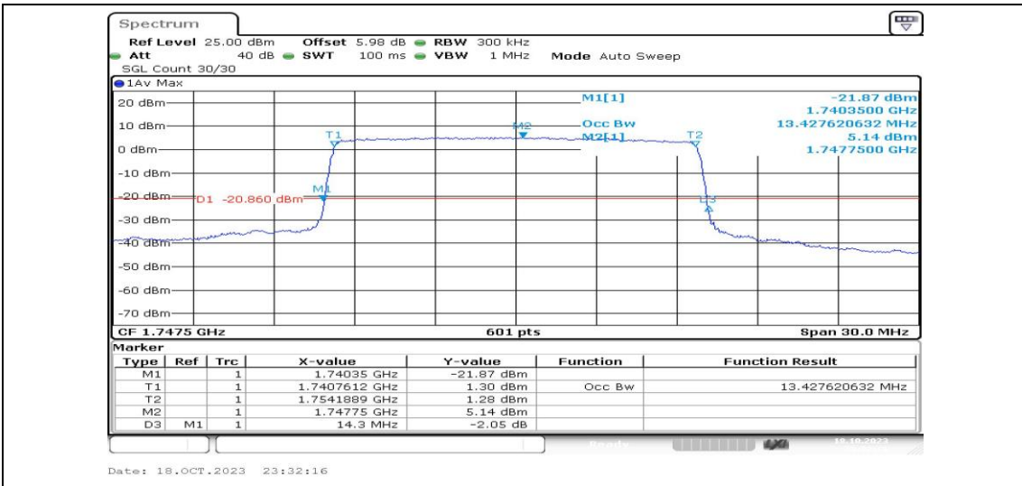
Band4-15MHz-QPSK-20325-75RB#0-PASS
