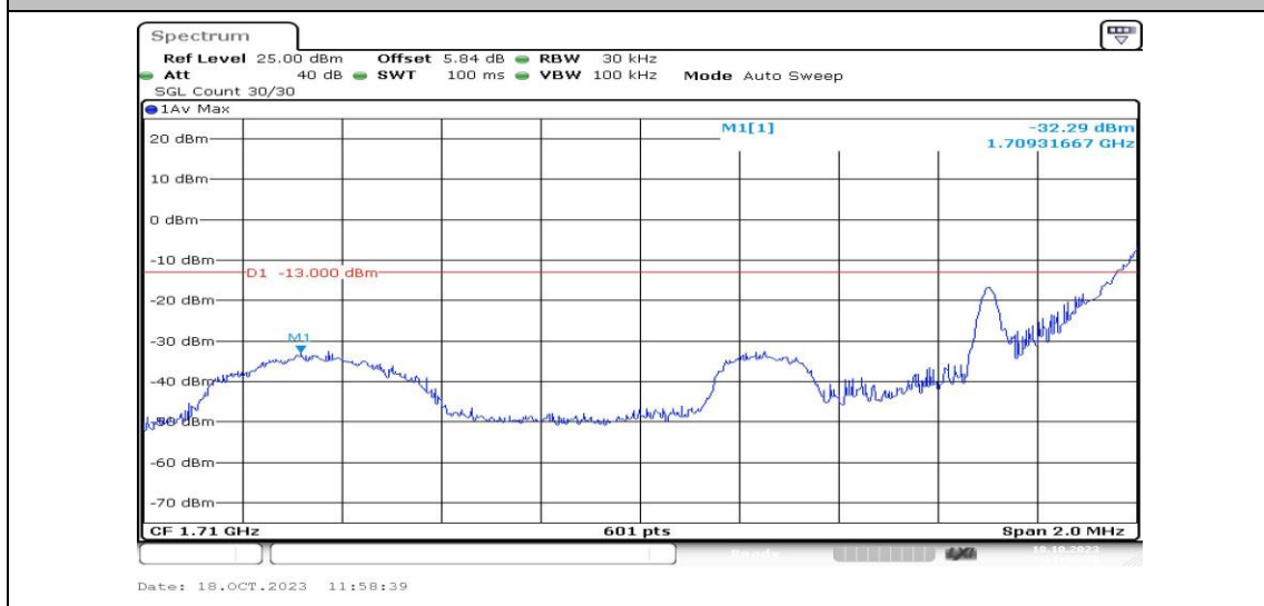
Band4-1.4MHz-16QAM-19957-1RB#0-PASS
