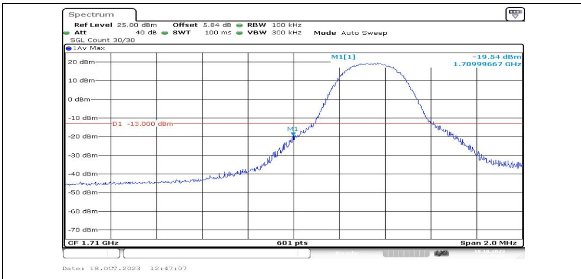
Band4-5MHz-QPSK-19975-1RB#0-PASS
