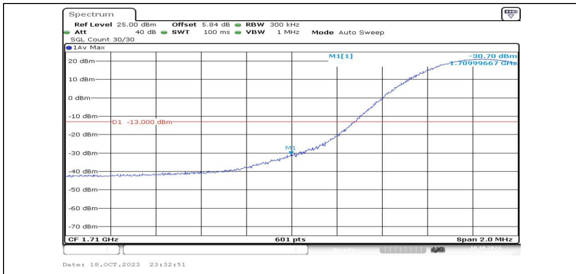
Band4-15MHz-QPSK-20025-1RB#0-PASS
