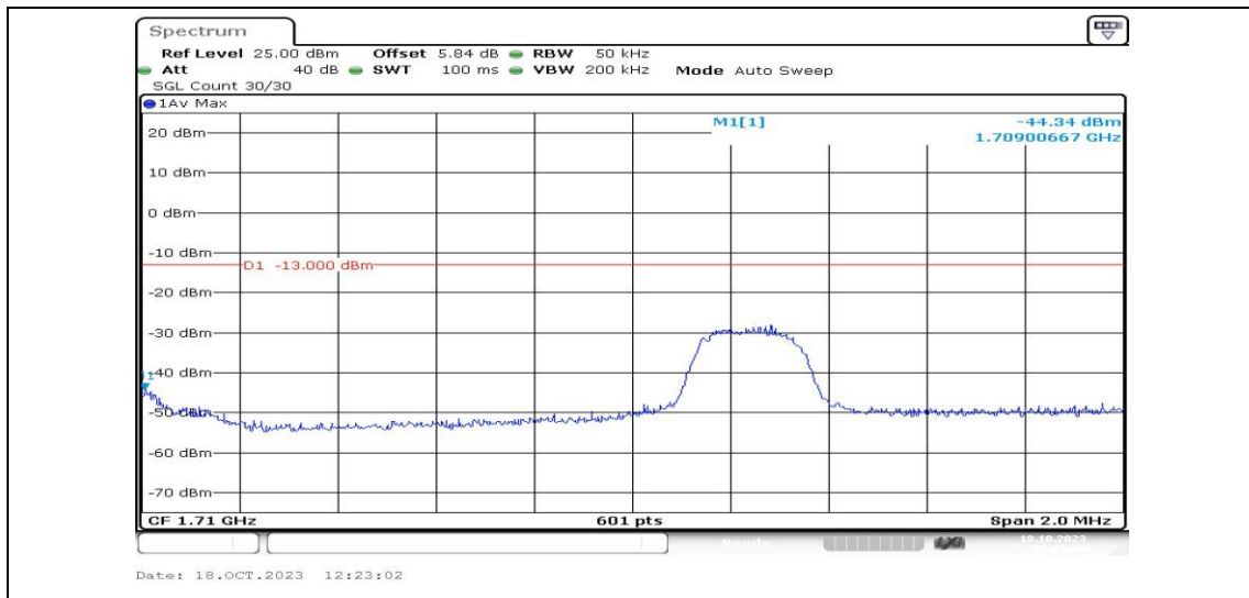
Band4-3MHz-16QAM-19965-1RB#14-PASS
