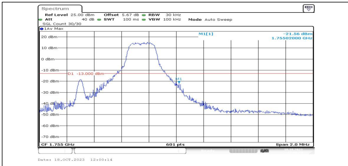
Band4-1.4MHz-16QAM-20393-1RB#5-PASS
