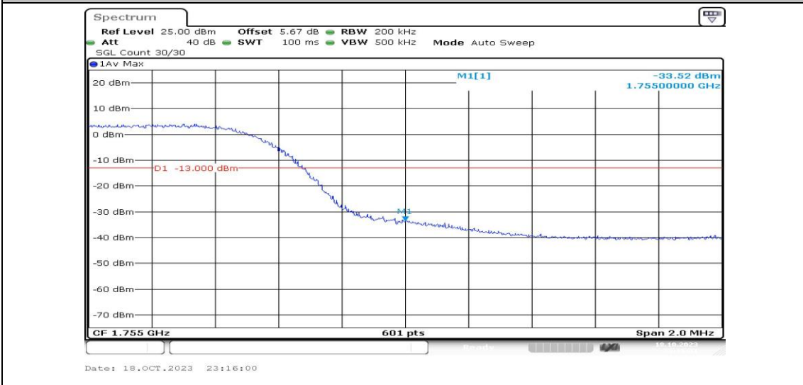
Band4-10MHz-QPSK-20350-50RB#0-PASS
