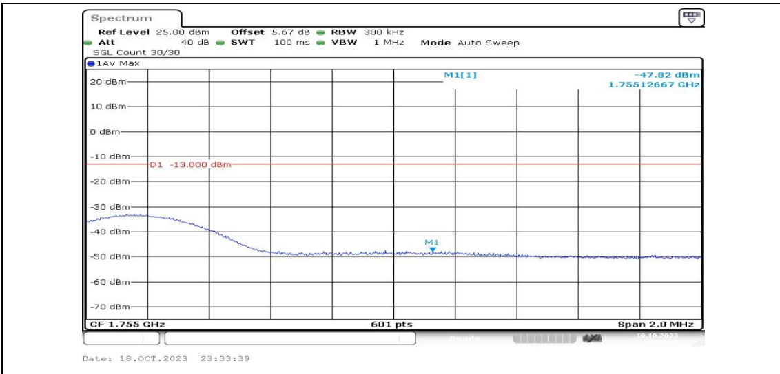
Band4-15MHz-QPSK-20325-1RB#0-PASS
