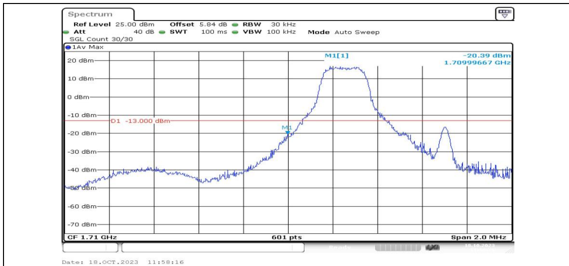
Band4-1.4MHz-QPSK-19957-1RB#0-PASS
