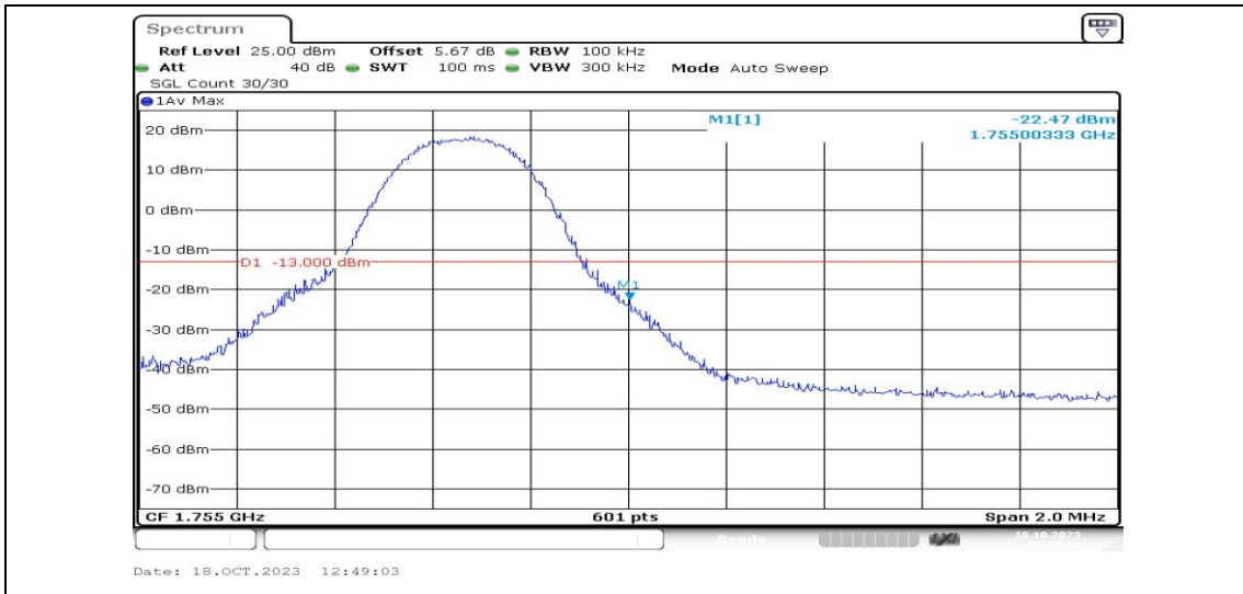
Band4-5MHz-16QAM-20375-1RB#24-PASS
