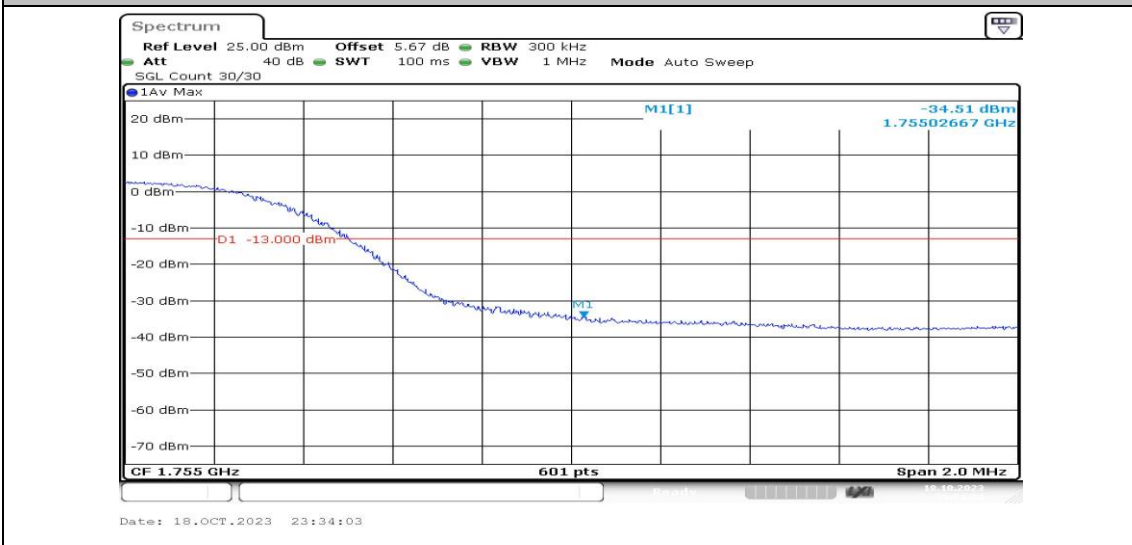
Band4-15MHz-QPSK-20325-75RB#0-PASS
