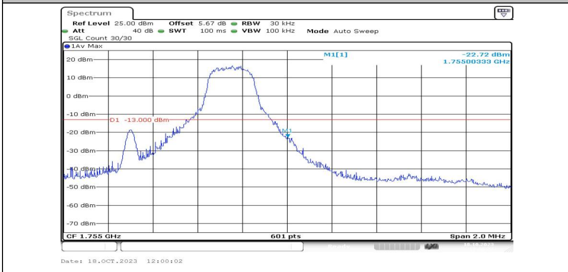
Band4-1.4MHz-QPSK-20393-1RB#5-PASS
