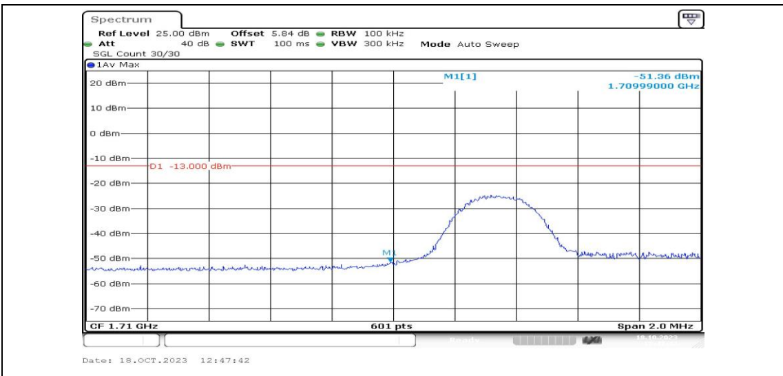
Band4-5MHz-16QAM-19975-1RB#24-PASS
