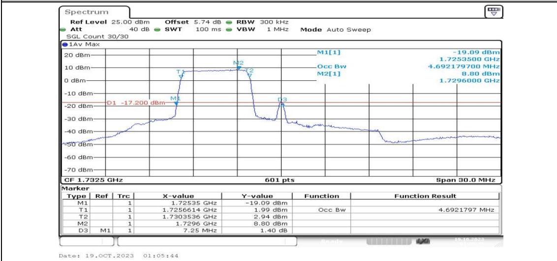
Band4-15MHz-16QAM-20175-25RB#0-PASS
