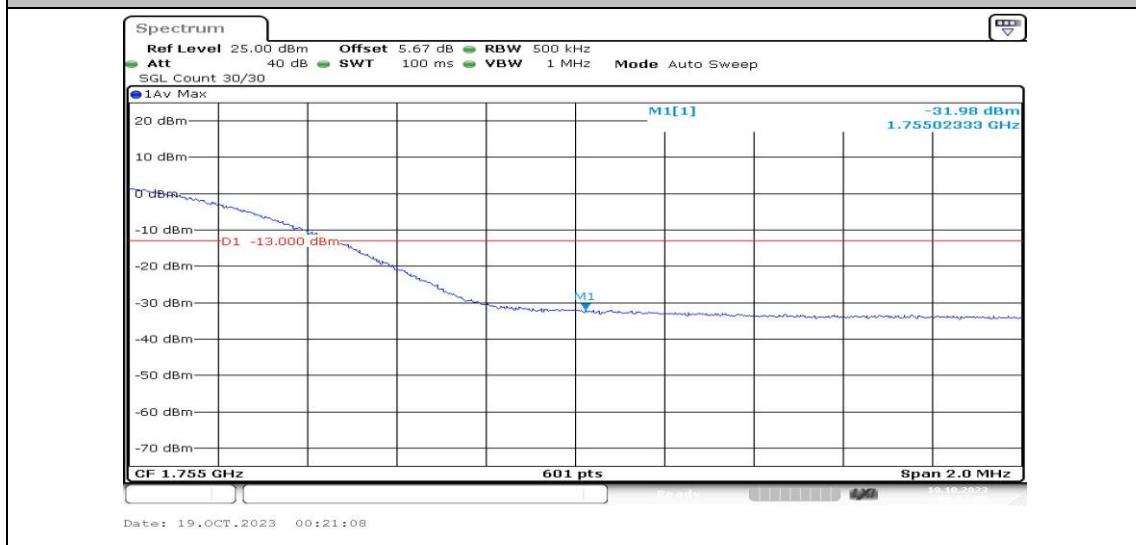
Band4-20MHz-QPSK-20300-100RB#0-PASS
