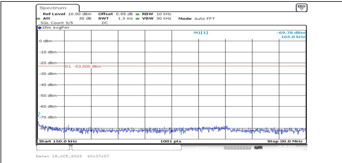
Band2-15MHz-QPSK-18900-1RB#0-Range2:0.15~30MHz-PASS
