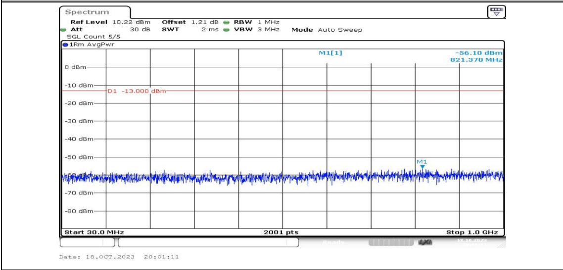
Band2-10MHz-QPSK-19150-1RB#0-Range3:30~1000MHz-PASS
