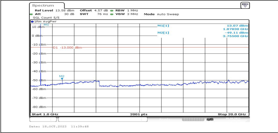
Band2-5MHz-16QAM-18900-1RB#0-Range4:1000~20000MHz-PASS
