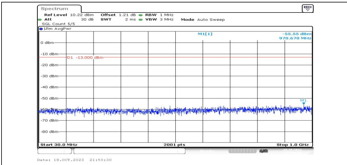
Band2-10MHz-16QAM-18650-1RB#0-Range3:30~1000MHz-PASS
