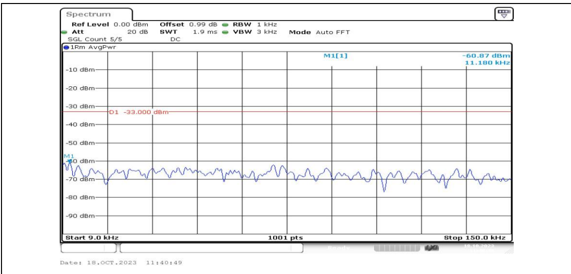
Band2-5MHz-16QAM-19175-1RB#0-Range1:0.009~0.15MHz-PASS
