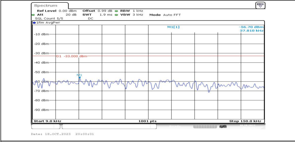
Band2-10MHz-QPSK-18900-1RB#0-Range1:0.009~0.15MHz-PASS
