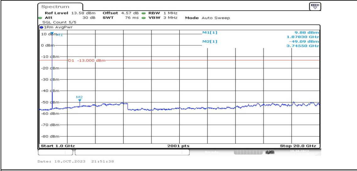
Band2-10MHz-16QAM-18900-1RB#0-Range4:1000~20000MHz-PASS
