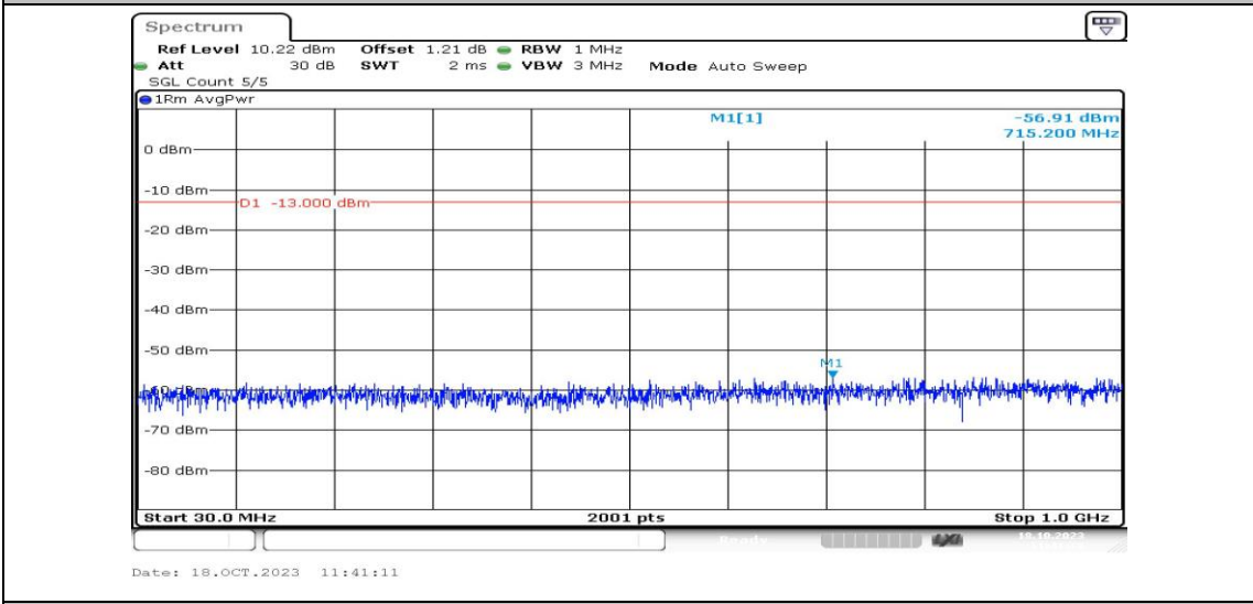
Band2-5MHz-16QAM-19175-1RB#0-Range3:30~1000MHz-PASS
