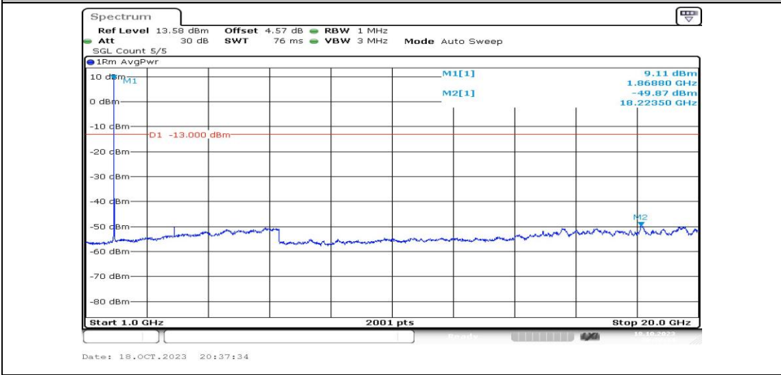
Band2-15MHz-QPSK-18900-1RB#0-Range4:1000~20000MHz-PASS
