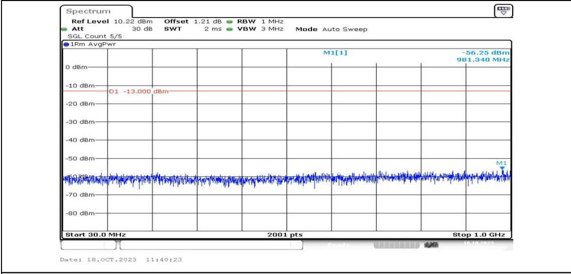
Band2-5MHz-QPSK-19175-1RB#0-Range3:30~1000MHz-PASS
