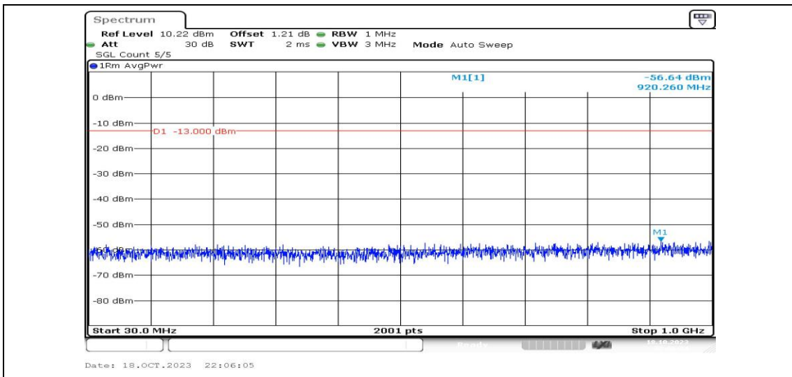
Band2-15MHz-16QAM-18675-1RB#0-Range3:30~1000MHz-PASS
