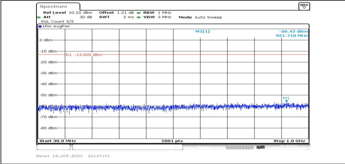
Band2-15MHz-16QAM-19125-1RB#0-Range3:30~1000MHz-PASS
