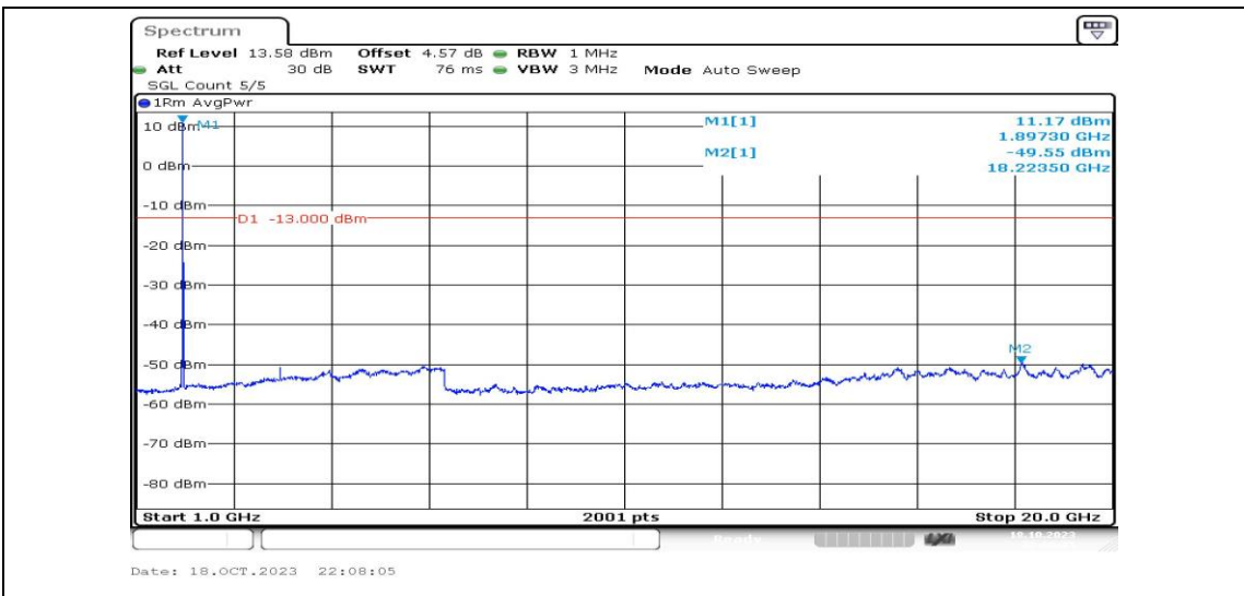
Band2-15MHz-16QAM-19125-1RB#0-Range4:1000~20000MHz-PASS
