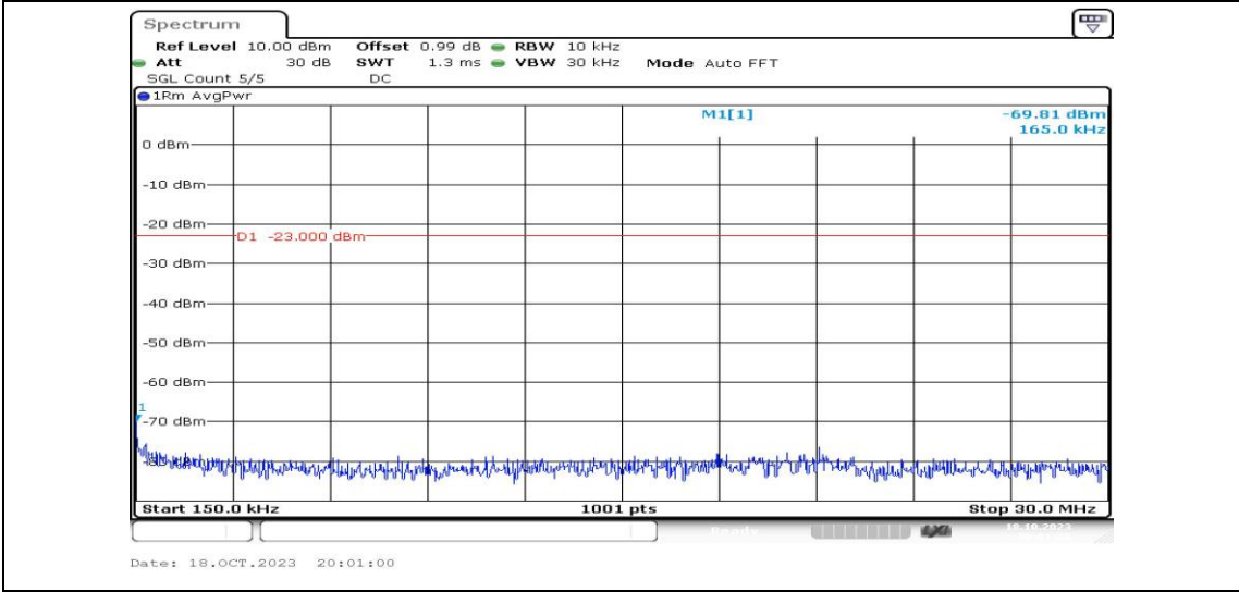
Band2-10MHz-QPSK-19150-1RB#0-Range2:0.15~30MHz-PASS
