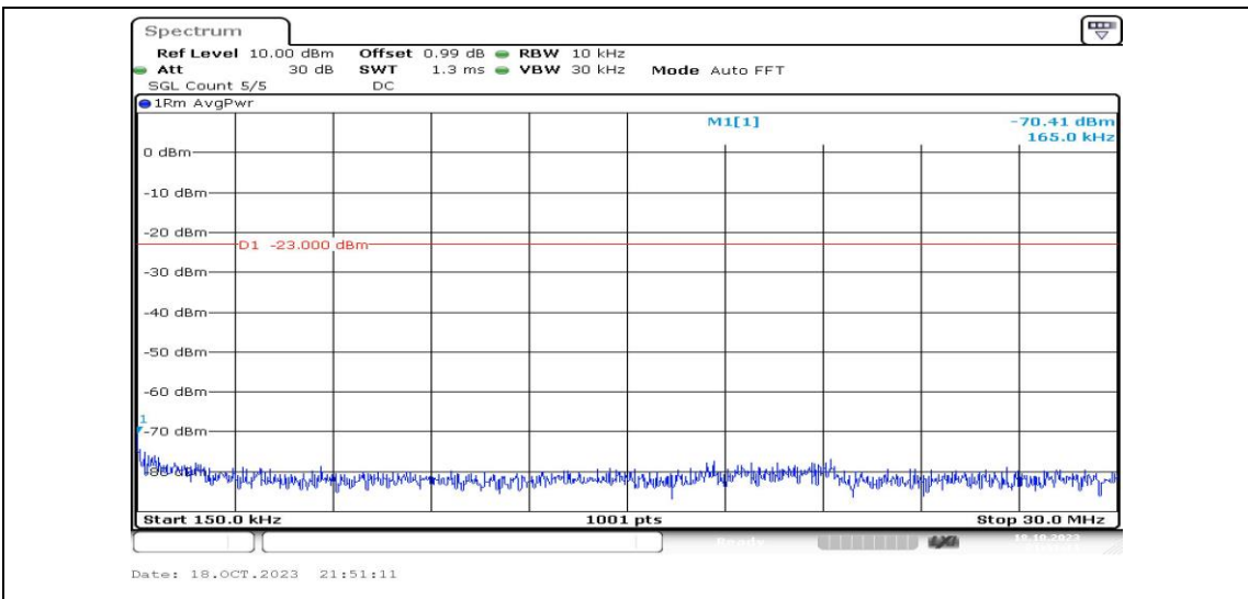
Band2-10MHz-16QAM-18900-1RB#0-Range2:0.15~30MHz-PASS
