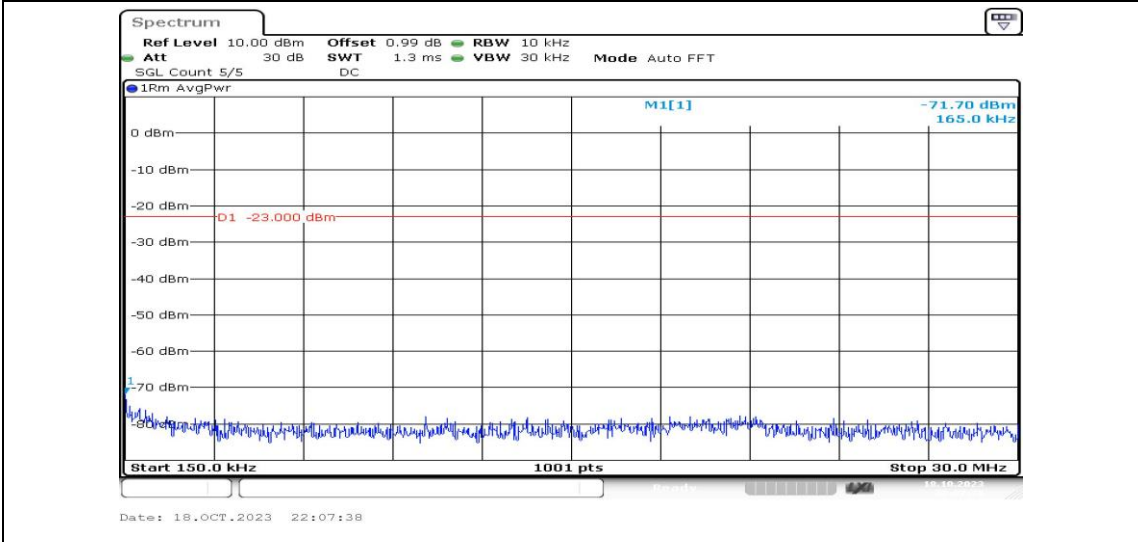
Band2-15MHz-16QAM-19125-1RB#0-Range2:0.15~30MHz-PASS
