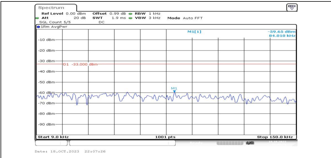
Band2-15MHz-16QAM-19125-1RB#0-Range1:0.009~0.15MHz-PASS
