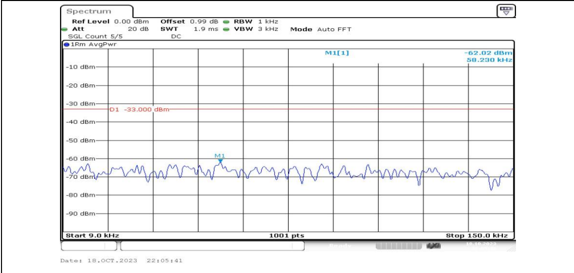
Band2-15MHz-16QAM-18675-1RB#0-Range1:0.009~0.15MHz-PASS
