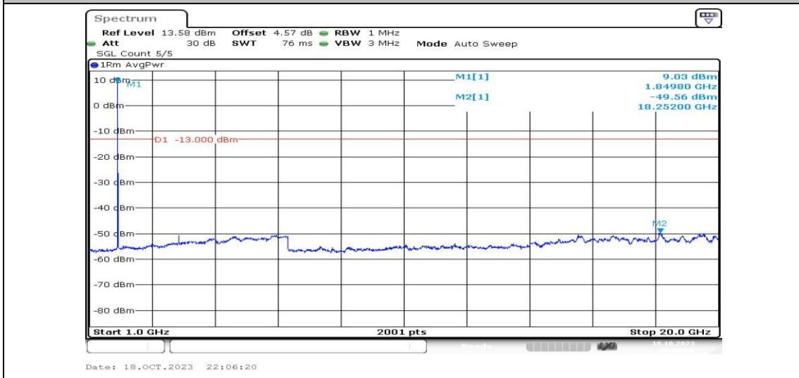
Band2-15MHz-16QAM-18675-1RB#0-Range4:1000~20000MHz-PASS
