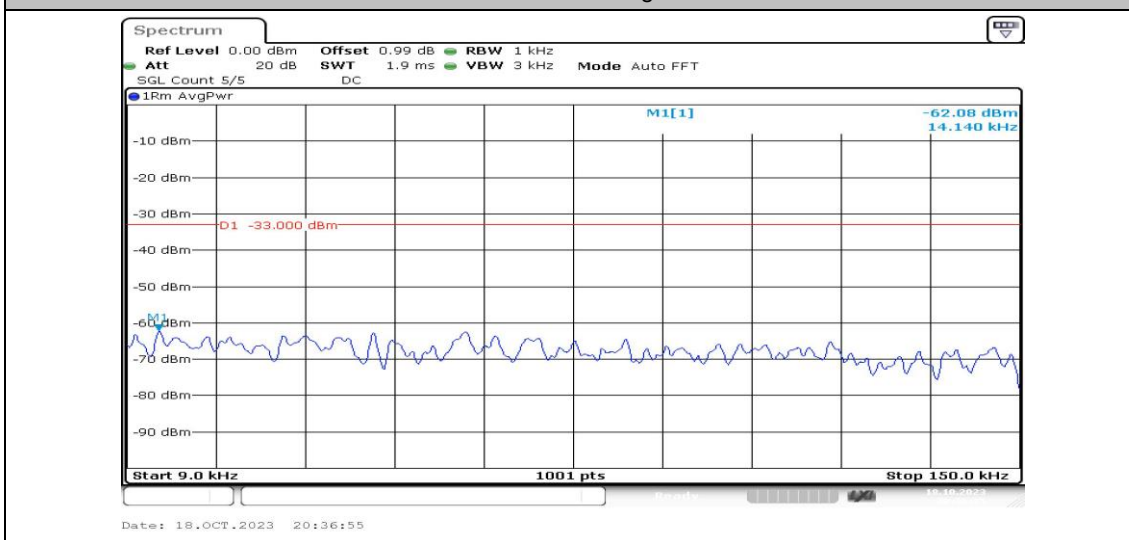
Band2-15MHz-QPSK-18900-1RB#0-Range1:0.009~0.15MHz-PASS
