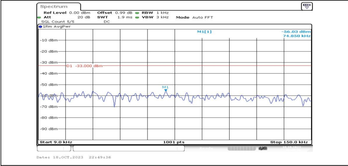
Band2-20MHz-16QAM-18900-1RB#0-Range1:0.009~0.15MHz-PASS
