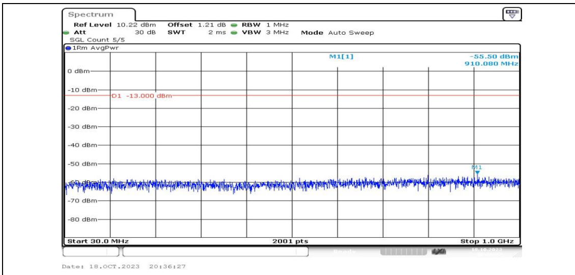
Band2-15MHz-QPSK-18675-1RB#0-Range3:30~1000MHz-PASS
