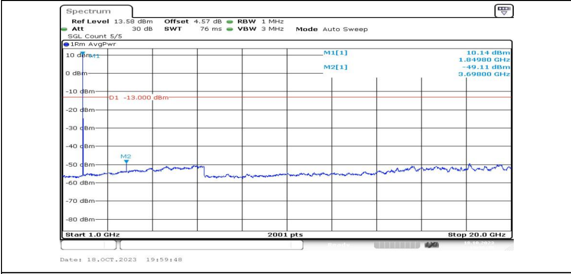
Band2-10MHz-QPSK-18650-1RB#0-Range4:1000~20000MHz-PASS
