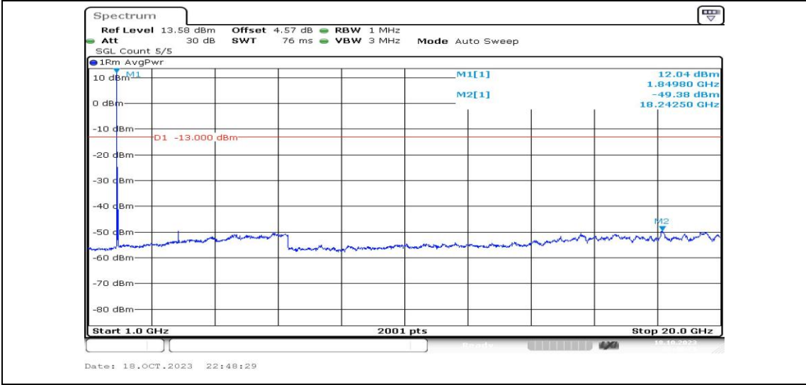
Band2-20MHz-16QAM-18700-1RB#0-Range4:1000~20000MHz-PASS
