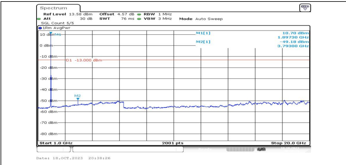
Band2-15MHz-QPSK-19125-1RB#0-Range4:1000~20000MHz-PASS
