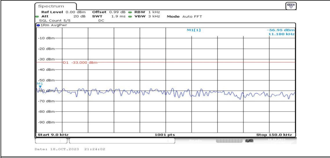
Band2-20MHz-QPSK-18900-1RB#0-Range1:0.009~0.15MHz-PASS
