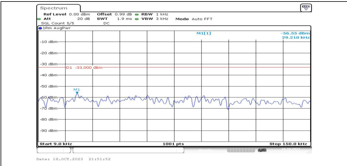
Band2-10MHz-16QAM-19150-1RB#0-Range1:0.009~0.15MHz-PASS
