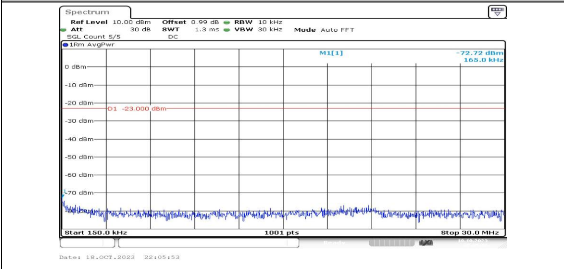
Band2-15MHz-16QAM-18675-1RB#0-Range2:0.15~30MHz-PASS
