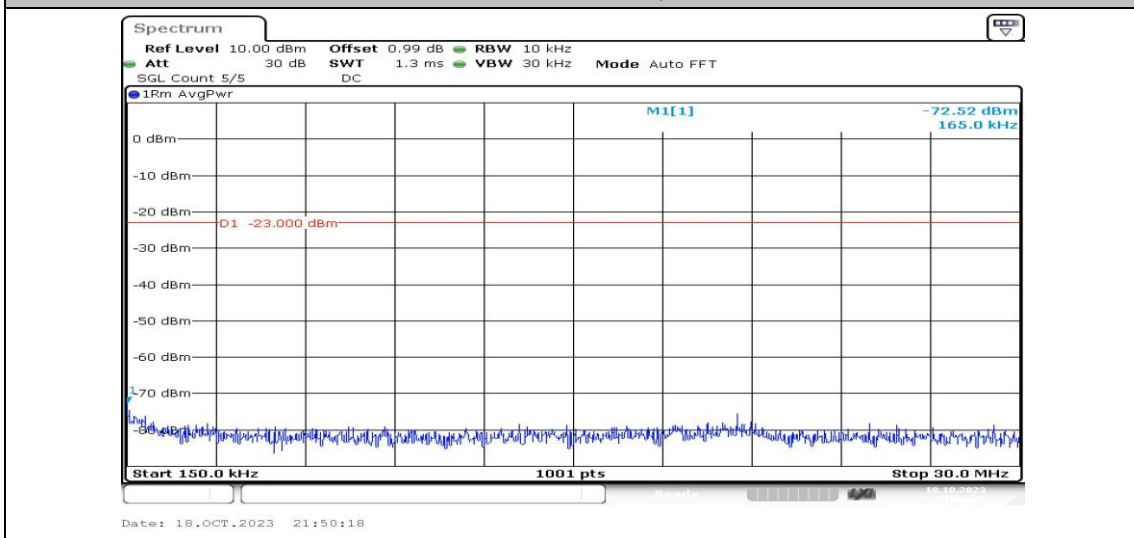
Band2-10MHz-16QAM-18650-1RB#0-Range2:0.15~30MHz-PASS
