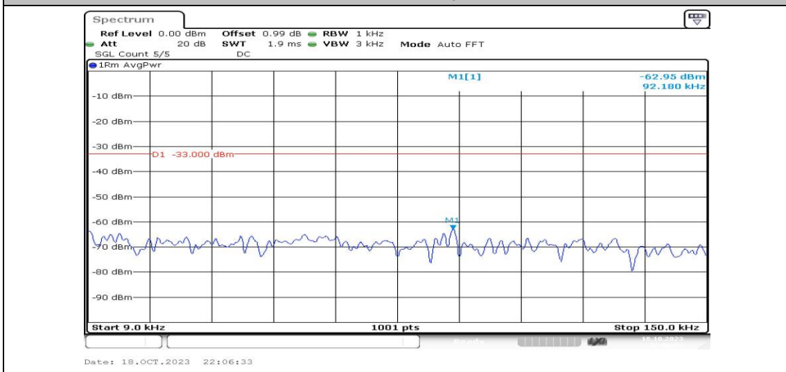
Band2-15MHz-16QAM-18900-1RB#0-Range1:0.009~0.15MHz-PASS
