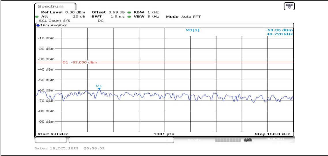
Band2-15MHz-QPSK-18675-1RB#0-Range1:0.009~0.15MHz-PASS
