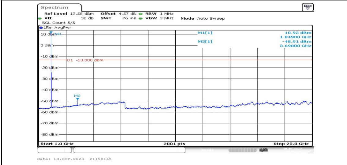
Band2-10MHz-16QAM-18650-1RB#0-Range4:1000~20000MHz-PASS
