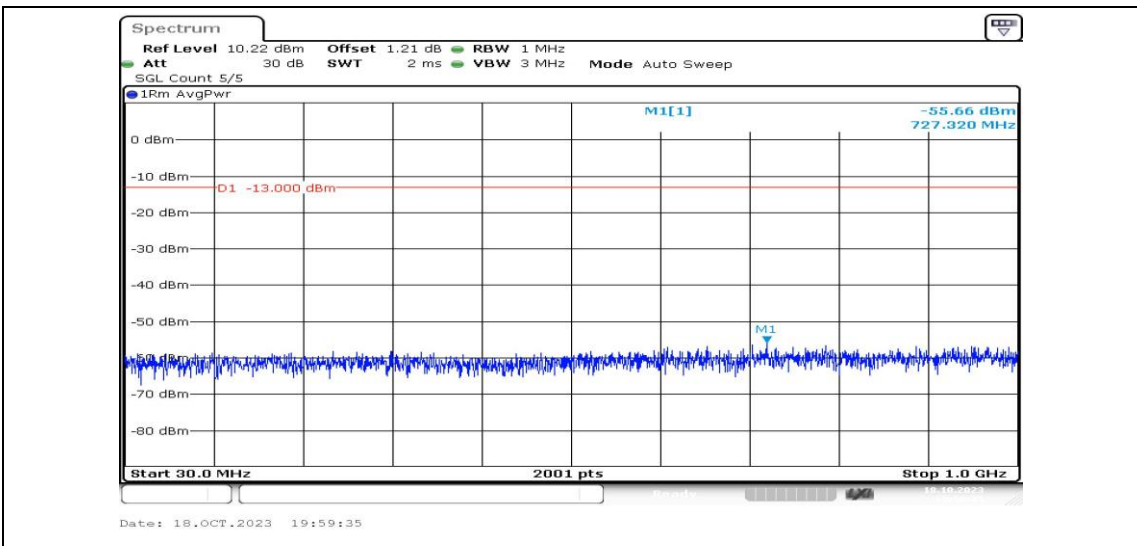
Band2-10MHz-QPSK-18650-1RB#0-Range3:30~1000MHz-PASS
