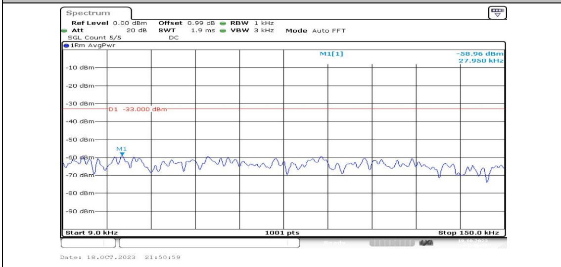
Band2-10MHz-16QAM-18900-1RB#0-Range1:0.009~0.15MHz-PASS
