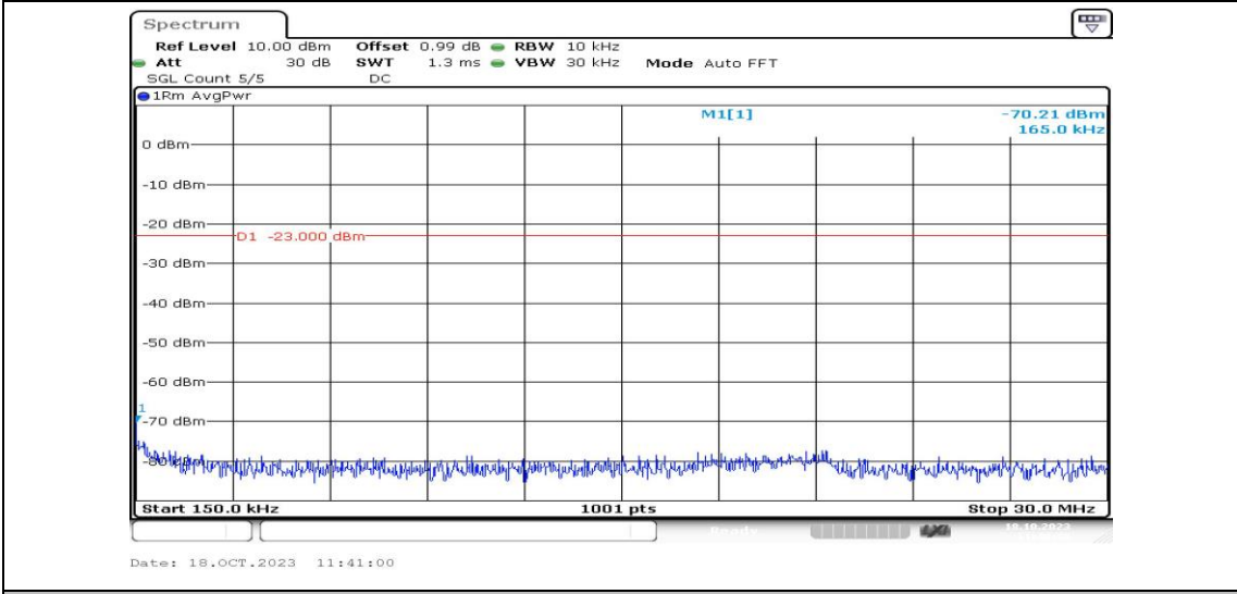
Band2-5MHz-16QAM-19175-1RB#0-Range2:0.15~30MHz-PASS
