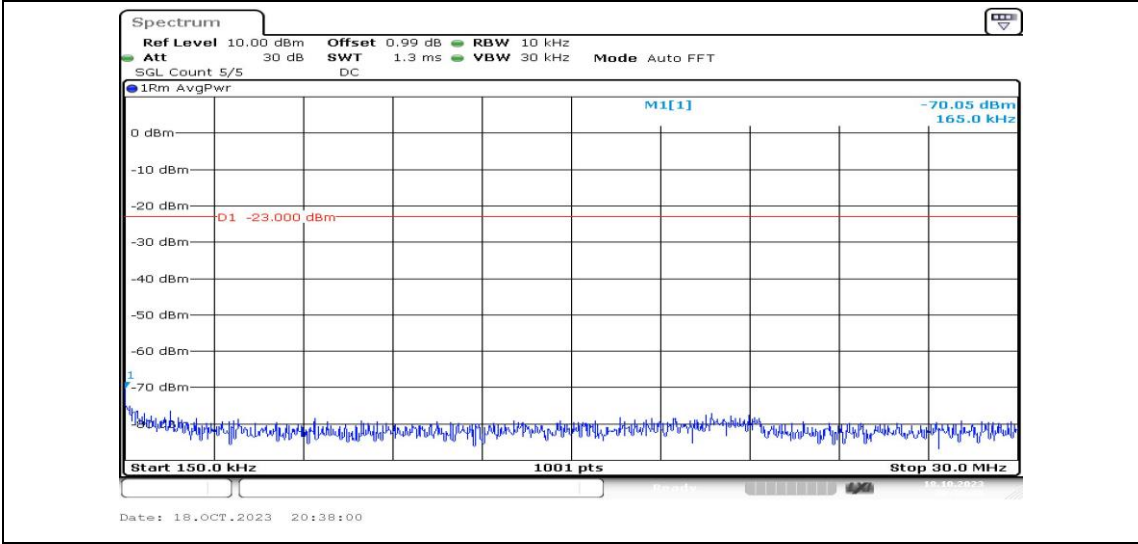
Band2-15MHz-QPSK-19125-1RB#0-Range2:0.15~30MHz-PASS
