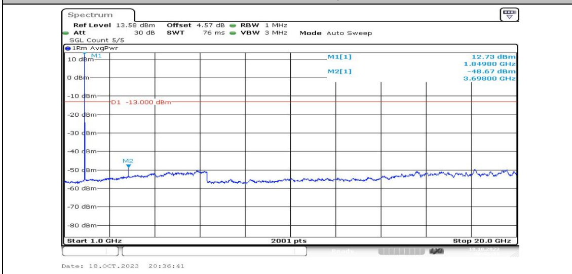
Band2-15MHz-QPSK-18675-1RB#0-Range4:1000~20000MHz-PASS
