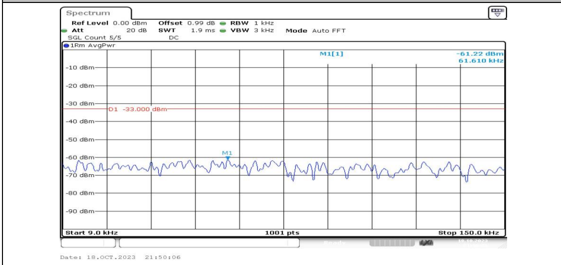
Band2-10MHz-16QAM-18650-1RB#0-Range1:0.009~0.15MHz-PASS
