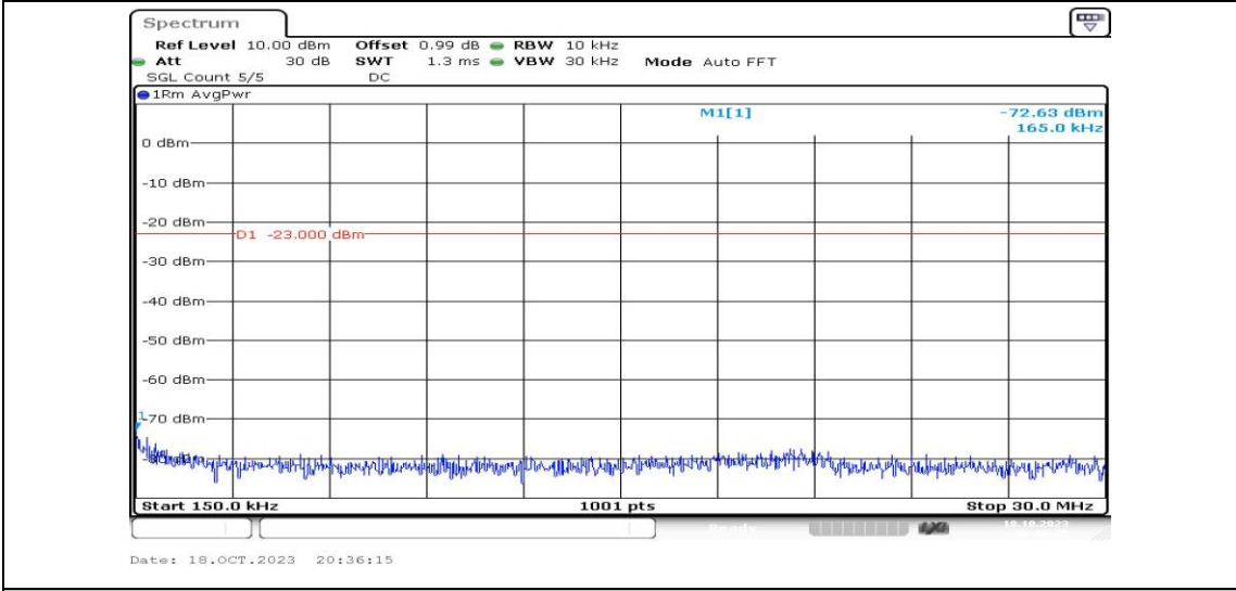
Band2-15MHz-QPSK-18675-1RB#0-Range2:0.15~30MHz-PASS
