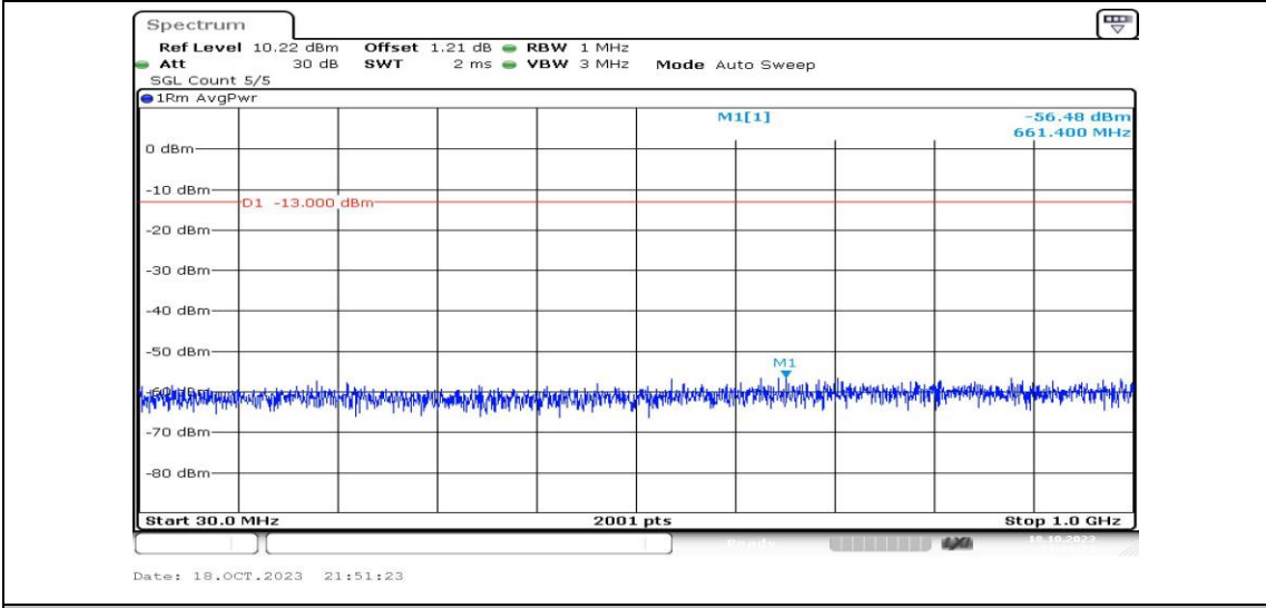
Band2-10MHz-16QAM-18900-1RB#0-Range3:30~1000MHz-PASS
