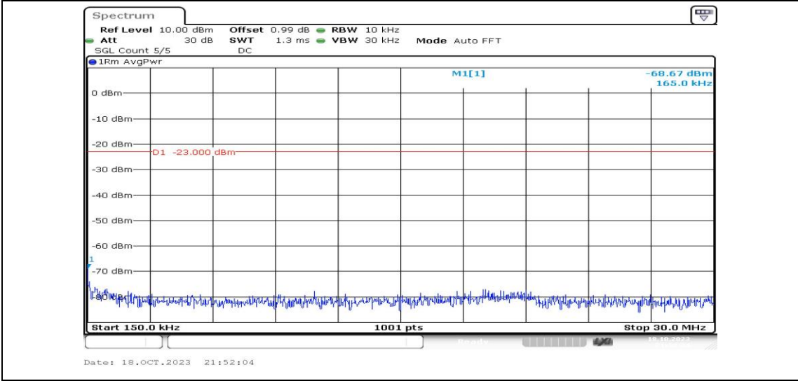
Band2-10MHz-16QAM-19150-1RB#0-Range2:0.15~30MHz-PASS
