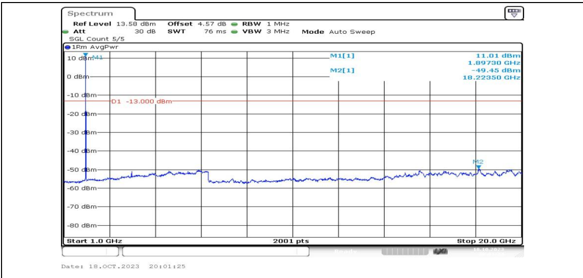
Band2-10MHz-QPSK-19150-1RB#0-Range4:1000~20000MHz-PASS
