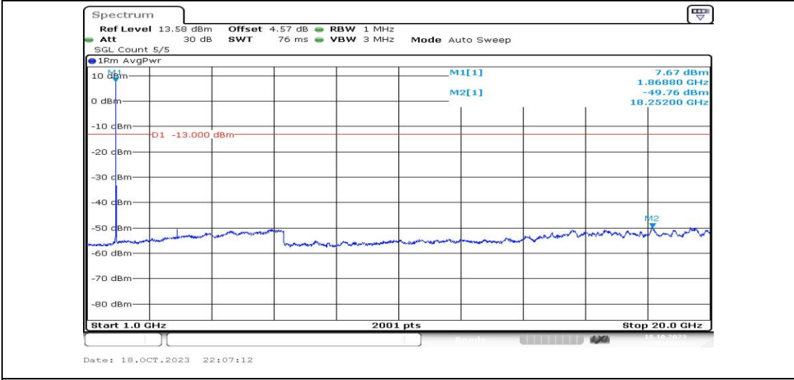
Band2-15MHz-16QAM-18900-1RB#0-Range4:1000~20000MHz-PASS
