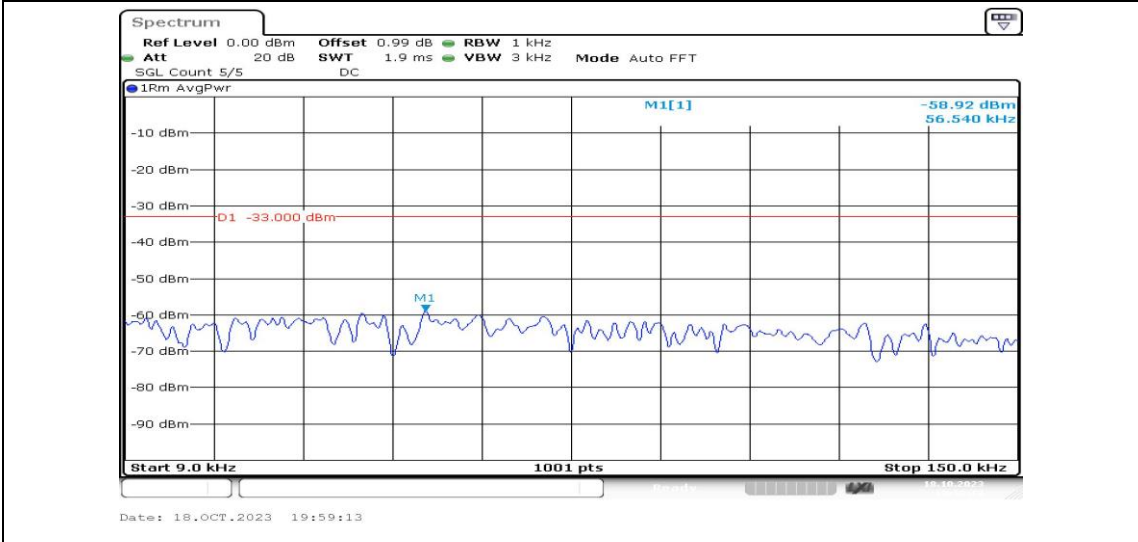
Band2-10MHz-QPSK-18650-1RB#0-Range1:0.009~0.15MHz-PASS
