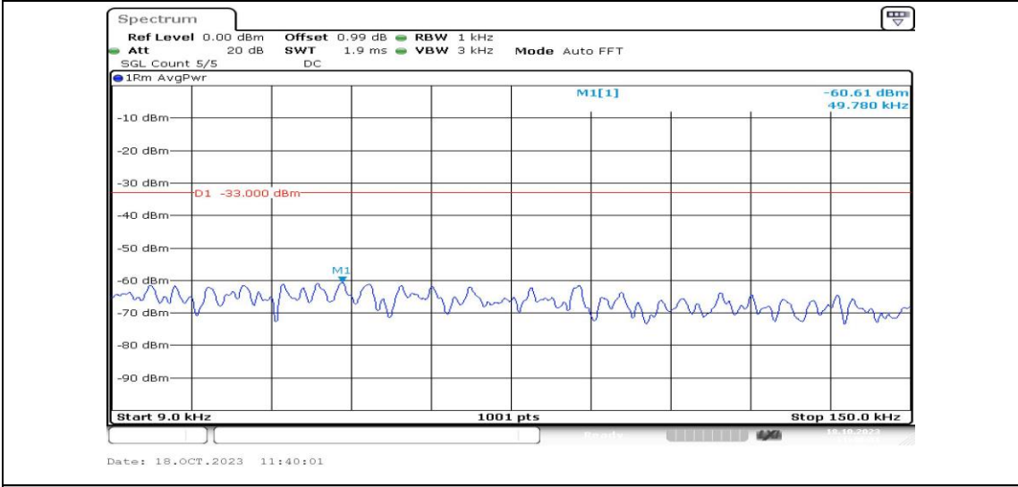
Band2-5MHz-QPSK-19175-1RB#0-Range1:0.009~0.15MHz-PASS
