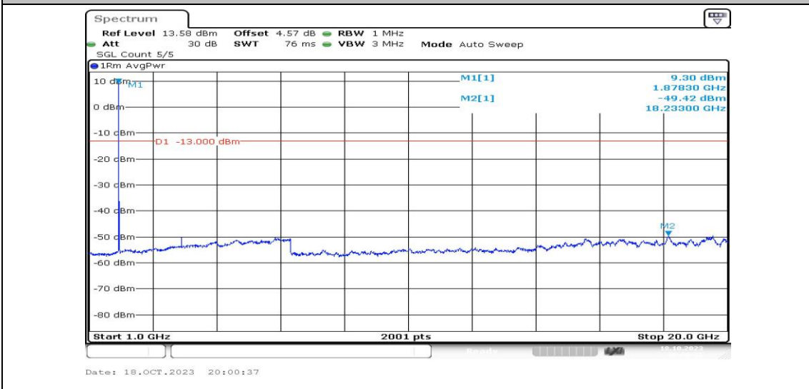
Band2-10MHz-QPSK-18900-1RB#0-Range4:1000~20000MHz-PASS
