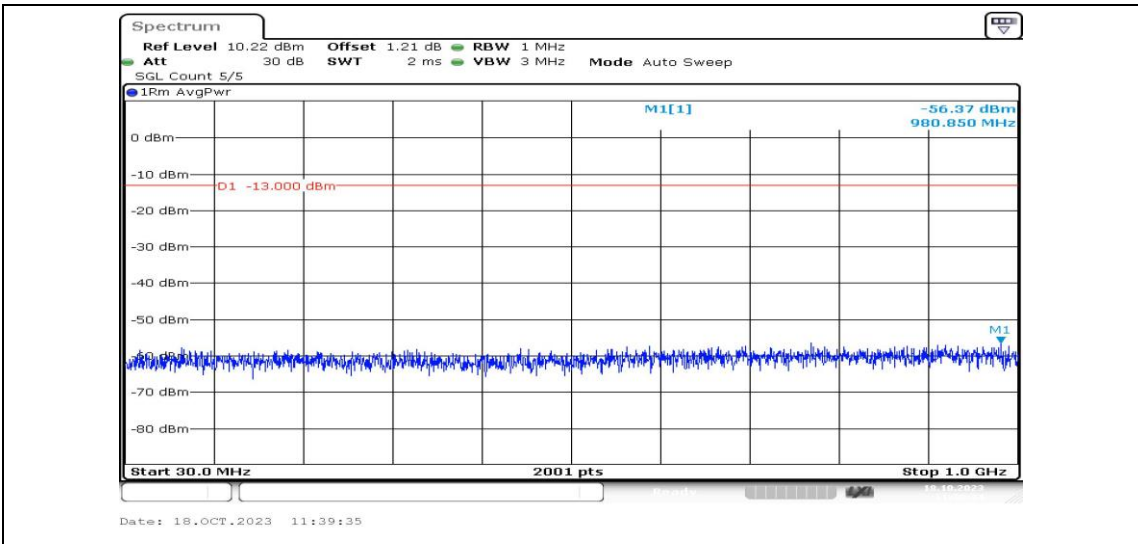
Band2-5MHz-16QAM-18900-1RB#0-Range3:30~1000MHz-PASS
