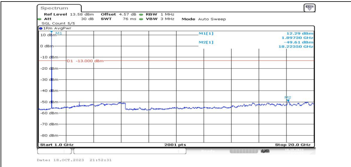
Band2-10MHz-16QAM-19150-1RB#0-Range4:1000~20000MHz-PASS
