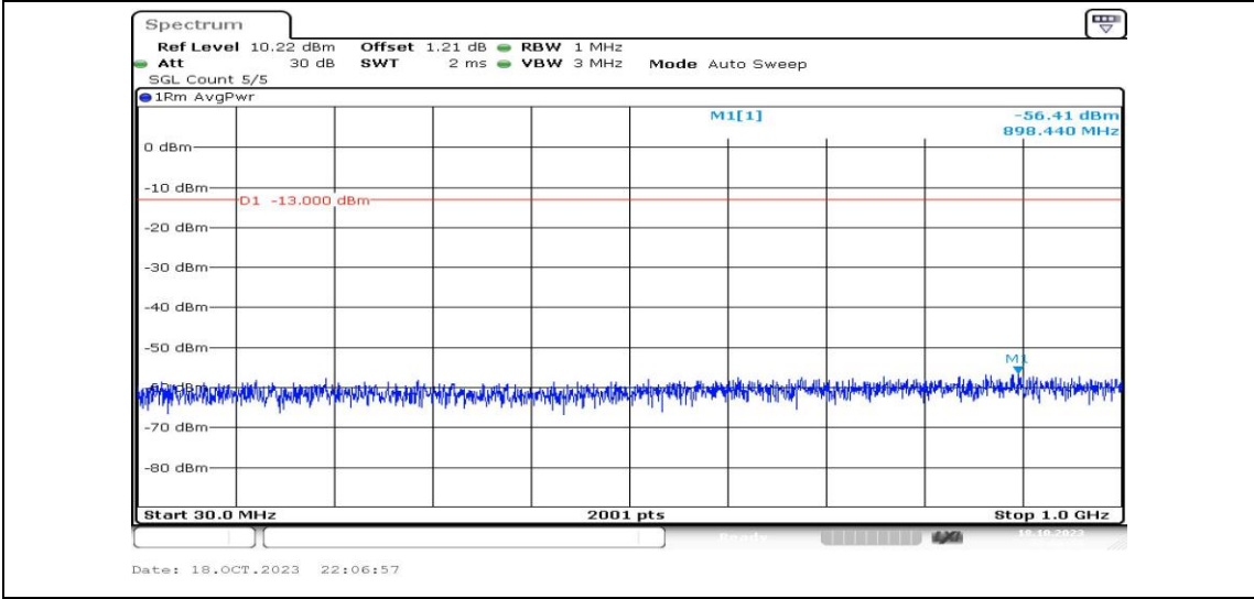
Band2-15MHz-16QAM-18900-1RB#0-Range3:30~1000MHz-PASS
