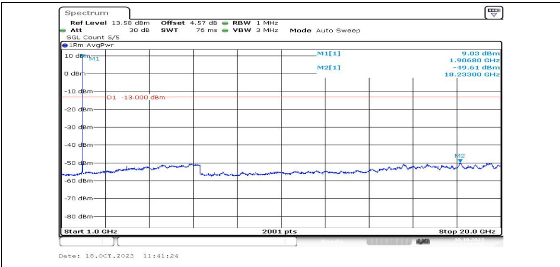
Band2-5MHz-16QAM-19175-1RB#0-Range4:1000~20000MHz-PASS
