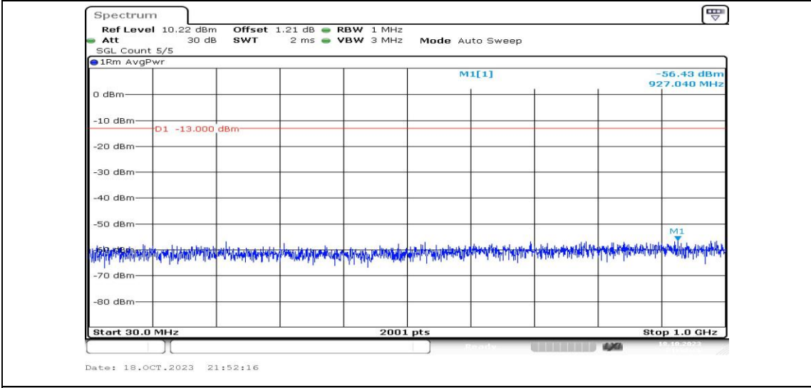
Band2-10MHz-16QAM-19150-1RB#0-Range3:30~1000MHz-PASS
