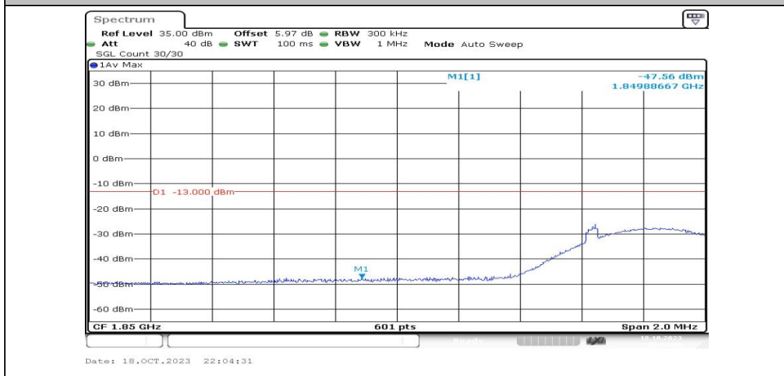
Band2-15MHz-16QAM-18675-1RB#74-PASS
