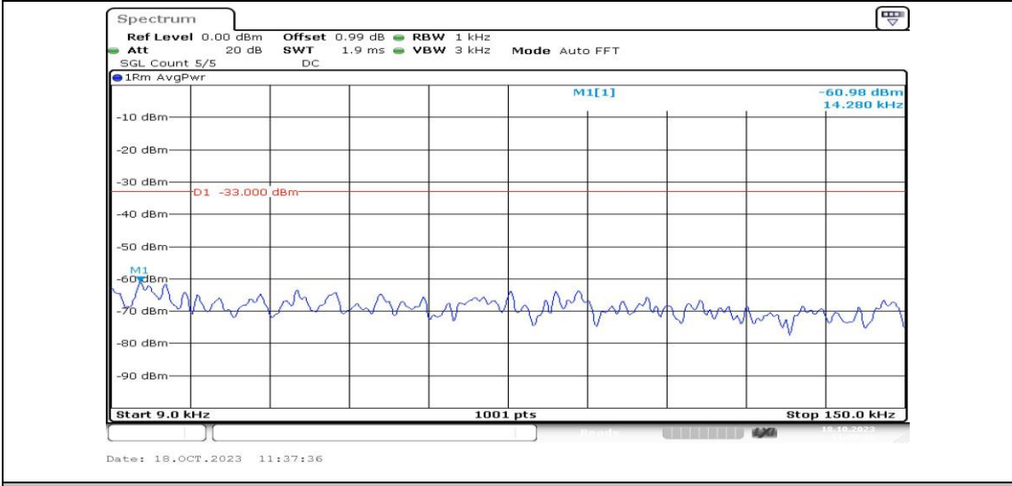
Band2-5MHz-16QAM-18625-1RB#0-Range1:0.009~0.15MHz-PASS
