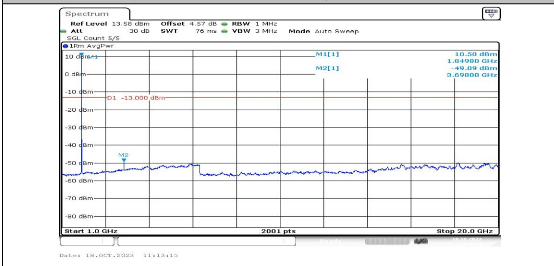
Band2-3MHz-16QAM-18615-1RB#0-Range4:1000~20000MHz-PASS
