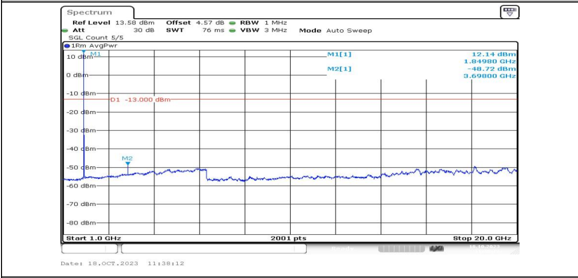
Band2-5MHz-16QAM-18625-1RB#0-Range4:1000~20000MHz-PASS
