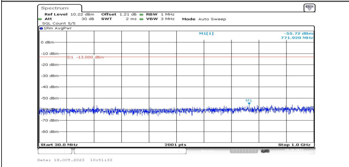
Band2-1.4MHz-QPSK-19193-1RB#0-Range3:30~1000MHz-PASS
