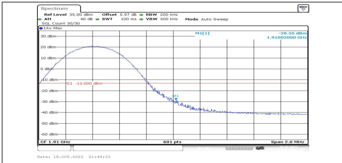
Band2-10MHz-16QAM-19150-1RB#49-PASS
