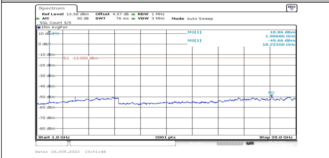
Band2-1.4MHz-QPSK-19193-1RB#0-Range4:1000~20000MHz-PASS
