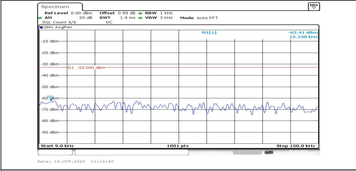
Band2-3MHz-16QAM-18615-1RB#0-Range1:0.009~0.15MHz-PASS
