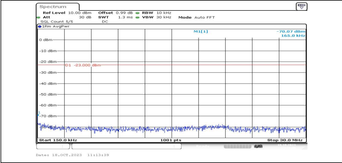
Band2-3MHz-QPSK-18900-1RB#0-Range2:0.15~30MHz-PASS
