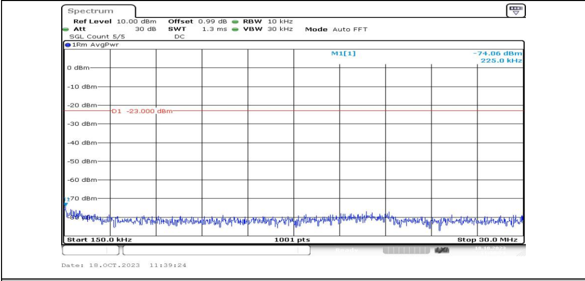
Band2-5MHz-16QAM-18900-1RB#0-Range2:0.15~30MHz-PASS
