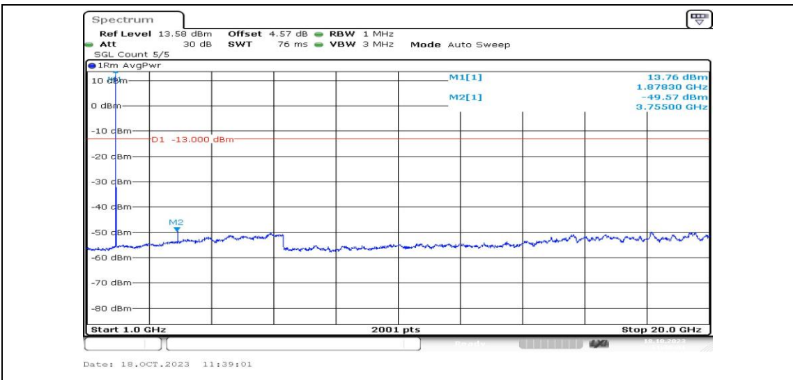
Band2-5MHz-QPSK-18900-1RB#0-Range4:1000~20000MHz-PASS
