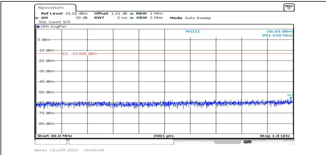
Band2-1.4MHz-16QAM-18900-1RB#0-Range3:30~1000MHz-PASS
