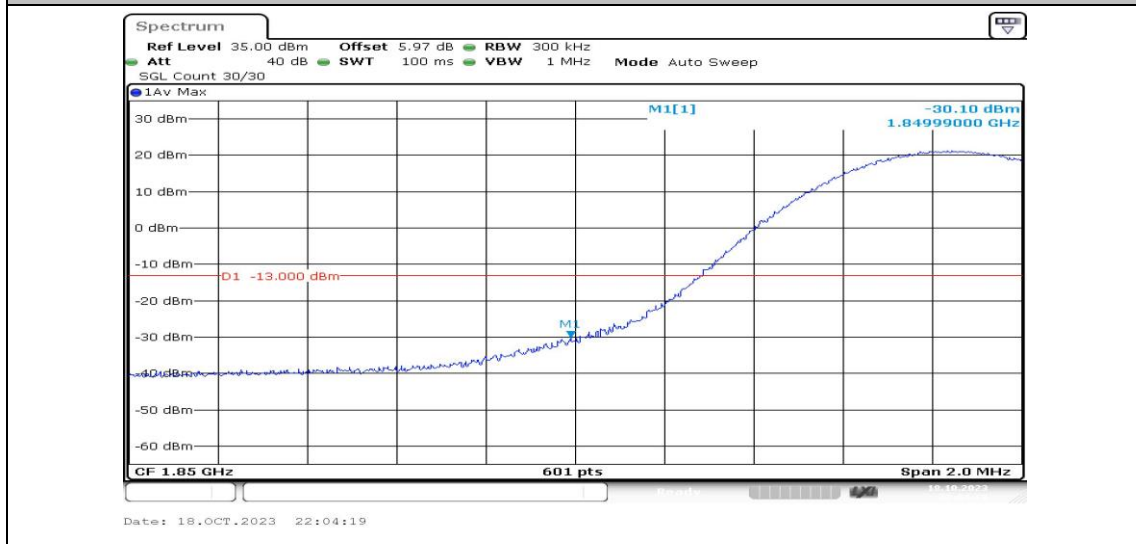
Band2-15MHz-16QAM-18675-1RB#0-PASS
