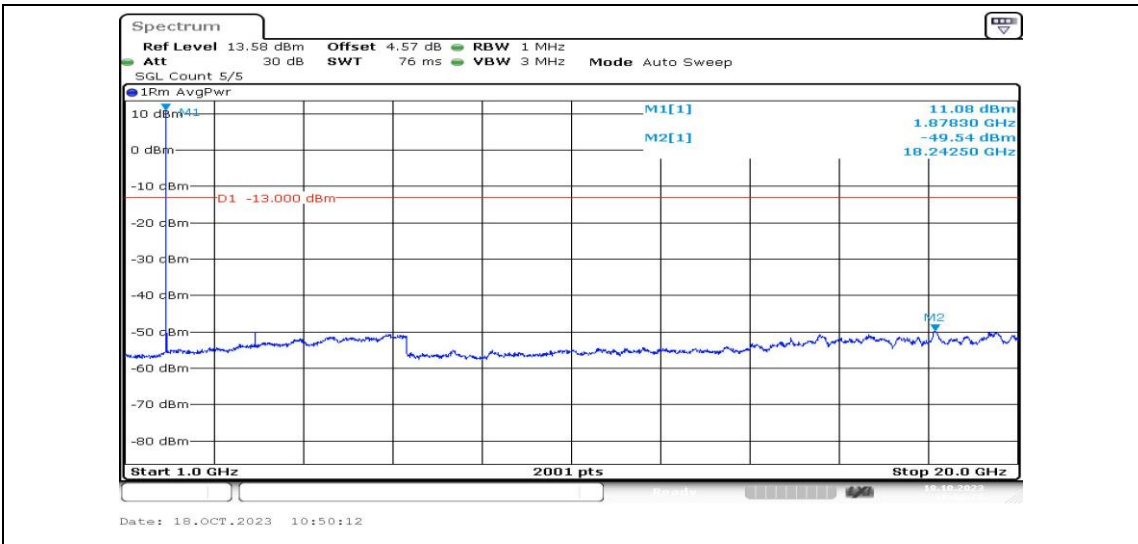
Band2-1.4MHz-QPSK-18900-1RB#0-Range4:1000~20000MHz-PASS
