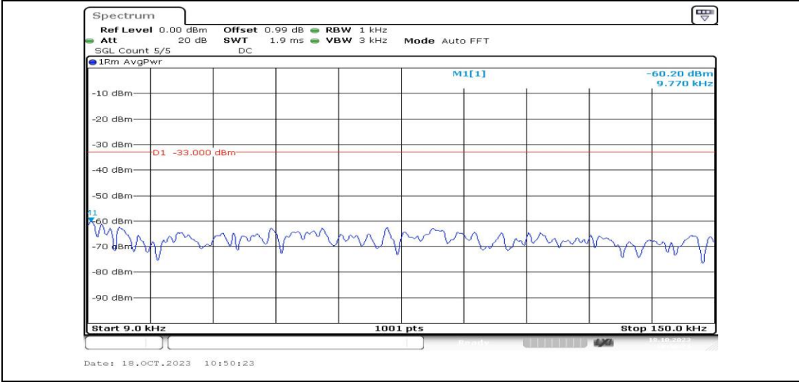
Band2-1.4MHz-16QAM-18900-1RB#0-Range1:0.009~0.15MHz-PASS
