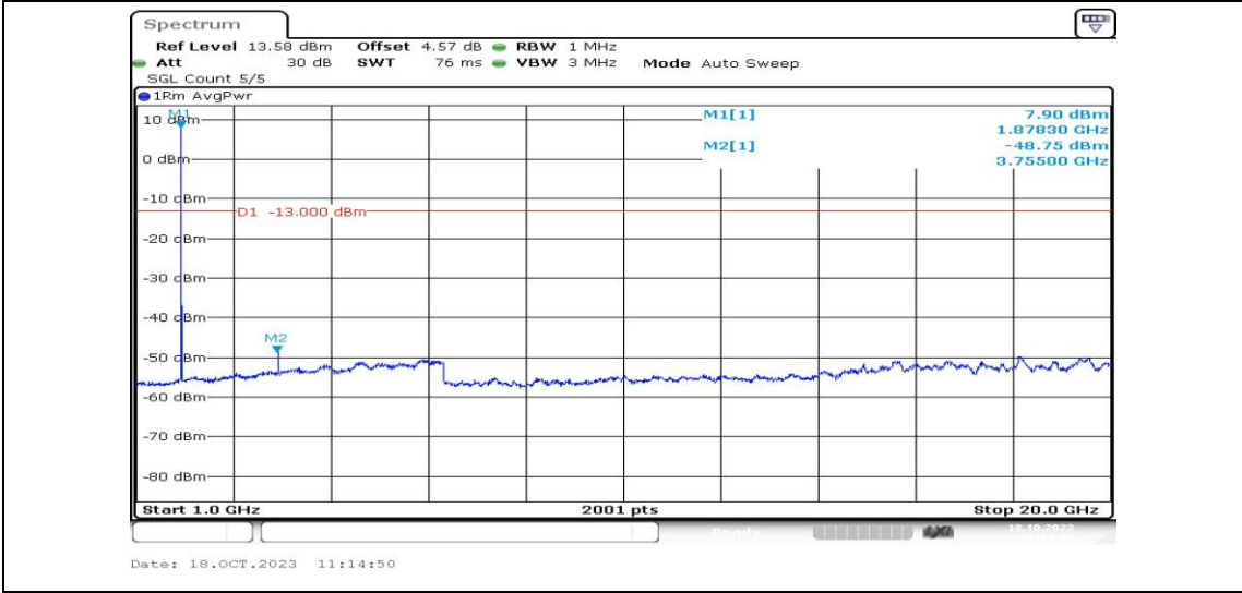
Band2-3MHz-16QAM-18900-1RB#0-Range4:1000~20000MHz-PASS
