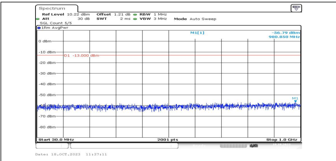
Band2-5MHz-QPSK-18625-1RB#0-Range3:30~1000MHz-PASS
