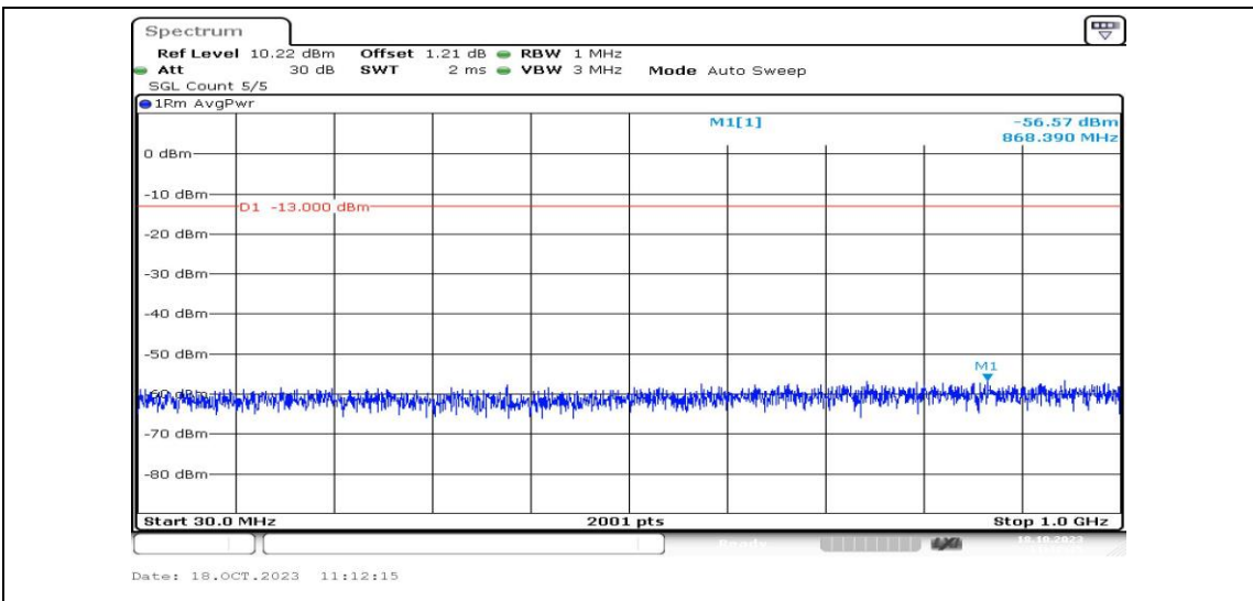
Band2-3MHz-QPSK-18615-1RB#0-Range3:30~1000MHz-PASS
