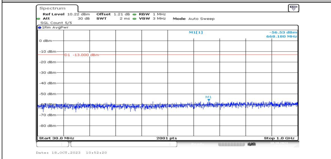
Band2-1.4MHz-16QAM-19193-1RB#0-Range3:30~1000MHz-PASS
