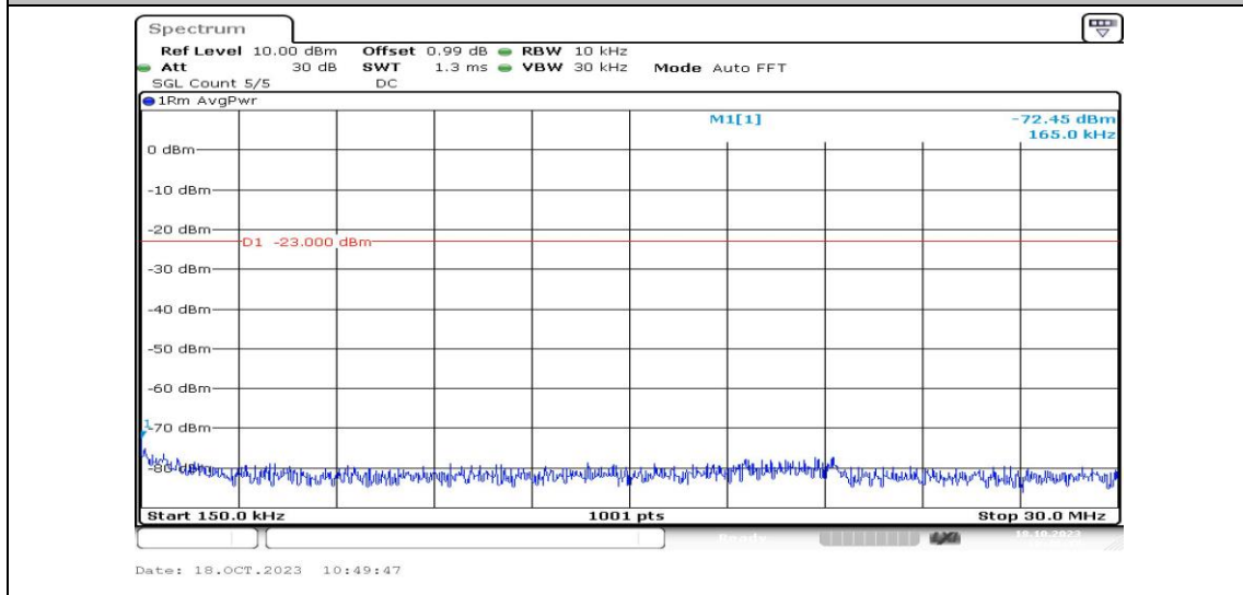
Band2-1.4MHz-QPSK-18900-1RB#0-Range2:0.15~30MHz-PASS
