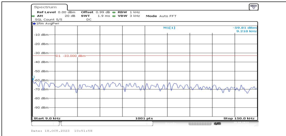
Band2-1.4MHz-16QAM-19193-1RB#0-Range1:0.009~0.15MHz-PASS
