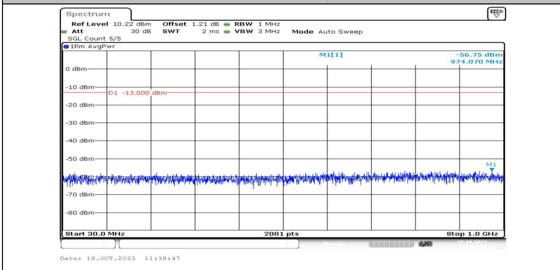
Band2-5MHz-QPSK-18900-1RB#0-Range3:30~1000MHz-PASS
