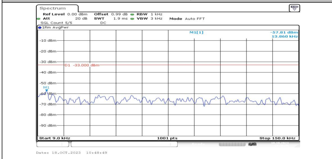
Band2-1.4MHz-16QAM-18607-1RB#0-Range1:0.009~0.15MHz-PASS
