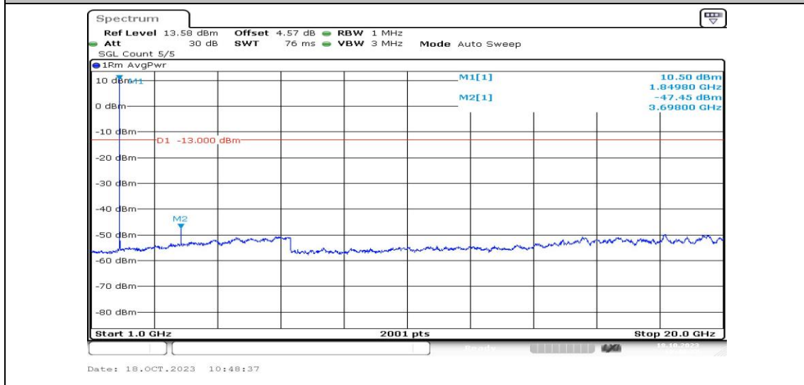
Band2-1.4MHz-QPSK-18607-1RB#0-Range4:1000~20000MHz-PASS
