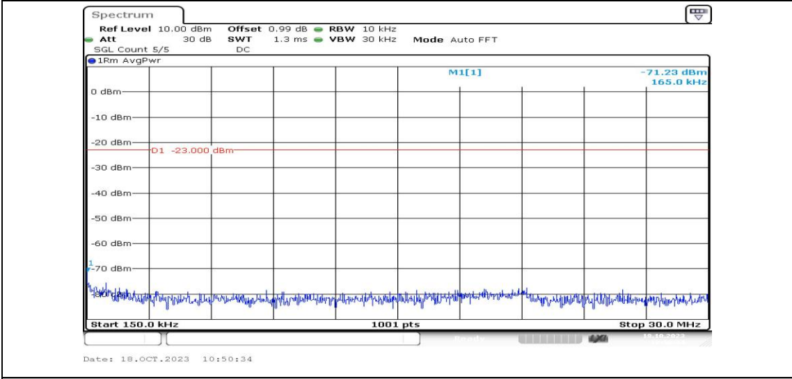
Band2-1.4MHz-16QAM-18900-1RB#0-Range2:0.15~30MHz-PASS
