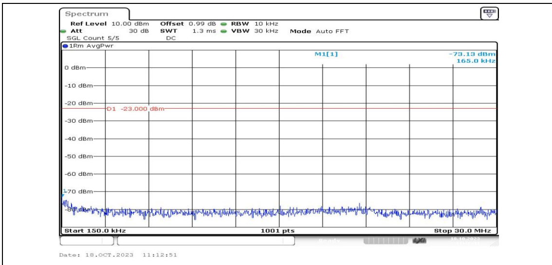
Band2-3MHz-16QAM-18615-1RB#0-Range2:0.15~30MHz-PASS
