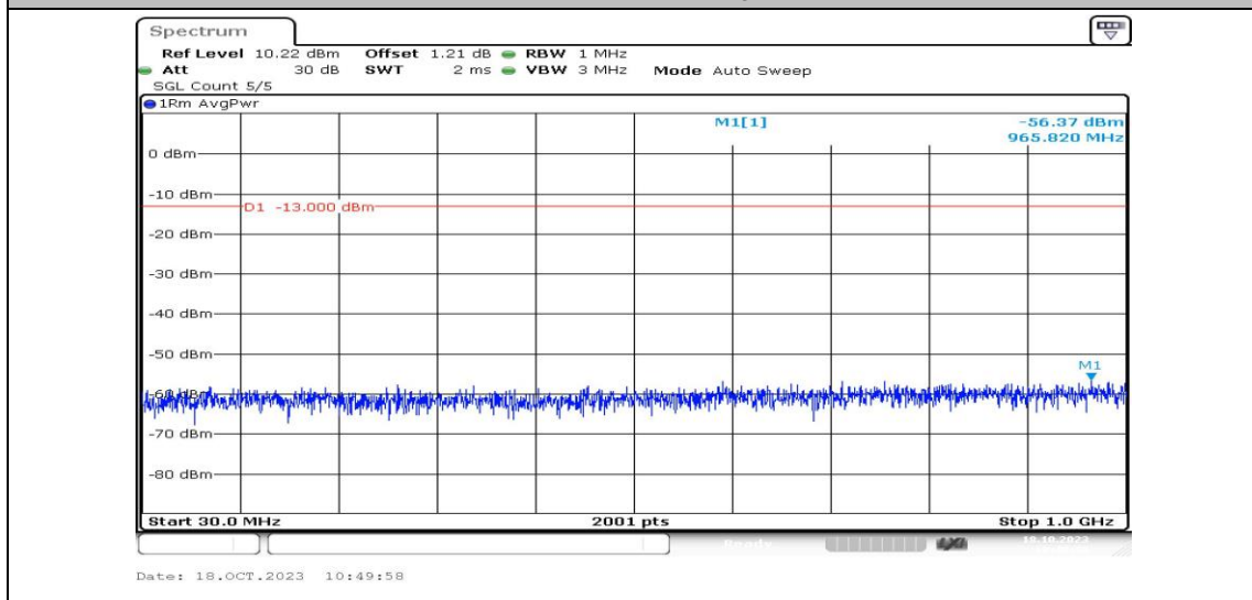
Band2-1.4MHz-QPSK-18900-1RB#0-Range3:30~1000MHz-PASS
