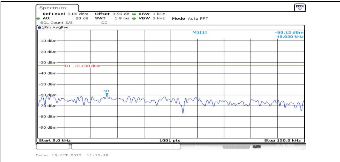
Band2-3MHz-QPSK-18900-1RB#0-Range1:0.009~0.15MHz-PASS
