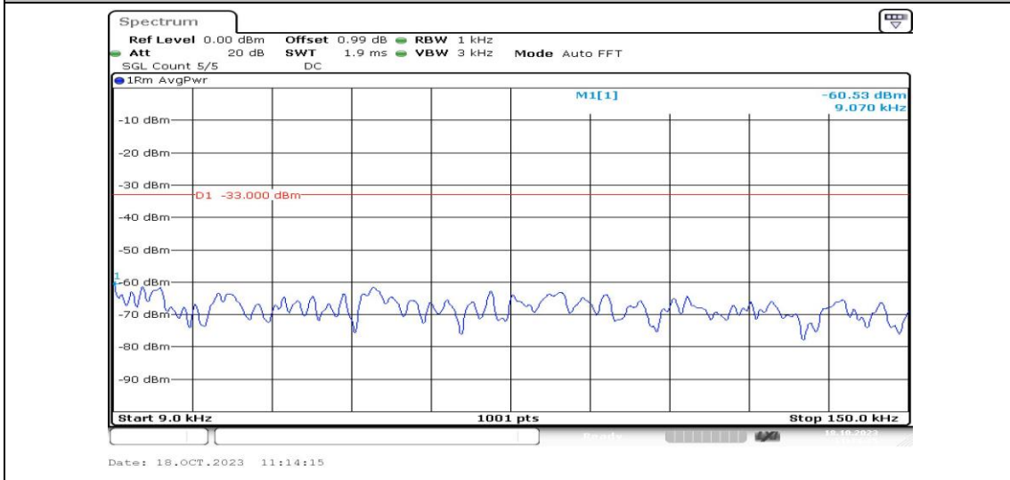
Band2-3MHz-16QAM-18900-1RB#0-Range1:0.009~0.15MHz-PASS
