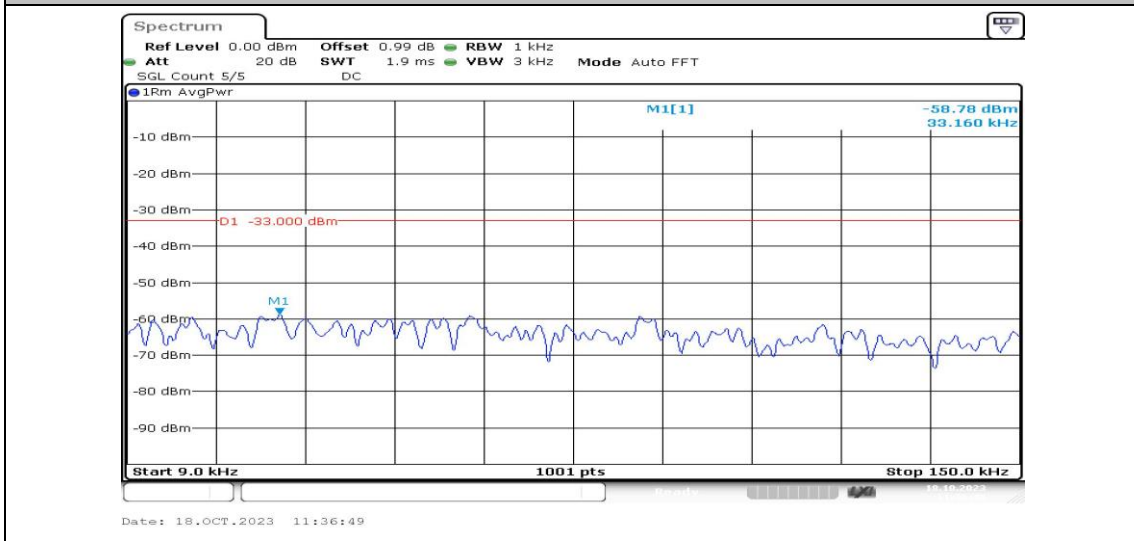
Band2-5MHz-QPSK-18625-1RB#0-Range1:0.009~0.15MHz-PASS
