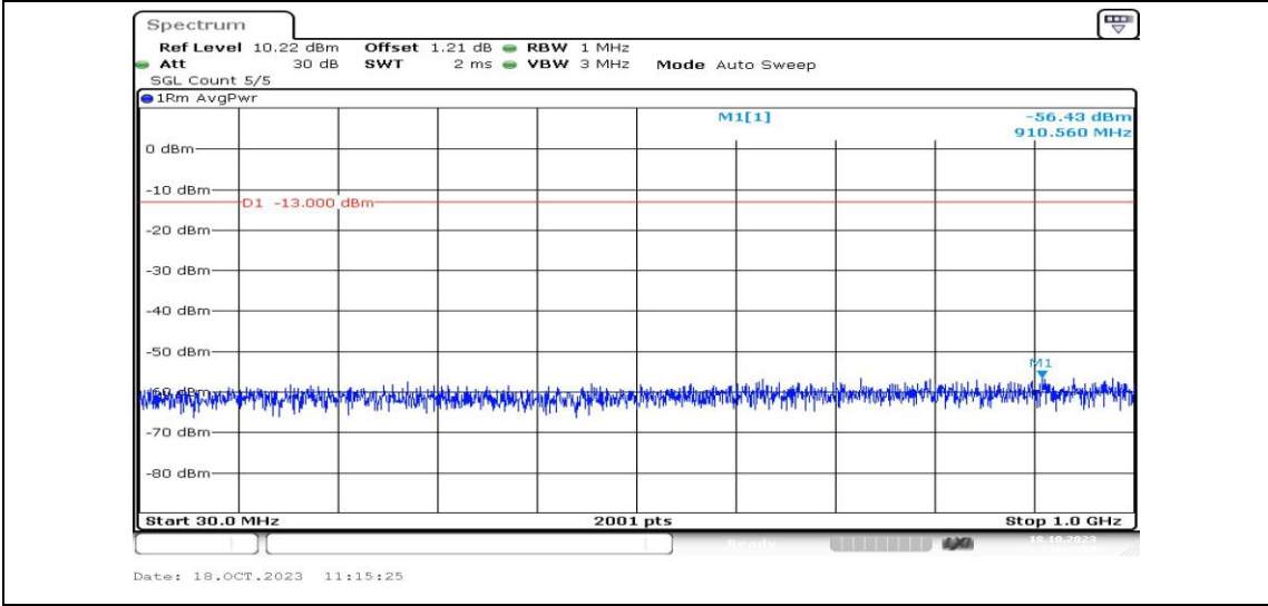
Band2-3MHz-QPSK-19185-1RB#0-Range3:30~1000MHz-PASS
