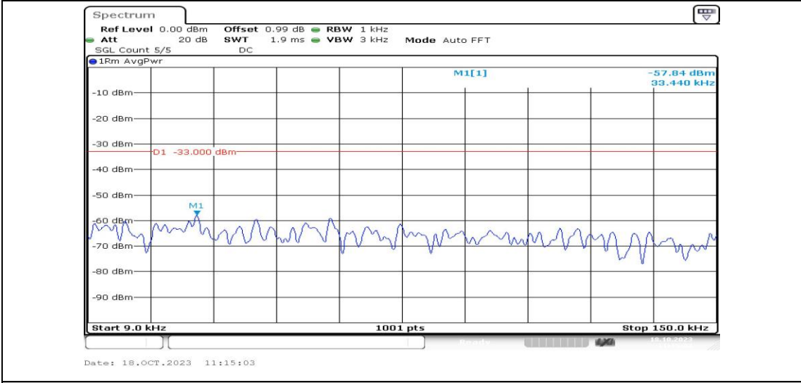
Band2-3MHz-QPSK-19185-1RB#0-Range1:0.009~0.15MHz-PASS
