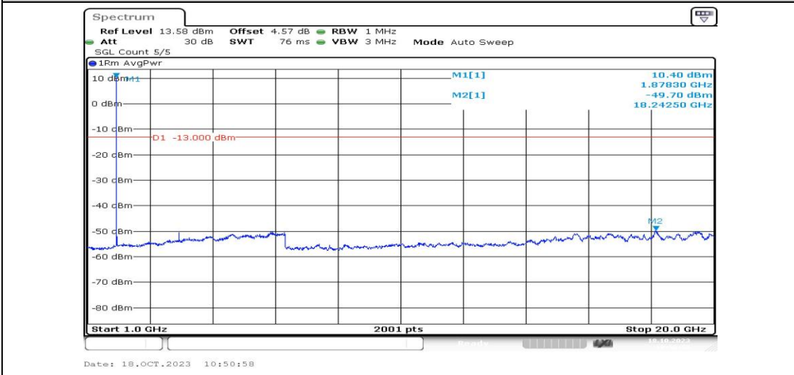
Band2-1.4MHz-16QAM-18900-1RB#0-Range4:1000~20000MHz-PASS
