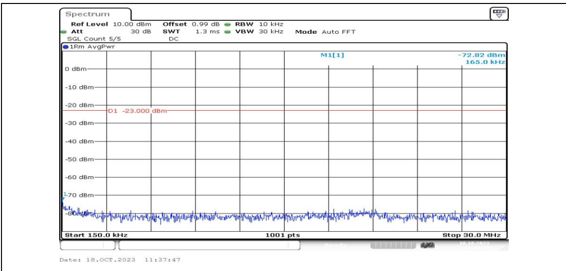
Band2-5MHz-16QAM-18625-1RB#0-Range2:0.15~30MHz-PASS
