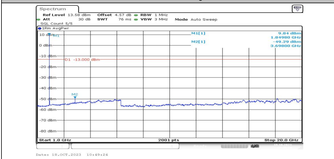
Band2-1.4MHz-16QAM-18607-1RB#0-Range4:1000~20000MHz-PASS
