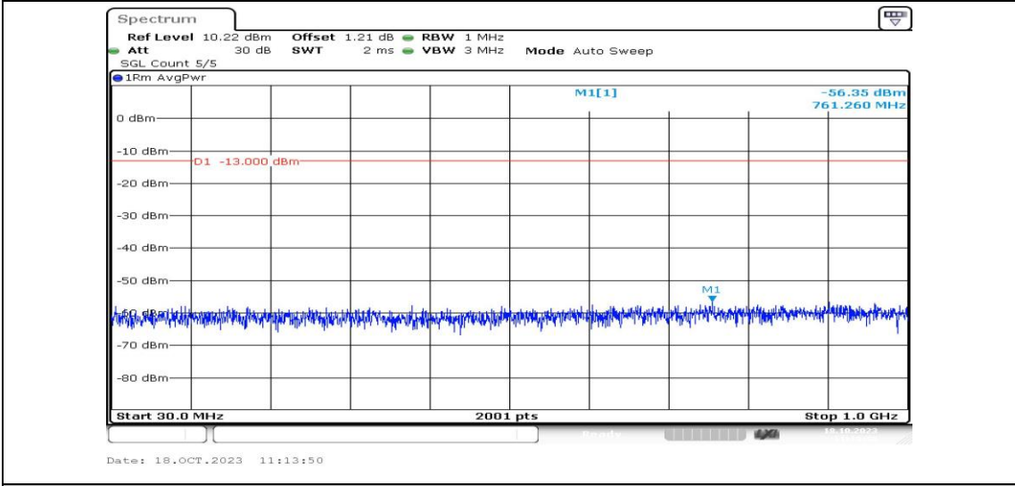
Band2-3MHz-QPSK-18900-1RB#0-Range3:30~1000MHz-PASS
