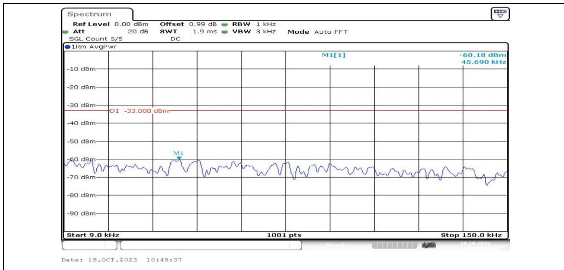
Band2-1.4MHz-QPSK-18900-1RB#0-Range1:0.009~0.15MHz-PASS
