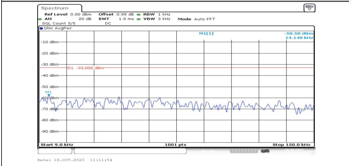
Band2-3MHz-QPSK-18615-1RB#0-Range1:0.009~0.15MHz-PASS
