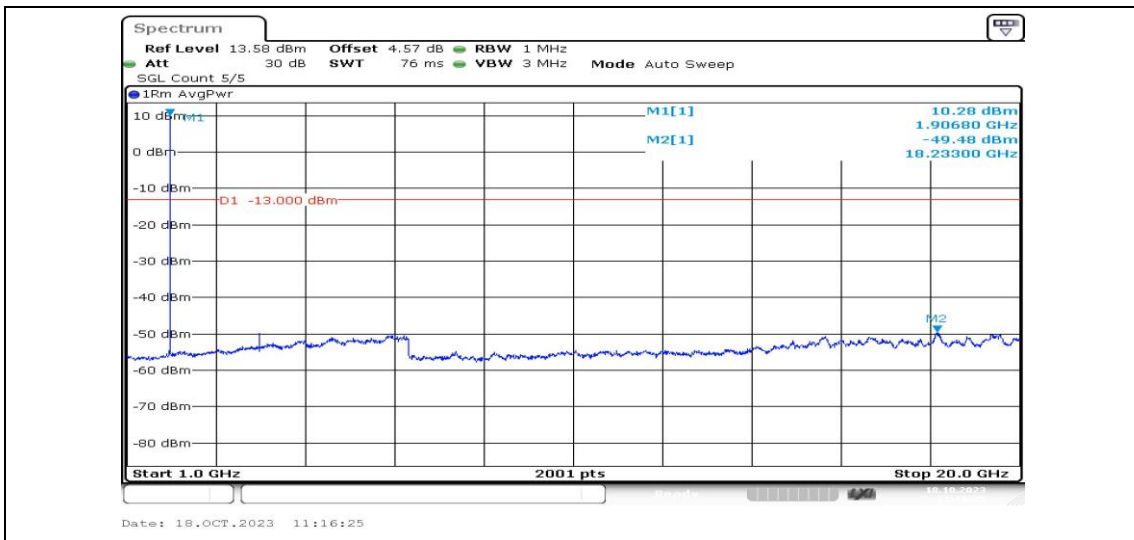
Band2-3MHz-16QAM-19185-1RB#0-Range4:1000~20000MHz-PASS
