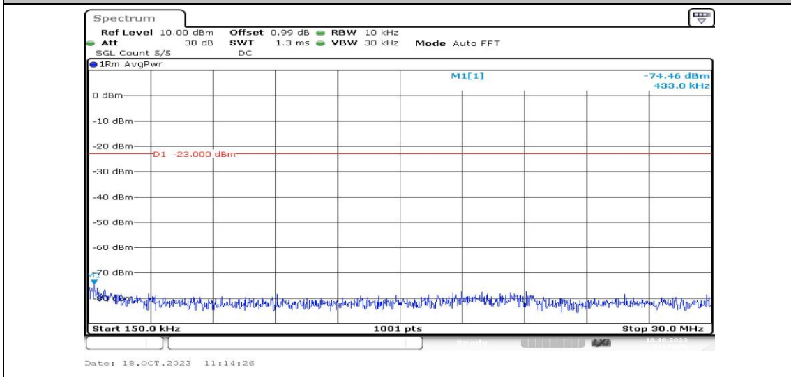
Band2-3MHz-16QAM-18900-1RB#0-Range2:0.15~30MHz-PASS
