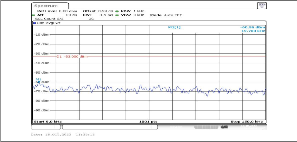
Band2-5MHz-16QAM-18900-1RB#0-Range1:0.009~0.15MHz-PASS
