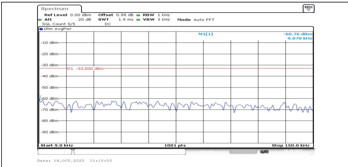
Band2-3MHz-16QAM-19185-1RB#0-Range1:0.009~0.15MHz-PASS
