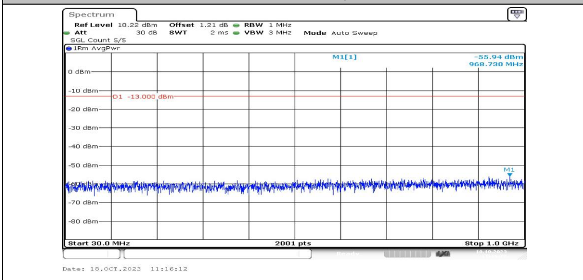
Band2-3MHz-16QAM-19185-1RB#0-Range3:30~1000MHz-PASS
