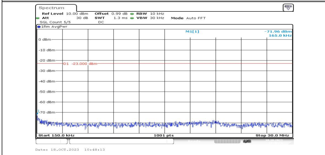
Band2-1.4MHz-QPSK-18607-1RB#0-Range2:0.15~30MHz-PASS
