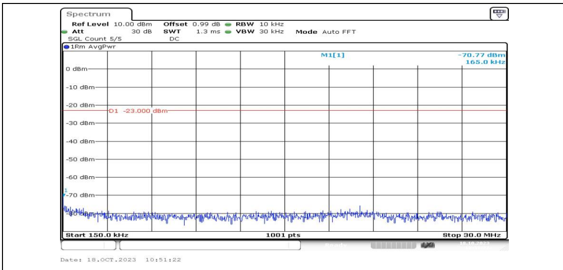
Band2-1.4MHz-QPSK-19193-1RB#0-Range2:0.15~30MHz-PASS
