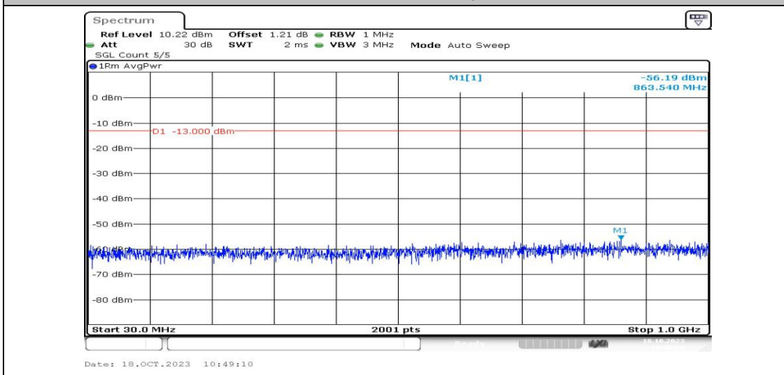
Band2-1.4MHz-16QAM-18607-1RB#0-Range3:30~1000MHz-PASS
