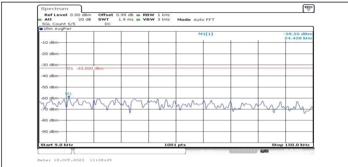
Band2-5MHz-QPSK-18900-1RB#0-Range1:0.009~0.15MHz-PASS
