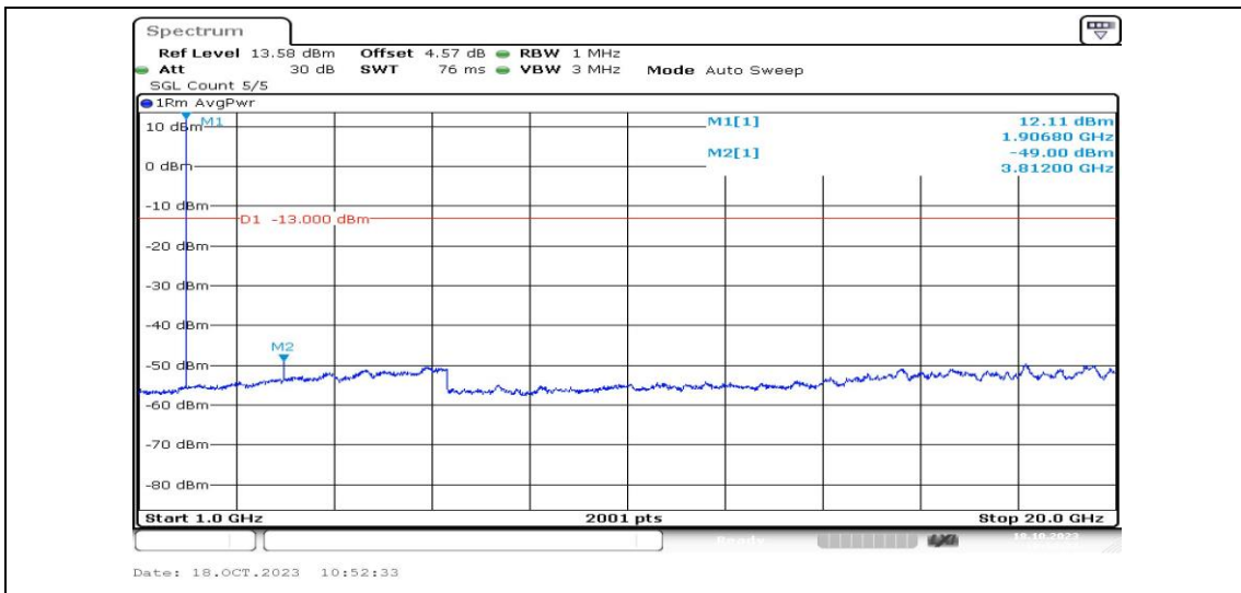
Band2-1.4MHz-16QAM-19193-1RB#0-Range4:1000~20000MHz-PASS
