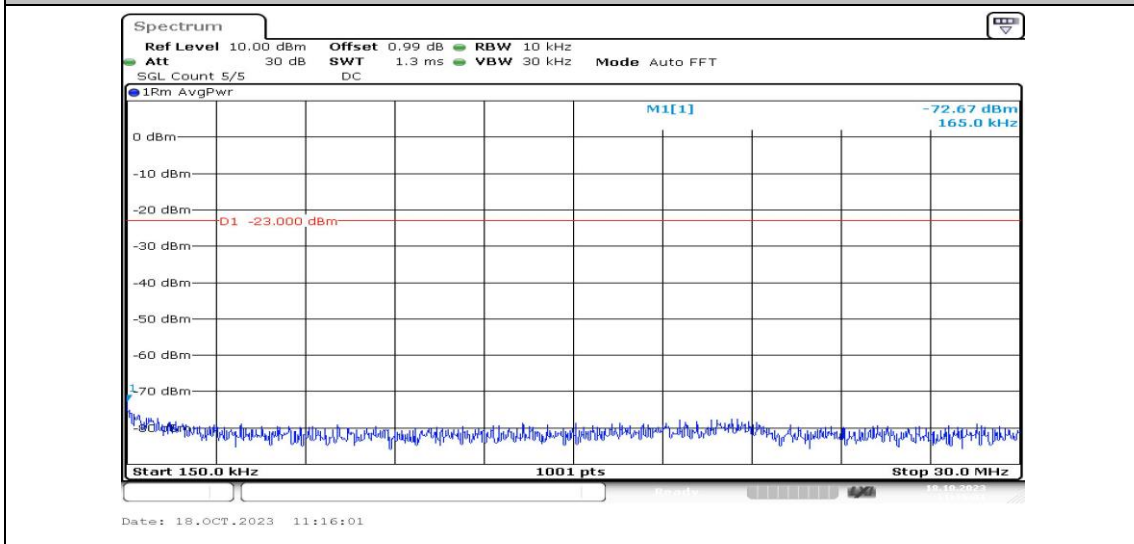
Band2-3MHz-16QAM-19185-1RB#0-Range2:0.15~30MHz-PASS
