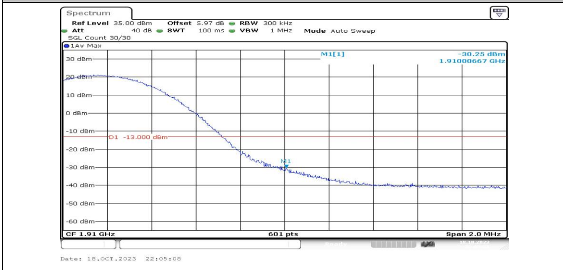
Band2-15MHz-16QAM-19125-1RB#74-PASS
