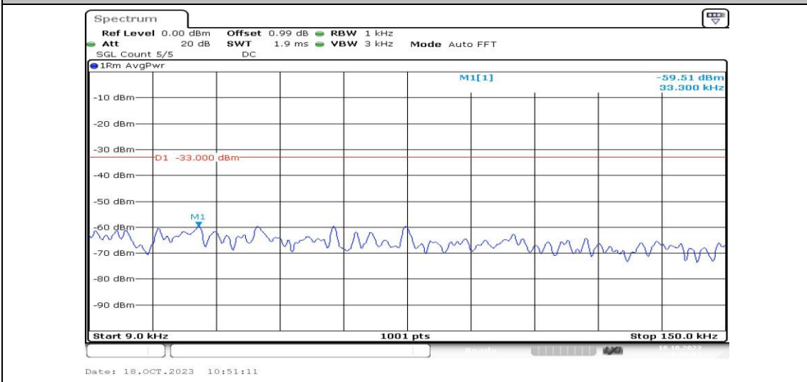
Band2-1.4MHz-QPSK-19193-1RB#0-Range1:0.009~0.15MHz-PASS
