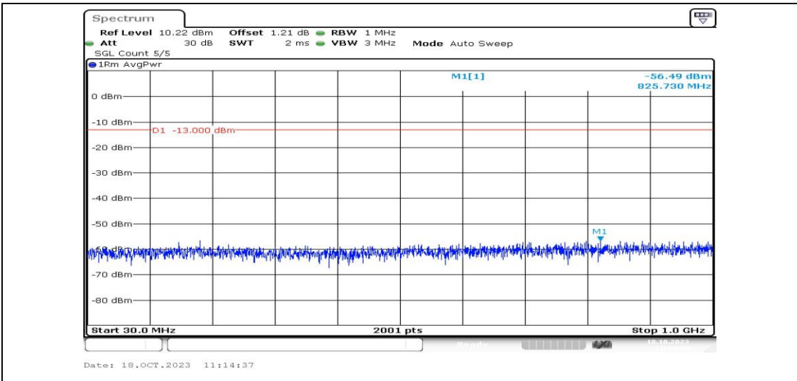
Band2-3MHz-16QAM-18900-1RB#0-Range3:30~1000MHz-PASS
