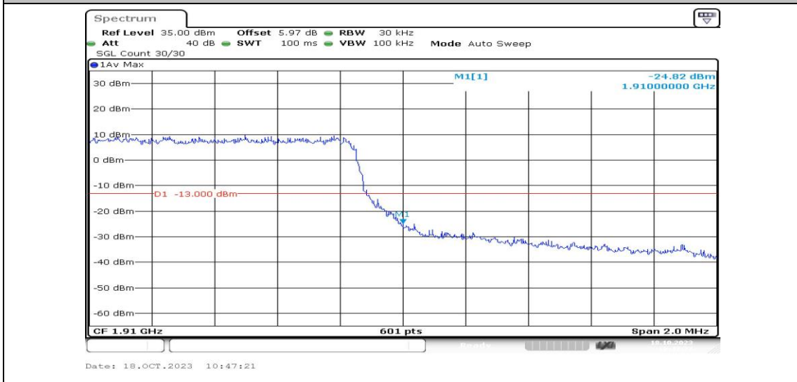
Band2-1.4MHz-QPSK-19193-6RB#0-PASS
