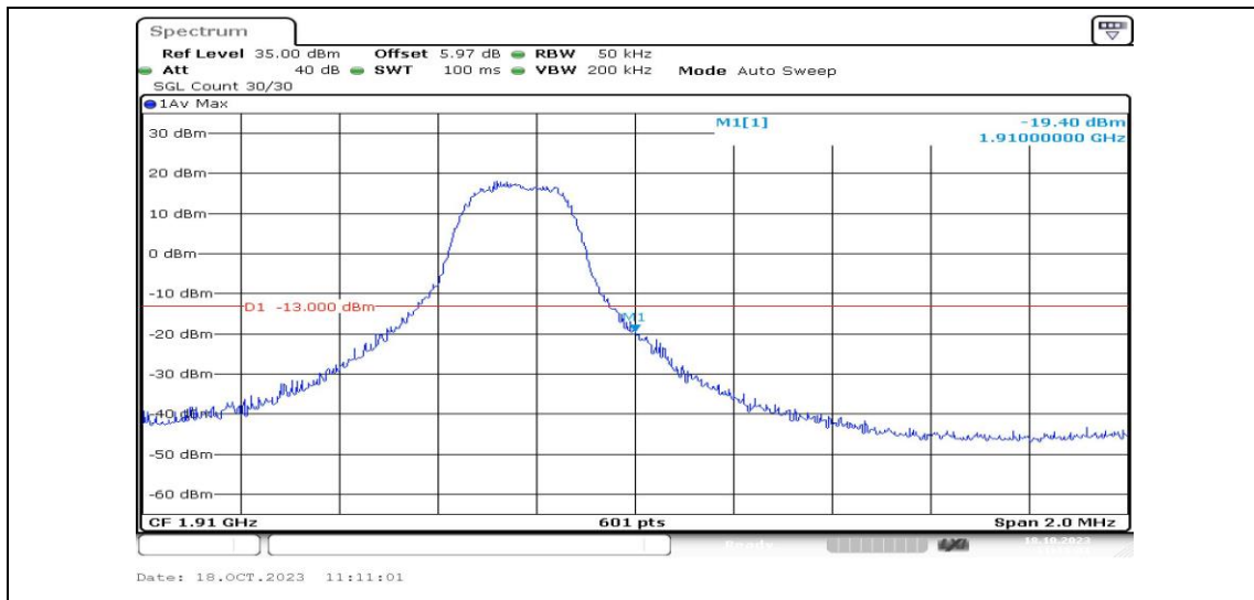
Band2-3MHz-16QAM-19185-1RB#14-PASS
