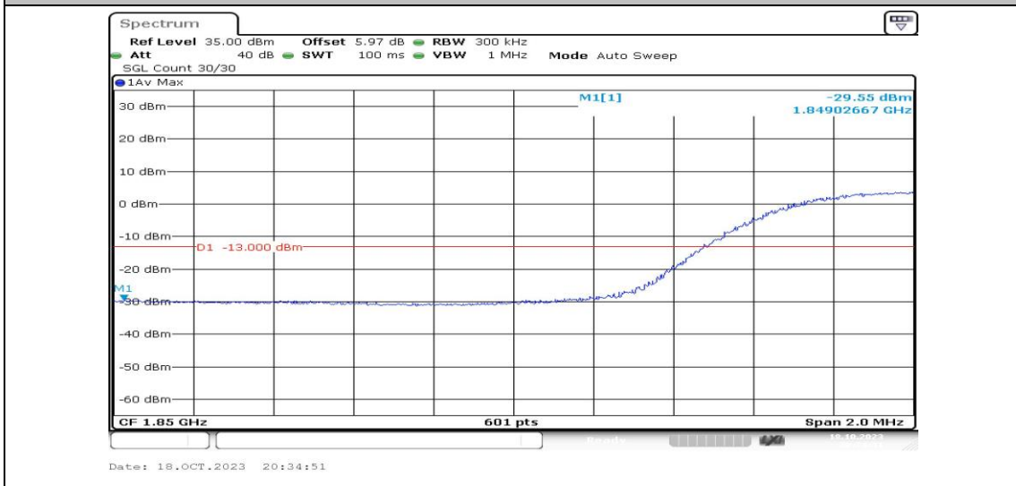
Band2-15MHz-QPSK-18675-75RB#0-PASS
