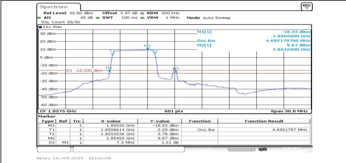
Band2-15MHz-16QAM-18675-25RB#0-PASS
