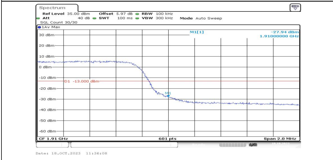
Band2-5MHz-QPSK-19175-25RB#0-PASS
