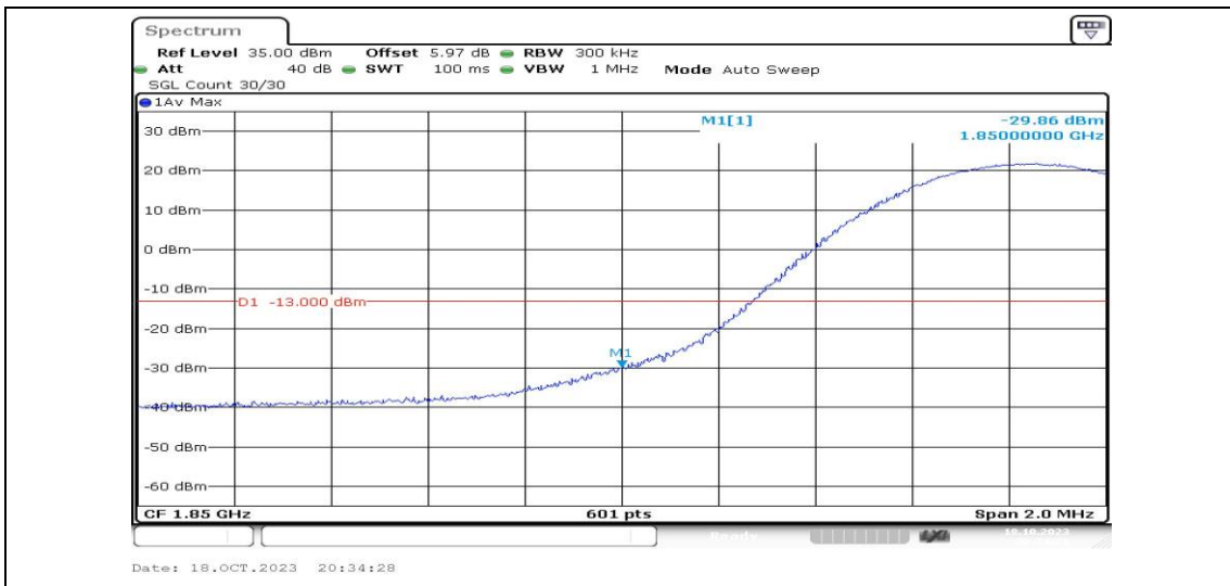
Band2-15MHz-QPSK-18675-1RB#0-PASS
