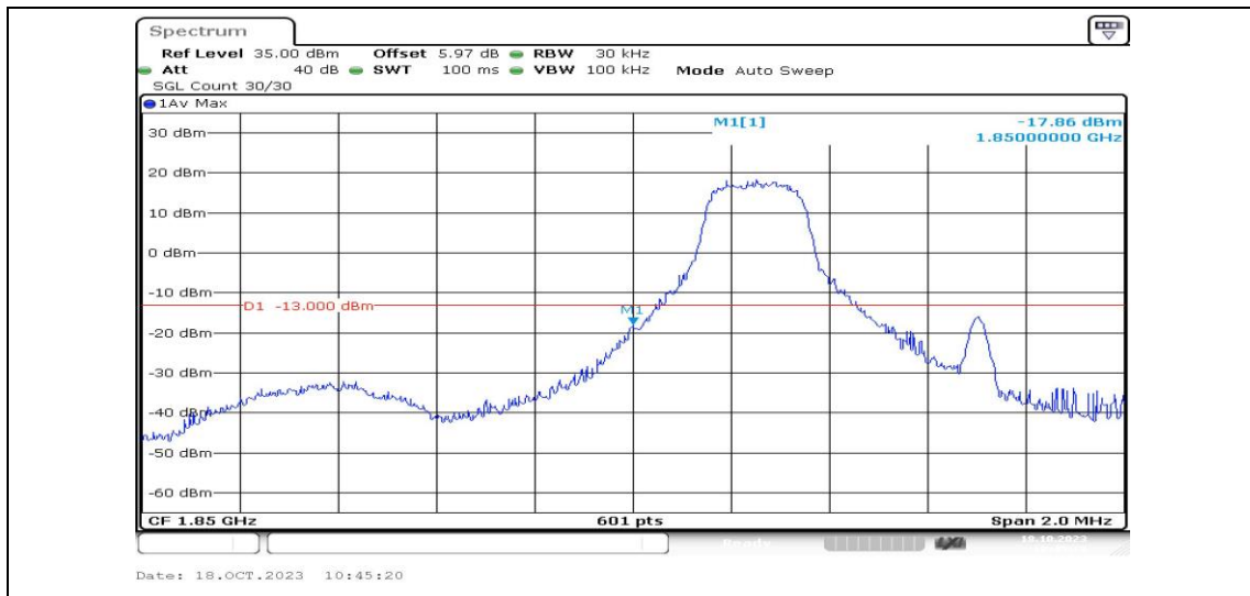
Band2-1.4MHz-QPSK-18607-1RB#0-PASS
