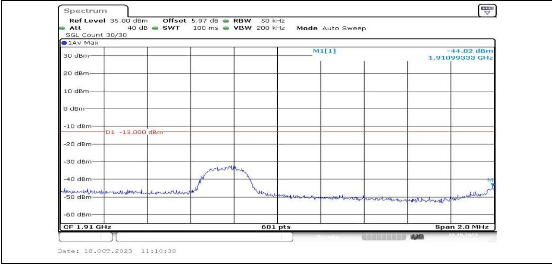
Band2-3MHz-16QAM-19185-1RB#0-PASS
