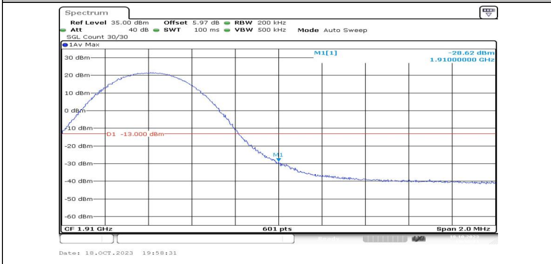
Band2-10MHz-QPSK-19150-1RB#49-PASS
