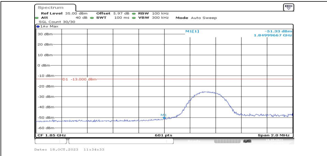
Band2-5MHz-16QAM-18625-1RB#24-PASS
