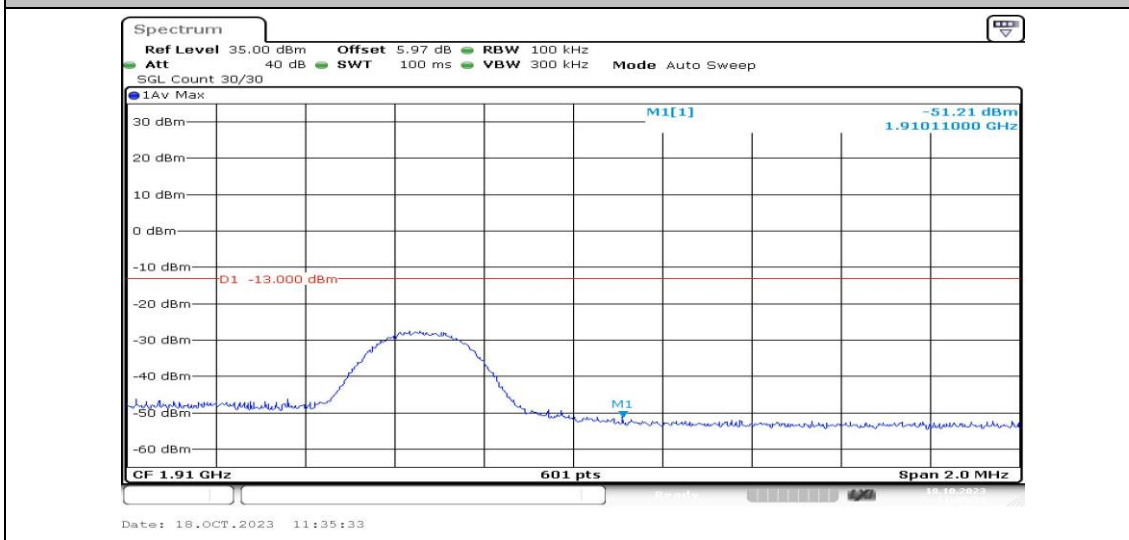
Band2-5MHz-16QAM-19175-1RB#0-PASS
