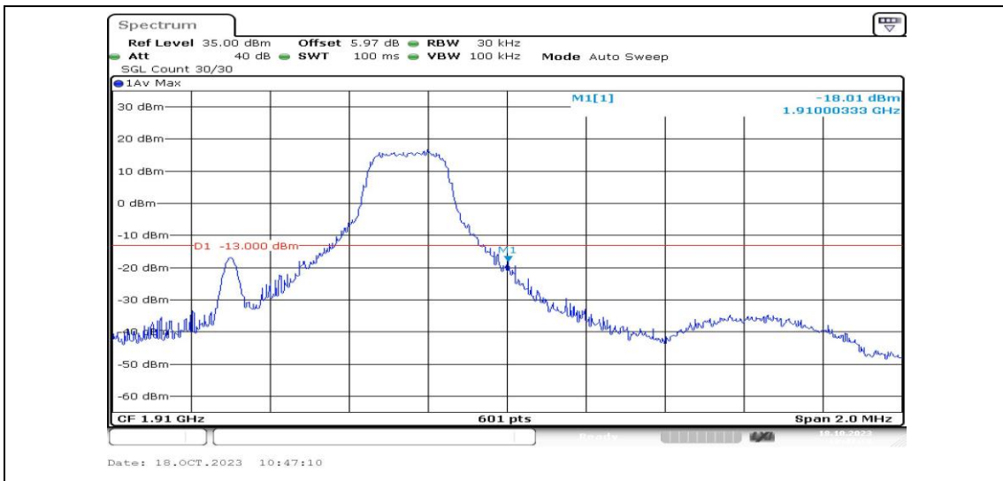
Band2-1.4MHz-16QAM-19193-1RB#5-PASS
