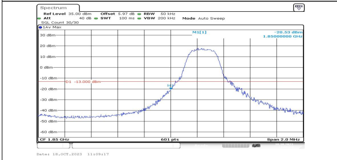
Band2-3MHz-16QAM-18615-1RB#0-PASS
