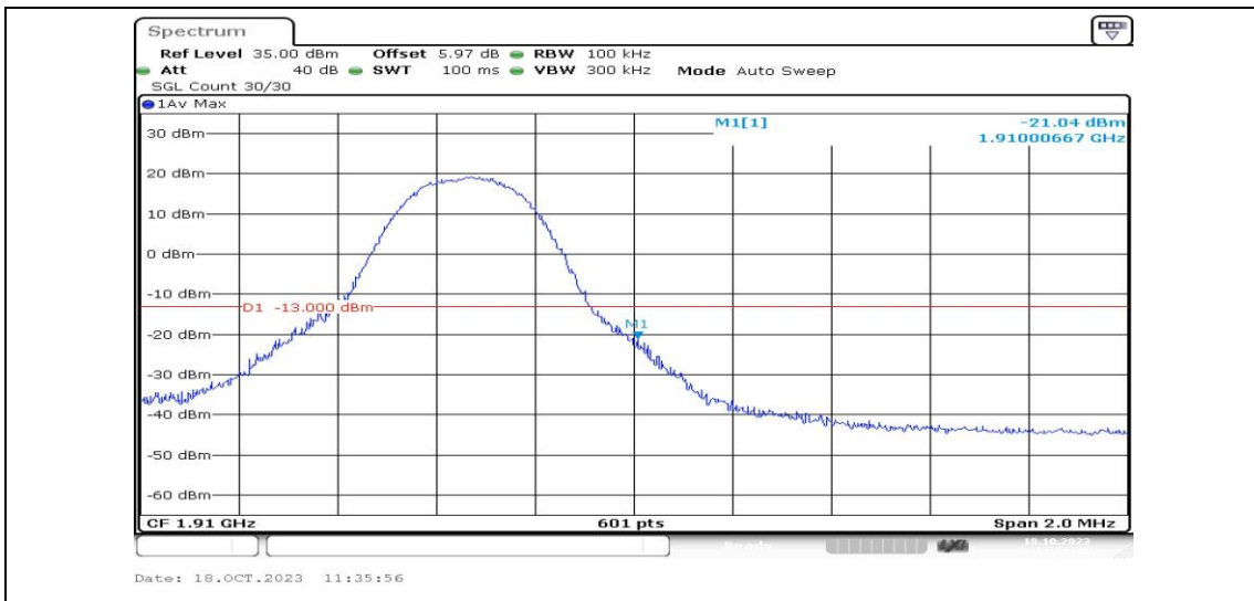
Band2-5MHz-16QAM-19175-1RB#24-PASS
