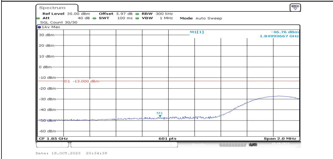
Band2-15MHz-QPSK-18675-1RB#74-PASS
