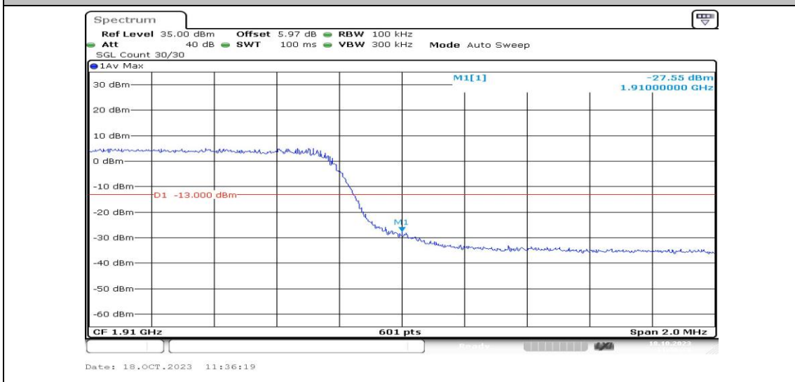
Band2-5MHz-16QAM-19175-25RB#0-PASS
