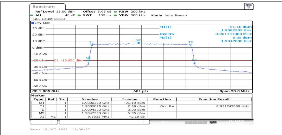
Band2-10MHz-QPSK-19150-50RB#0-PASS
