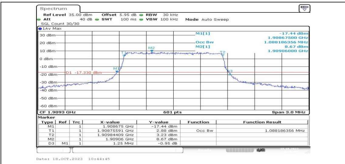
Band2-1.4MHz-16QAM-19193-6RB#0-PASS
