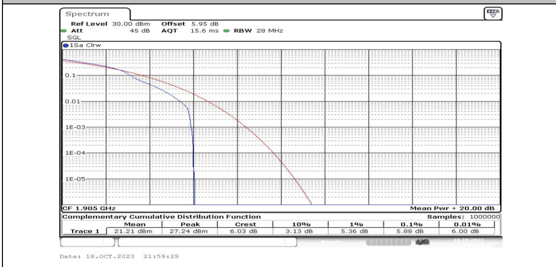
Band2-10MHz-16QAM-19150-1RB#0-PASS
