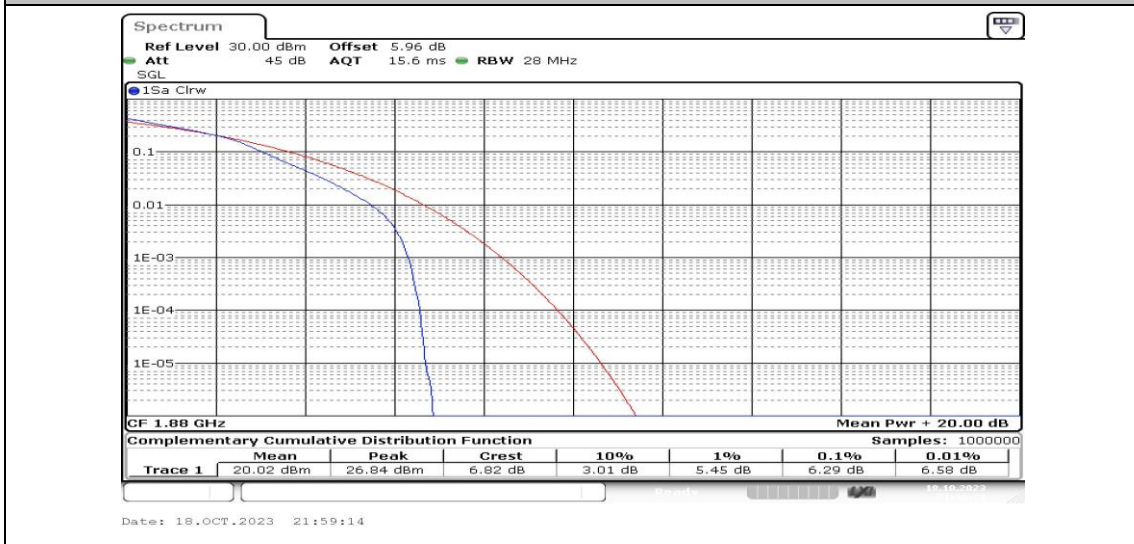
Band2-10MHz-16QAM-18900-25RB#0-PASS
