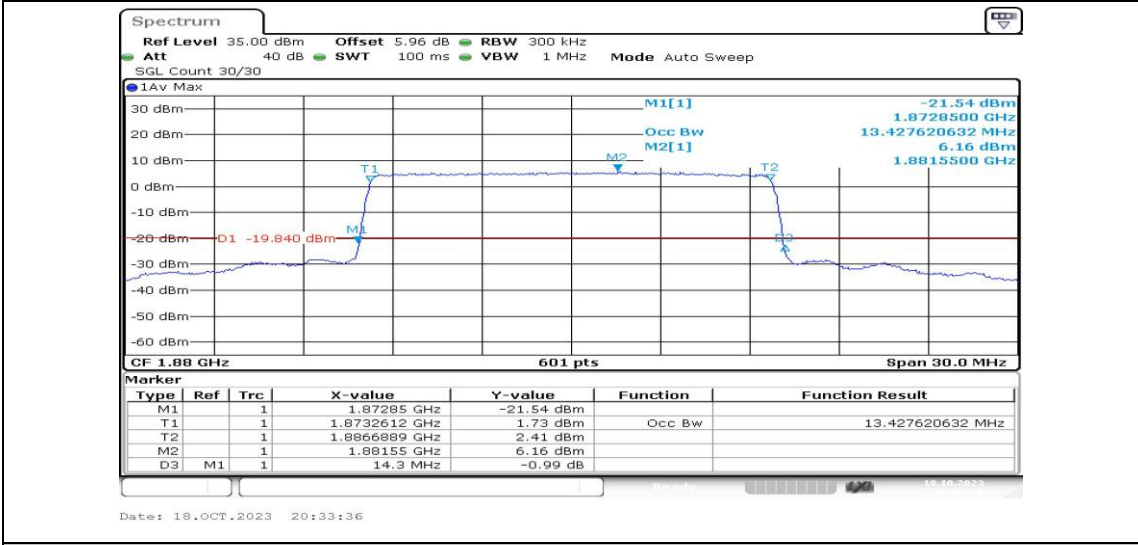
Band2-15MHz-QPSK-18900-75RB#0-PASS
