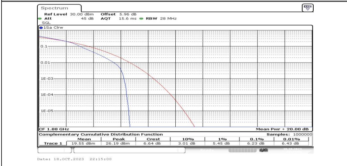
Band2-15MHz-16QAM-18900-25RB#0-PASS
