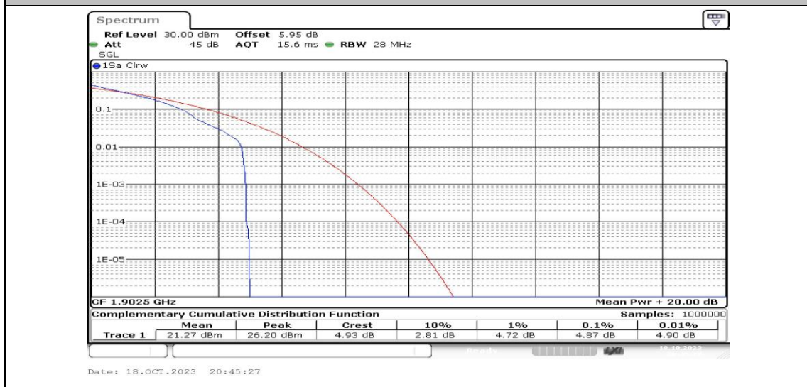
Band2-15MHz-QPSK-19125-1RB#0-PASS
