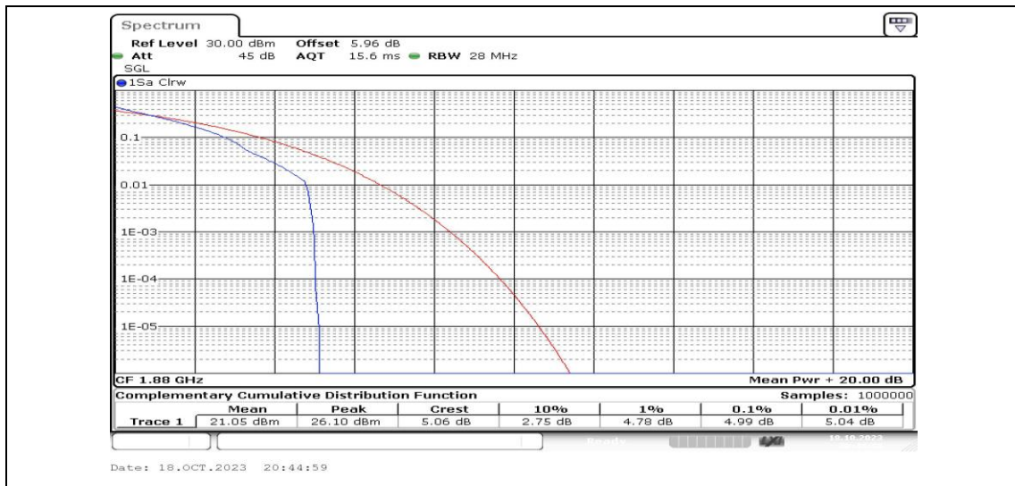
Band2-15MHz-QPSK-18900-1RB#0-PASS
