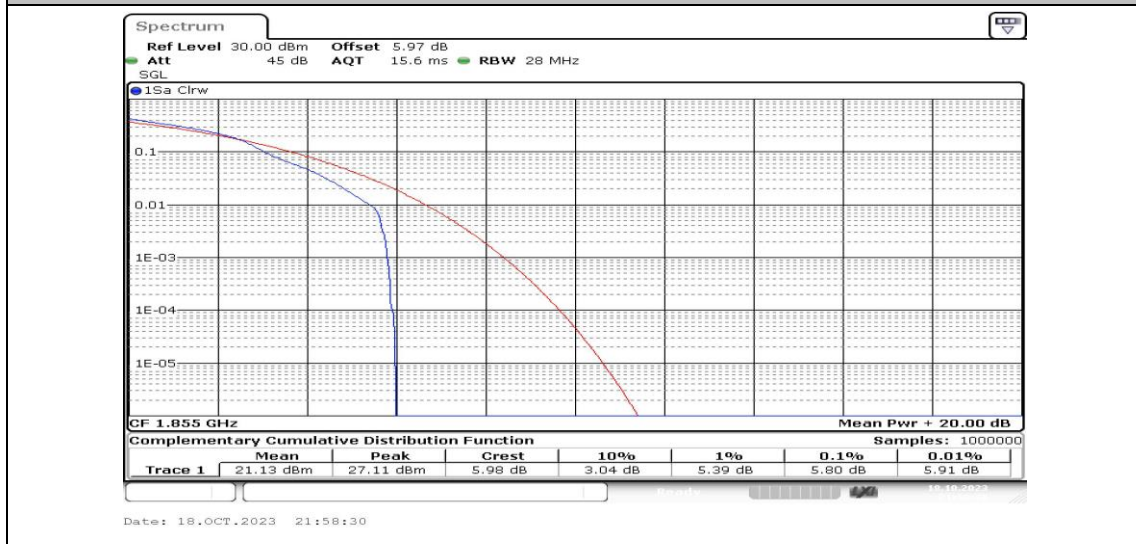
Band2-10MHz-16QAM-18650-1RB#0-PASS
