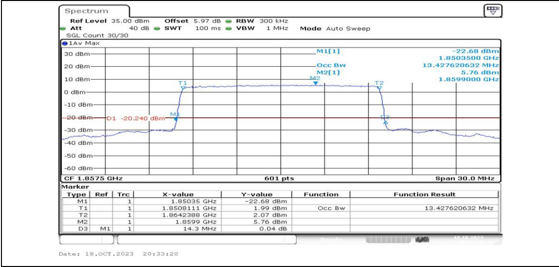
Band2-15MHz-QPSK-18675-75RB#0-PASS
