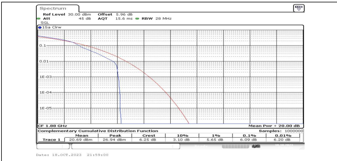
Band2-10MHz-16QAM-18900-1RB#0-PASS
