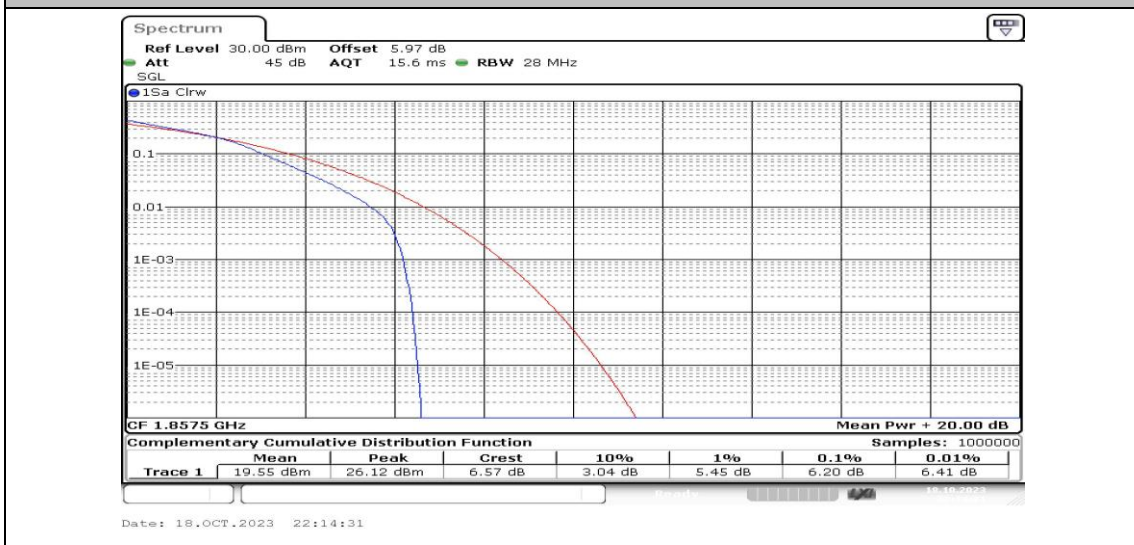
Band2-15MHz-16QAM-18675-25RB#0-PASS
