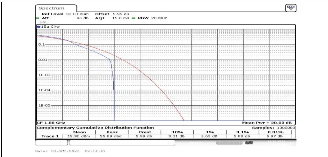
Band2-15MHz-16QAM-18900-1RB#0-PASS
