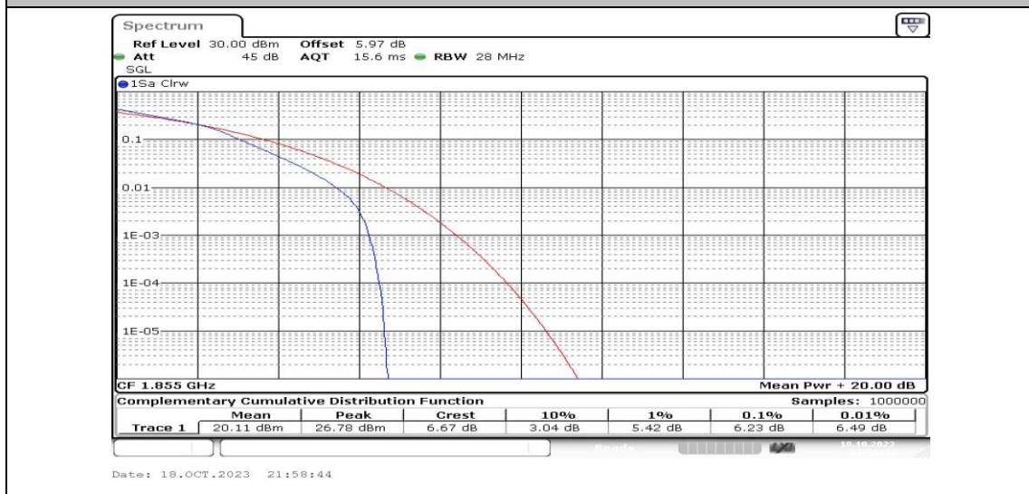
Band2-10MHz-16QAM-18650-25RB#0-PASS
