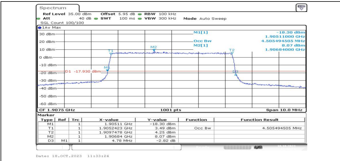
Band2-5MHz-16QAM-19175-25RB#0-PASS
