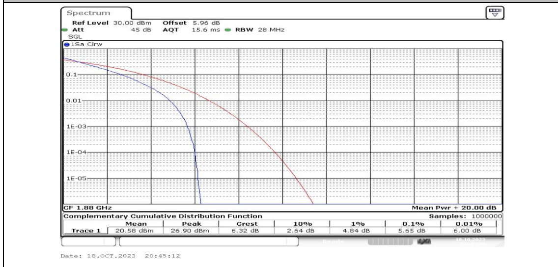
Band2-15MHz-QPSK-18900-75RB#0-PASS
