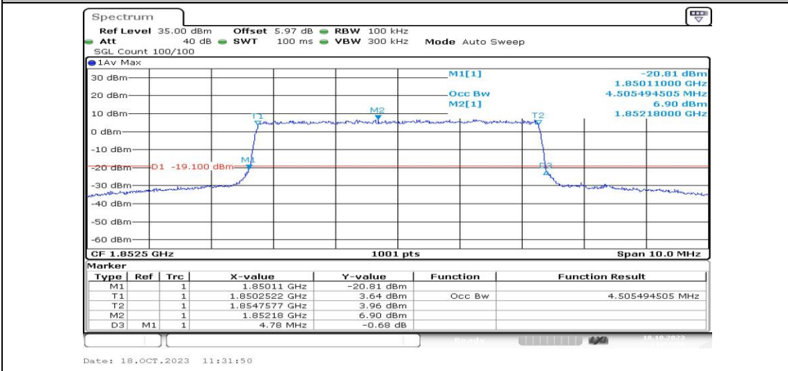
Band2-5MHz-16QAM-18625-25RB#0-PASS
