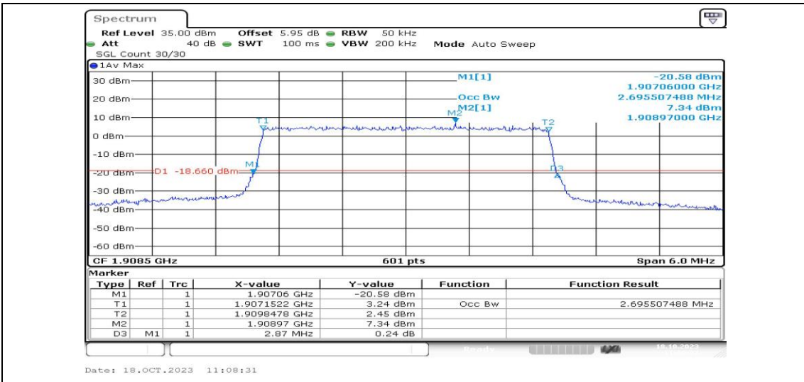
Band2-3MHz-16QAM-19185-15RB#0-PASS
