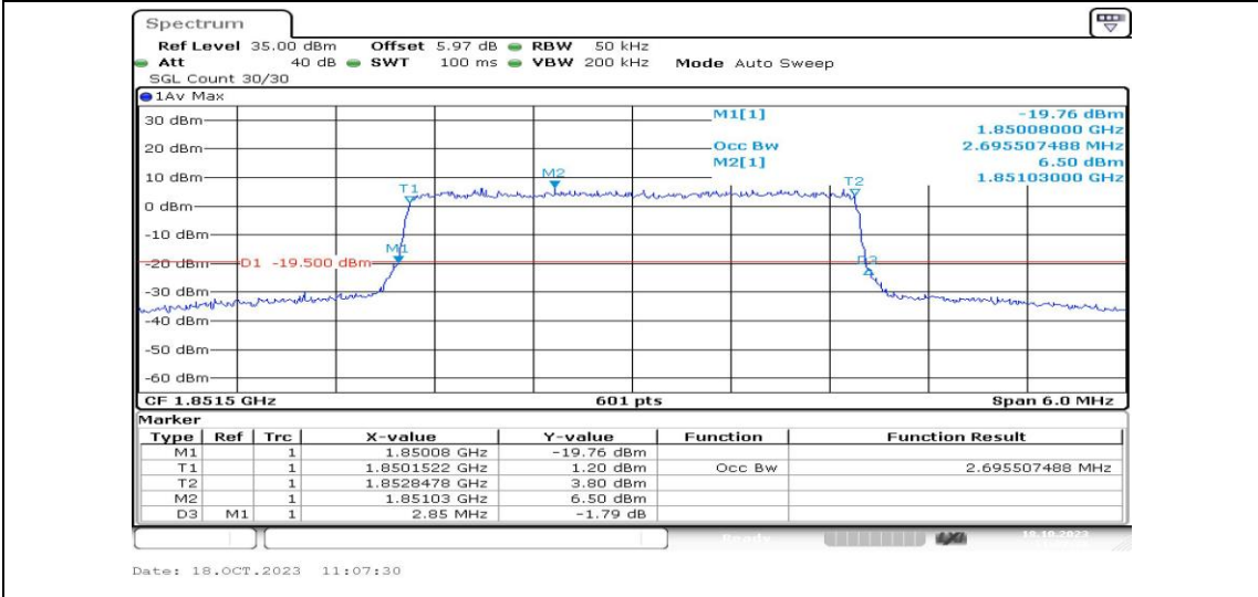
Band2-3MHz-16QAM-18615-15RB#0-PASS
