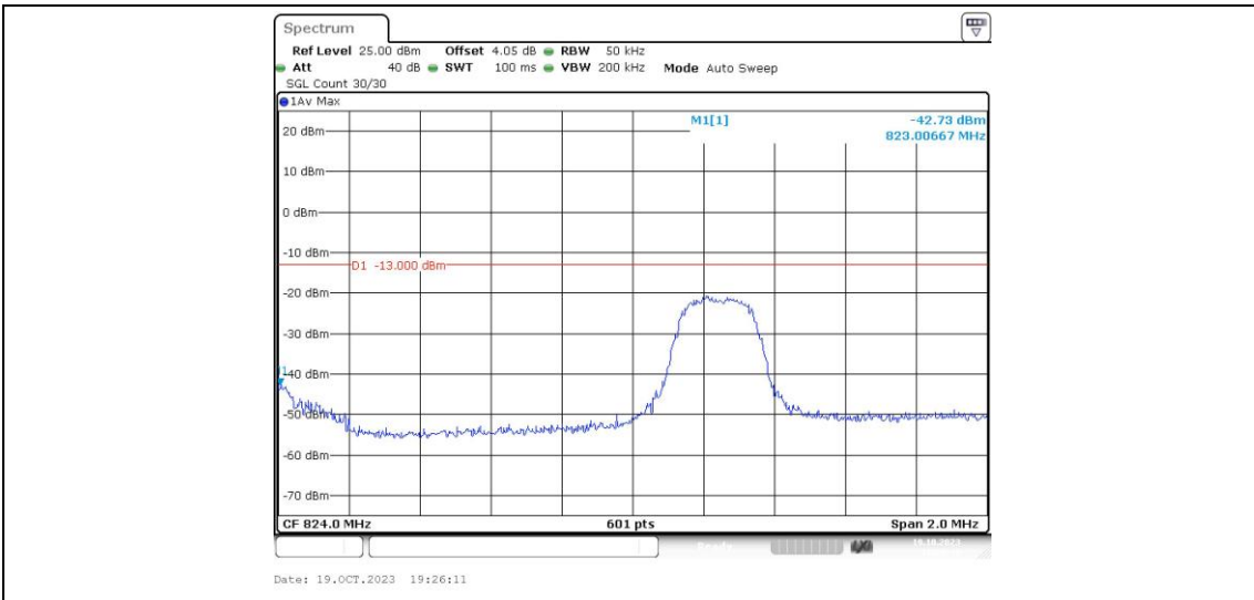
Band26-3MHz-16QAM-26805-15RB#0
