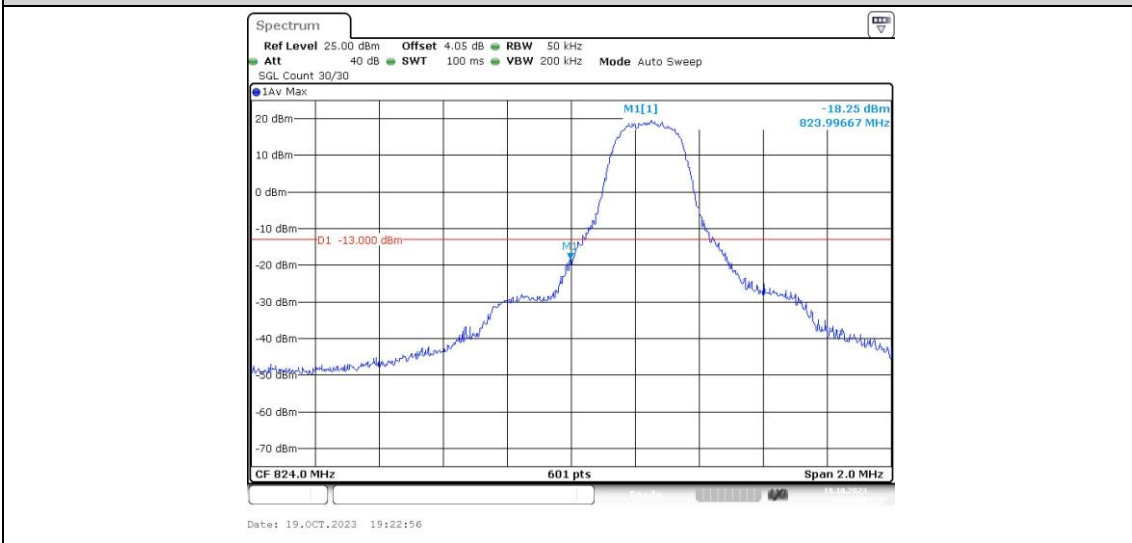
Band26-3MHz-QPSK-26805-1RB#14
