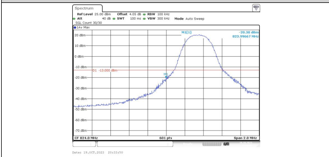
Band26-5MHz-QPSK-26815-1RB#24
