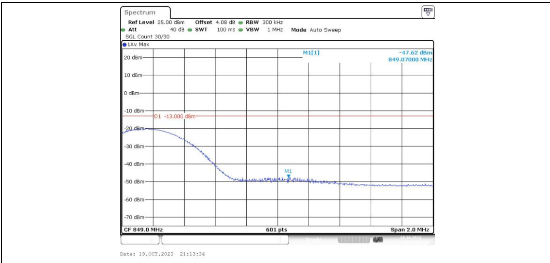
Band26-15MHz-QPSK-26965-1RB#74
