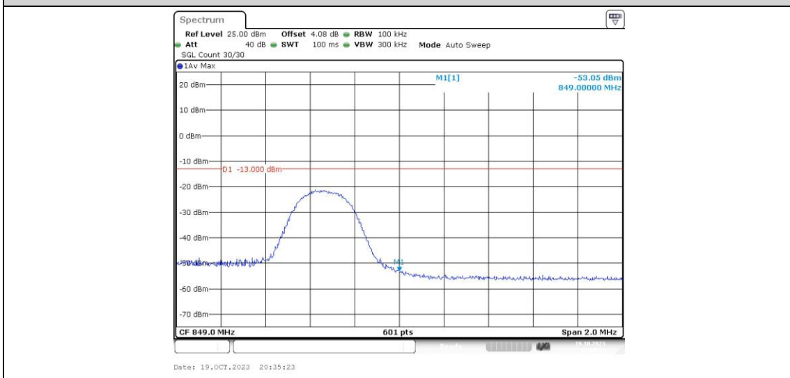
Band26-5MHz-16QAM-27015-1RB#24
