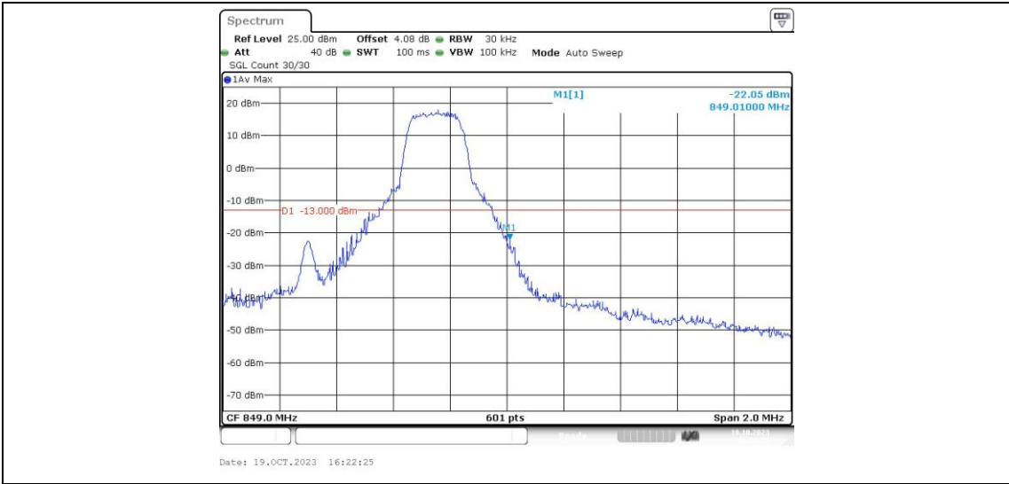
Band26-1.4MHz-QPSK-27033-6RB#0
