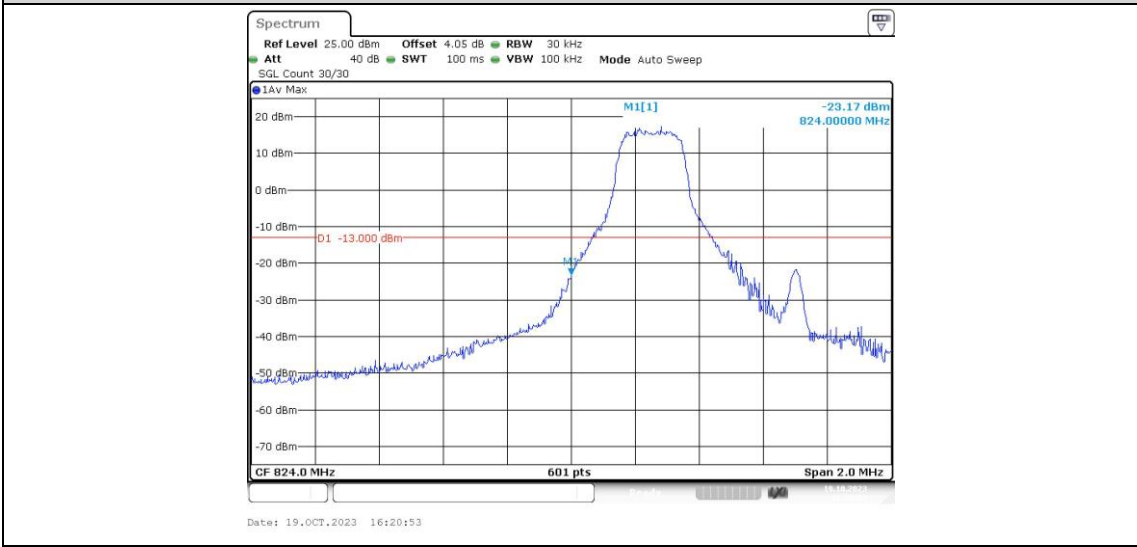
Band26-1.4MHz-16QAM-26797-1RB#5
