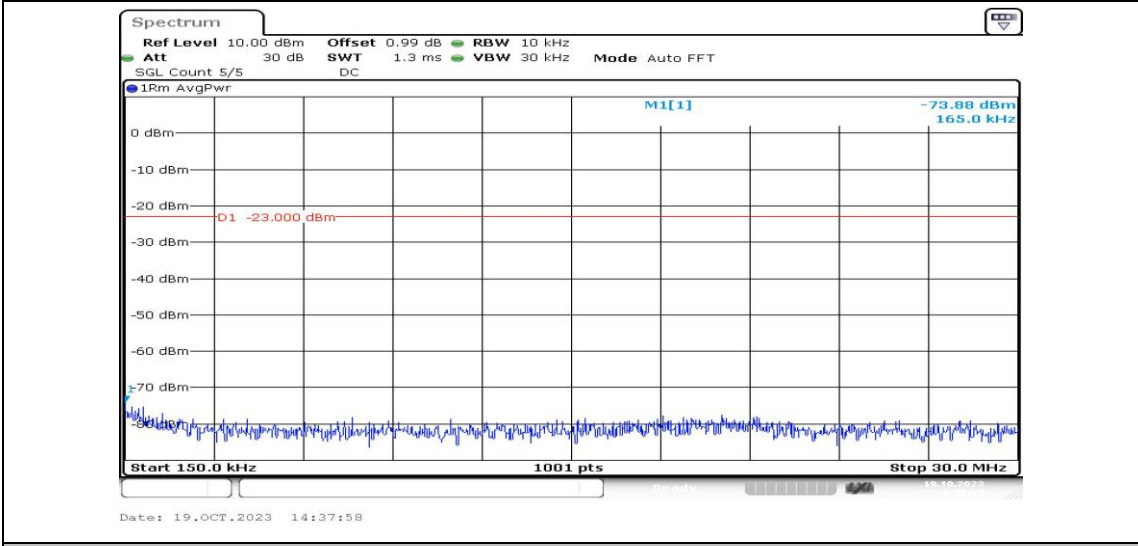
Band26-5MHz-QPSK-26740-1RB#0-Range2:0.15~30MHz-PASS
