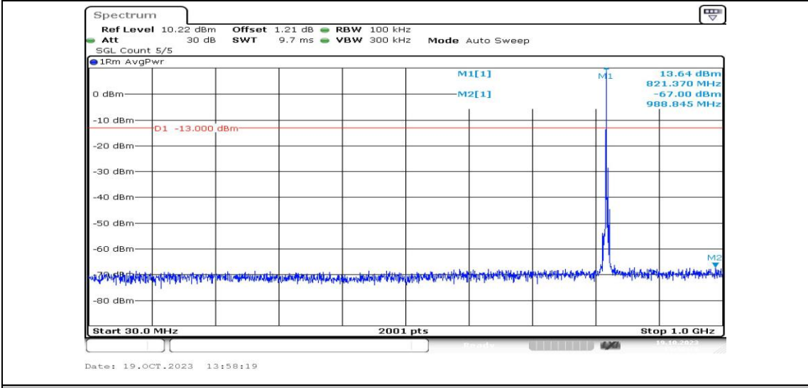
Band26-3MHz-16QAM-26775-1RB#0-Range3:30~1000MHz-PASS
