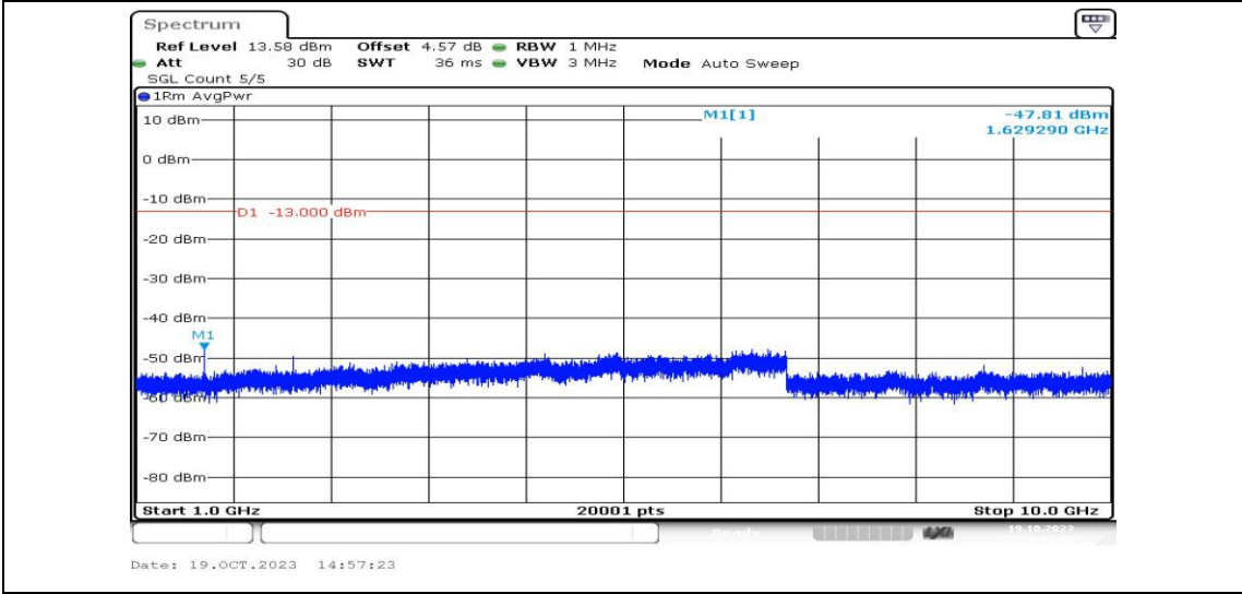
Band26-10MHz-QPSK-26740-1RB#0-Range4:1000~10000MHz-PASS
