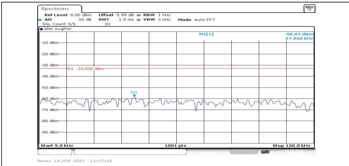
Band26-1.4MHz-16QAM-26783-1RB#0-Range1:0.009~0.15MHz-PASS
