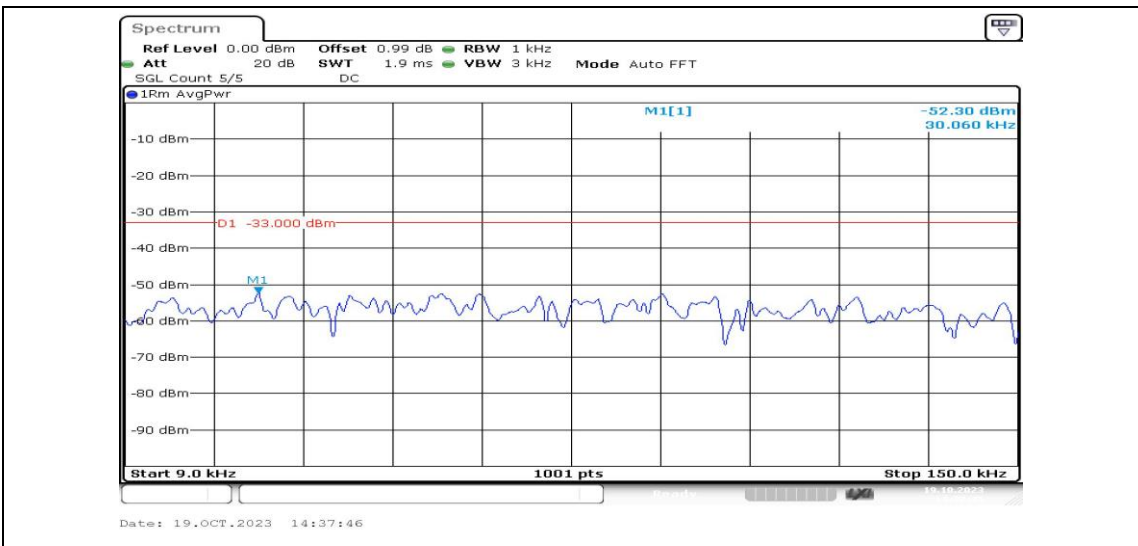
Band26-5MHz-QPSK-26740-1RB#0-Range1:0.009~0.15MHz-PASS
