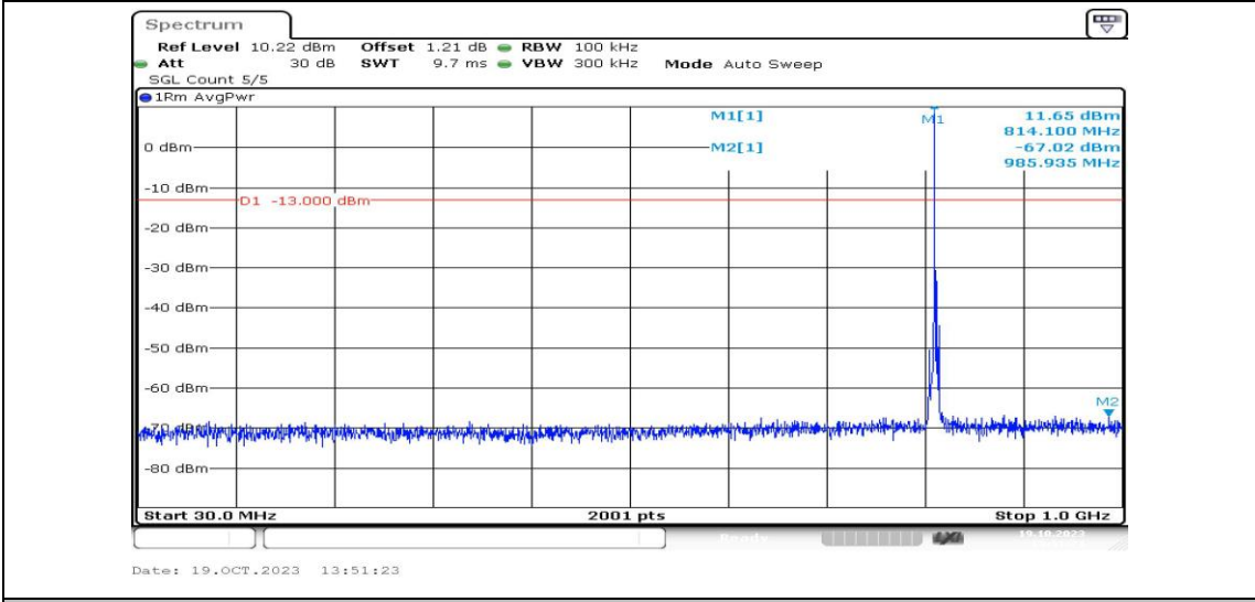
Band26-3MHz-16QAM-26705-1RB#0-Range3:30~1000MHz-PASS
