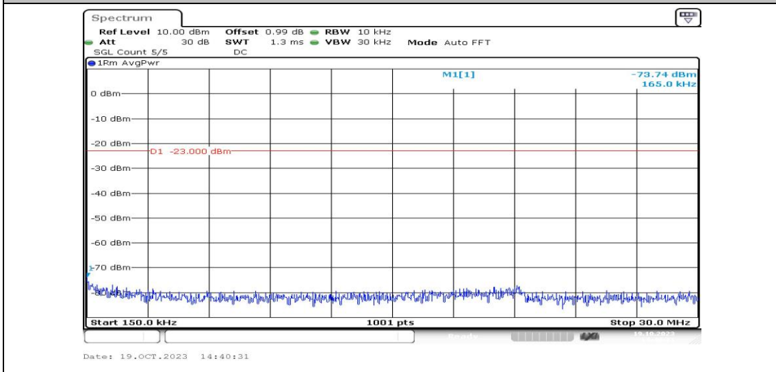
Band26-5MHz-16QAM-26765-1RB#0-Range2:0.15~30MHz-PASS
