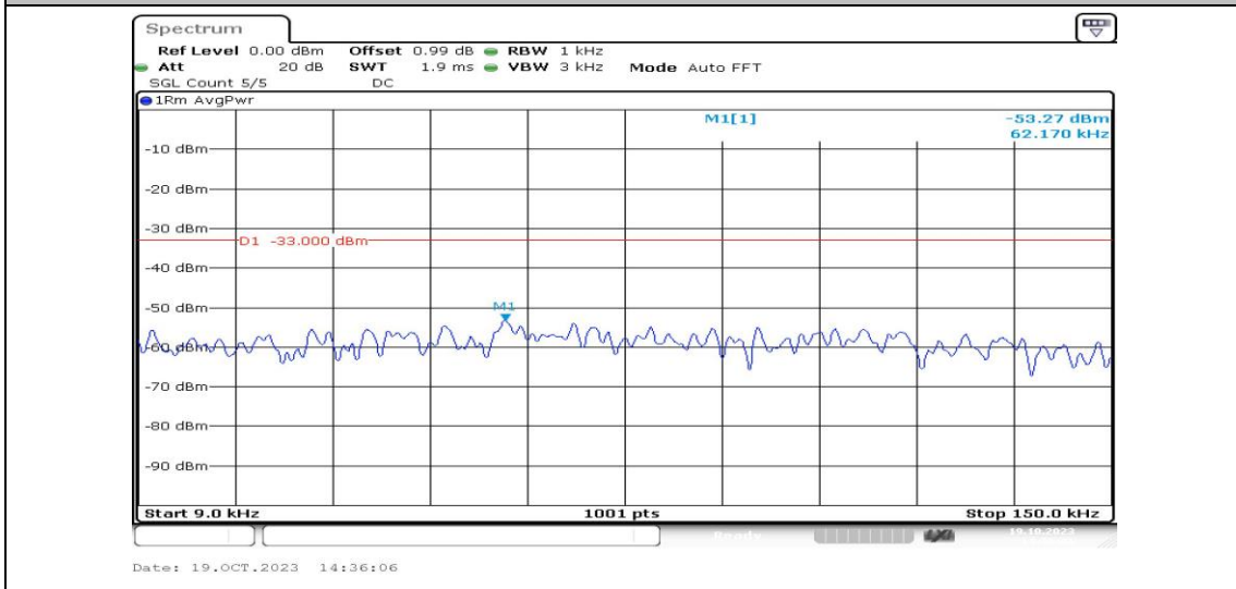
Band26-5MHz-QPSK-26715-1RB#0-Range1:0.009~0.15MHz-PASS
