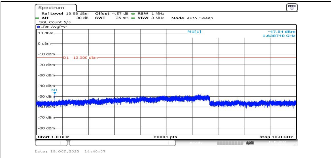
Band26-5MHz-16QAM-26765-1RB#0-Range4:1000~10000MHz-PASS
