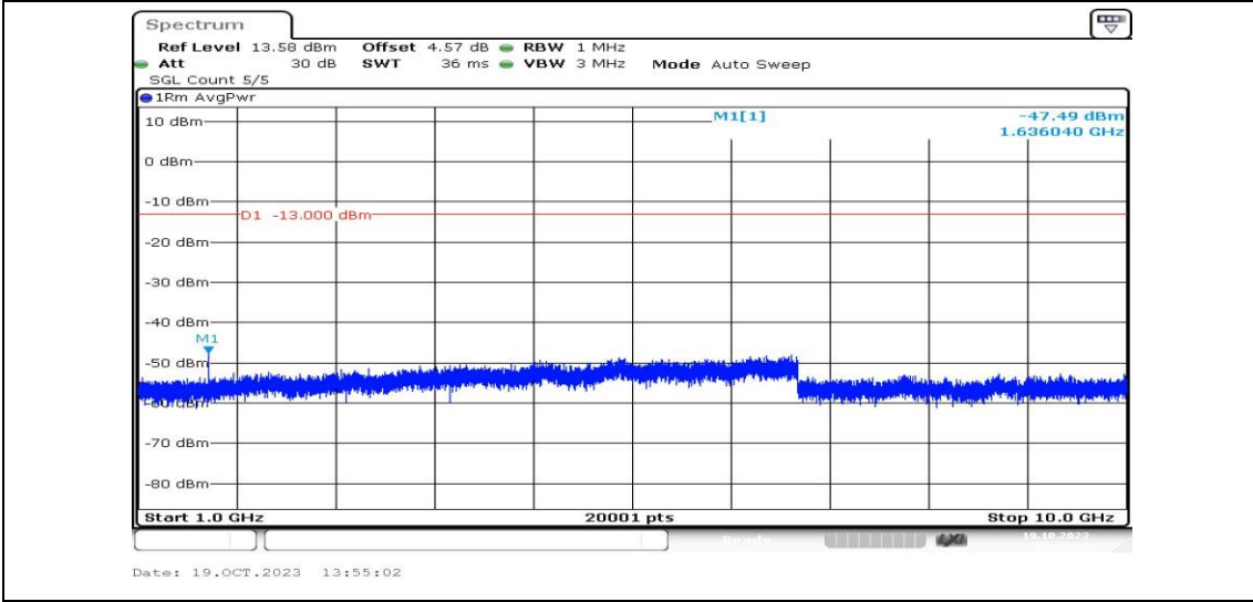
Band26-3MHz-16QAM-26740-1RB#0-Range4:1000~10000MHz-PASS
