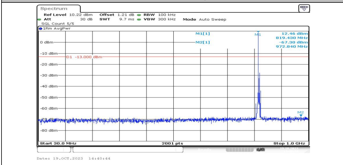
Band26-5MHz-16QAM-26765-1RB#0-Range3:30~1000MHz-PASS
