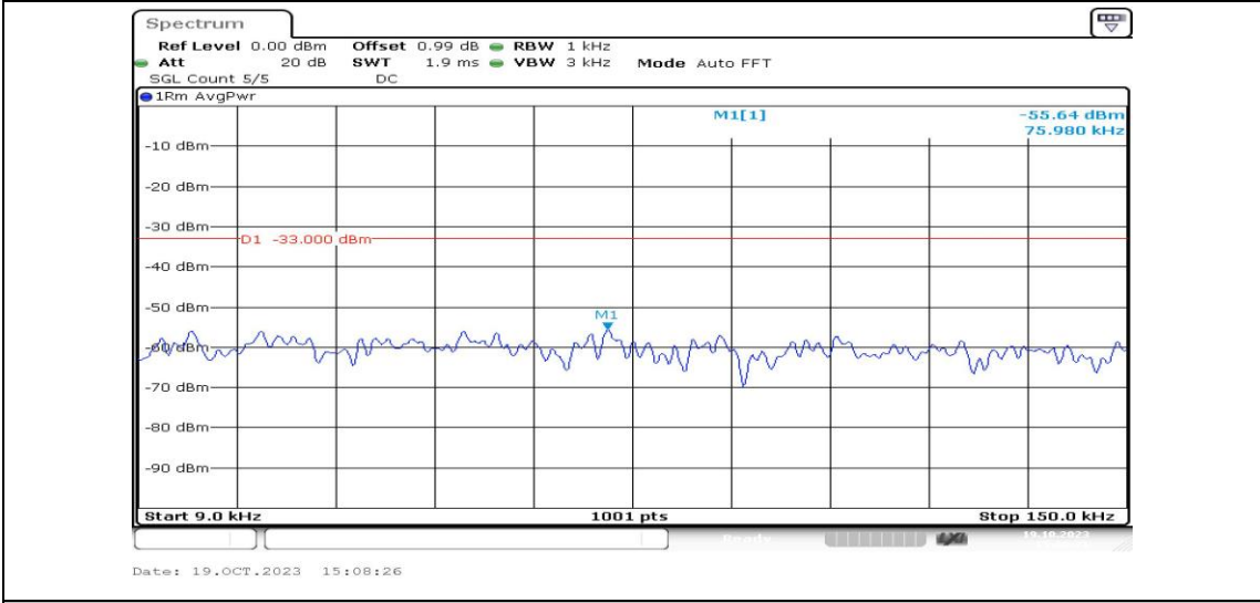
Band26-10MHz-16QAM-26740-1RB#0-Range1:0.009~0.15MHz-PASS
