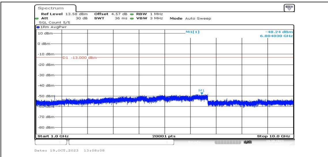
Band26-1.4MHz-16QAM-26783-1RB#0-Range4:1000~10000MHz-PASS
