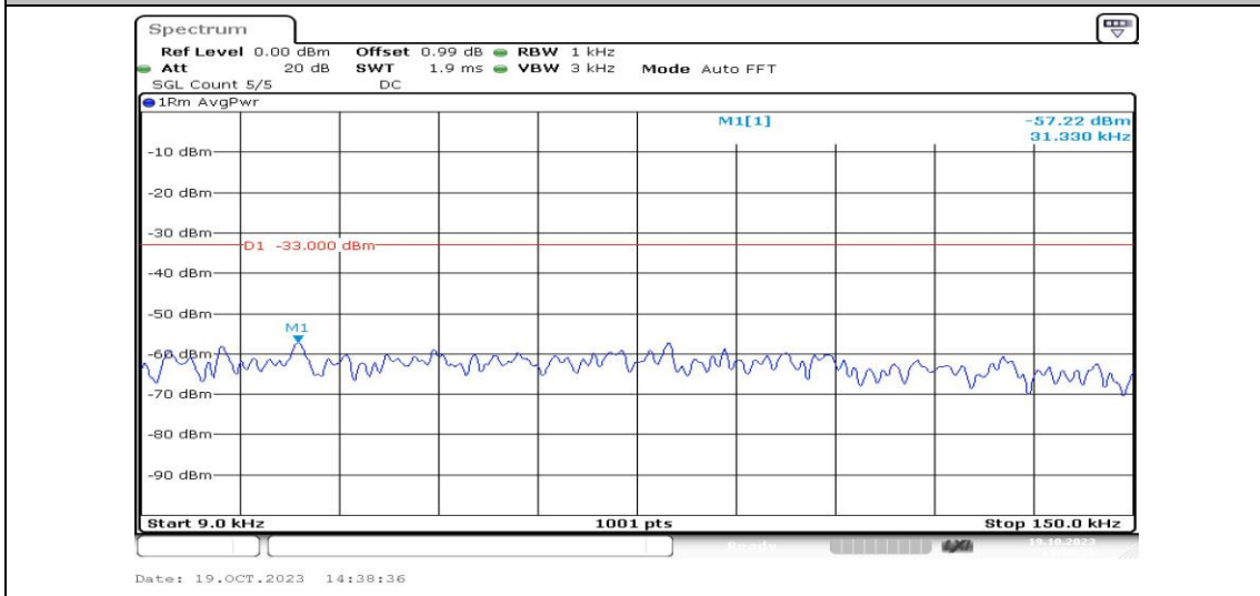
Band26-5MHz-16QAM-26740-1RB#0-Range1:0.009~0.15MHz-PASS
