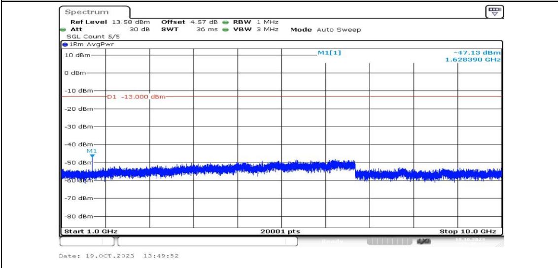
Band26-3MHz-QPSK-26705-1RB#0-Range4:1000~10000MHz-PASS
