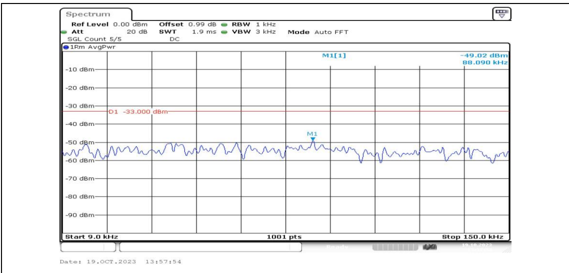
Band26-3MHz-16QAM-26775-1RB#0-Range1:0.009~0.15MHz-PASS
