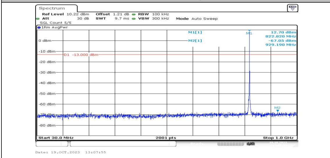
Band26-1.4MHz-16QAM-26783-1RB#0-Range3:30~1000MHz-PASS
