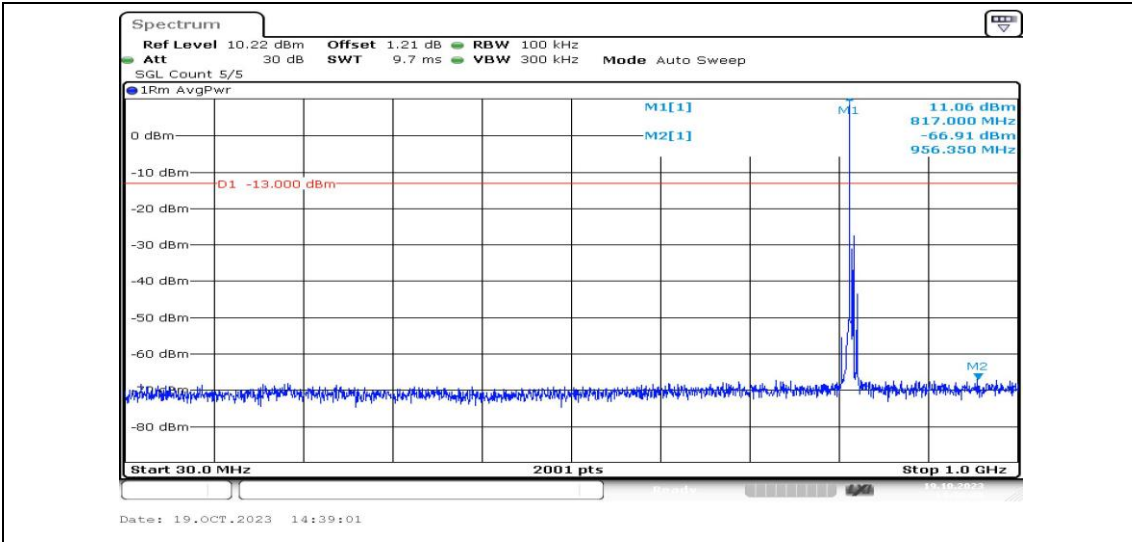
Band26-5MHz-16QAM-26740-1RB#0-Range3:30~1000MHz-PASS
