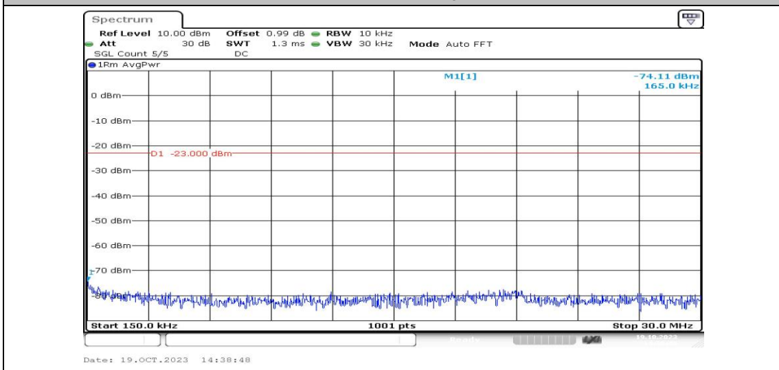
Band26-5MHz-16QAM-26740-1RB#0-Range2:0.15~30MHz-PASS
