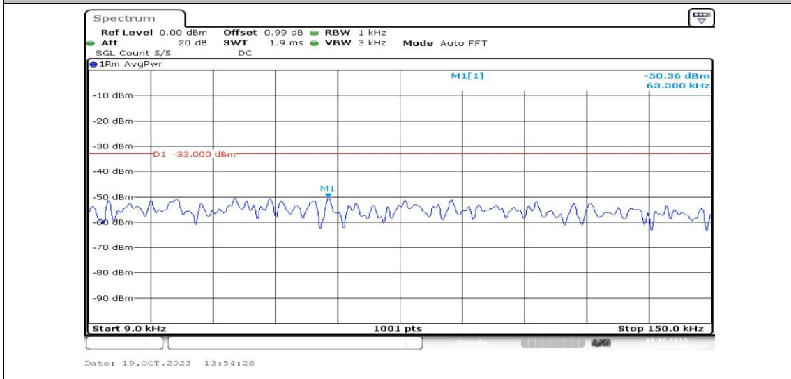
Band26-3MHz-16QAM-26740-1RB#0-Range1:0.009~0.15MHz-PASS
