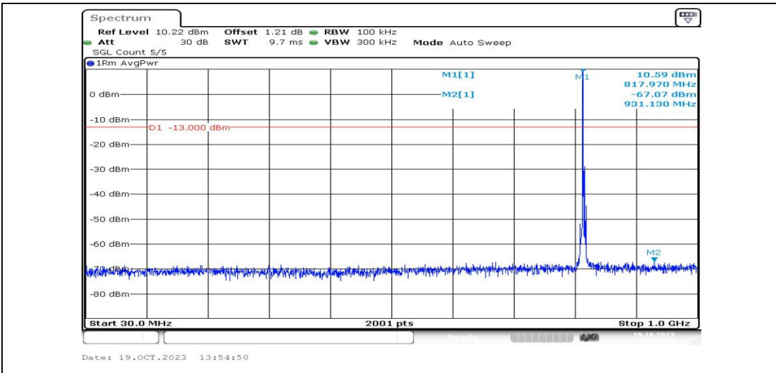
Band26-3MHz-16QAM-26740-1RB#0-Range3:30~1000MHz-PASS
