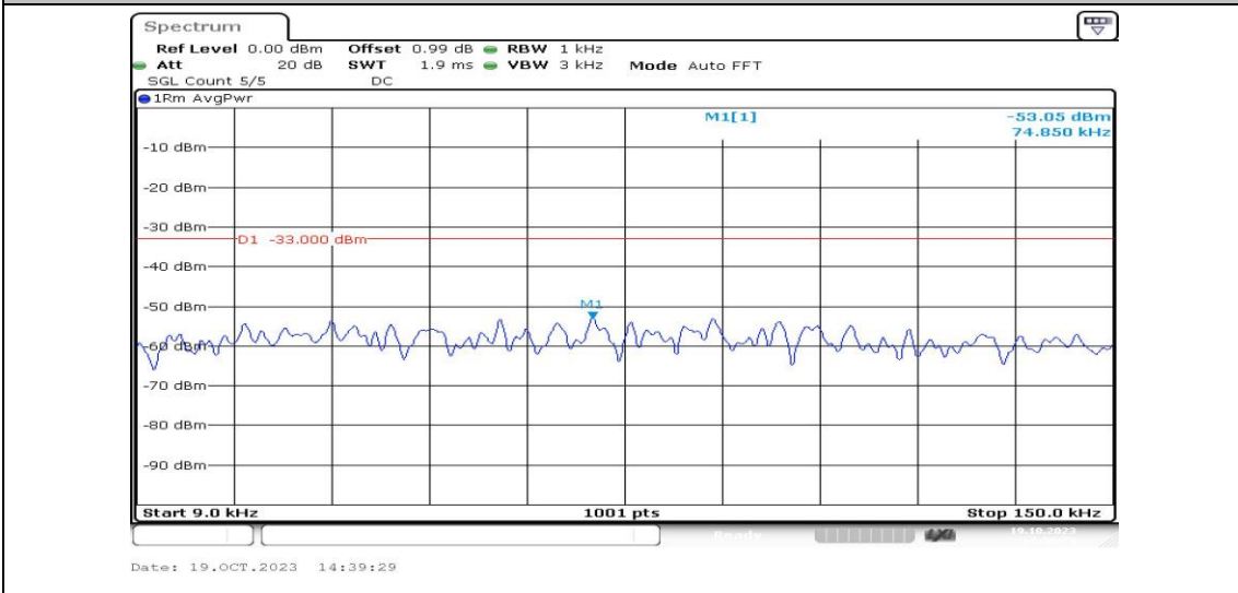
Band26-5MHz-QPSK-26765-1RB#0-Range1:0.009~0.15MHz-PASS
