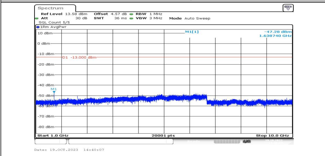
Band26-5MHz-QPSK-26765-1RB#0-Range4:1000~10000MHz-PASS
