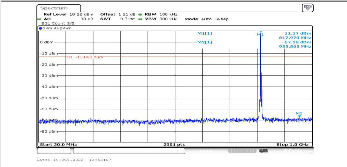
Band26-3MHz-QPSK-26740-1RB#0-Range3:30~1000MHz-PASS
