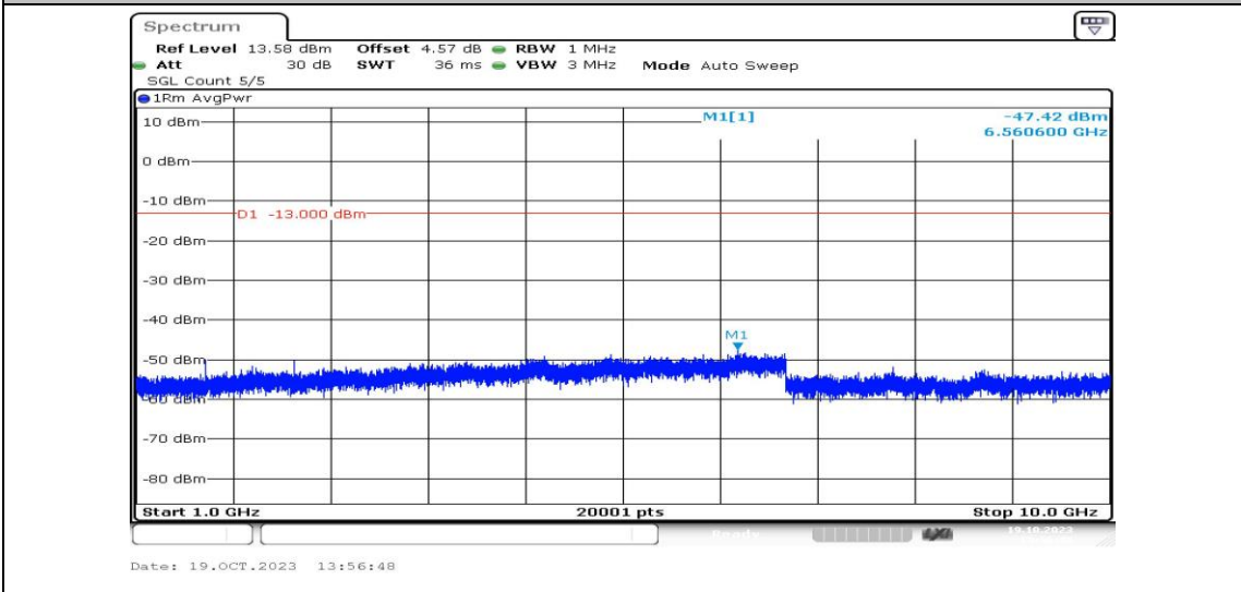
Band26-3MHz-QPSK-26775-1RB#0-Range4:1000~10000MHz-PASS
