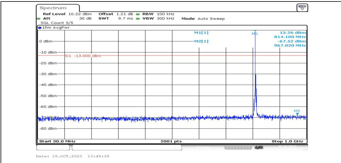
Band26-3MHz-QPSK-26705-1RB#0-Range3:30~1000MHz-PASS
