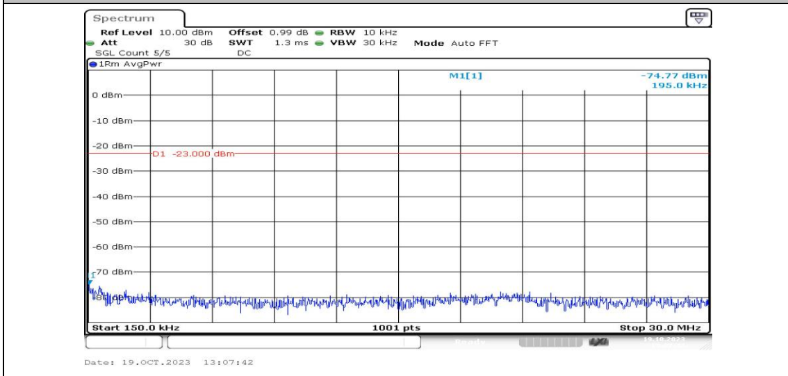
Band26-1.4MHz-16QAM-26783-1RB#0-Range2:0.15~30MHz-PASS
