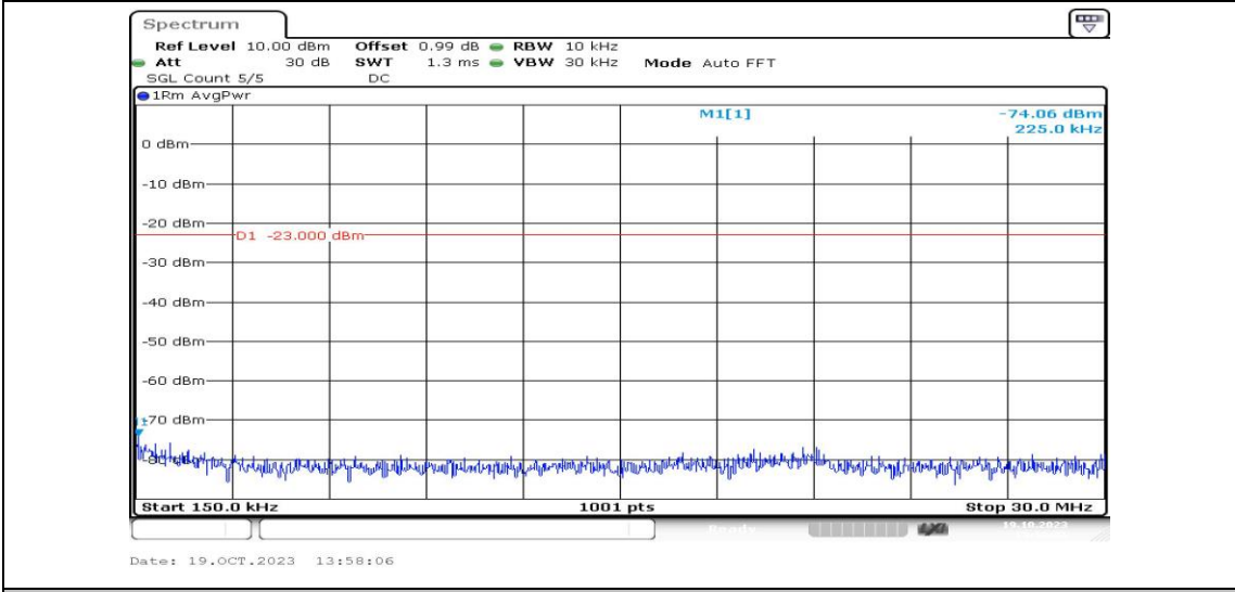
Band26-3MHz-16QAM-26775-1RB#0-Range2:0.15~30MHz-PASS
