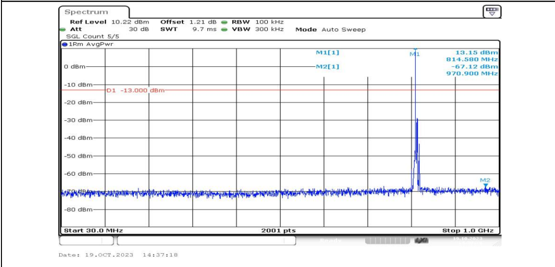
Band26-5MHz-16QAM-26715-1RB#0-Range3:30~1000MHz-PASS
