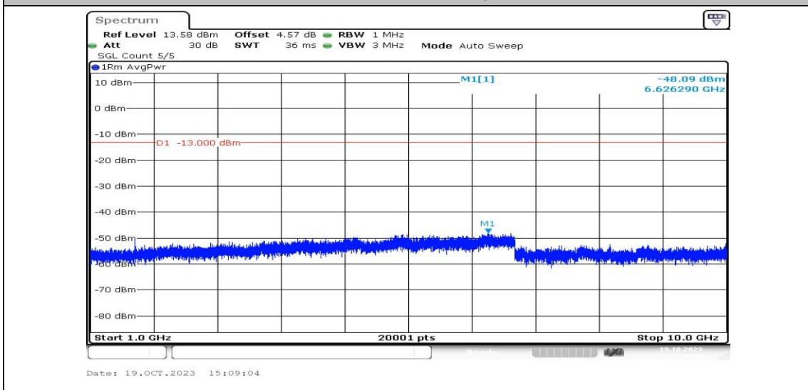
Band26-10MHz-16QAM-26740-1RB#0-Range4:1000~10000MHz-PASS
