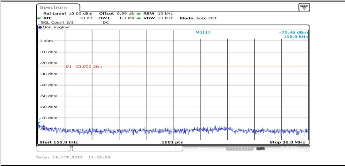
Band26-3MHz-QPSK-26705-1RB#0-Range2:0.15~30MHz-PASS
