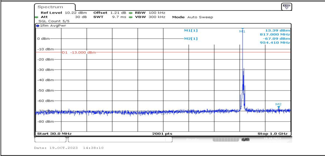
Band26-5MHz-QPSK-26740-1RB#0-Range3:30~1000MHz-PASS
