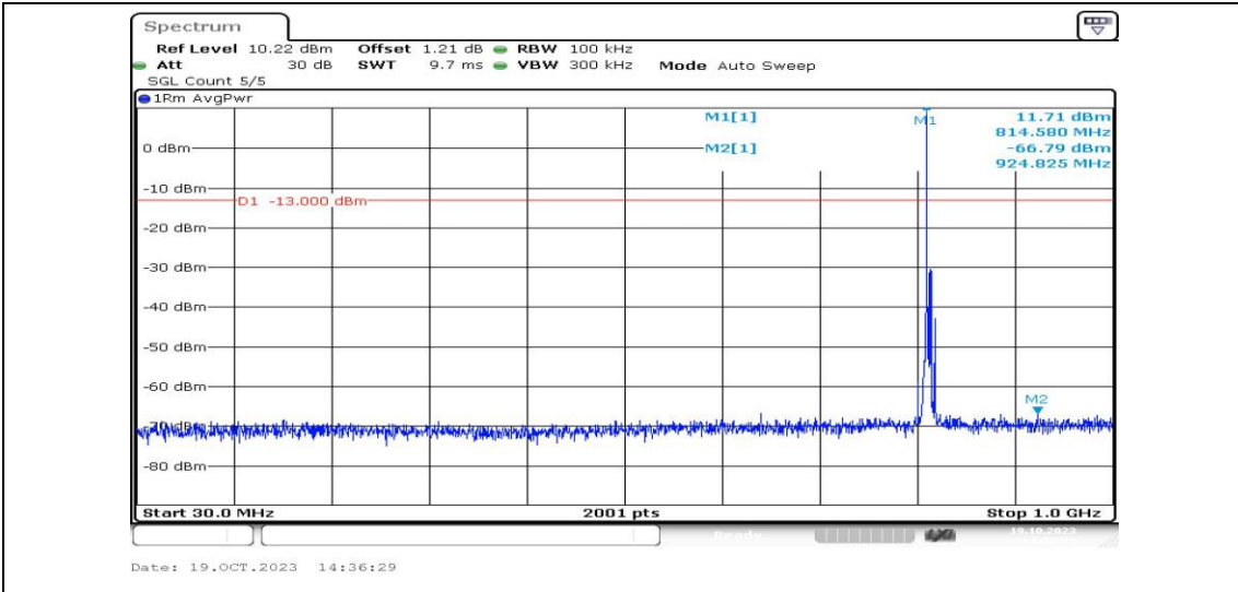
Band26-5MHz-QPSK-26715-1RB#0-Range3:30~1000MHz-PASS
