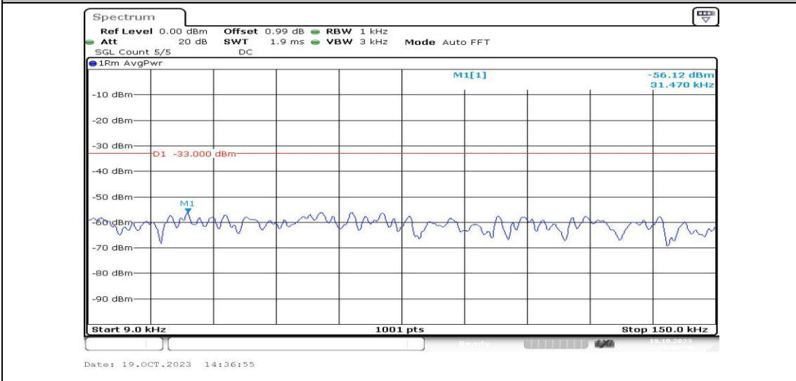
Band26-5MHz-16QAM-26715-1RB#0-Range1:0.009~0.15MHz-PASS
