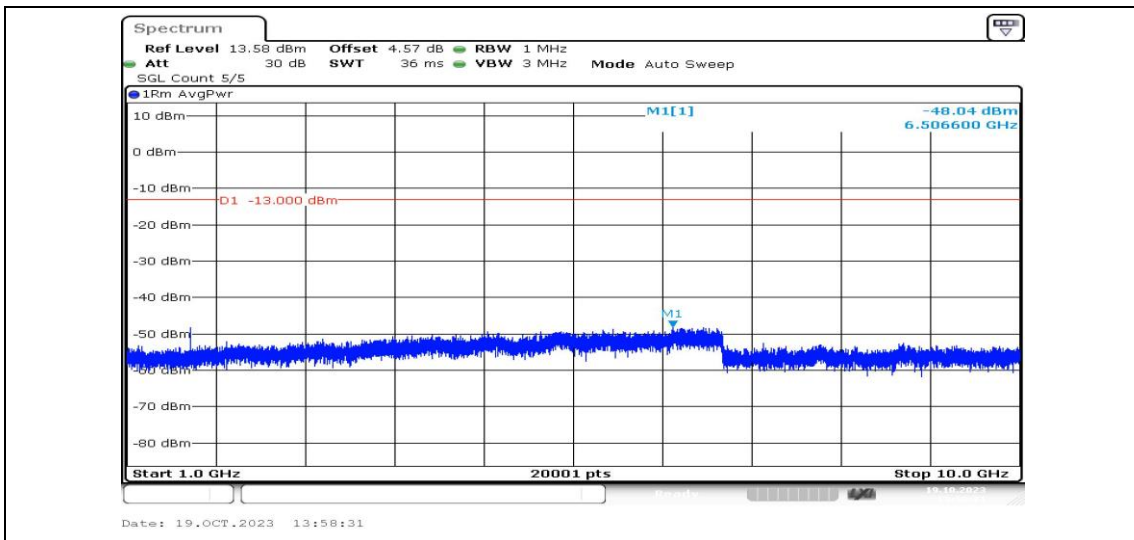
Band26-3MHz-16QAM-26775-1RB#0-Range4:1000~10000MHz-PASS
