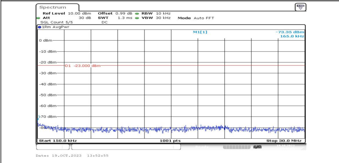
Band26-3MHz-QPSK-26740-1RB#0-Range2:0.15~30MHz-PASS
