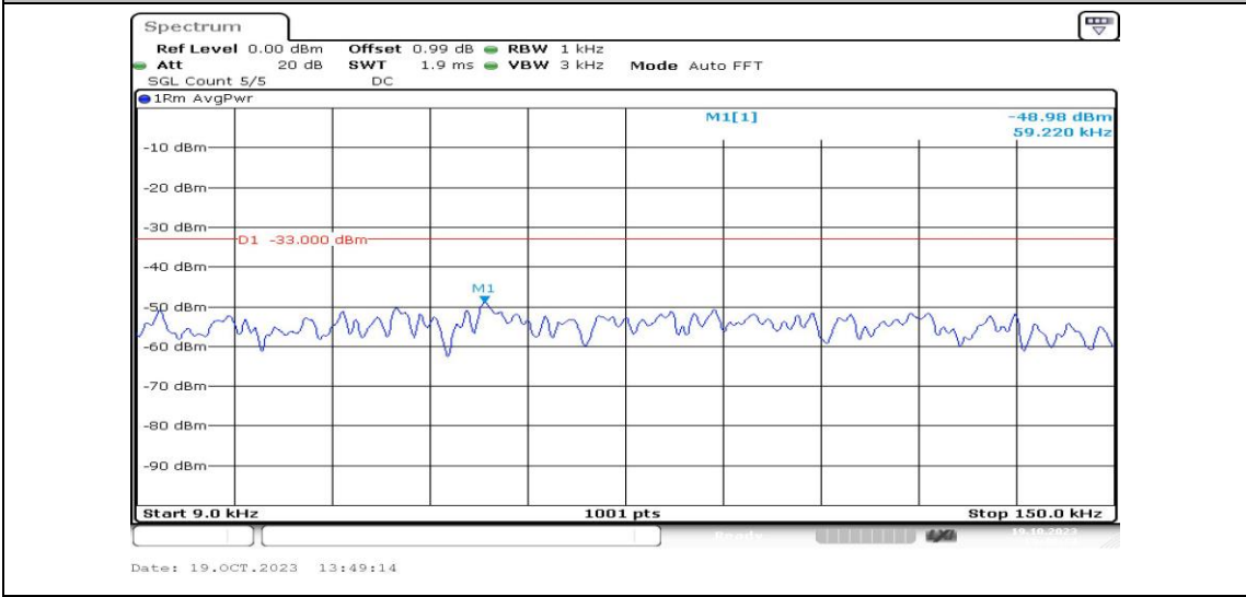
Band26-3MHz-QPSK-26705-1RB#0-Range1:0.009~0.15MHz-PASS
