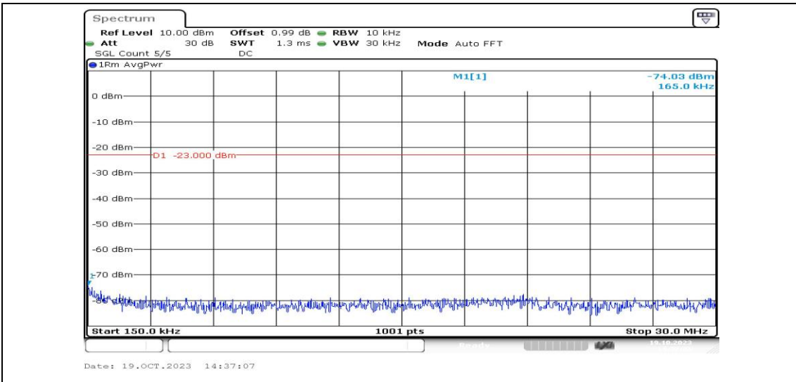
Band26-5MHz-16QAM-26715-1RB#0-Range2:0.15~30MHz-PASS
