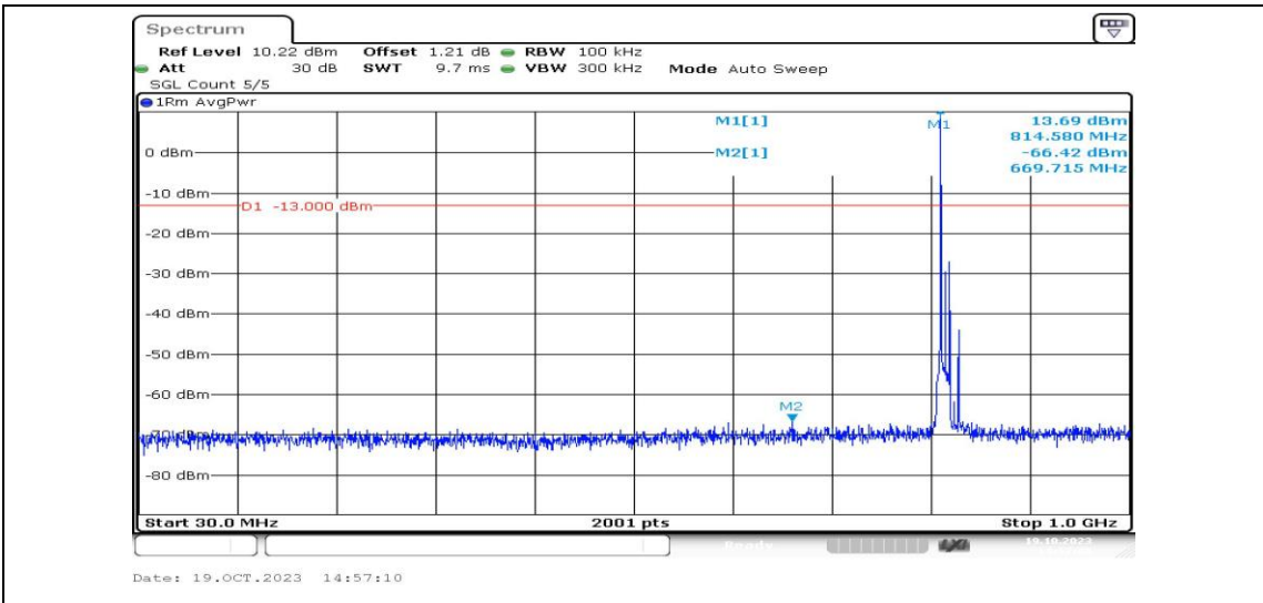
Band26-10MHz-QPSK-26740-1RB#0-Range3:30~1000MHz-PASS
