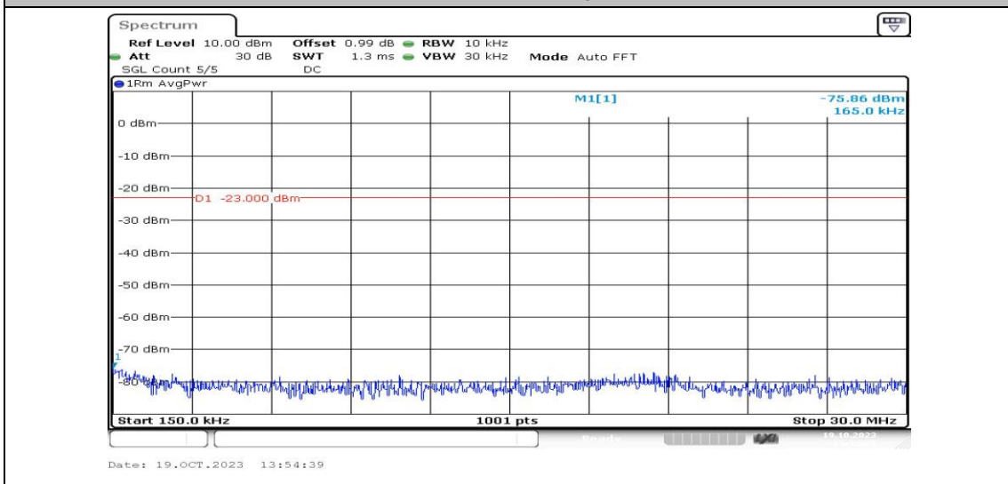
Band26-3MHz-16QAM-26740-1RB#0-Range2:0.15~30MHz-PASS
