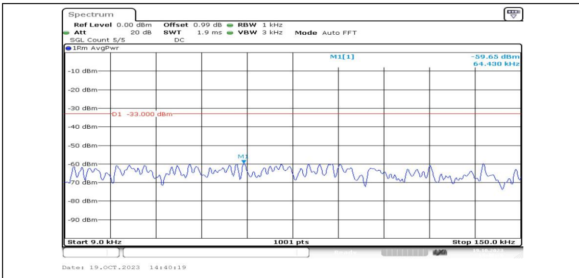
Band26-5MHz-16QAM-26765-1RB#0-Range1:0.009~0.15MHz-PASS
