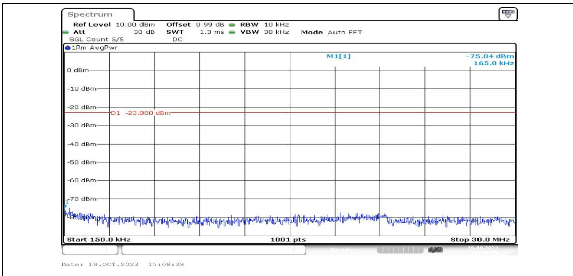
Band26-10MHz-16QAM-26740-1RB#0-Range2:0.15~30MHz-PASS
