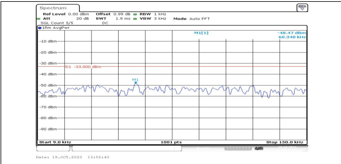
Band26-3MHz-QPSK-26740-1RB#0-Range1:0.009~0.15MHz-PASS
