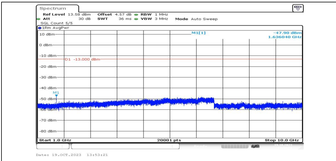
Band26-3MHz-QPSK-26740-1RB#0-Range4:1000~10000MHz-PASS
