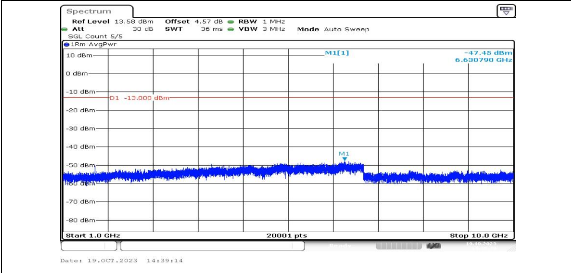
Band26-5MHz-16QAM-26740-1RB#0-Range4:1000~10000MHz-PASS
