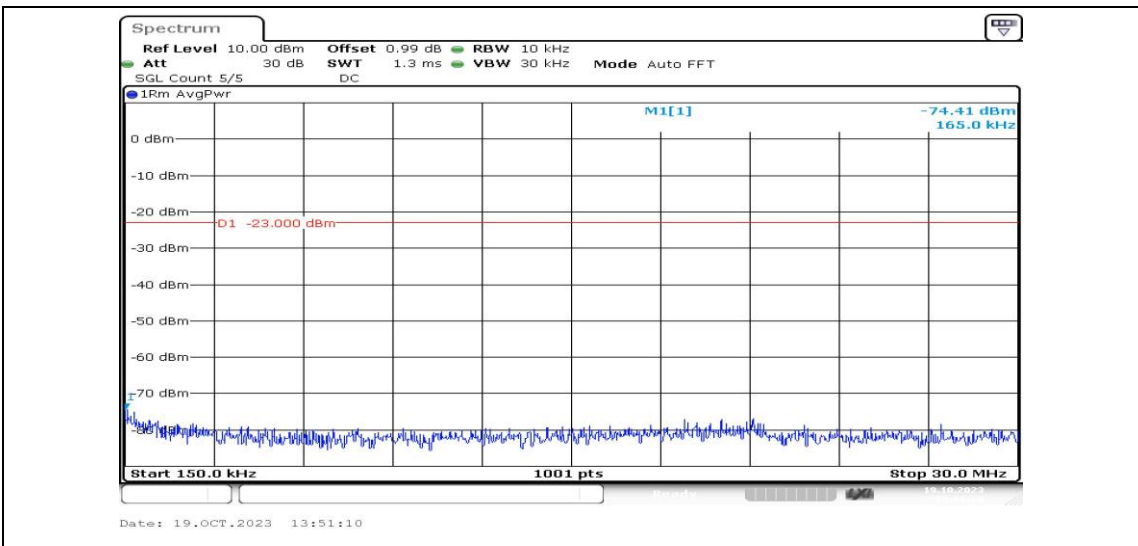
Band26-3MHz-16QAM-26705-1RB#0-Range2:0.15~30MHz-PASS
