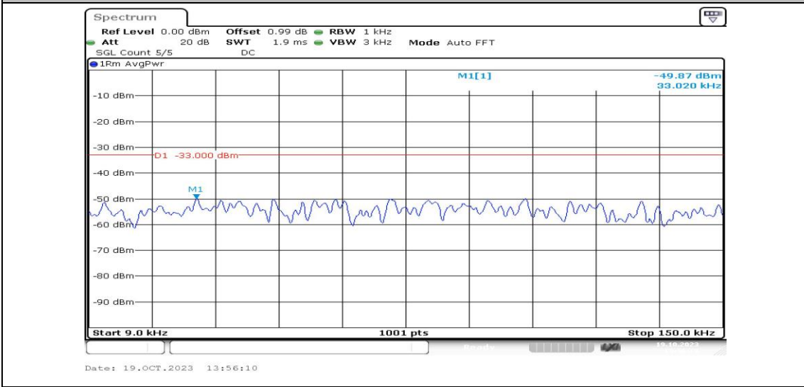
Band26-3MHz-QPSK-26775-1RB#0-Range1:0.009~0.15MHz-PASS
