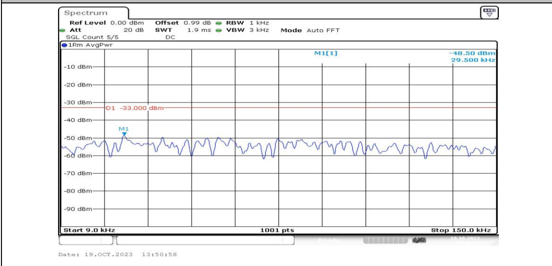
Band26-3MHz-16QAM-26705-1RB#0-Range1:0.009~0.15MHz-PASS
