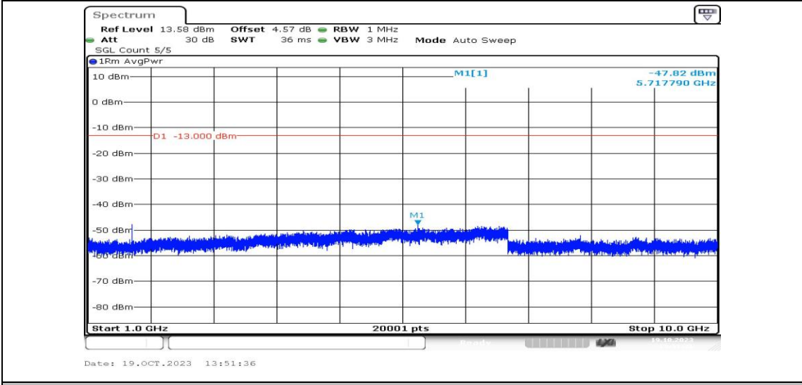
Band26-3MHz-16QAM-26705-1RB#0-Range4:1000~10000MHz-PASS
