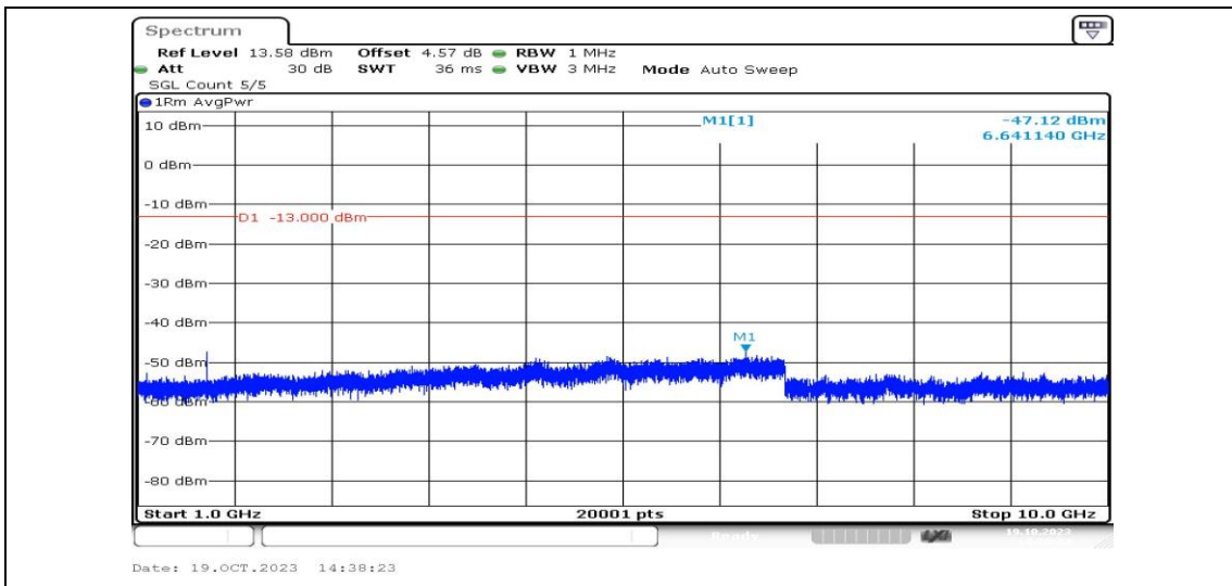
Band26-5MHz-QPSK-26740-1RB#0-Range4:1000~10000MHz-PASS
