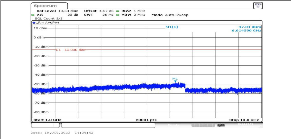
Band26-5MHz-QPSK-26715-1RB#0-Range4:1000~10000MHz-PASS
