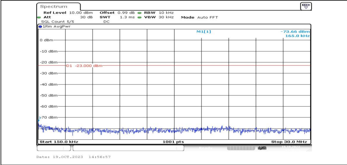
Band26-10MHz-QPSK-26740-1RB#0-Range2:0.15~30MHz-PASS
