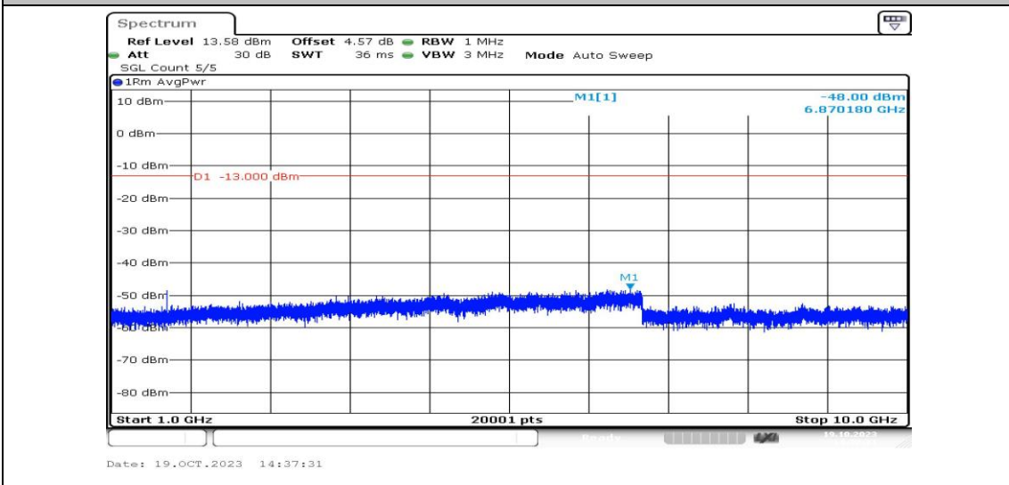
Band26-5MHz-16QAM-26715-1RB#0-Range4:1000~10000MHz-PASS
