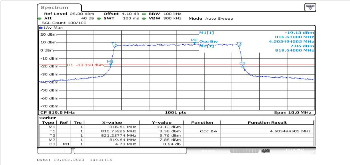
Band26-5MHz-QPSK-26740-25RB#0-PASS
