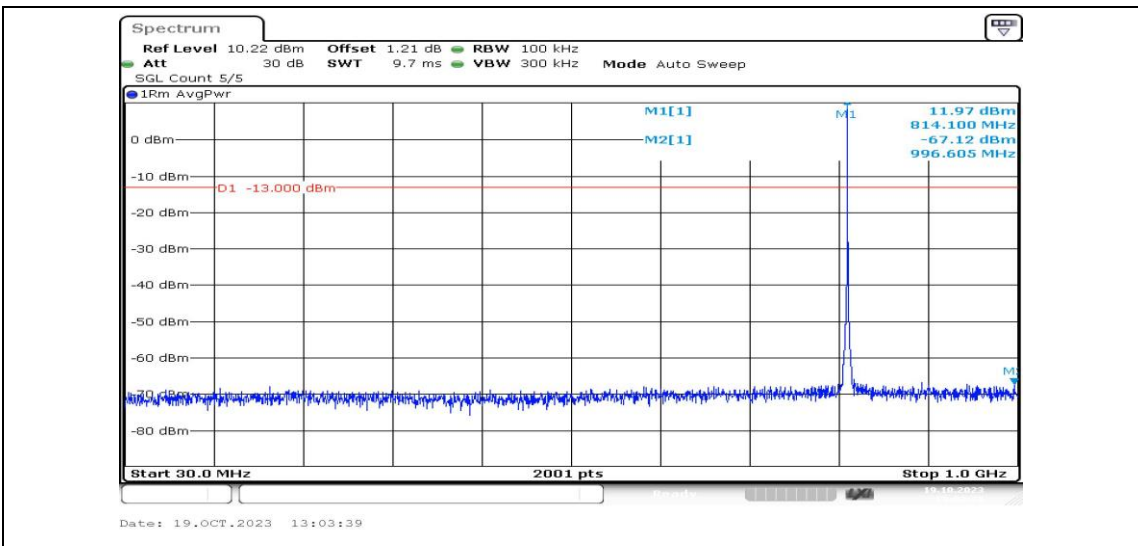
Band26-1.4MHz-QPSK-26697-1RB#0-Range3:30~1000MHz-PASS
