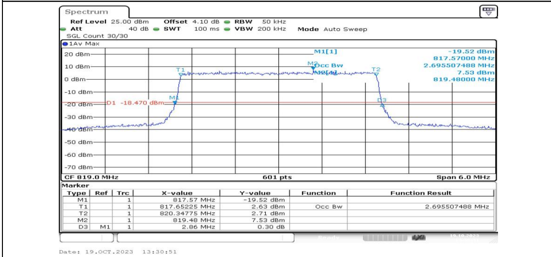
Band26-3MHz-16QAM-26740-15RB#0-PASS
