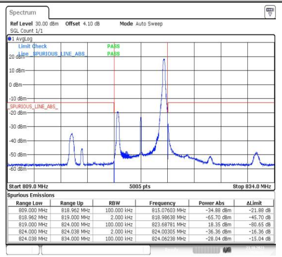
Band26_5MHz_16QAM_26765_1RB#0
