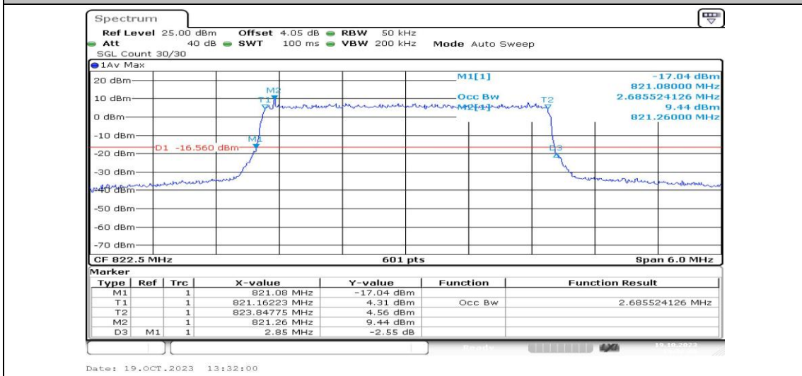
Band26-3MHz-QPSK-26775-15RB#0-PASS
