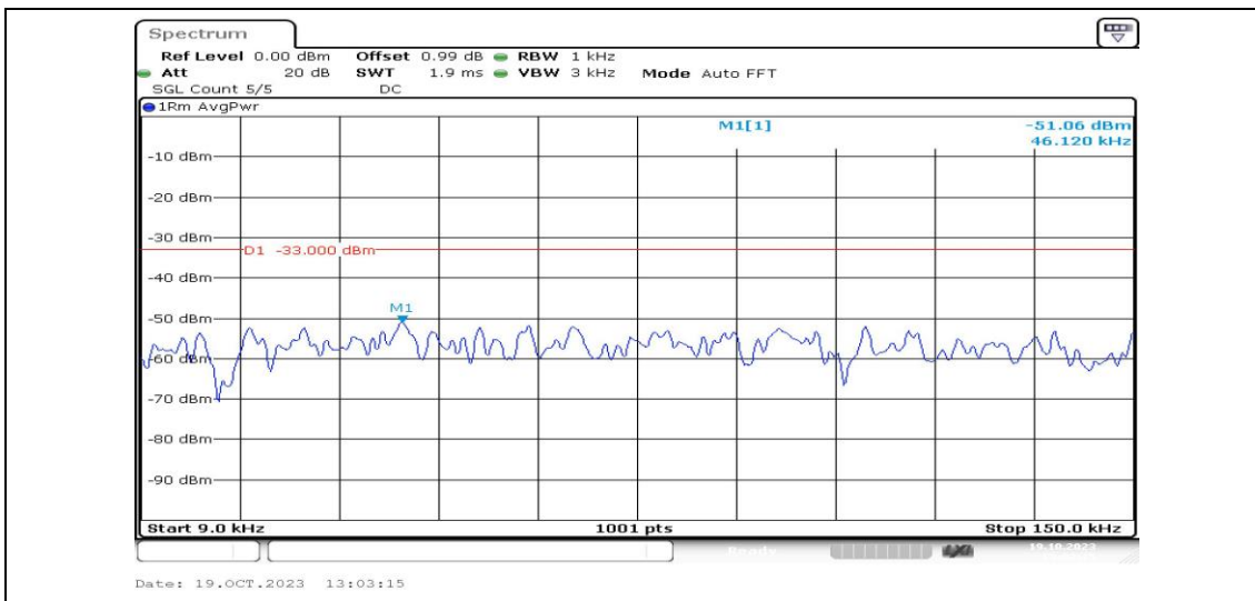
Band26-1.4MHz-QPSK-26697-1RB#0-Range1:0.009~0.15MHz-PASS
