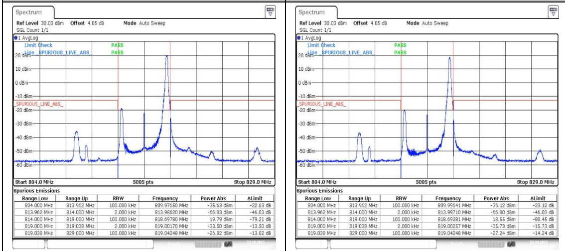
Band26_5MHz_QPSK_26715_1RB#0
