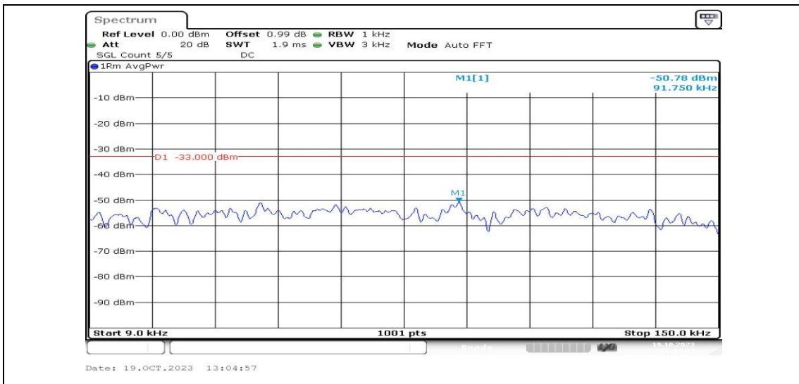
Band26-1.4MHz-QPSK-26740-1RB#0-Range1:0.009~0.15MHz-PASS
