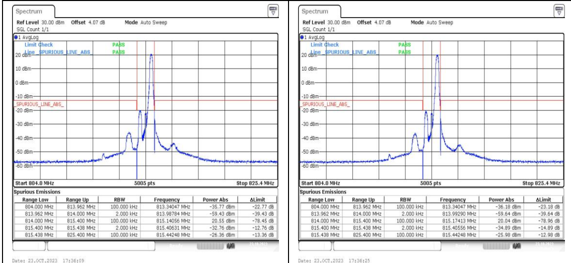
Band26_1.4MHz_QPSK_26697_1RB#5
