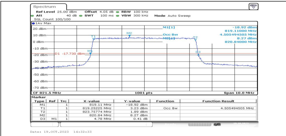
Band26-5MHz-16QAM-26765-25RB#0-PASS
