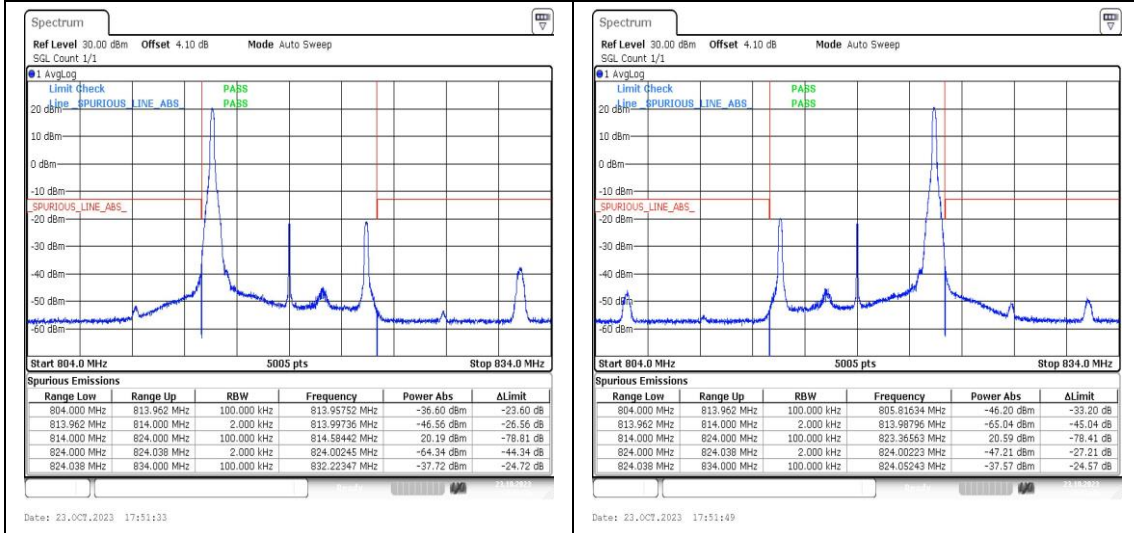
Band26_10MHz_QPSK_26740_1RB#0 Band26_10MHz_16QAM_26740_1RB#49
