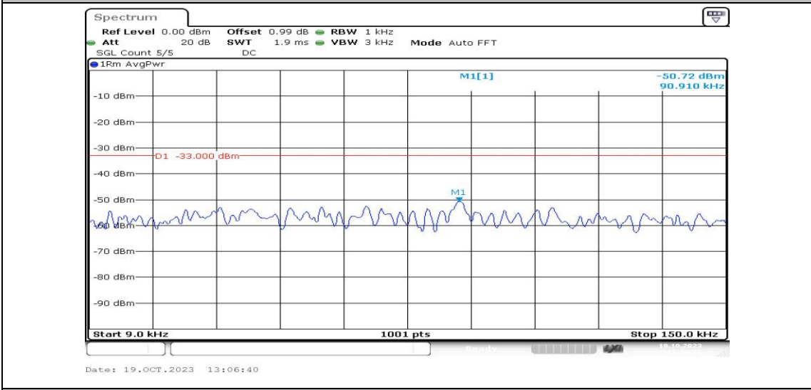
Band26-1.4MHz-QPSK-26783-1RB#0-Range1:0.009~0.15MHz-PASS
