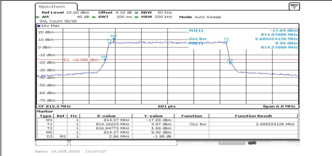
Band26-3MHz-QPSK-26705-15RB#0-PASS
