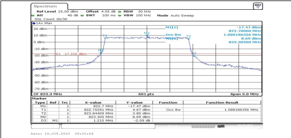
Band26-1.4MHz-16QAM-26783-6RB#0-PASS
