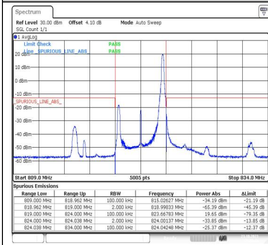
Band26_5MHz_QPSK_26765_1RB#0
