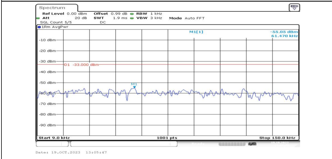
Band26-1.4MHz-16QAM-26740-1RB#0-Range1:0.009~0.15MHz-PASS
