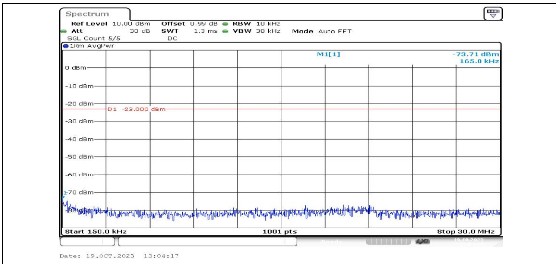
Band26-1.4MHz-16QAM-26697-1RB#0-Range2:0.15~30MHz-PASS
