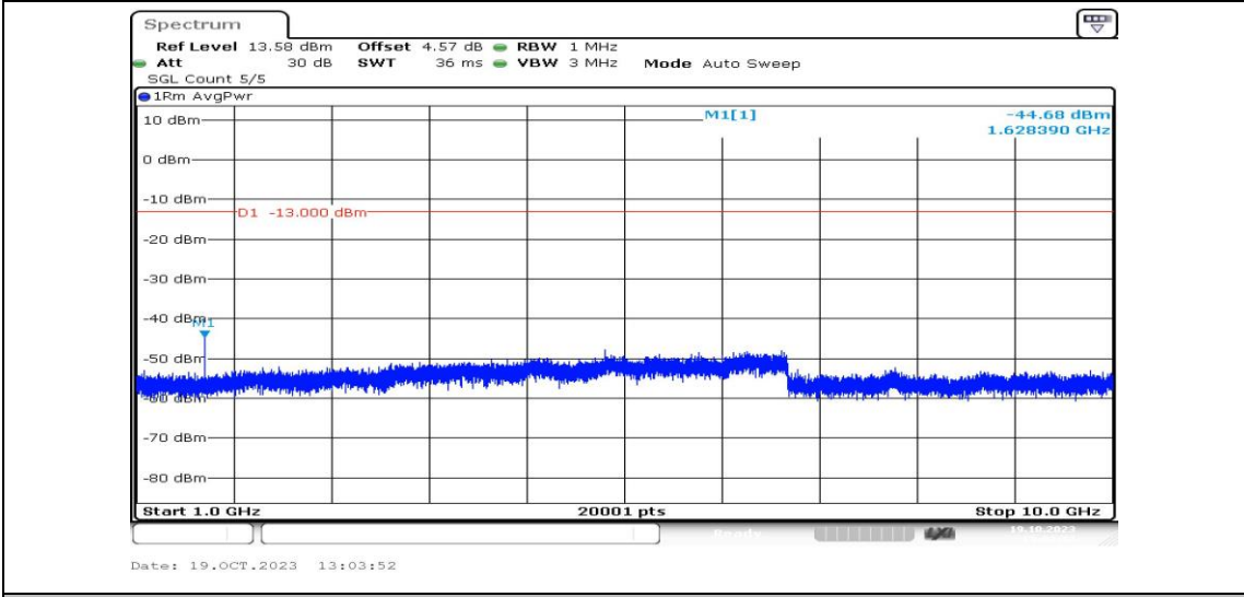
Band26-1.4MHz-QPSK-26697-1RB#0-Range4:1000~10000MHz-PASS
