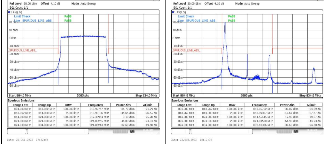
Band26_10MHz_QPSK_26740_50RB#0 Band26_10MHz_16QAM_26740_1RB#0
