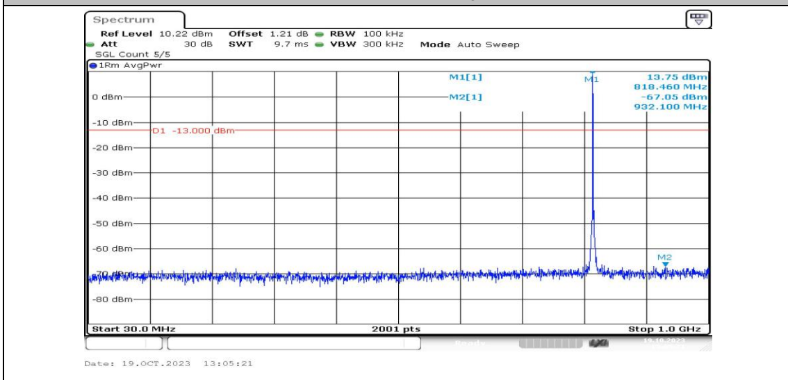
Band26-1.4MHz-QPSK-26740-1RB#0-Range3:30~1000MHz-PASS
