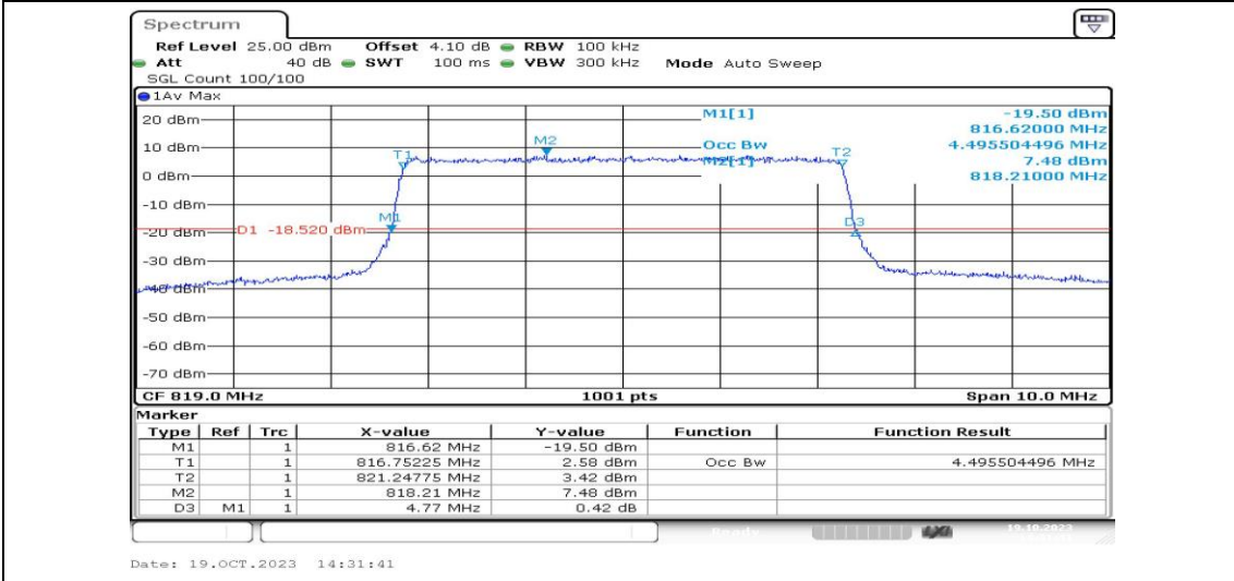
Band26-5MHz-16QAM-26740-25RB#0-PASS
