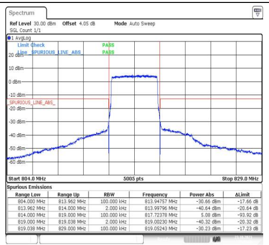
Band26_5MHz_16QAM_26715_25RB#0
