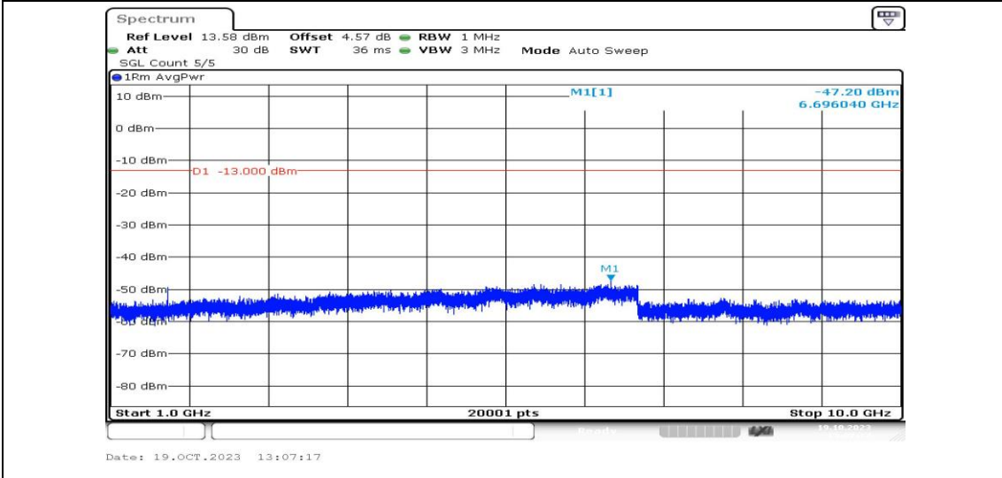
Band26-1.4MHz-QPSK-26783-1RB#0-Range4:1000~10000MHz-PASS
