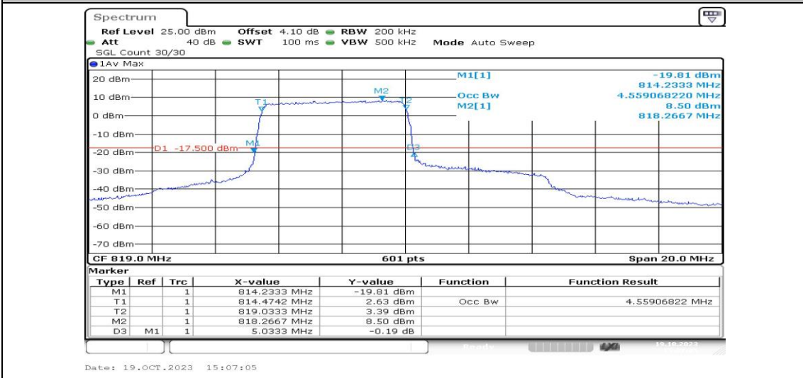
Band26-10MHz-16QAM-26740-25RB#0-PASS
