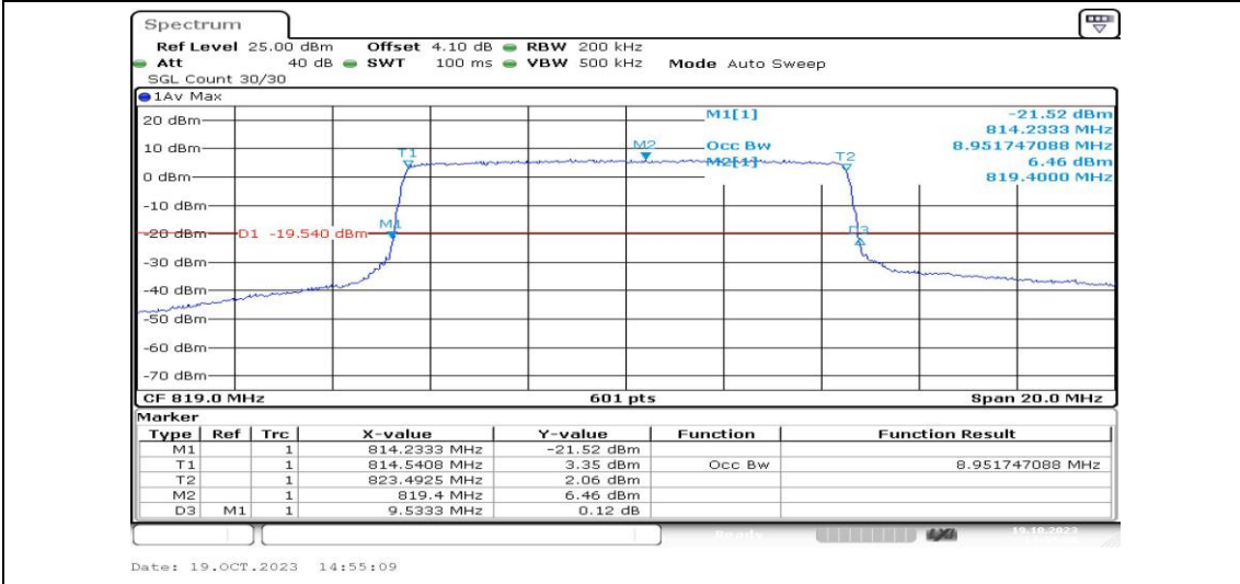
Band26-10MHz-QPSK-26740-50RB#0-PASS
