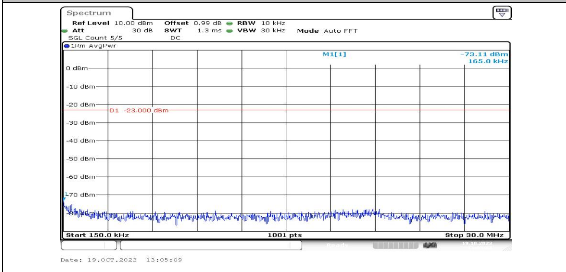
Band26-1.4MHz-QPSK-26740-1RB#0-Range2:0.15~30MHz-PASS
