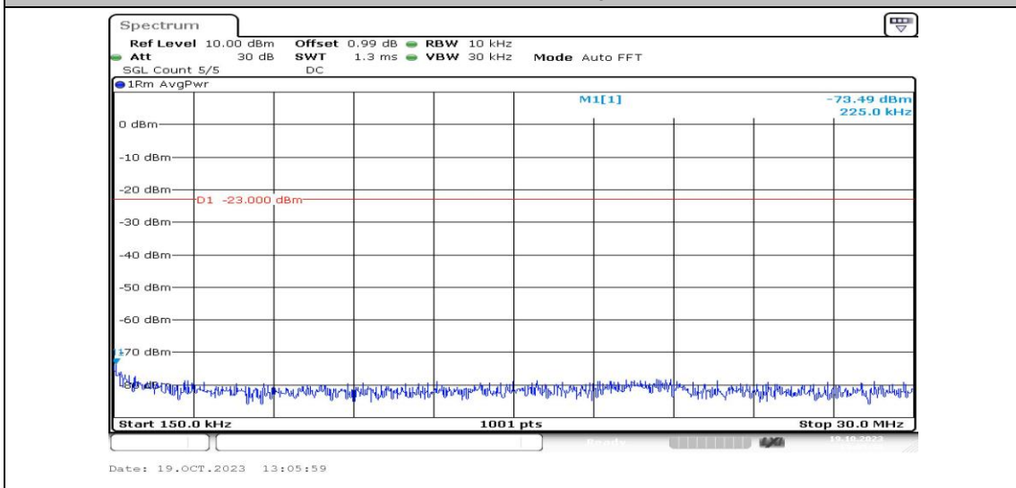
Band26-1.4MHz-16QAM-26740-1RB#0-Range2:0.15~30MHz-PASS
