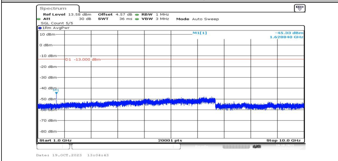
Band26-1.4MHz-16QAM-26697-1RB#0-Range4:1000~10000MHz-PASS
