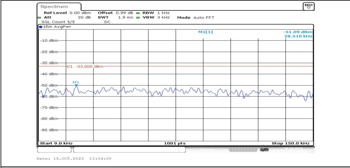
Band26-1.4MHz-16QAM-26697-1RB#0-Range1:0.009~0.15MHz-PASS
