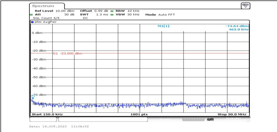
Band26-1.4MHz-QPSK-26783-1RB#0-Range2:0.15~30MHz-PASS
