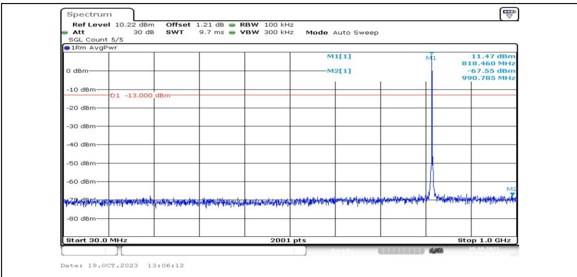
Band26-1.4MHz-16QAM-26740-1RB#0-Range3:30~1000MHz-PASS
