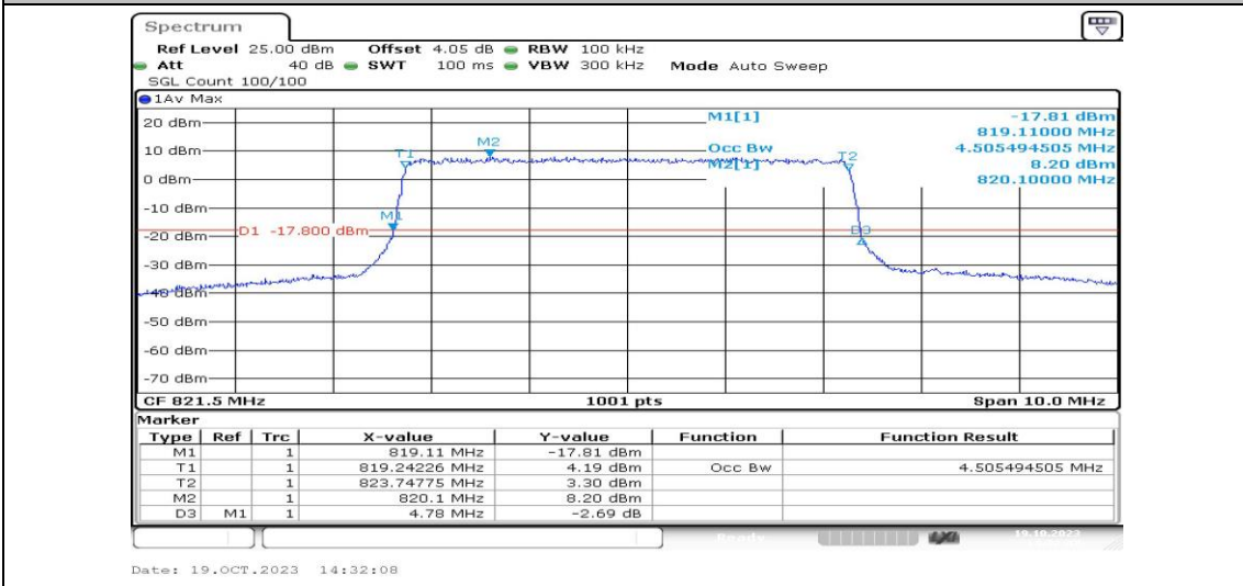
Band26-5MHz-QPSK-26765-25RB#0-PASS
