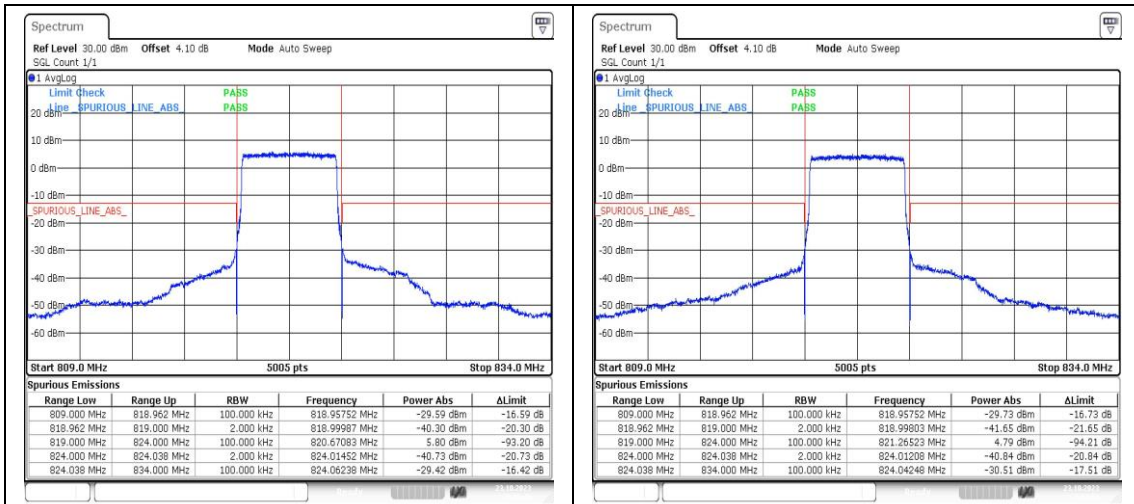
Band26_5MHz_QPSK_26765_25RB#0 Band26_5MHz_16QAM_26765_25RB#0
