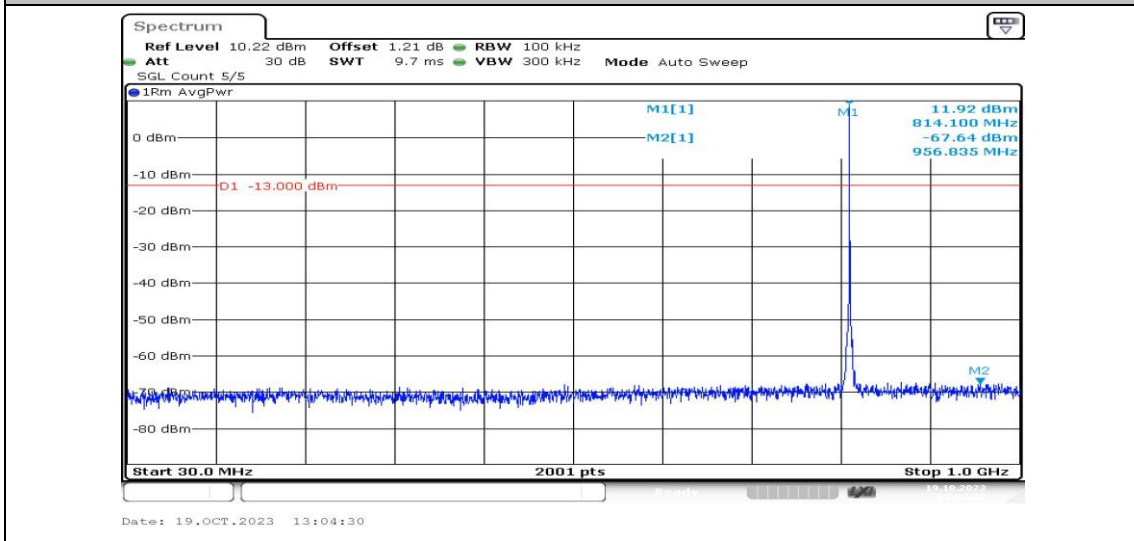
Band26-1.4MHz-16QAM-26697-1RB#0-Range3:30~1000MHz-PASS
