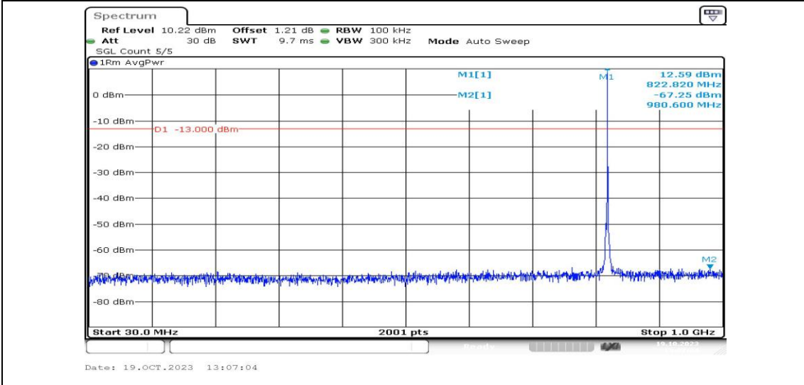
Band26-1.4MHz-QPSK-26783-1RB#0-Range3:30~1000MHz-PASS
