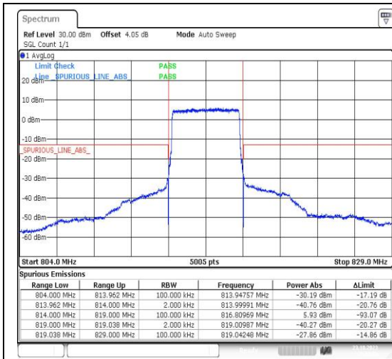
Band26_5MHz_QPSK_26715_25RB#0
