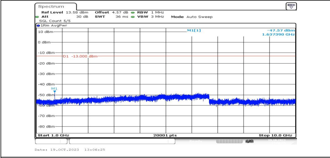
Band26-1.4MHz-16QAM-26740-1RB#0-Range4:1000~10000MHz-PASS
