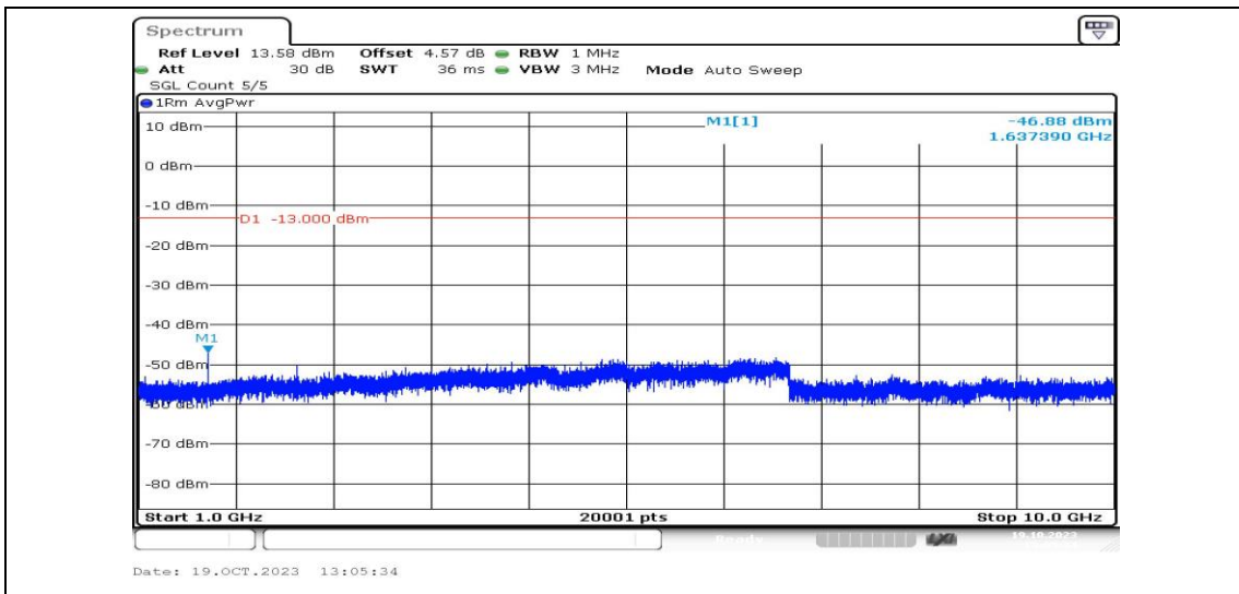
Band26-1.4MHz-QPSK-26740-1RB#0-Range4:1000~10000MHz-PASS
