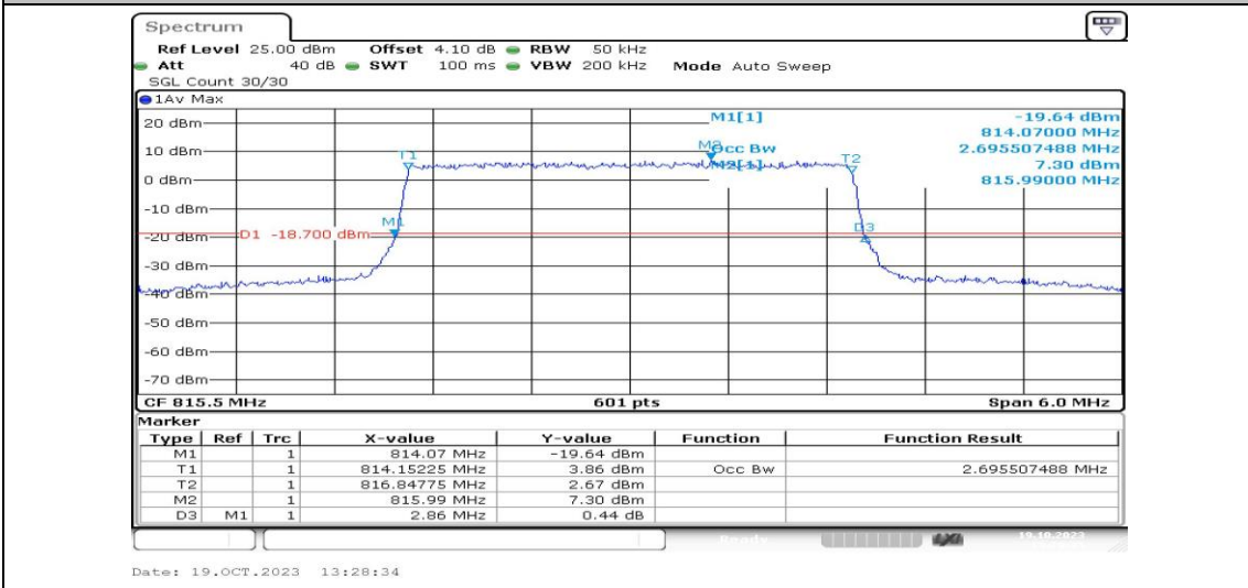
Band26-3MHz-16QAM-26705-15RB#0-PASS
