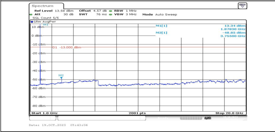
Band25-10MHz-16QAM-26365-1RB#0-Range4:1000~20000MHz-PASS
