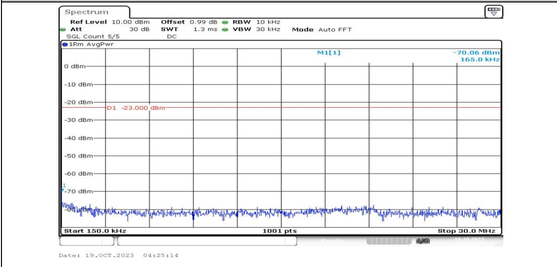
Band25-15MHz-QPSK-26115-1RB#0-Range2:0.15~30MHz-PASS
