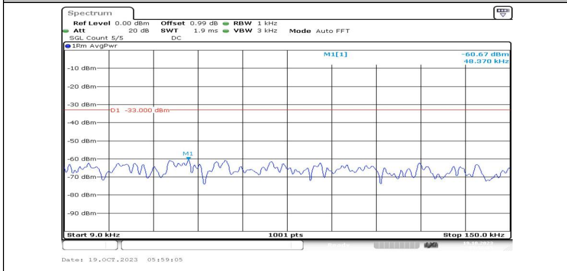
Band25-15MHz-16QAM-26115-1RB#0-Range1:0.009~0.15MHz-PASS
