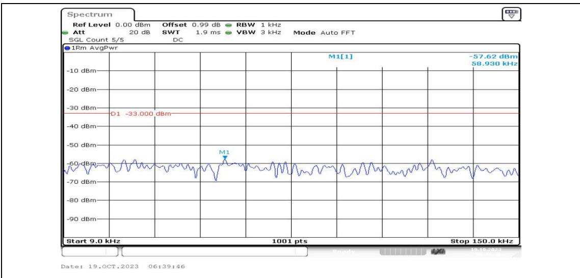
Band25-20MHz-16QAM-26590-1RB#0-Range1:0.009~0.15MHz-PASS
