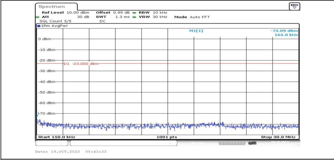
Band25-10MHz-16QAM-26640-1RB#0-Range2:0.15~30MHz-PASS
