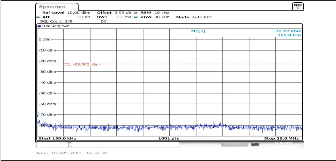
Band25-5MHz-16QAM-26665-1RB#0-Range2:0.15~30MHz-PASS
