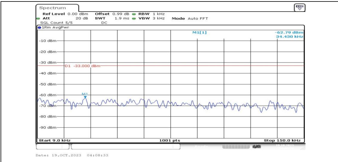
Band25-10MHz-QPSK-26640-1RB#0-Range1:0.009~0.15MHz-PASS
