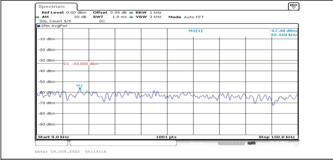
Band25-20MHz-QPSK-26140-1RB#0-Range1:0.009~0.15MHz-PASS
