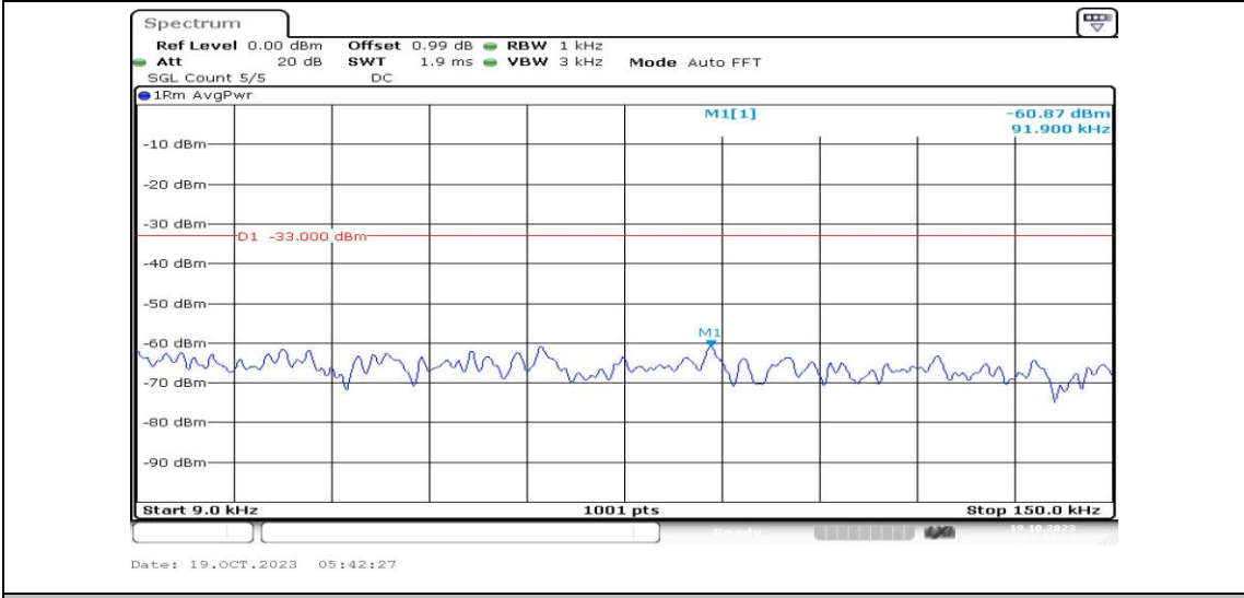
Band25-10MHz-16QAM-26365-1RB#0-Range1:0.009~0.15MHz-PASS
