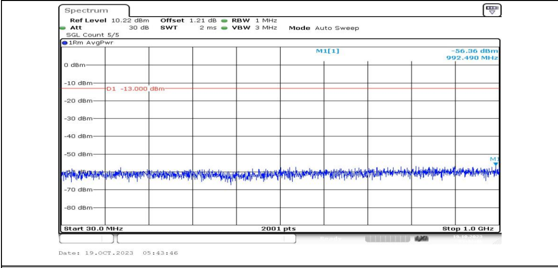
Band25-10MHz-16QAM-26640-1RB#0-Range3:30~1000MHz-PASS
