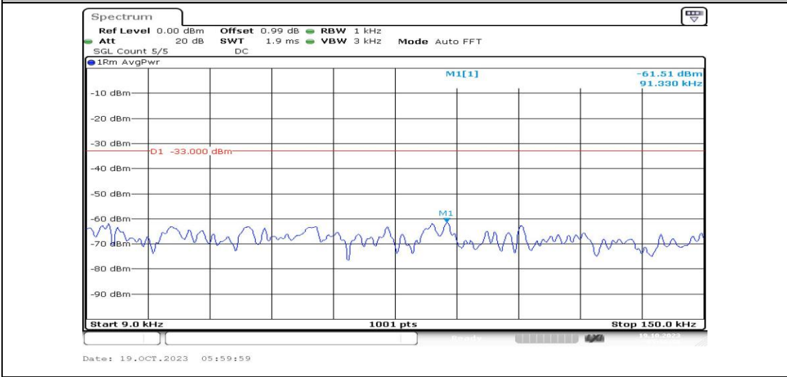
Band25-15MHz-16QAM-26365-1RB#0-Range1:0.009~0.15MHz-PASS
