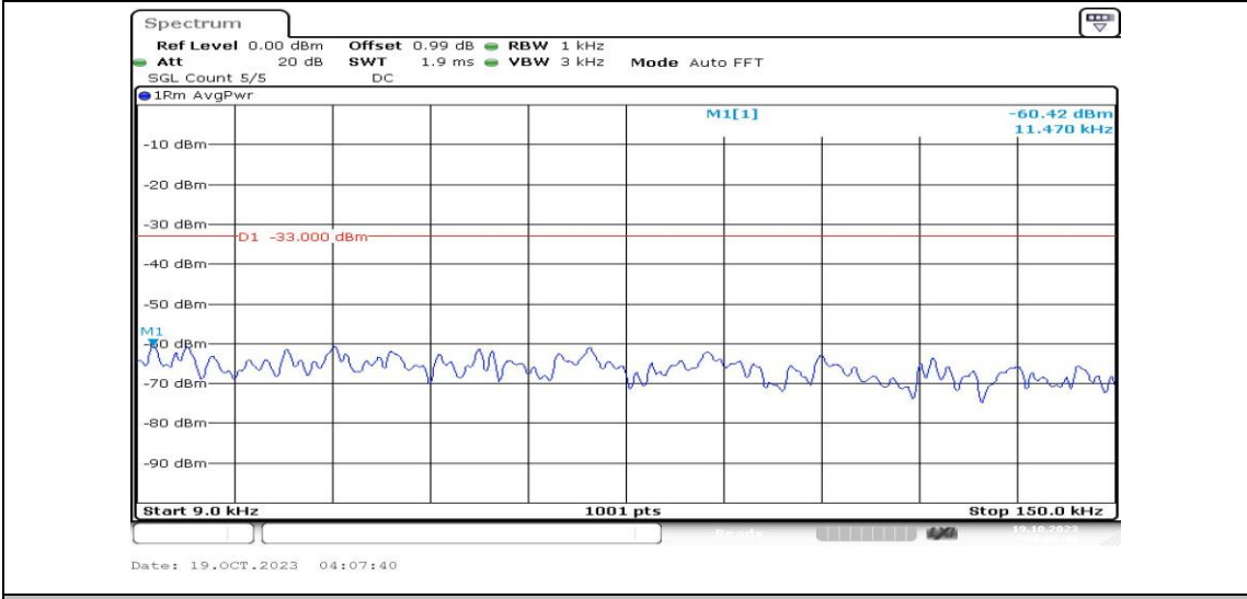
Band25-10MHz-QPSK-26365-1RB#0-Range1:0.009~0.15MHz-PASS
