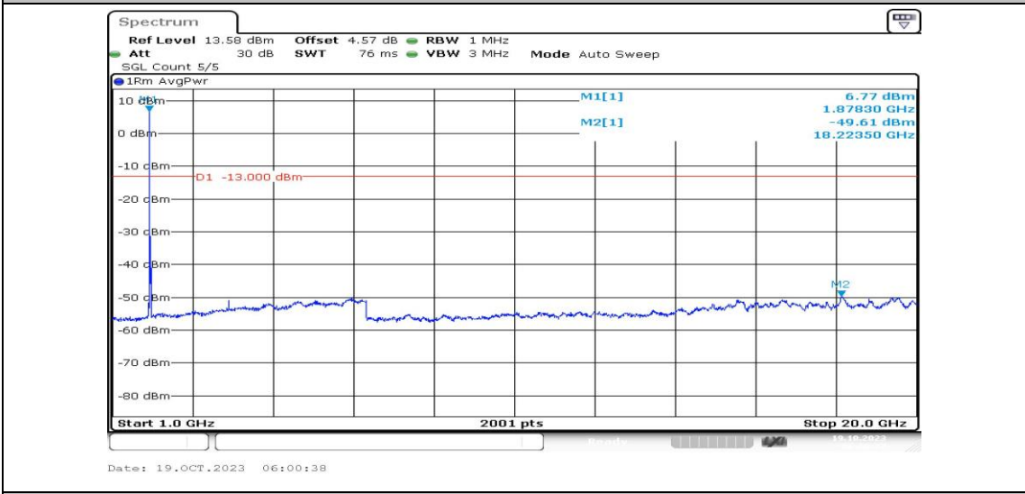
Band25-15MHz-16QAM-26365-1RB#0-Range4:1000~20000MHz-PASS
