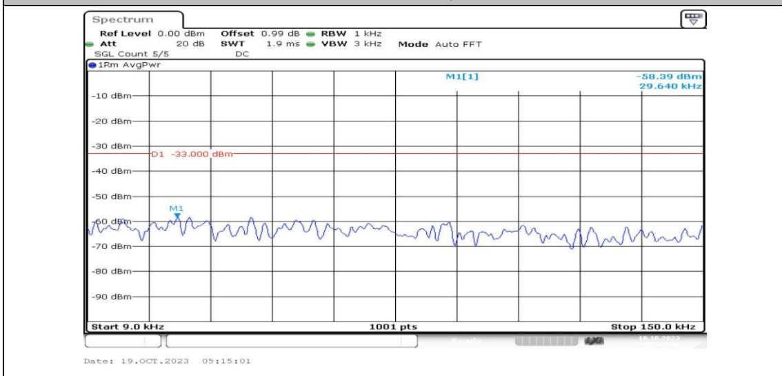
Band25-20MHz-QPSK-26365-1RB#0-Range1:0.009~0.15MHz-PASS
