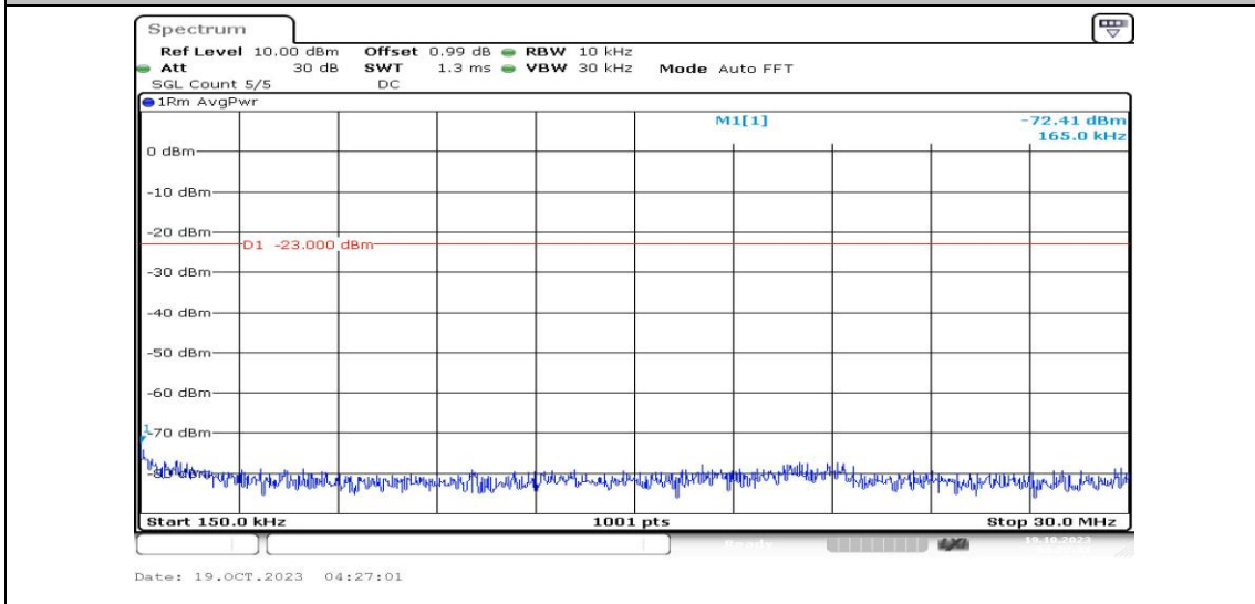
Band25-15MHz-QPSK-26615-1RB#0-Range2:0.15~30MHz-PASS
