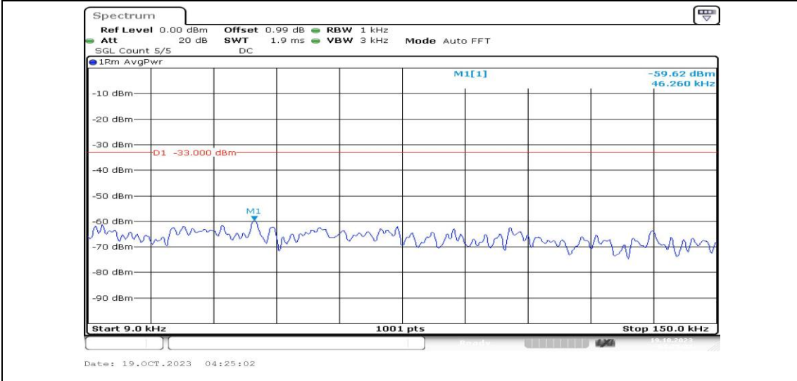
Band25-15MHz-QPSK-26115-1RB#0-Range1:0.009~0.15MHz-PASS
