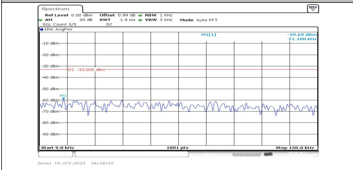
Band25-20MHz-16QAM-26365-1RB#0-Range1:0.009~0.15MHz-PASS
