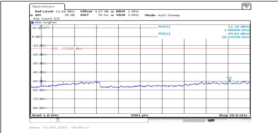
Band25-10MHz-QPSK-26640-1RB#0-Range4:1000~20000MHz-PASS
