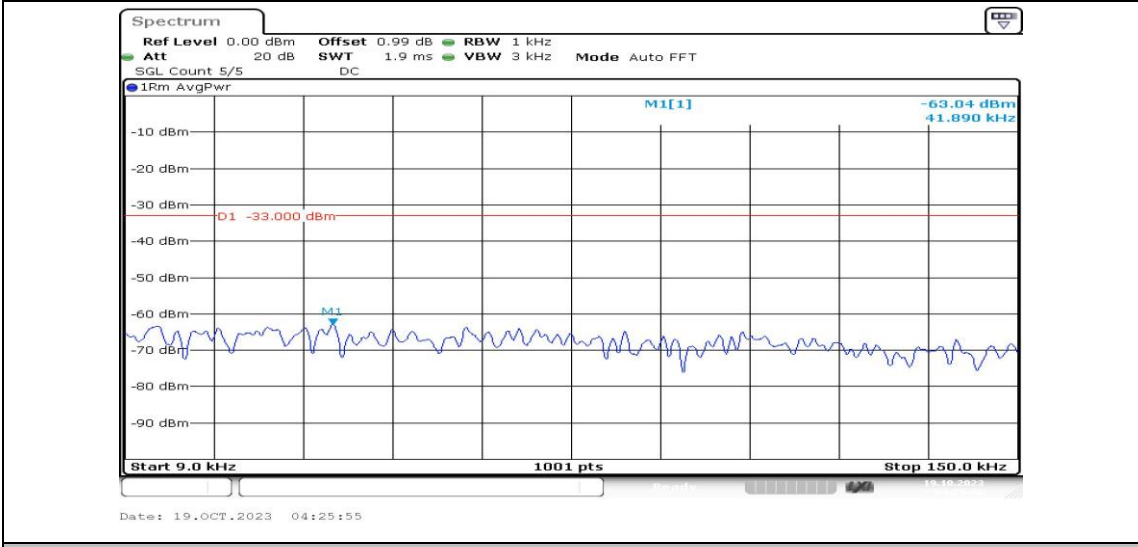
Band25-15MHz-QPSK-26365-1RB#0-Range1:0.009~0.15MHz-PASS
