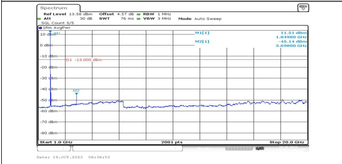
Band25-20MHz-16QAM-26140-1RB#0-Range4:1000~20000MHz-PASS
