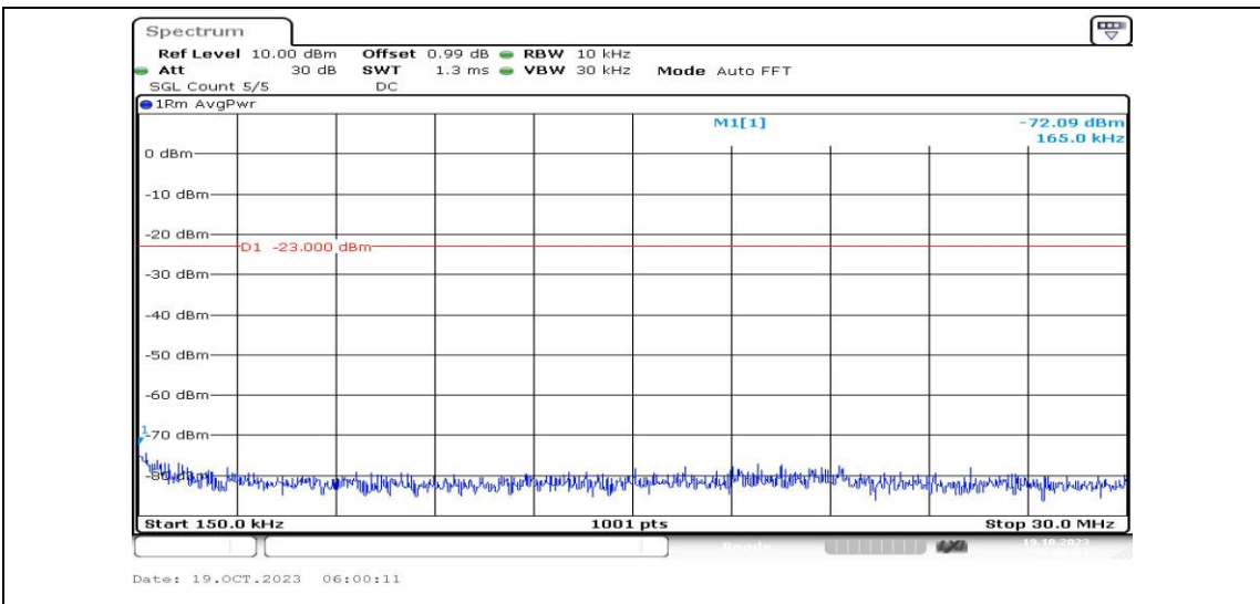
Band25-15MHz-16QAM-26365-1RB#0-Range2:0.15~30MHz-PASS
