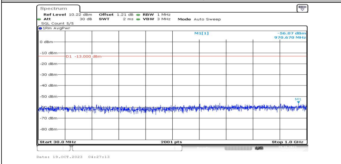
Band25-15MHz-QPSK-26615-1RB#0-Range3:30~1000MHz-PASS
