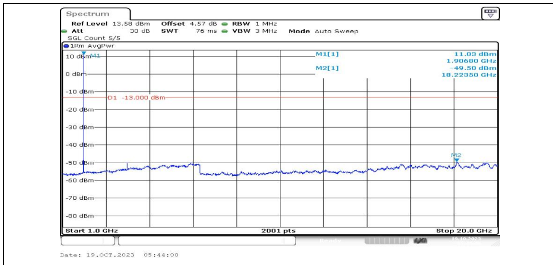
Band25-10MHz-16QAM-26640-1RB#0-Range4:1000~20000MHz-PASS
