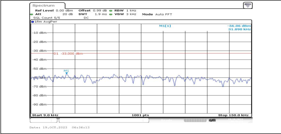
Band25-20MHz-16QAM-26140-1RB#0-Range1:0.009~0.15MHz-PASS
