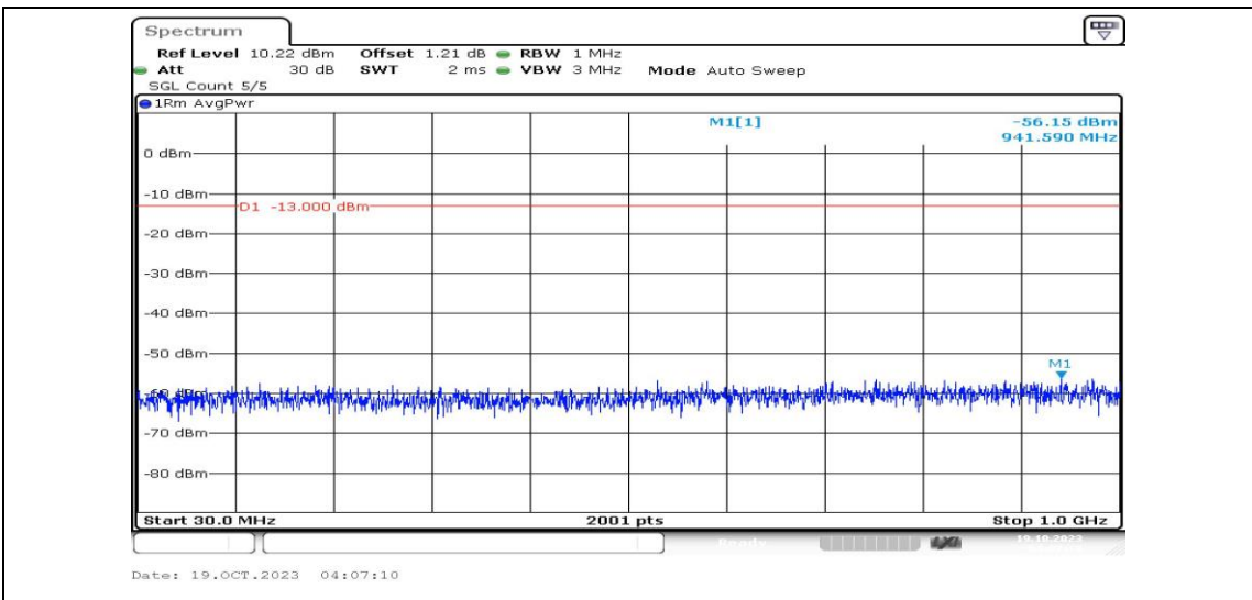
Band25-10MHz-QPSK-26090-1RB#0-Range3:30~1000MHz-PASS
