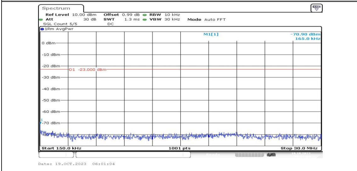
Band25-15MHz-16QAM-26615-1RB#0-Range2:0.15~30MHz-PASS
