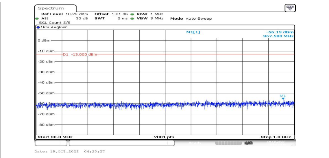
Band25-15MHz-QPSK-26115-1RB#0-Range3:30~1000MHz-PASS
