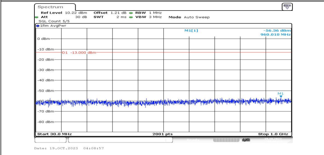
Band25-10MHz-QPSK-26640-1RB#0-Range3:30~1000MHz-PASS
