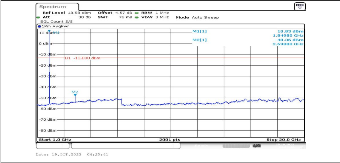
Band25-15MHz-QPSK-26115-1RB#0-Range4:1000~20000MHz-PASS
