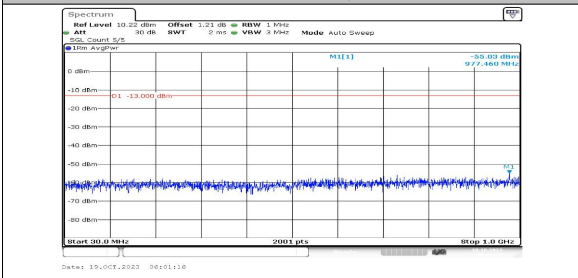
Band25-15MHz-16QAM-26615-1RB#0-Range3:30~1000MHz-PASS
