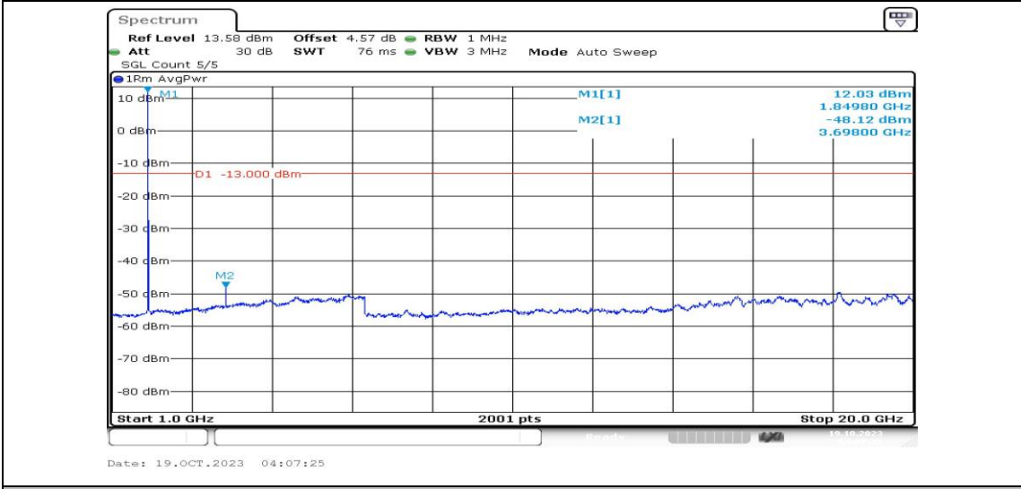
Band25-10MHz-QPSK-26090-1RB#0-Range4:1000~20000MHz-PASS
