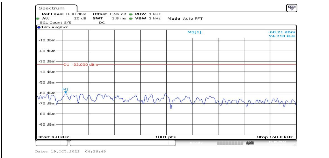
Band25-15MHz-QPSK-26615-1RB#0-Range1:0.009~0.15MHz-PASS
