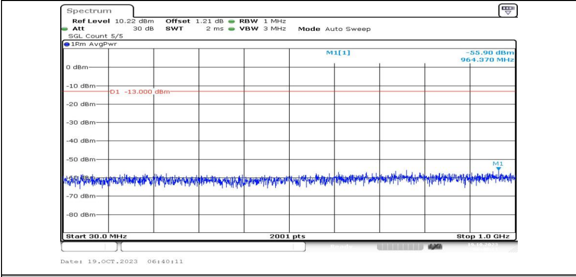
Band25-20MHz-16QAM-26590-1RB#0-Range3:30~1000MHz-PASS
