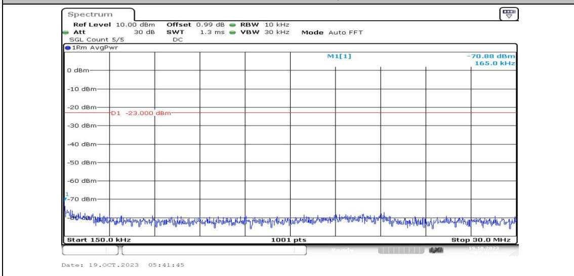
Band25-10MHz-16QAM-26090-1RB#0-Range2:0.15~30MHz-PASS
