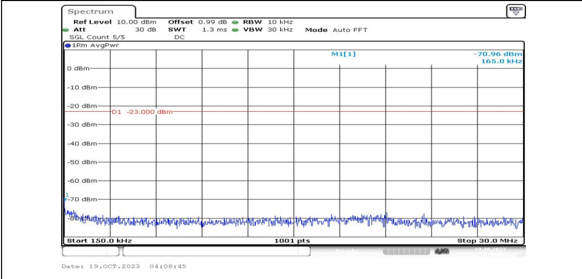
Band25-10MHz-QPSK-26640-1RB#0-Range2:0.15~30MHz-PASS
