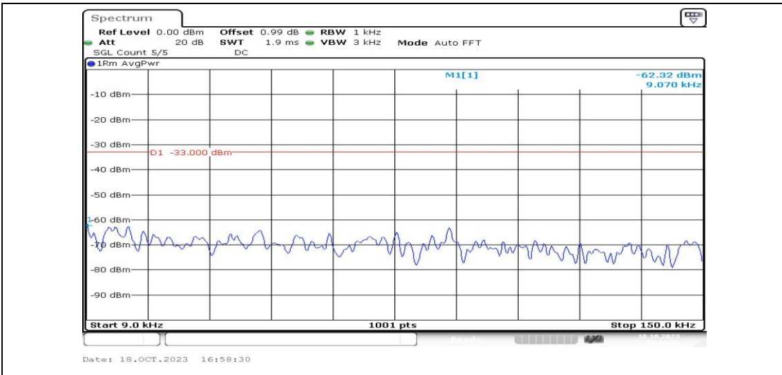
Band25-5MHz-16QAM-26665-1RB#0-Range1:0.009~0.15MHz-PASS
