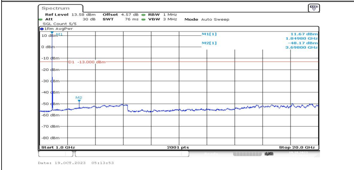
Band25-20MHz-QPSK-26140-1RB#0-Range4:1000~20000MHz-PASS
