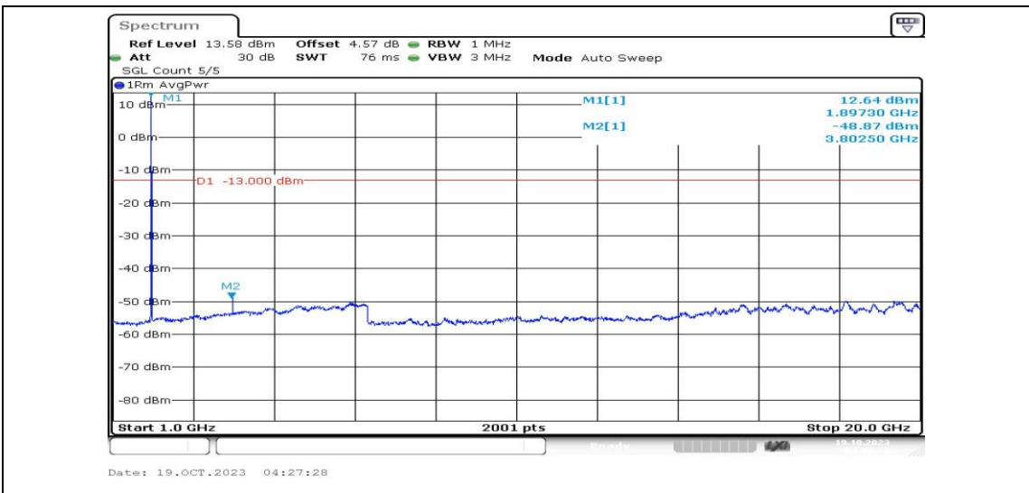
Band25-15MHz-QPSK-26615-1RB#0-Range4:1000~20000MHz-PASS
