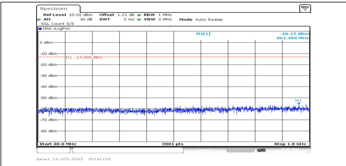
Band25-10MHz-16QAM-26090-1RB#0-Range3:30~1000MHz-PASS
