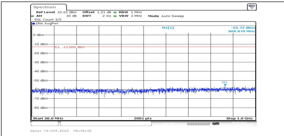
Band25-20MHz-16QAM-26140-1RB#0-Range3:30~1000MHz-PASS
