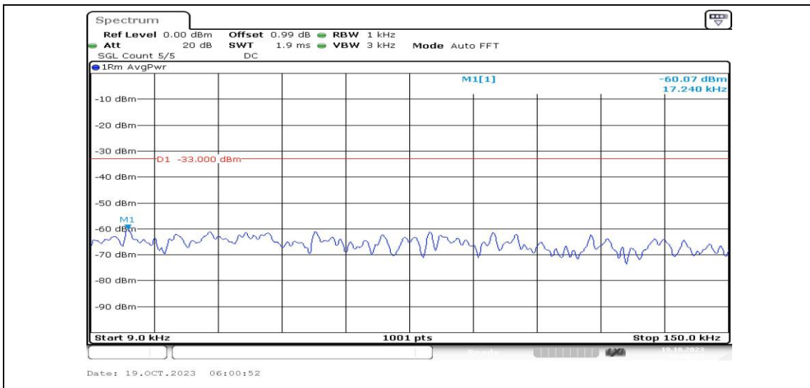
Band25-15MHz-16QAM-26615-1RB#0-Range1:0.009~0.15MHz-PASS
