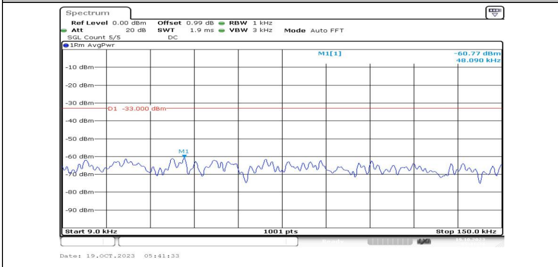
Band25-10MHz-16QAM-26090-1RB#0-Range1:0.009~0.15MHz-PASS
