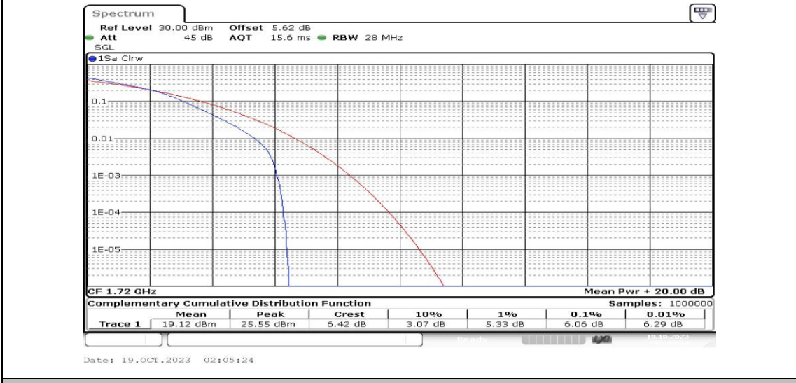
Band4-20MHz-16QAM-20050-25RB#0-PASS
