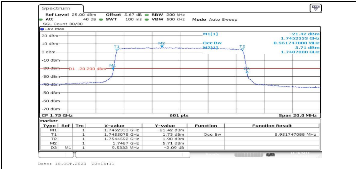
Band4-10MHz-QPSK-20350-50RB#0-PASS
