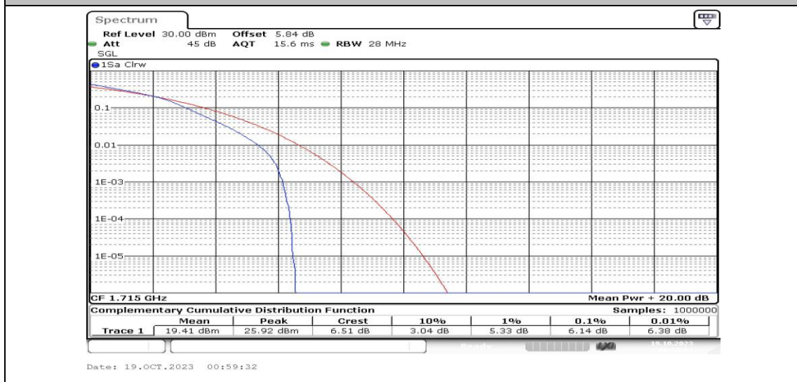
Band4-10MHz-16QAM-20000-25RB#0-PASS
