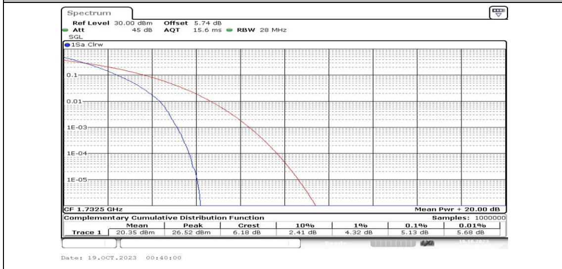
Band4-20MHz-QPSK-20175-100RB#0-PASS
