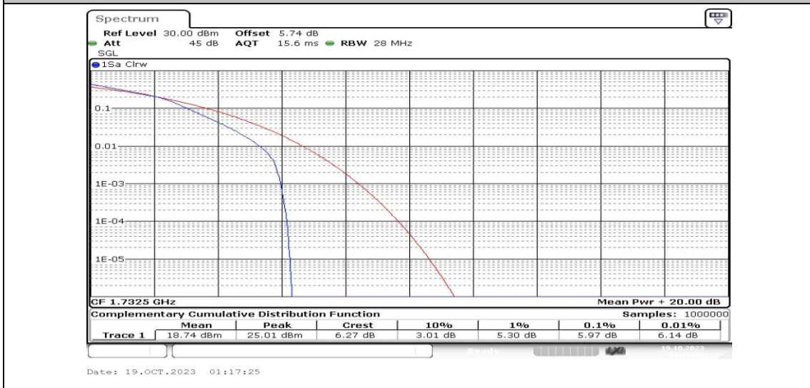
Band4-15MHz-16QAM-20175-25RB#0-PASS
