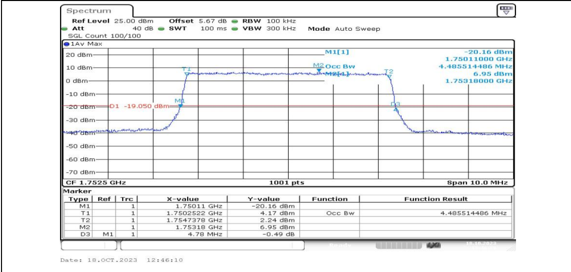
Band4-5MHz-QPSK-20375-25RB#0-PASS
