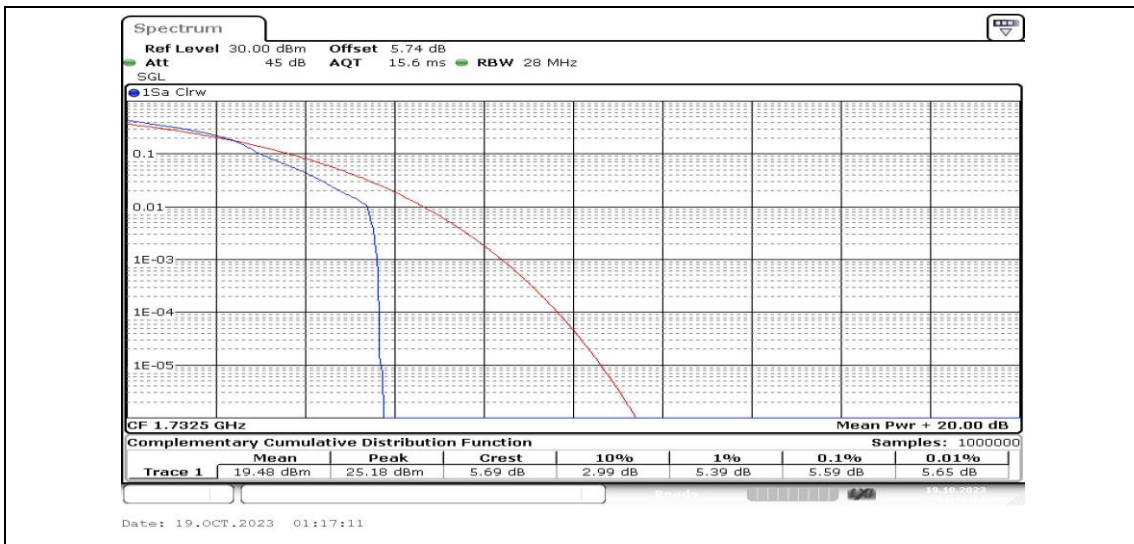
Band4-15MHz-16QAM-20175-1RB#0-PASS
