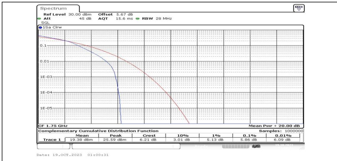
Band4-10MHz-16QAM-20350-25RB#0-PASS
