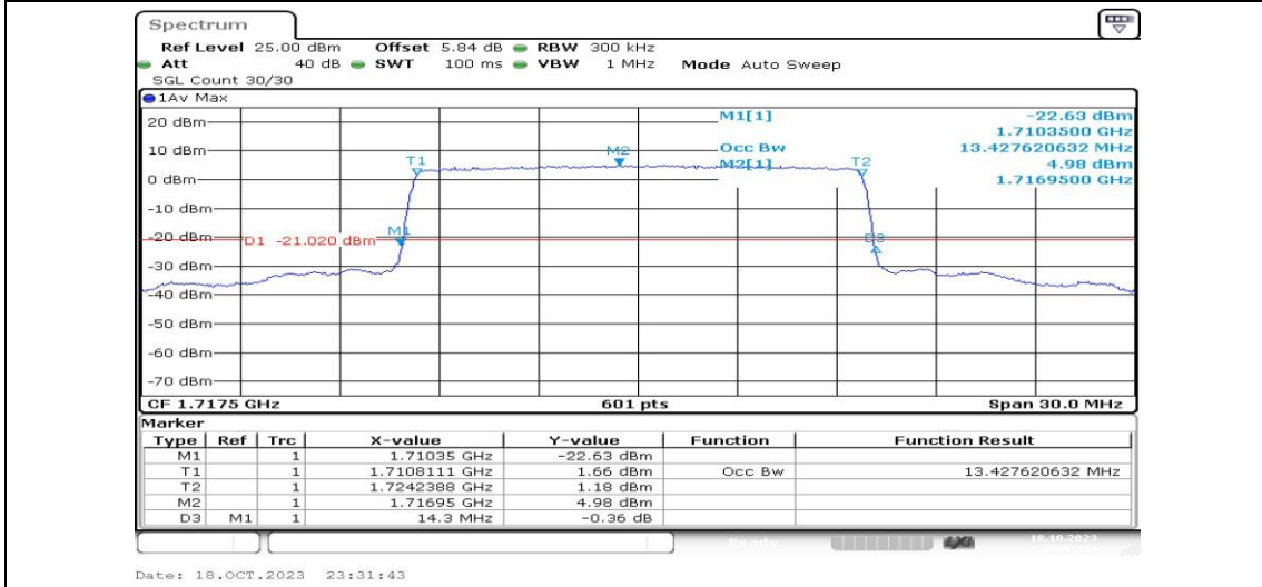
Band4-15MHz-QPSK-20025-75RB#0-PASS
