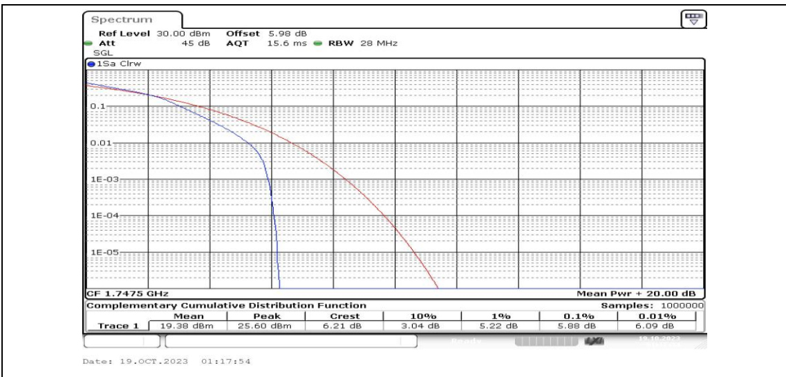
Band4-15MHz-16QAM-20325-25RB#0-PASS
