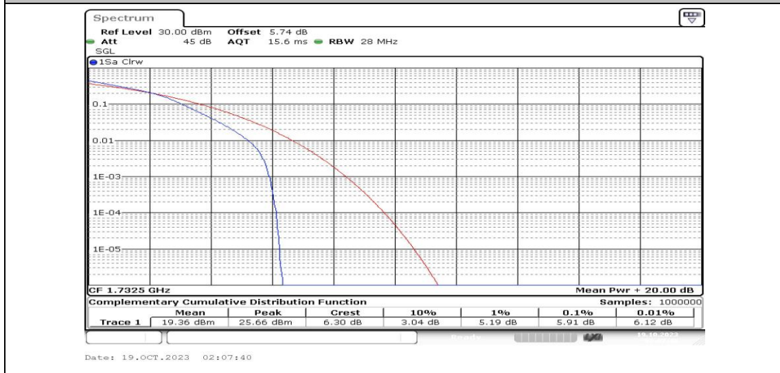
Band4-20MHz-16QAM-20175-25RB#0-PASS
