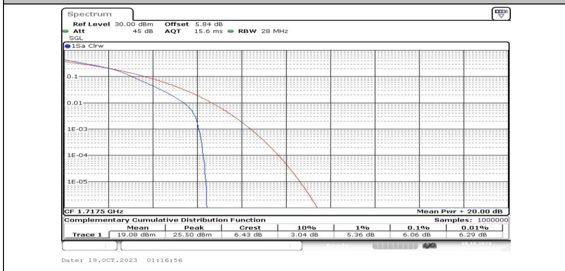
Band4-15MHz-16QAM-20025-25RB#0-PASS
