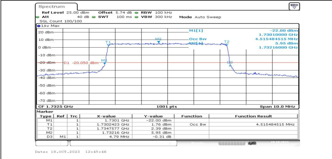
Band4-5MHz-16QAM-20175-25RB#0-PASS
