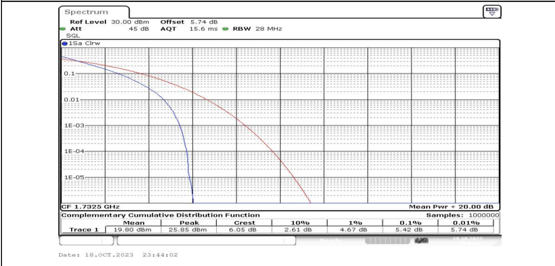
Band4-15MHz-QPSK-20175-75RB#0-PASS
