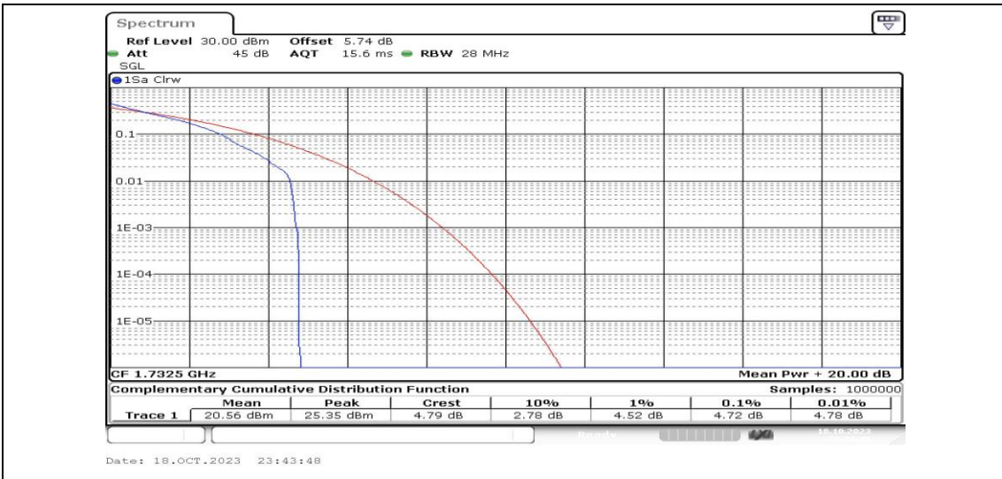
Band4-15MHz-QPSK-20175-1RB#0-PASS
