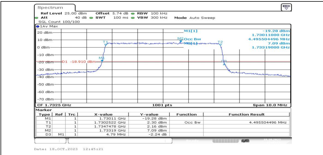
Band4-5MHz-QPSK-20175-25RB#0-PASS
