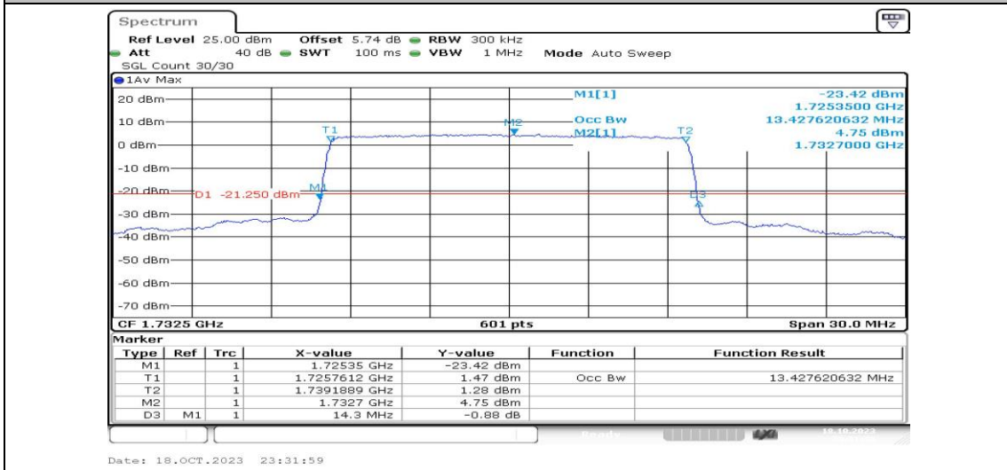
Band4-15MHz-QPSK-20175-75RB#0-PASS
