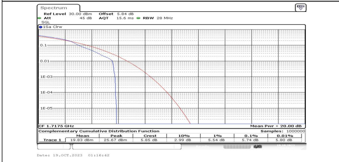
Band4-15MHz-16QAM-20025-1RB#0-PASS
