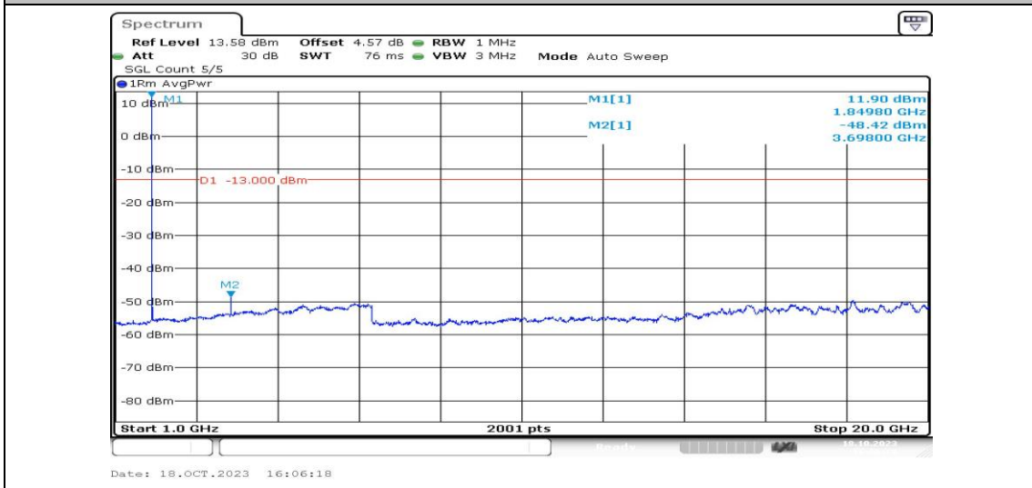
Band25-1.4MHz-QPSK-26047-1RB#0-Range4:1000~20000MHz-PASS
