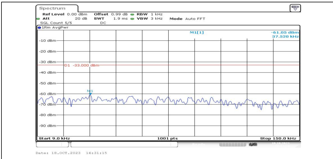
Band25-3MHz-QPSK-26365-1RB#0-Range1:0.009~0.15MHz-PASS
