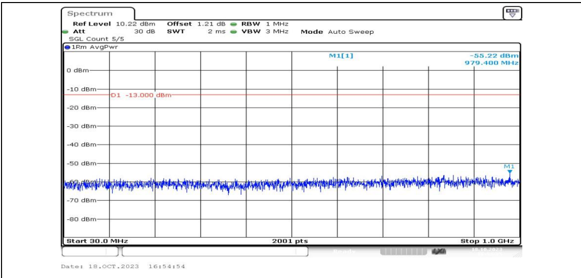
Band25-5MHz-QPSK-26065-1RB#0-Range3:30~1000MHz-PASS
