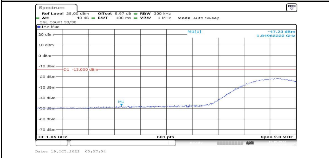
Band25-15MHz-16QAM-26115-1RB#74-PASS
