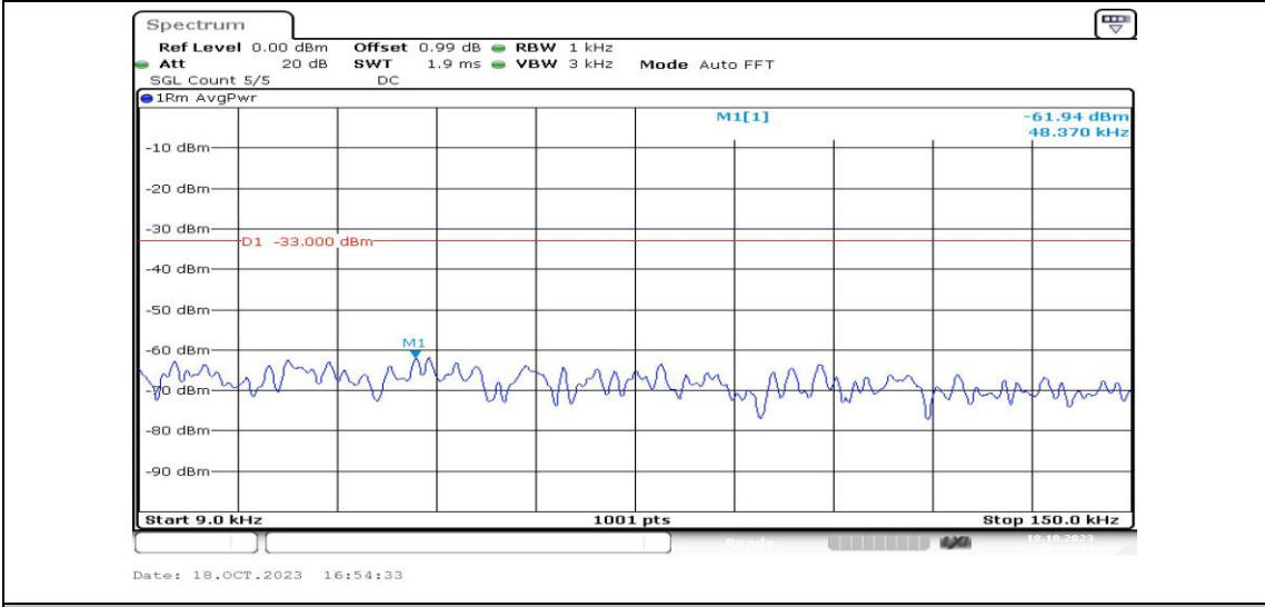
Band25-5MHz-QPSK-26065-1RB#0-Range1:0.009~0.15MHz-PASS
