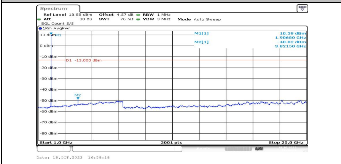
Band25-5MHz-QPSK-26665-1RB#0-Range4:1000~20000MHz-PASS
