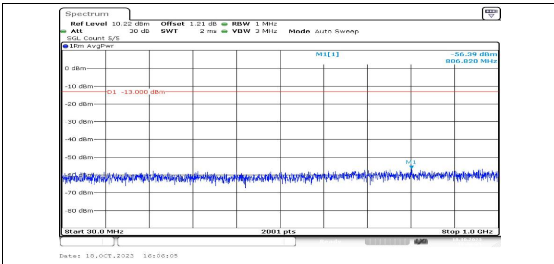
Band25-1.4MHz-QPSK-26047-1RB#0-Range3:30~1000MHz-PASS
