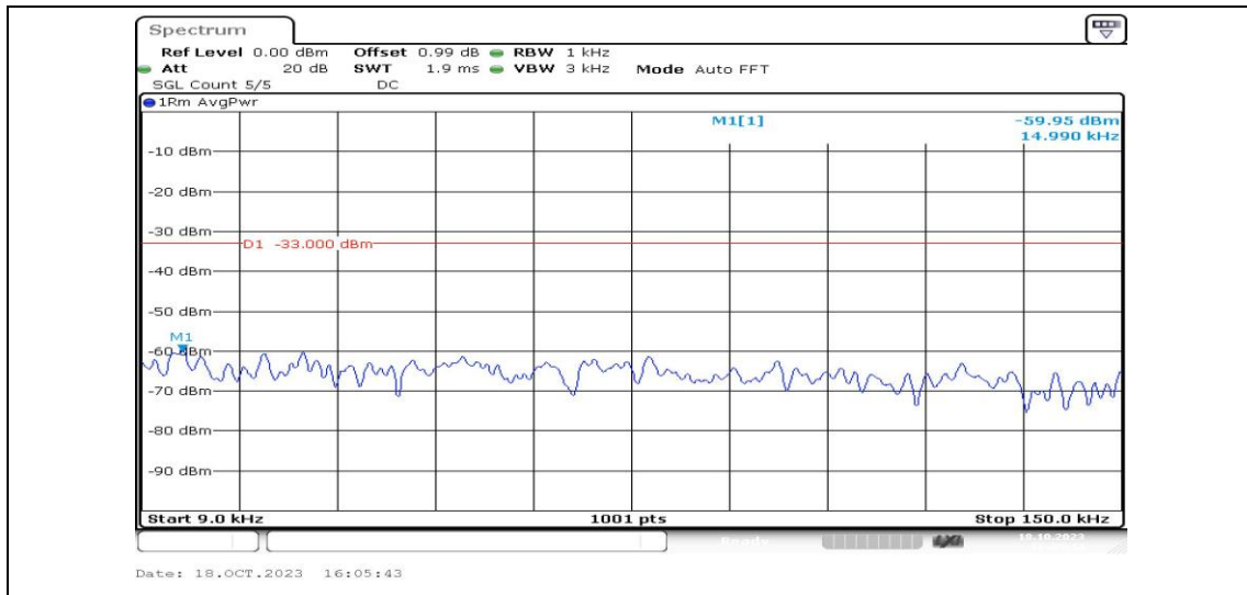
Band25-1.4MHz-QPSK-26047-1RB#0-Range1:0.009~0.15MHz-PASS
