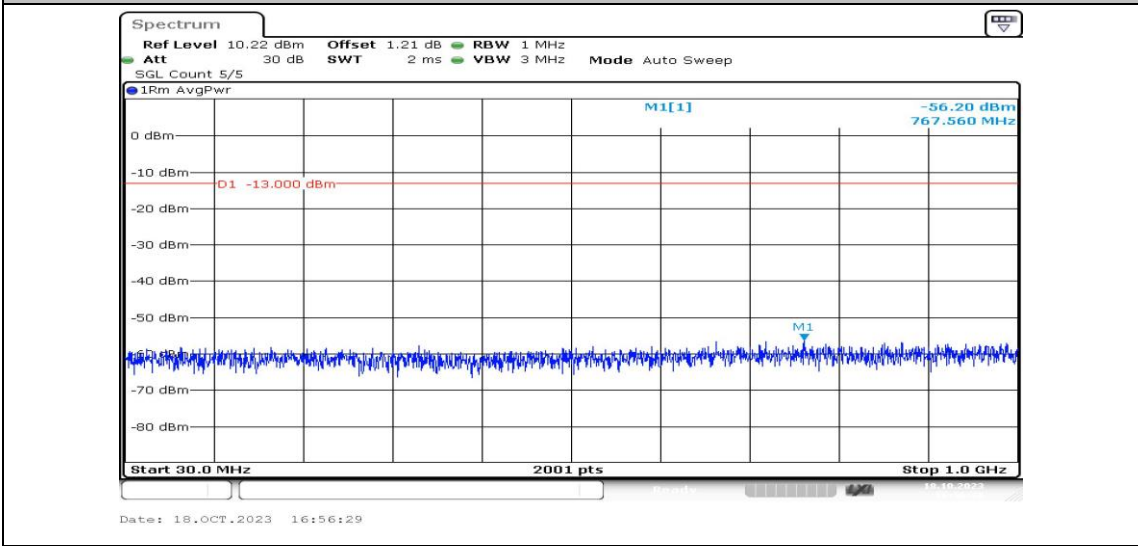
Band25-5MHz-QPSK-26365-1RB#0-Range3:30~1000MHz-PASS
