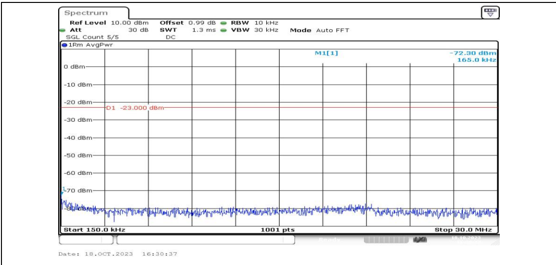
Band25-3MHz-16QAM-26055-1RB#0-Range2:0.15~30MHz-PASS
