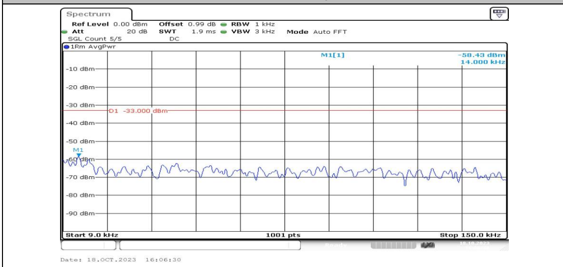
Band25-1.4MHz-16QAM-26047-1RB#0-Range1:0.009~0.15MHz-PASS
