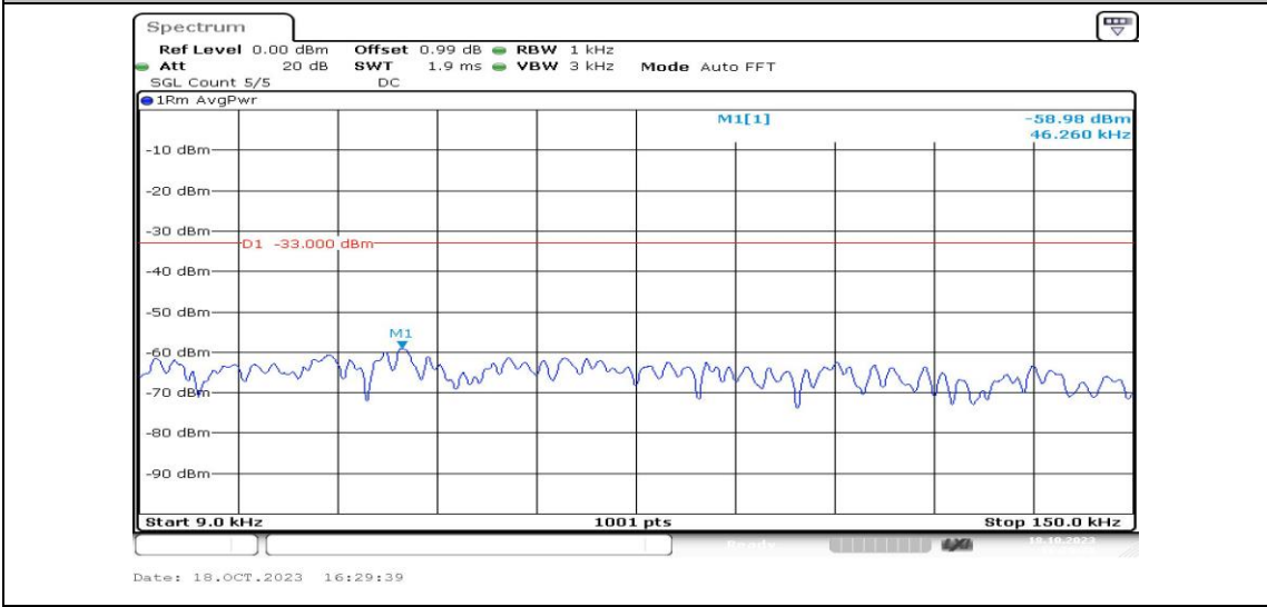
Band25-3MHz-QPSK-26055-1RB#0-Range1:0.009~0.15MHz-PASS
