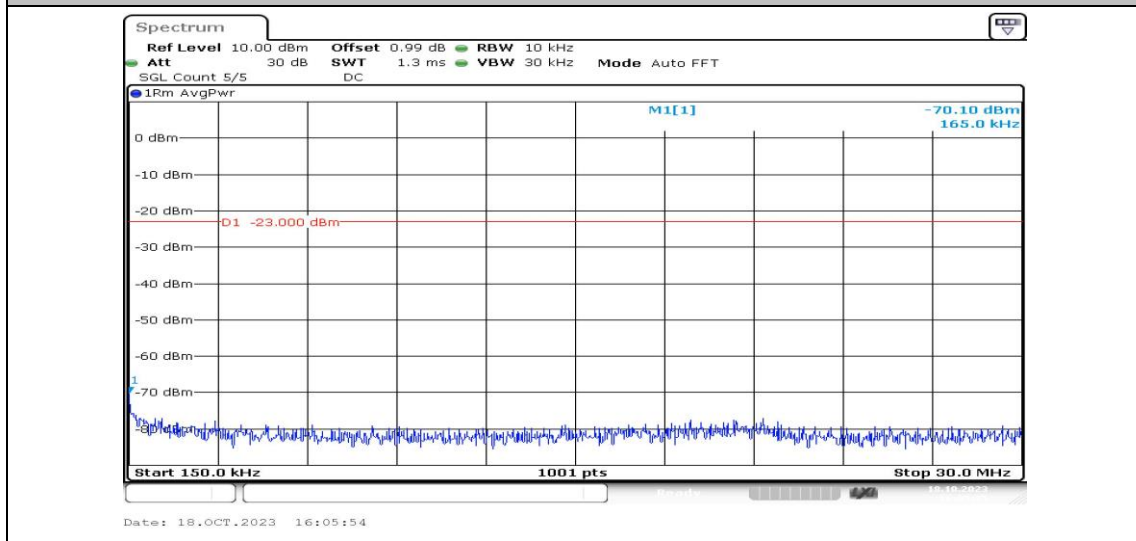
Band25-1.4MHz-QPSK-26047-1RB#0-Range2:0.15~30MHz-PASS
