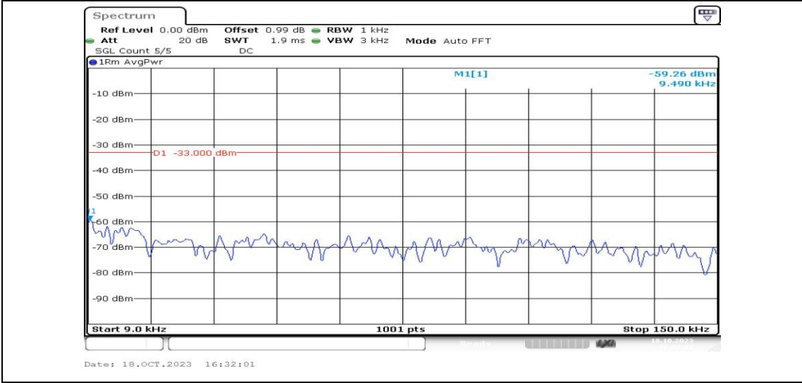
Band25-3MHz-16QAM-26365-1RB#0-Range1:0.009~0.15MHz-PASS
