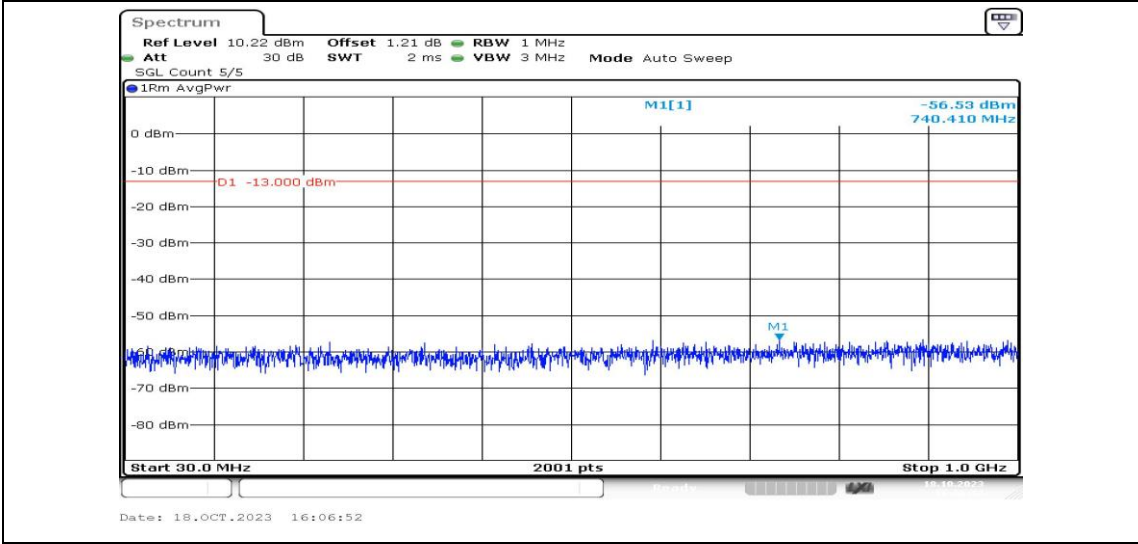
Band25-1.4MHz-16QAM-26047-1RB#0-Range3:30~1000MHz-PASS
