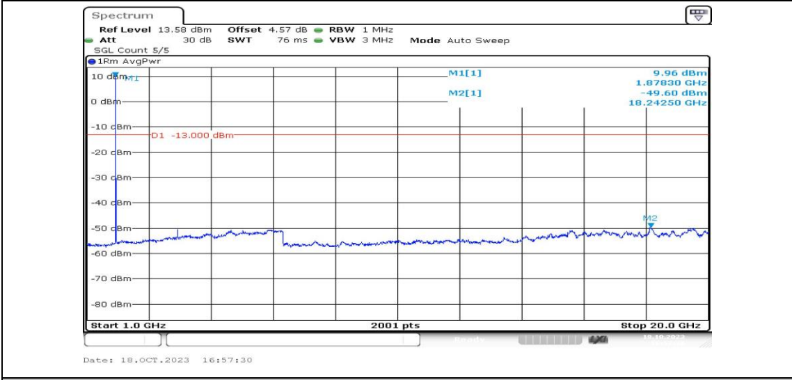
Band25-5MHz-16QAM-26365-1RB#0-Range4:1000~20000MHz-PASS
