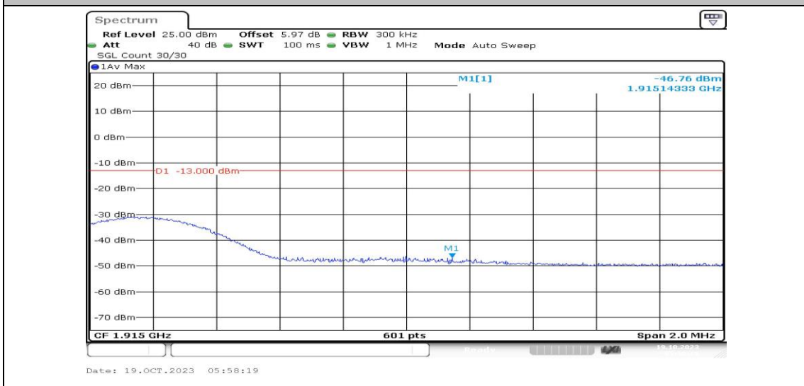
Band25-15MHz-16QAM-26615-1RB#0-PASS
