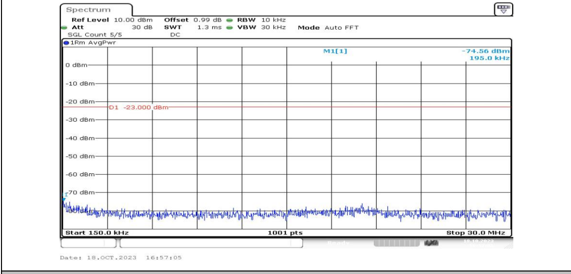
Band25-5MHz-16QAM-26365-1RB#0-Range2:0.15~30MHz-PASS
