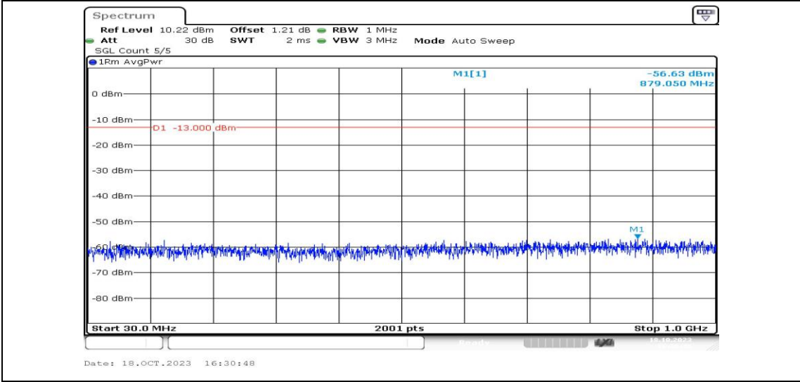
Band25-3MHz-16QAM-26055-1RB#0-Range3:30~1000MHz-PASS
