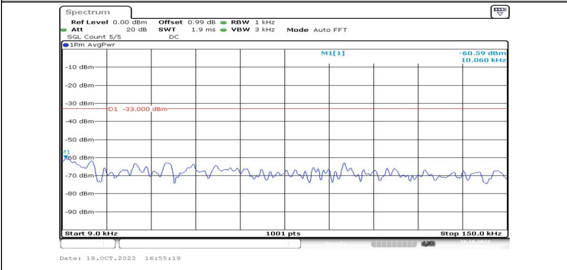
Band25-5MHz-16QAM-26065-1RB#0-Range1:0.009~0.15MHz-PASS
