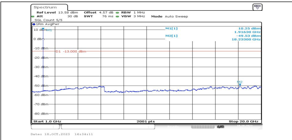
Band25-3MHz-16QAM-26675-1RB#0-Range4:1000~20000MHz-PASS
