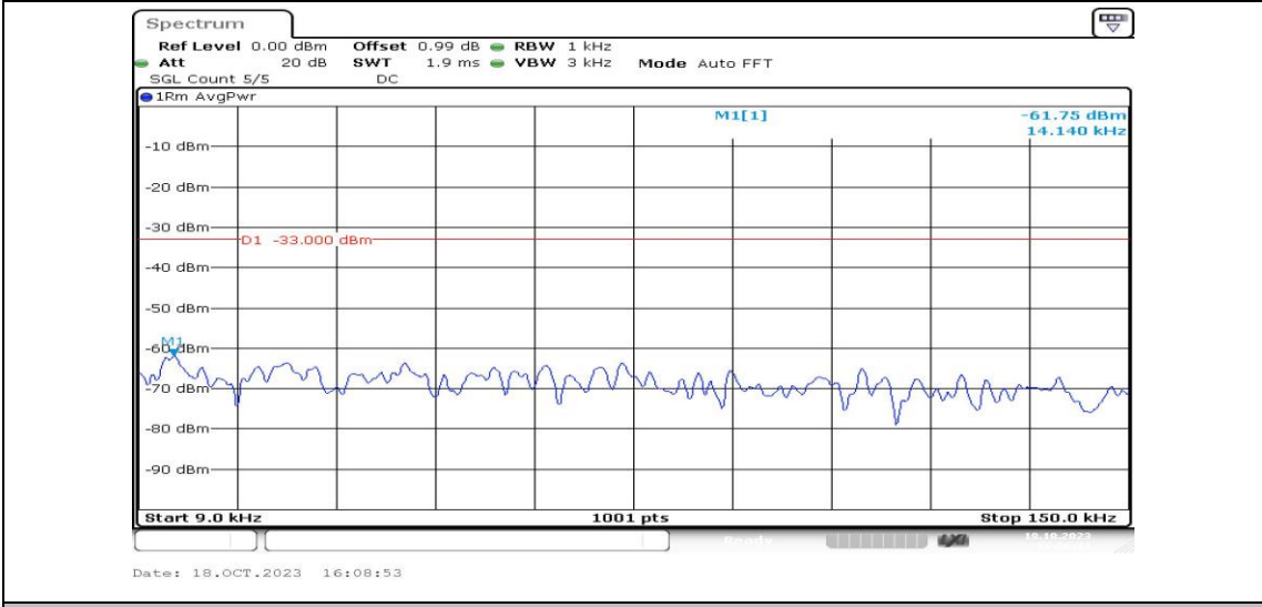
Band25-1.4MHz-QPSK-26683-1RB#0-Range1:0.009~0.15MHz-PASS
