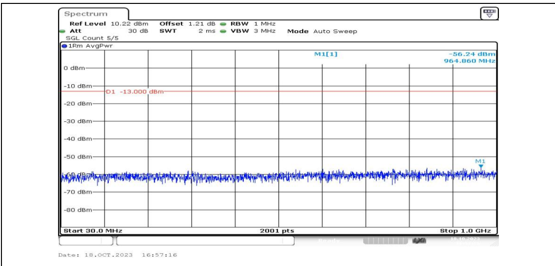
Band25-5MHz-16QAM-26365-1RB#0-Range3:30~1000MHz-PASS
