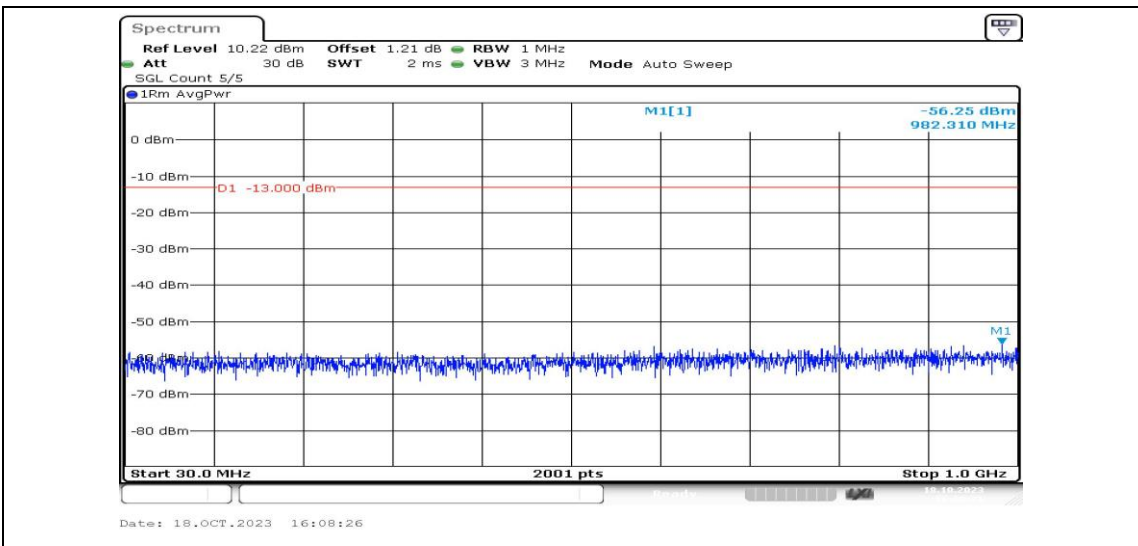
Band25-1.4MHz-16QAM-26365-1RB#0-Range3:30~1000MHz-PASS
