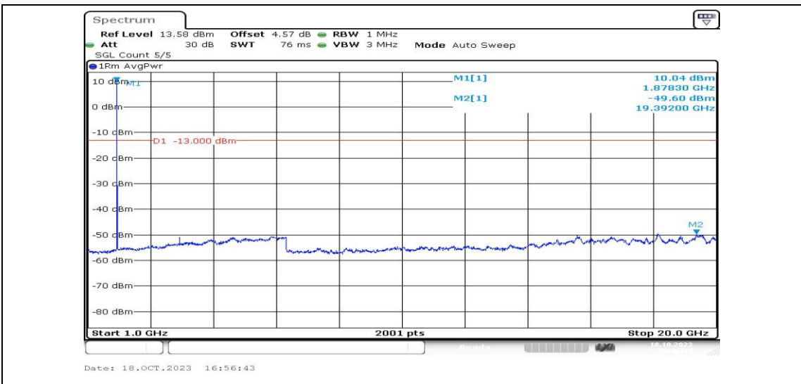
Band25-5MHz-QPSK-26365-1RB#0-Range4:1000~20000MHz-PASS
