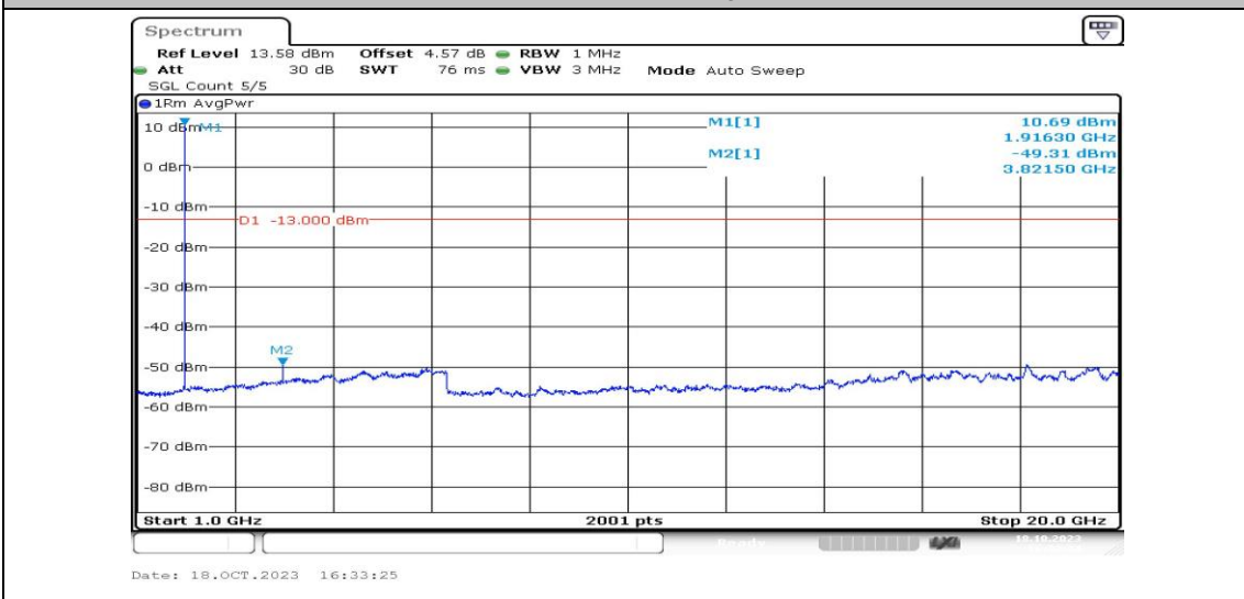
Band25-3MHz-QPSK-26675-1RB#0-Range4:1000~20000MHz-PASS
