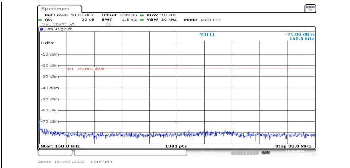
Band25-5MHz-QPSK-26665-1RB#0-Range2:0.15~30MHz-PASS
