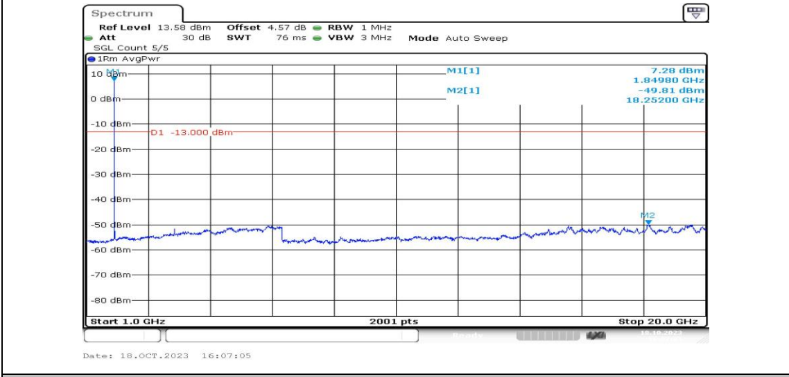
Band25-1.4MHz-16QAM-26047-1RB#0-Range4:1000~20000MHz-PASS
