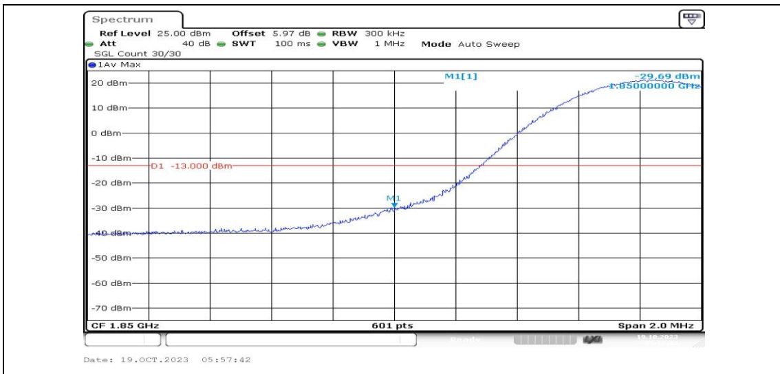
Band25-15MHz-16QAM-26115-1RB#0-PASS
