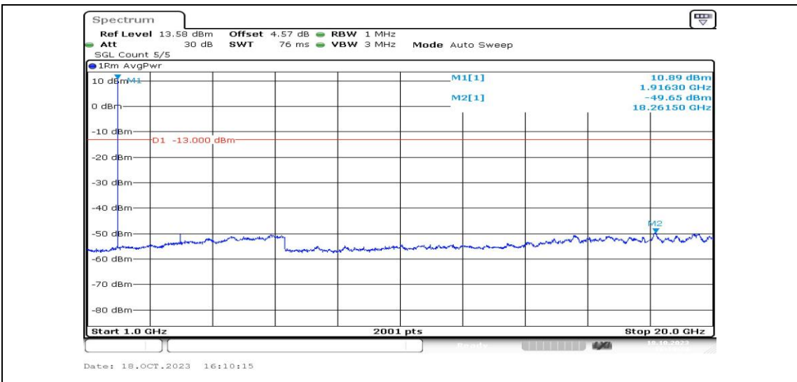
Band25-1.4MHz-16QAM-26683-1RB#0-Range4:1000~20000MHz-PASS
