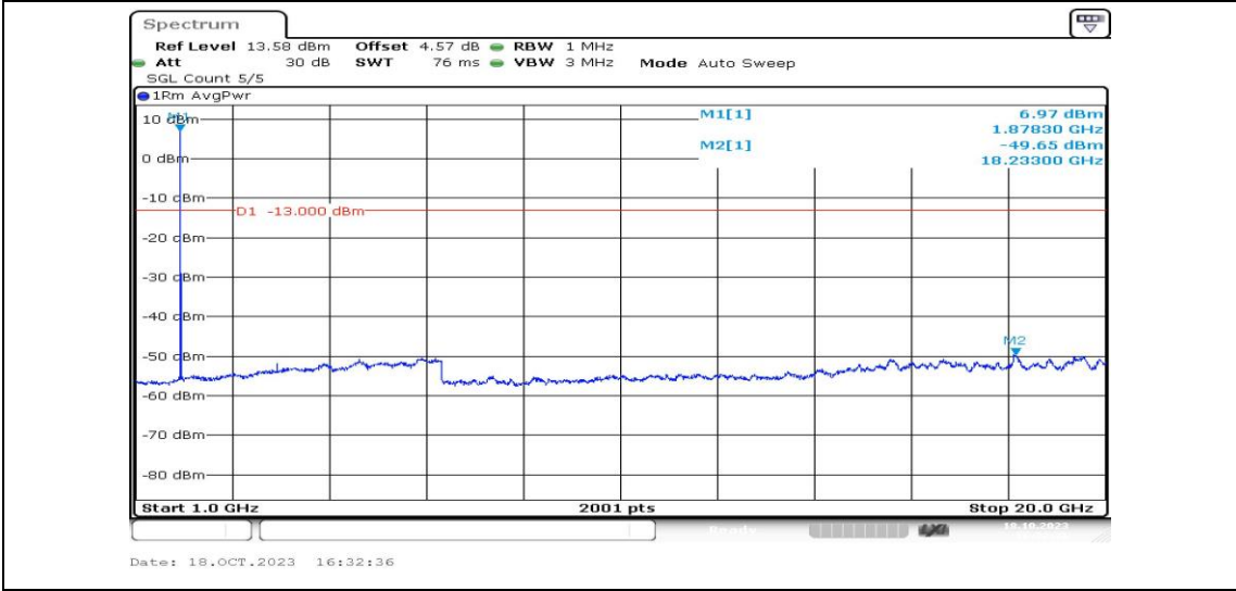
Band25-3MHz-16QAM-26365-1RB#0-Range4:1000~20000MHz-PASS
