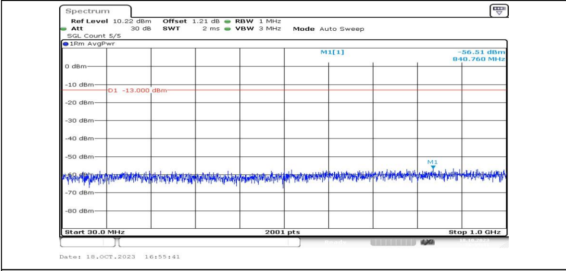
Band25-5MHz-16QAM-26065-1RB#0-Range3:30~1000MHz-PASS
