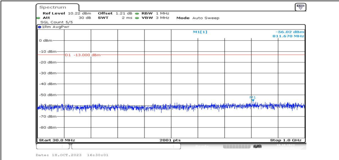
Band25-3MHz-QPSK-26055-1RB#0-Range3:30~1000MHz-PASS
