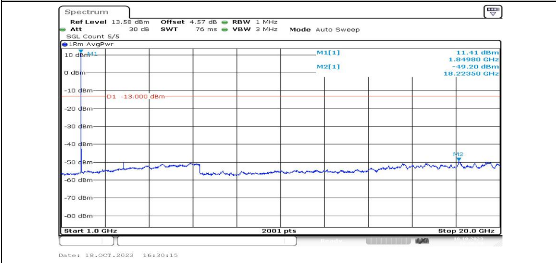
Band25-3MHz-QPSK-26055-1RB#0-Range4:1000~20000MHz-PASS
