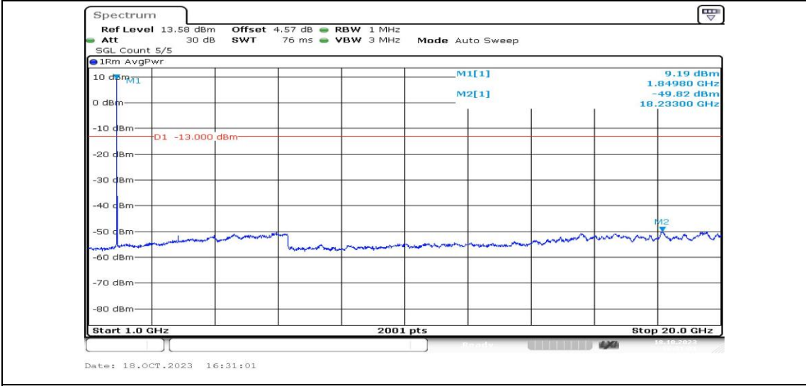
Band25-3MHz-16QAM-26055-1RB#0-Range4:1000~20000MHz-PASS
