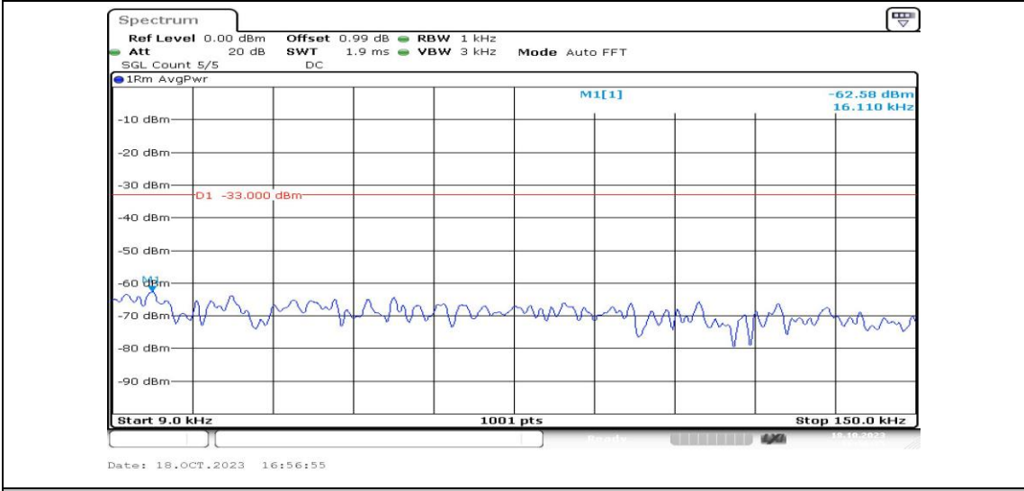
Band25-5MHz-16QAM-26365-1RB#0-Range1:0.009~0.15MHz-PASS
