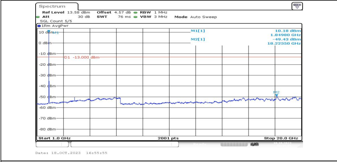
Band25-5MHz-16QAM-26065-1RB#0-Range4:1000~20000MHz-PASS
