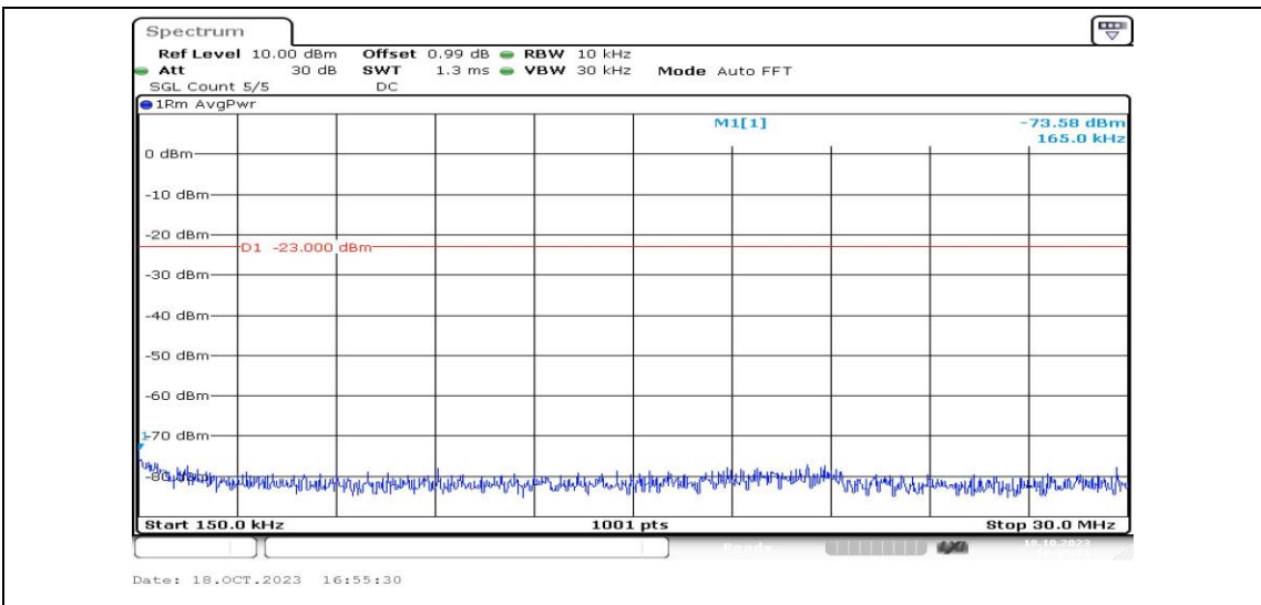
Band25-5MHz-16QAM-26065-1RB#0-Range2:0.15~30MHz-PASS
