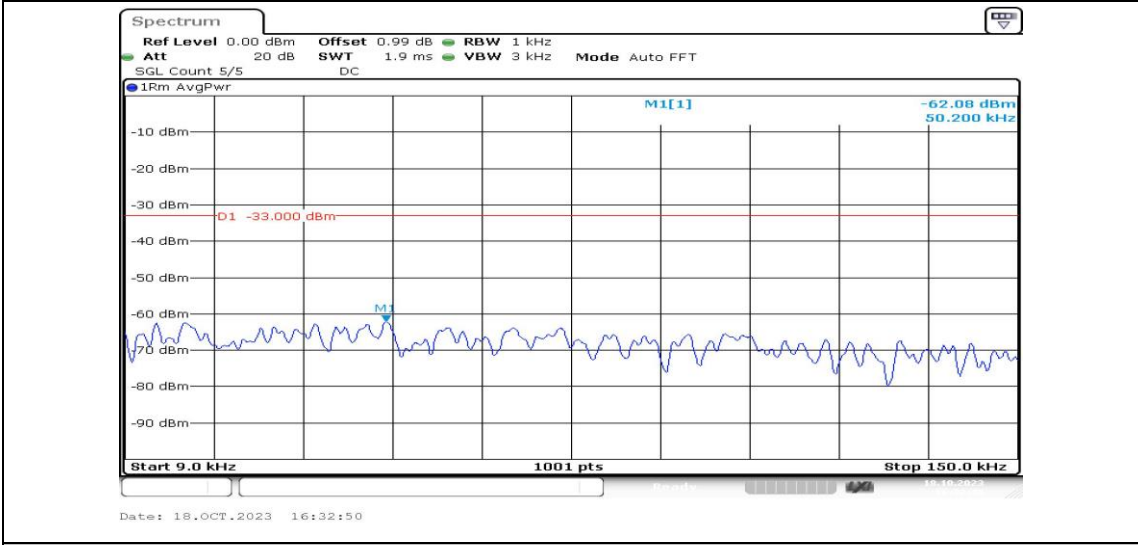
Band25-3MHz-QPSK-26675-1RB#0-Range1:0.009~0.15MHz-PASS
