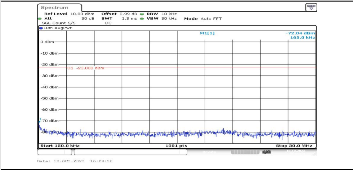
Band25-3MHz-QPSK-26055-1RB#0-Range2:0.15~30MHz-PASS
