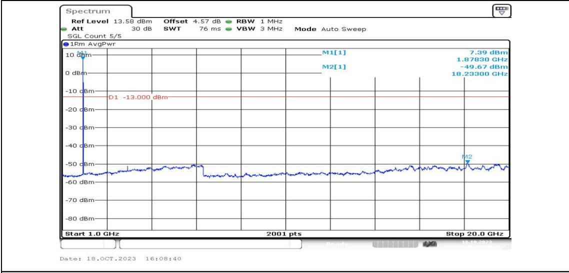
Band25-1.4MHz-16QAM-26365-1RB#0-Range4:1000~20000MHz-PASS
