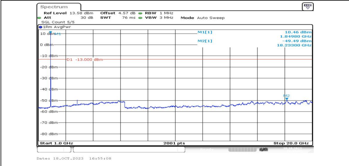
Band25-5MHz-QPSK-26065-1RB#0-Range4:1000~20000MHz-PASS
