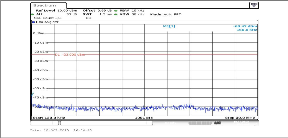
Band25-5MHz-QPSK-26065-1RB#0-Range2:0.15~30MHz-PASS
