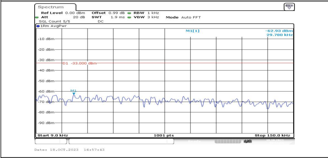
Band25-5MHz-QPSK-26665-1RB#0-Range1:0.009~0.15MHz-PASS
