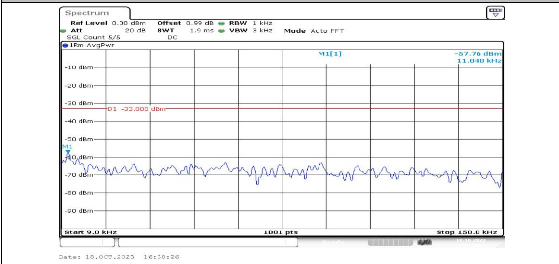
Band25-3MHz-16QAM-26055-1RB#0-Range1:0.009~0.15MHz-PASS
